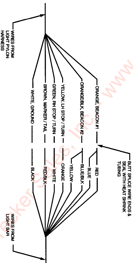
DETAIL B
