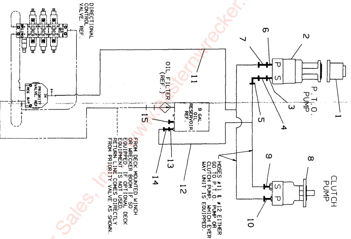
CIRCUIT FOR P. T. O. PUMP OR CLUTCH PUMP
