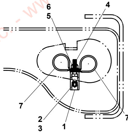
TYPICAL HOSE ROUTING / MOUNTING
