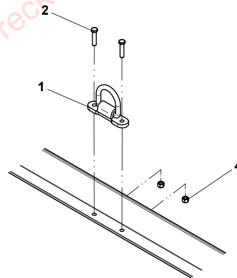
STEEL DECK
