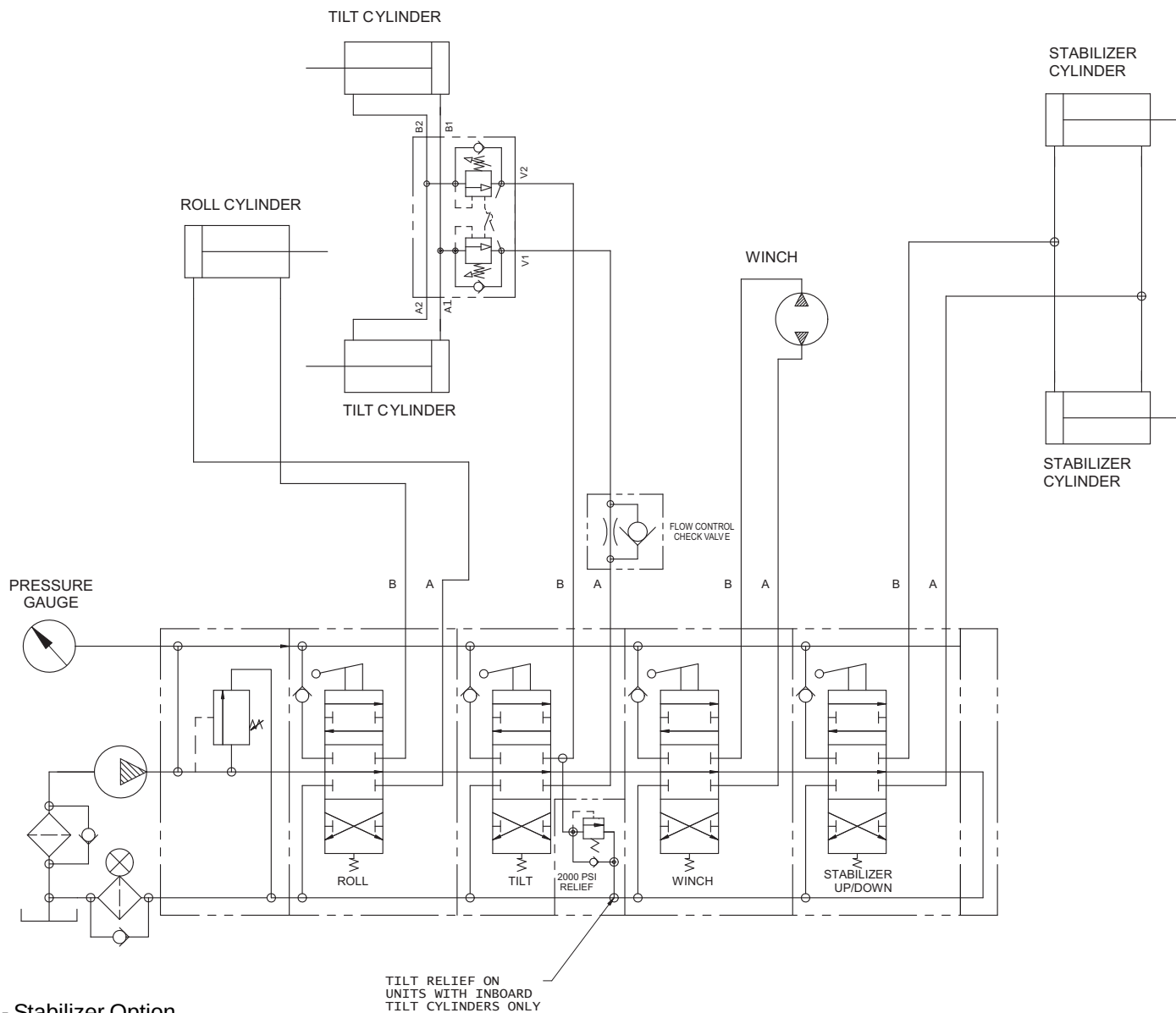
4 Bank Control Valve - Stabilizer Option
