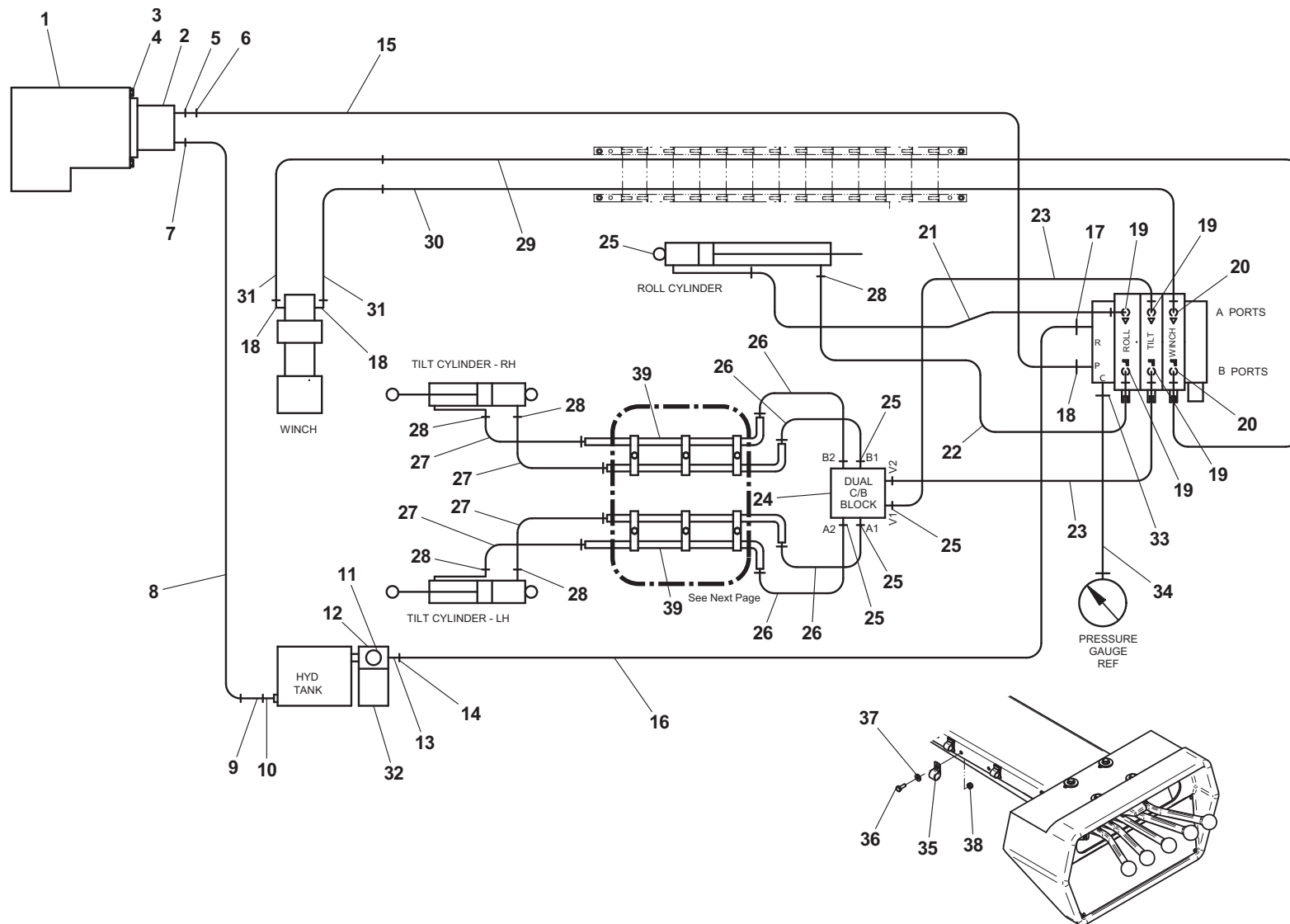
CLAMP FOR PRESSURE GAUGE HOSE, ITEM #34
