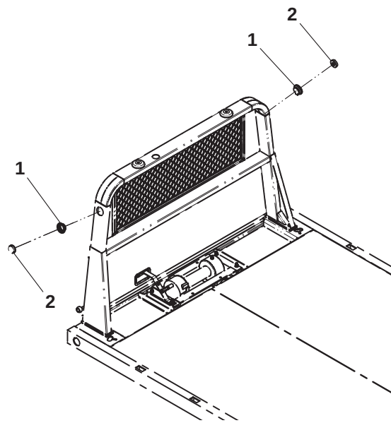
FOR 36" & 40" HEADBOARD
