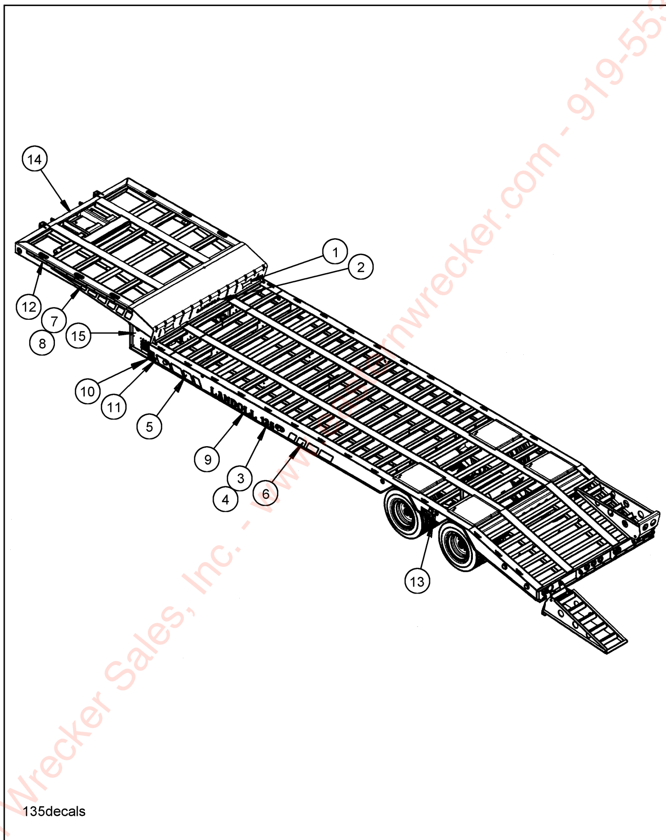
Figure 1-20 Decal Placement
