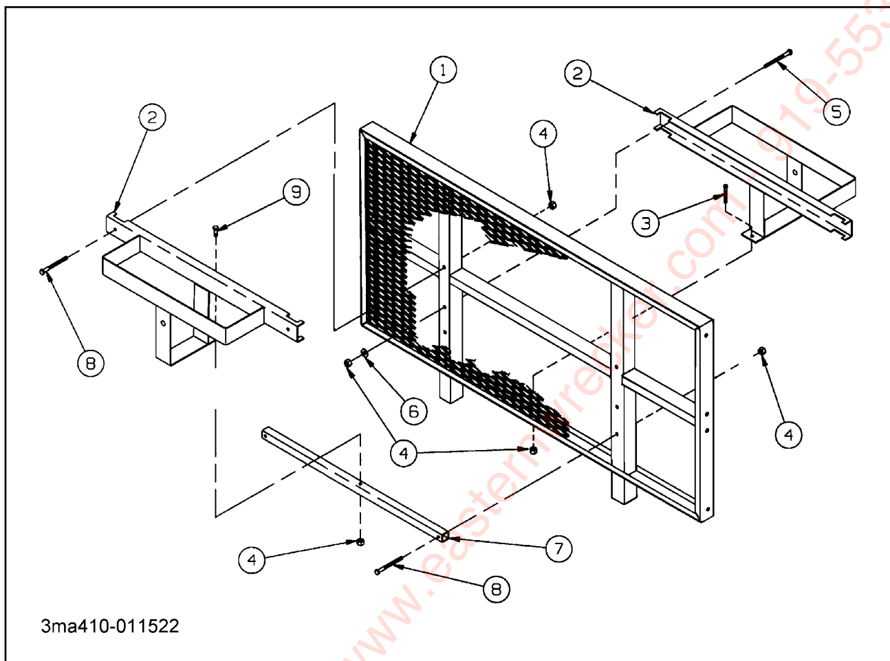
Figure 1-33 Spare Tire Carrier (Option)
