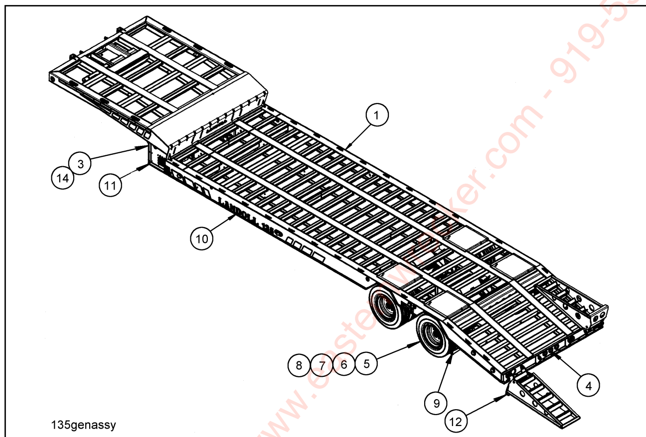
Figure 1-1 General Assembly
