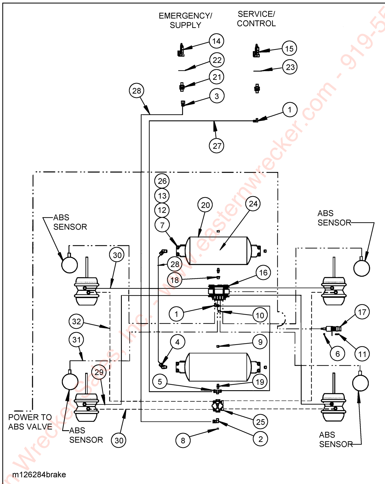
Figure 1-15 Spring Air Brake System w/ ABS, Tandem Axle (Spring Ride)
