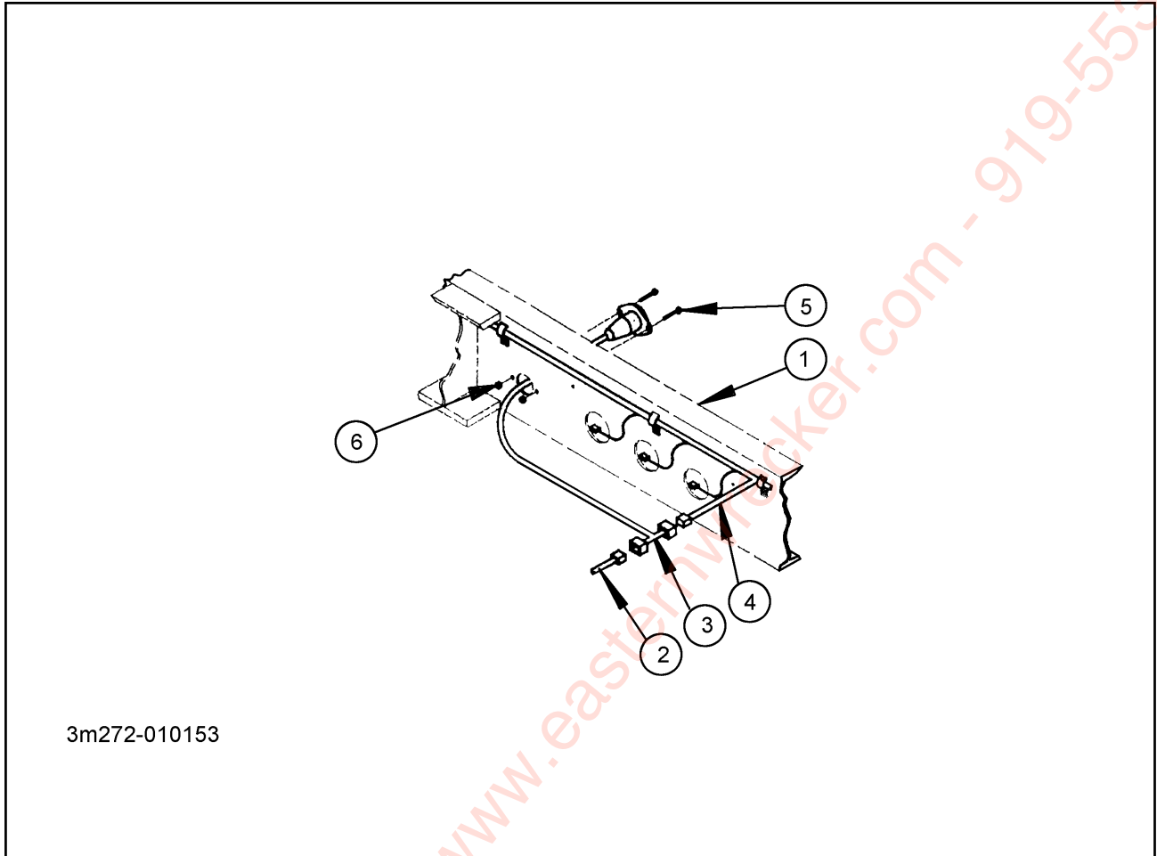
Figure 1-39 7 Way Recp. Bumper Electrical Installation (Option)
