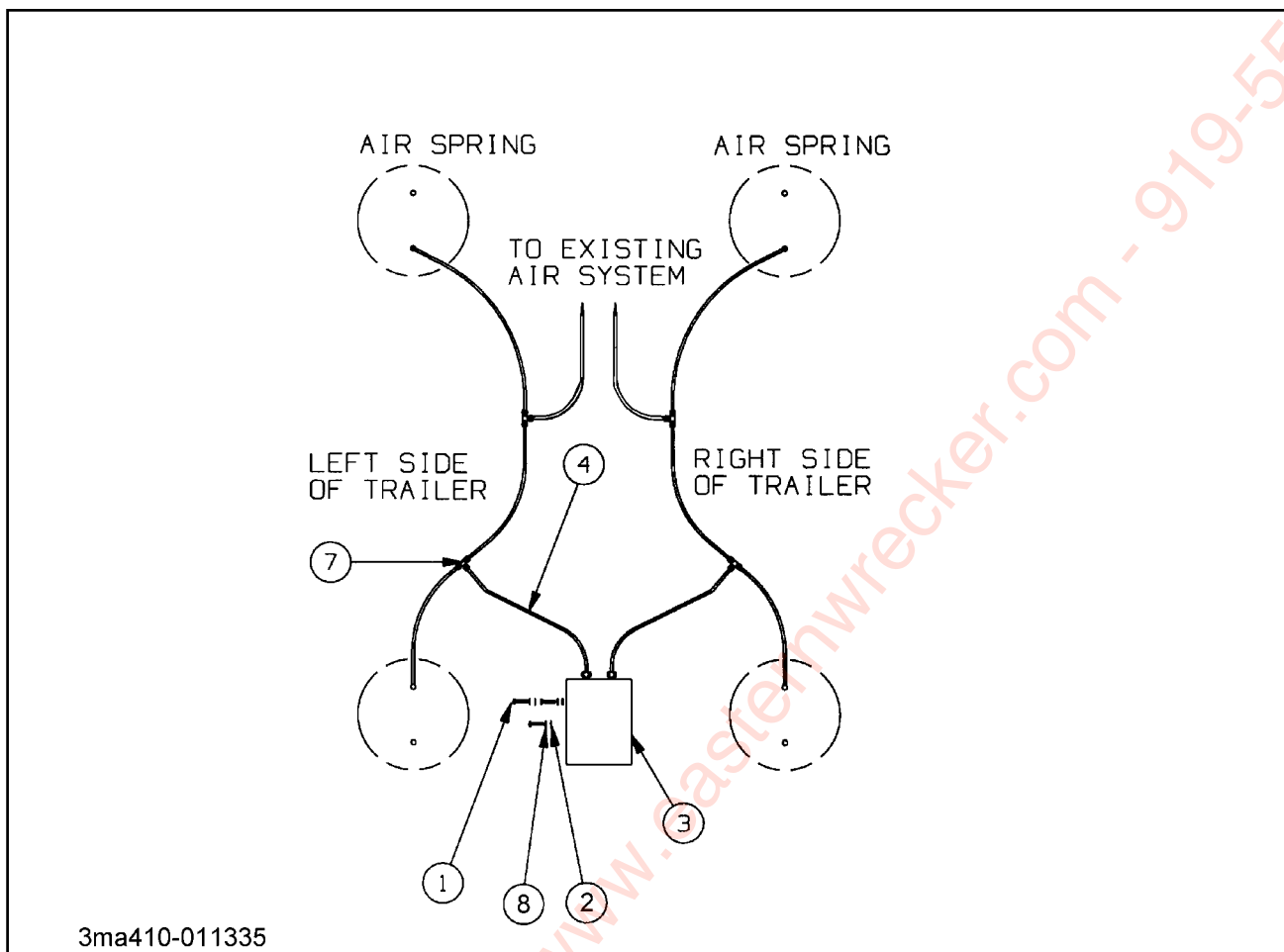
Figure 1-34 Scale-o-matic Installation (Option)
