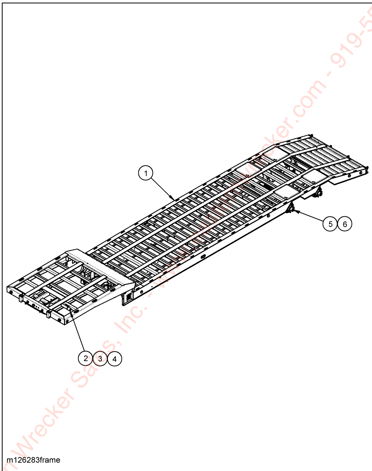
Figure 1-2 Frame Assembly
