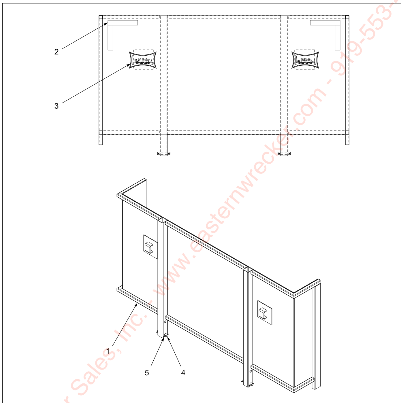
Figure 1-15: Bulkhead Assembly w/ Pocket - 48 x 102
