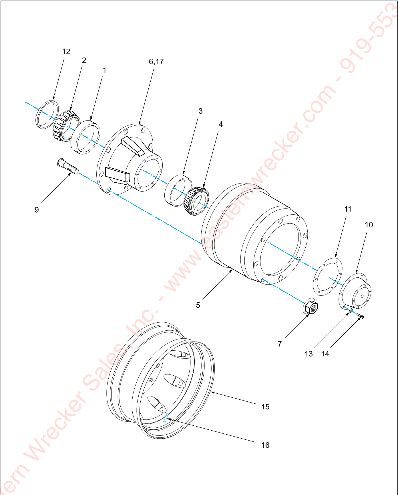
Figure 1-12: Outboard Pilot Mount Hub and Drum
