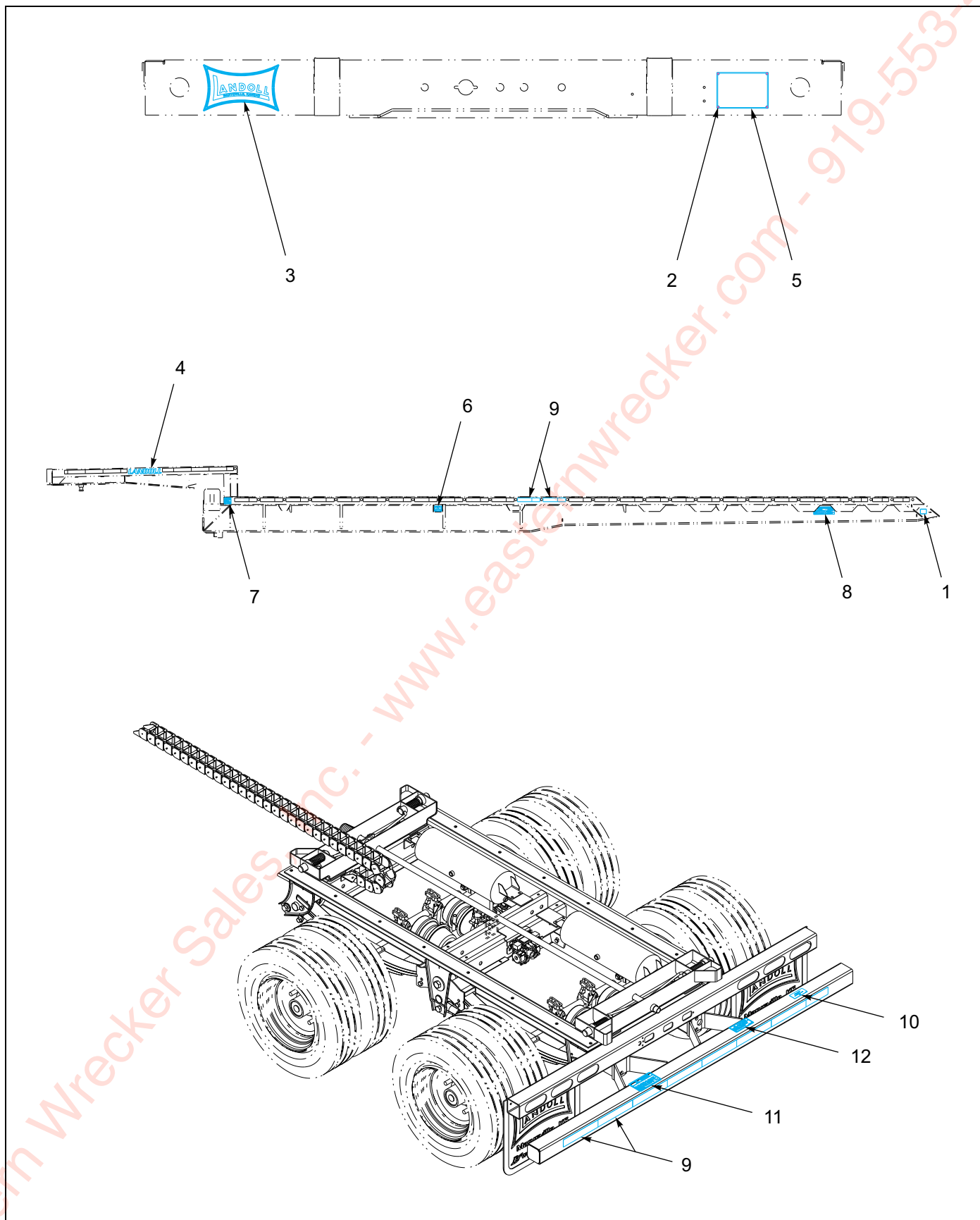
Figure 1-21: Decal Locations
