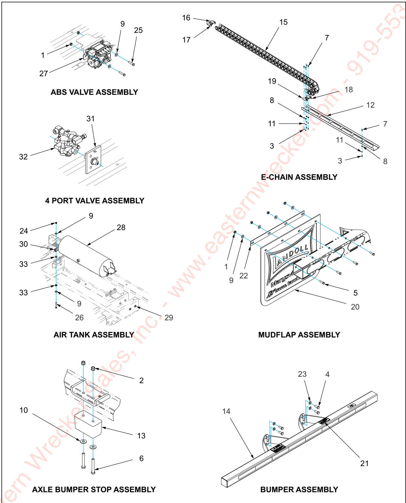
Figure 1-9: Undercarriage Assembly - Spring Ride (2 of 2)
