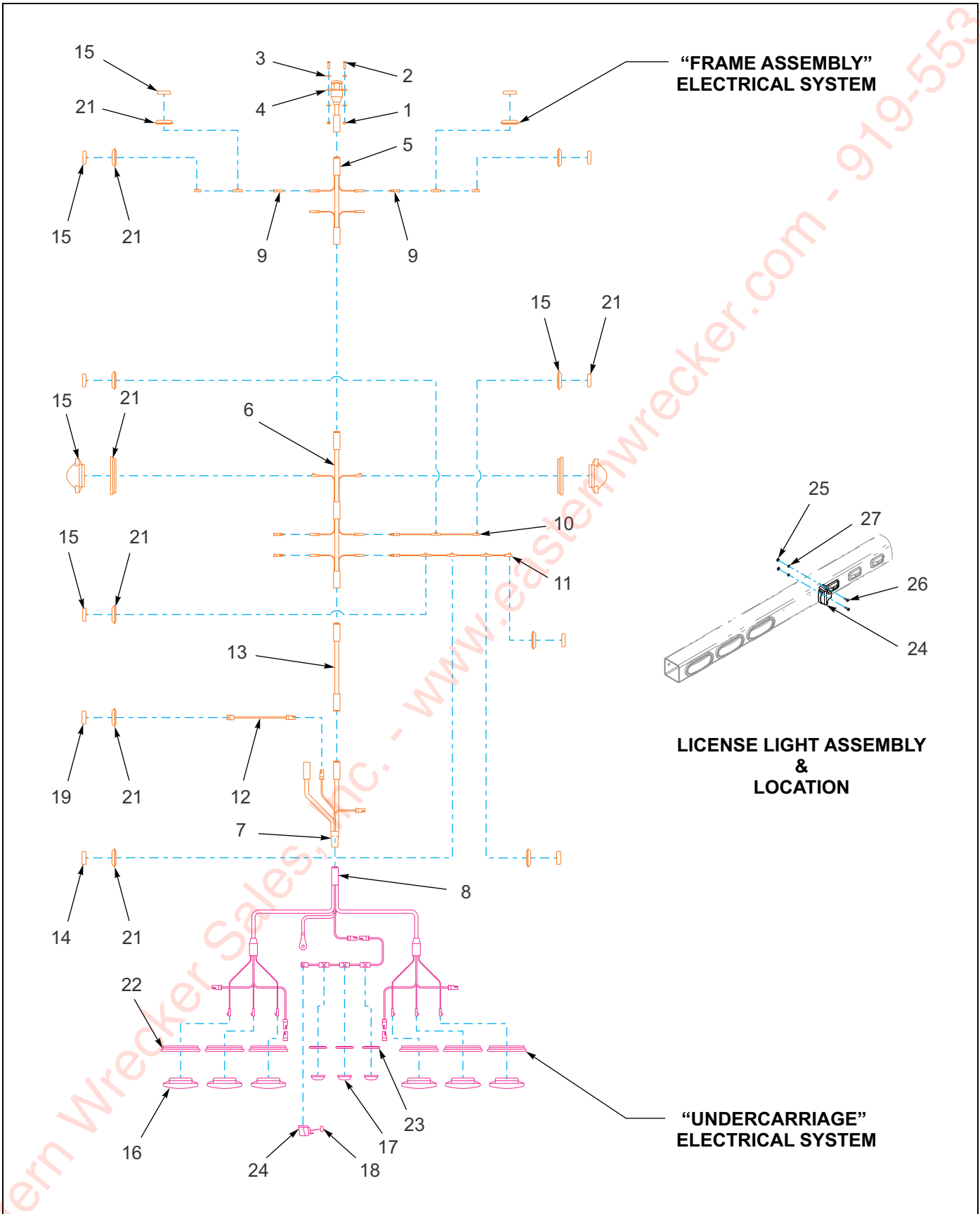
Figure 1-5: Electrical System
