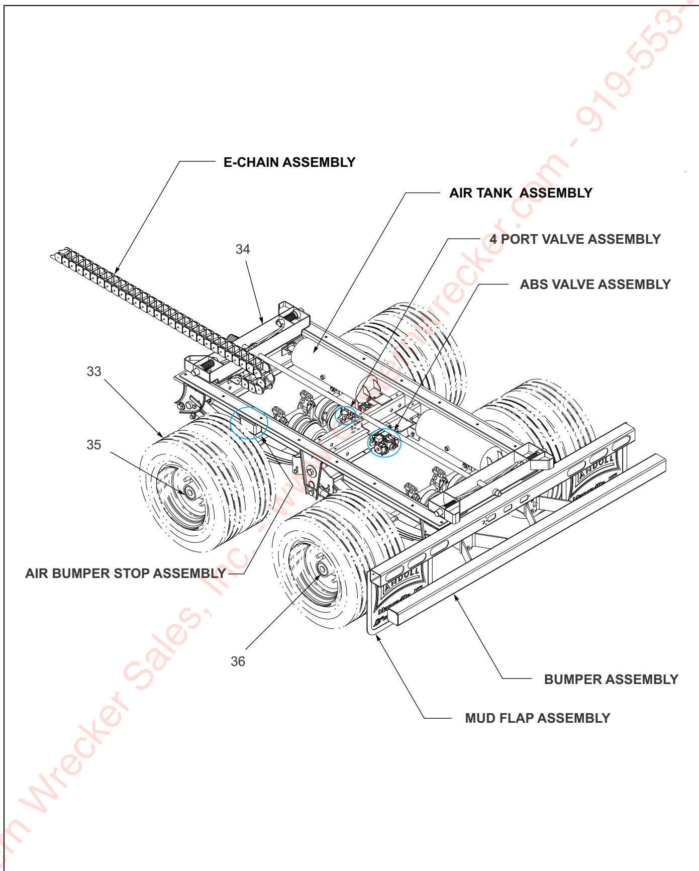
Figure 1-8: Undercarriage Assembly - Spring Ride (1 of 2)
