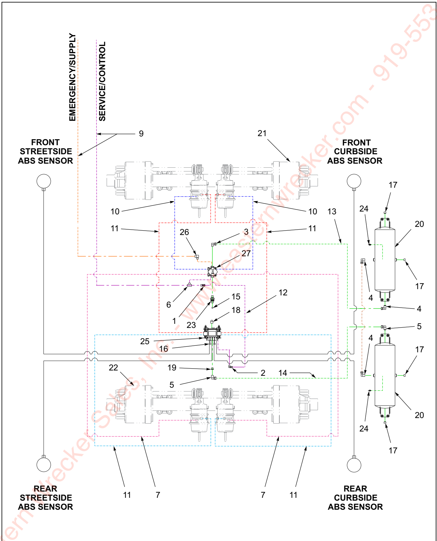
Figure 1-13: Air Brake System
