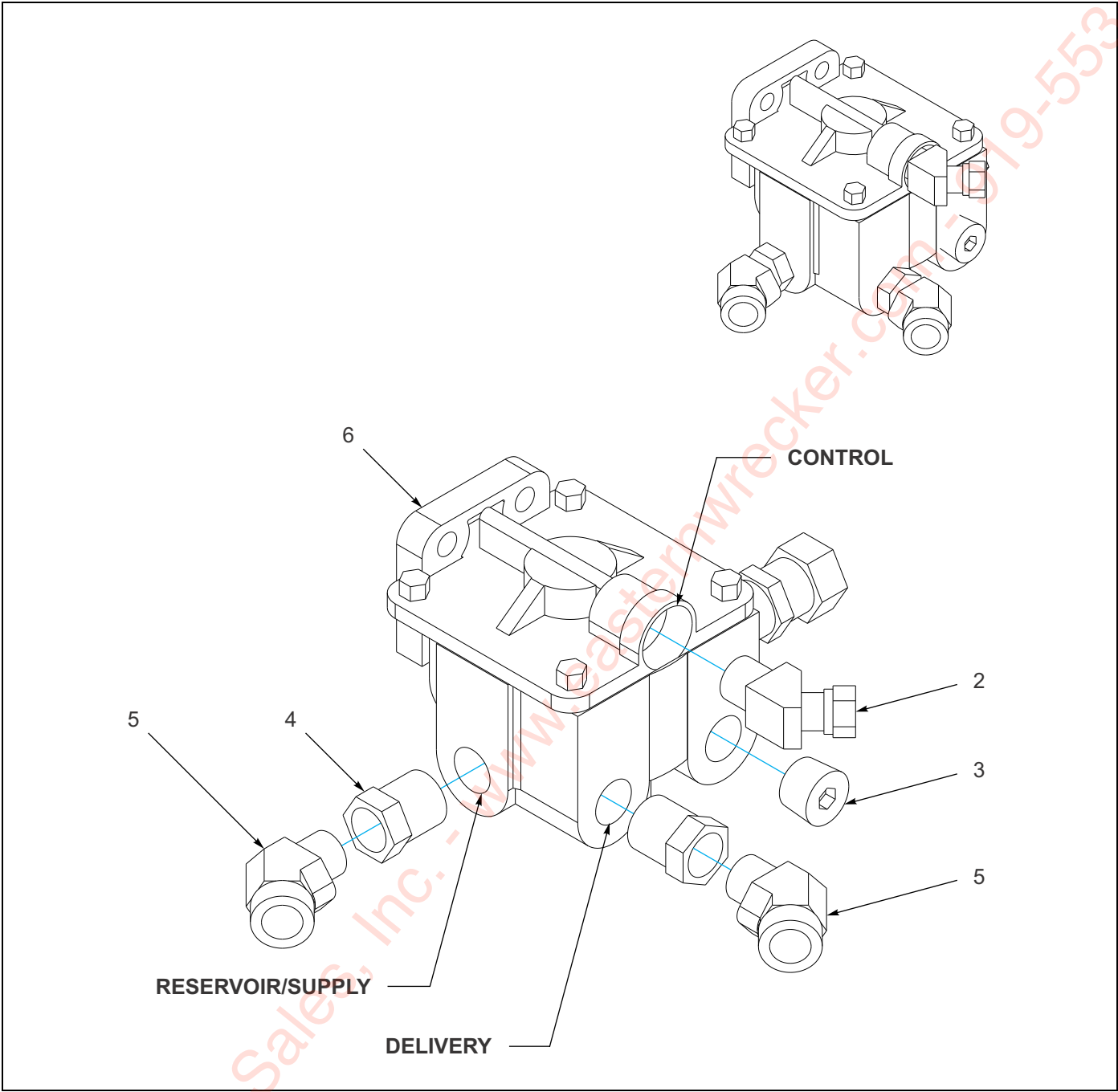
Figure 1-7: Valve Assembly - Air Booster
