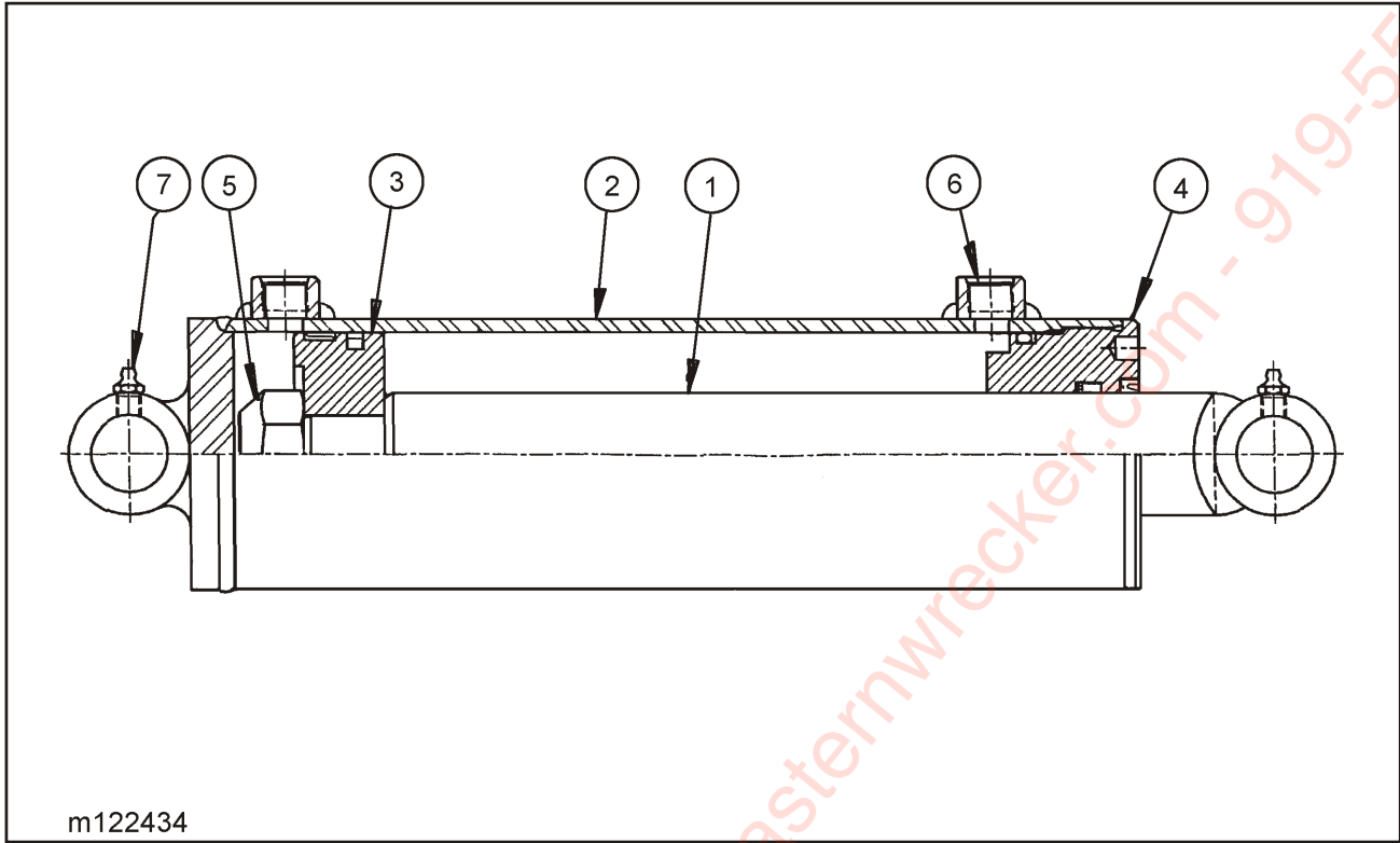
Figure 1-17 4 x 10 Hydraulic Cylinder Assembly
