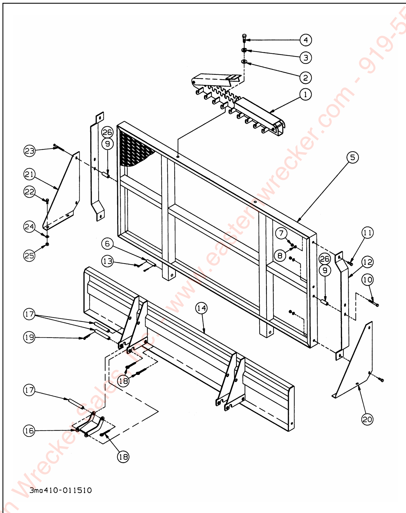
Figure 1-70 Front Extension and Bulkhead (Optional)
