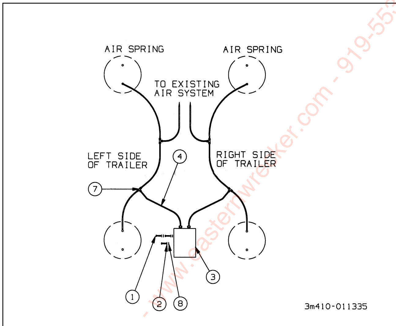
Figure 1-85 Scale-o-matic (Optional)
