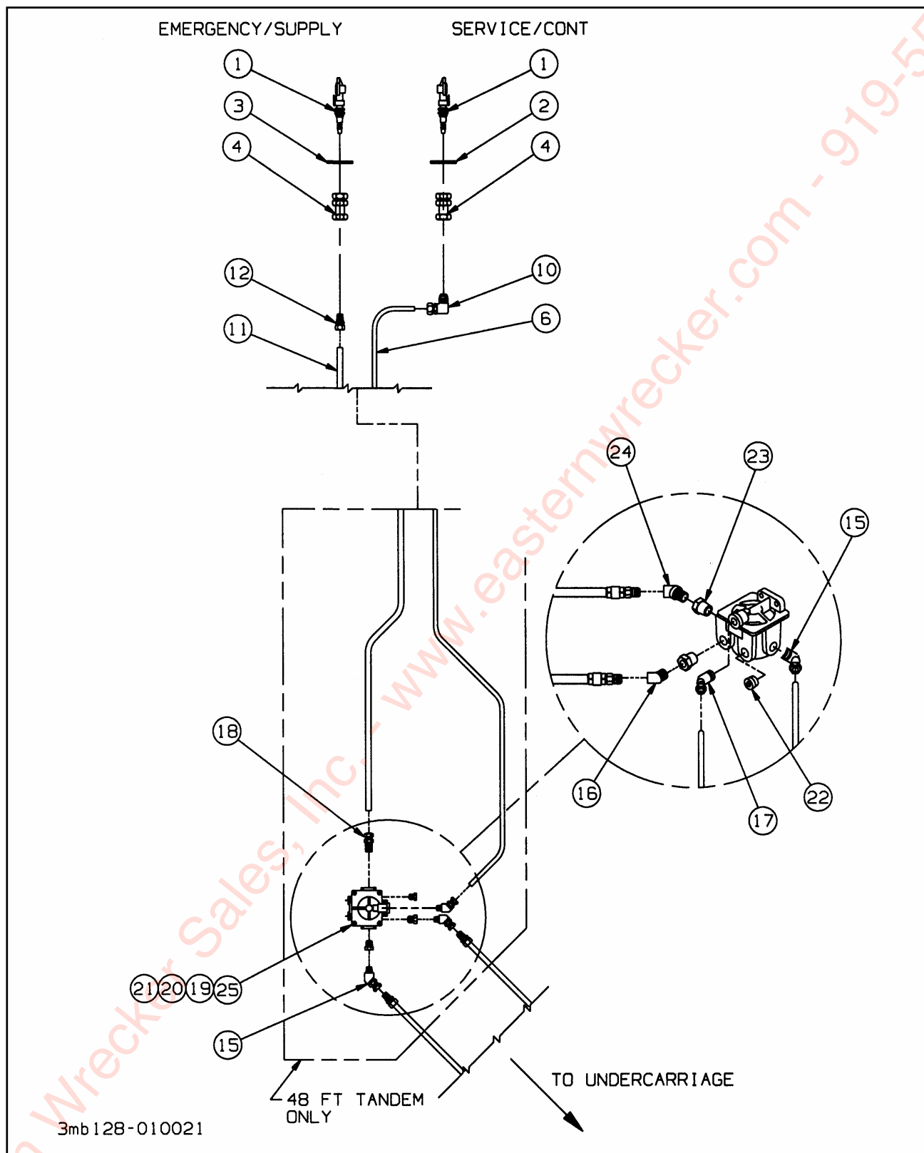
Figure 1-39 Air System, Main
