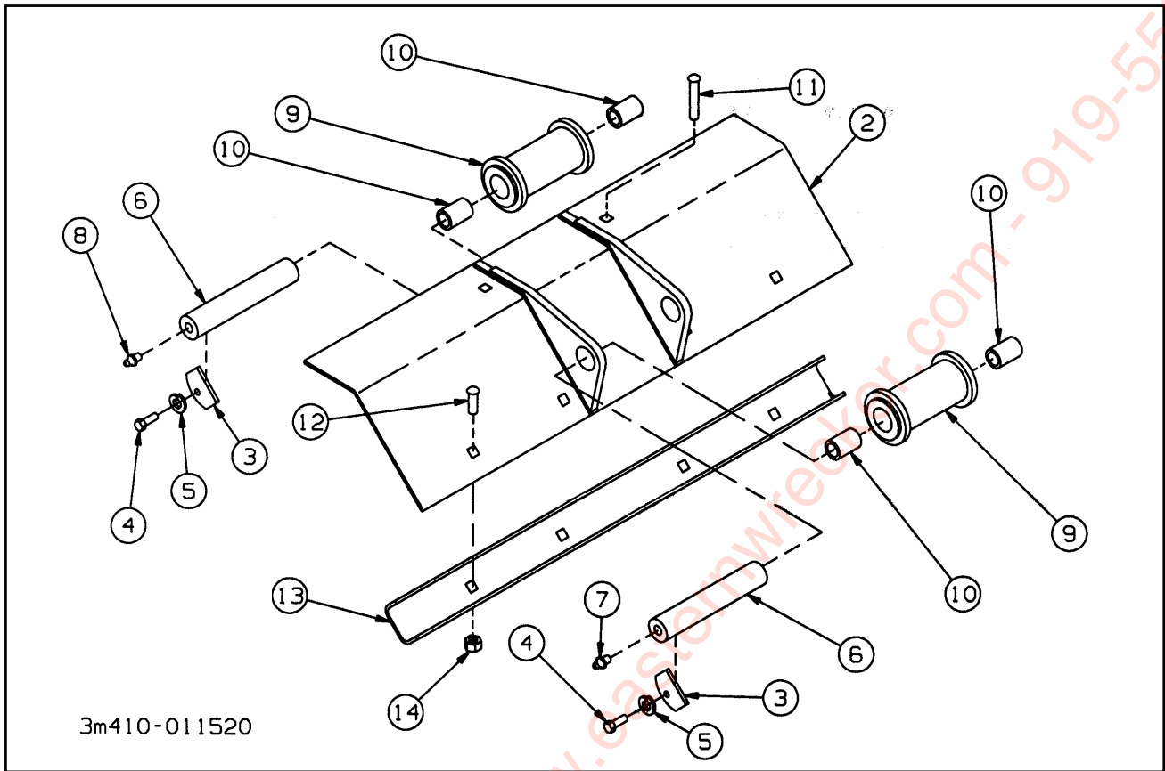
Figure 1-74 Slope Roller Guide 45 (Optional)
