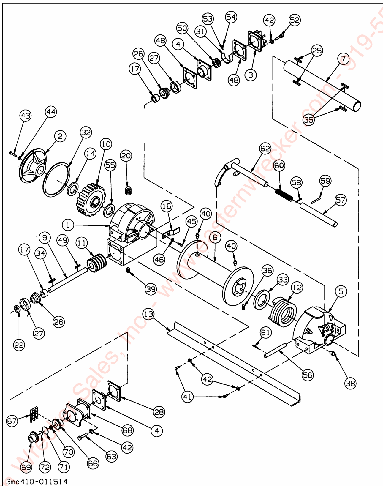
Figure 1-45 12,000# Winch Items
