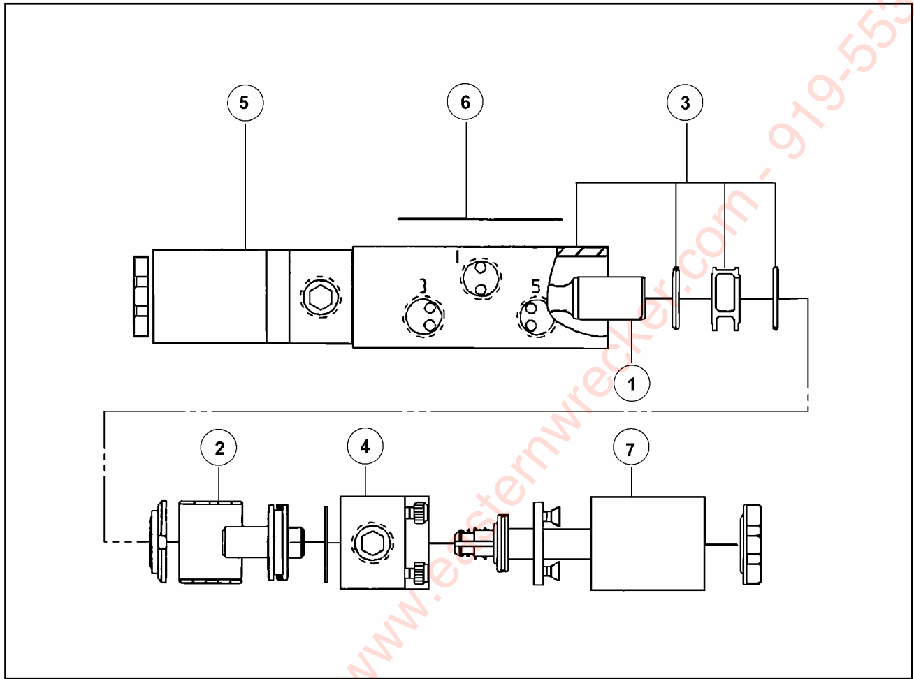
Figure 1-11 Pneumatic Valve
