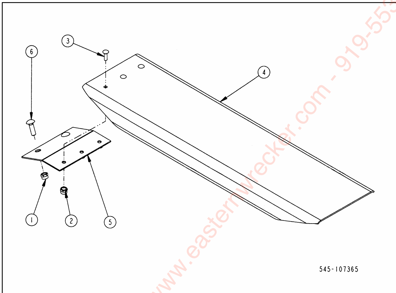
Figure 1-80 Ramps (Optional)
