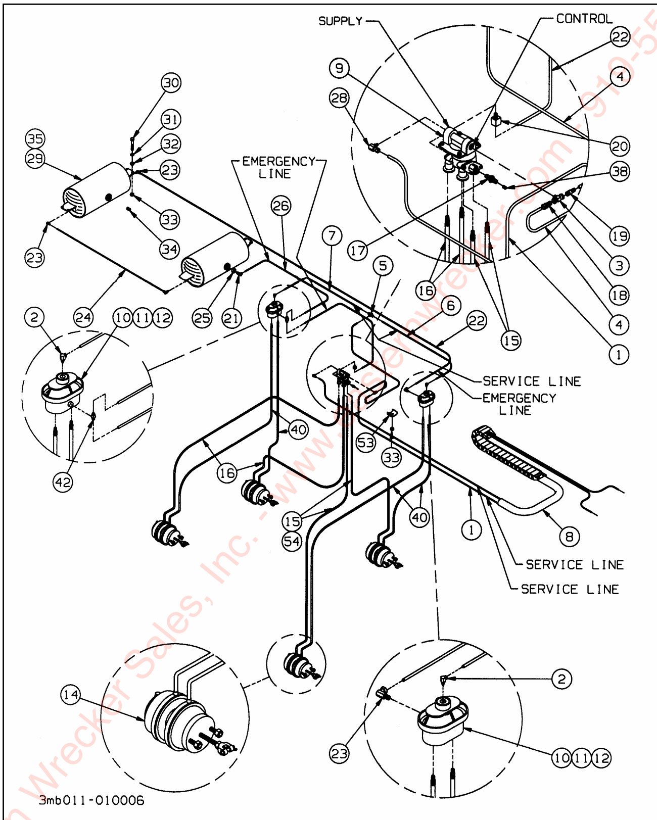
Figure 1-32 Air Brake System w/o ABS (Tandem Axle)
