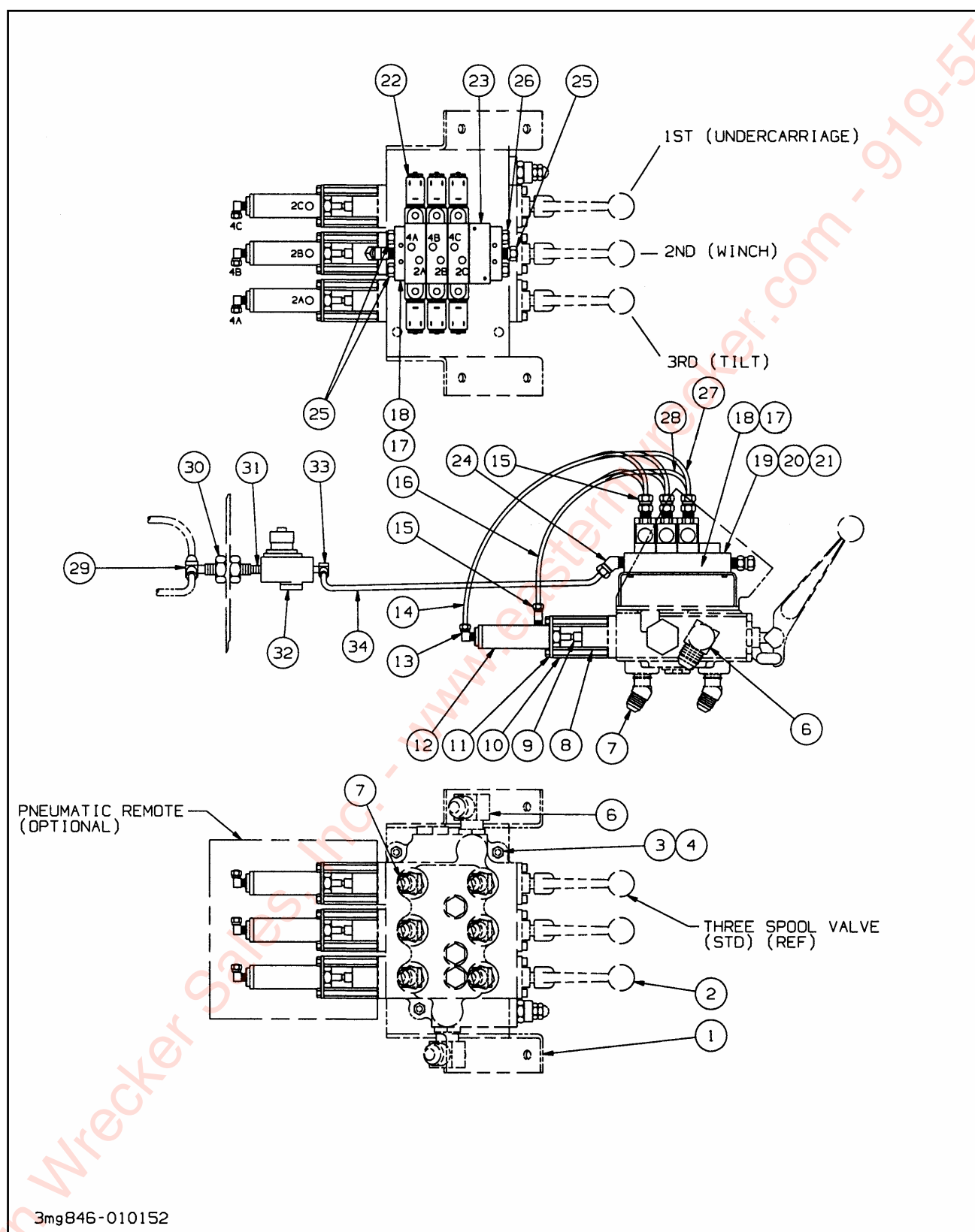
Figure 1-10 Valve Assembly, Three Spool
