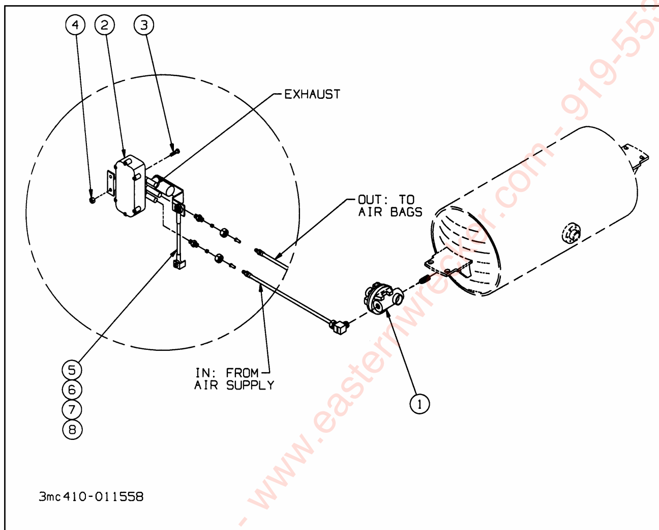
Figure 1-26 Air Control Kit, AR-45
