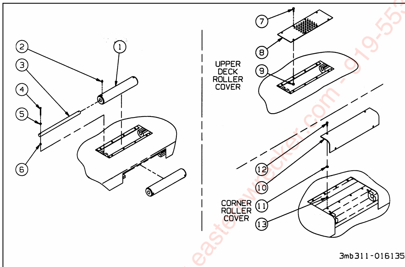
Figure 1-75 Slope Roller Guide 90 (Optional)
