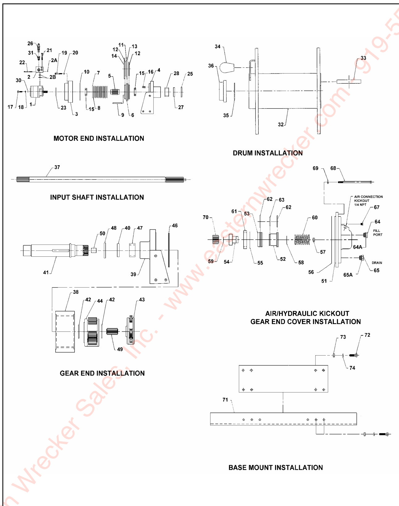
Figure 1-47 30,000# Winch Items
