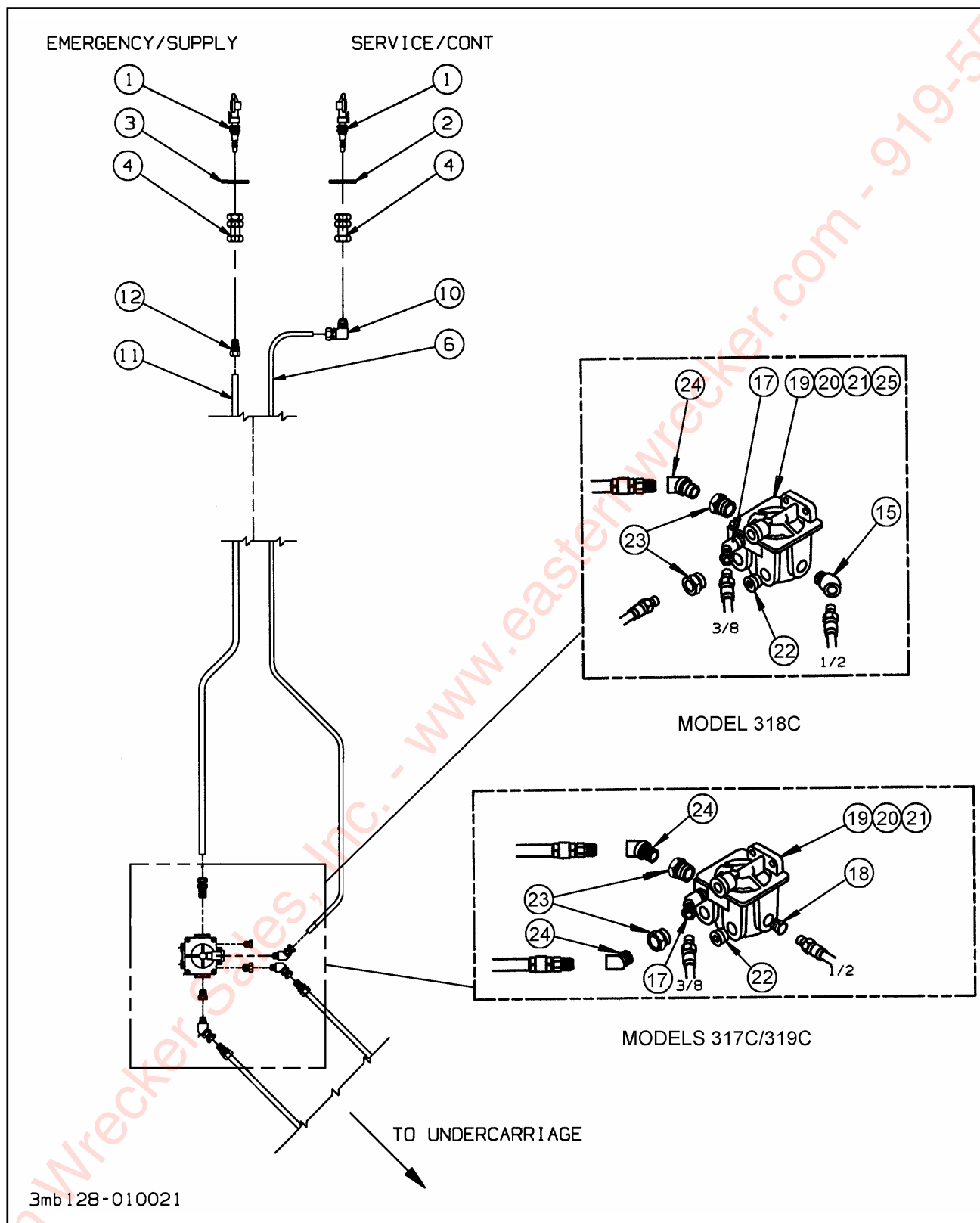
Figure 1-34 Air System, Main
