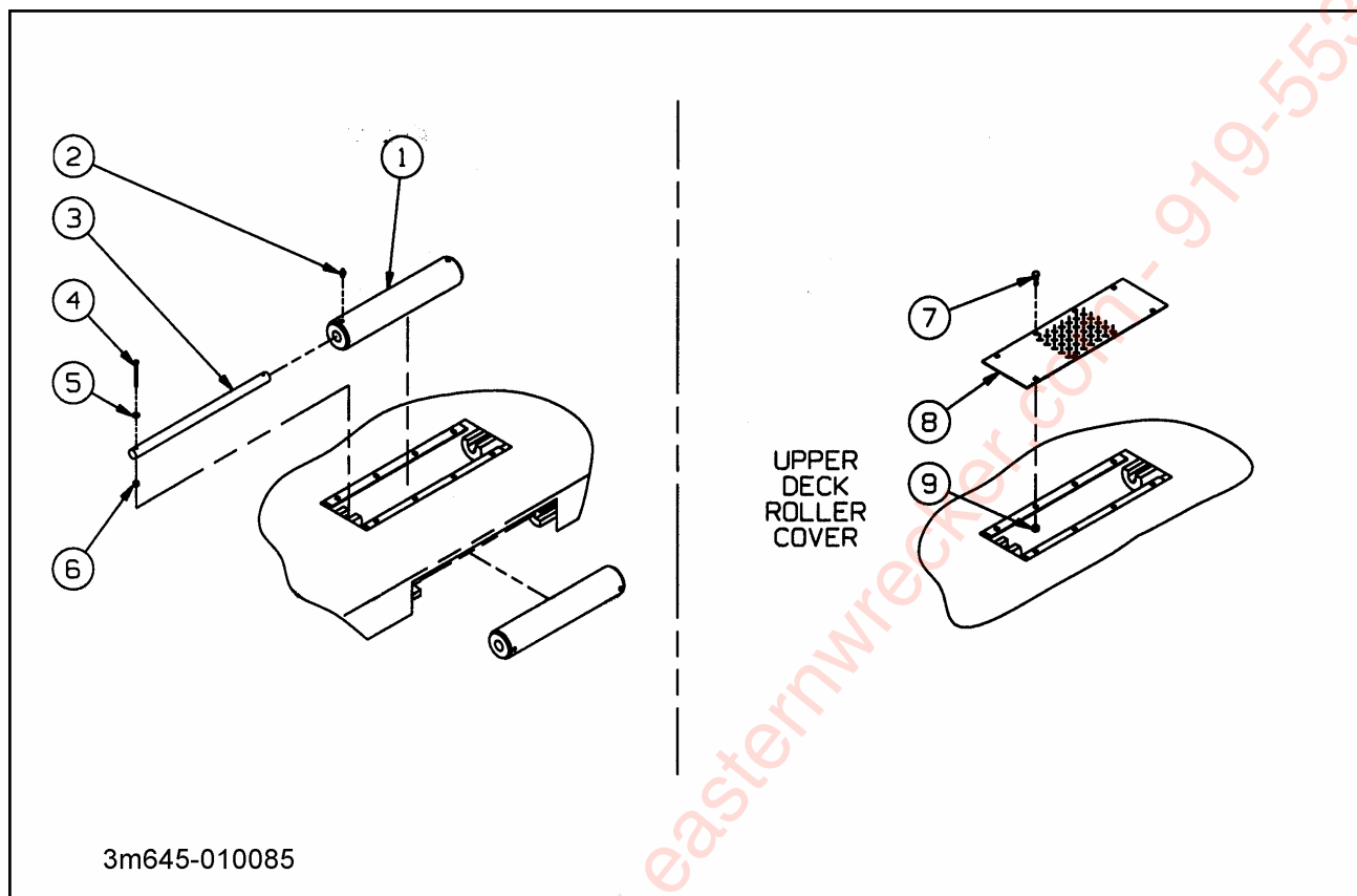
Figure 1-64 Slope Roller Guide 90 (Option)
