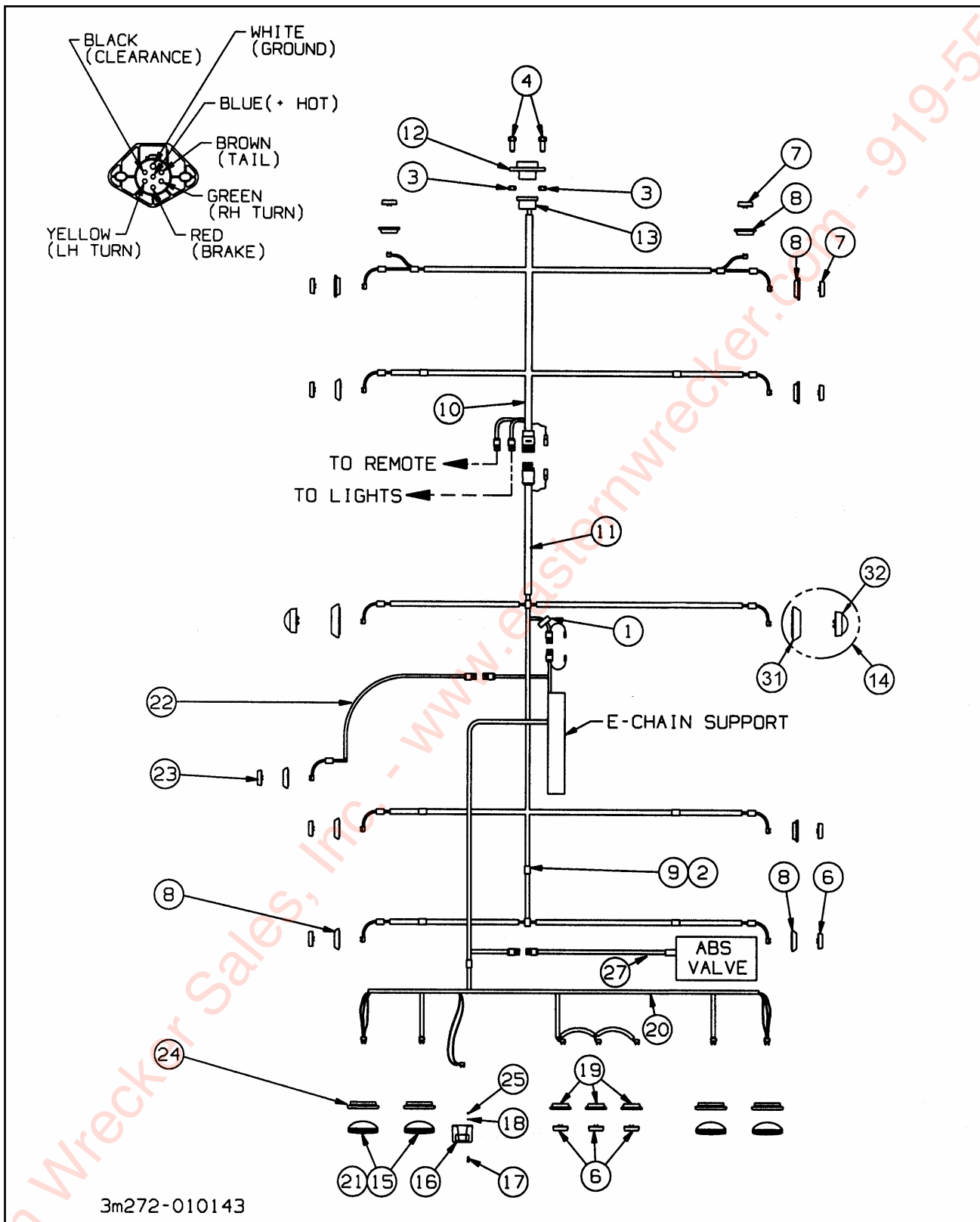
Figure 1-13 Electrical System Schematic (Prior 12/05/01)
