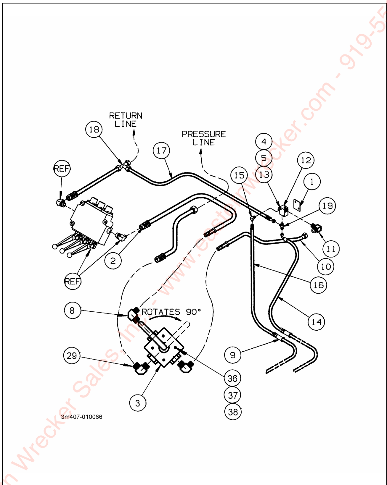
Figure 1-49 Dock Leveler, Hydraulic (Option)
