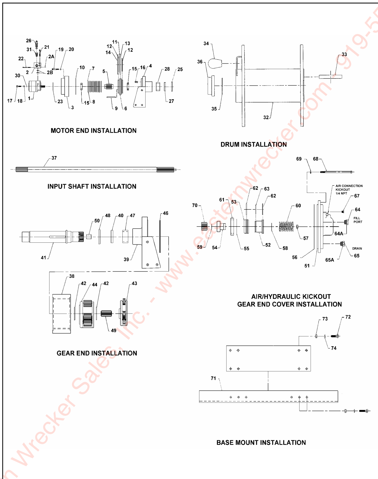
Figure 1-43 30,000# Winch Items
