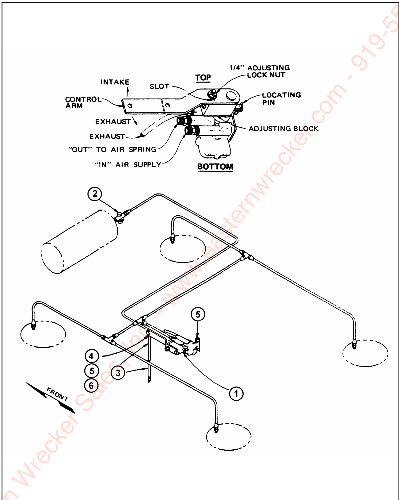
Figure 1-25 Air Control Kit, RLU-228
