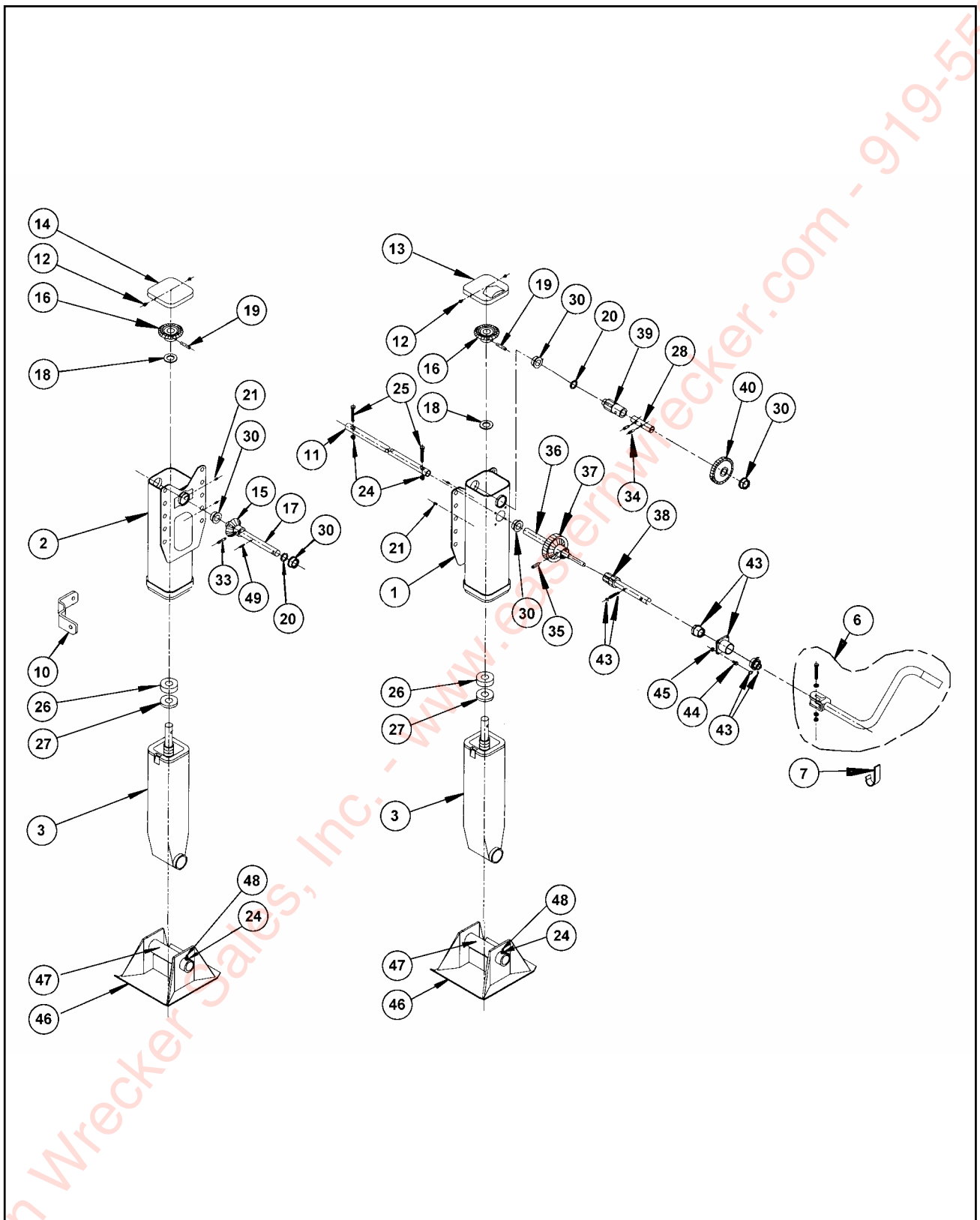
Figure 1-72 Landing Gear w/ Crank
