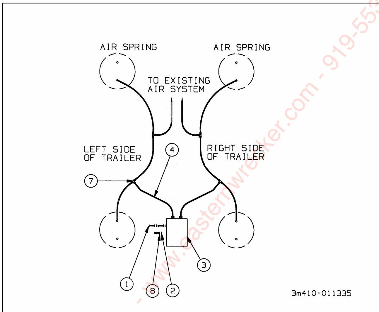
Figure 1-74 Scale-o-matic (Option)
