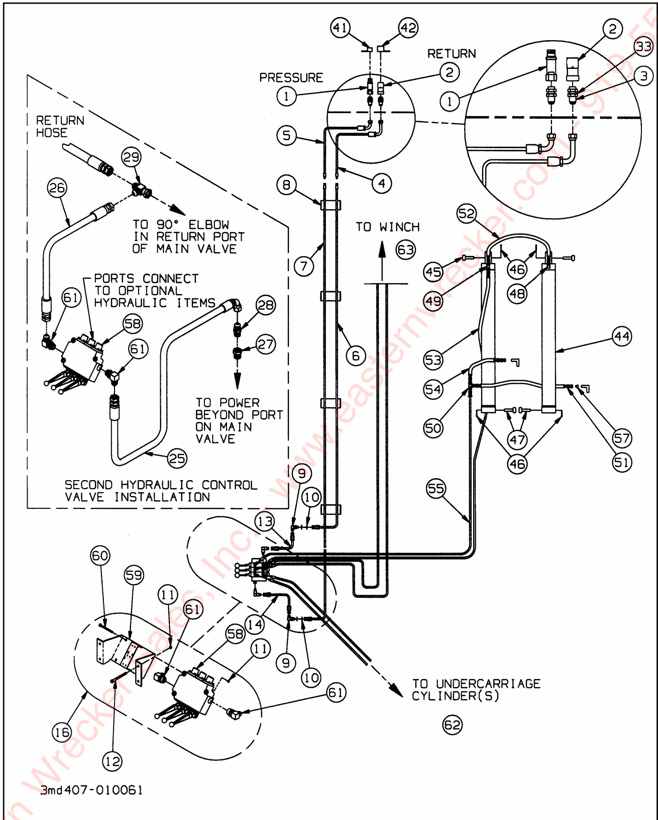
Figure 1-3 Hydraulic System (317C)
