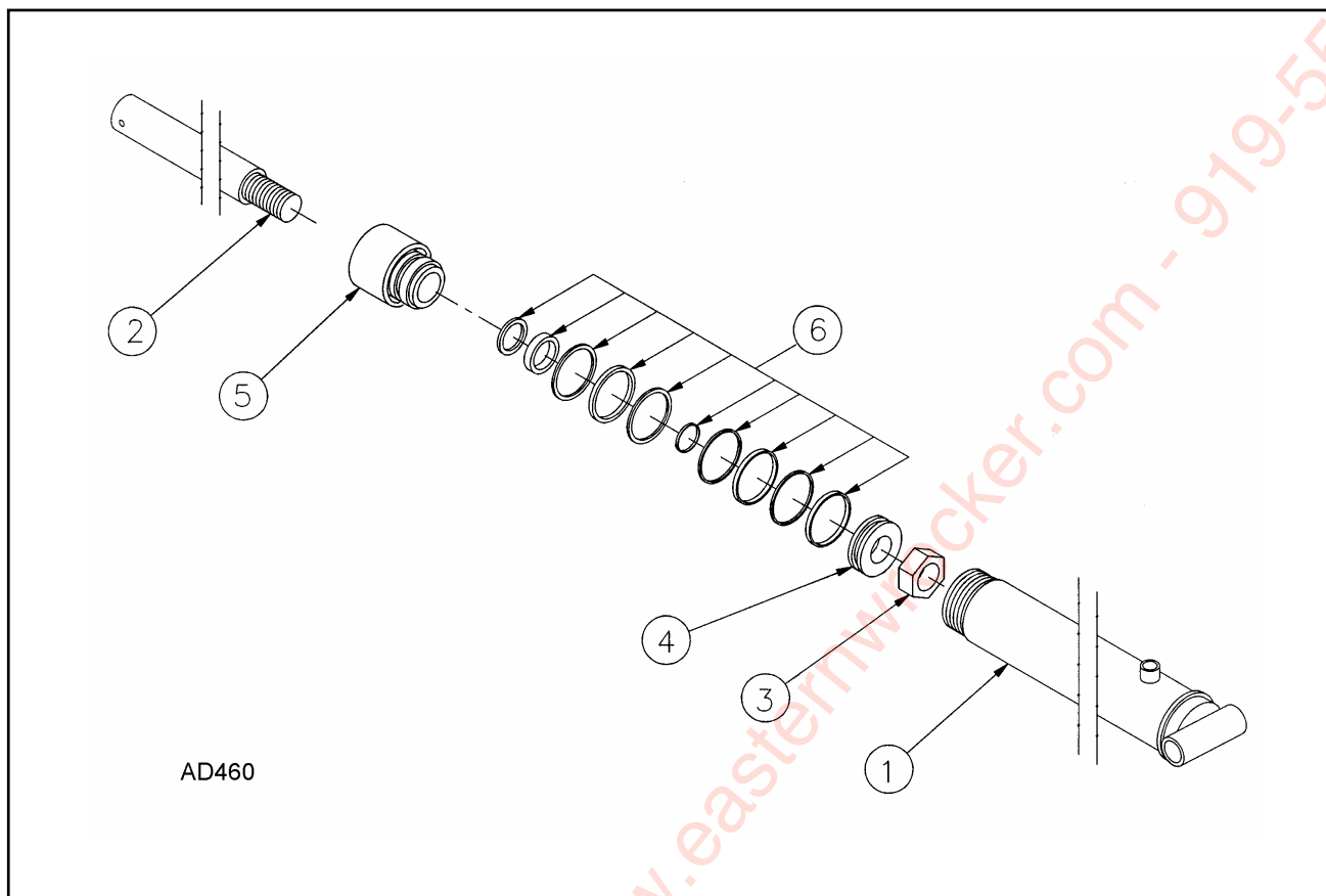
Figure 1-7 Cylinder 4" X 42"
