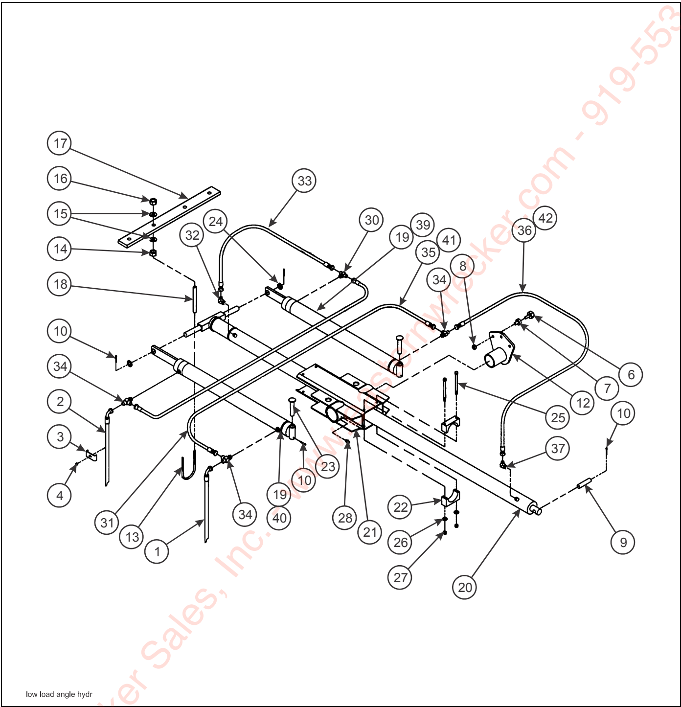
Figure 2-9: Hydraulic System - Low Load Angle
