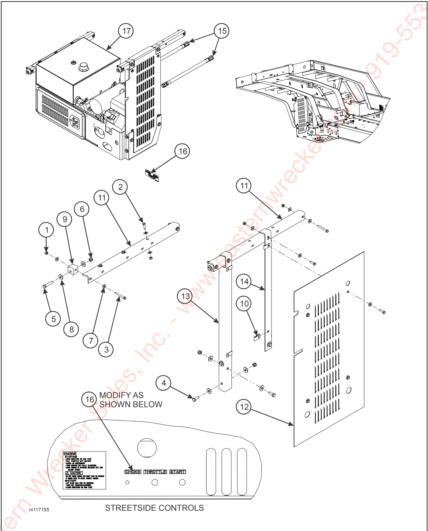
Figure 2-82: Engine Package Bracket Kit (Option)
