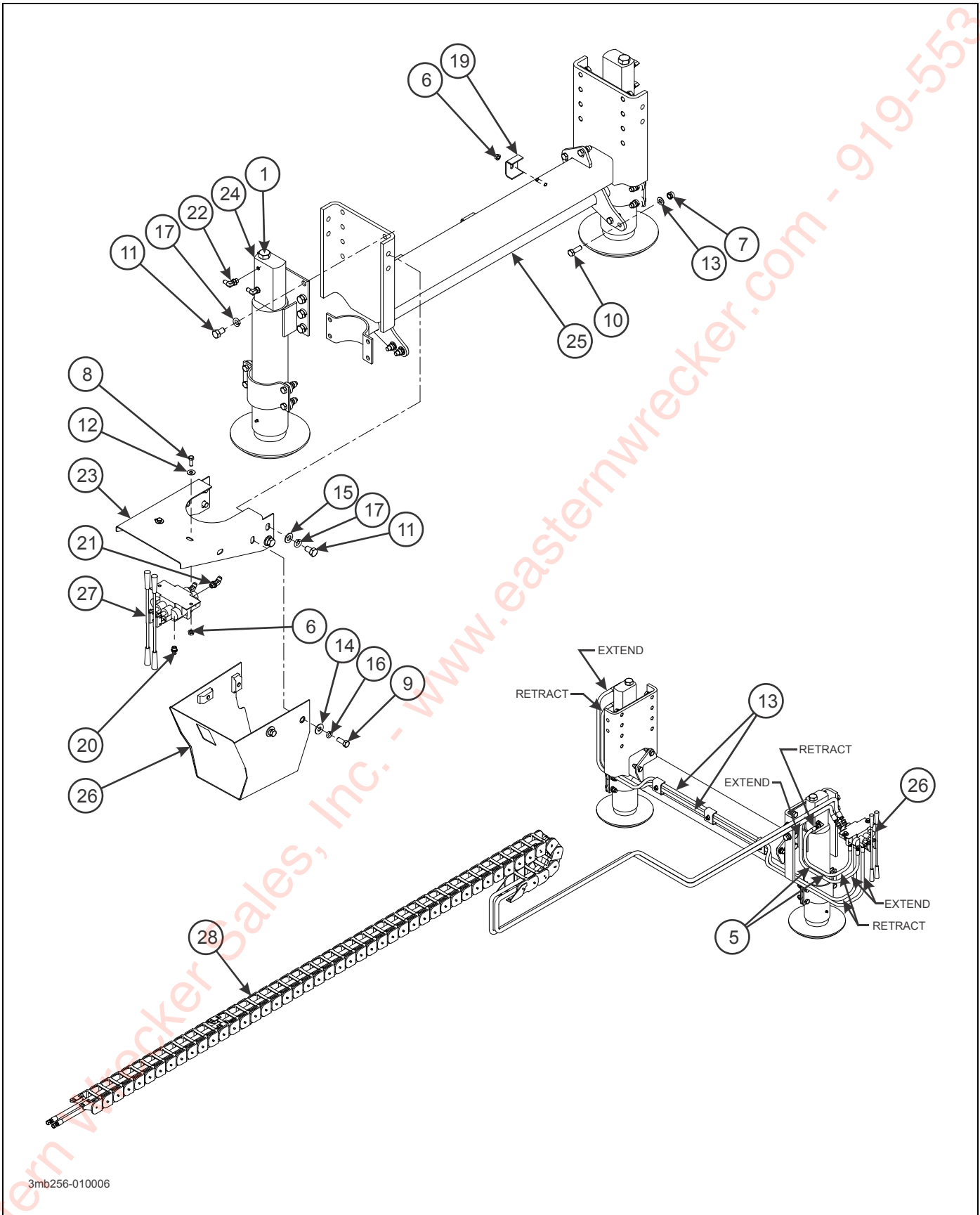
Figure 2-67: Dock Leveler Assembly, 60K (Option) (317D)
