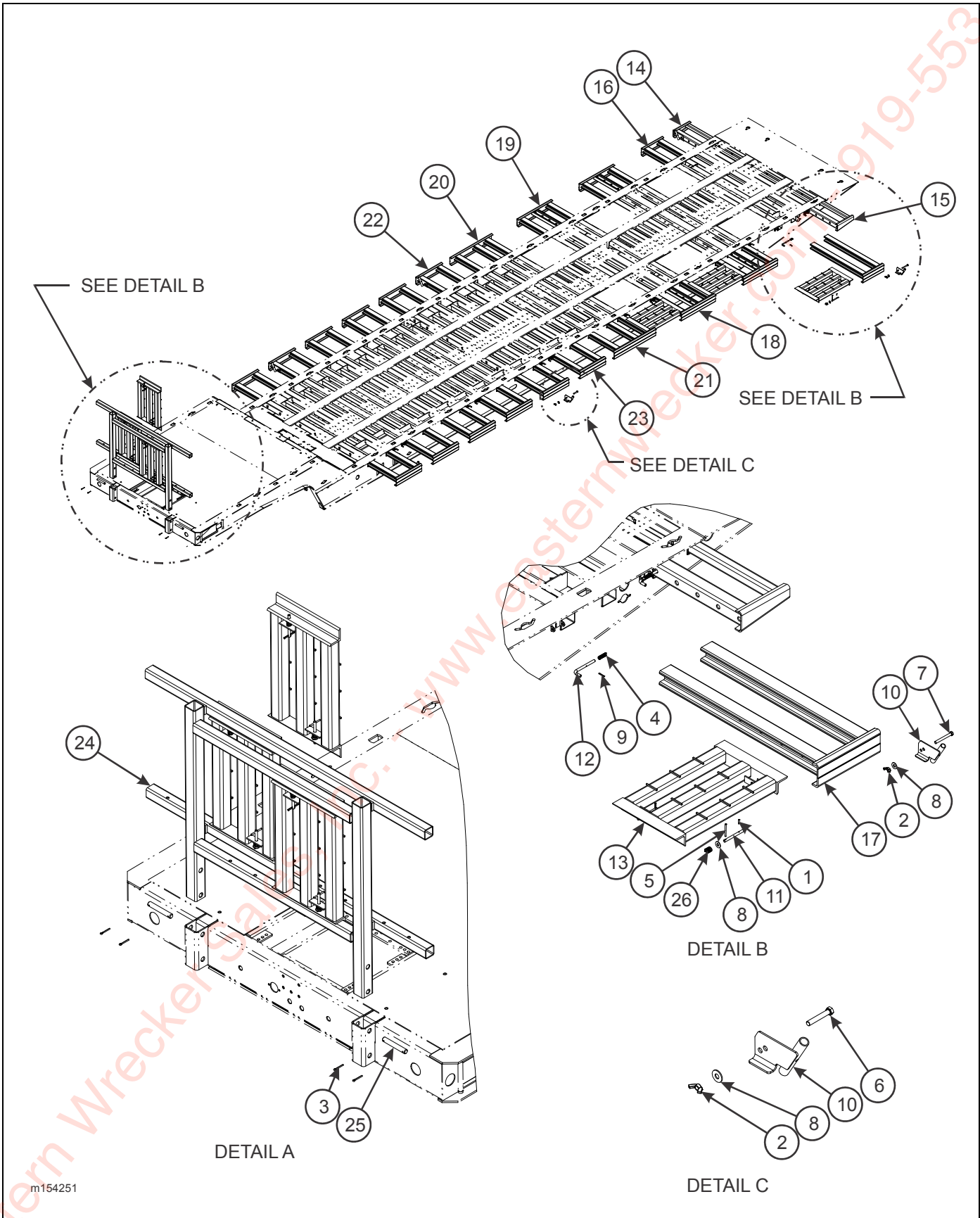
Figure 2-44: Pullout Extension Installation (318-48 x 96)
