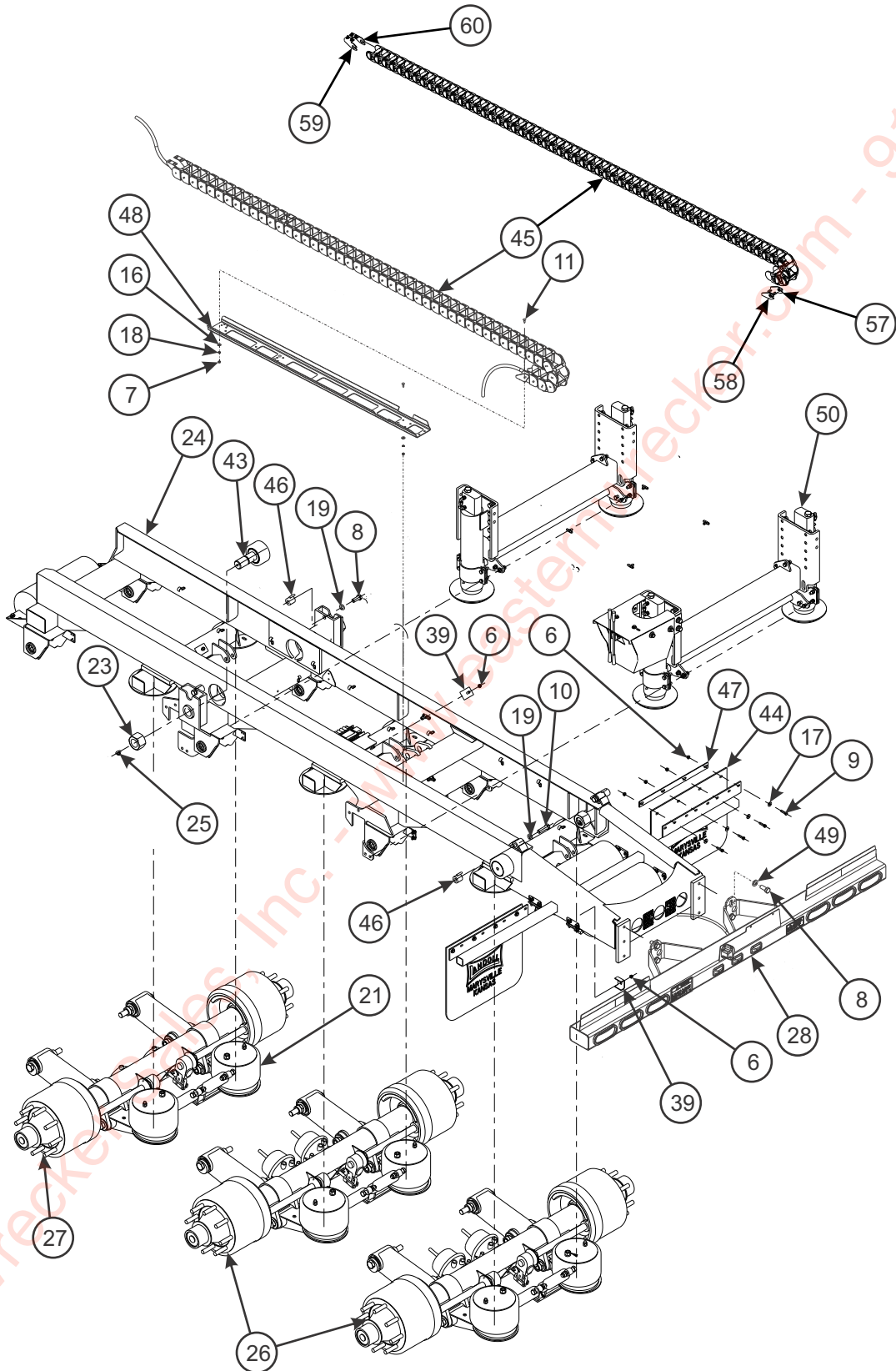
Figure 2-30: U/C Assembly, Air Ride Suspension (318D) (1 of 4)
