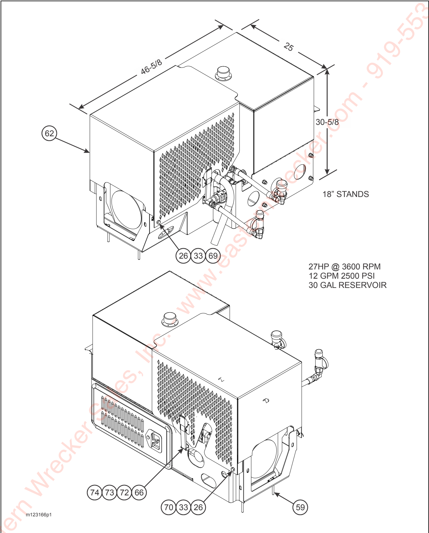
Figure 2-83: Upper Deck Engine Installation (1 of 4)
