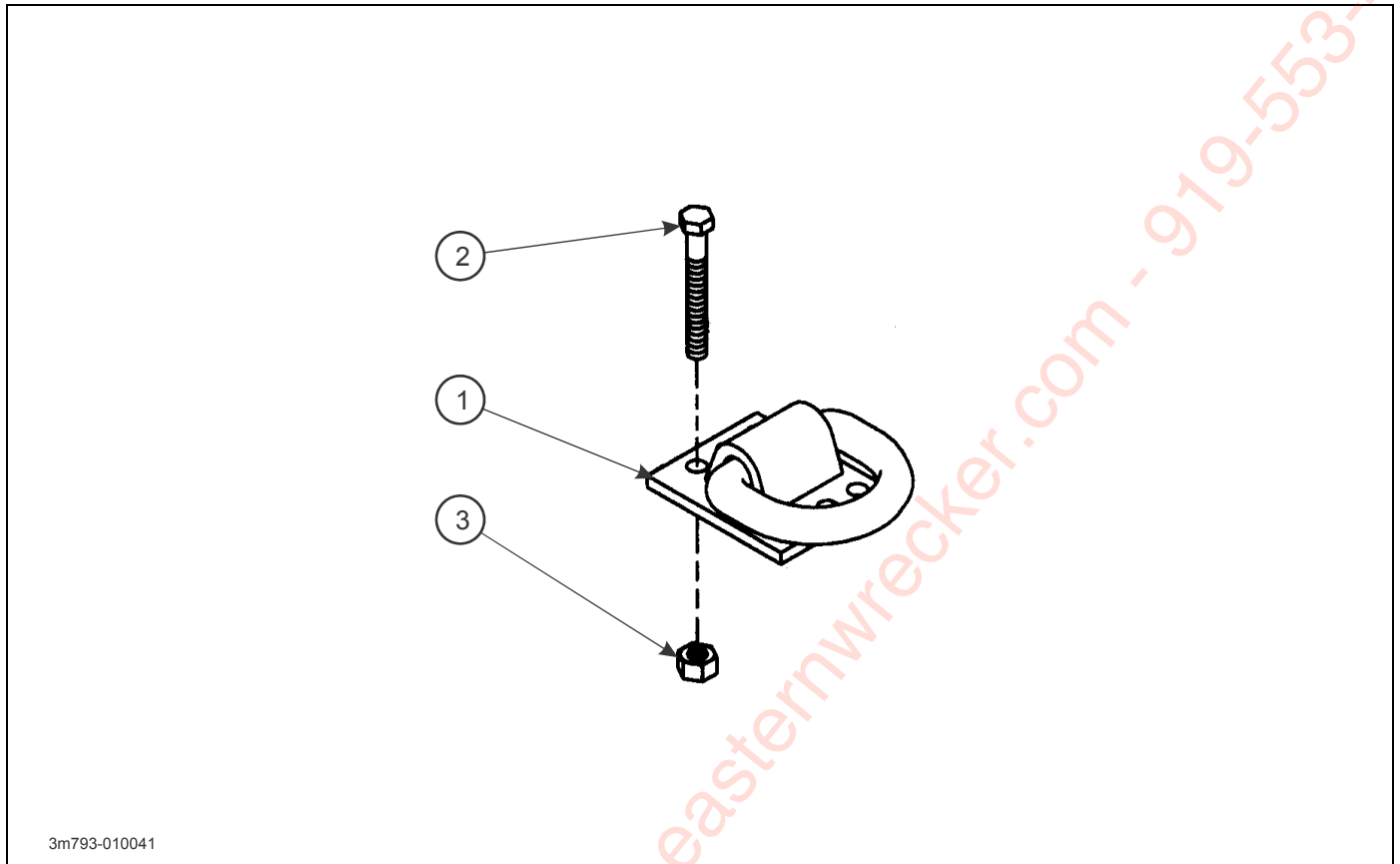
Figure 2-61: Tie Down Installation (Option)
