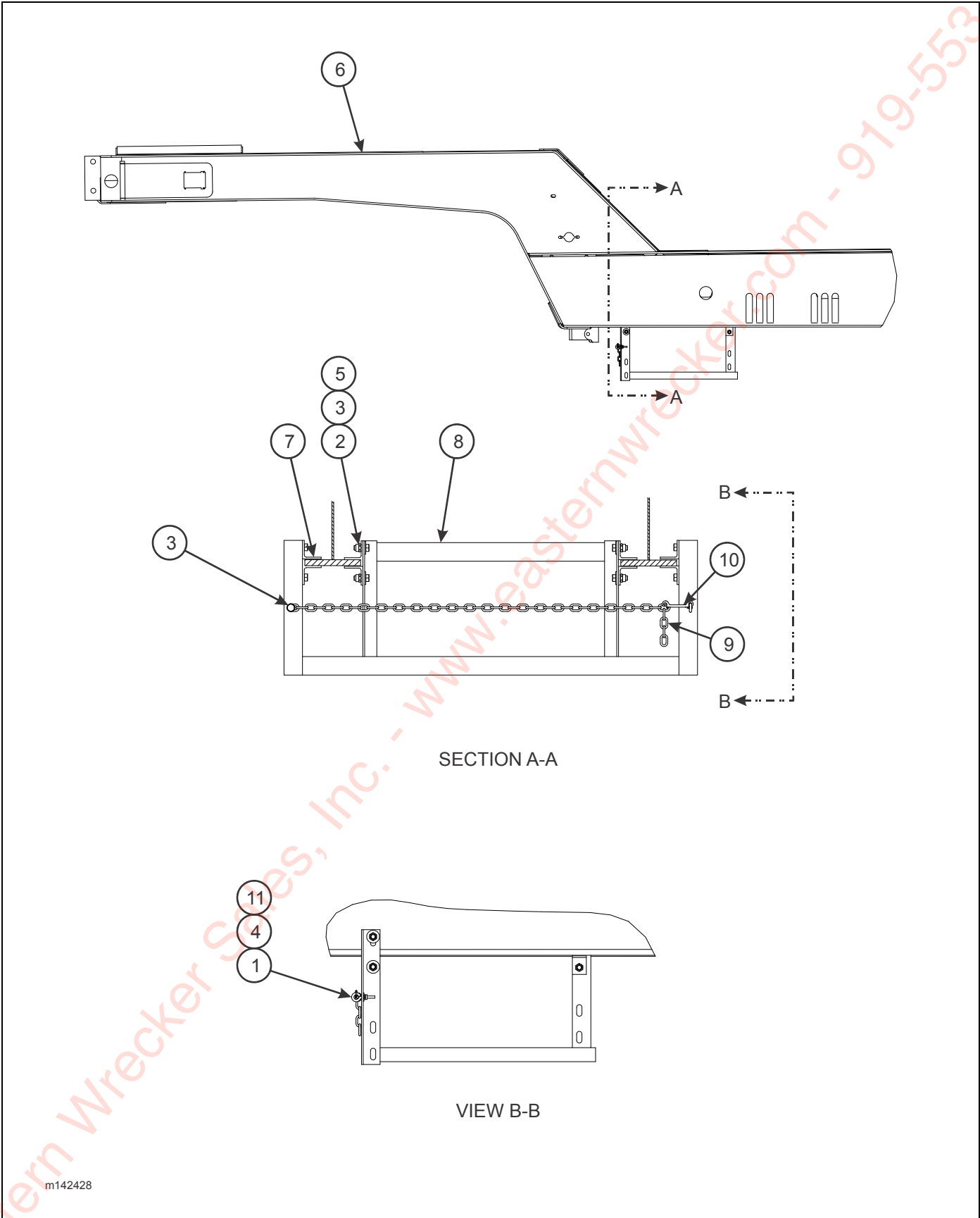
Figure 2-97: Spare Tire Carrier Installation (Option)
