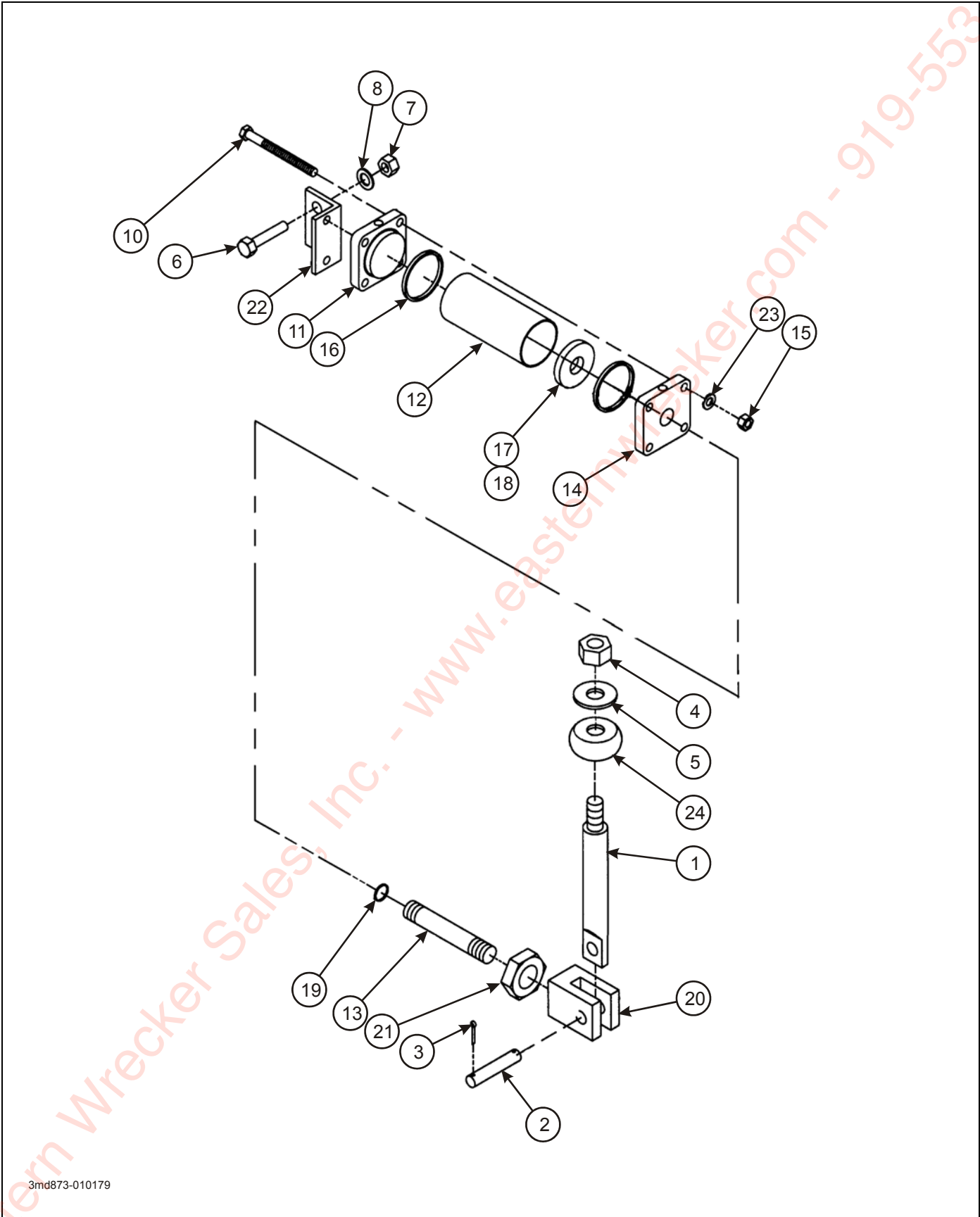
Figure 2-58: Winch Air Shift Cylinder
