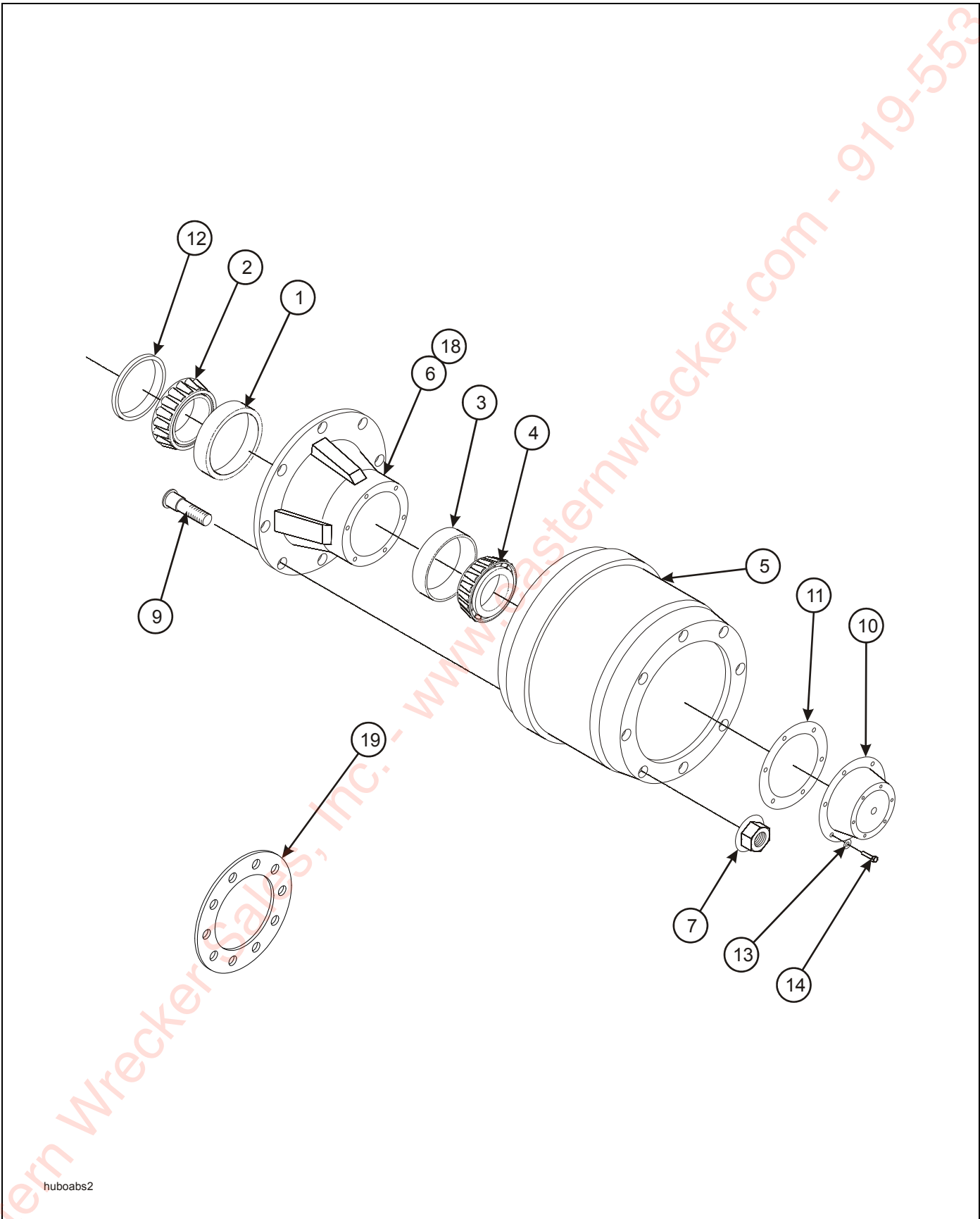
Figure 2-38: Outboard Pilot Mount Hub and Drum
