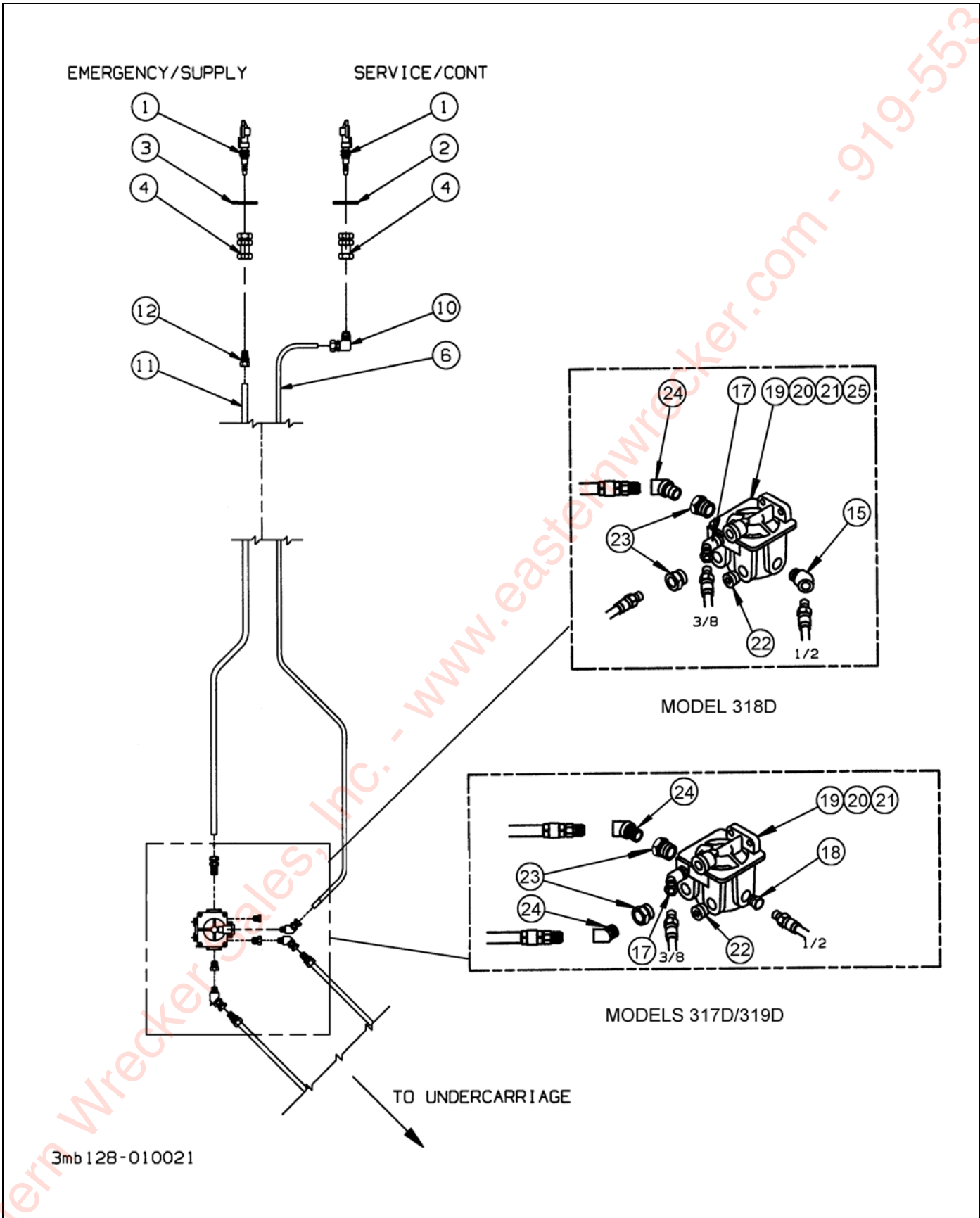
Figure 2-22: Air System, Main
