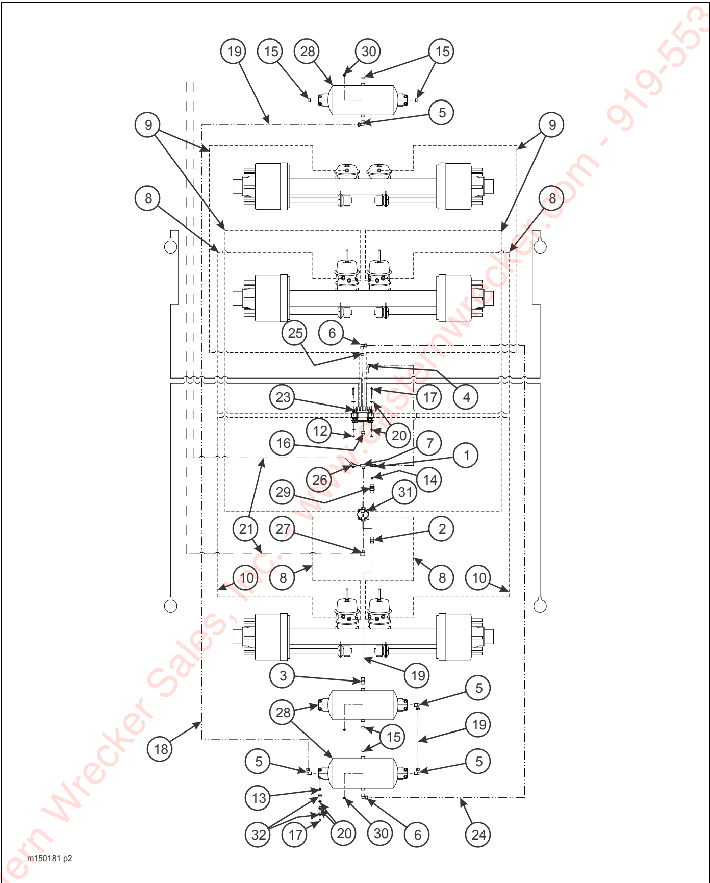
Figure 2-24: Spring Air Brake System w/ ABS (Triple Axle)
