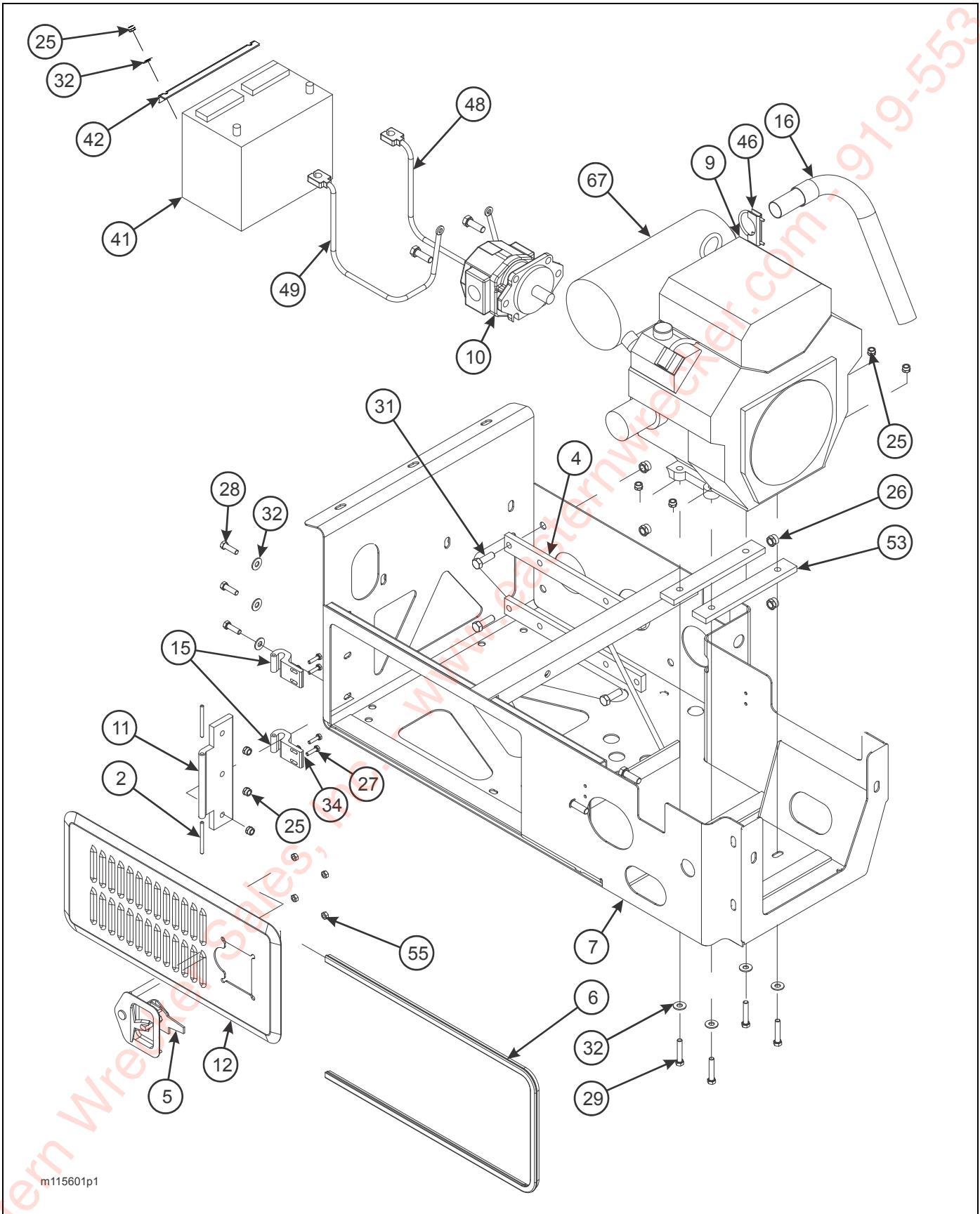
Figure 2-80: 27 HP Gas Engine Installation (1 of 2)
