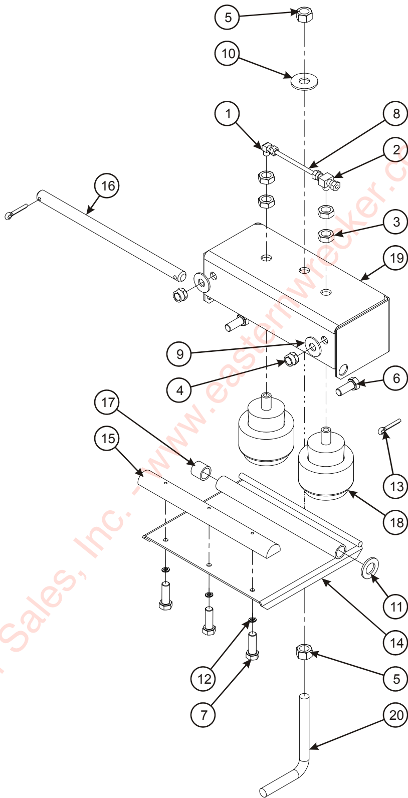
Figure 2-62: Winch, Cable Air Tension
