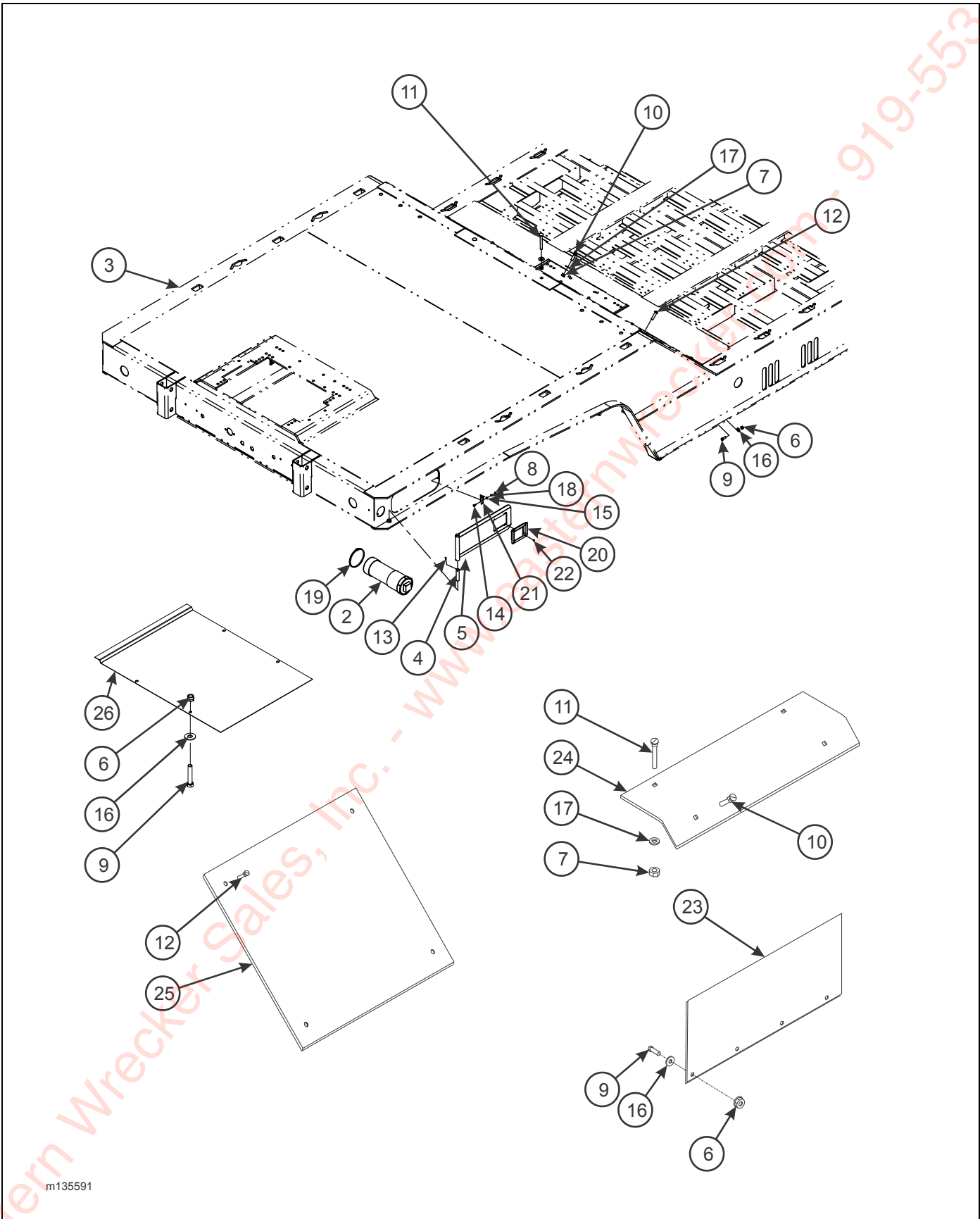
Figure 2-7: Door Latch Installation
