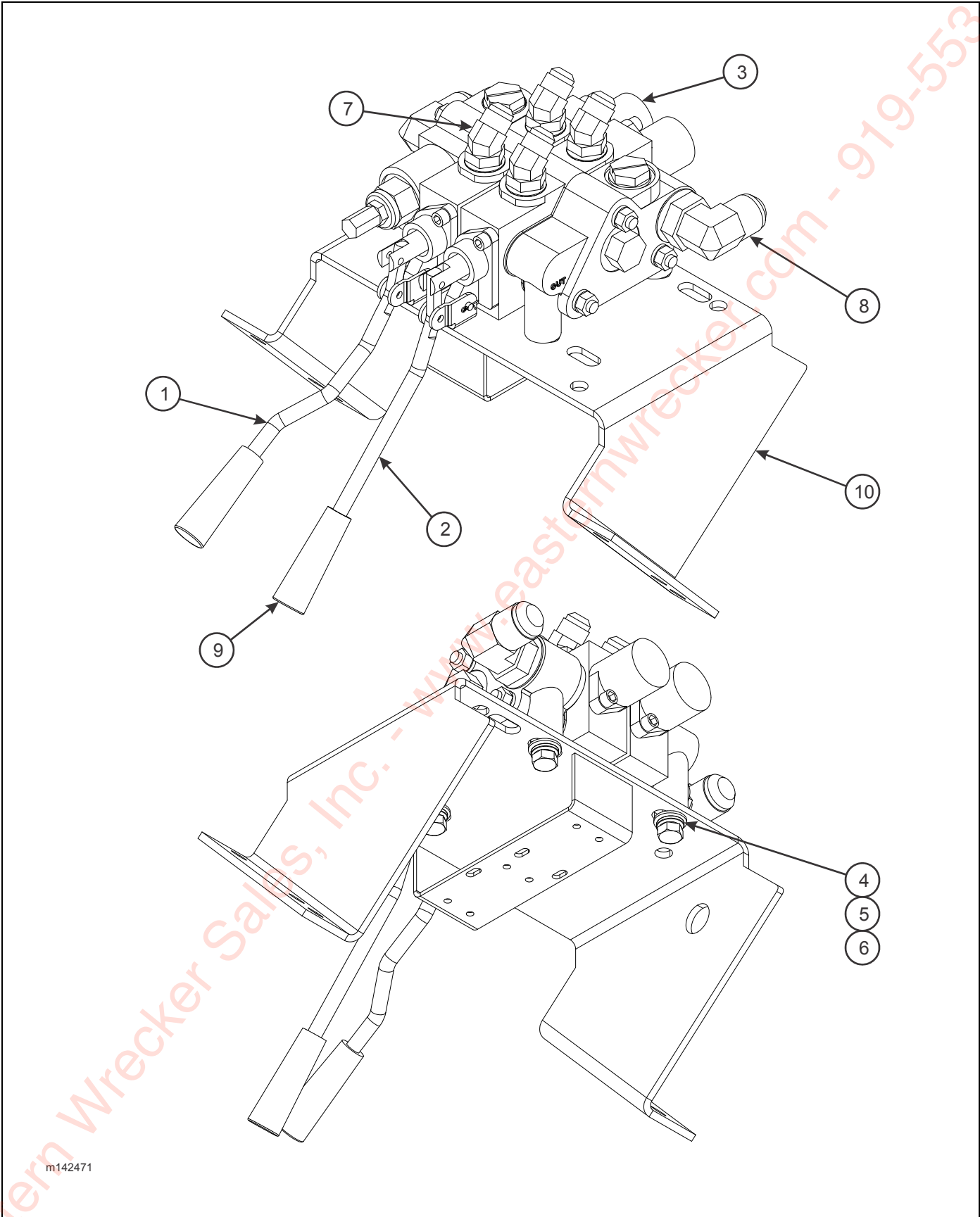
Figure 2-15: Valve Assembly, Two Spool
