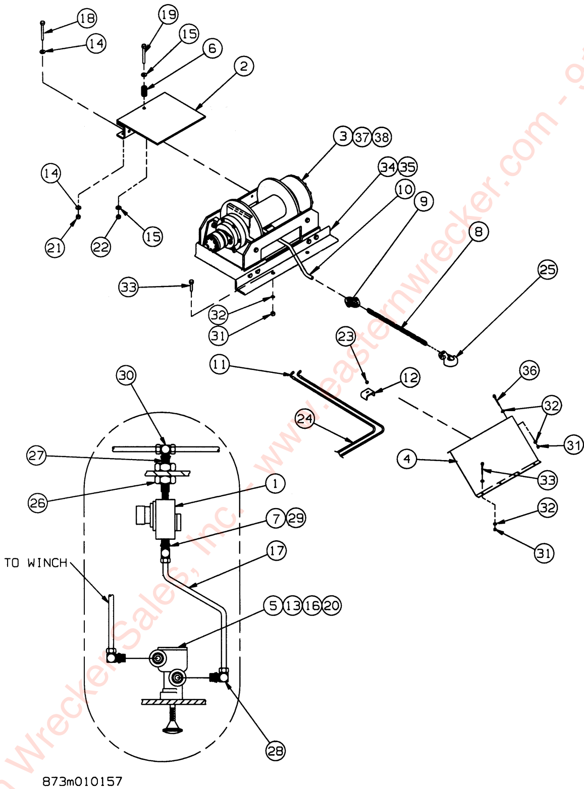
Figure 2-48: Winch Installation, 30K
