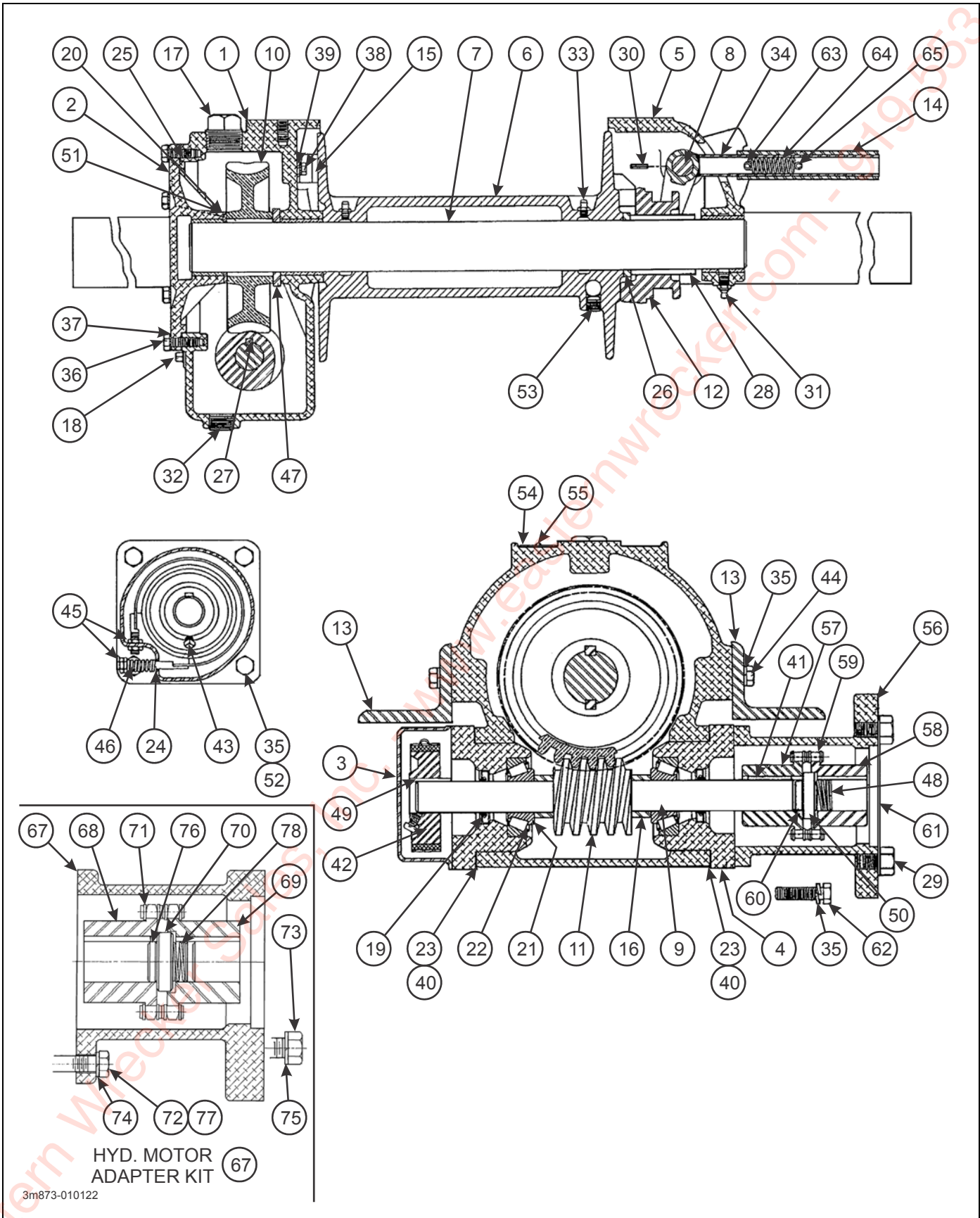
Figure 2-55: 12,000 Lb. Winch Items
