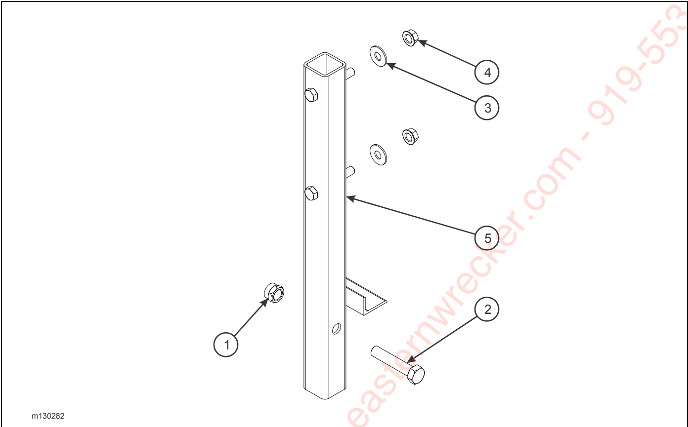
Figure 2-95: Spare Tire Mount Assembly
