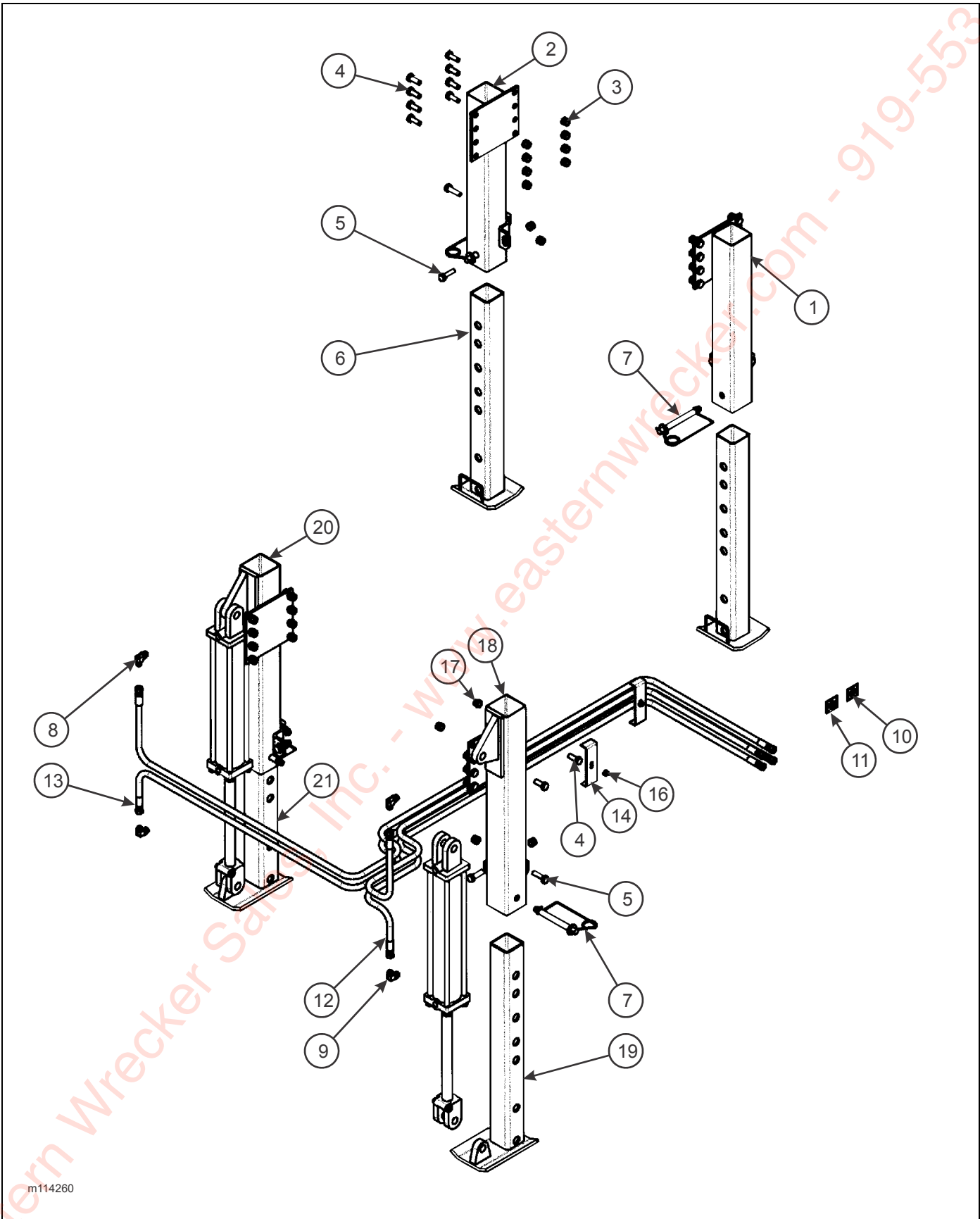
Figure 2-78: Landing Gear Installation - Bolt-On
