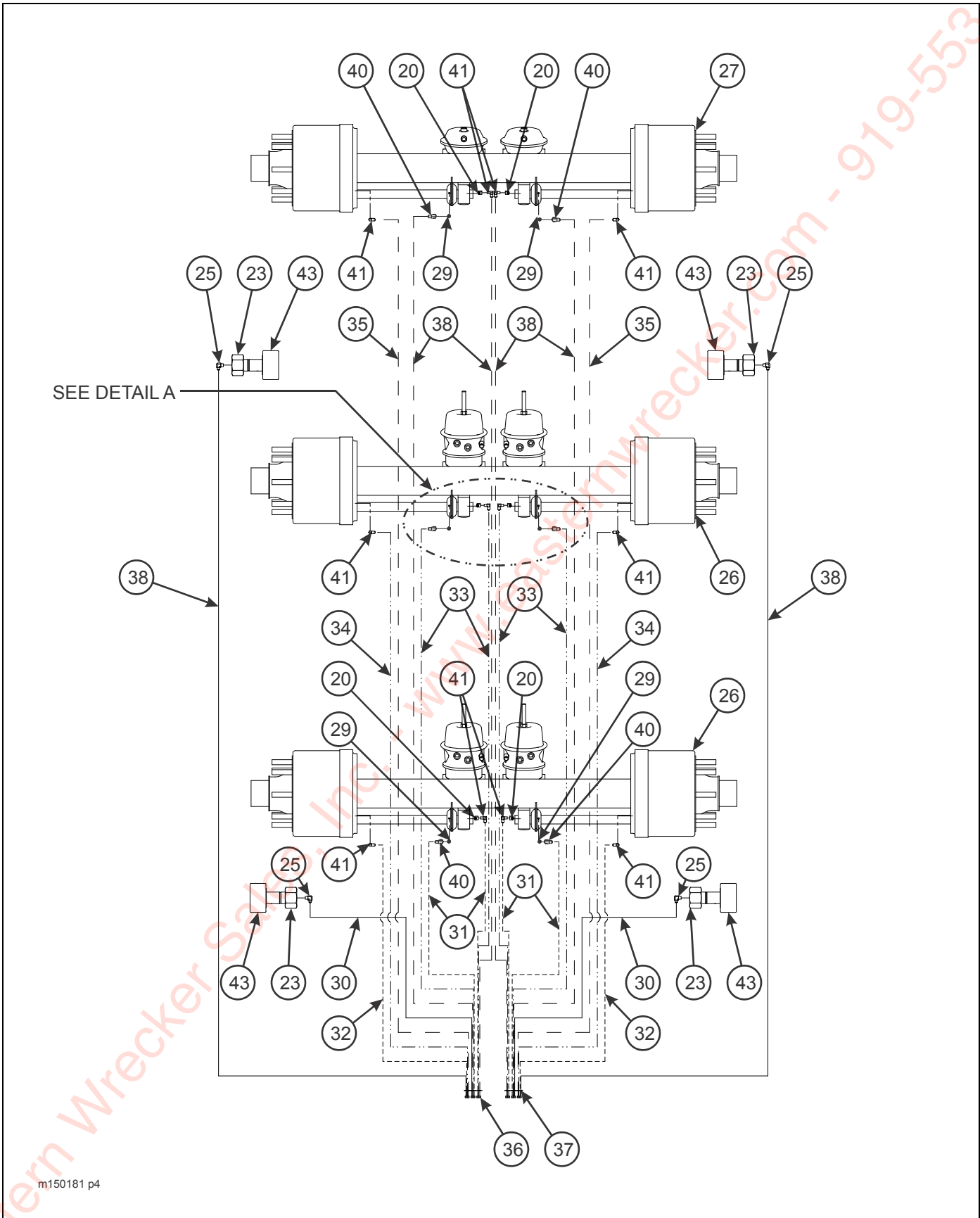
Figure 2-32: U/C Assembly, Air Ride Suspension (318D) (3 of 4)
