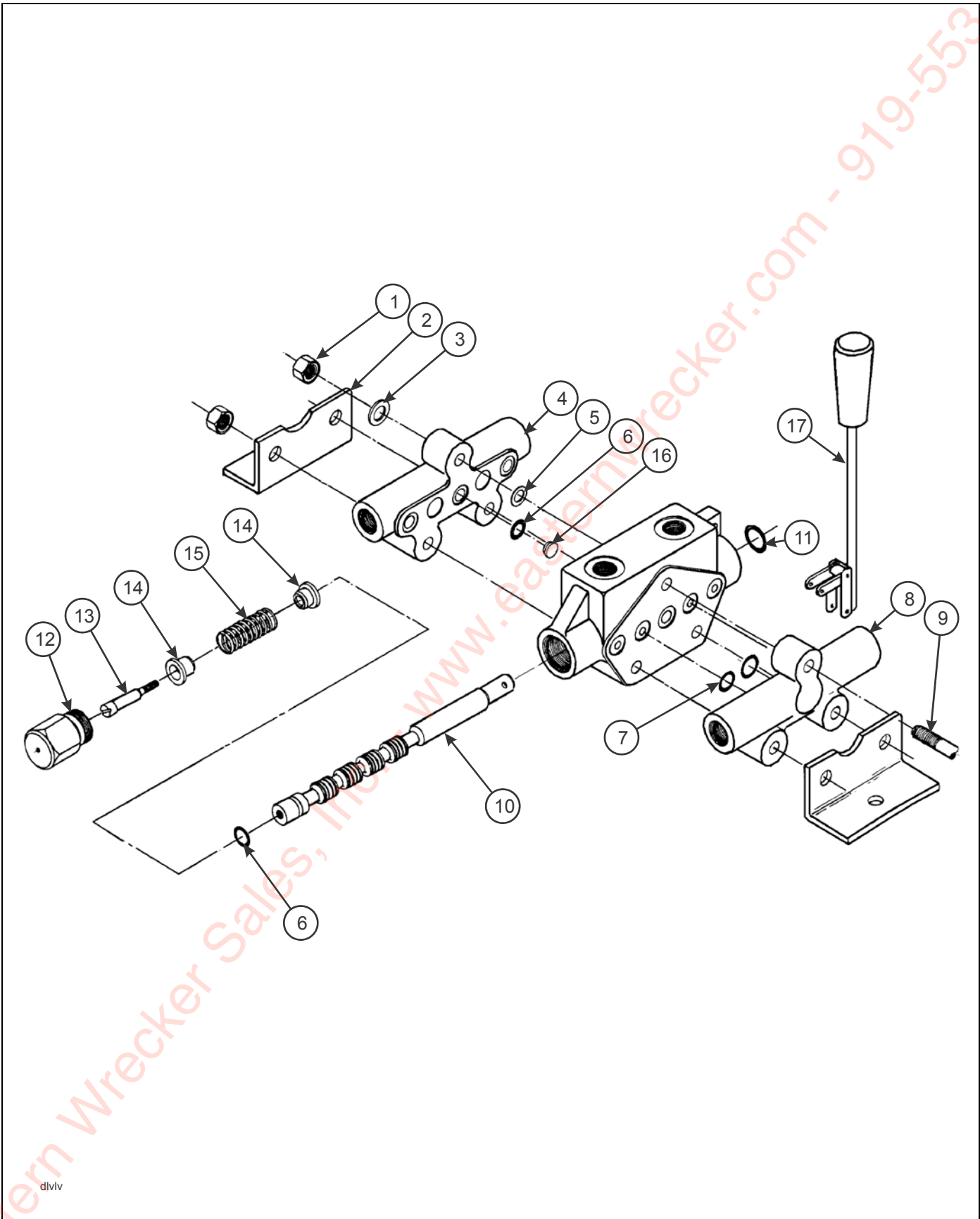
Figure 2-73: Dock Leveler Valve (Before 01/15/2014)
