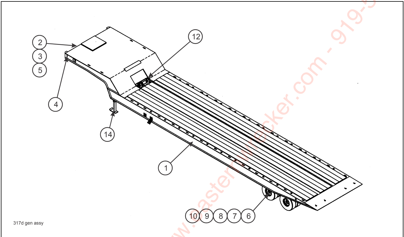
Figure 2-1: General Assembly
