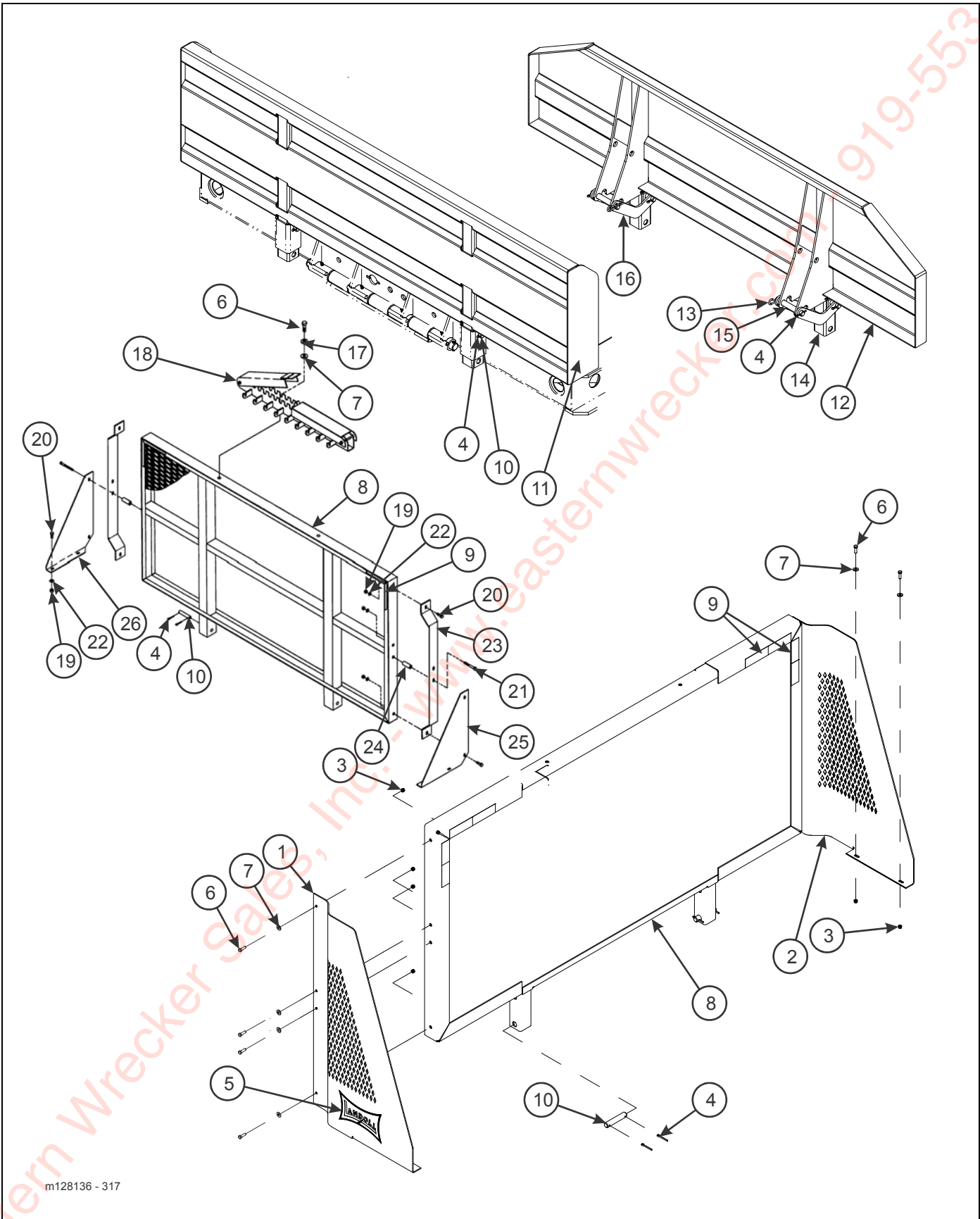
Figure 2-39: Bulkhead Assembly
