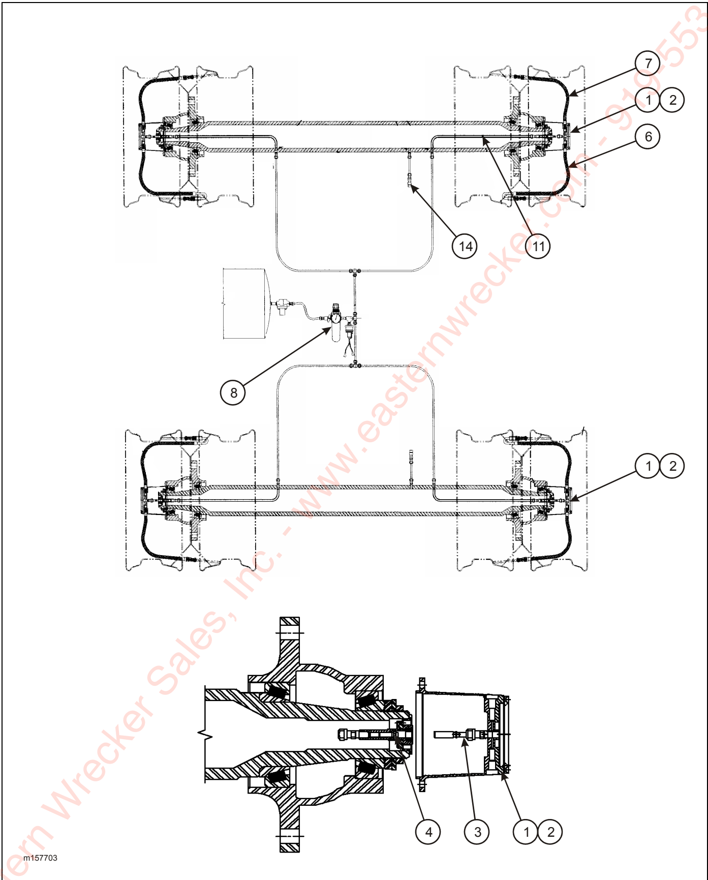
Figure 2-94: Tire Inflation System (Option)
