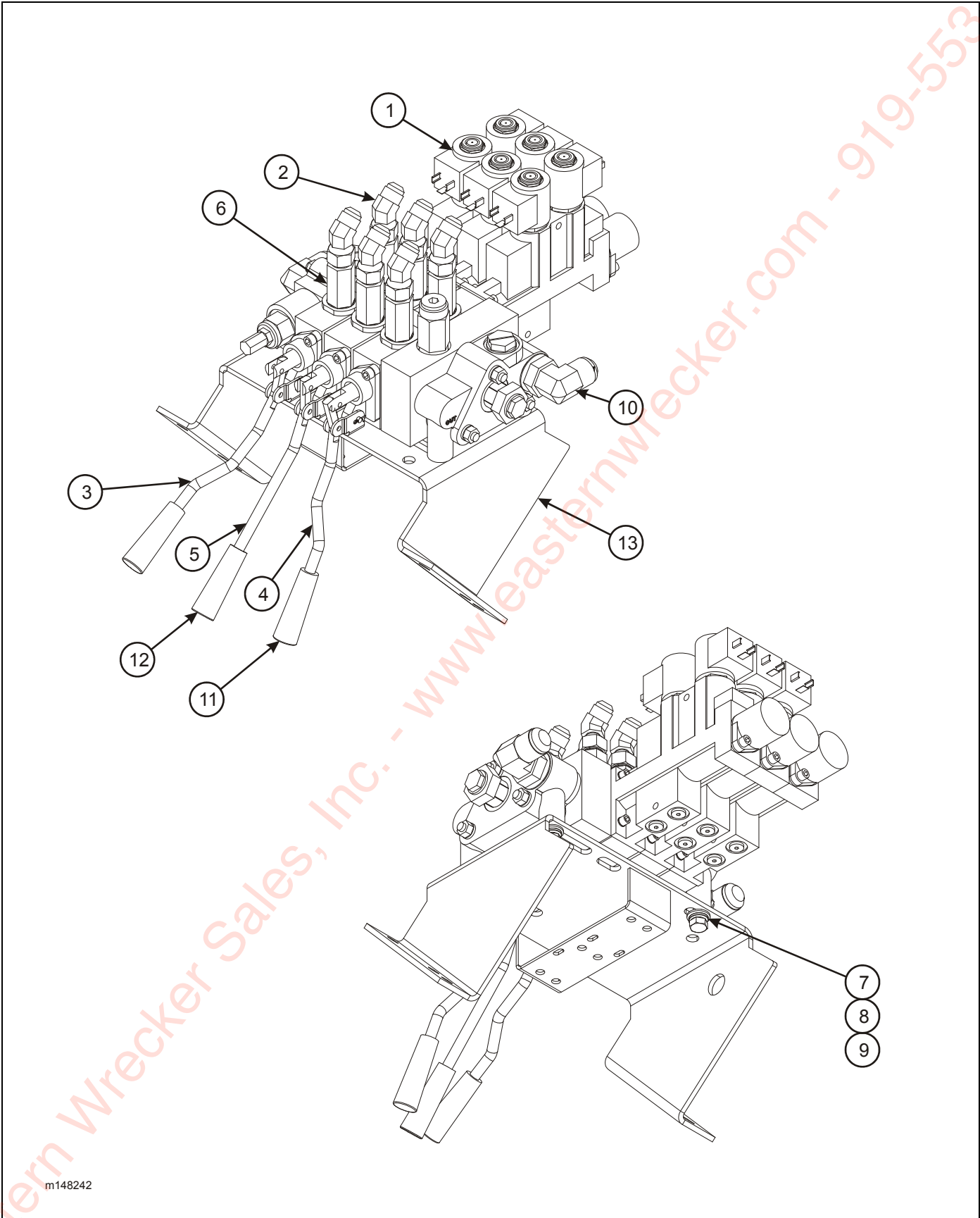
Figure 2-14: Valve Assembly, Three Spool
