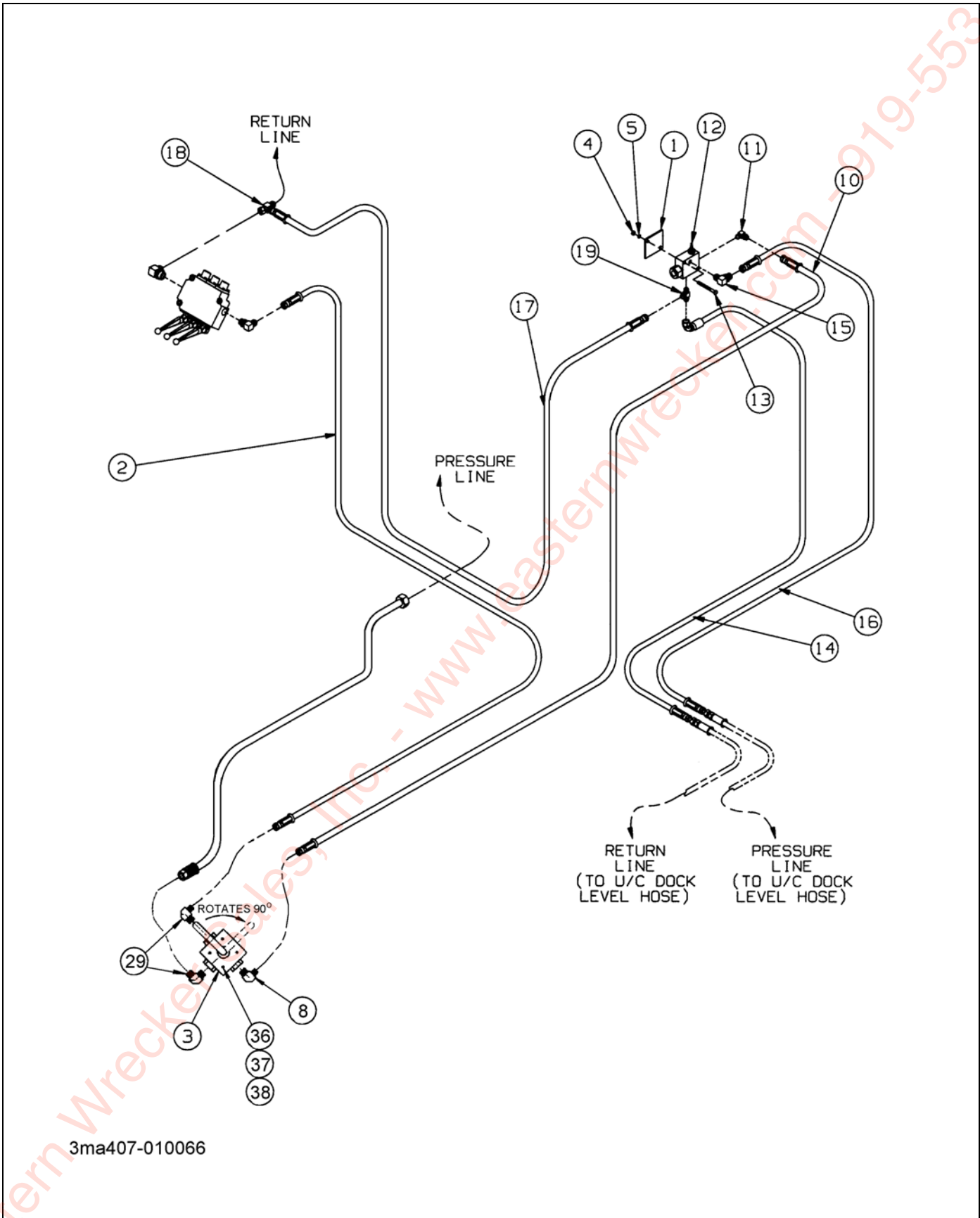
Figure 2-66: Dock Leveler Hydraulic Installation (Option)
