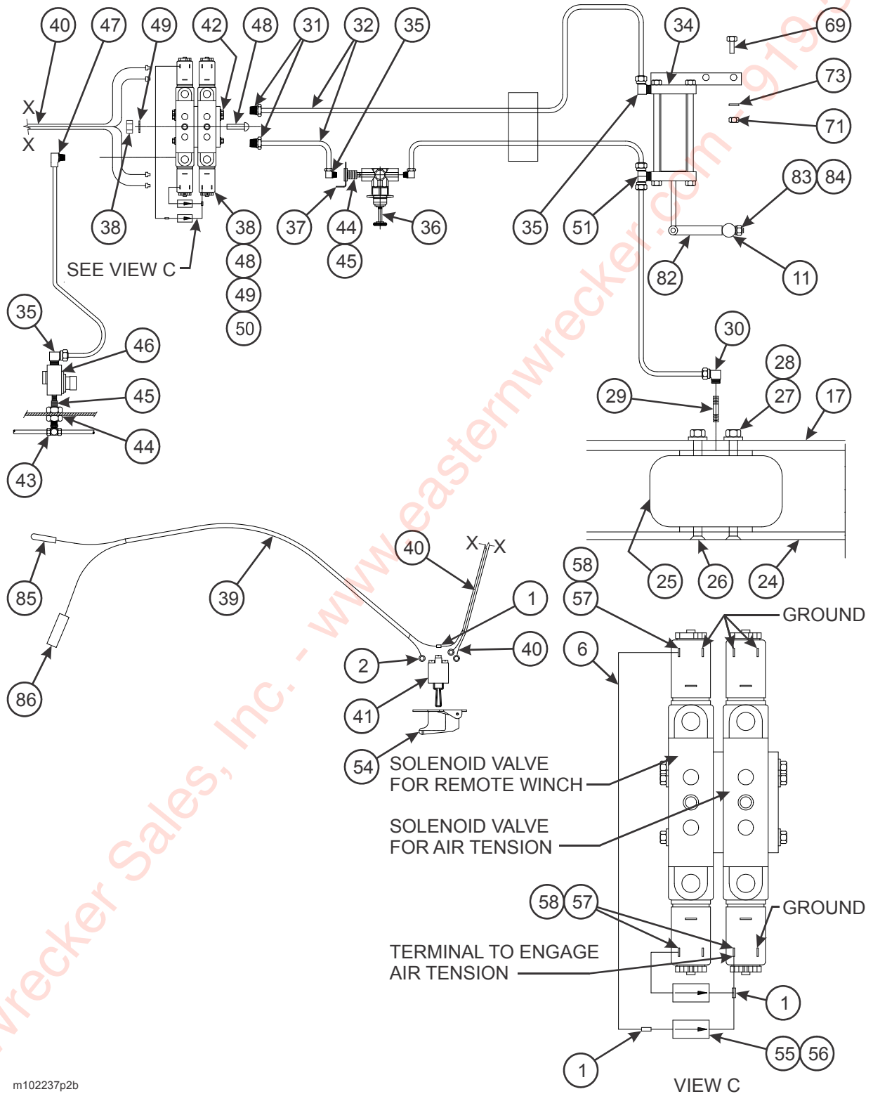
Figure 2-52: Winch Air Tension Installation, Upper Deck 20K (2 of 4)
