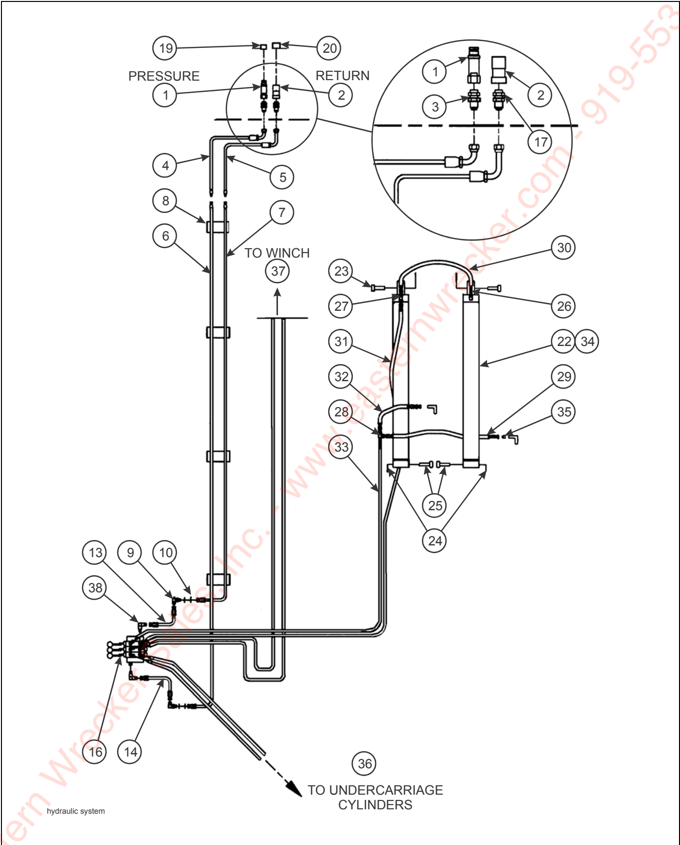
Figure 2-8: Hydraulic System
