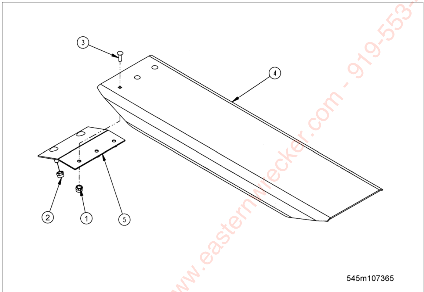
Figure 2-93: Ramps (Option)
