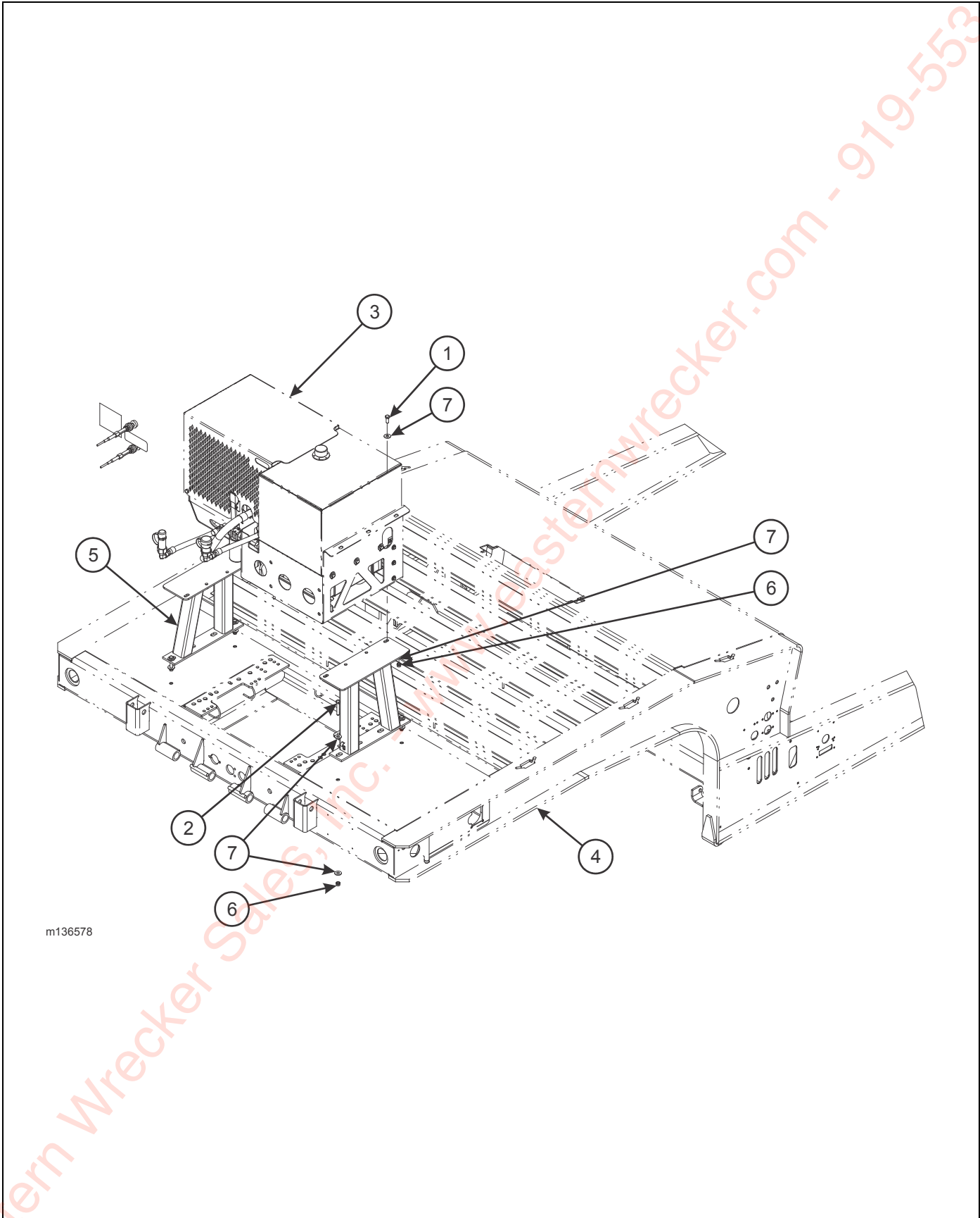
Figure 2-87: Upper Deck Engine Stand Installation
