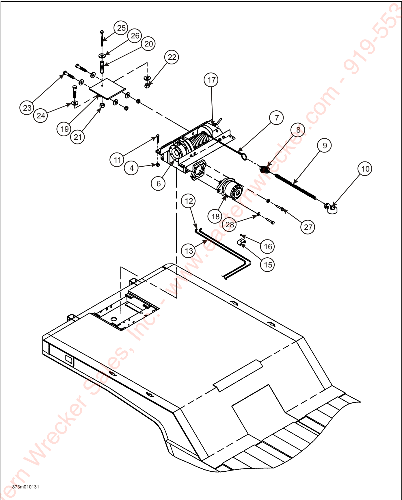
Figure 2-47: Winch Installation, Upperdeck
