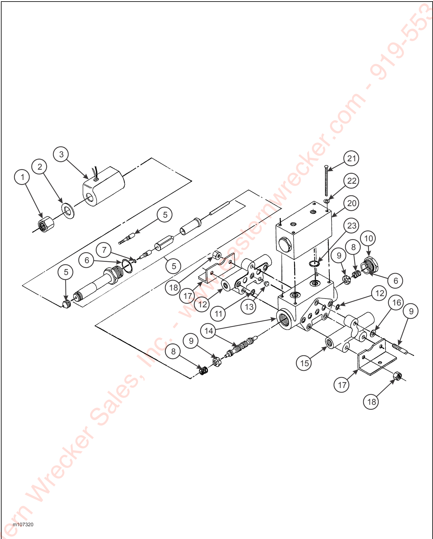
Figure 2-75: Dock Leveler Valve
