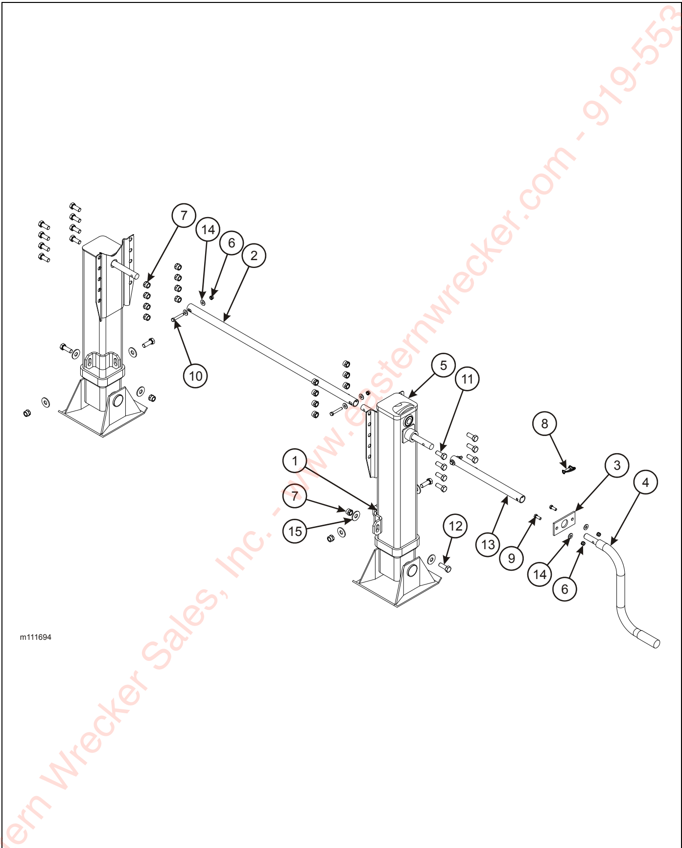
Figure 2-76: Landing Gear Installation
