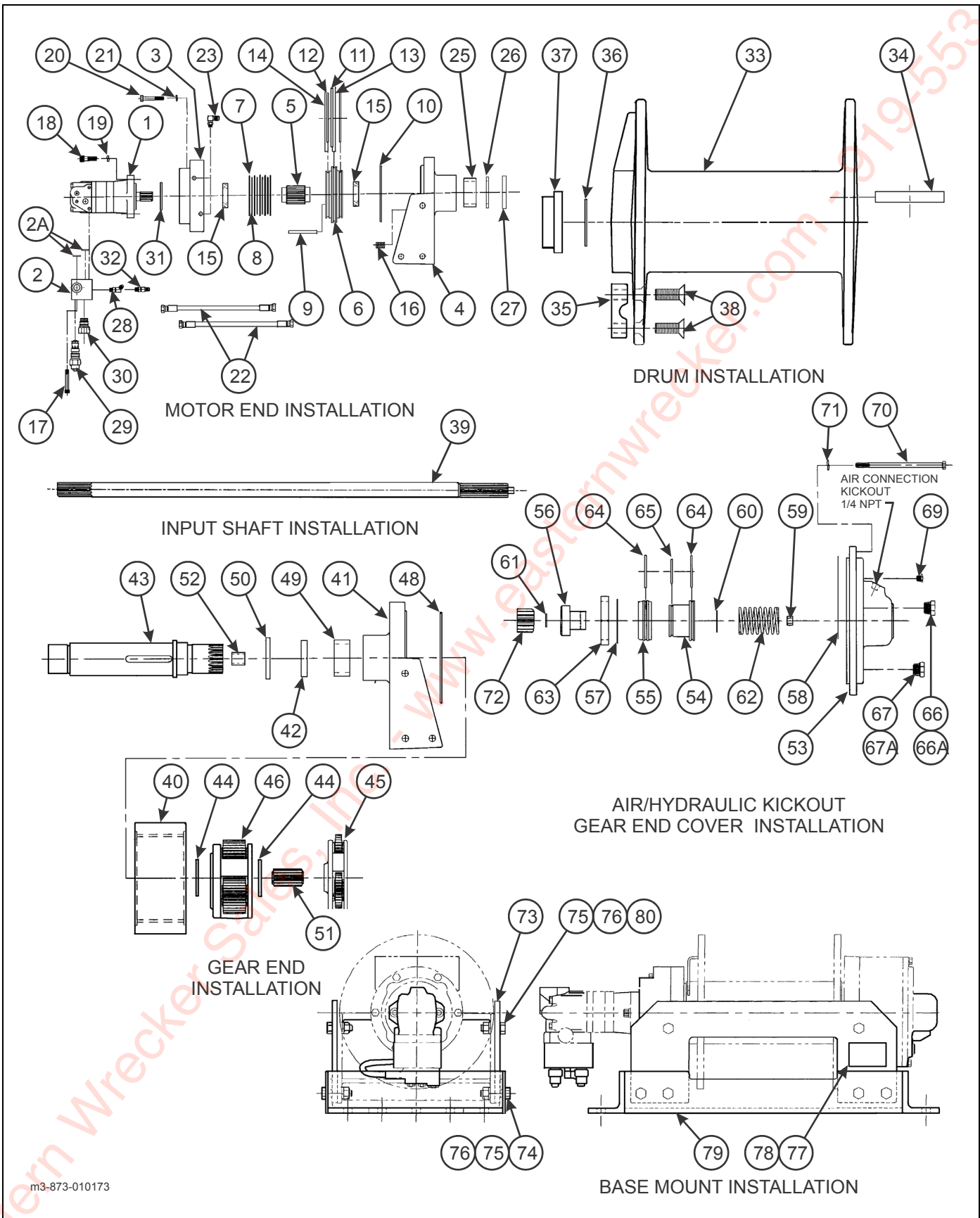
Figure 2-57: 30,000 Lb. Winch Items (DP)
