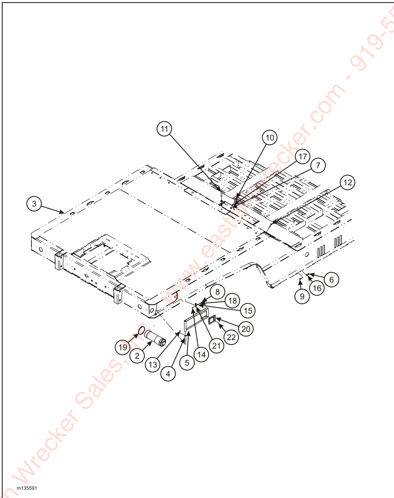
FIGURE 1-33 DOOR AND COVER INSTALLATION
