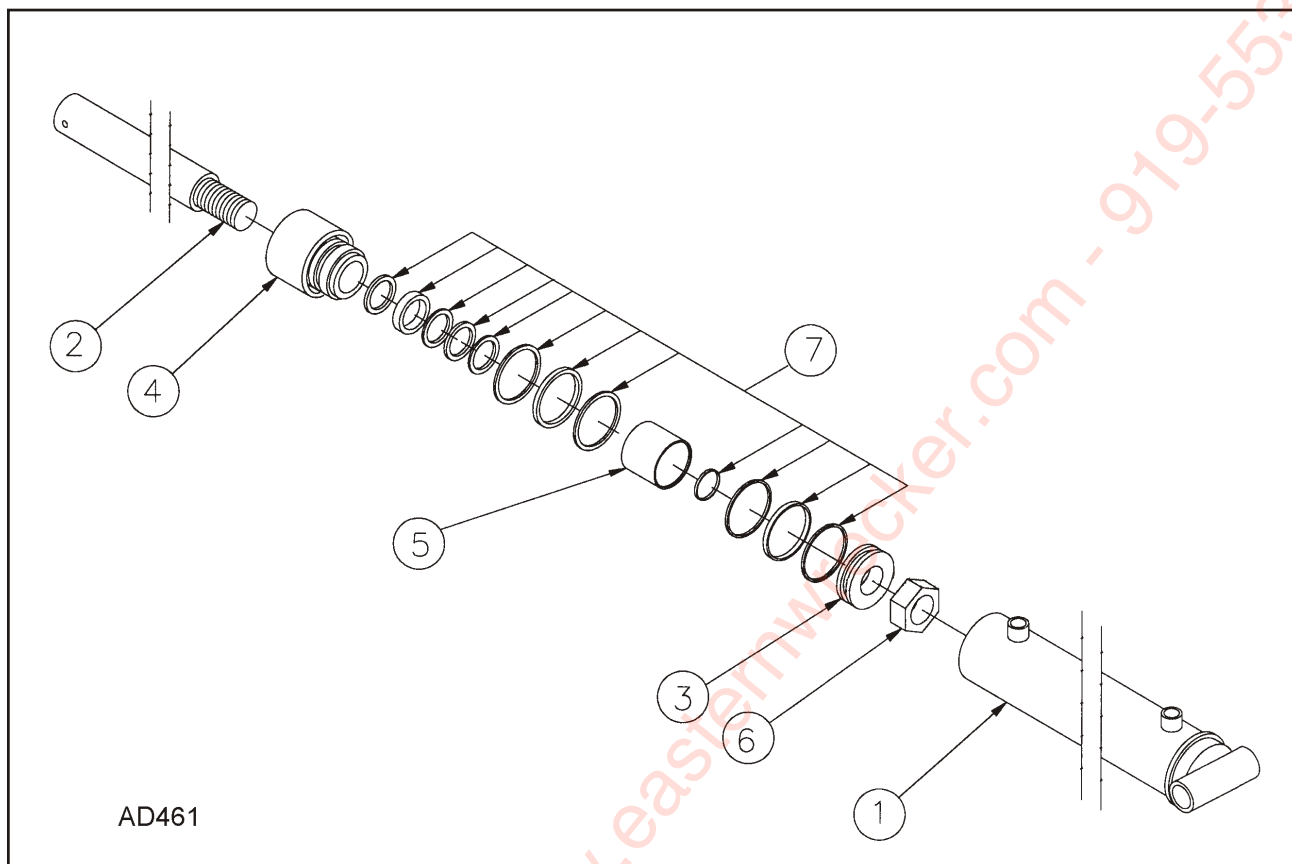
FIGURE 1-7 CYLINDER 4" X 126"
