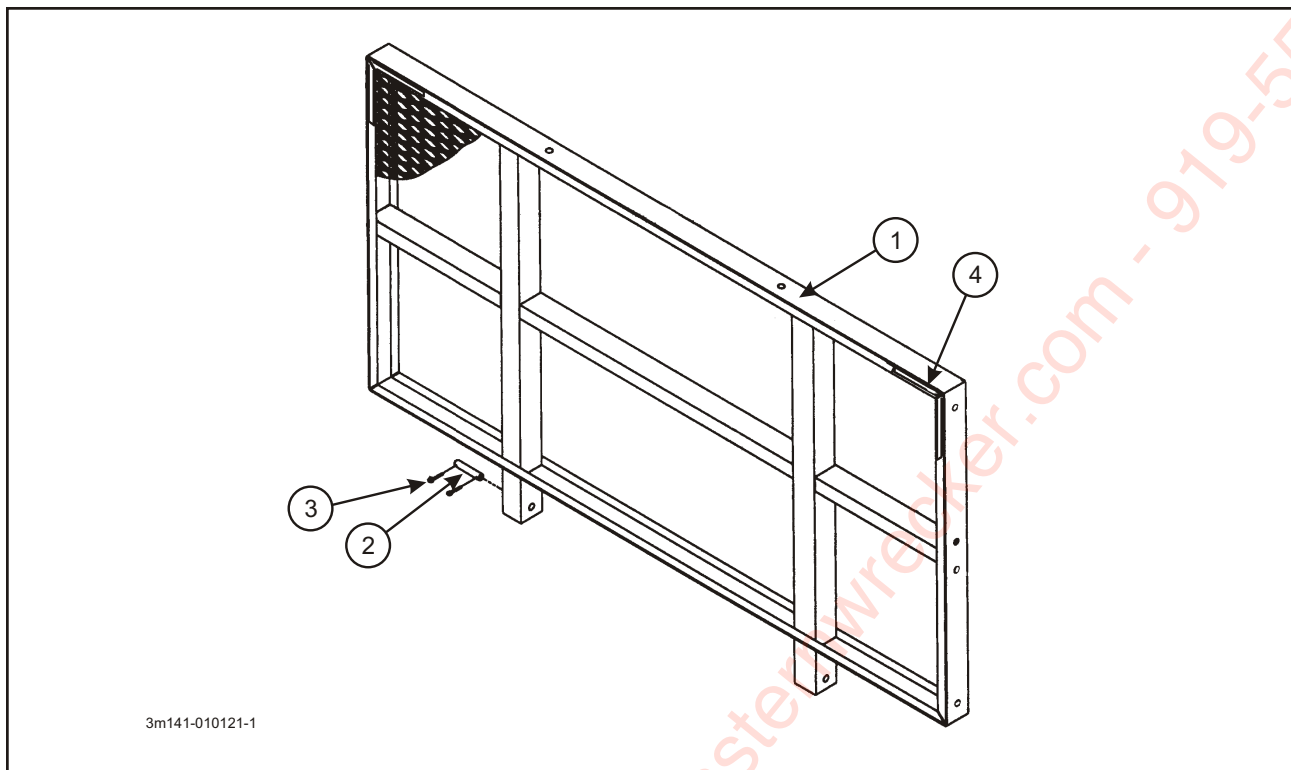
FIGURE 1-38 BULKHEAD ASSEMBLY
