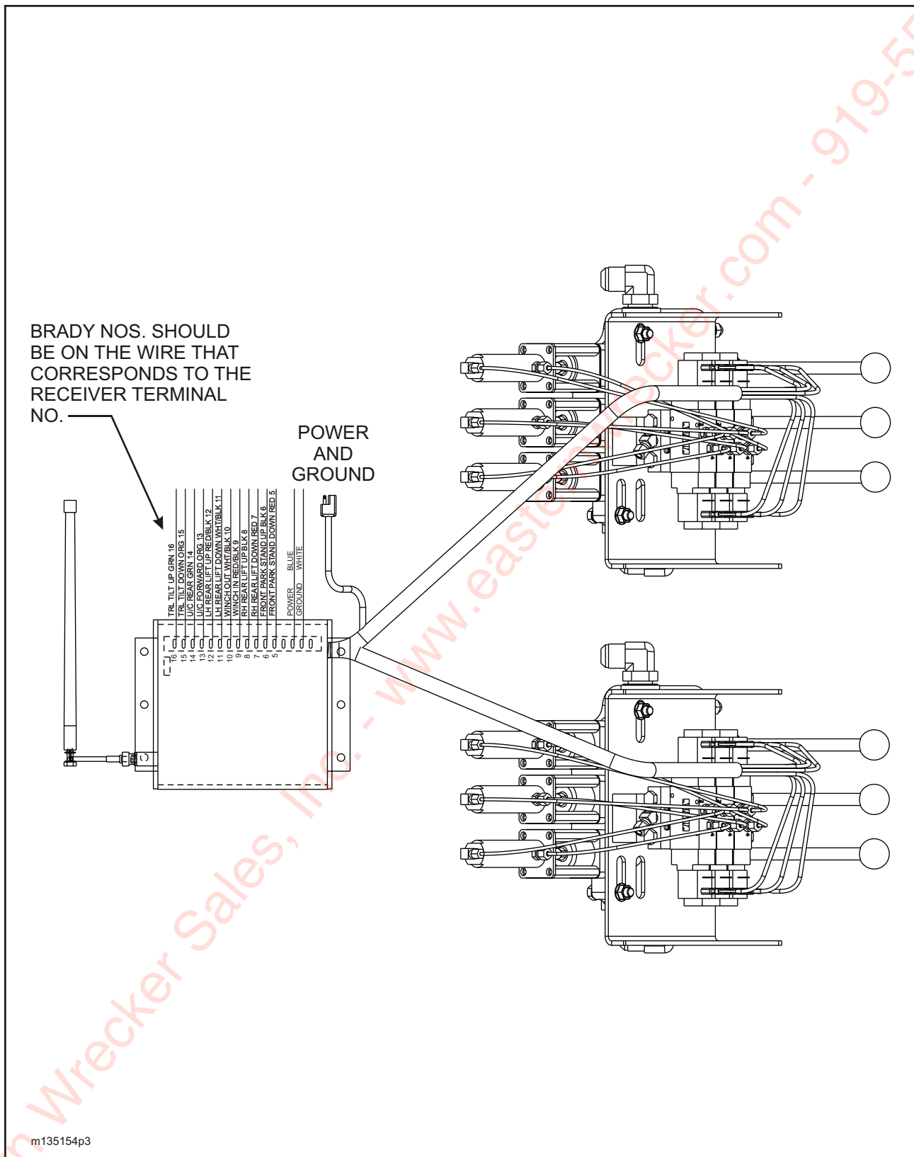
FIGURE 1-14 ELECTRICAL SYSTEM W/ REMOTE (3 OF 3)
