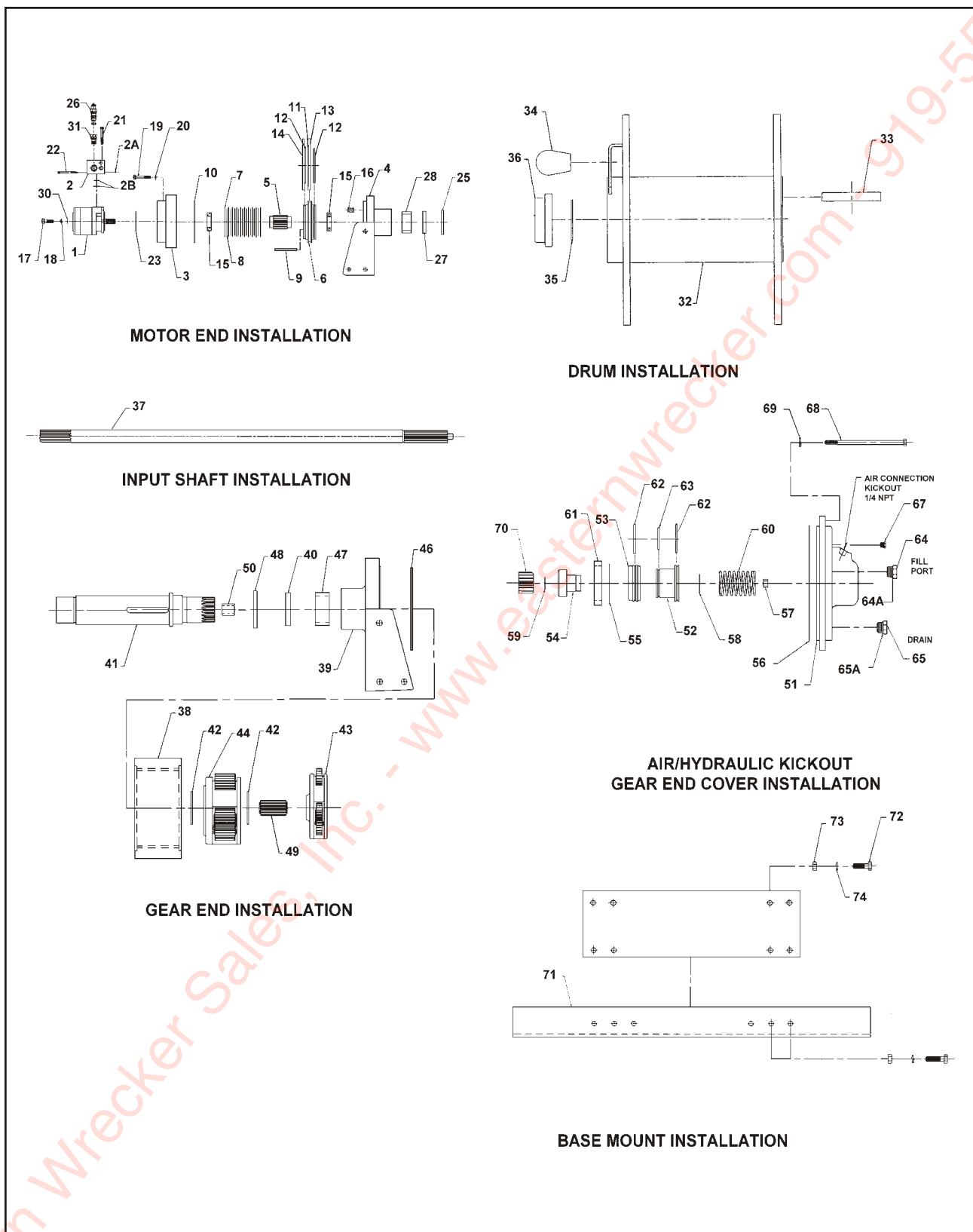
FIGURE 1-30 30,000# WINCH ITEMS
