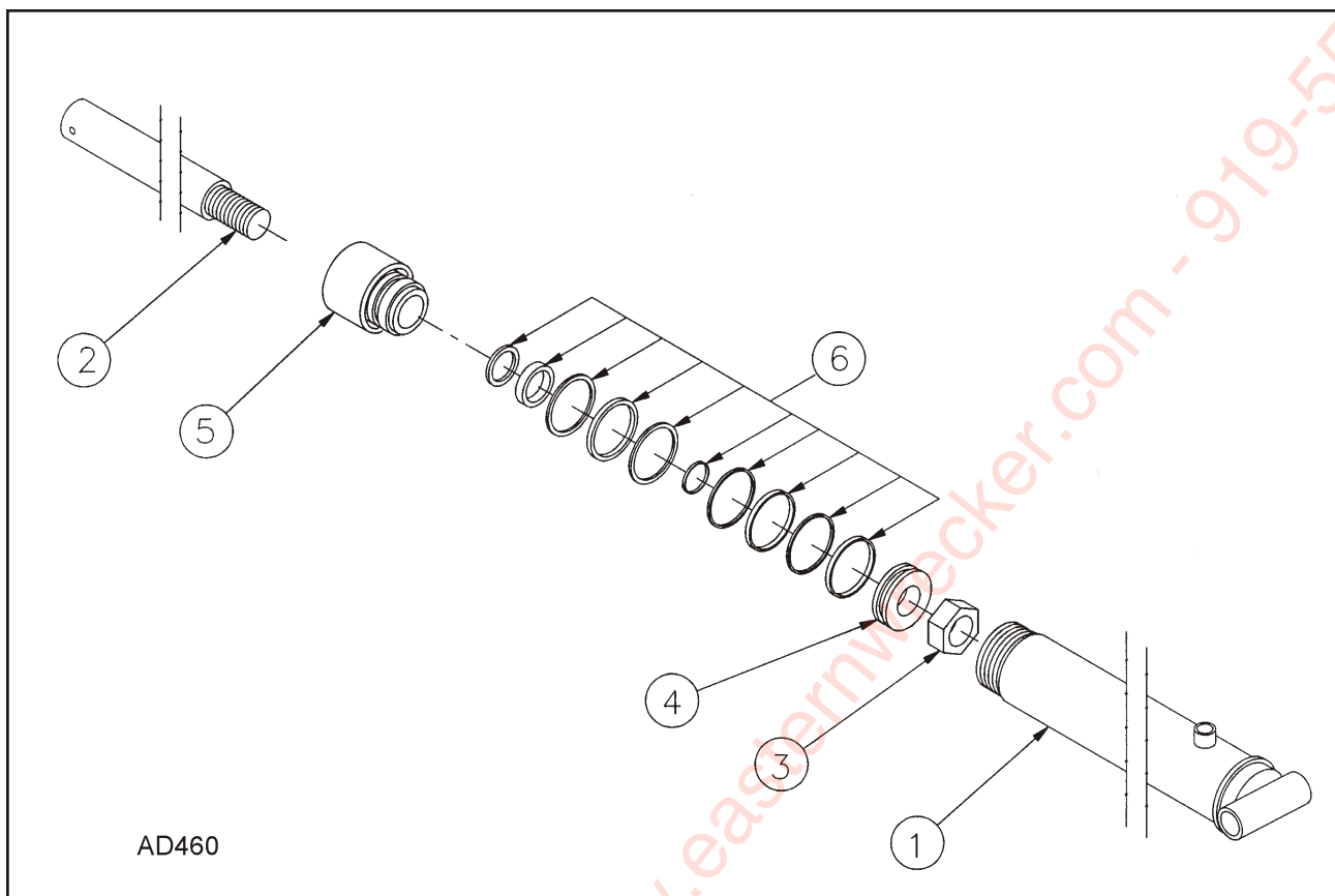
FIGURE 1-6 CYLINDER 4" X 42"
