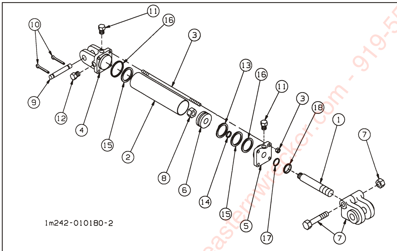
FIGURE 1-9 HYDRAULIC CYLINDER 3-1/2 X 20
