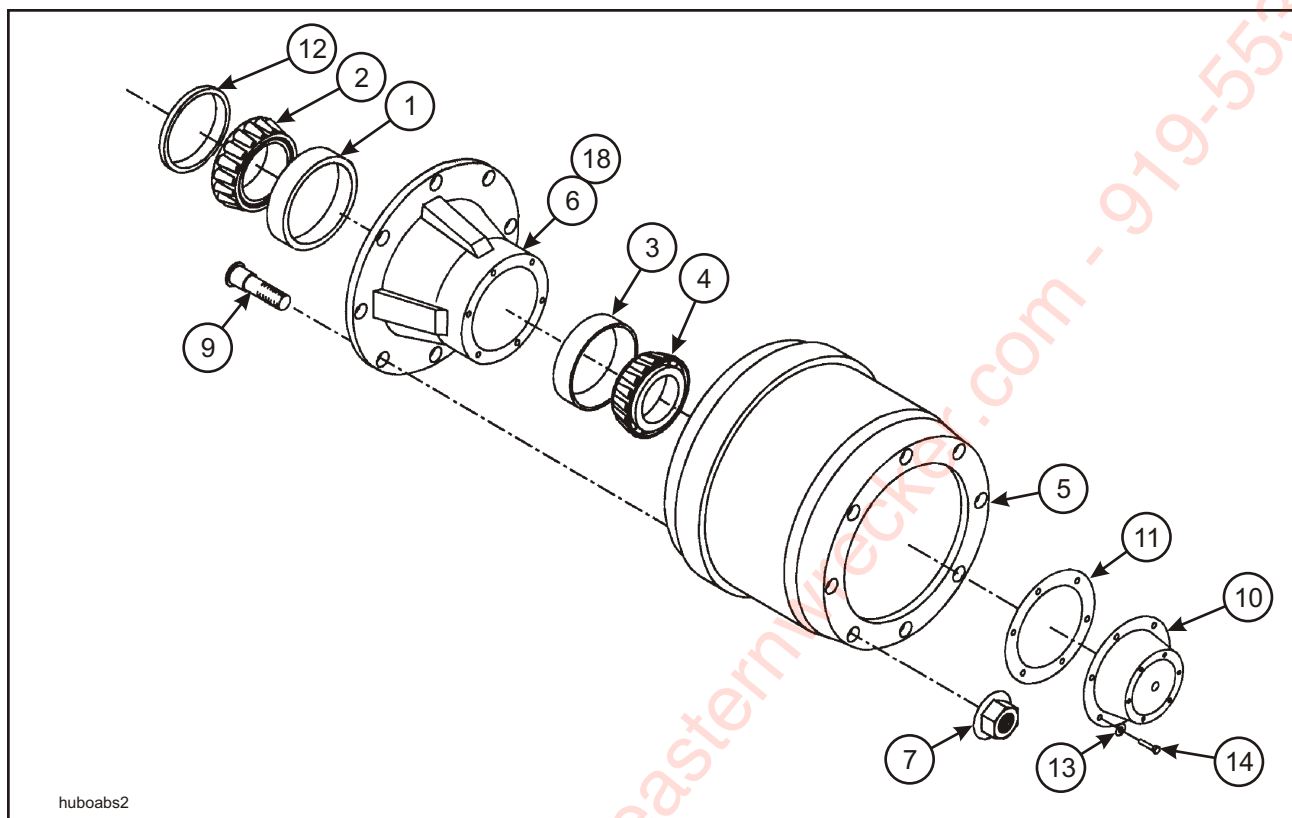
FIGURE 1-25 OUTBOARD PILOT MOUNT HUB AND DRUM
