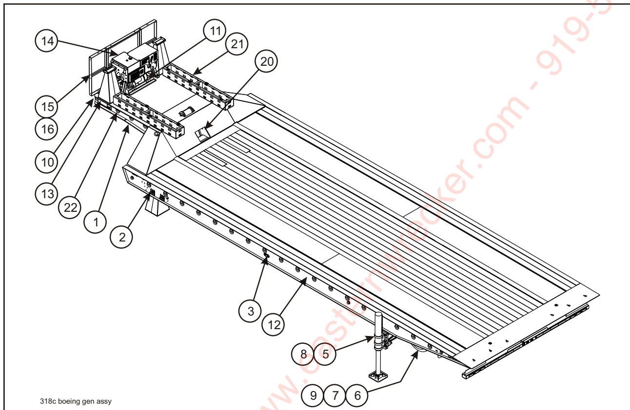
FIGURE 1-1 GENERAL ASSEMBLY
