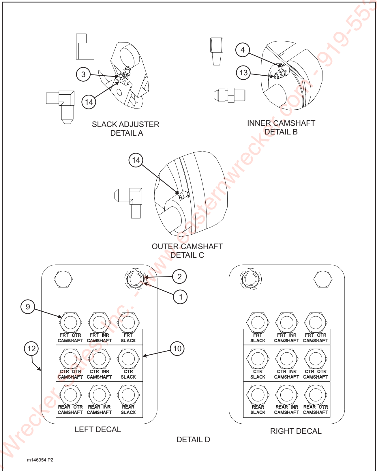
Figure 1-20 Grease System - Triple Axle (325C, 327C, 329C)
