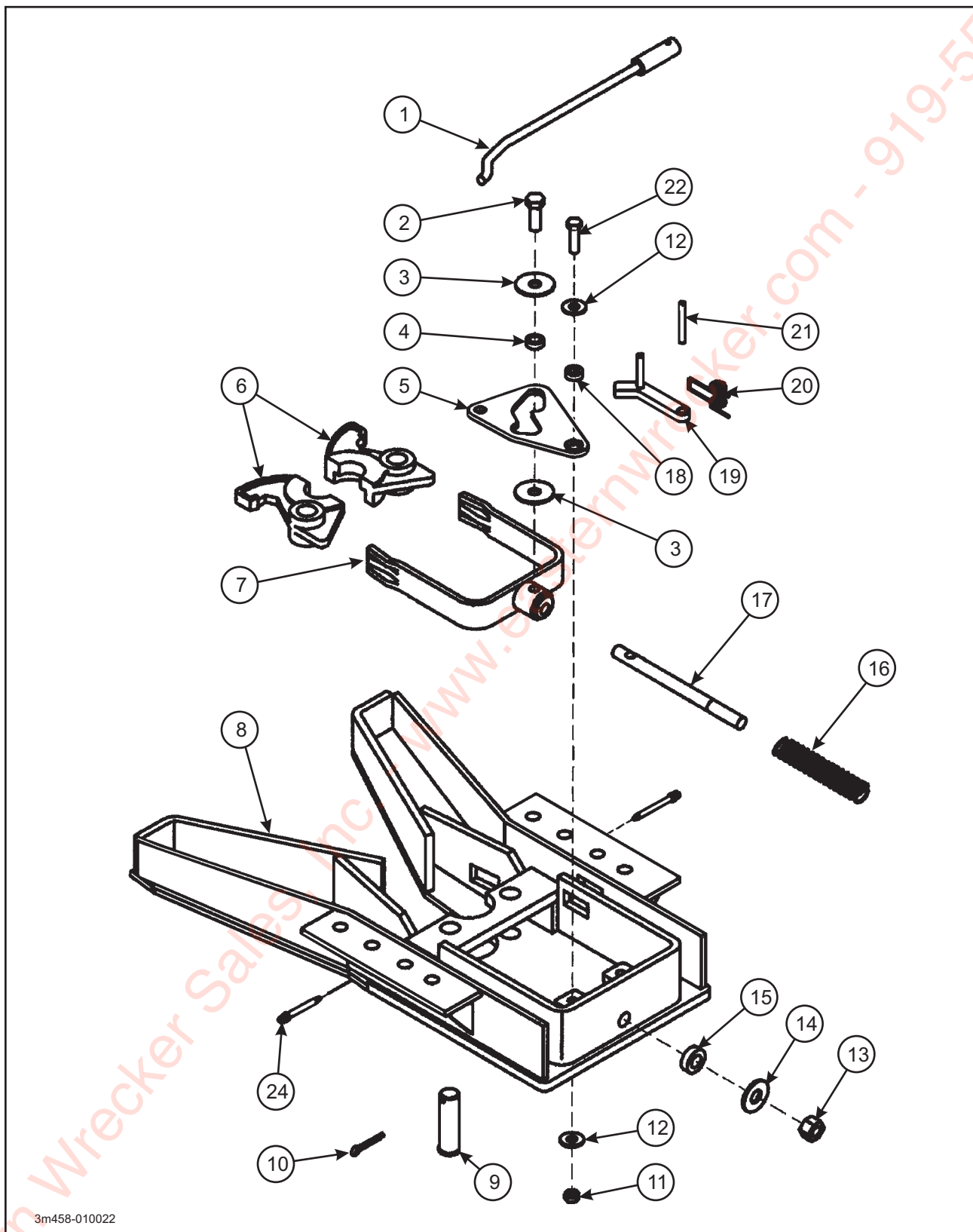
Figure 1-21 Lock Assembly
