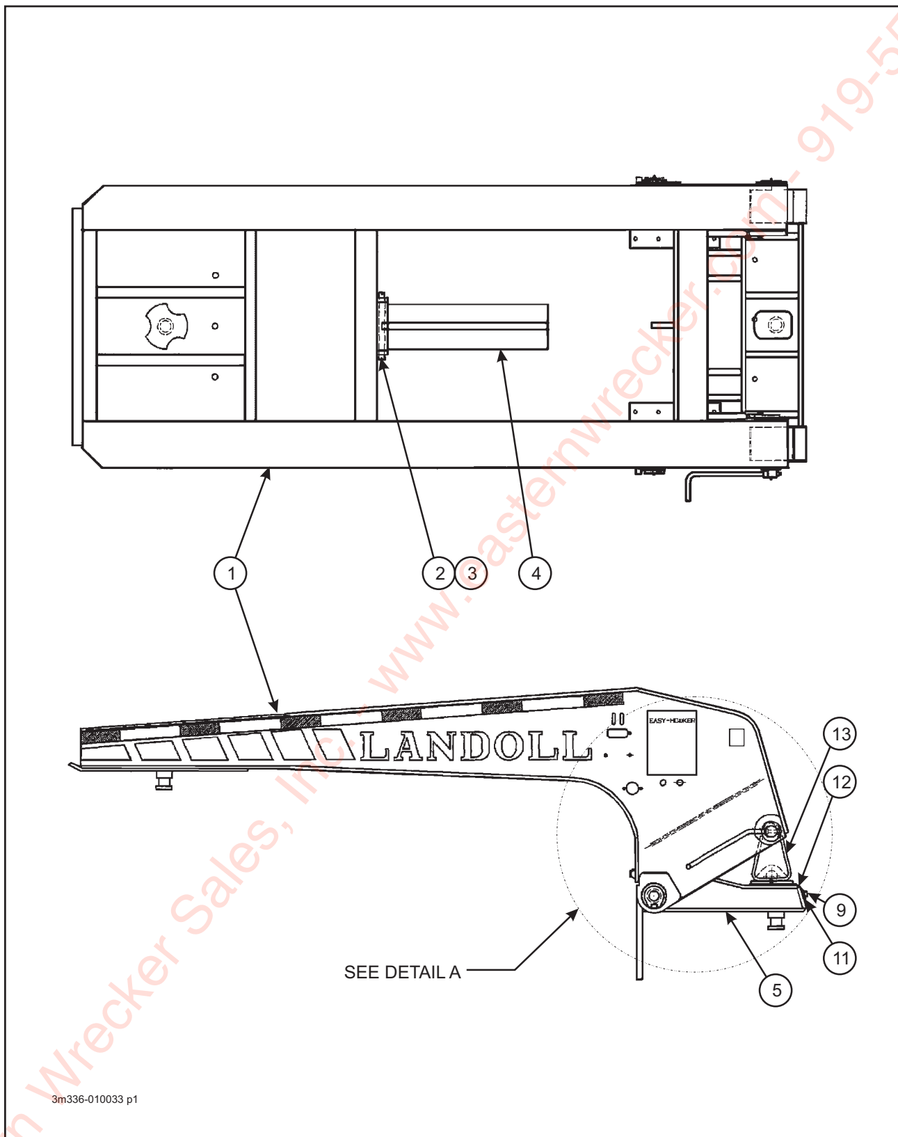
Figure 1-2 Gooseneck Assembly (1 of 5)
