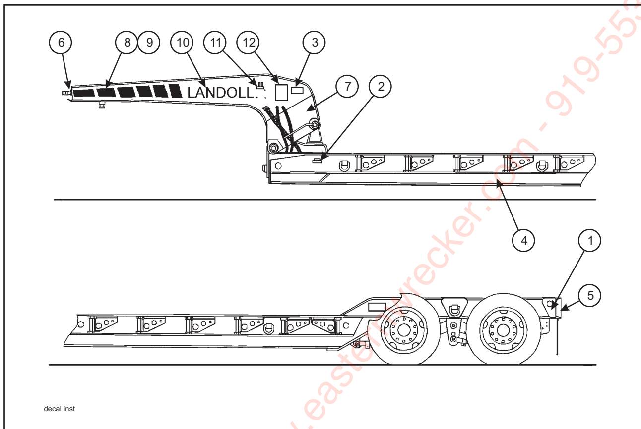
Figure 1-44 Decal Placement
