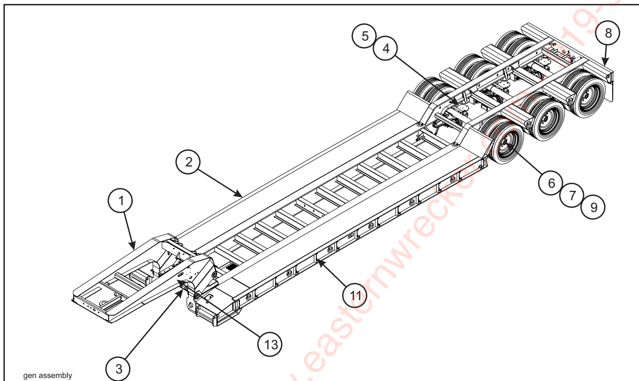
Figure 1-1 General Assembly
