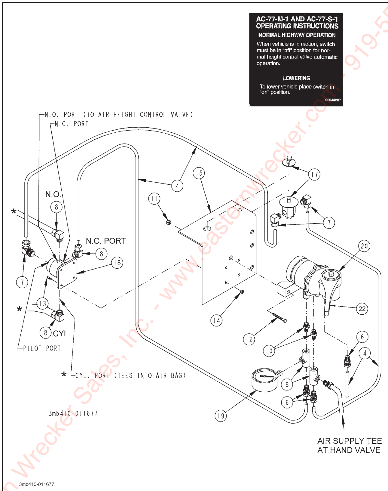
Figure 1-25 Manual Air Height Control Assembly (Option)
