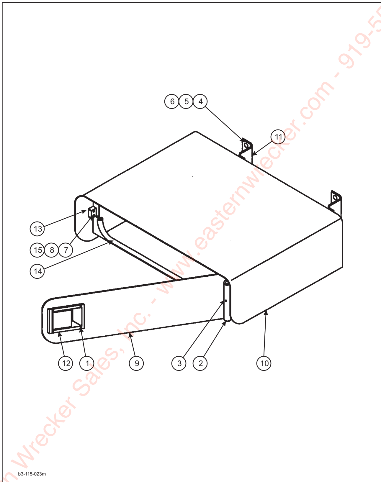
Figure 1-53 Toolbox and Mounting Installation
