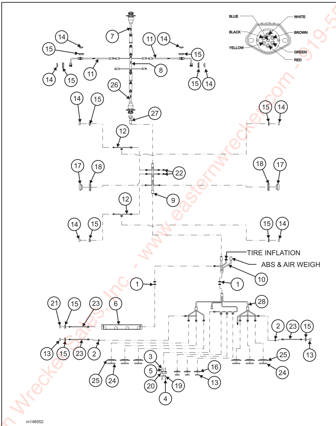
Figure 1-33 Electrical System
