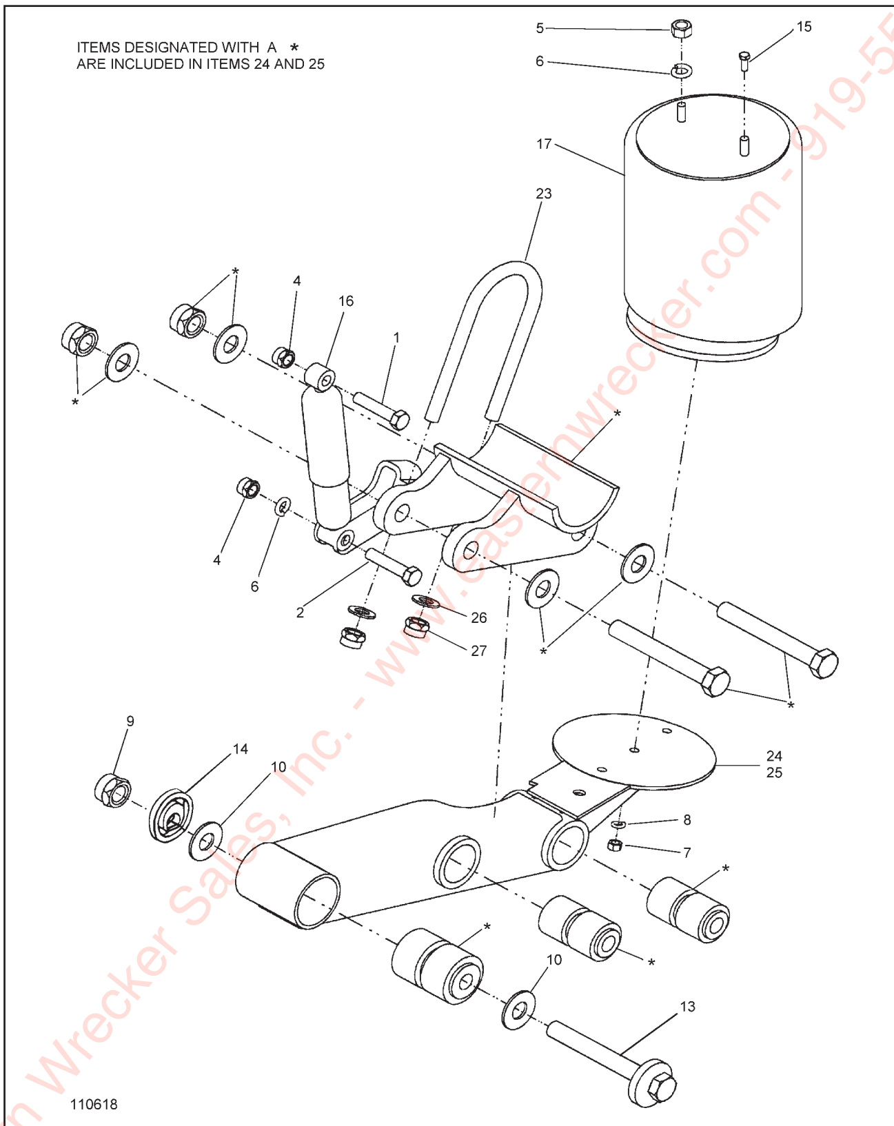
Figure 1-28 Suspension, Fastener RLU-250-9-4
