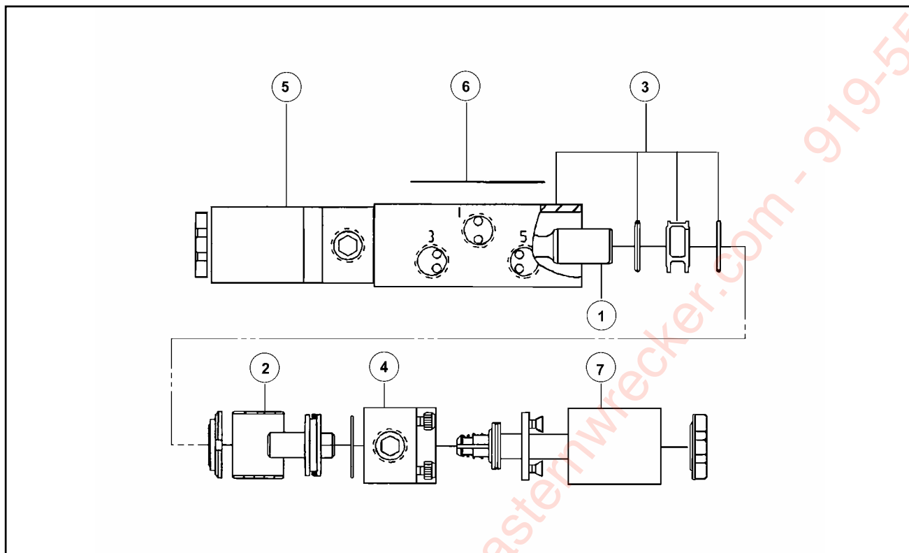
Figure 1-10 Pneumatic Valve
