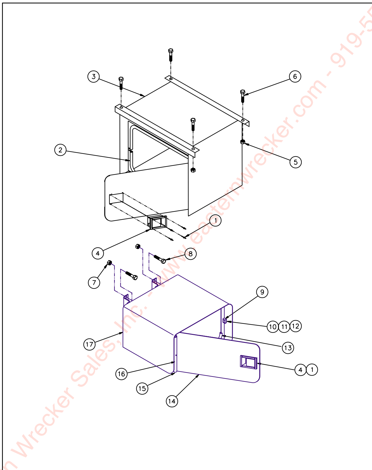
Figure 1-47 Tool Boxes
