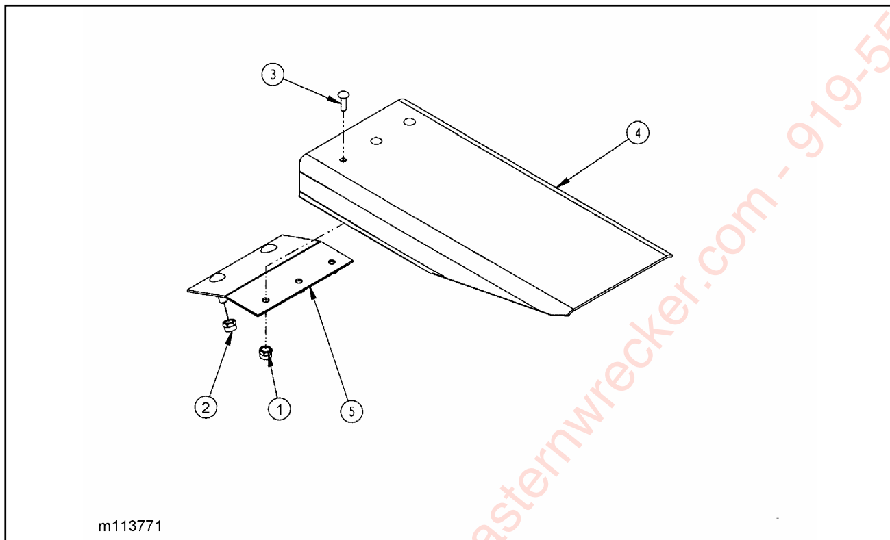
Figure 1-54 Aluminum Ramps (Option)
