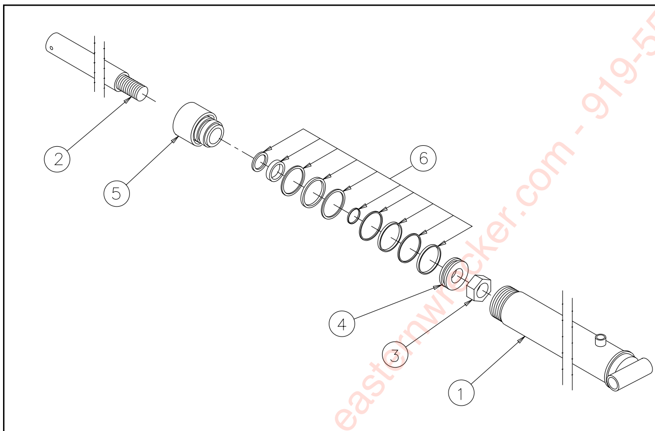
Figure 1-6 Trailer Tilt Cylinder Assembly
