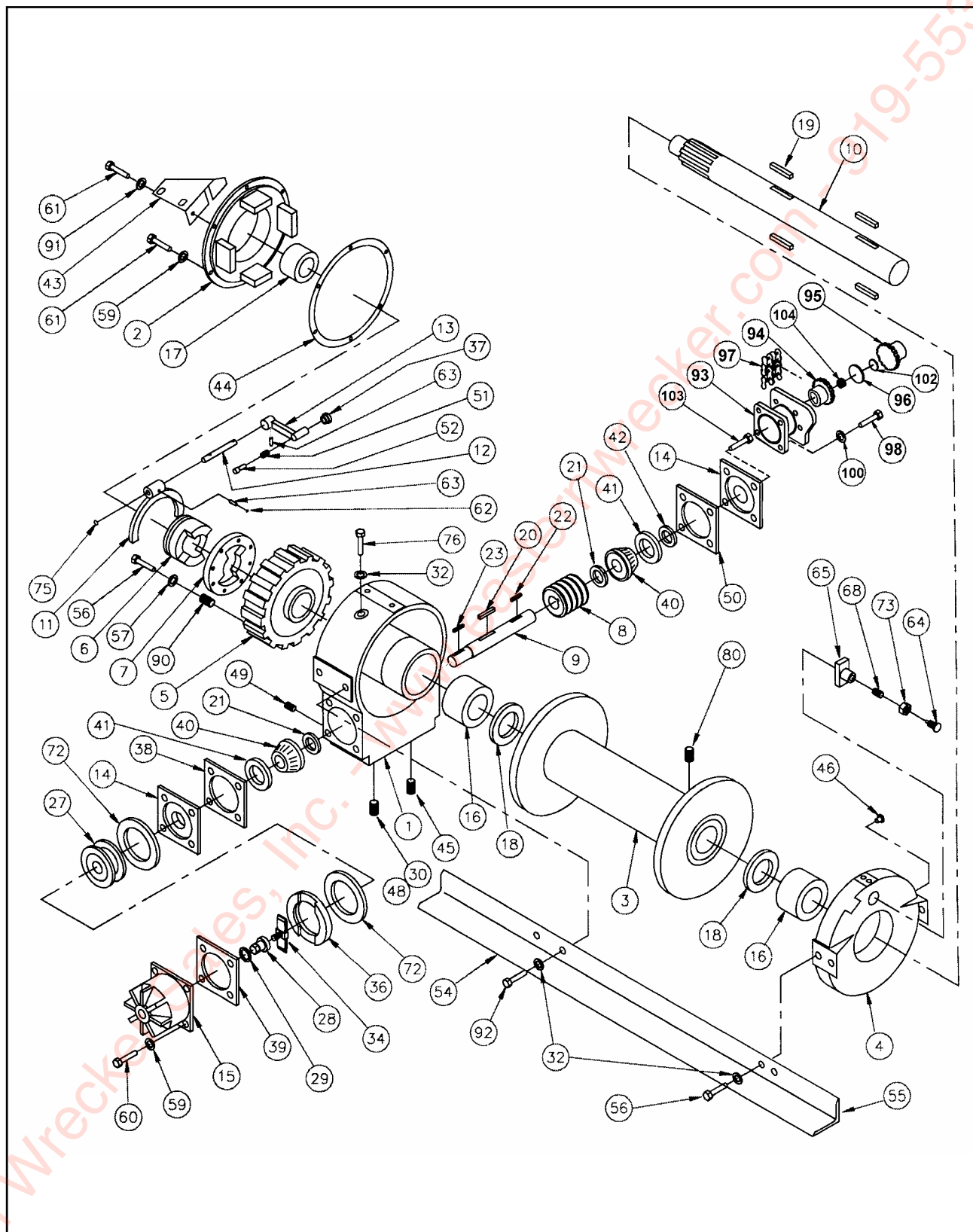
Figure 1-33 20,000# Winch Assembly
