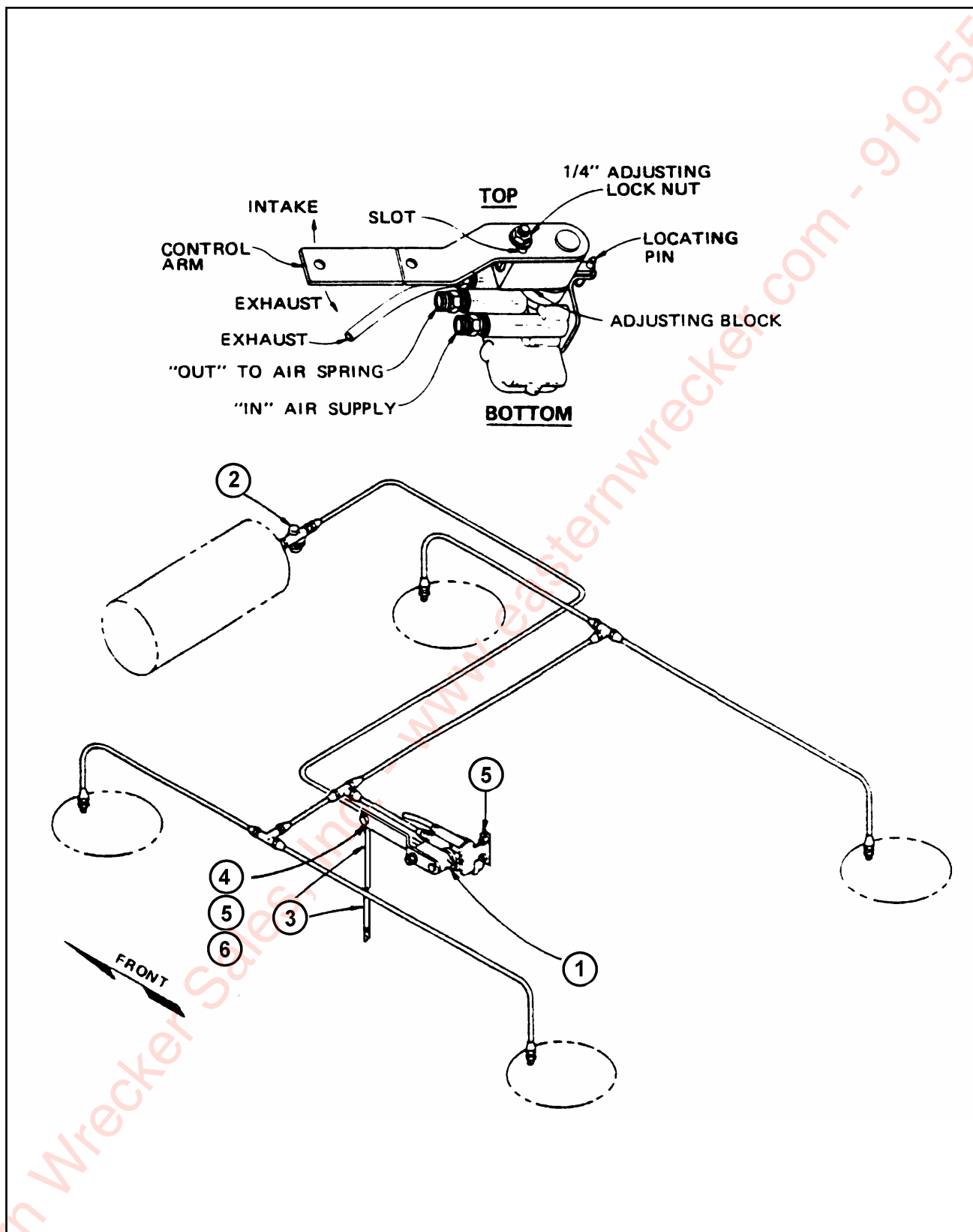
Figure 1-23 Air Control Kit
