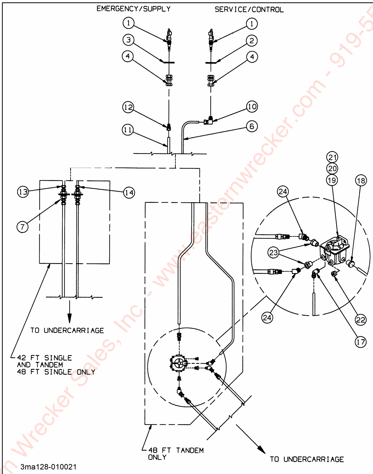
Figure 1-30 Air System
