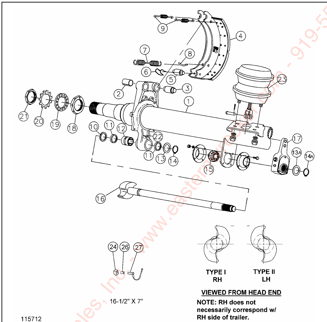
Figure 1-25 Axle and Brake Items
