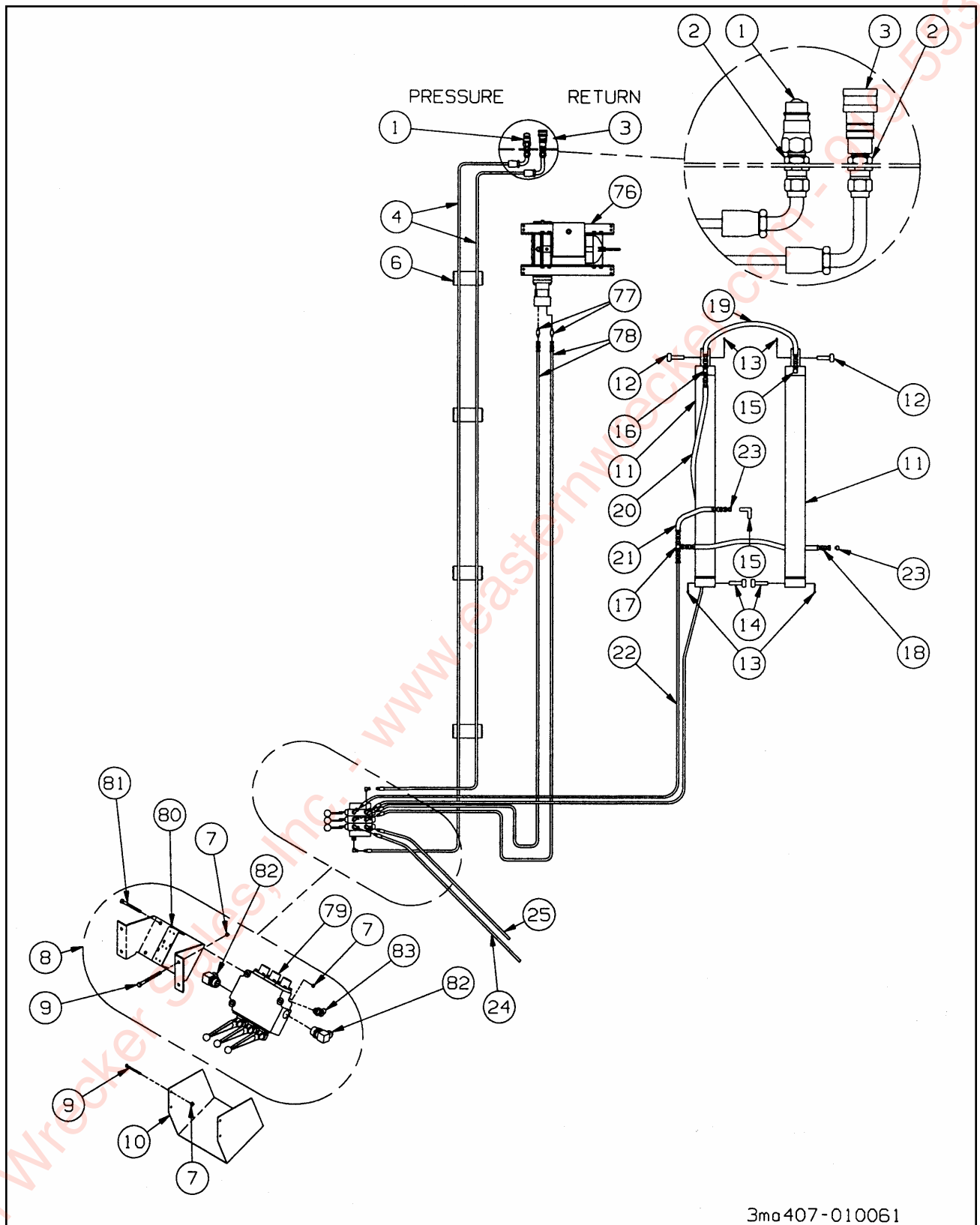
Figure 1-3 Hydraulic System
