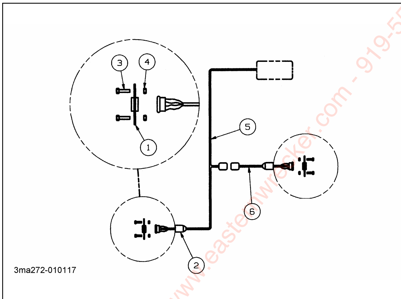
Figure 1-14 Electrical System Rear/Curb Remote
