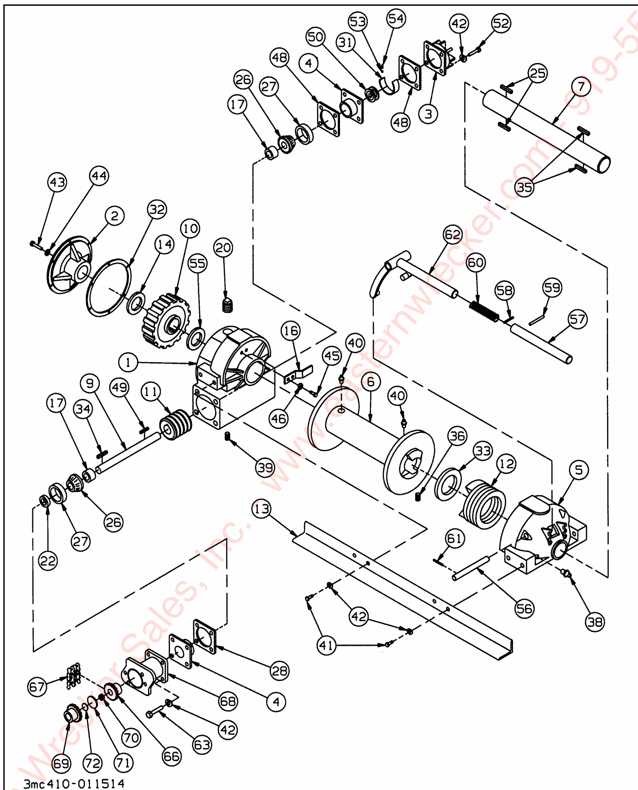
Figure 1-32 12,000# Winch Assembly
