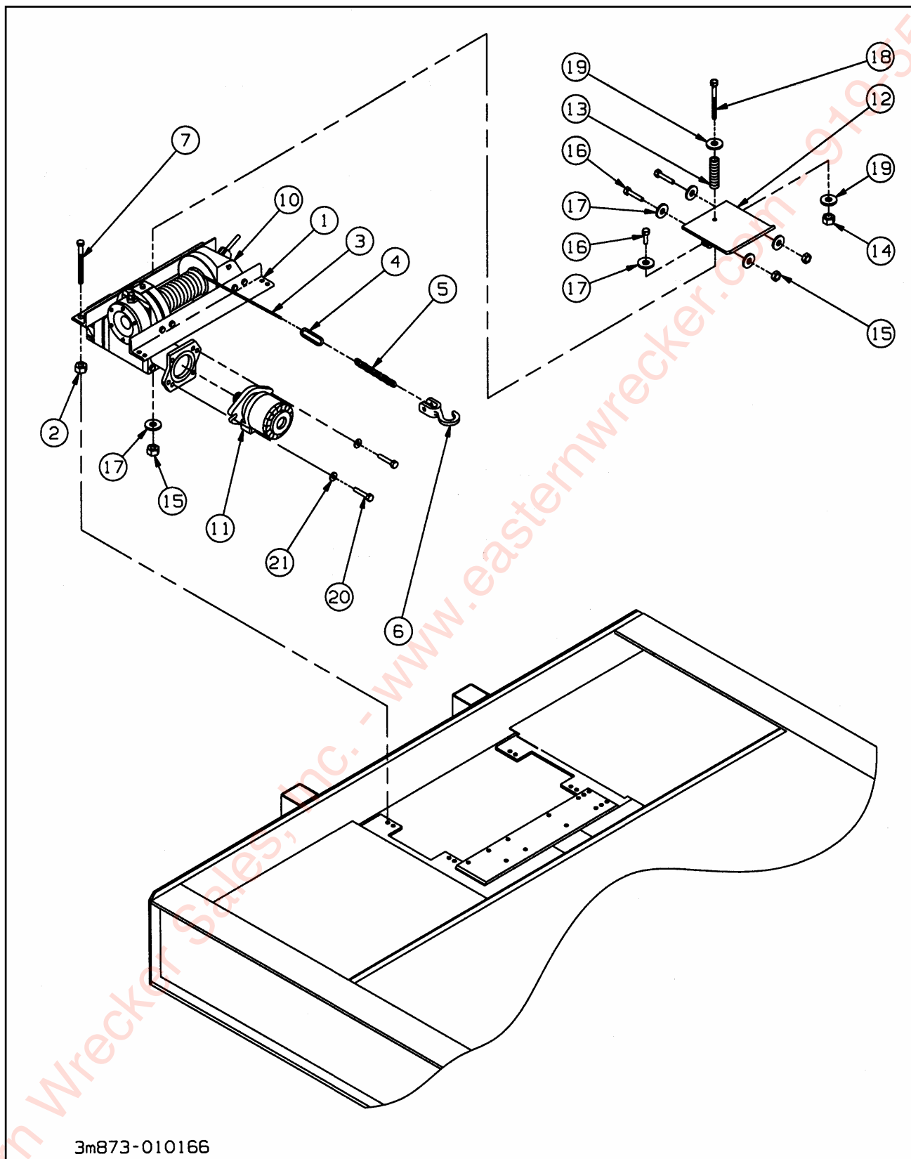
Figure 1-31 Winch Installation
