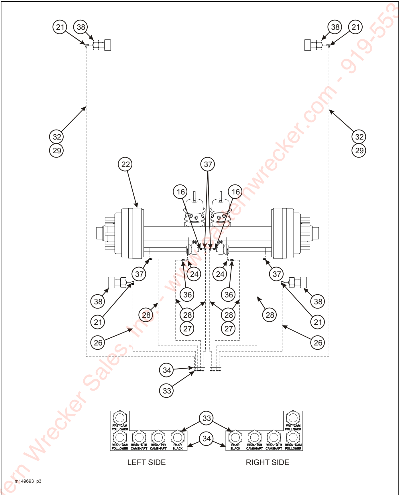
Figure 2-23: Grease System - Single
