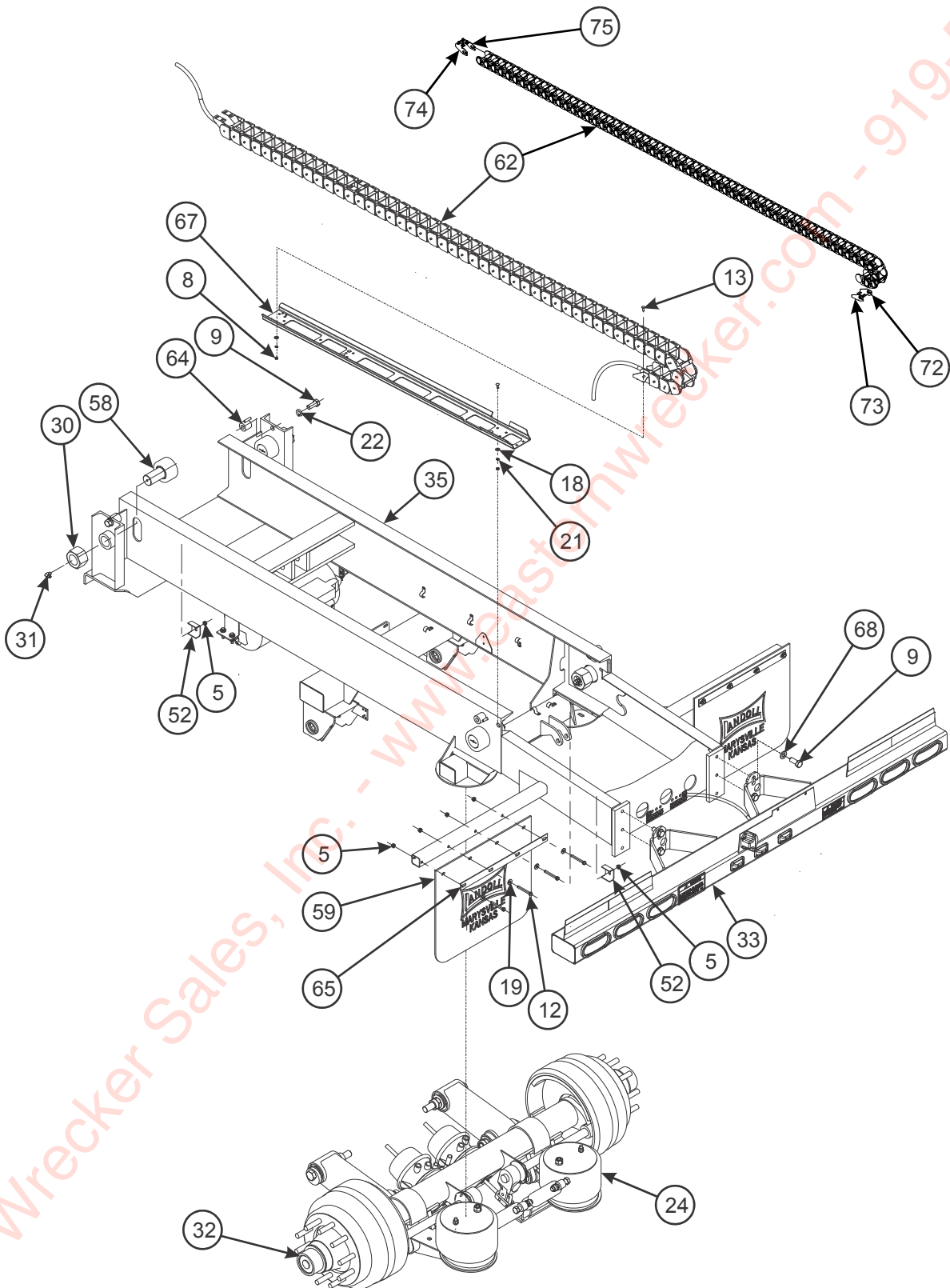
Figure 2-26: Undercarriage Assembly, Air Ride Single Axle
