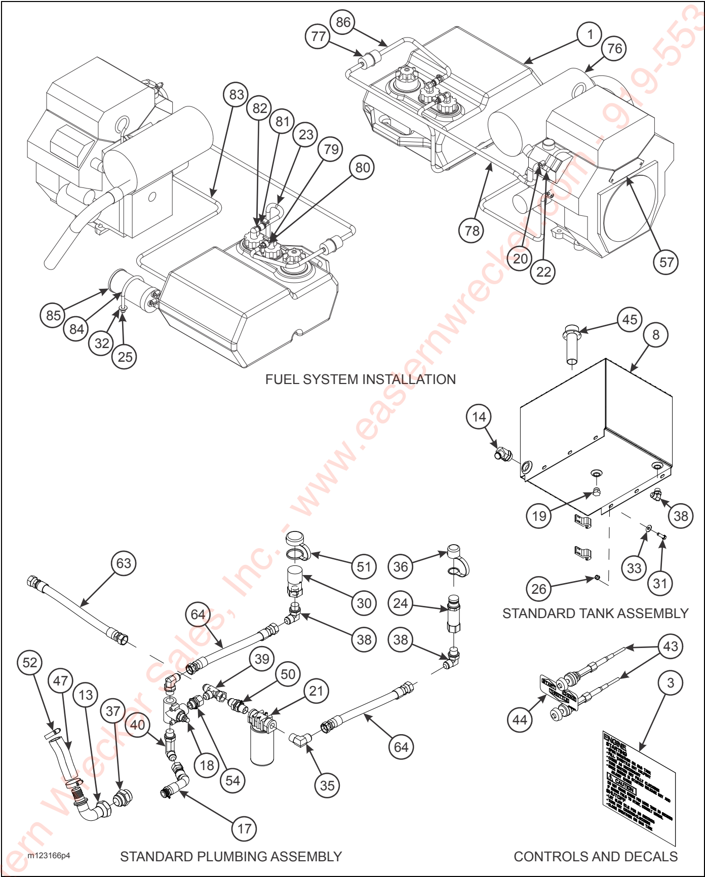
Figure 2-53: Engine Package, Front Mount (4 of 4)
