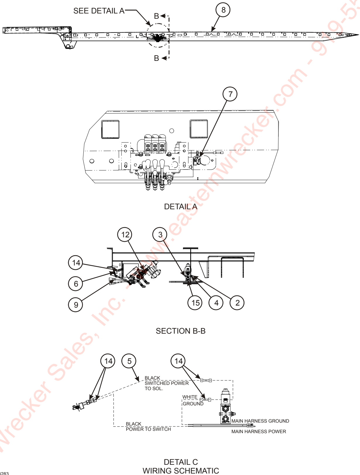
Figure 2-60: Hydraulic Bypass for 2 Hand Control (Option)
