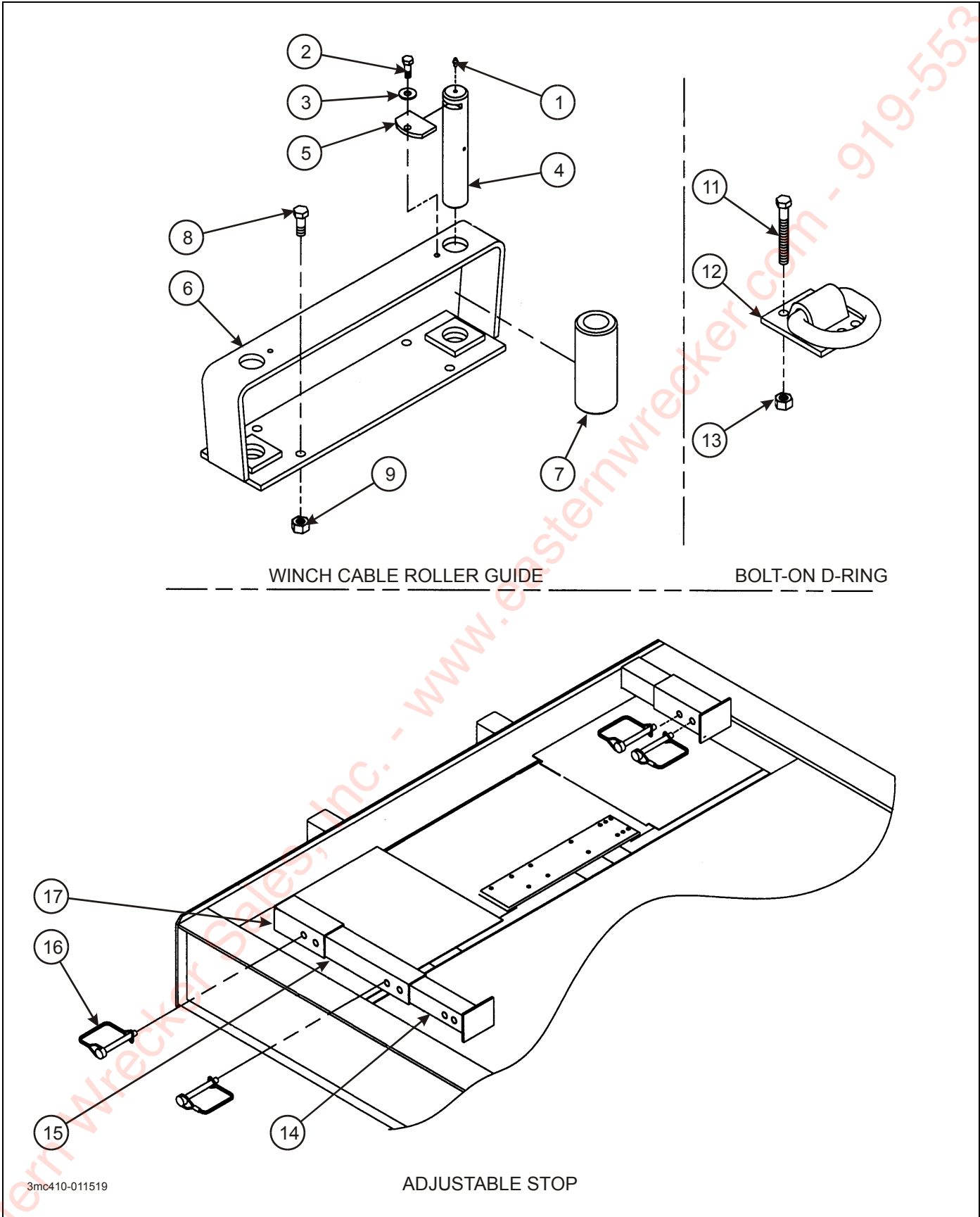
Figure 2-48: Winch Cable Roller Guide (Option)
