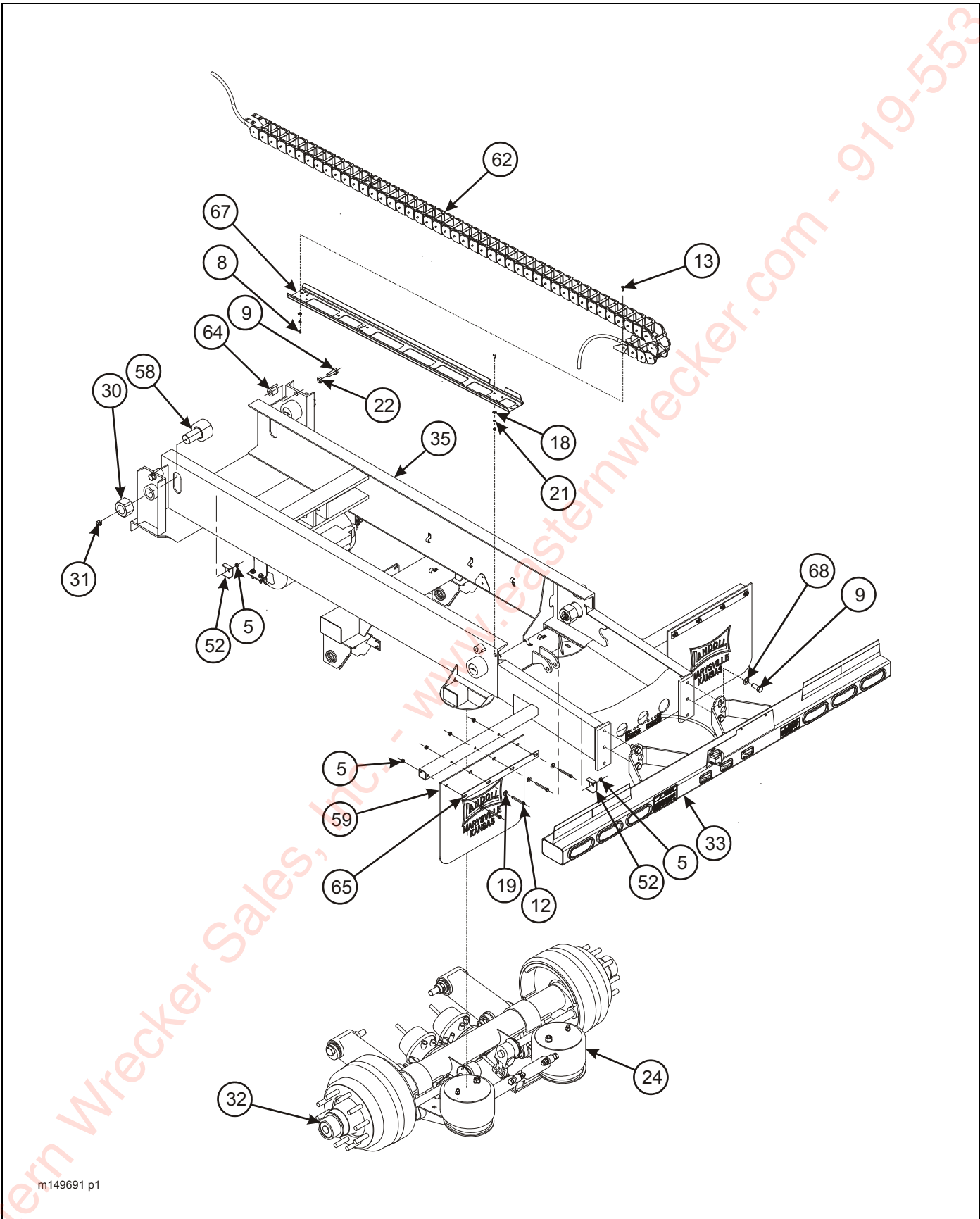
Figure 2-26: Undercarriage Assembly, Air Ride Single Axle
