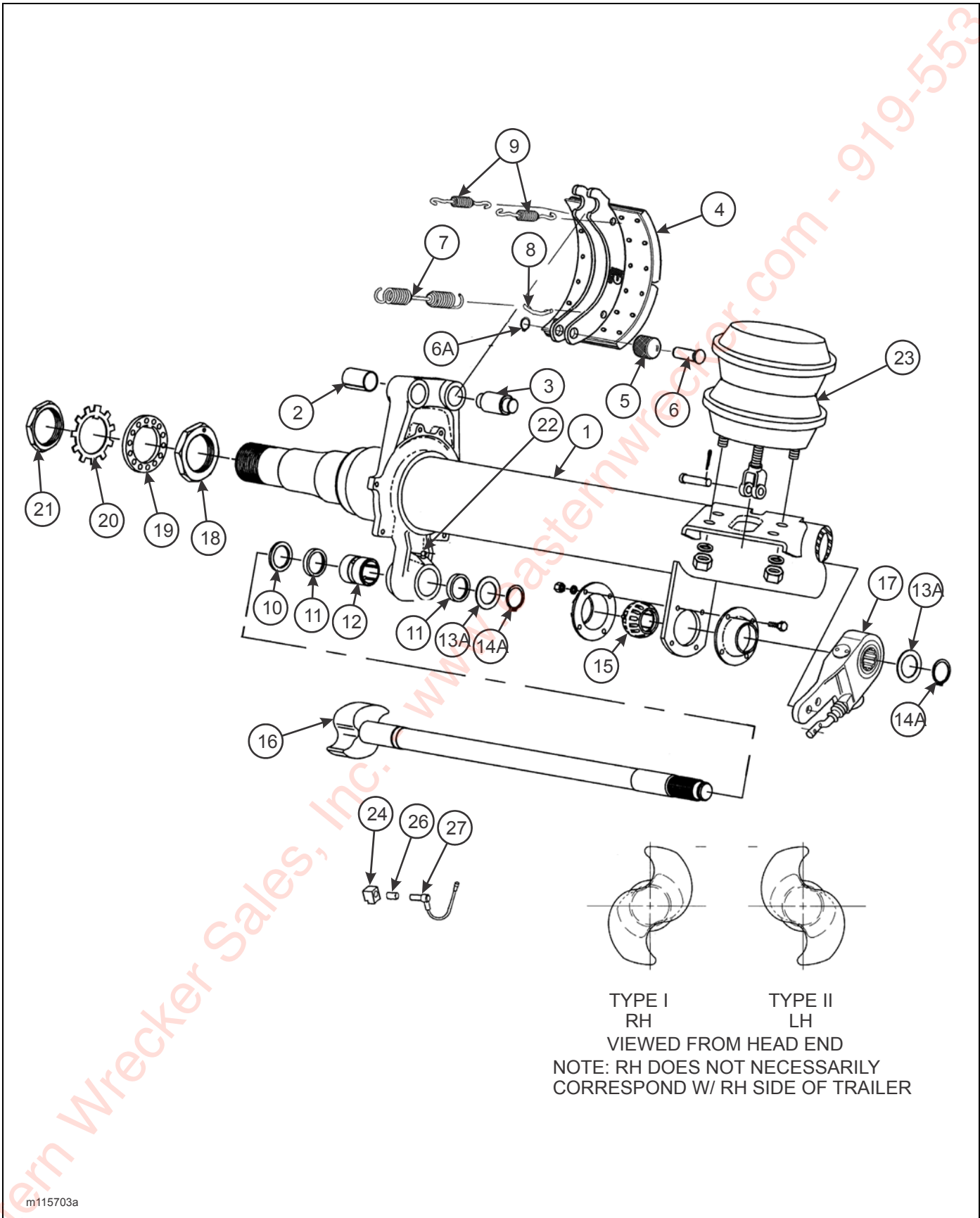
Figure 2-34: Axle and Brake Assembly (12-1/4 x 7-1/2")
