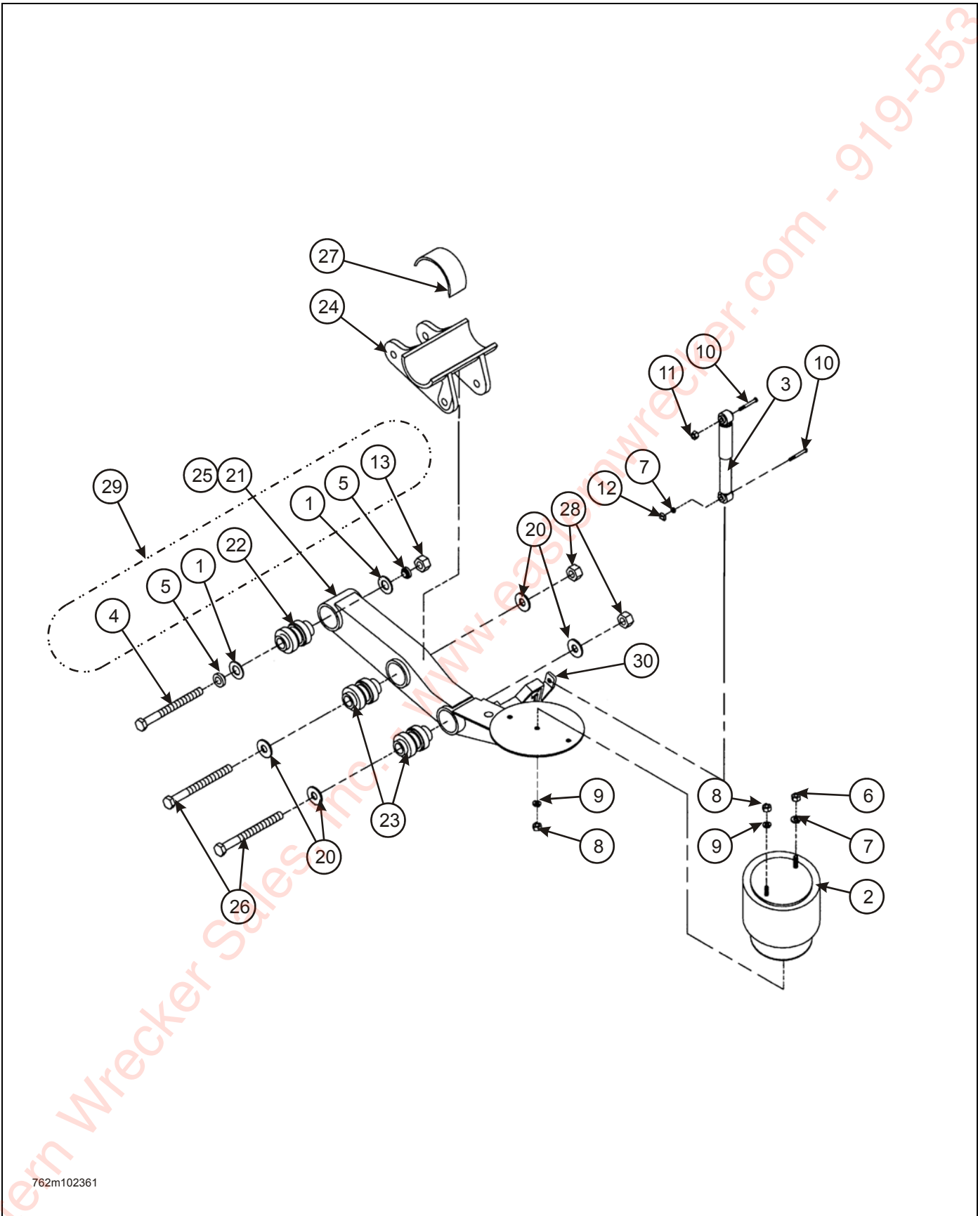
Figure 2-33: Suspension Air Ride Assembly
