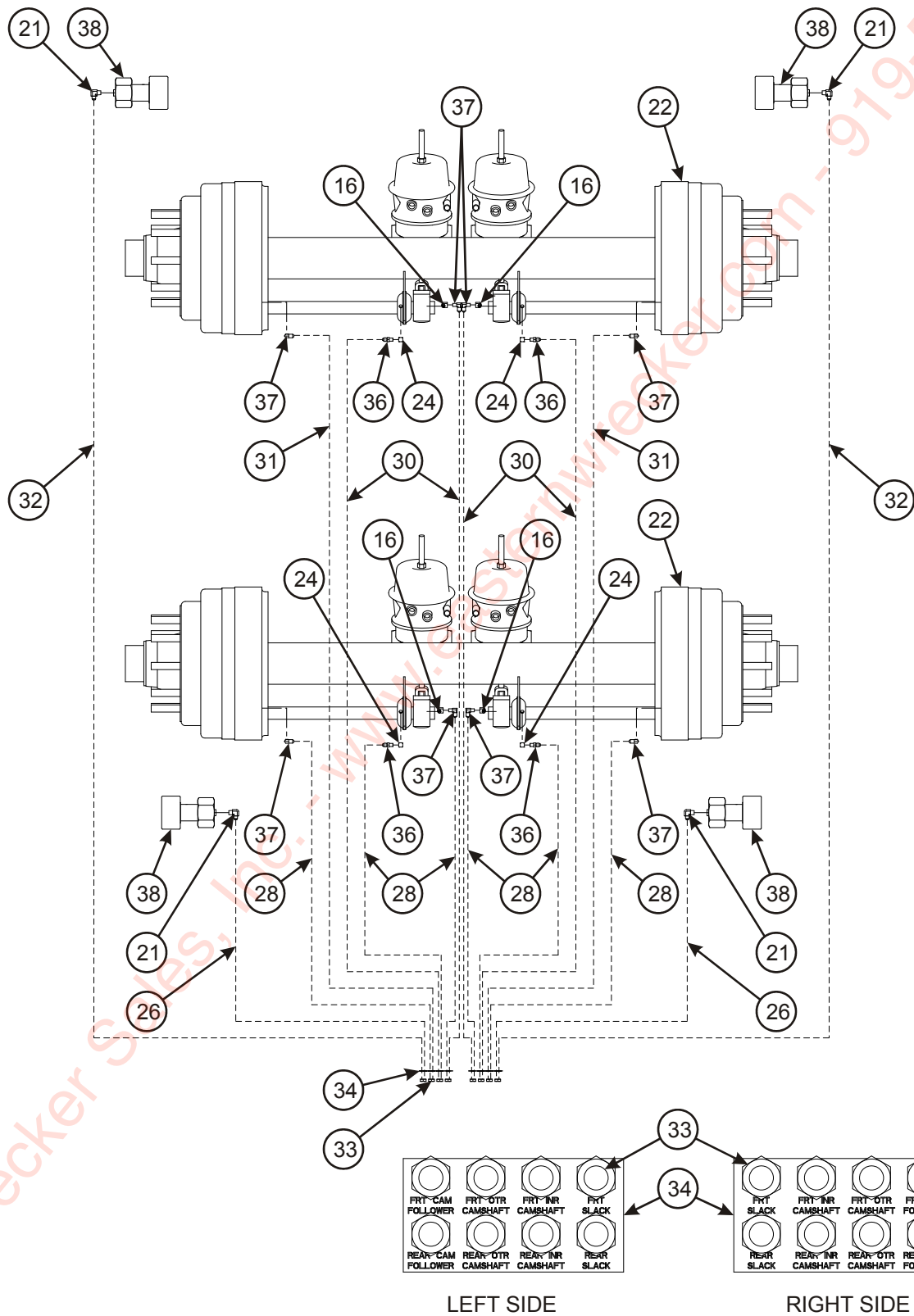
Figure 2-24: Grease System - Tandem
