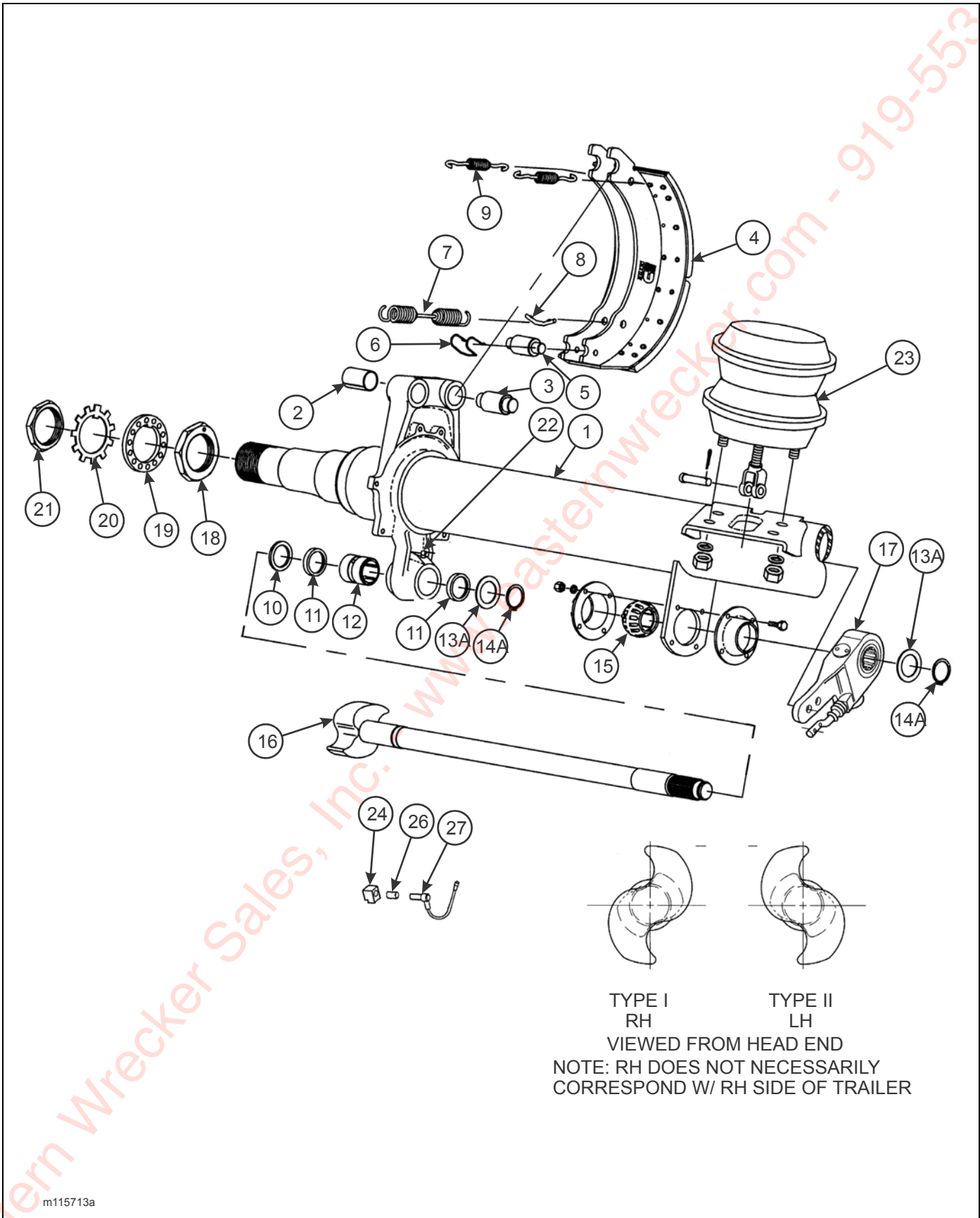
Figure 2-35: Axle and Brake Assembly (16-1/2" x 7")
