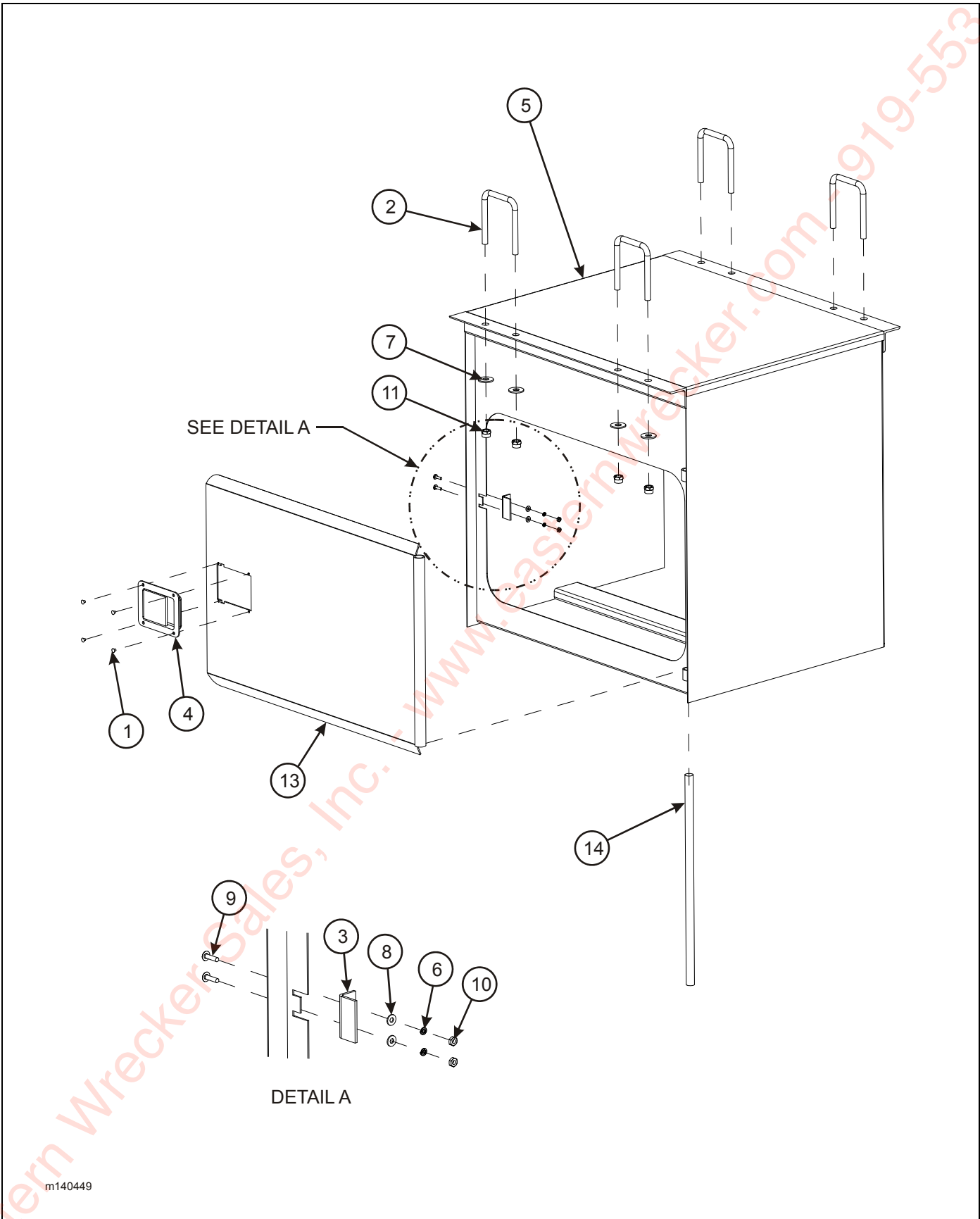
Figure 2-67: Top Mount Tool Box (Option)
