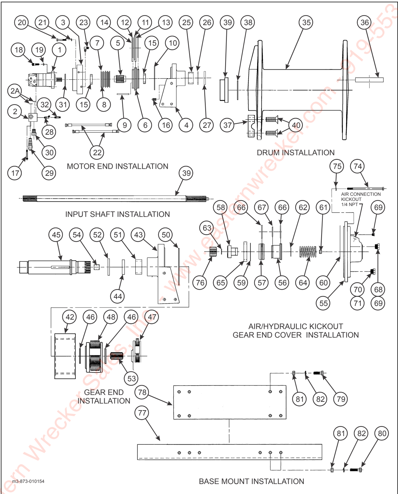
Figure 2-47: 30,000 Lb. Winch Items
