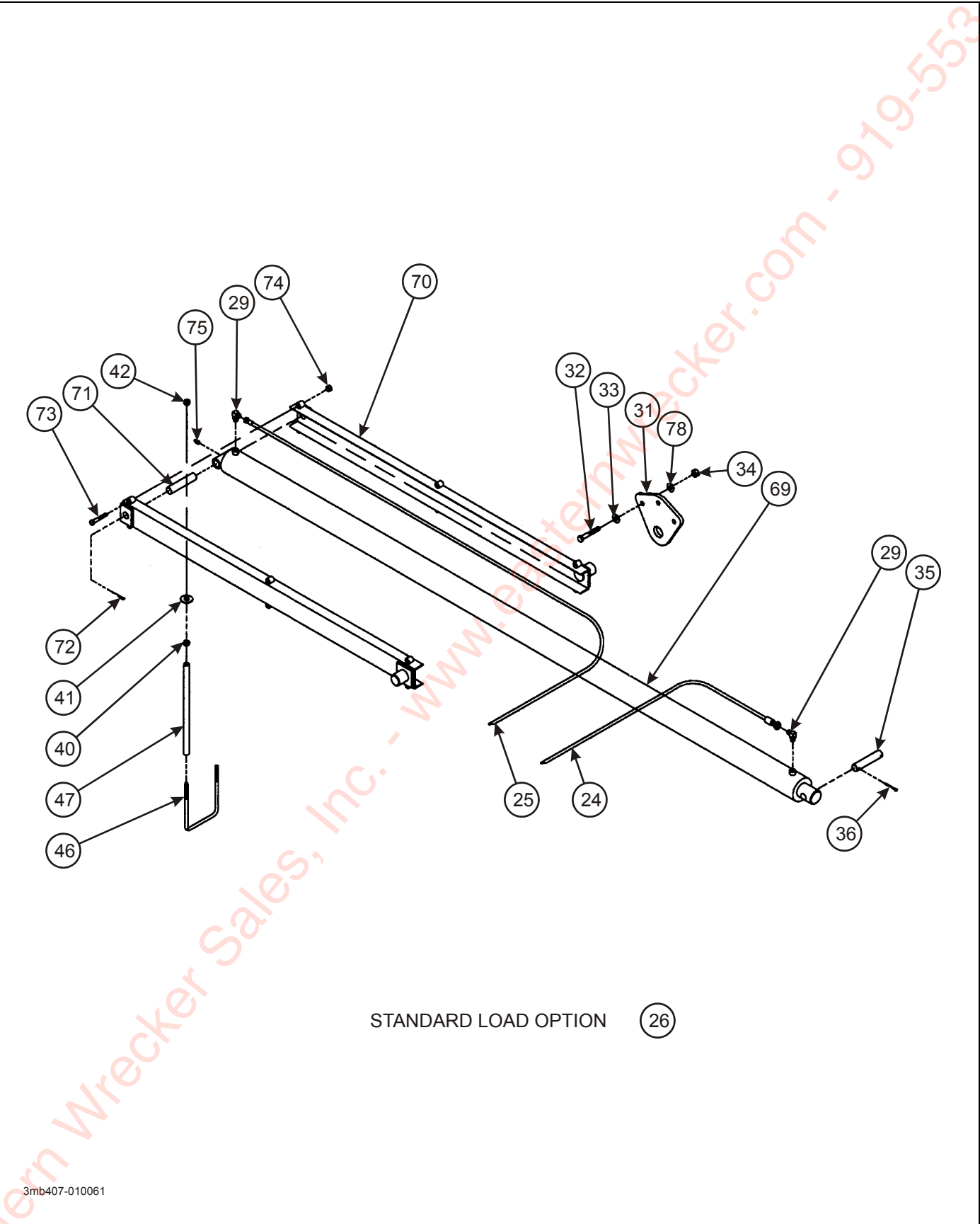
Figure 2-7: Hydraulic System, Standard Load Angle Option (2 of 3)
