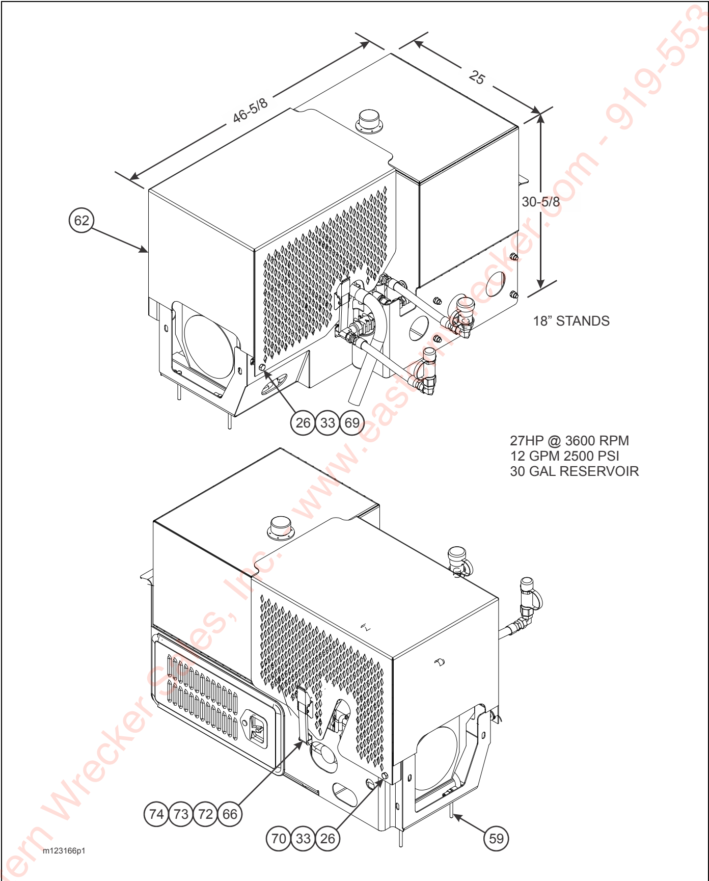
Figure 2-60: Engine Package, Front Mount (1 of 4)
