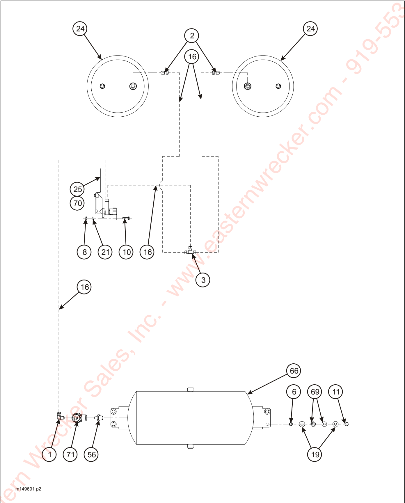
Figure 2-28: Air Ride Suspension System, Single Axle
