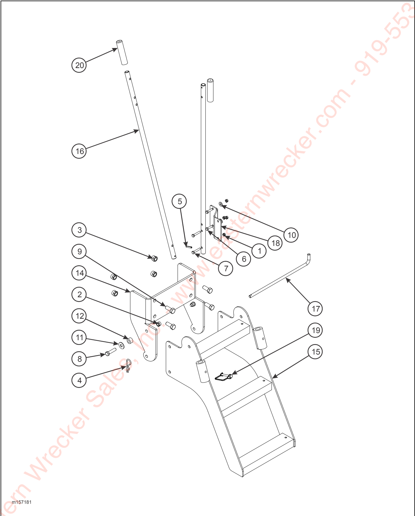
Figure 2-70: Ladder Assembly, Stor-Away (Option)
