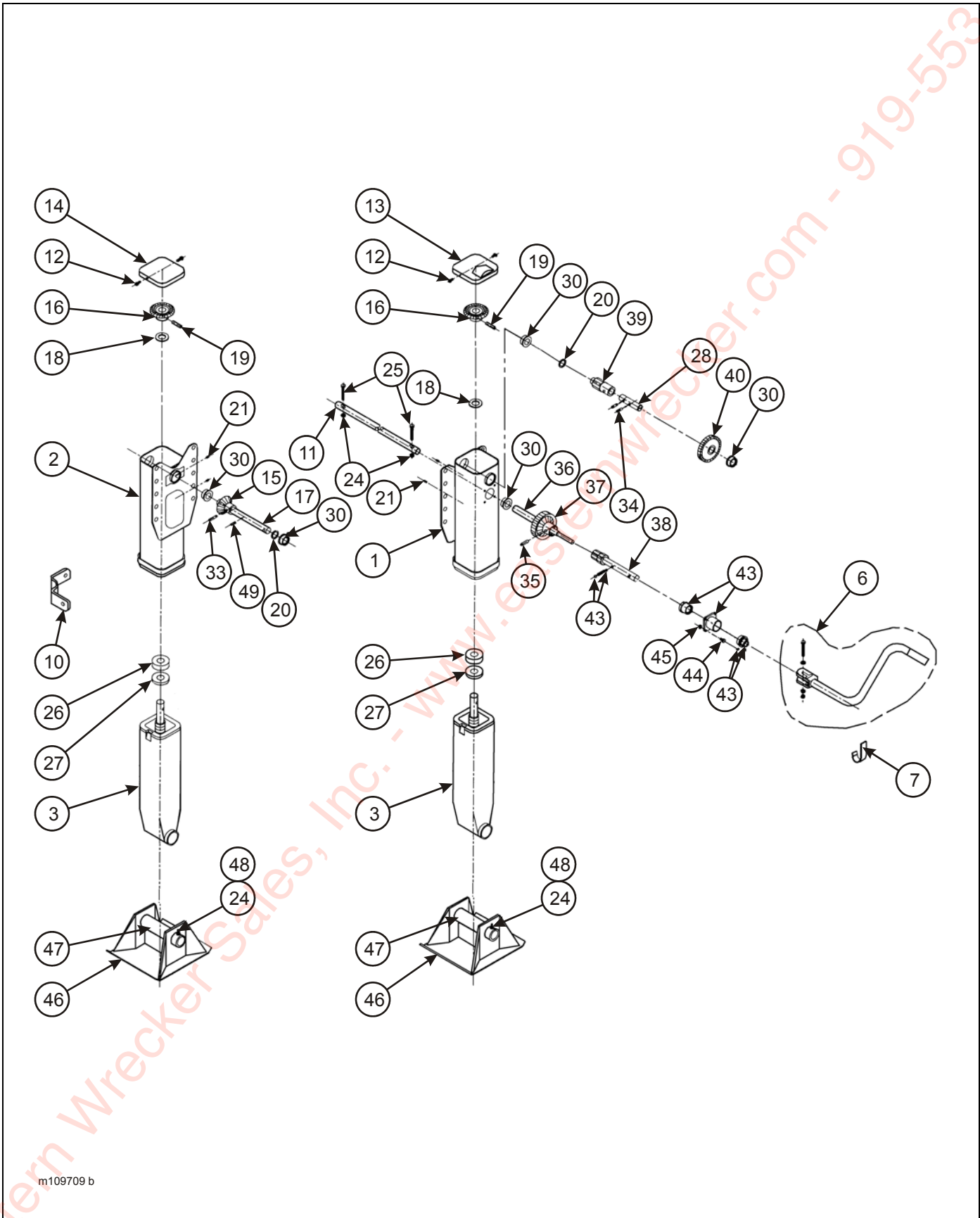
Figure 2-55: Crank Landing Gear
