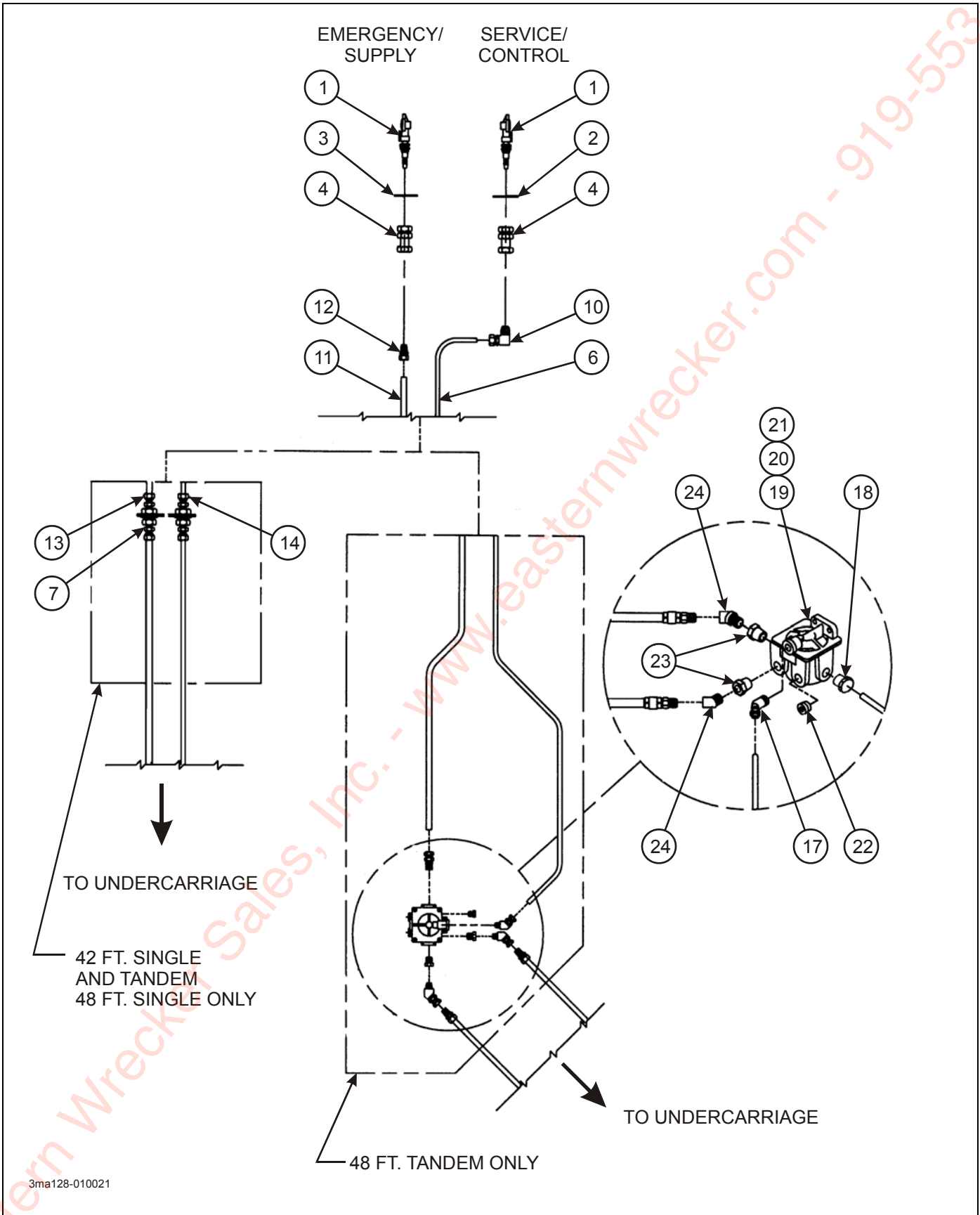
Figure 2-16: Air System
