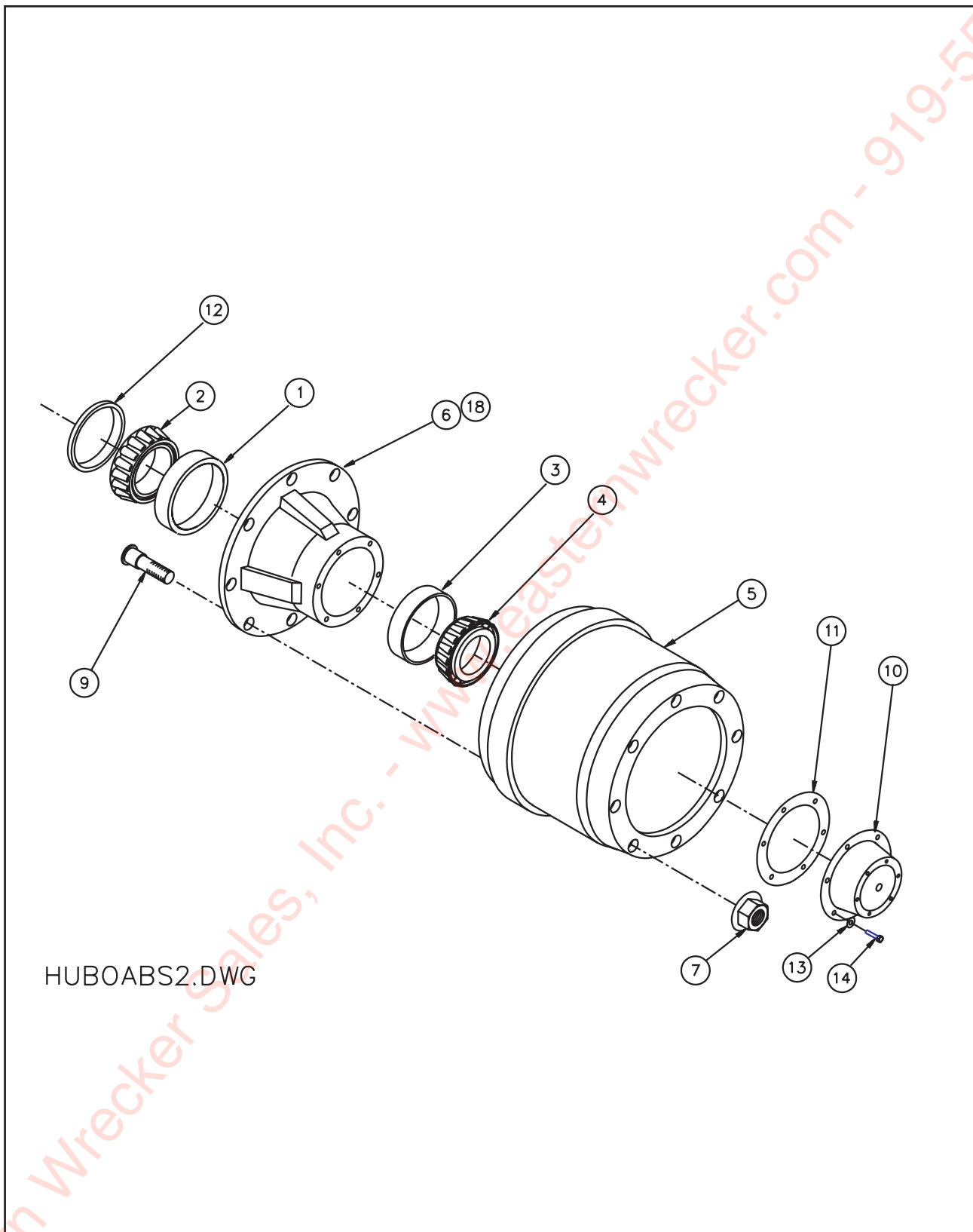
Figure 1-30 Outboard Pilot Mount Hub and Drum
