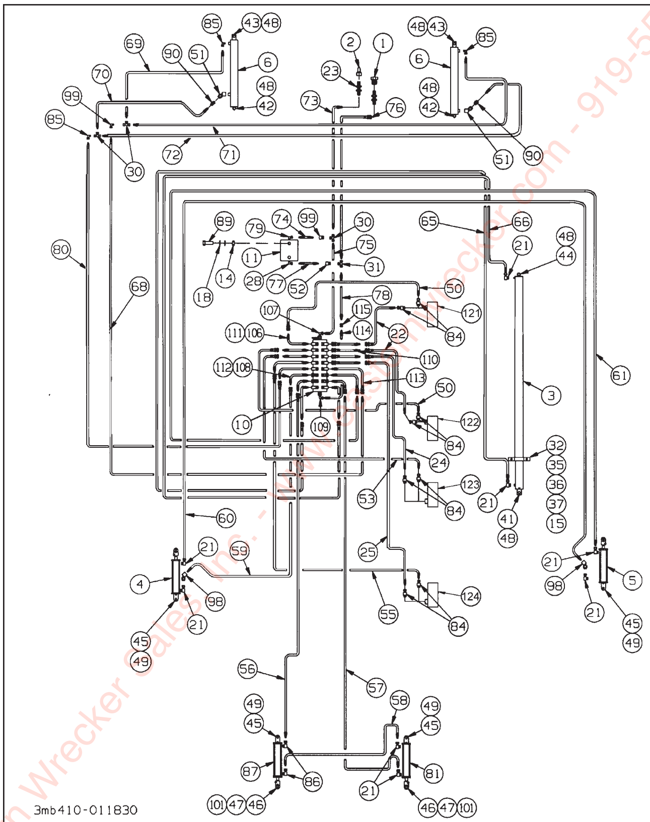
Figure 1-9 Hydraulic System
