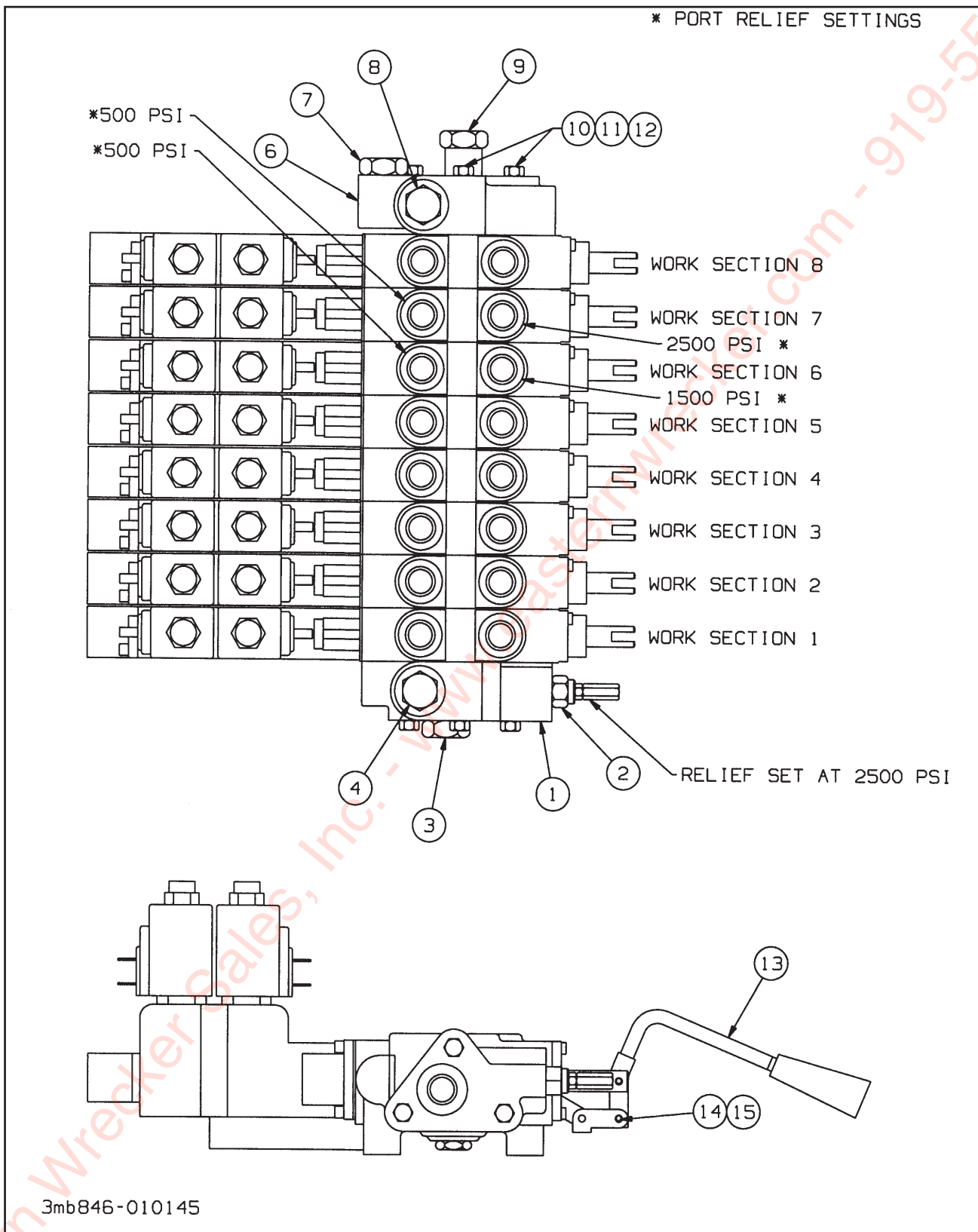
Figure 1-15 Eight Spool Valve
