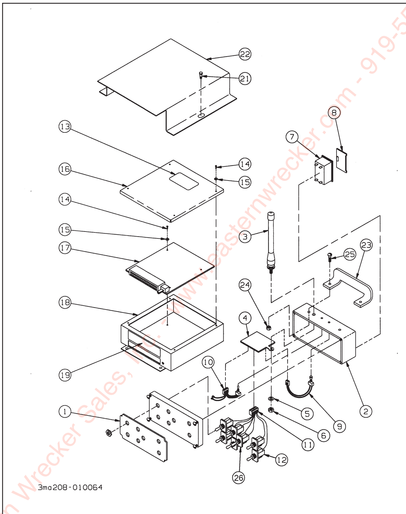
Figure 1-42 Remote Control
