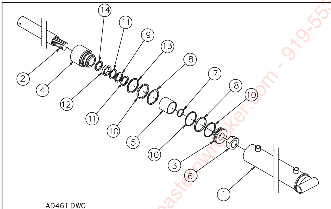
Figure 1-14 Hydraulic Cylinder Assembly, 4" x 126"
