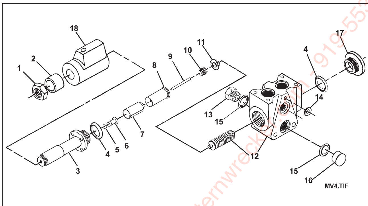
Figure 1-52 Hydraulic Solenoid Valve
