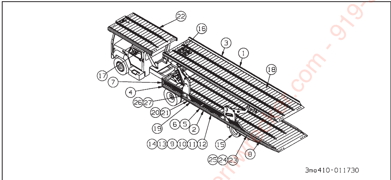
Figure 1-1 General Assembly
