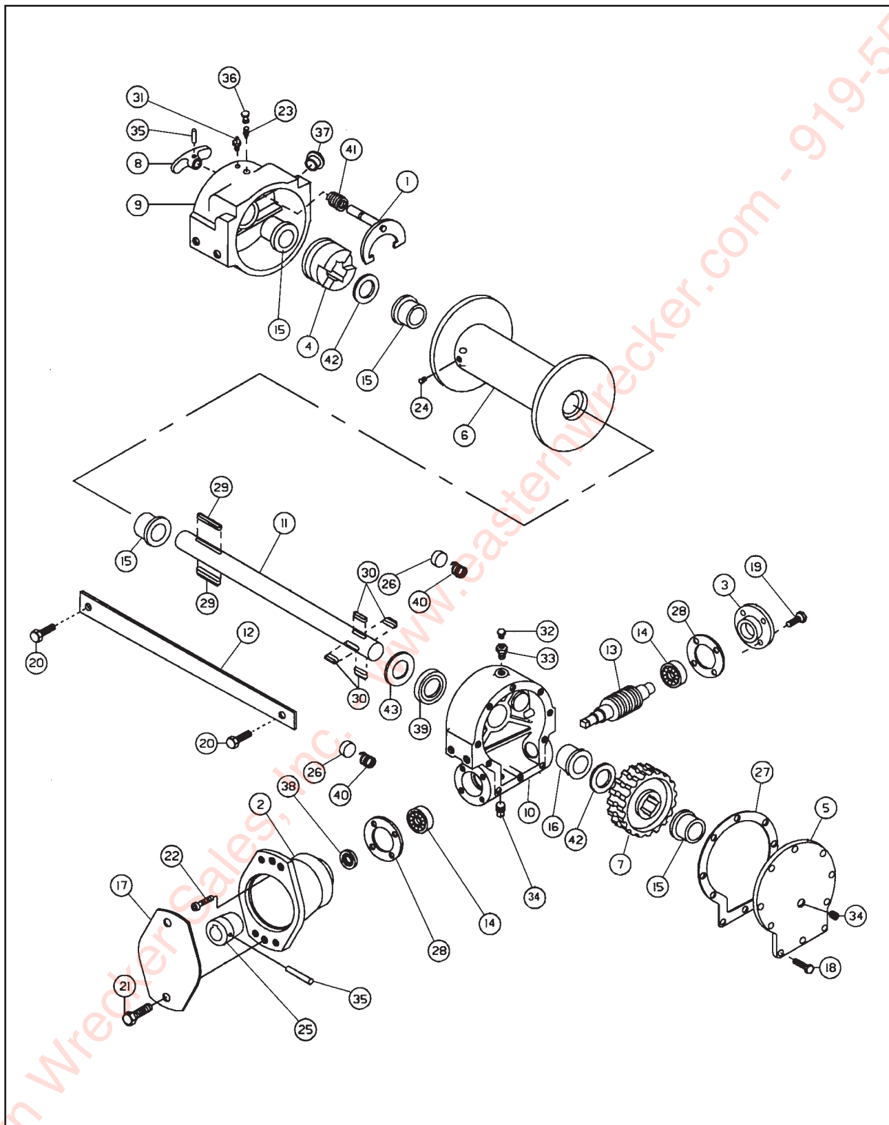
Figure 1-32 8,000# Winch Assembly
