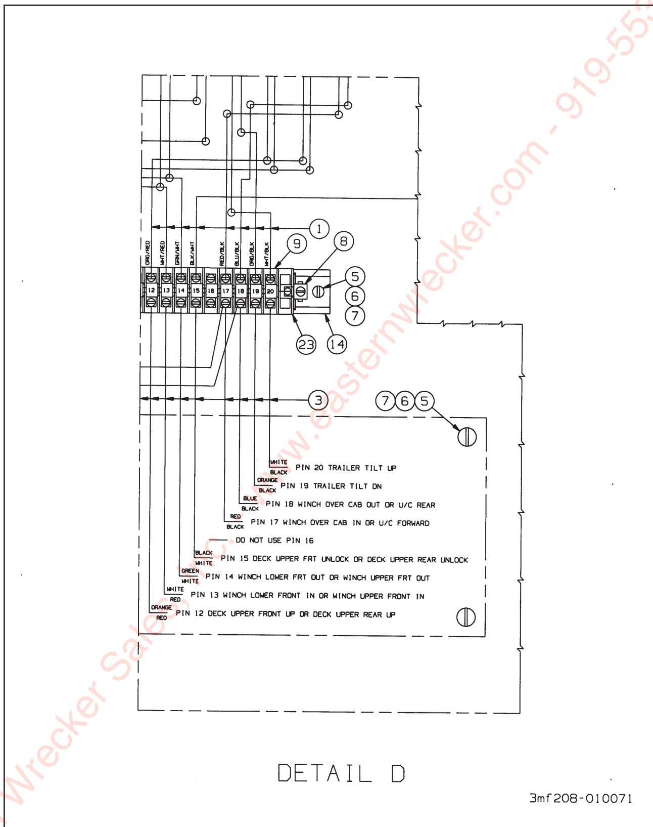
Figure 1-39 Electrical System, Remote Control Detail D
