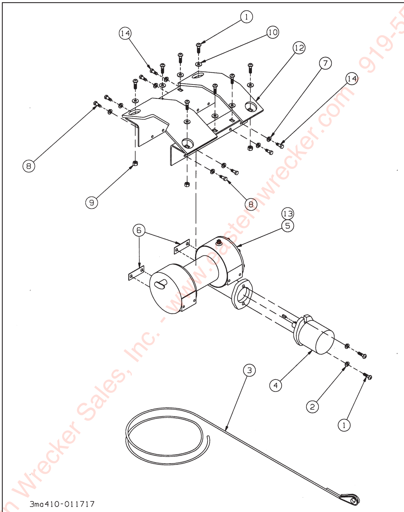
Figure 1-31 Winch Installation
