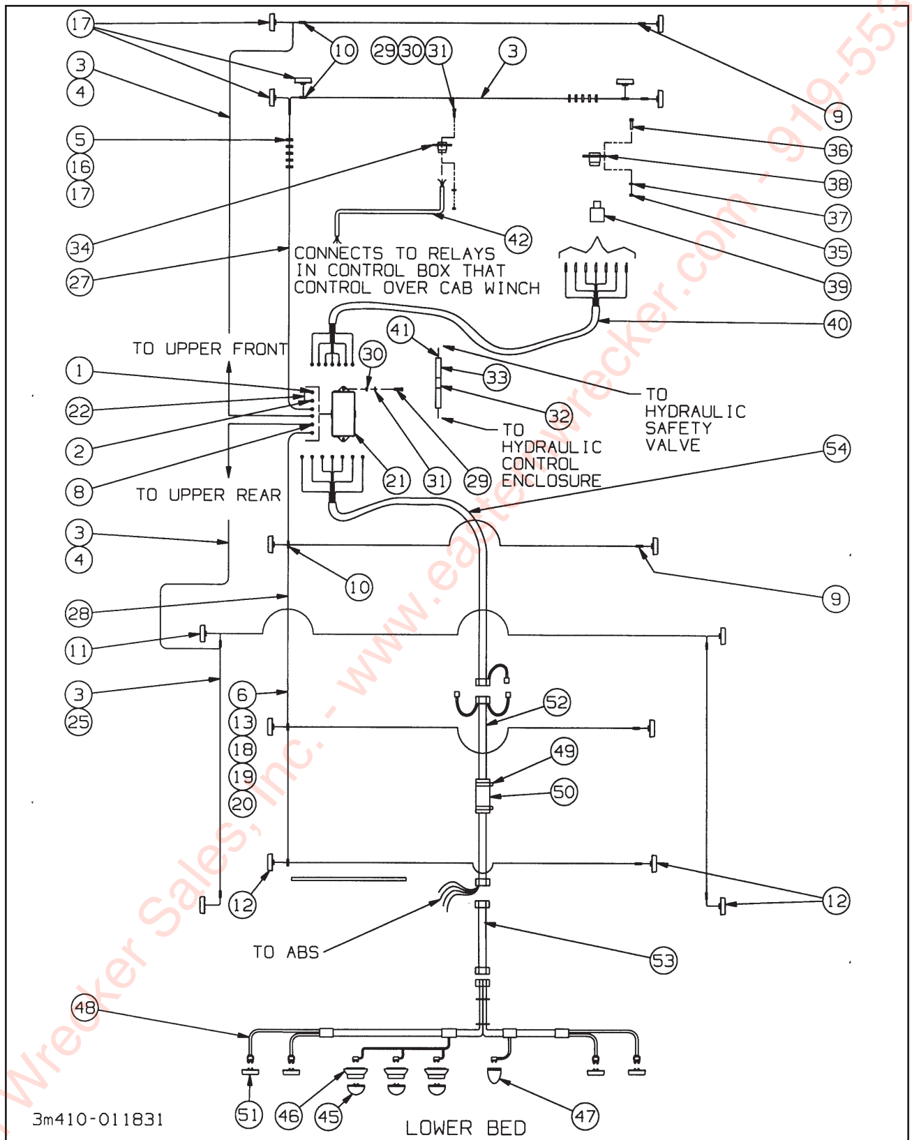
Figure 1-18 Electrical System
