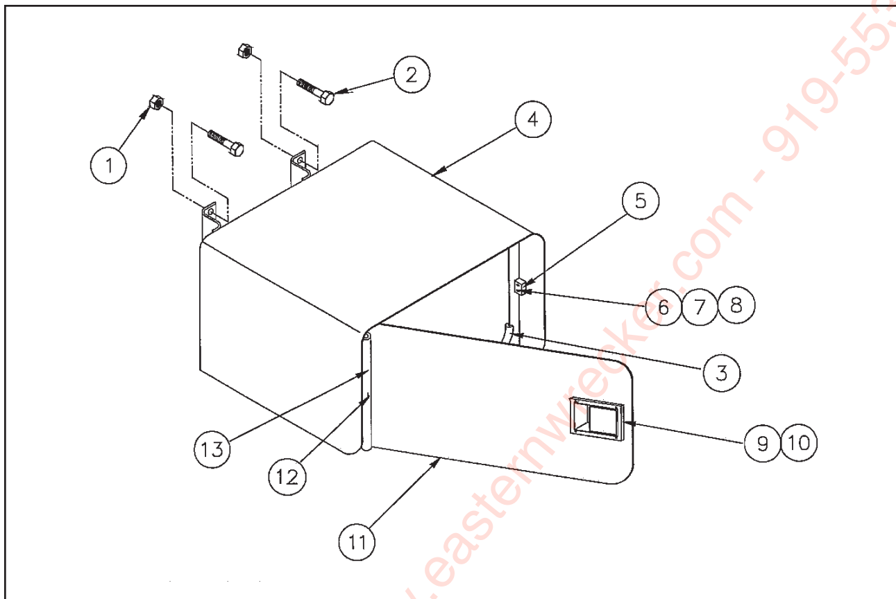
Figure 1-52 Tool Box
