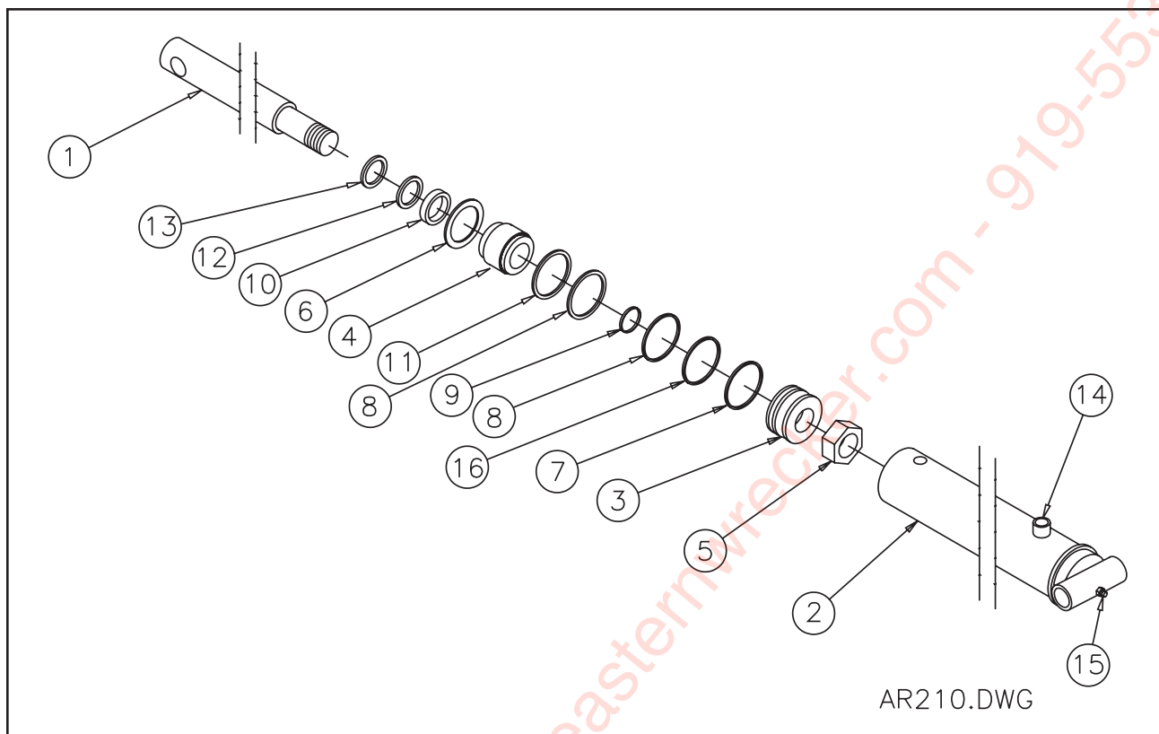
Figure 1-16 Hydraulic Cylinder Assembly, 4"x32"
