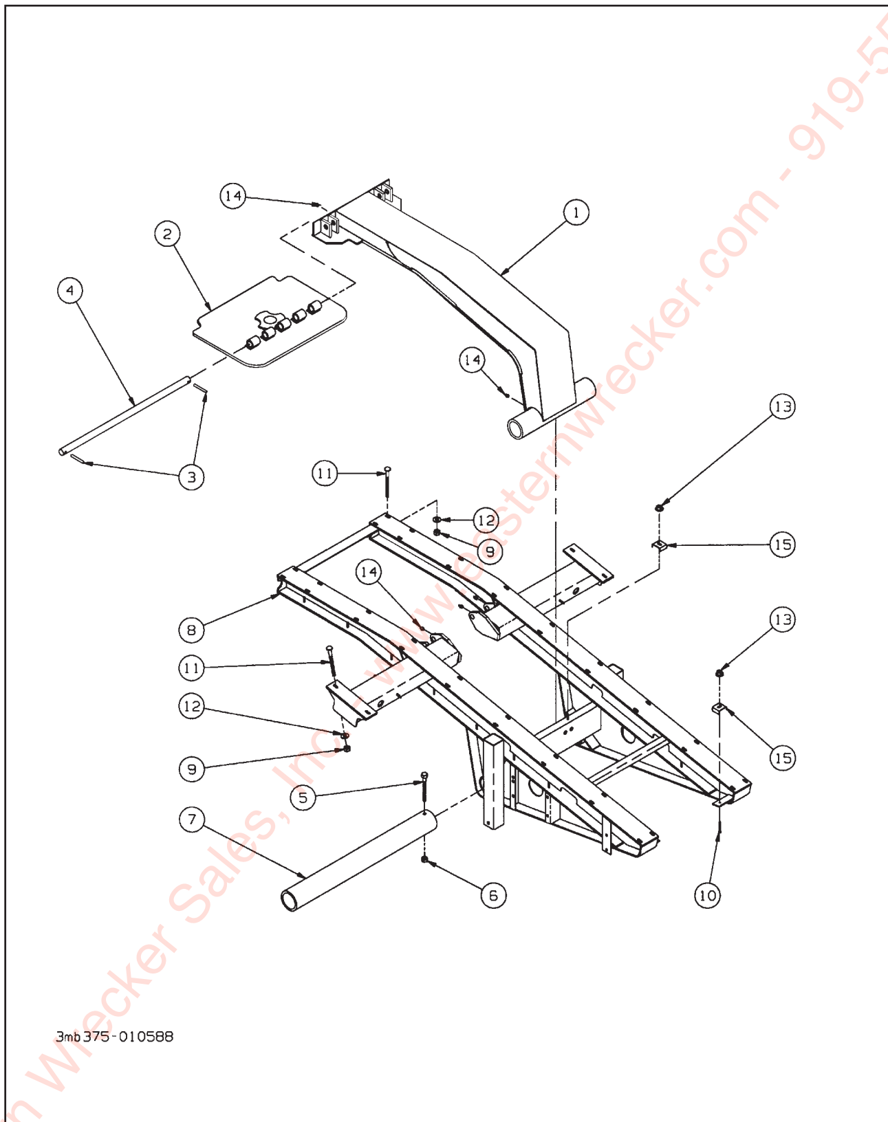
Figure 1-12 Hydraulic Tilt Assembly
