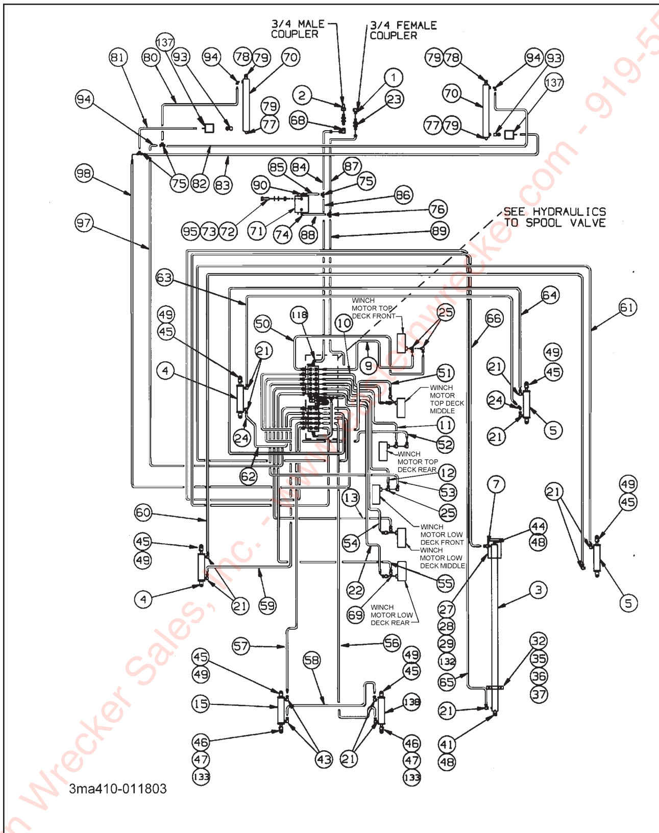
Figure 1-13 Hydraulic System
