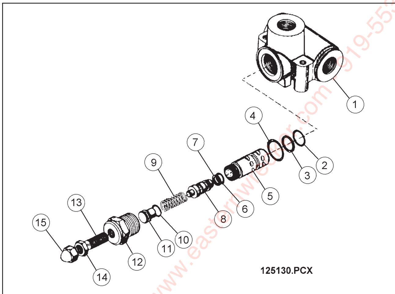
Figure 1-63 Pressure Relief Valve
