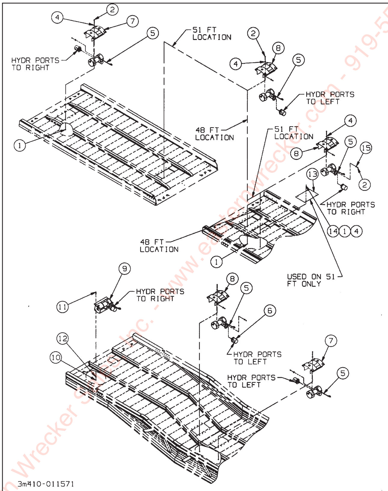
Figure 1-38 Winch Installation
