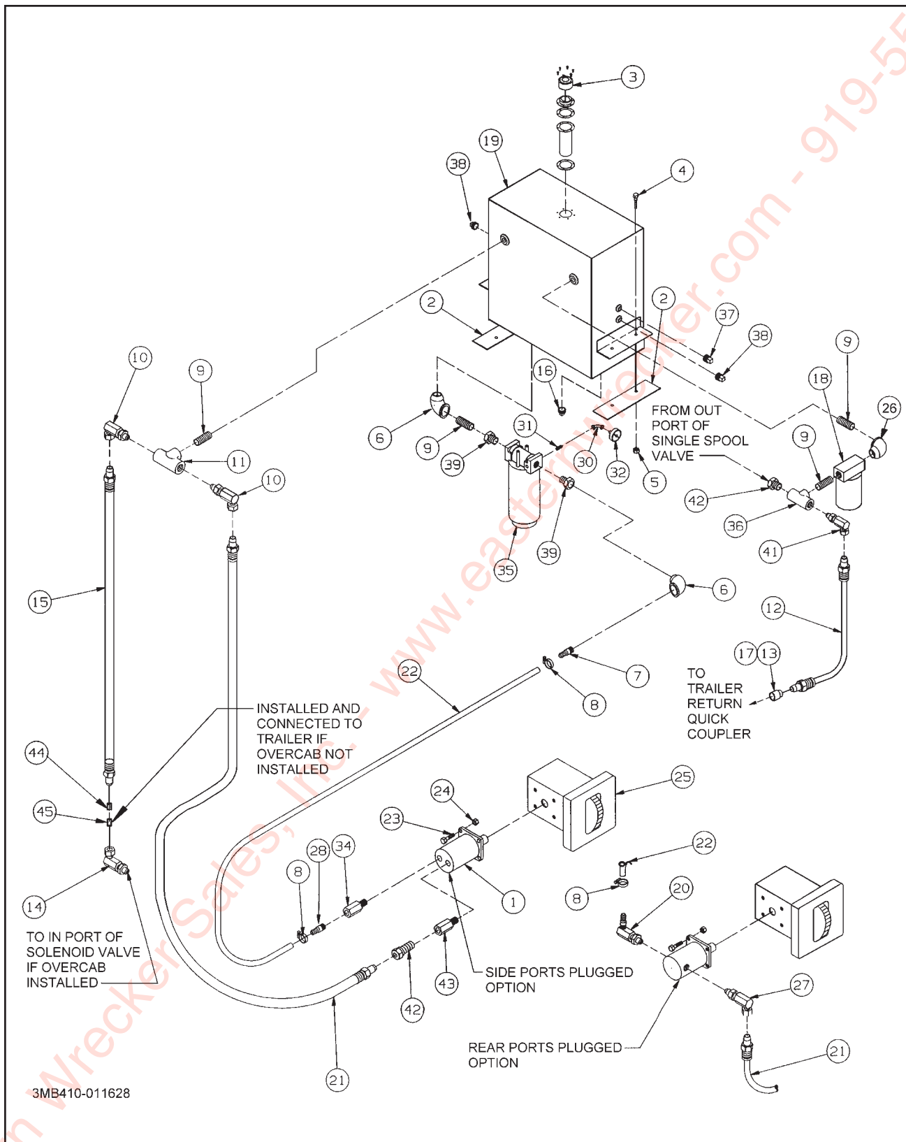
Figure 1-61 Wet Kit Assembly
