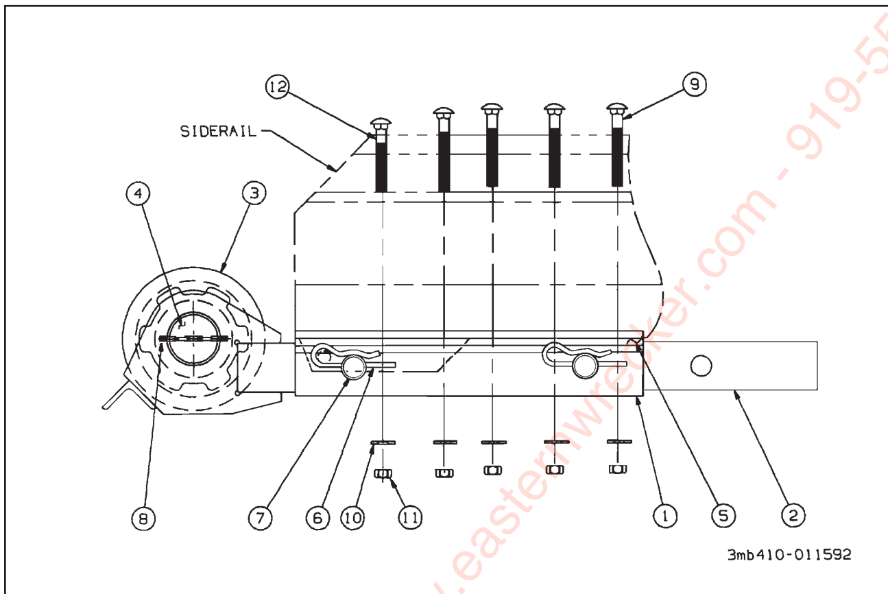
Figure 1-51 Cable Roller
