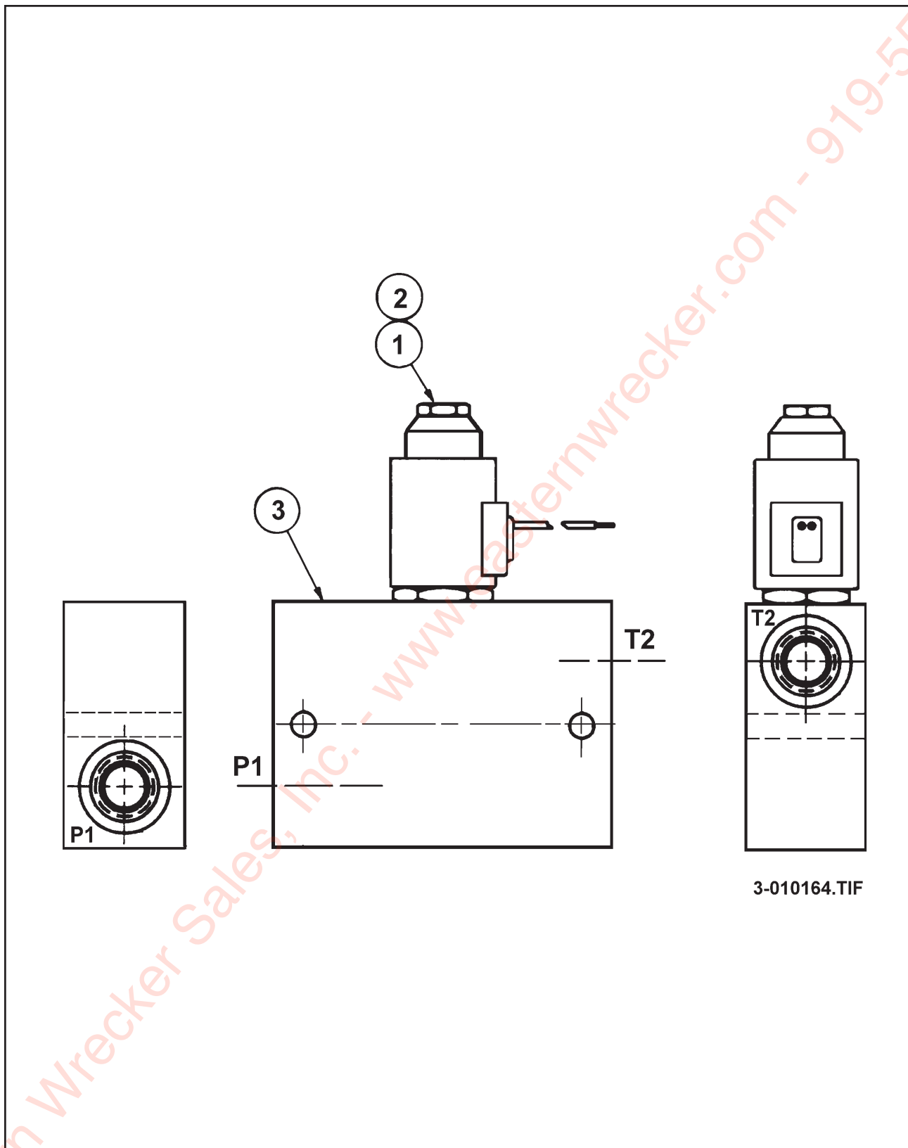
Figure 1-24 Valve N.O. Solenoid Hydraulic
