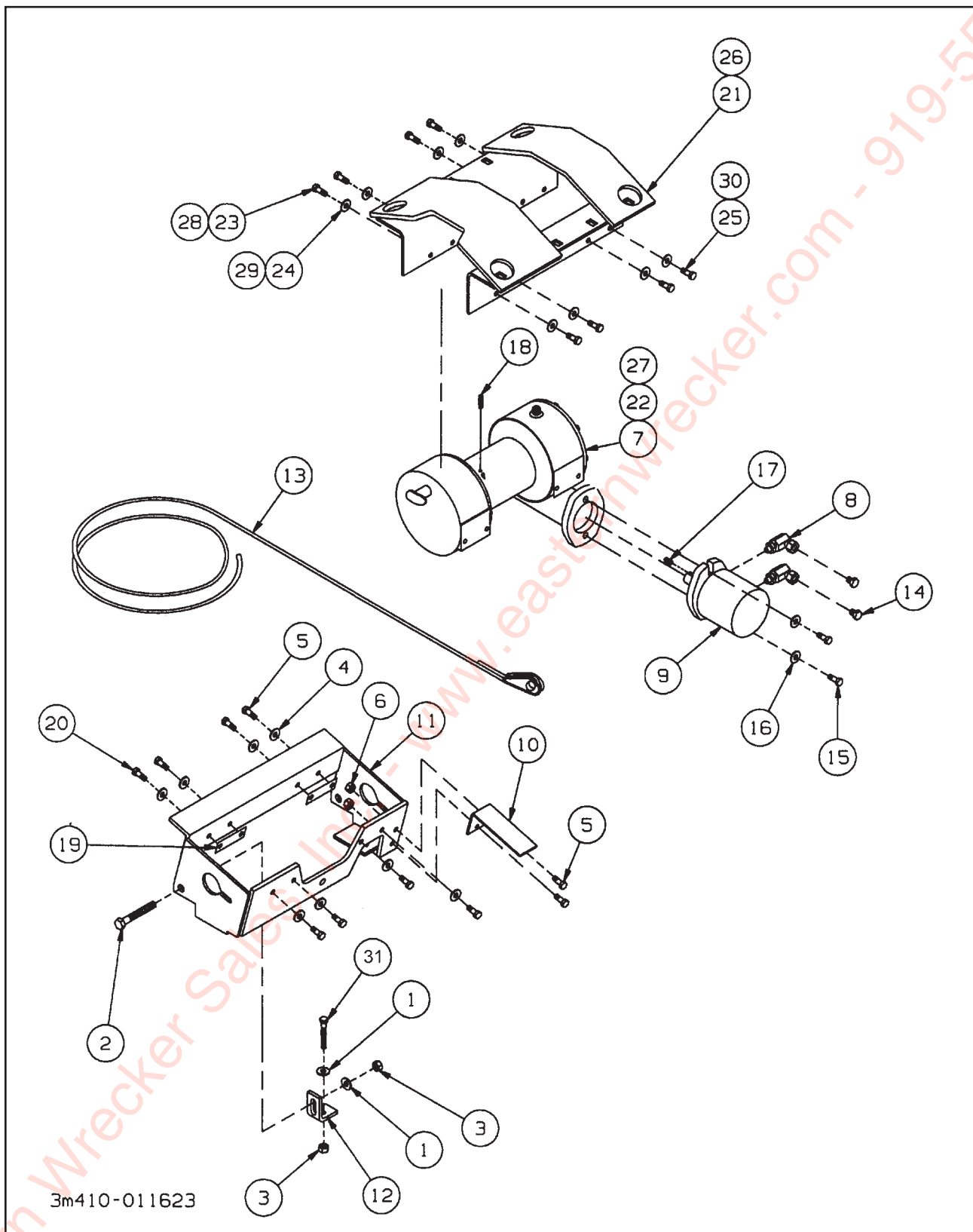
Figure 1-39 Winch Assembly
