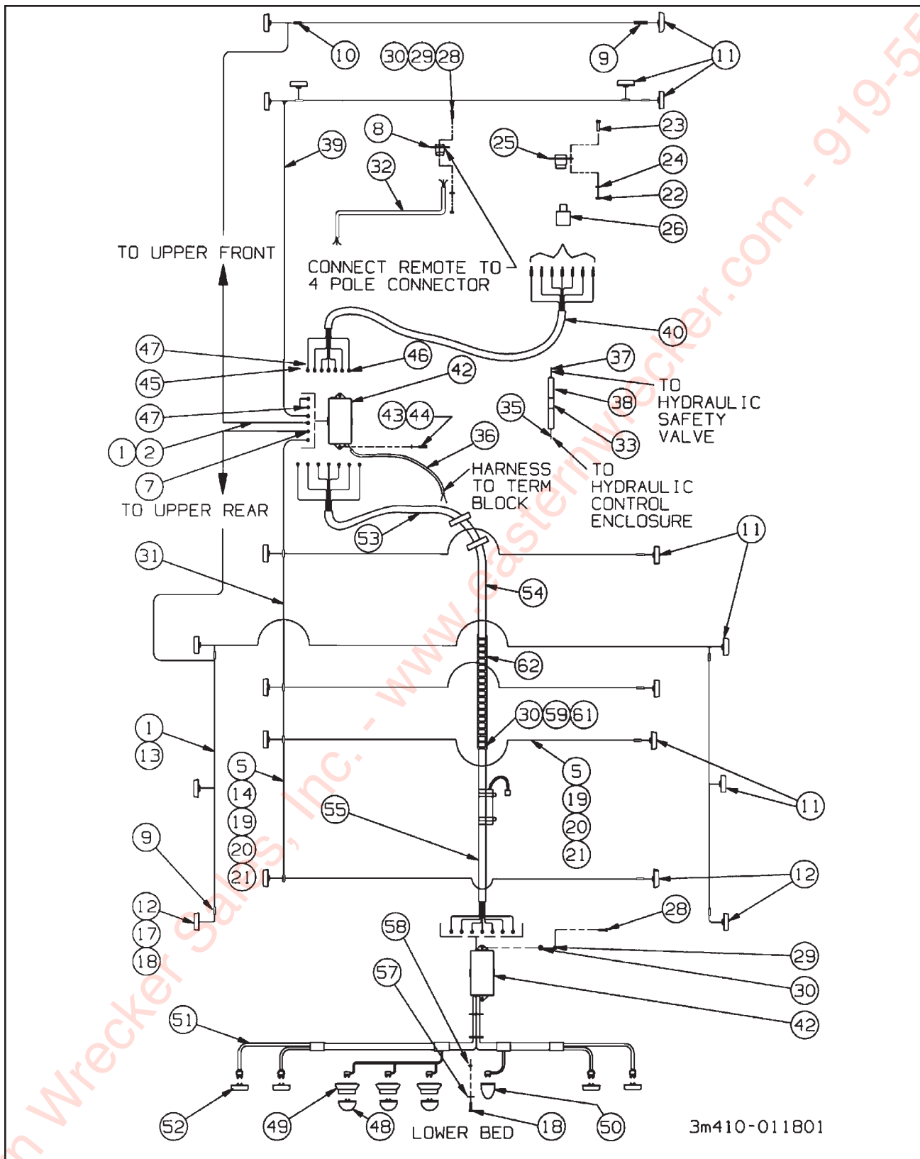
Figure 1-25 Electrical System
