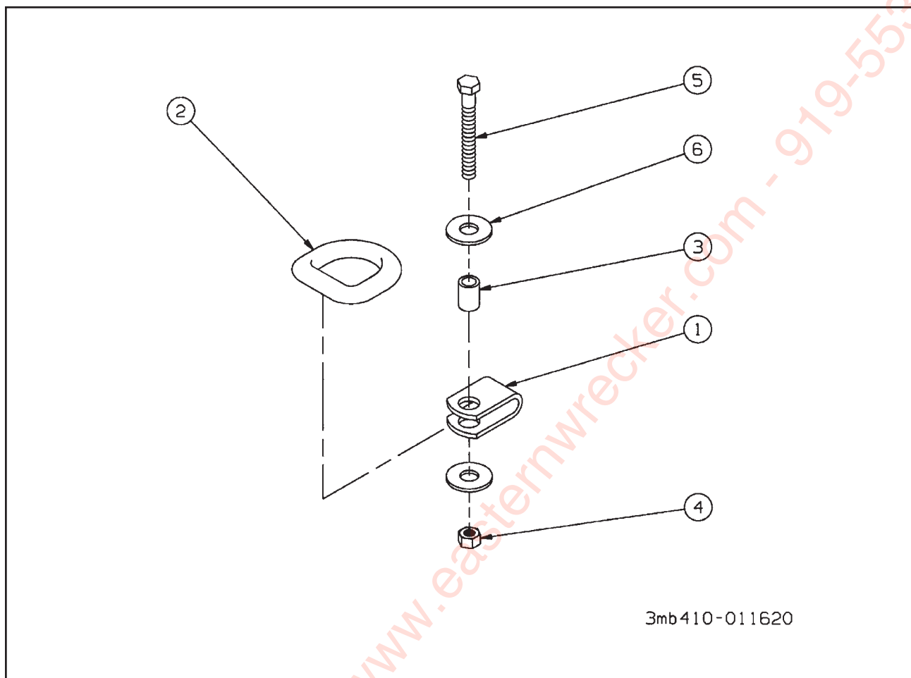
Figure 1-11 D-Ring Kit
