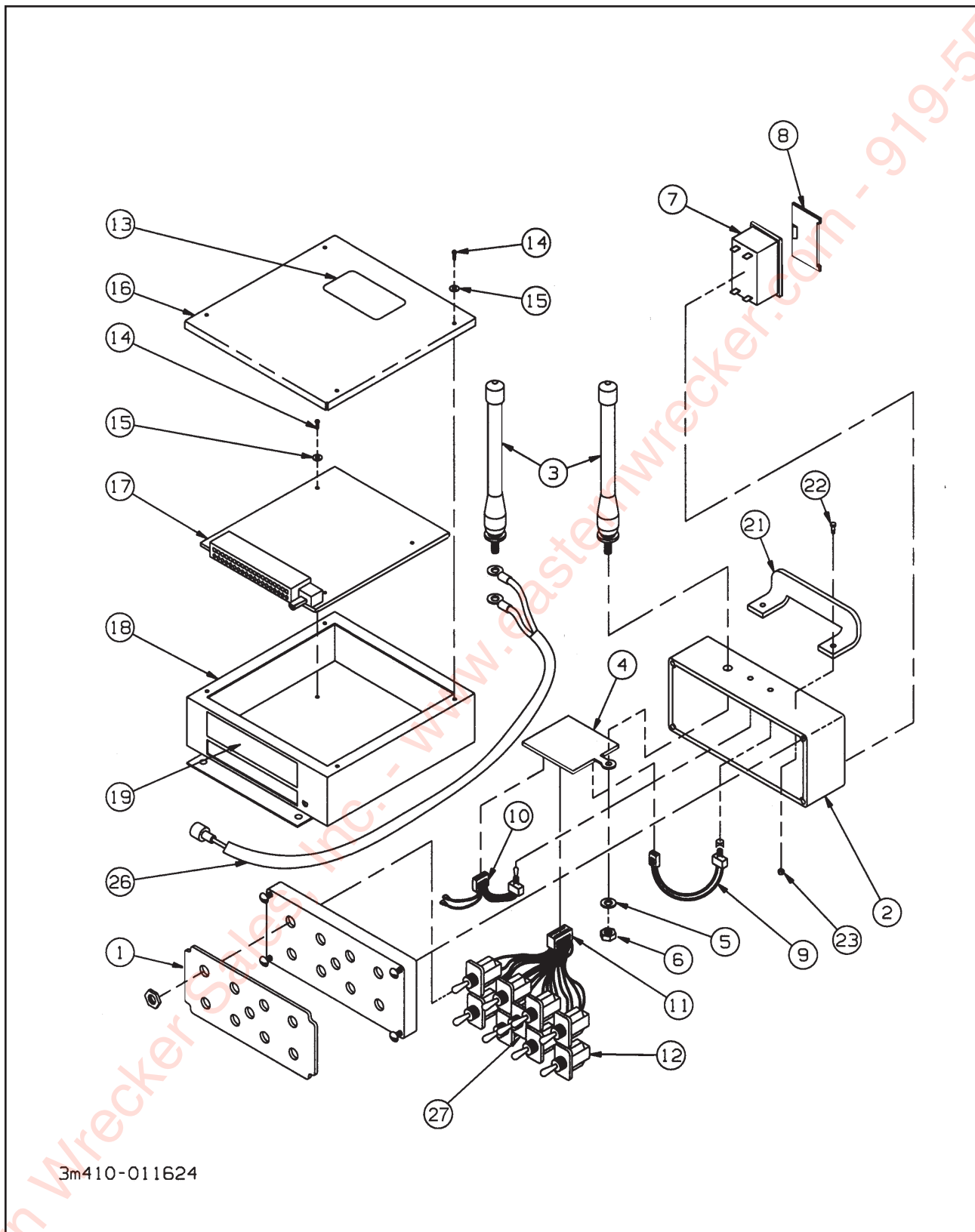
Figure 1-50 Remote Control
