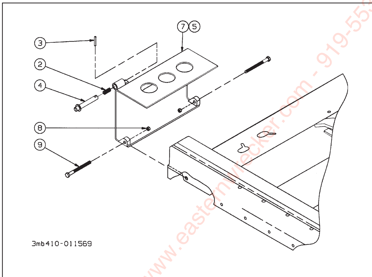
Figure 1-3 Wheel Stops
