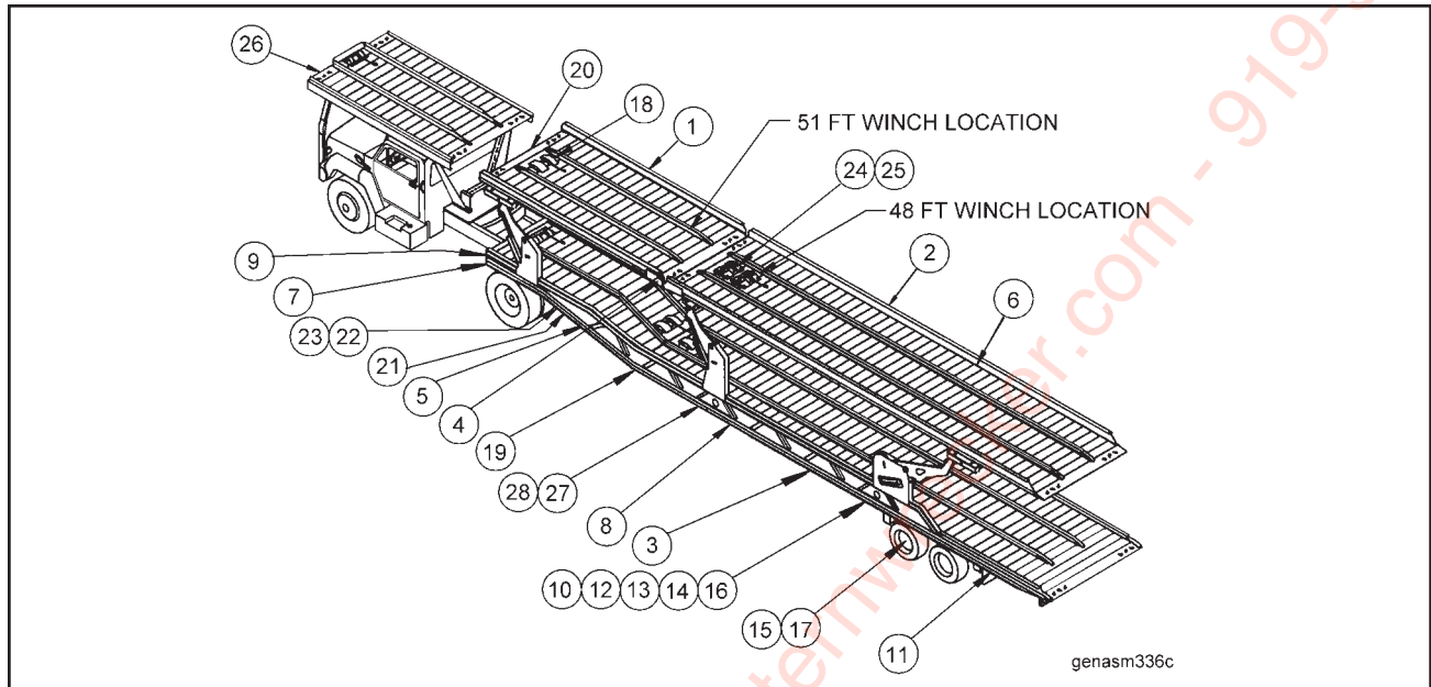
Figure 1-1 General Assembly
