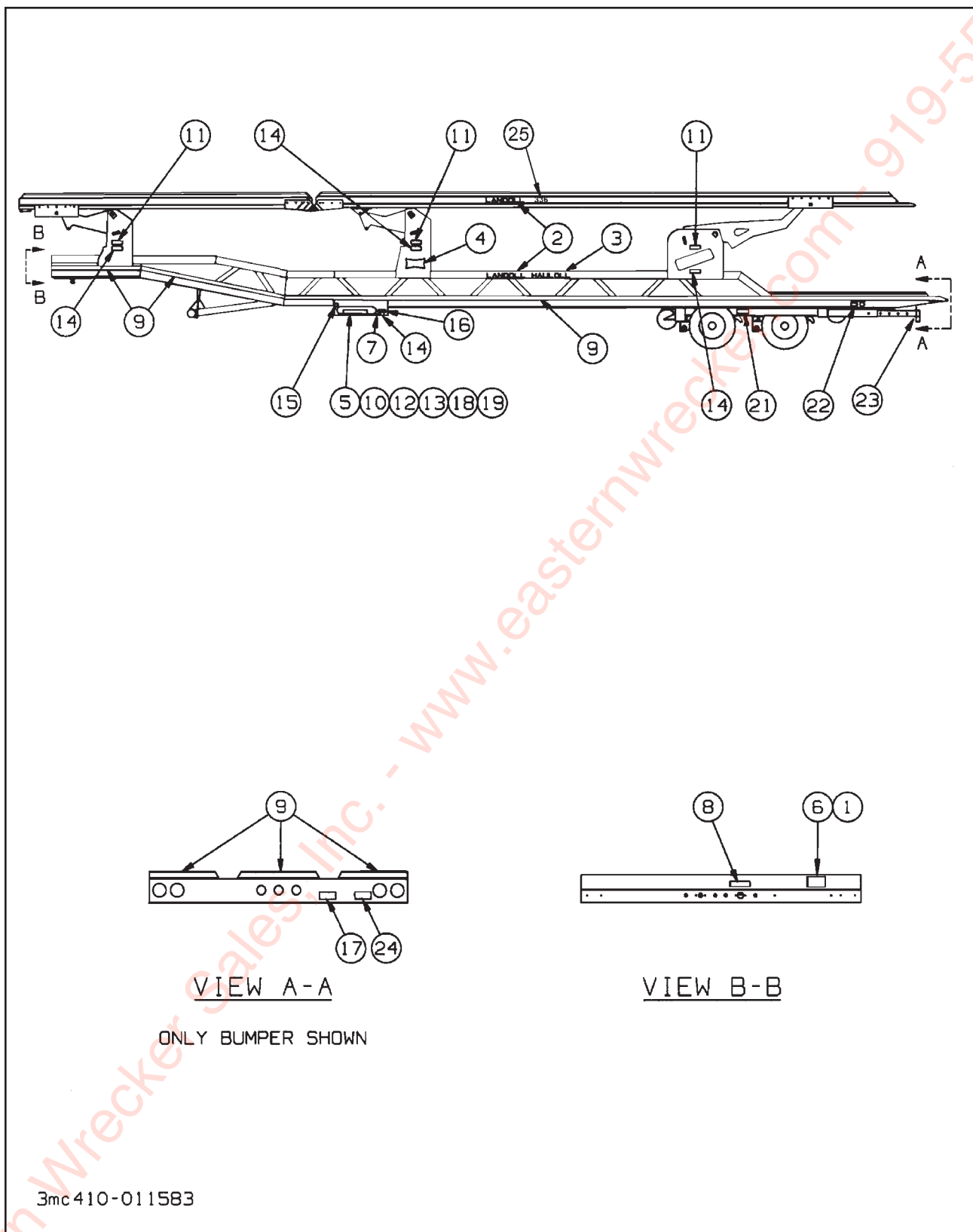
Figure 1-28 Decal Placement
