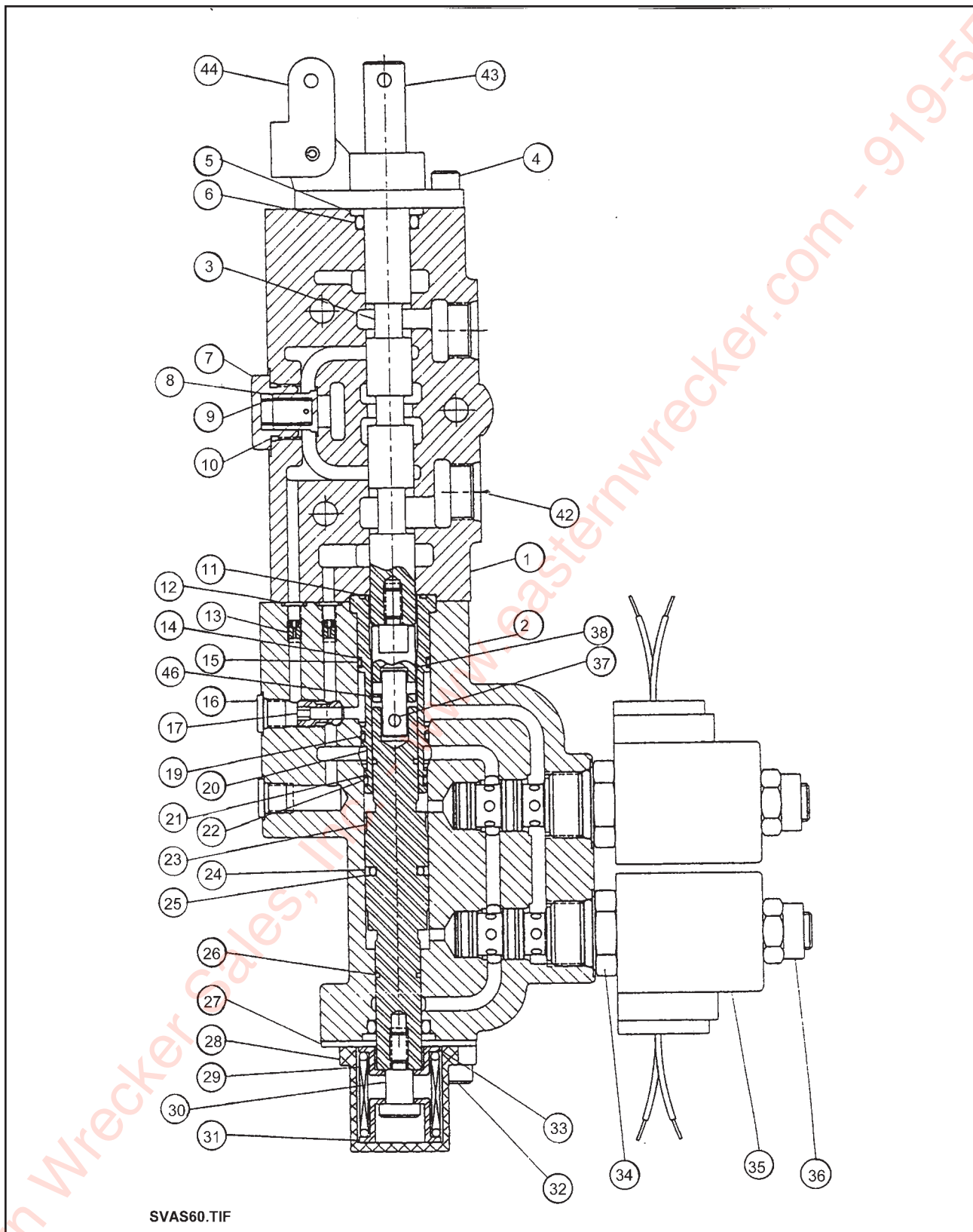
Figure 1-23 Spool Valve, Work Sections
