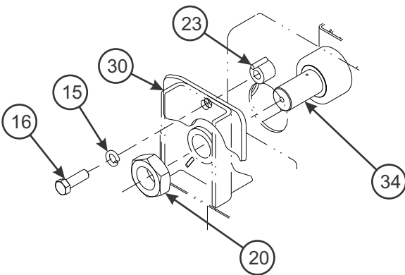
FRONT CAM FOLLOWER & HOLD DOWN ASSEMBLY
