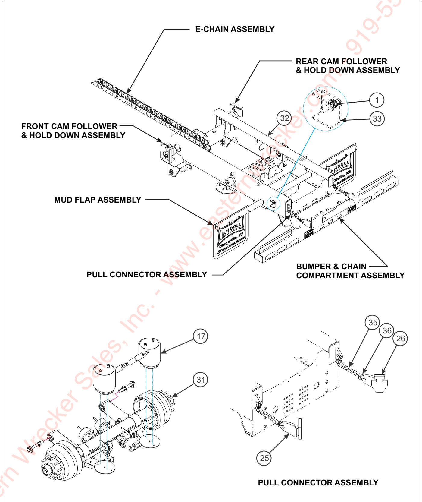
Figure 1-14: General Items (1 of 3)
