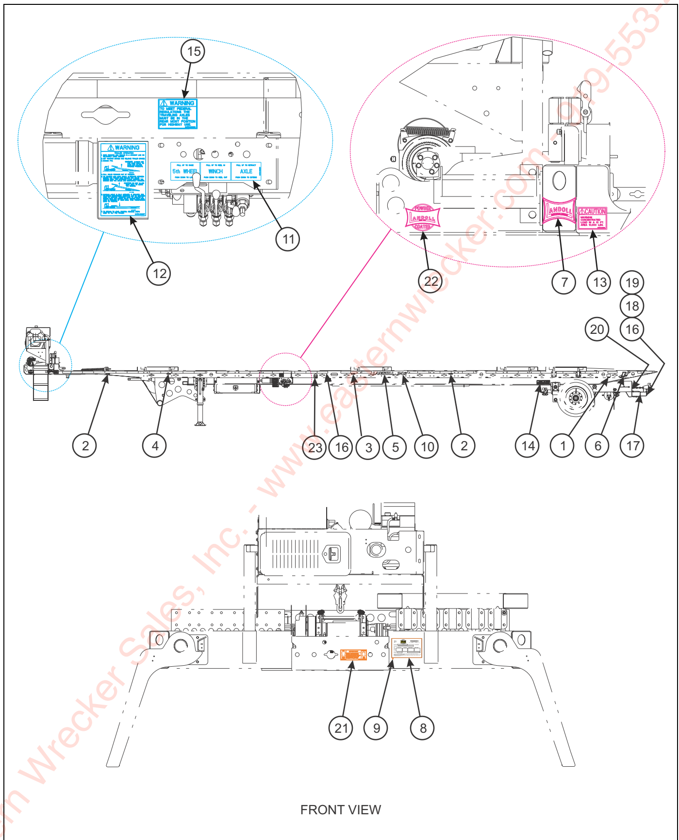
Figure 1-54: Decal Installation (2 of 2)
