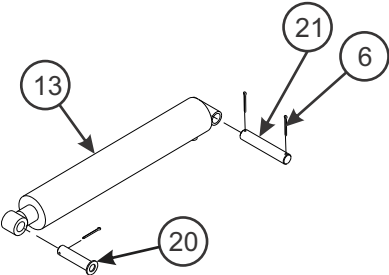
TILT CYLINDER ASSEMBLY
