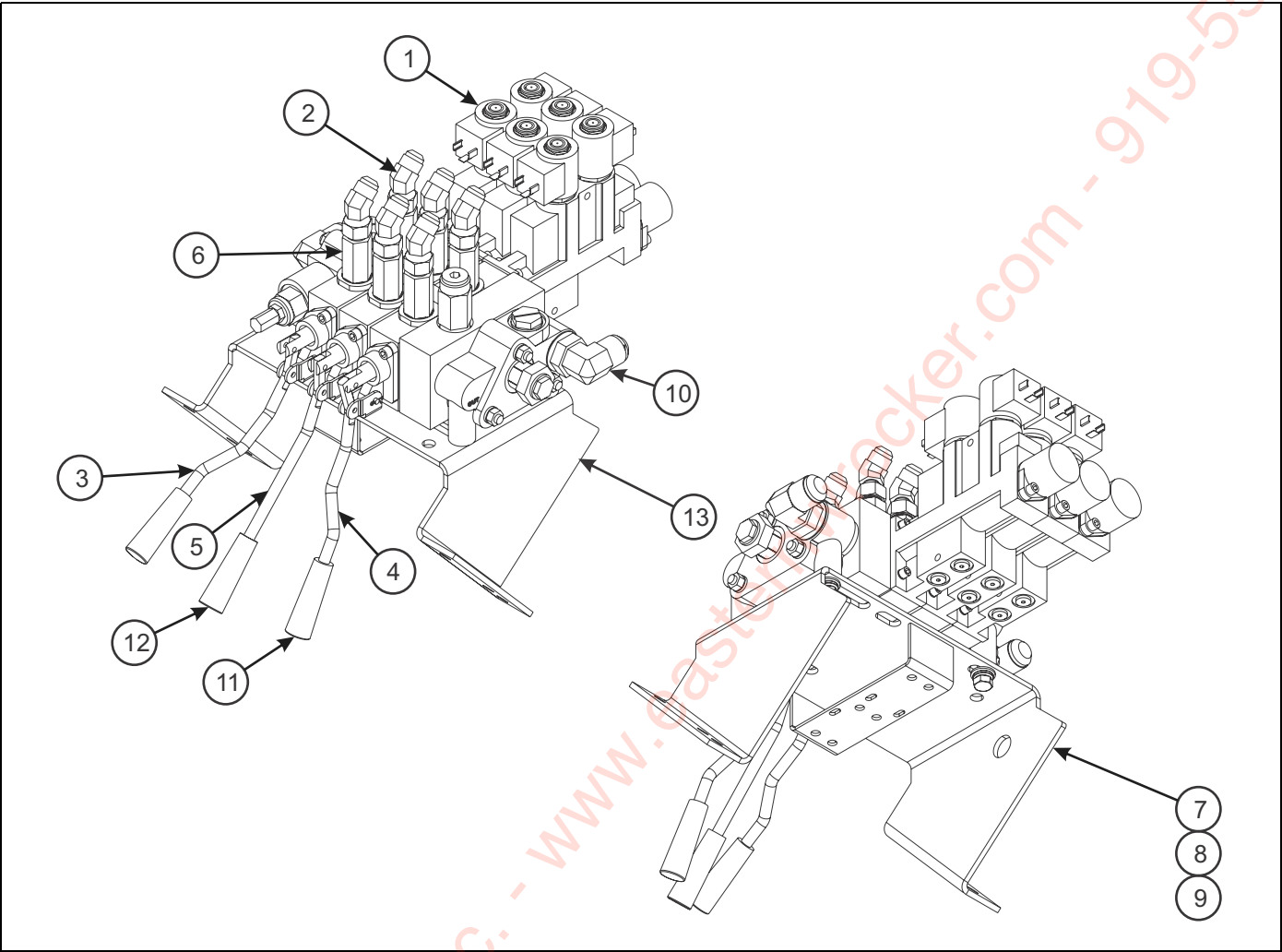
Figure 1-10: Valve Assembly - Three Spool
