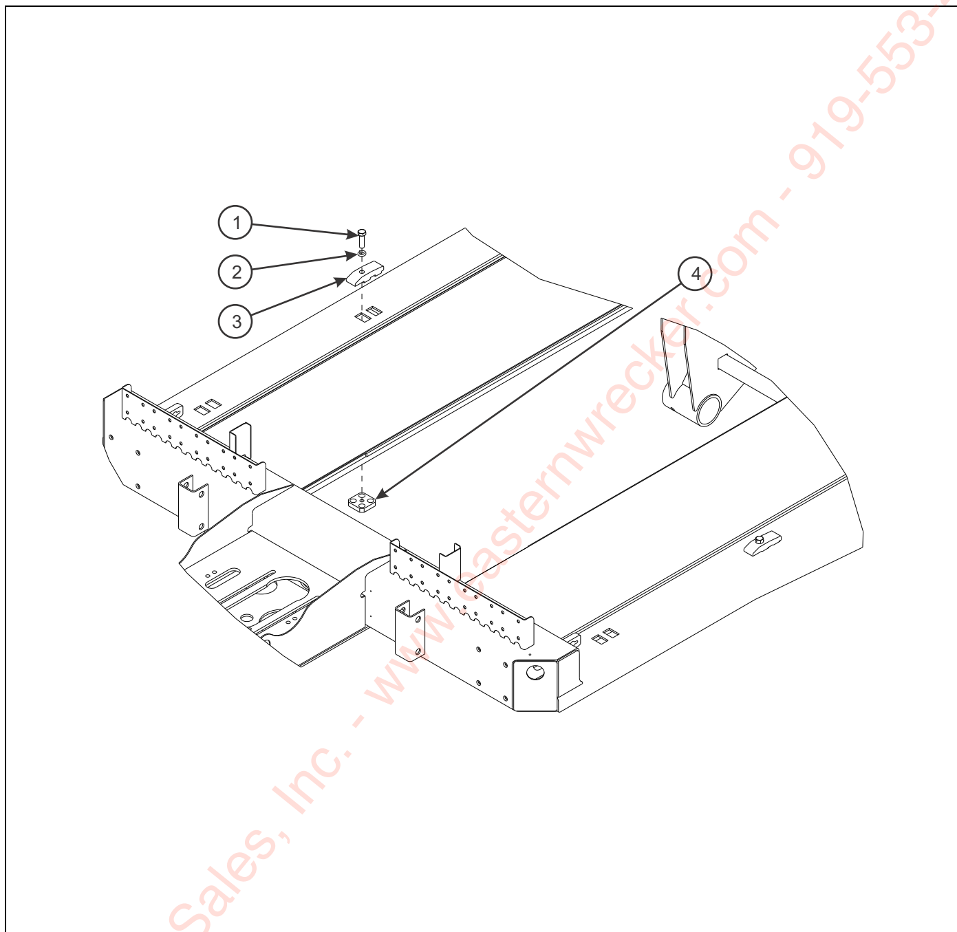
Figure 1-38: Container Pair - Front Pair
