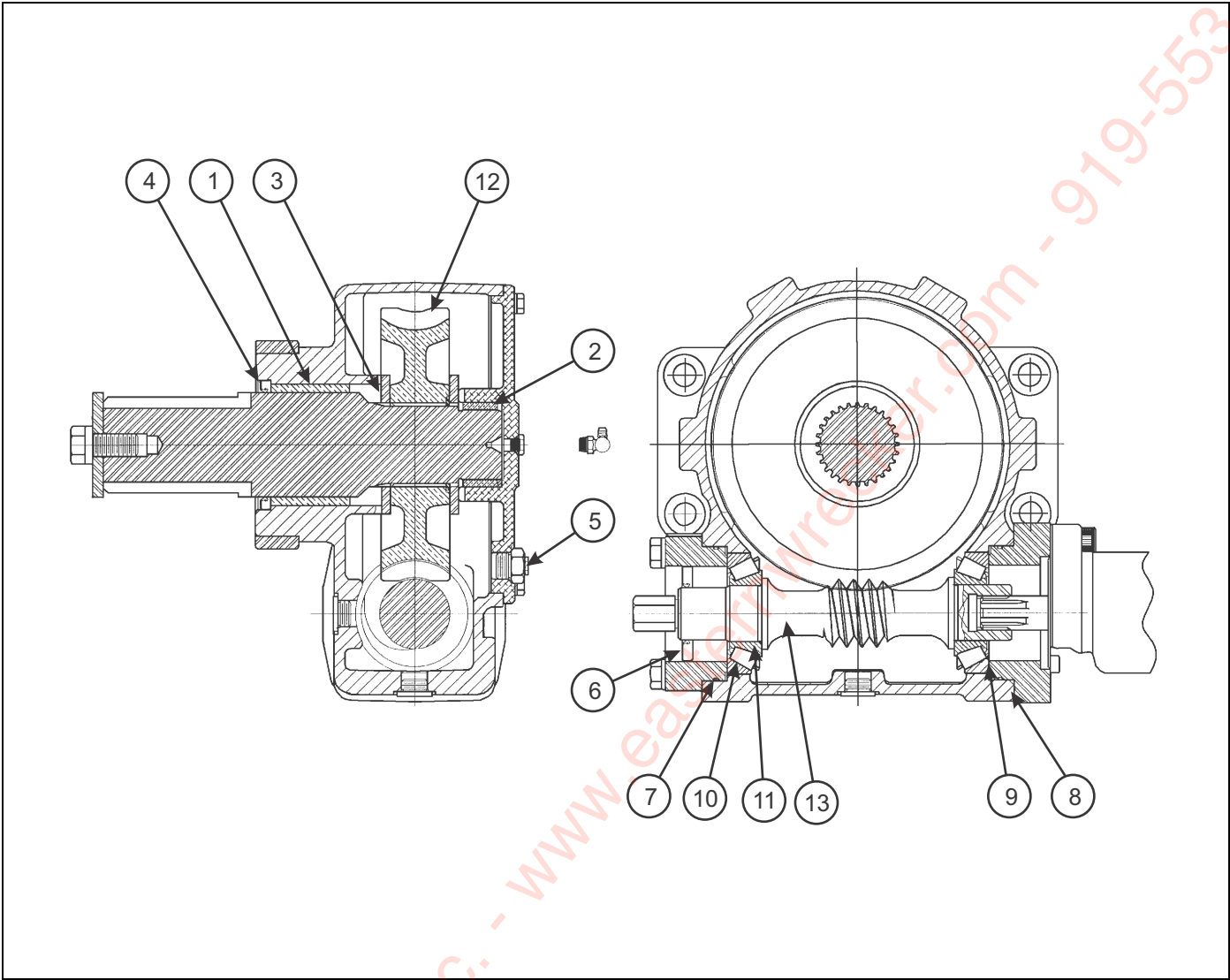
Figure 1-31: Gearbox Items
