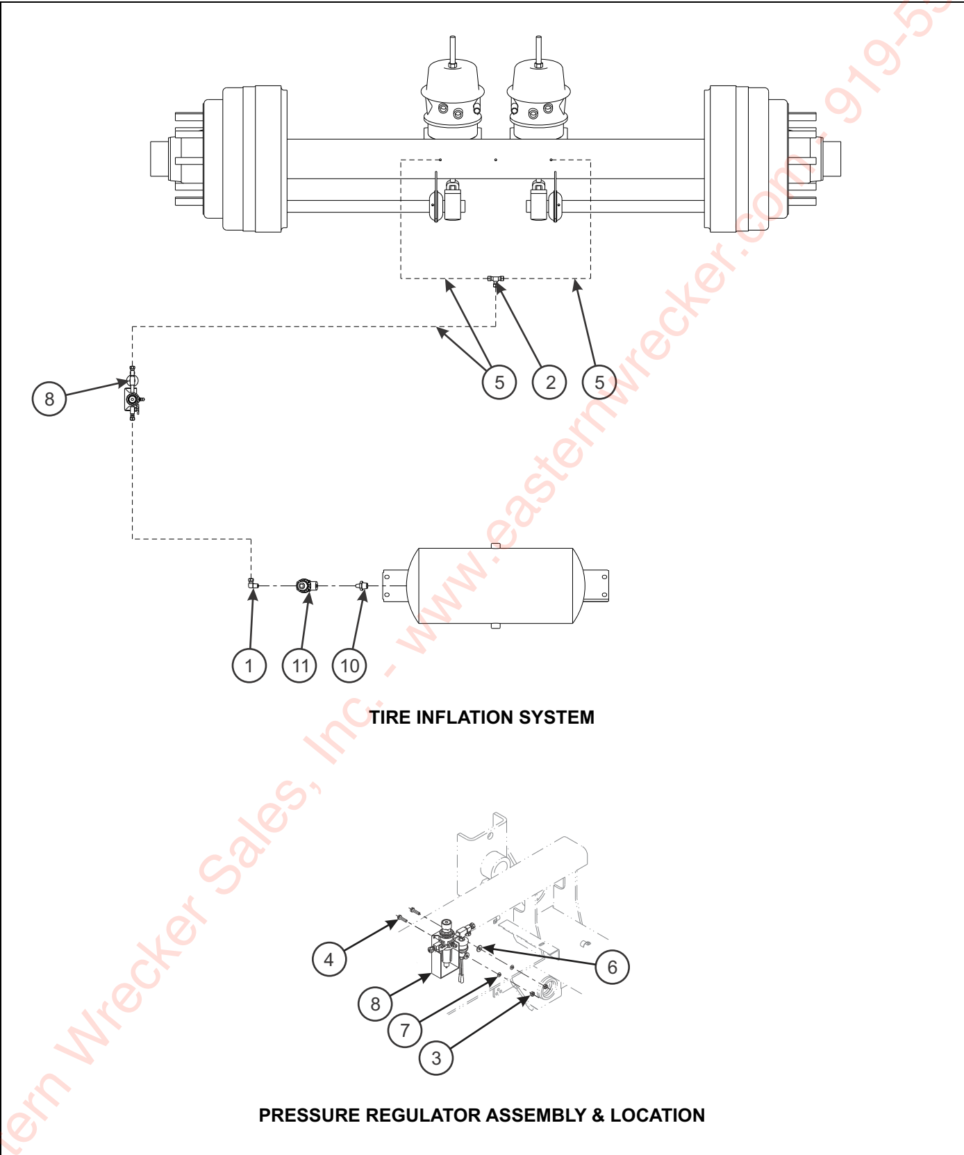
Figure 1-27: Tire Inflation System
