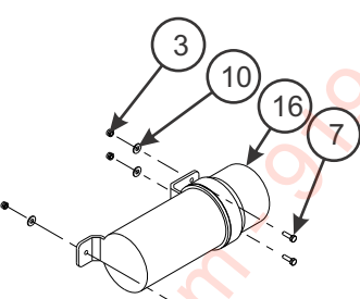
MANUAL TUBE ASSEMBLY
