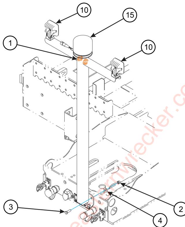
LIGHT SUPPORT ASSEMBLY
