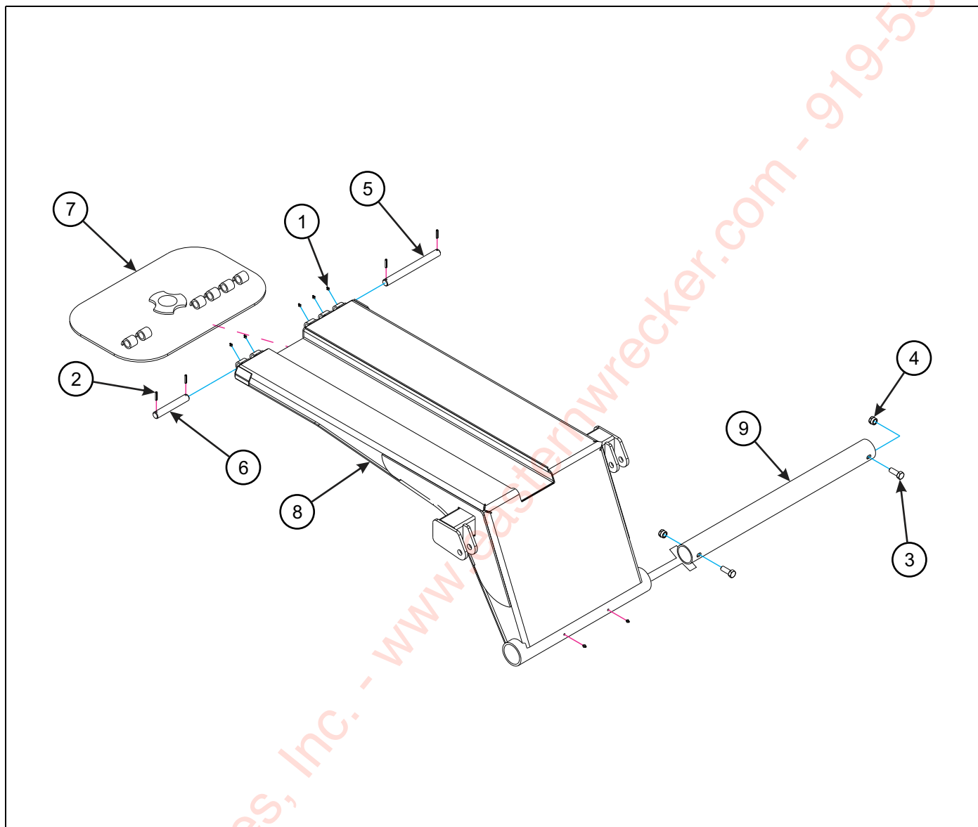
Figure 1-52: Hitch Installation
