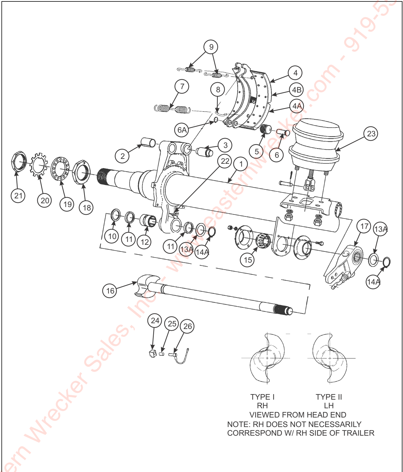
Figure 1-23: Axle and Brake Assembly - Dexter (12-1/4" X 7-1/2")
