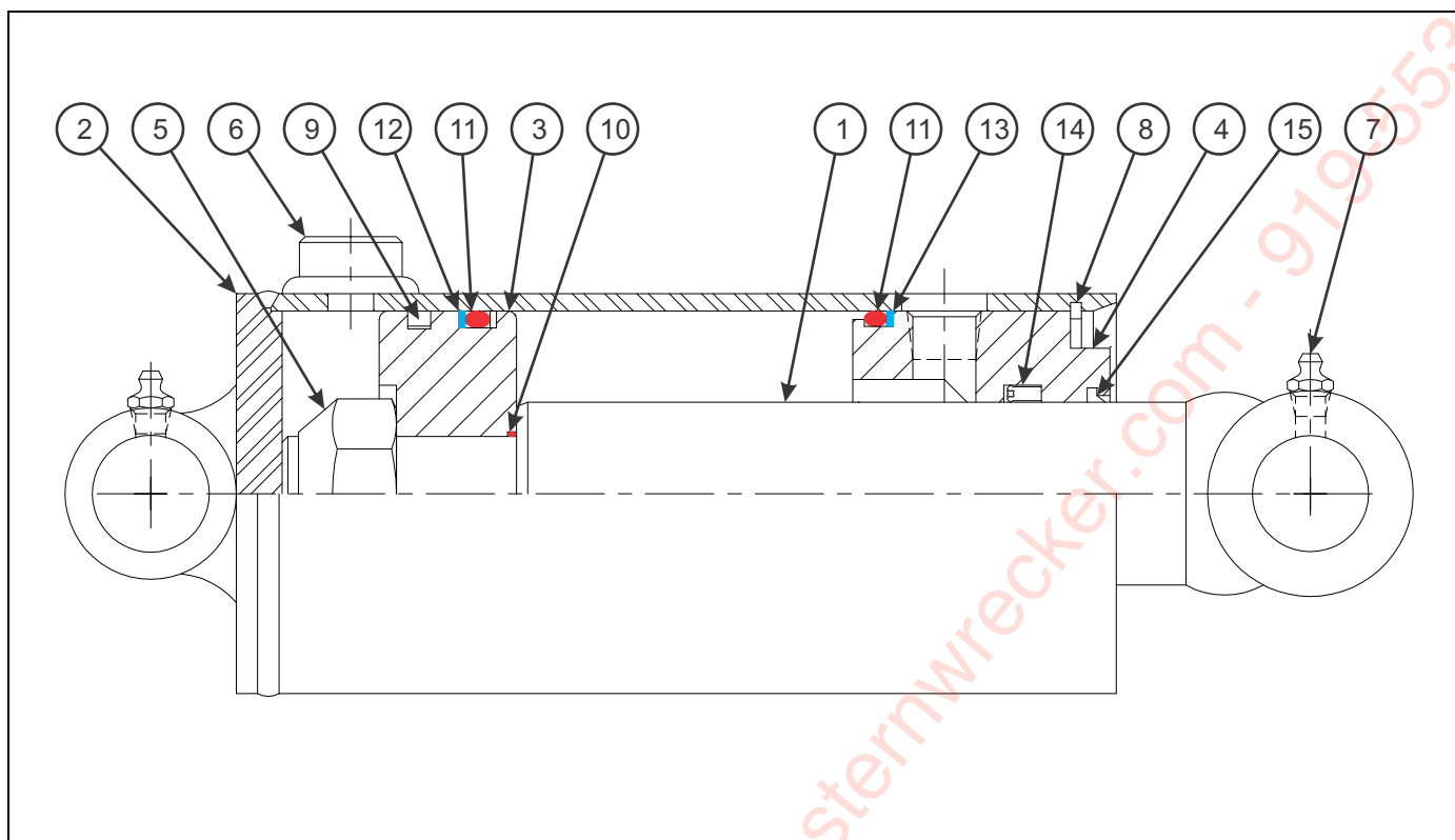
Figure 1-8: Hydraulic Cylinder - 4 x 20
