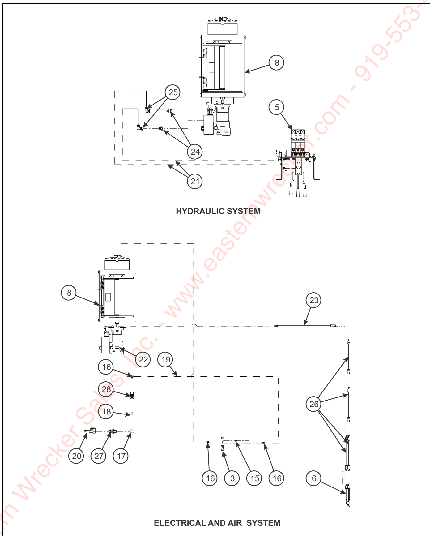
Figure 1-47: Winch Installation - 20K 2 Speed (WARN) (2 of 2)
