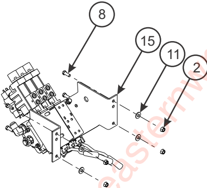
SPOOL VALVE ASSEMBLY
