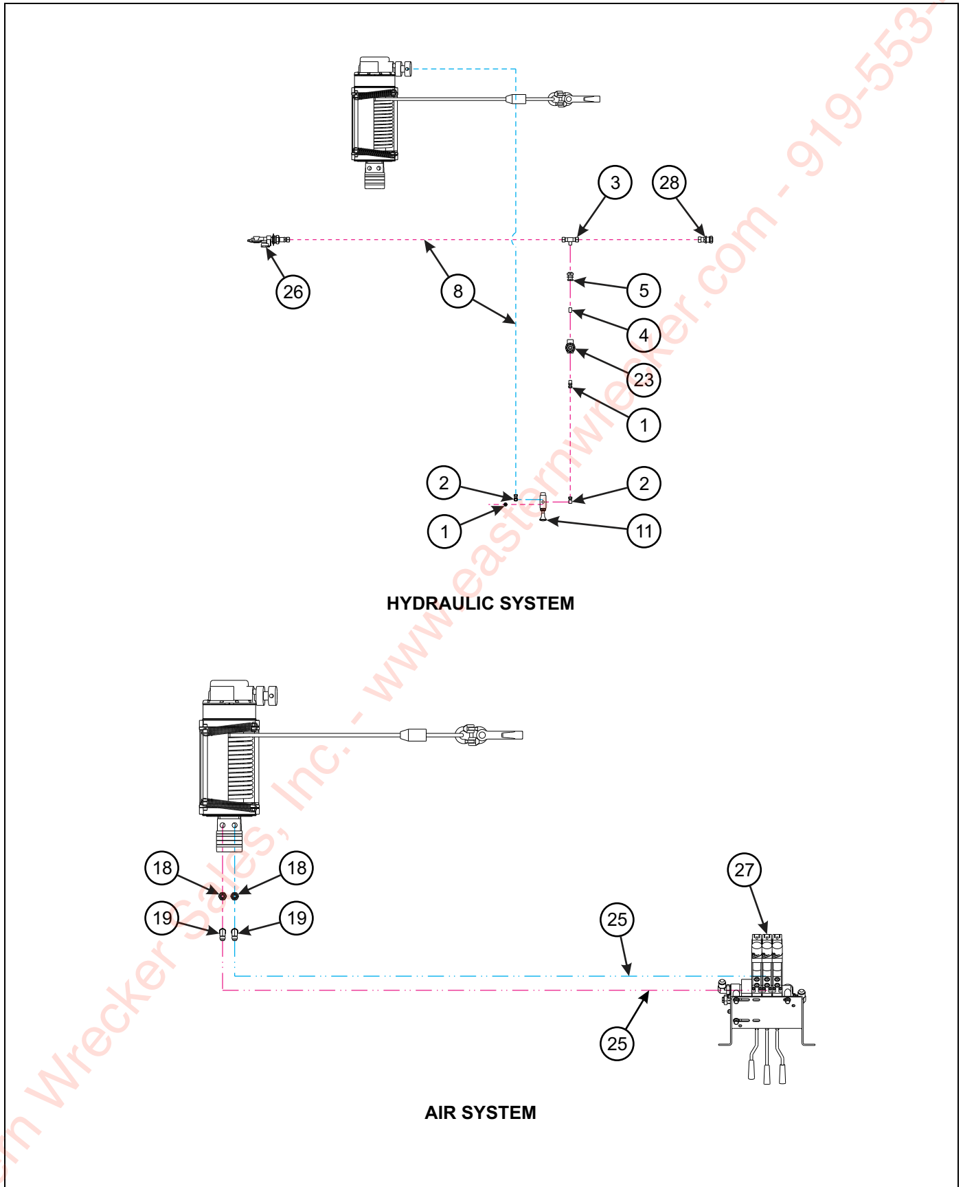
Figure 1-44: Winch Installation - 12K (WARN) 2 of 2
