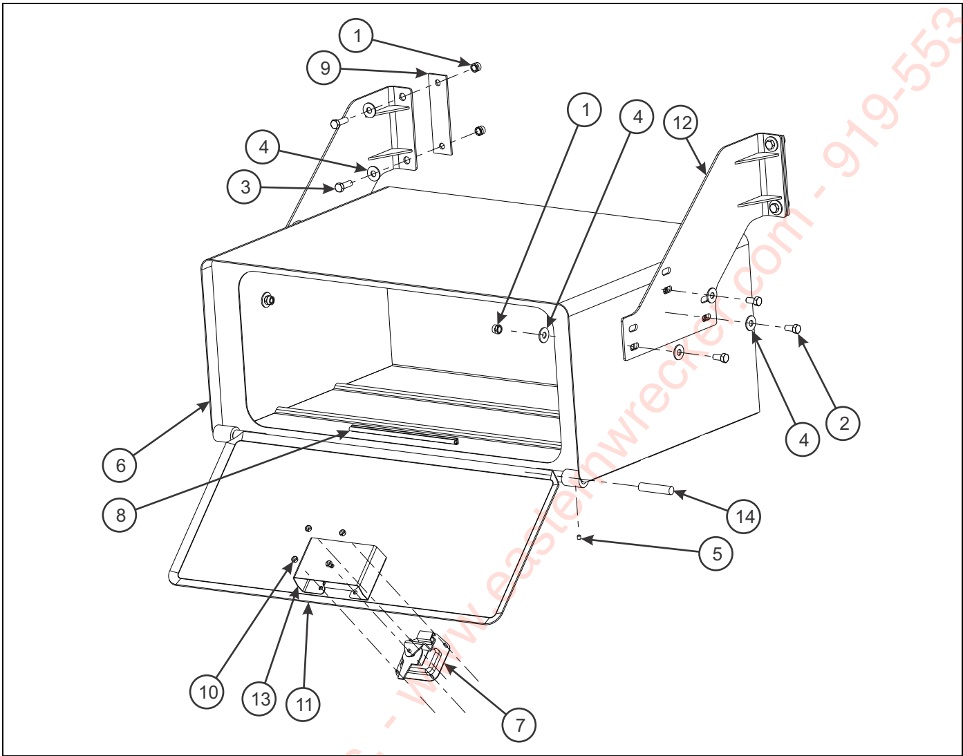
Figure 1-72: Tool Box Installation
