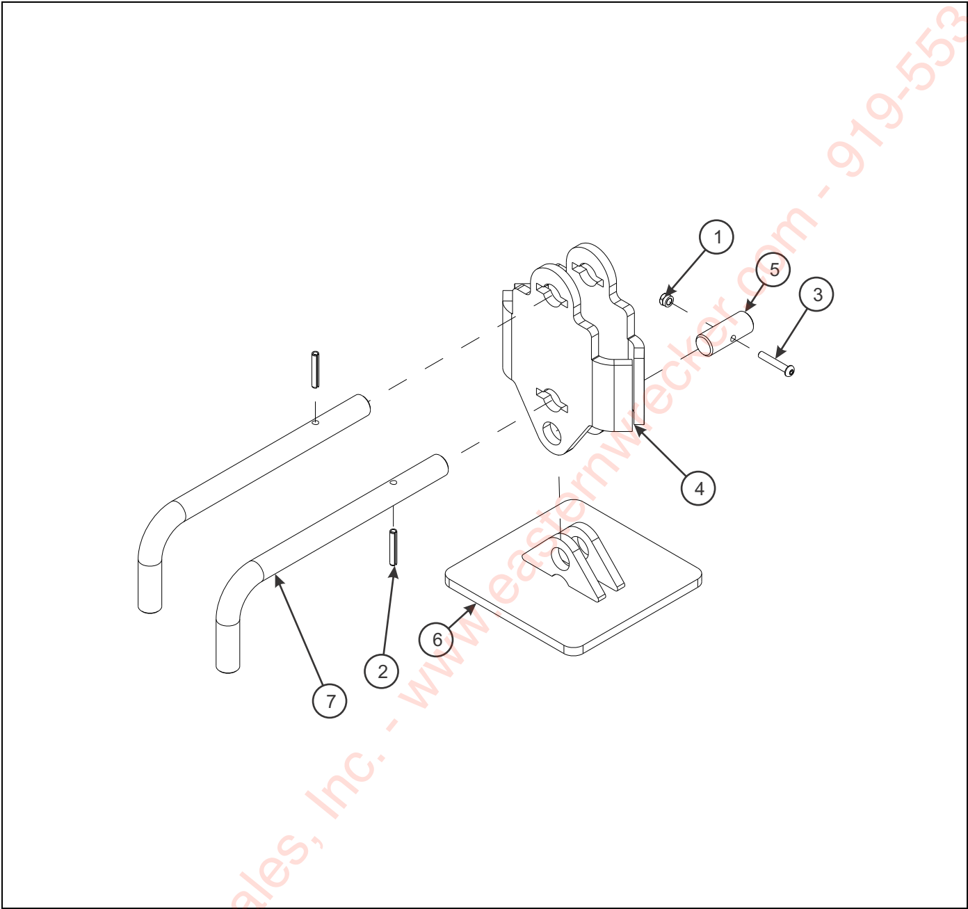
Figure 1-70: Tiedown Assembly - Shoe Lock
