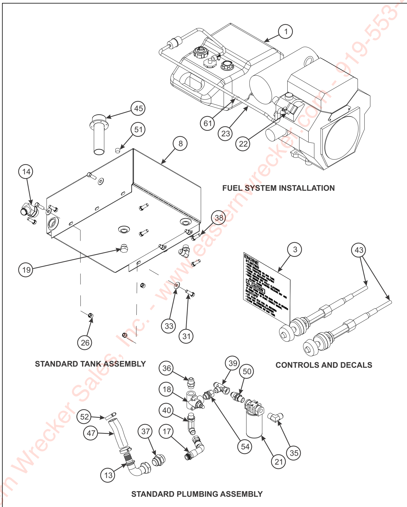
Figure 1-60: Engine - 27 HP Gas Package (2 of 2)
