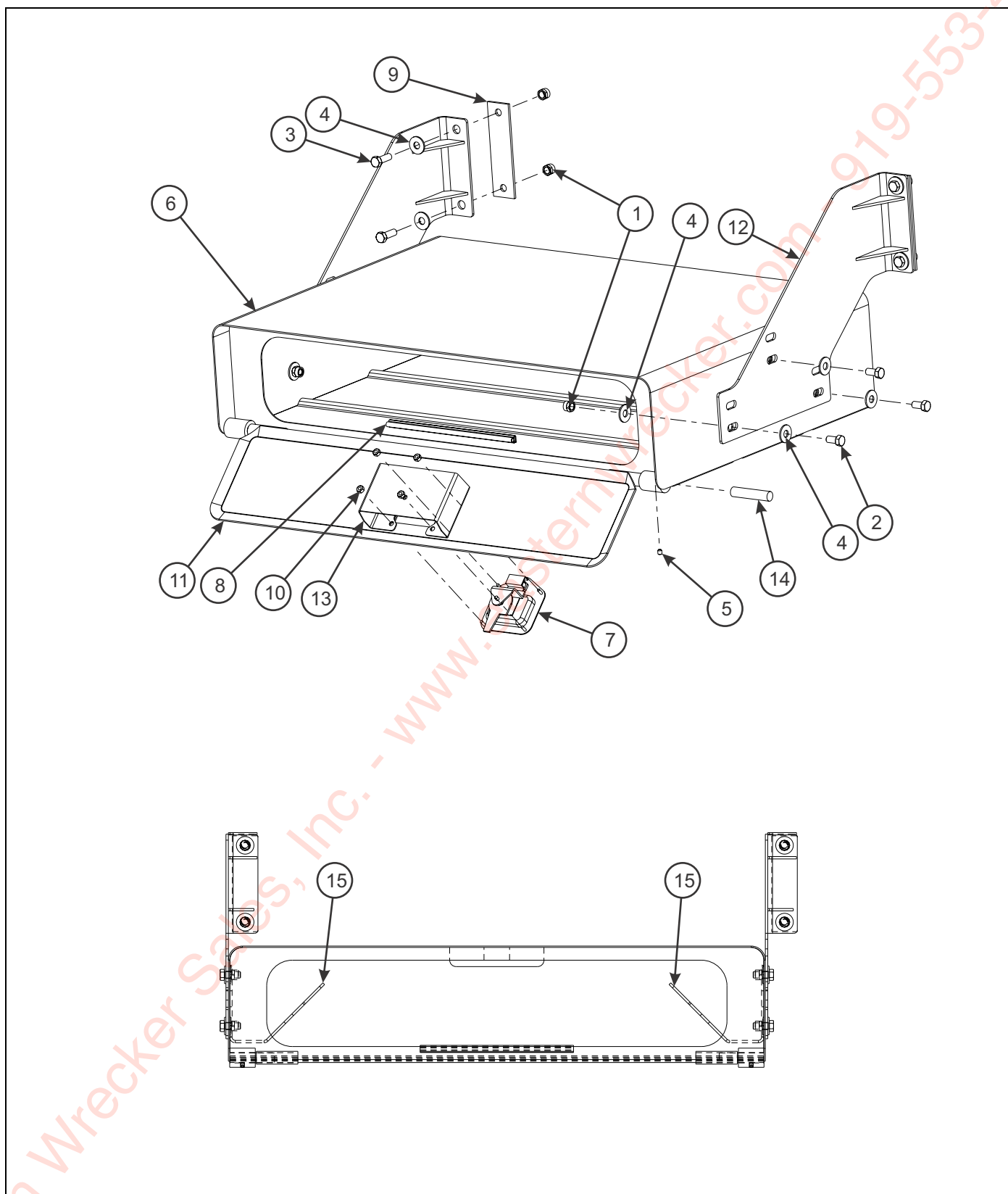
Figure 1-73: Tool Box Installation - Steel Door
