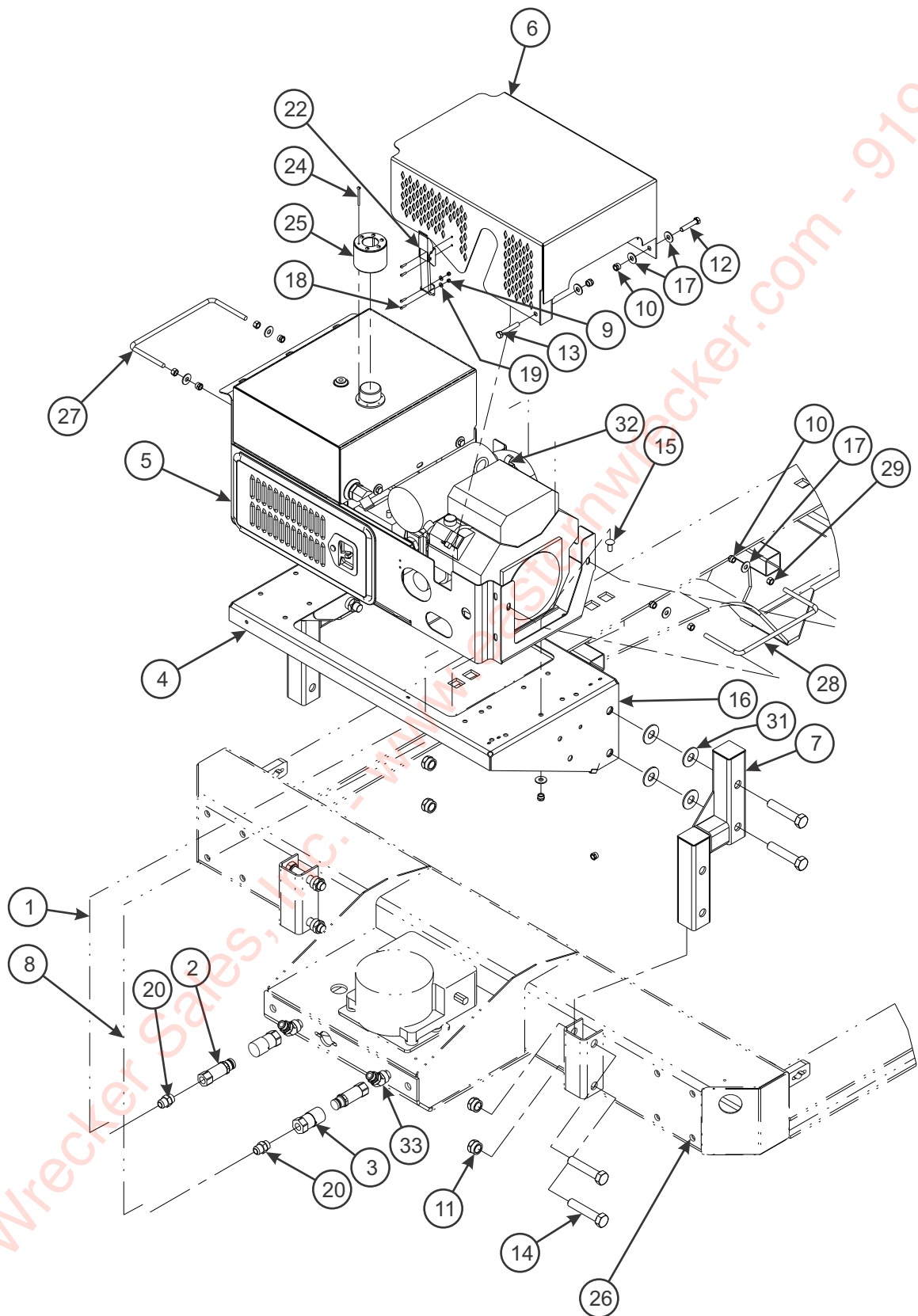
Figure 1-58: Engine - 27 HP Drive Installation
