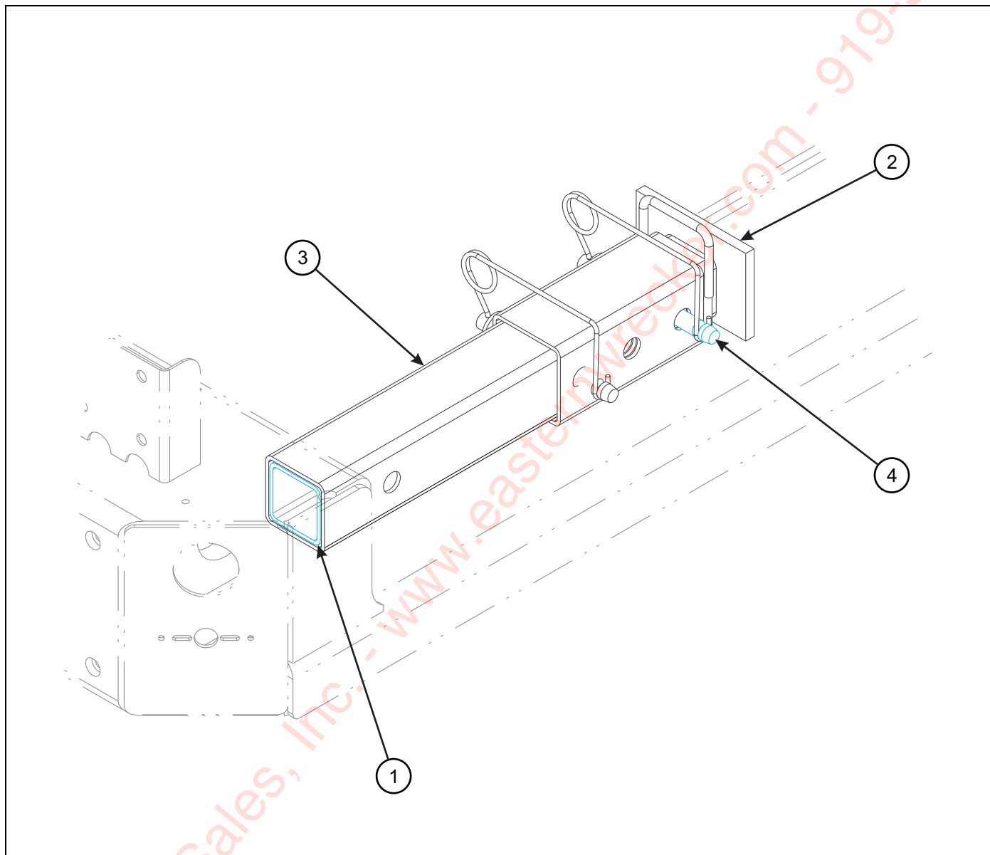
Figure 1-32: Adjustable Stop Assembly
