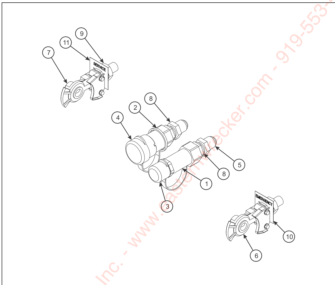
Figure 1-9: Connectors - Front Sub Assembly
