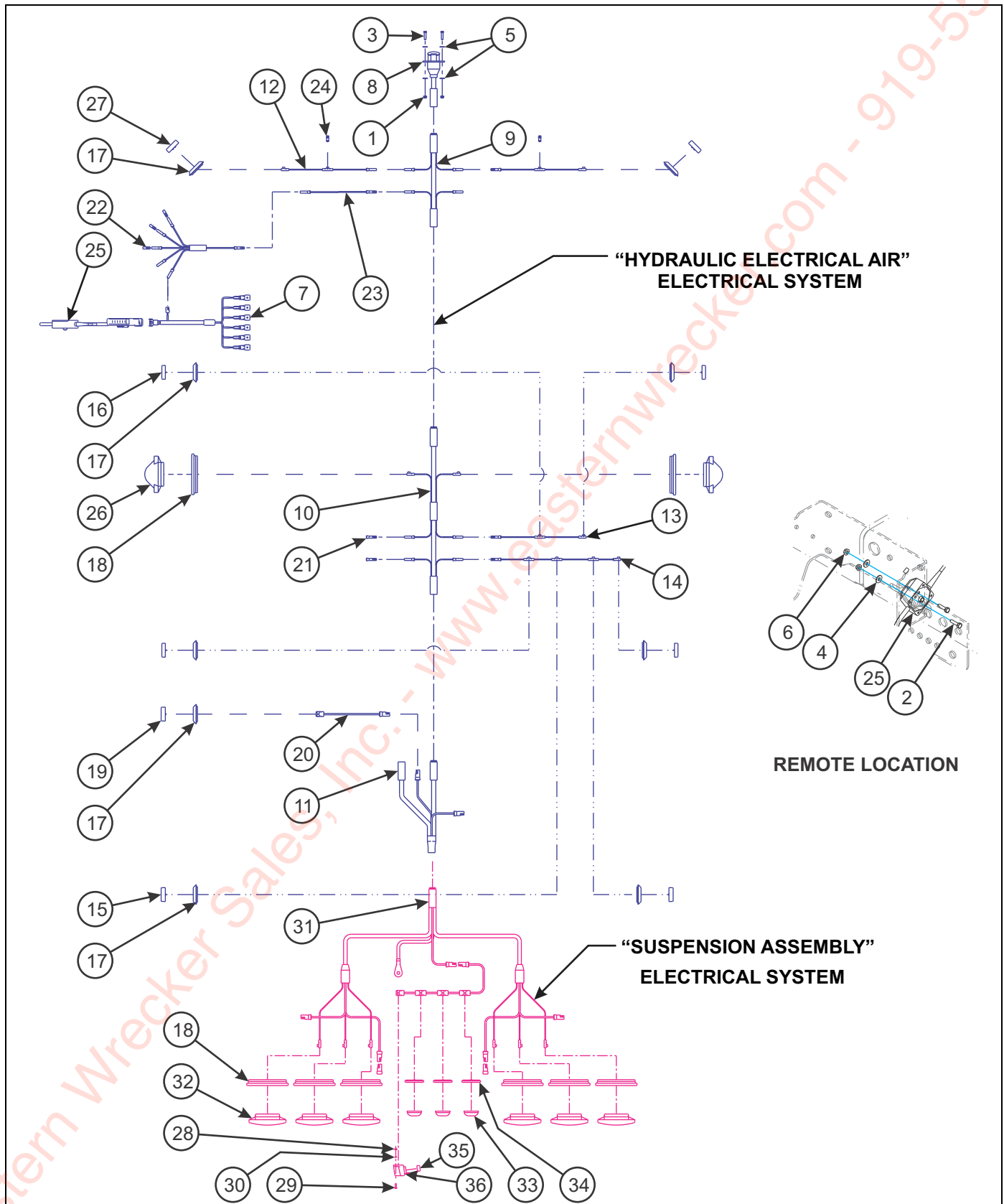
Figure 1-12: Electrical System
