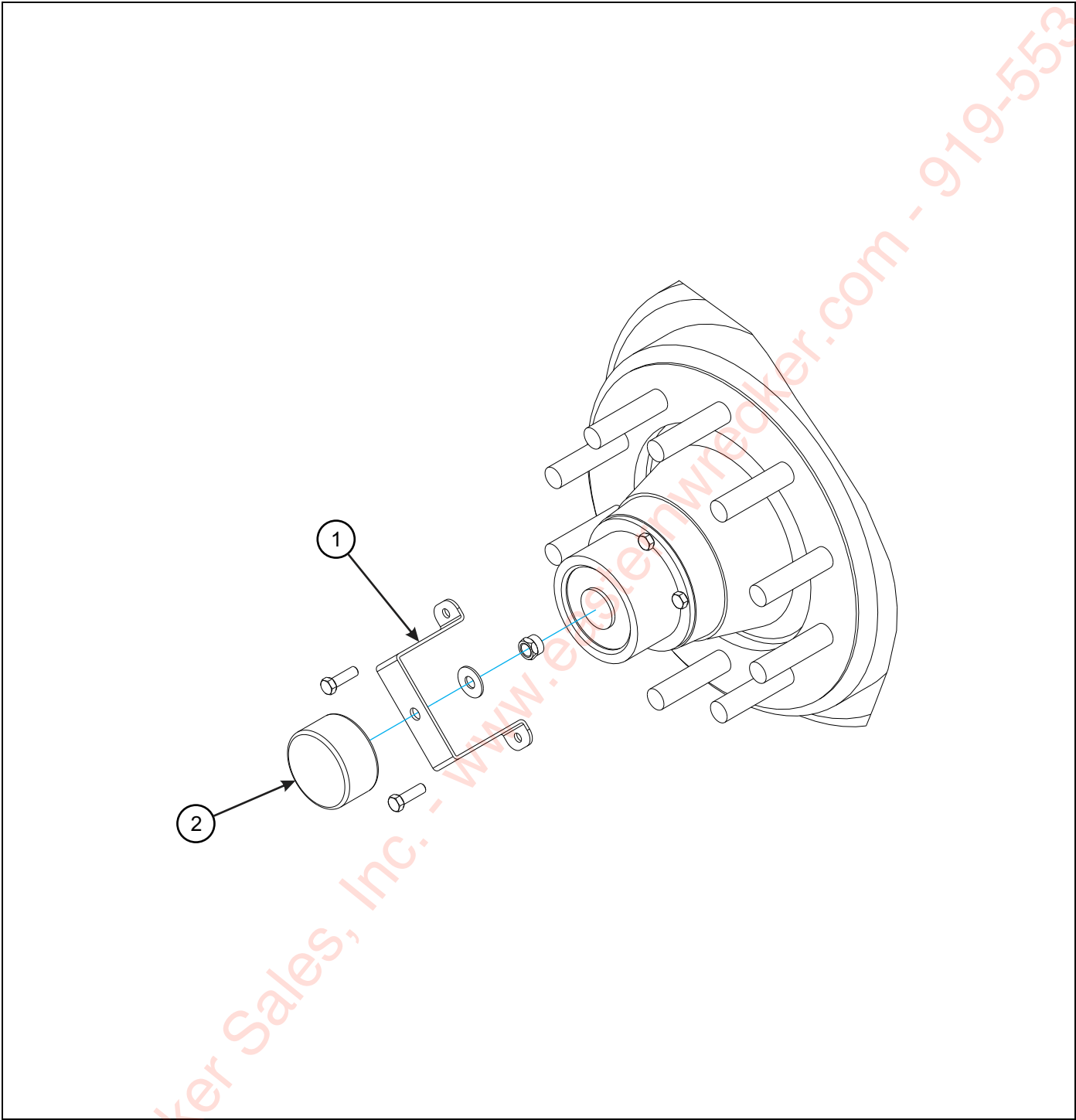
Figure 1-63: Hubodometer Installation- 255 Tires
