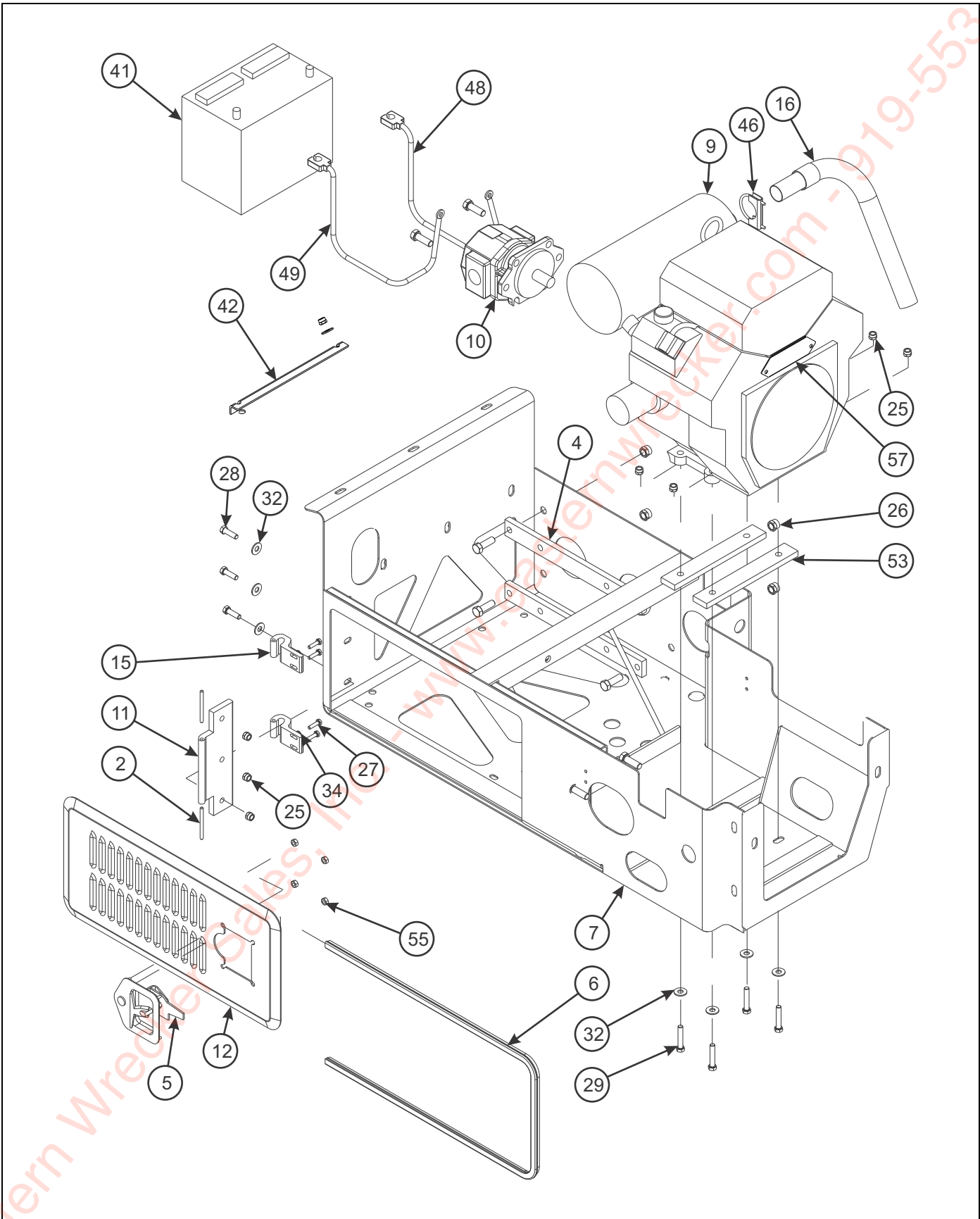
Figure 1-59: Engine - 27 HP Gas Package (1 of 2)
