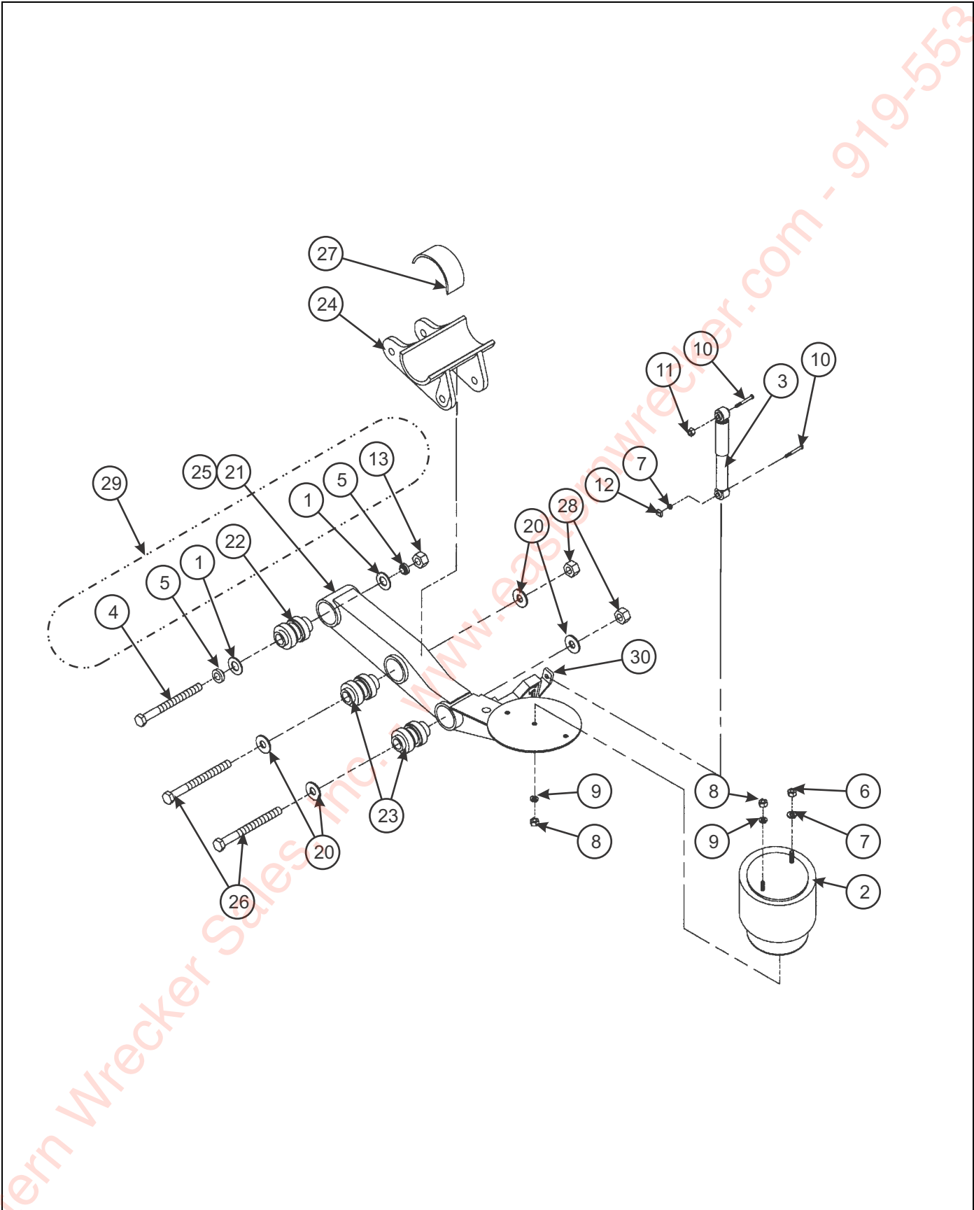
Figure 1-20: Suspension Hanger RLU-228
