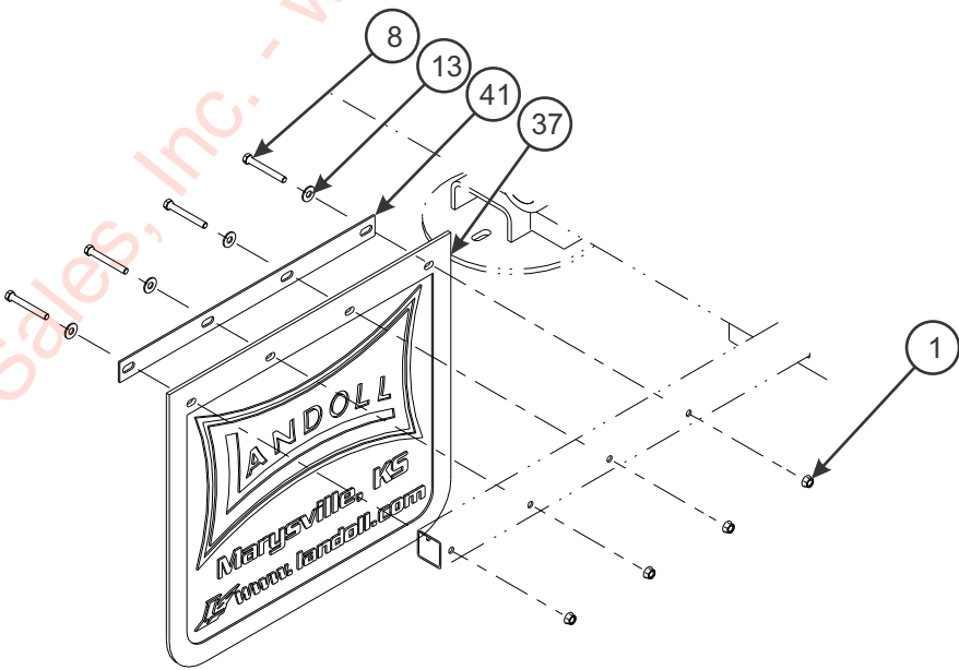
MUD FLAP ASSEMBLY
