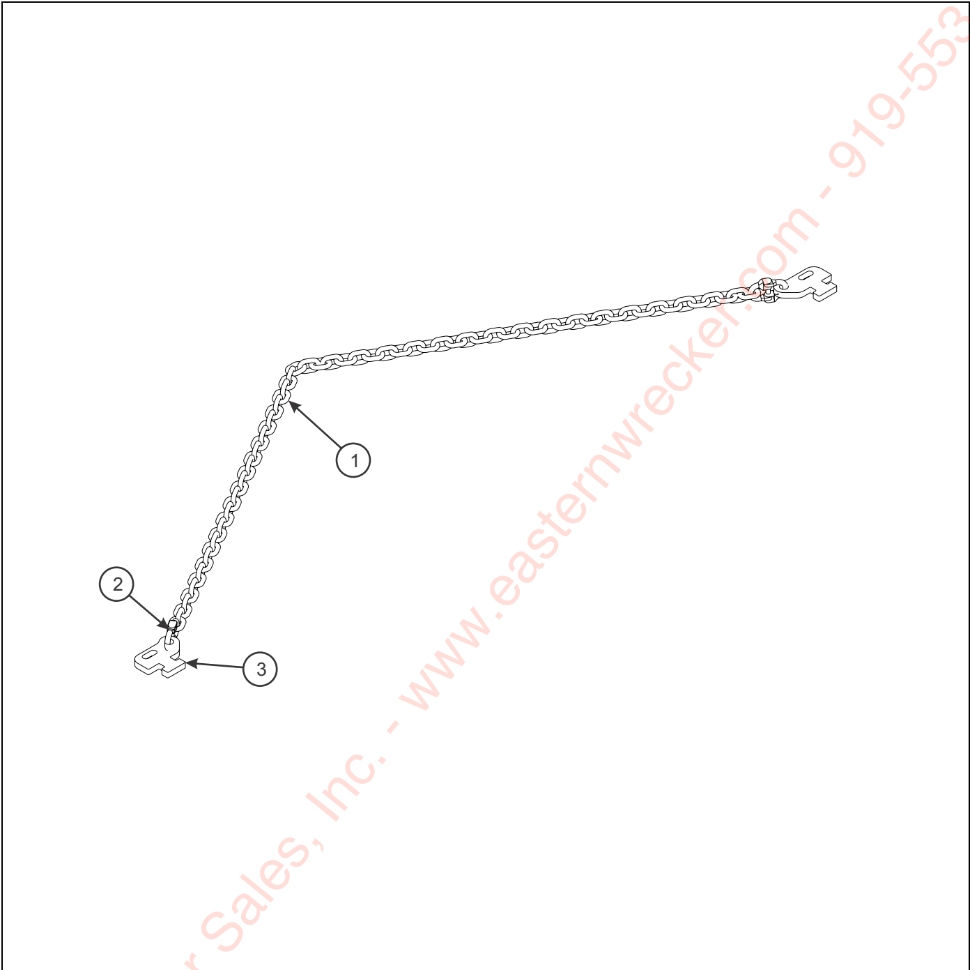
Figure 1-33: Chain Assembly -Container Load
