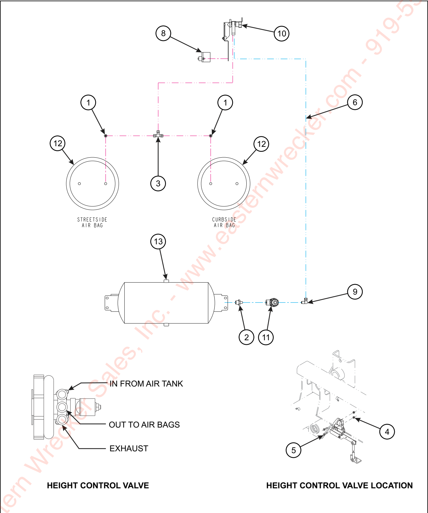
Figure 1-18: Air Ride Suspension
