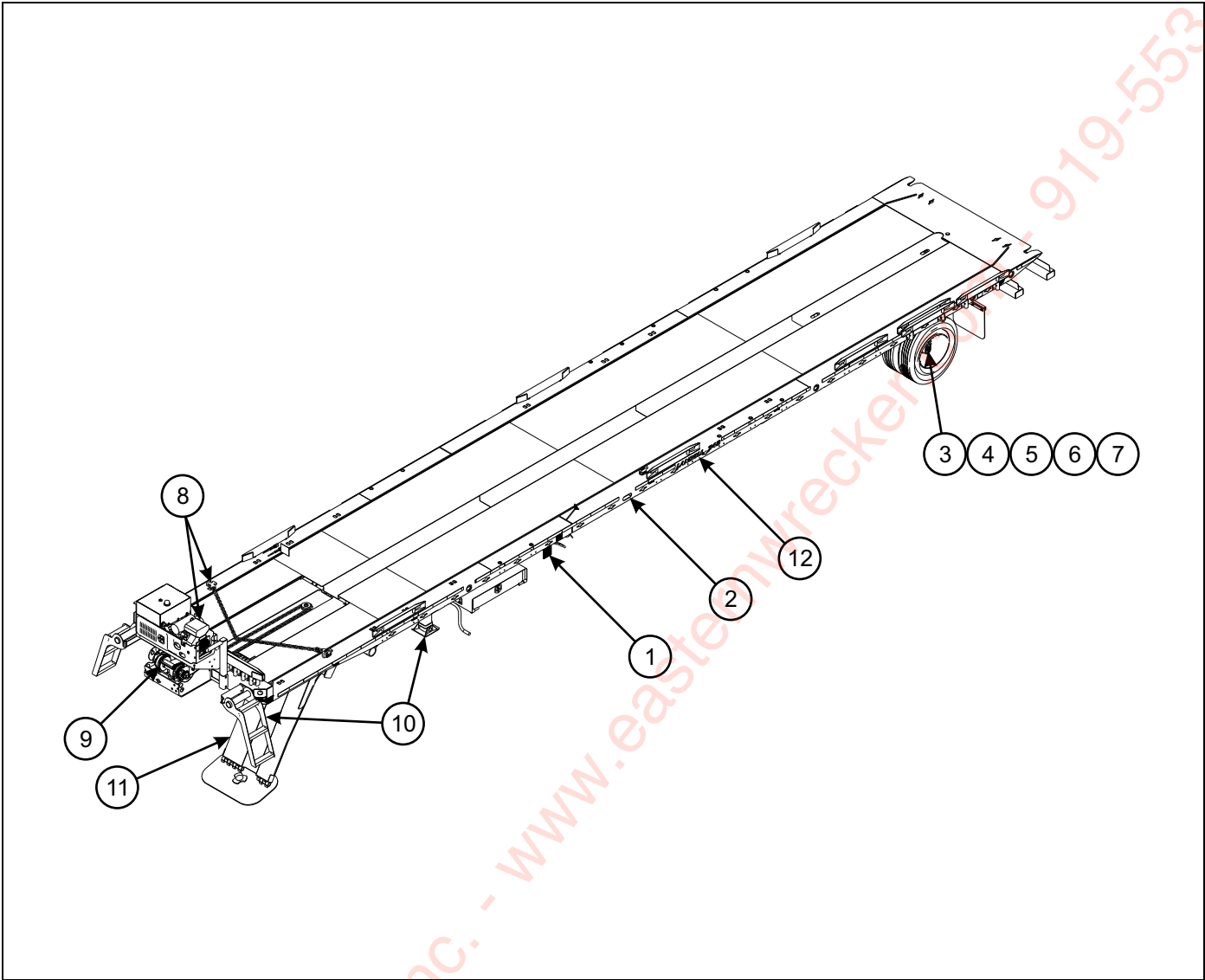
Figure 1-2: General Assembly
