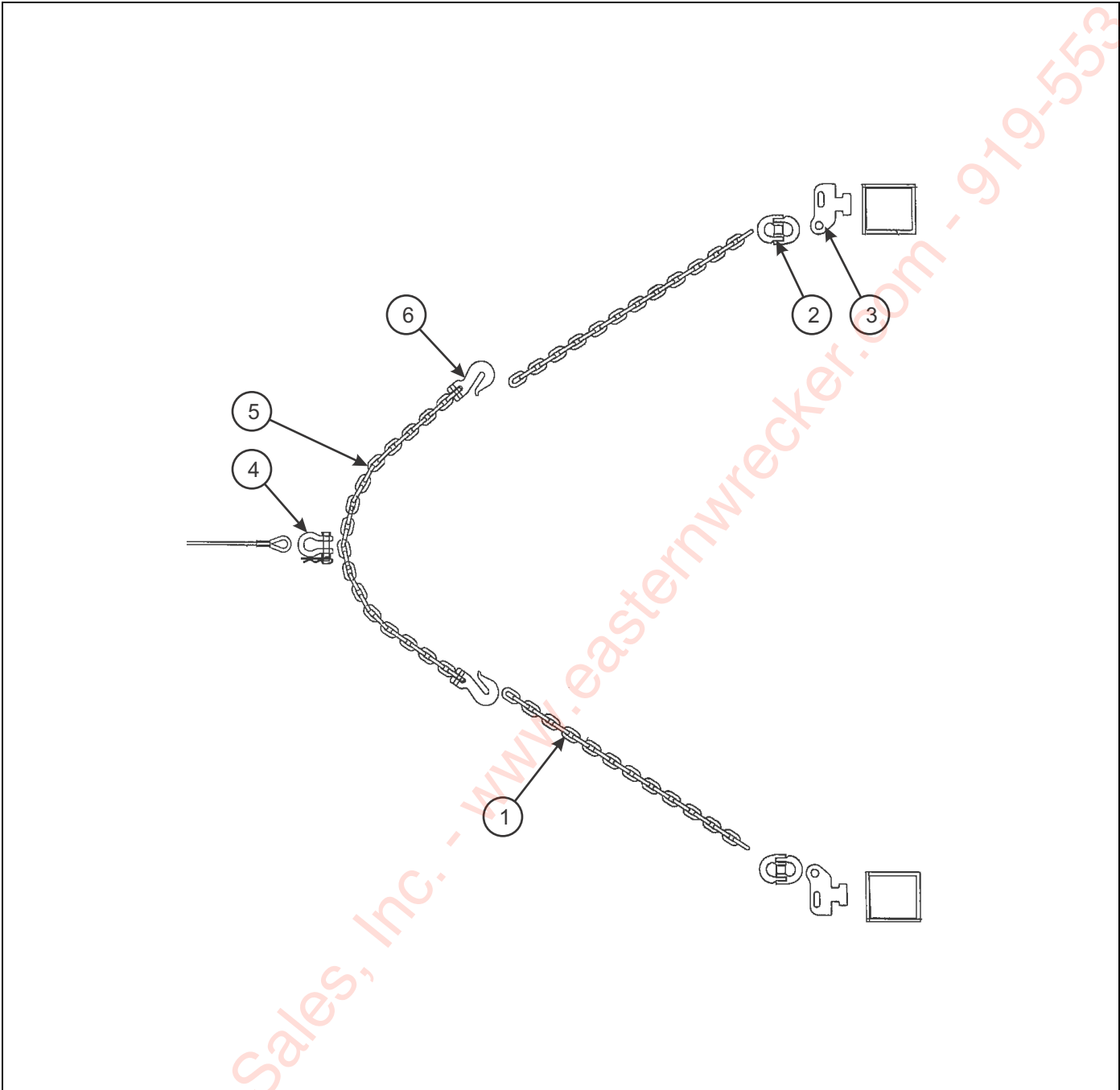
Figure 1-56: Container Chain and Bridle Assembly
