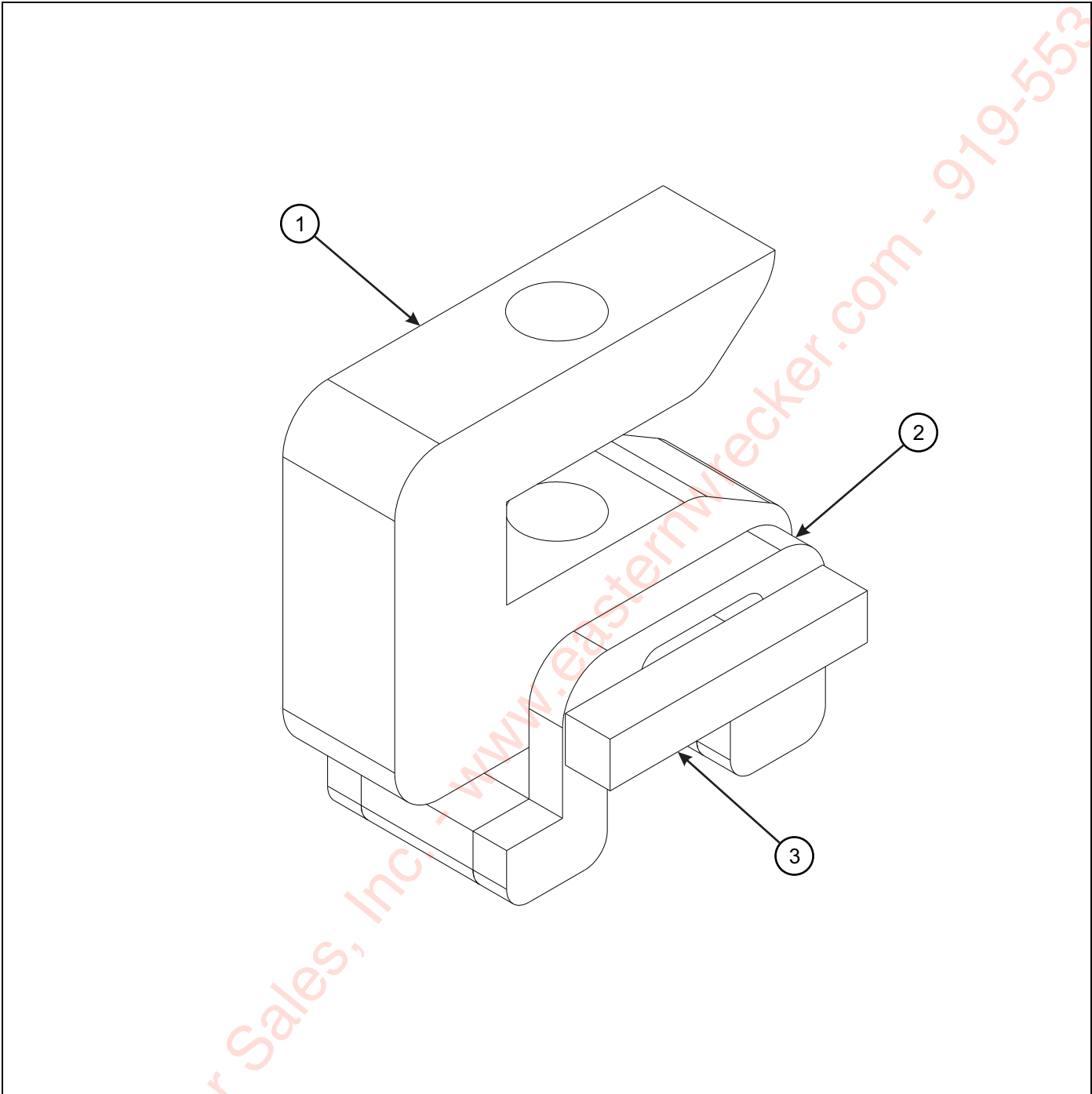
Figure 1-39: Container Stop - Front Weldment
