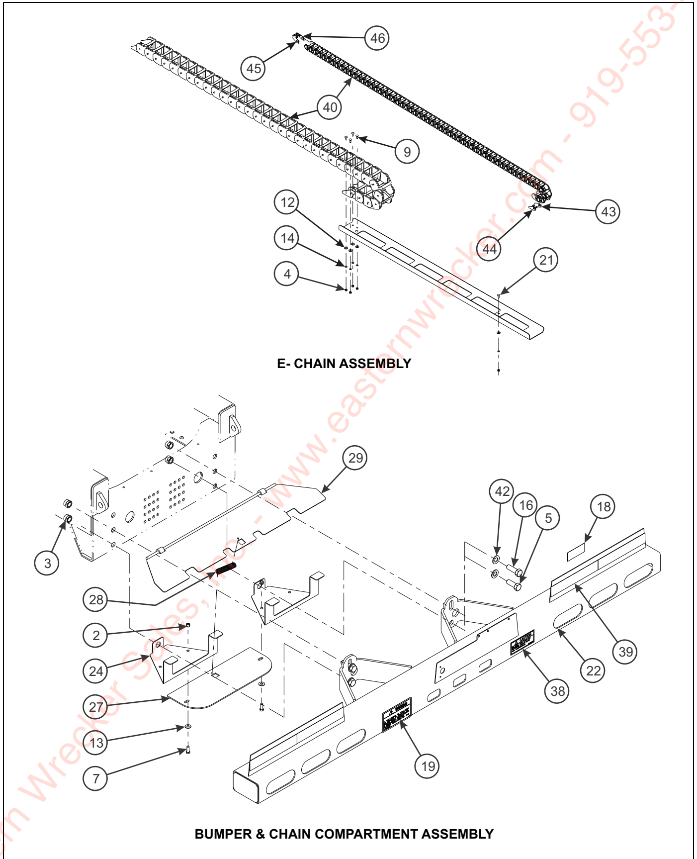
Figure 1-16: General Items (3 of 3)
