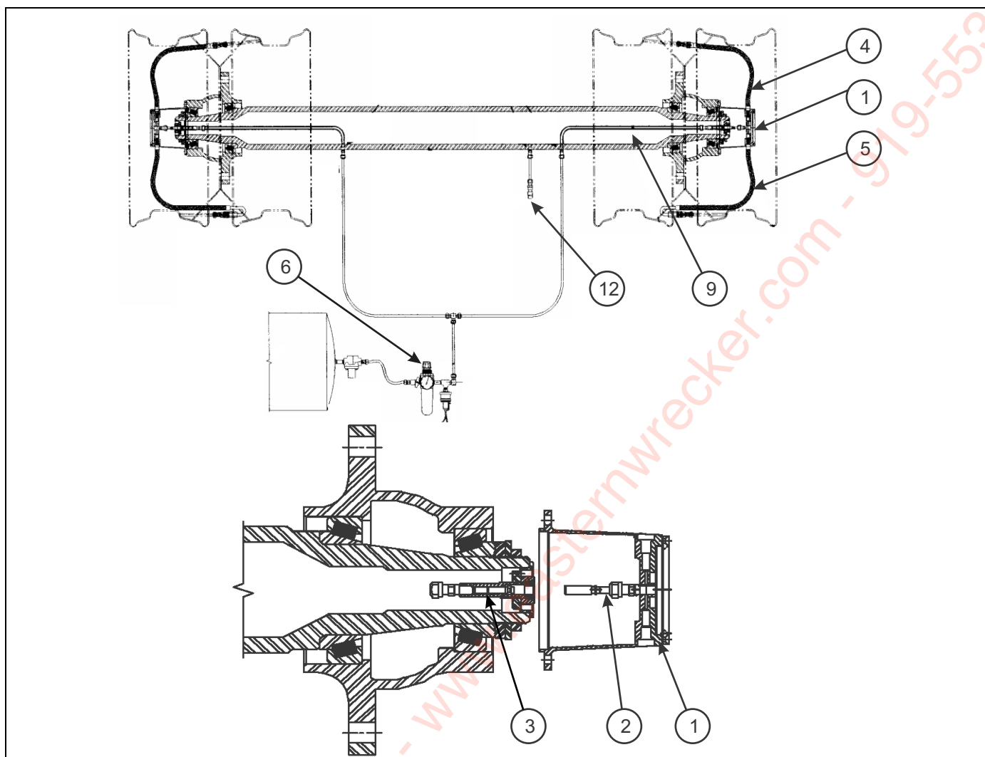
Figure 1-28: Tire Inflation System - 1AX (Option)
