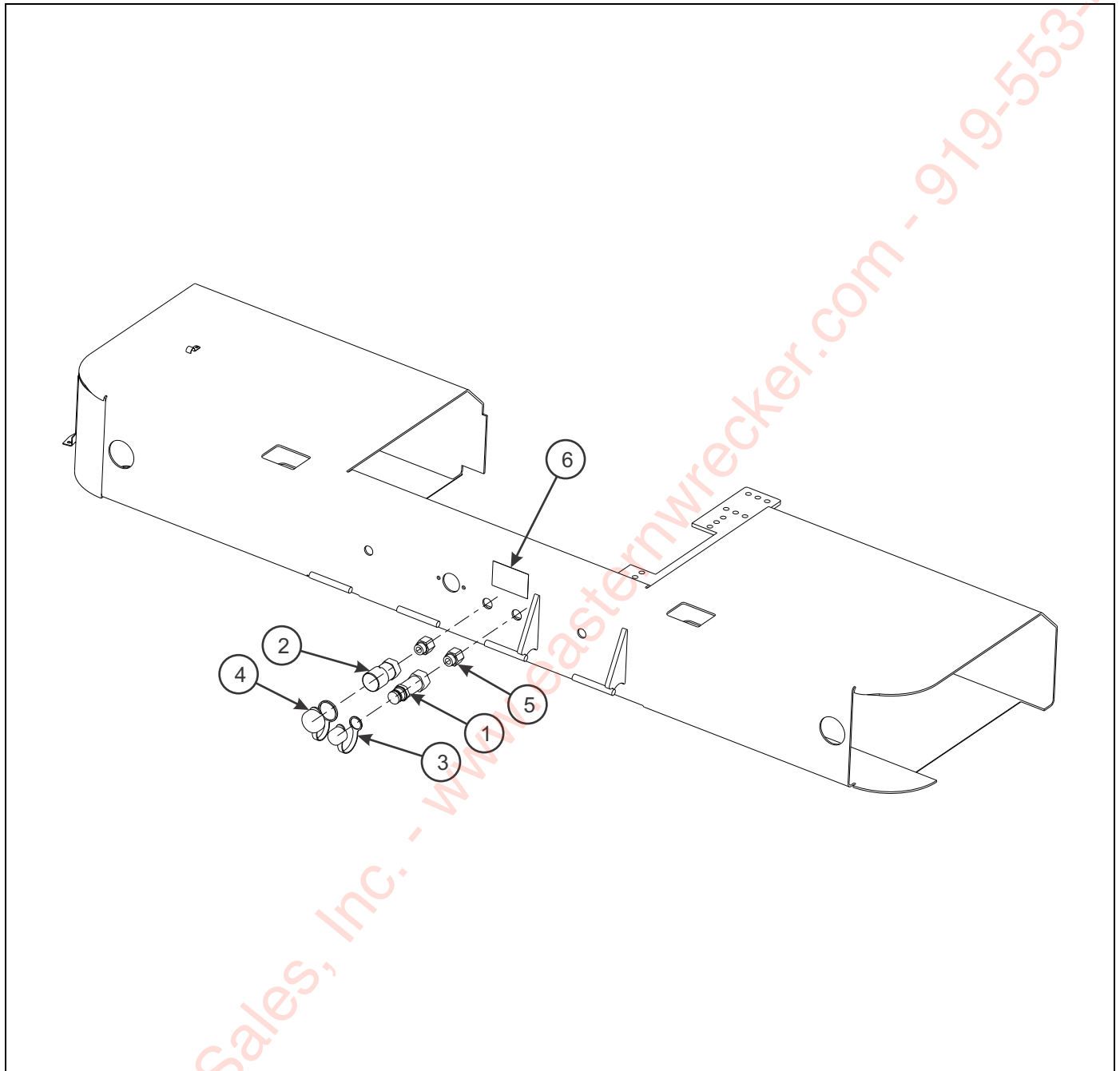
Figure 1-64: Hydraulic Conversion Kit - Ball to Flat
