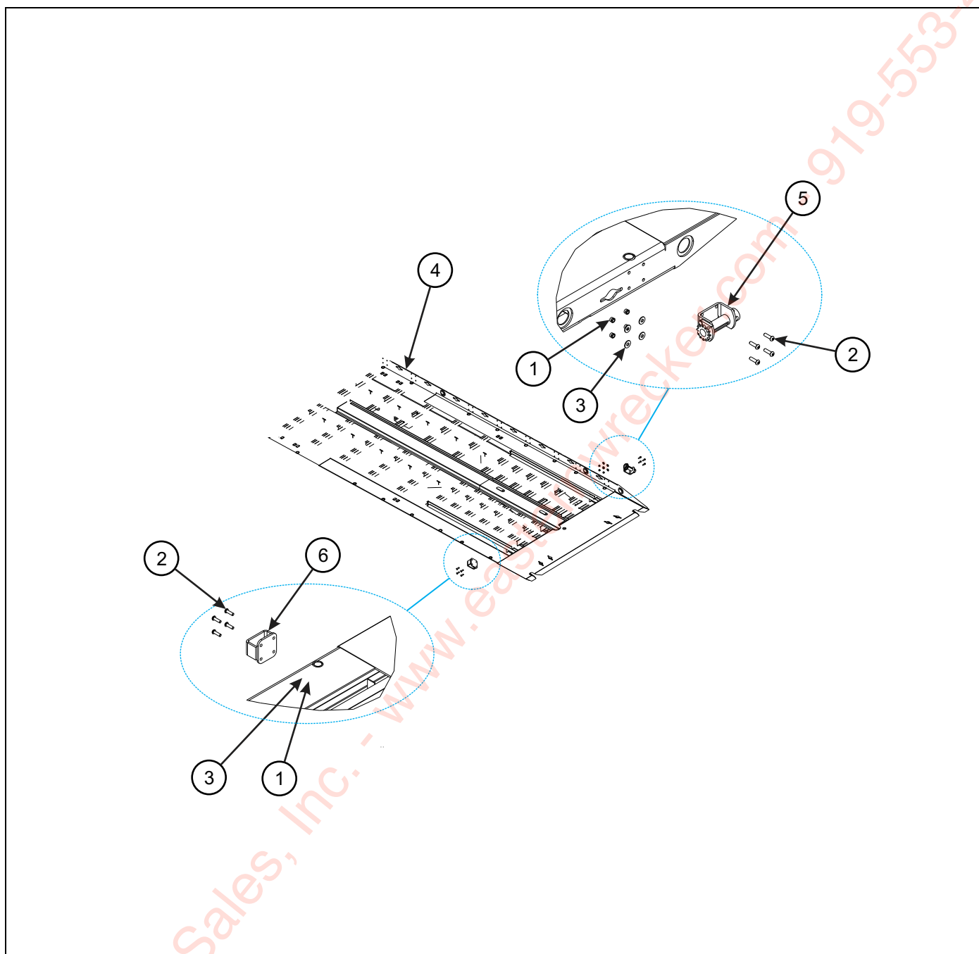
Figure 1-69: Strap Ratchet &amp; Hook Assembly
