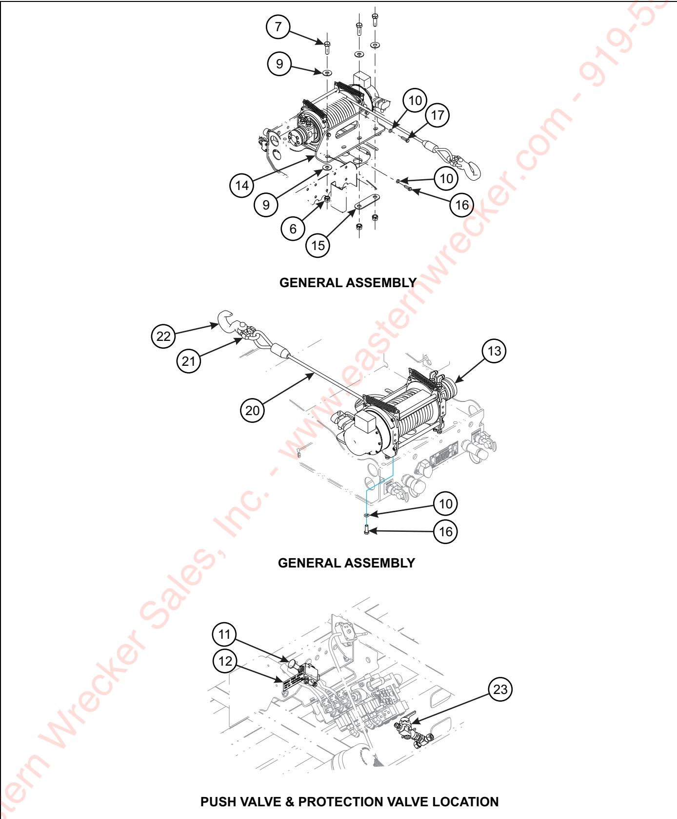
Figure 1-43: Winch Installation - 12K (WARN) (1 of 2)
