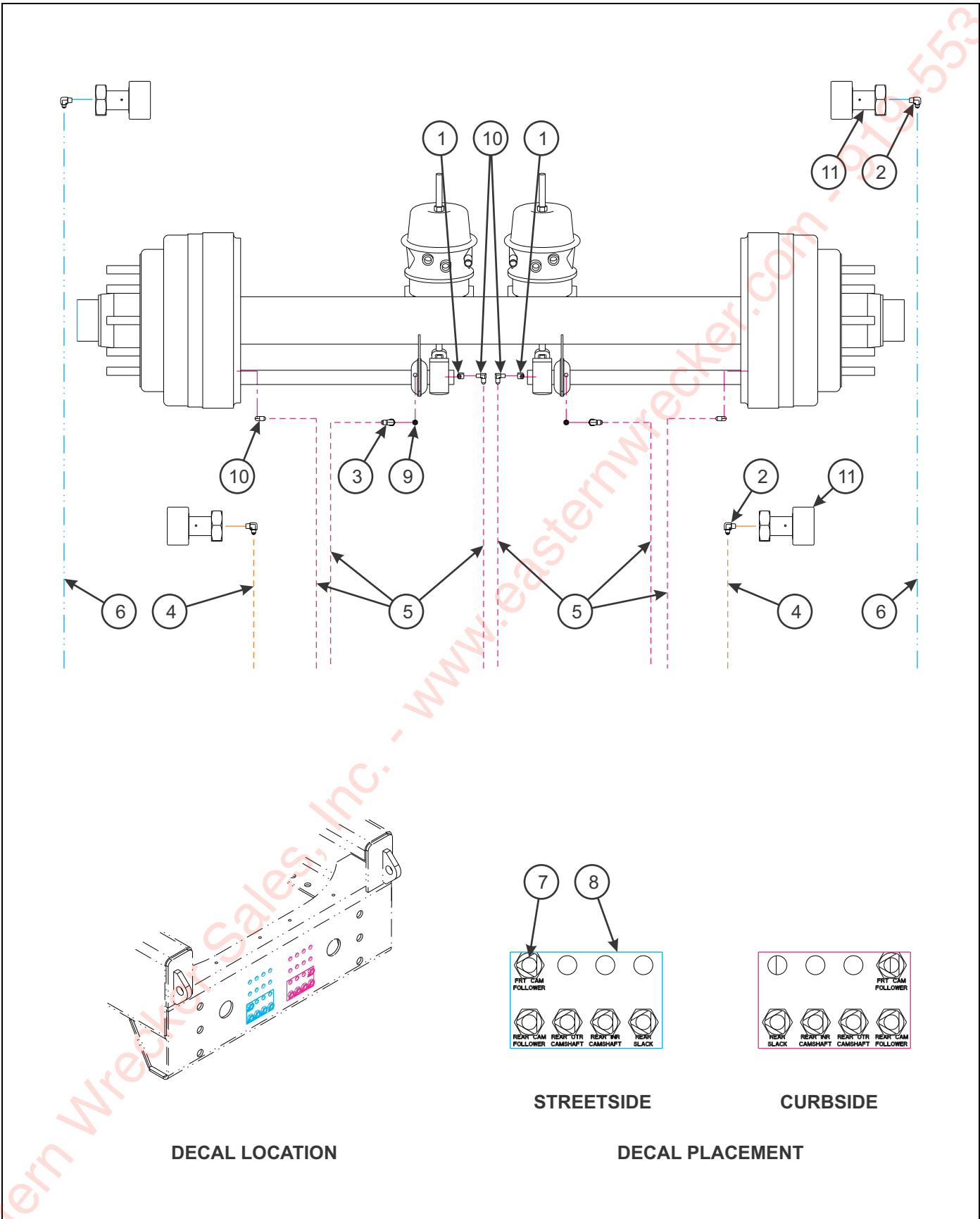
Figure 1-17: Grease System
