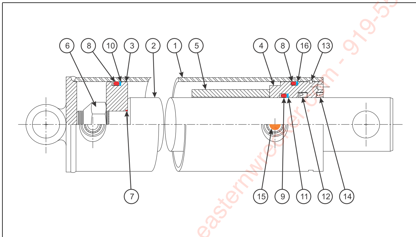
Figure 1-7: Hydraulic Cylinder - 4 x 126
