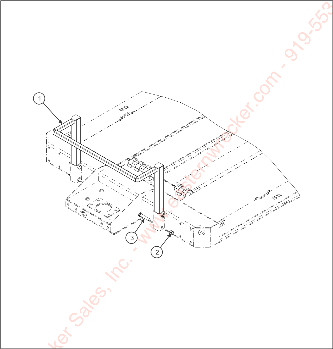
Figure 1-61: Front Grab Bar Assembly
