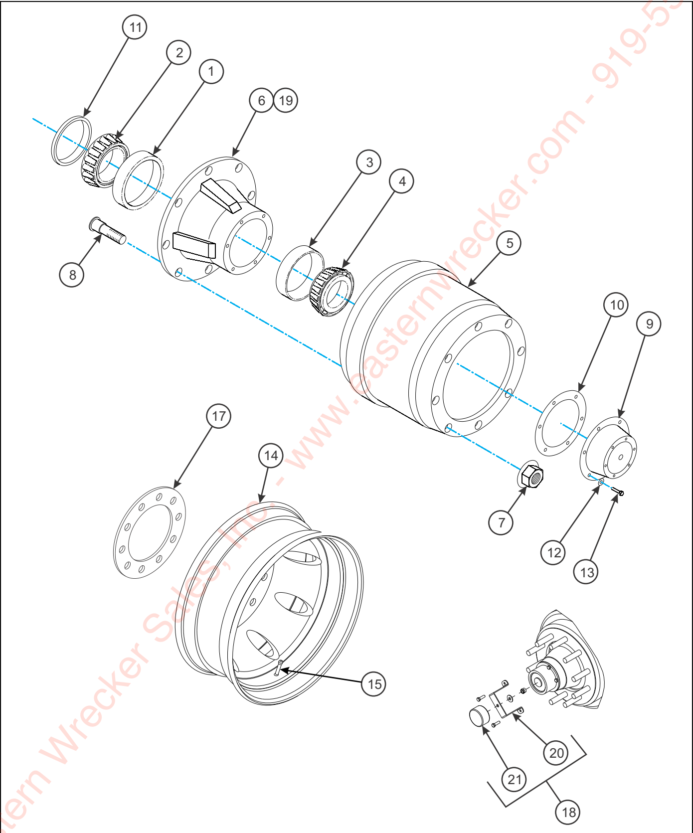
Figure 1-26: Outboard Pilot Mount Hub and Drum
