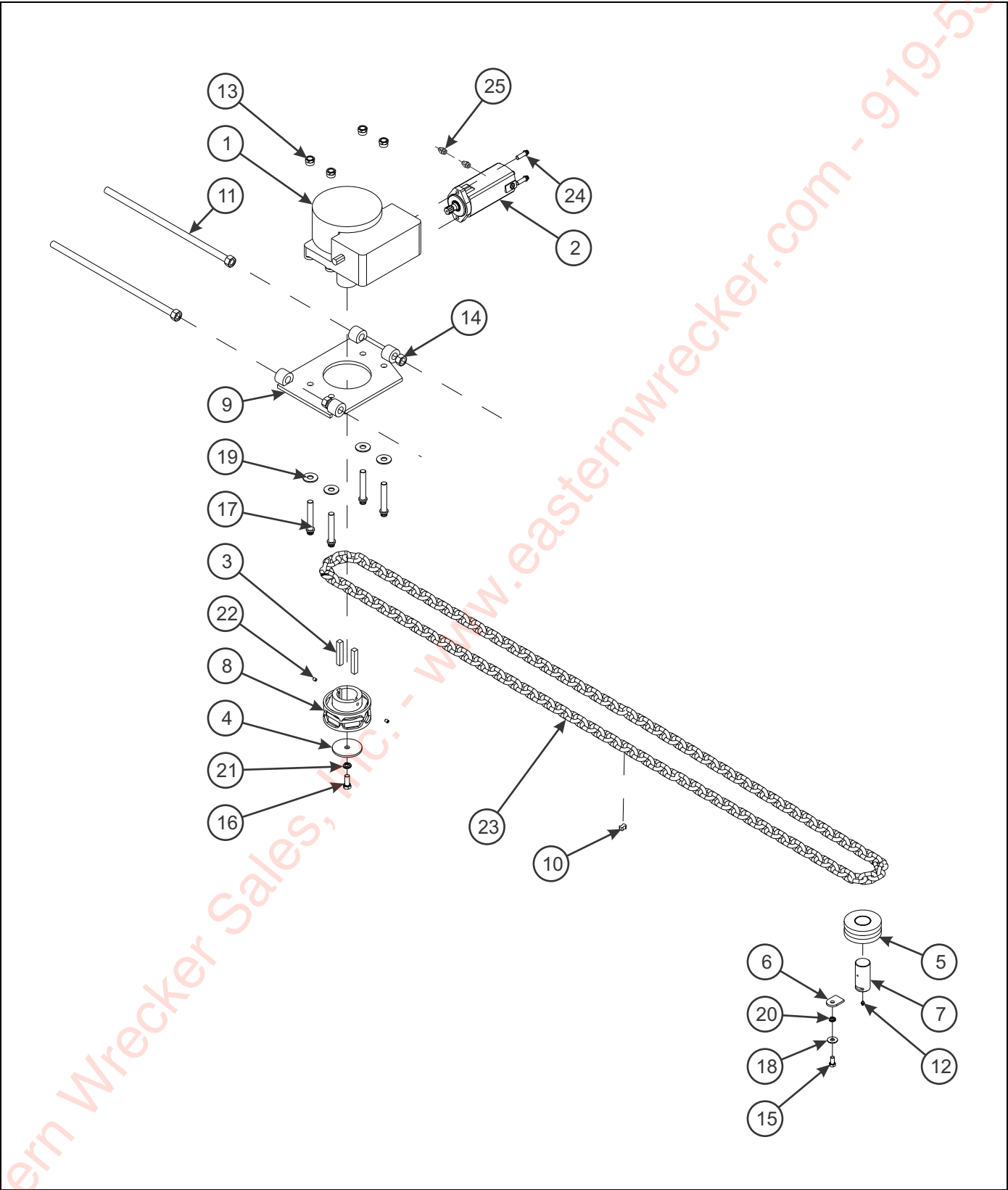
Figure 1-30: Gearbox Assembly
