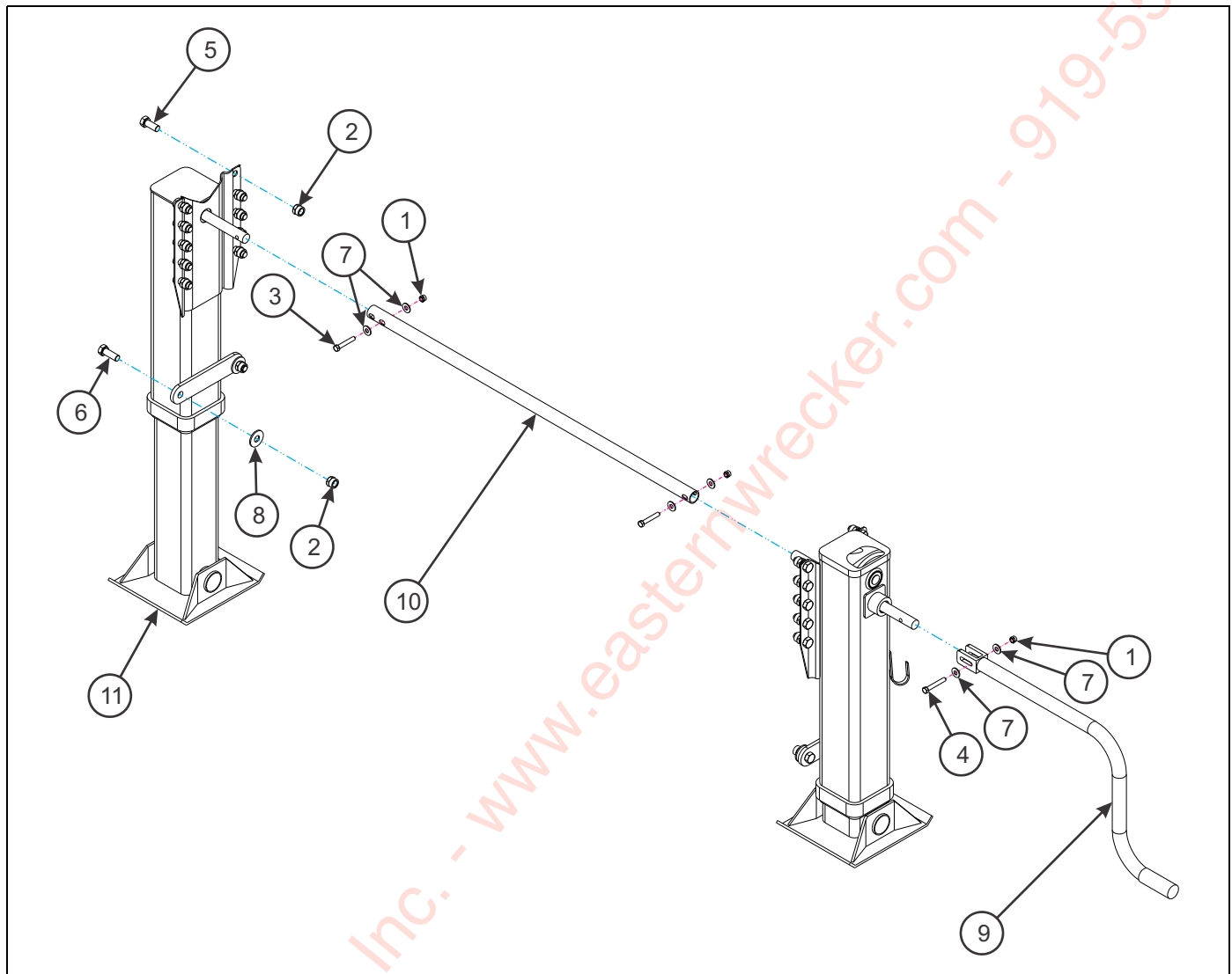
Figure 1-49: Landing Gear Installation - Jost 343
