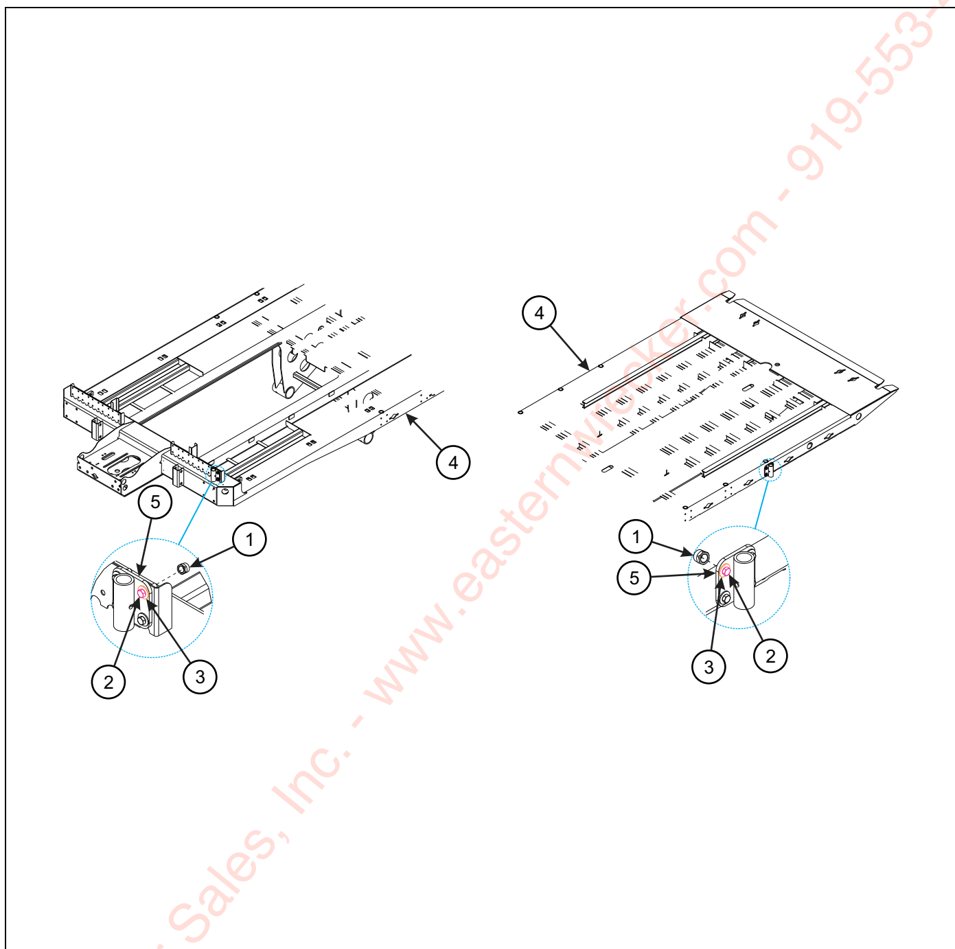
Figure 1-67: Side Guide - Anchor Pair
