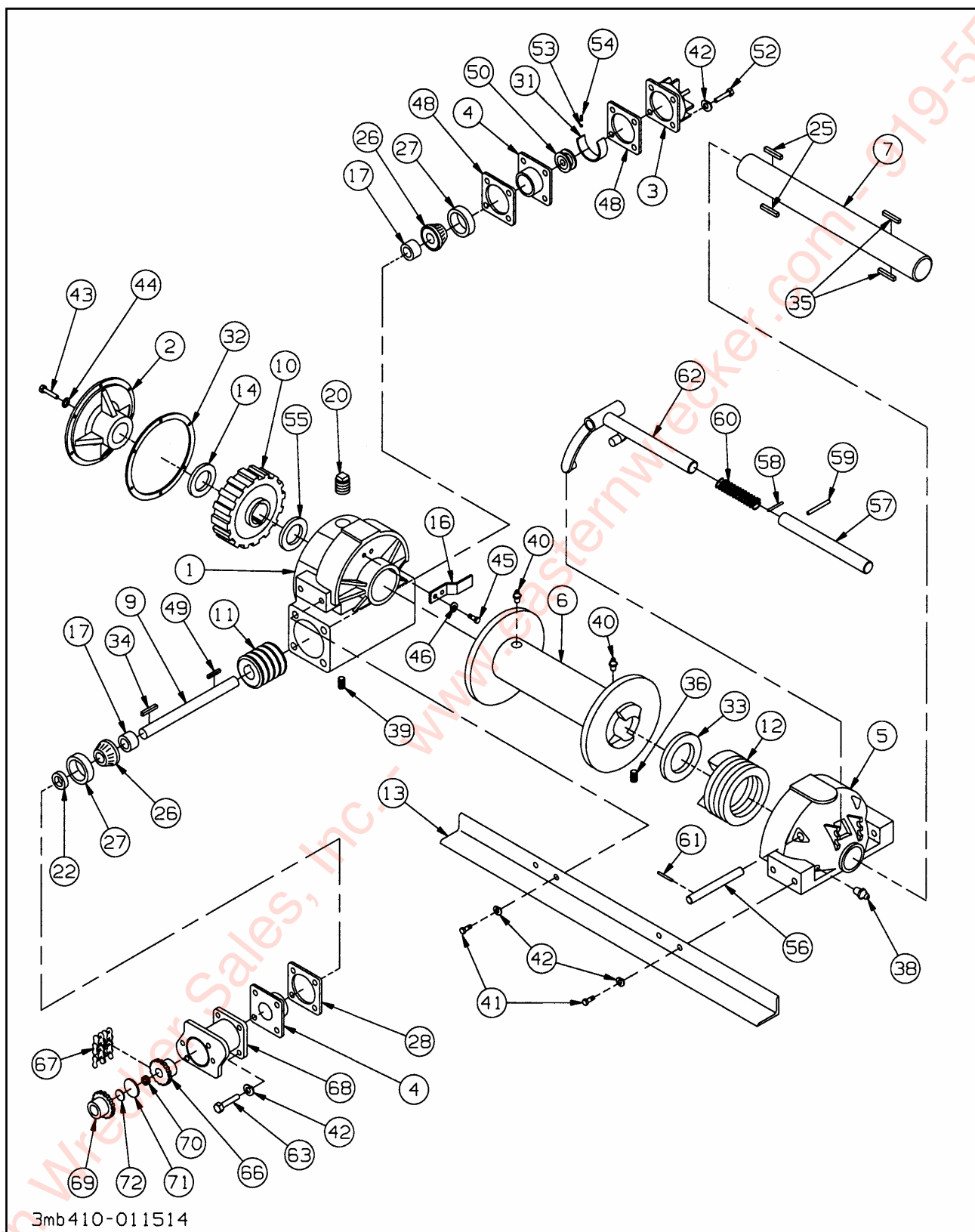
Figure 1-28 12,000 # Winch Items
