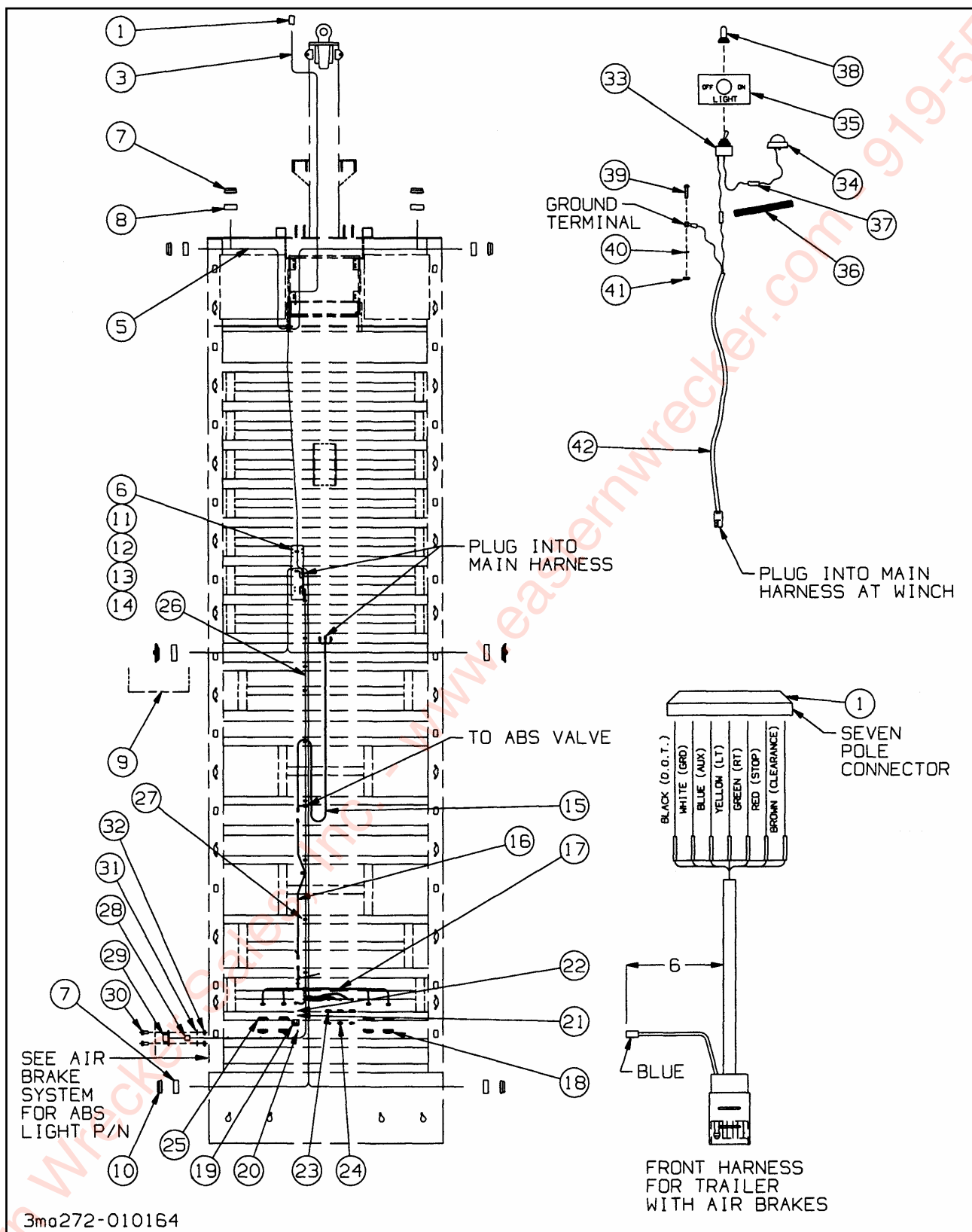
Figure 1-8 Electrical Assembly
