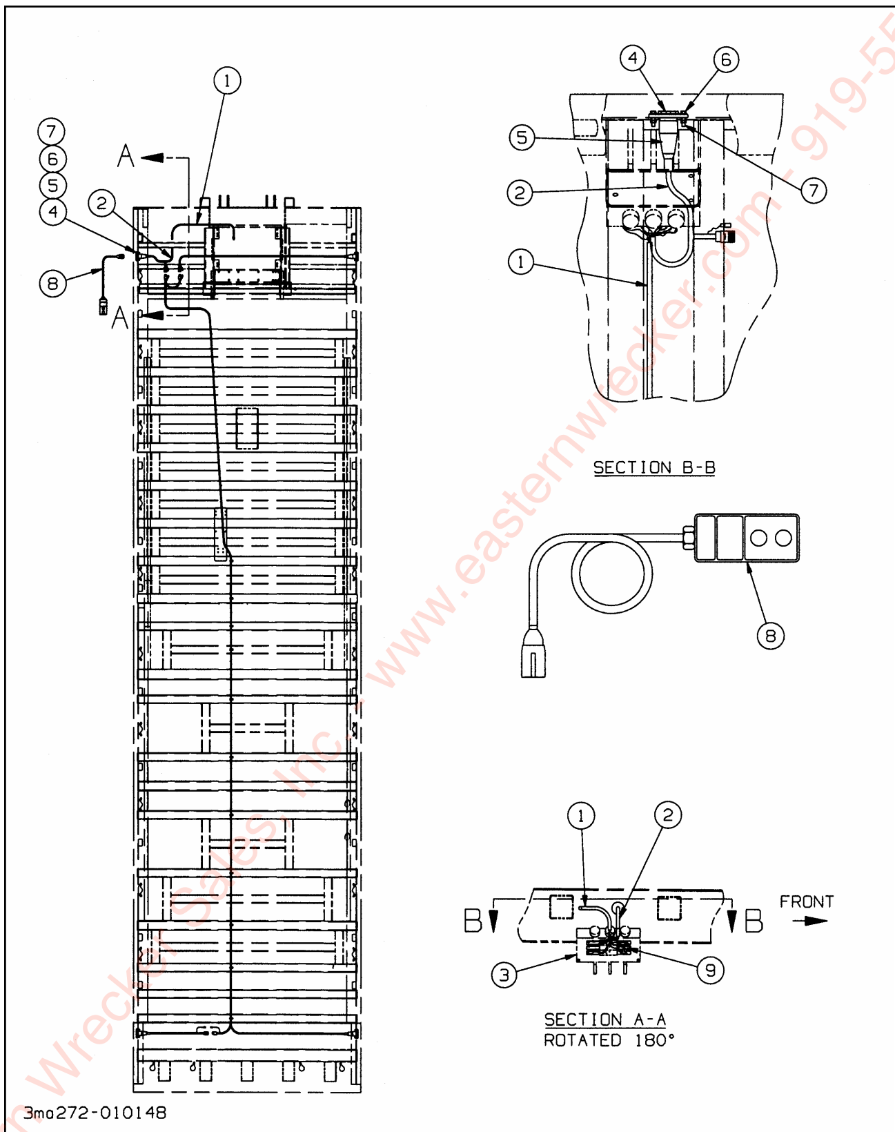
Figure 1-10 Electrical Installation - Remote Control (Option)
