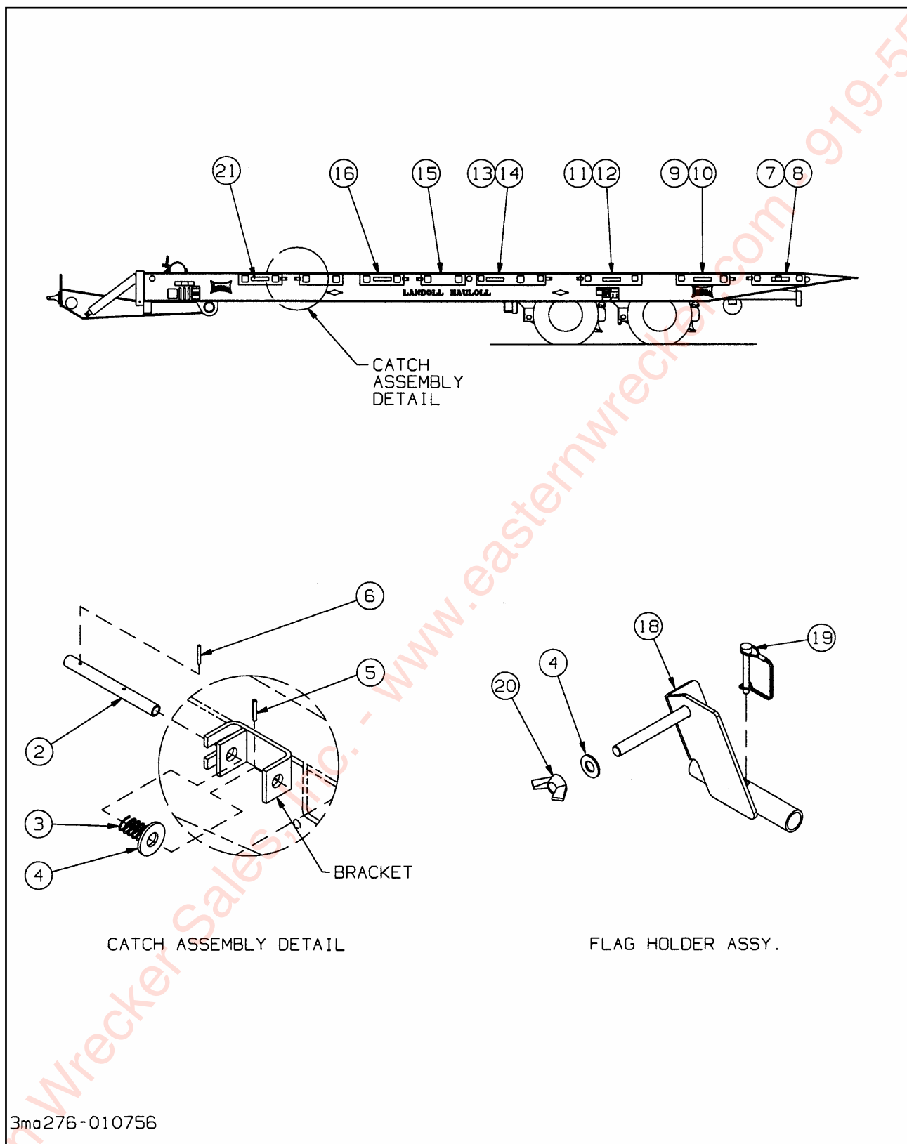
Figure 1-37 Extension Installation
