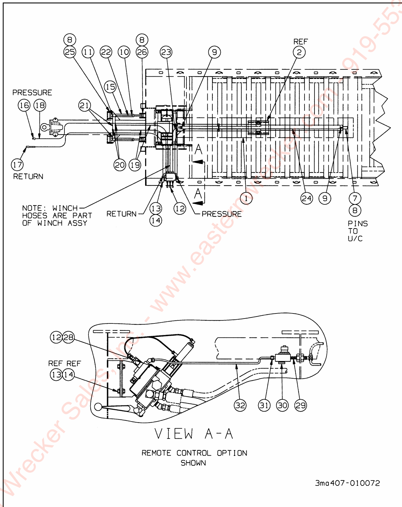
Figure 1-4 Hydraulic Assembly
