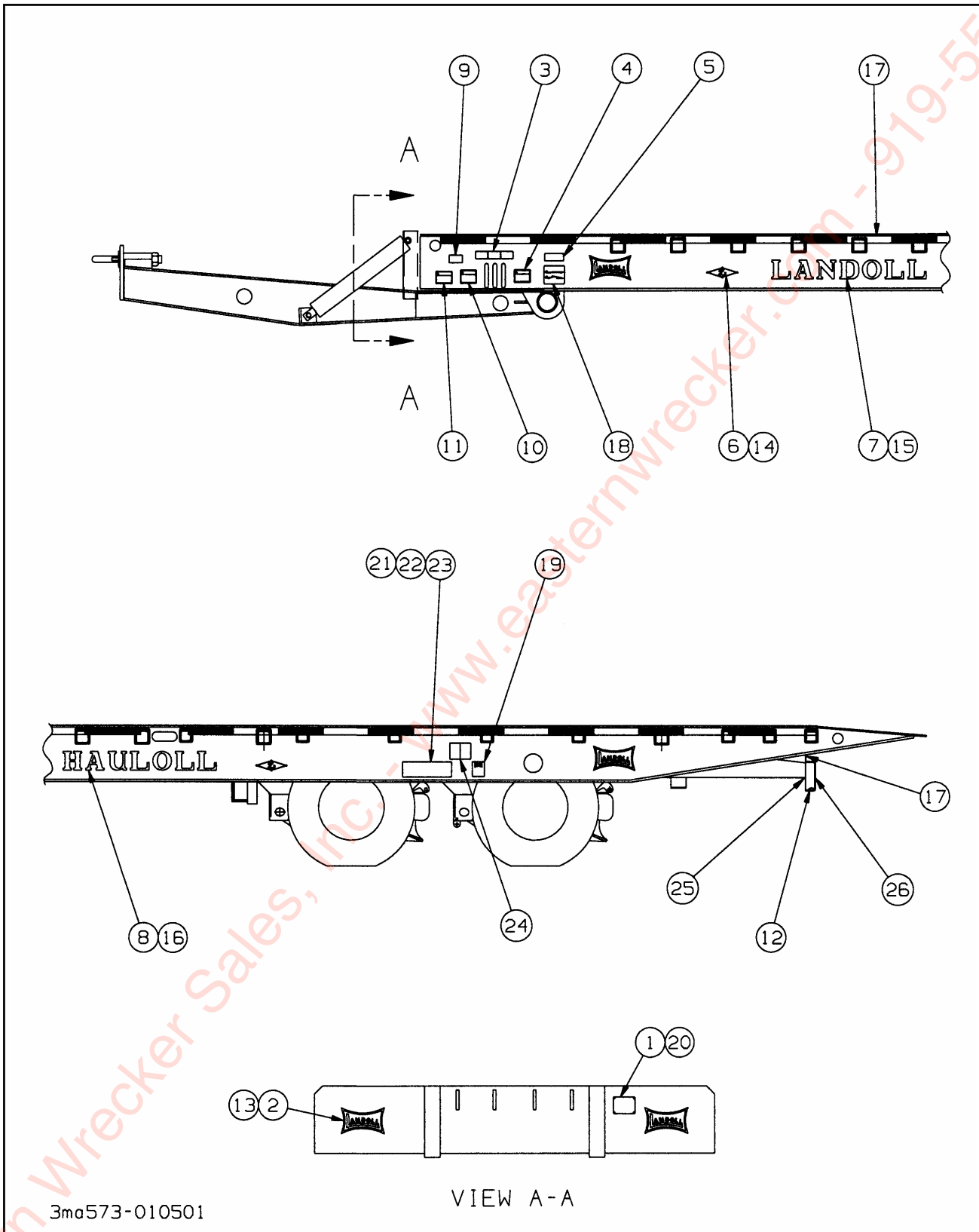
Figure 1-36 Decal Installation
