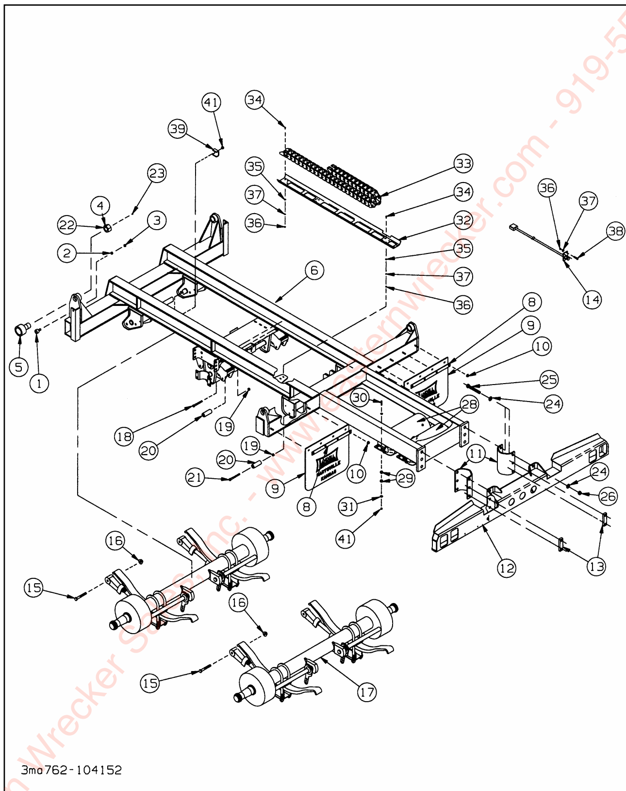
Figure 1-12 Undercarriage Assembly - Spring Ride
