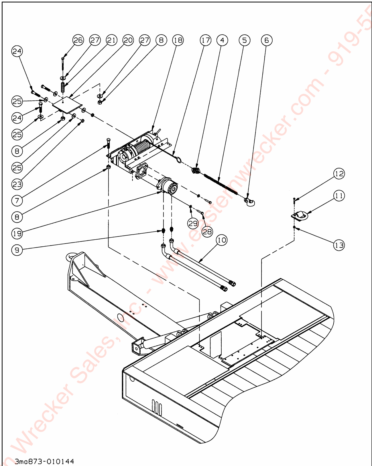
Figure 1-27 Winch Installation
