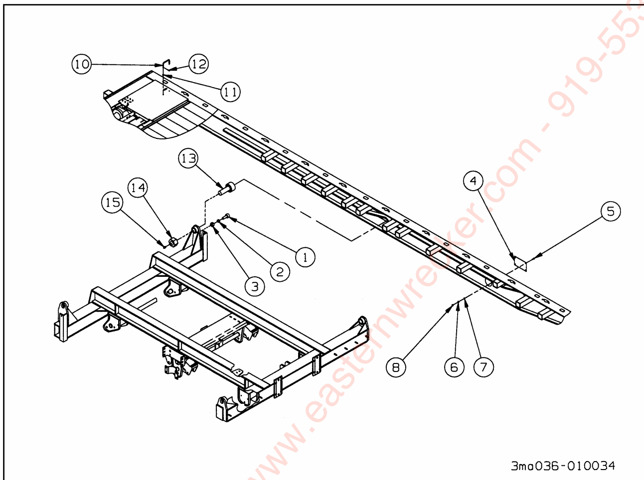
Figure 1-31 Attachments
