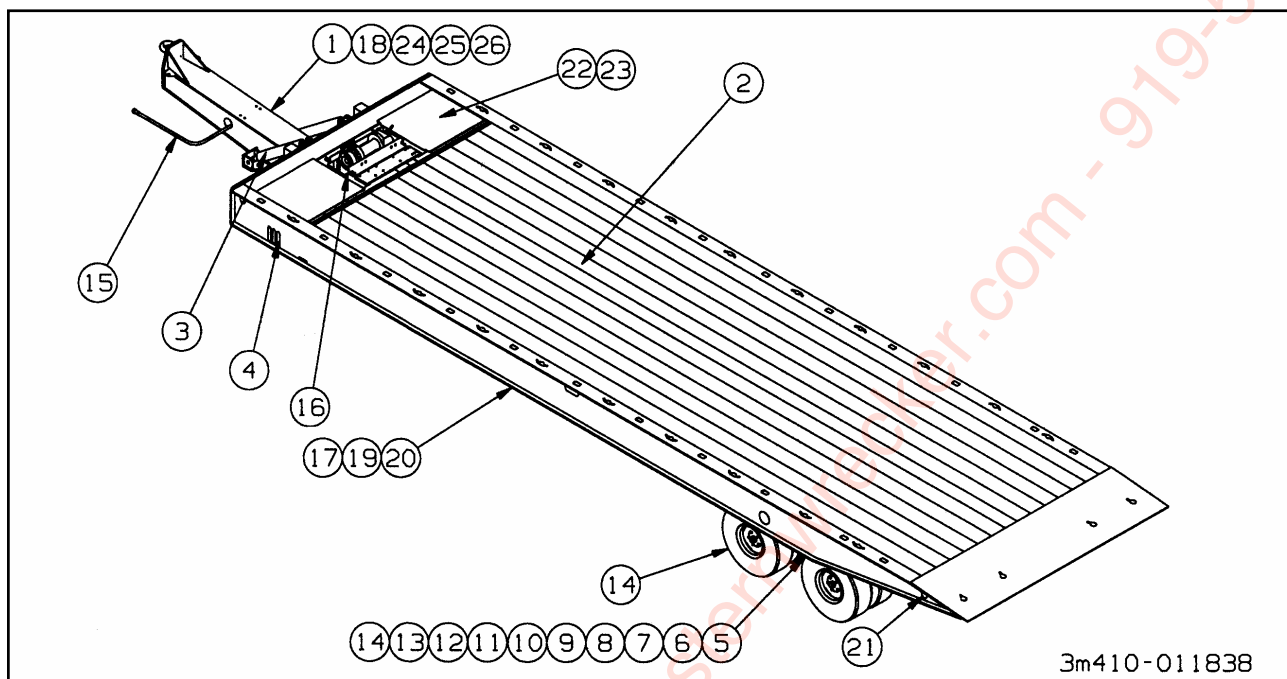
Figure 1-1 General Assembly
