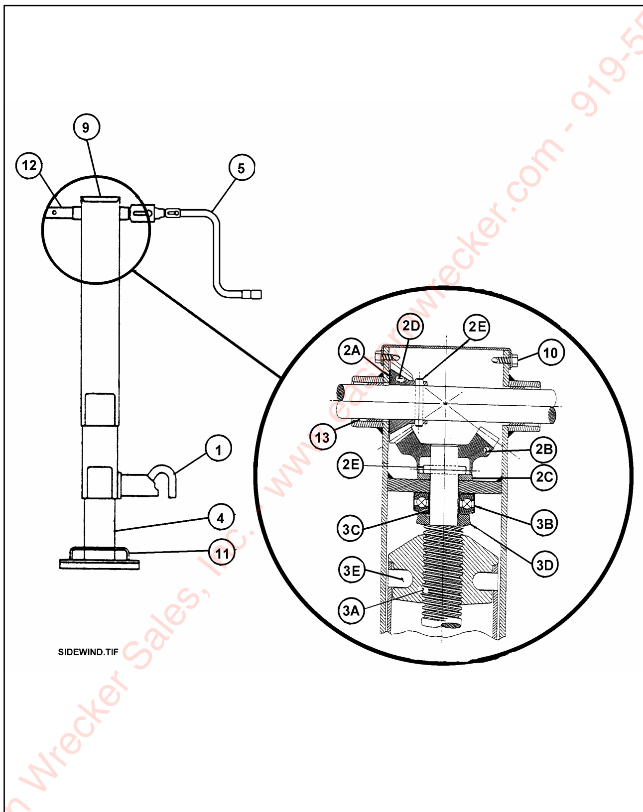
Figure 1-45 Jackstand Assembly
