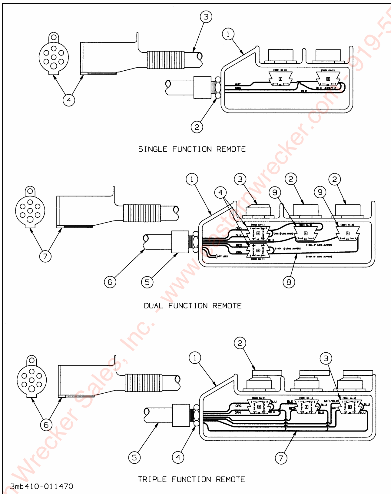
Figure 1-38 Wired Remote Control
