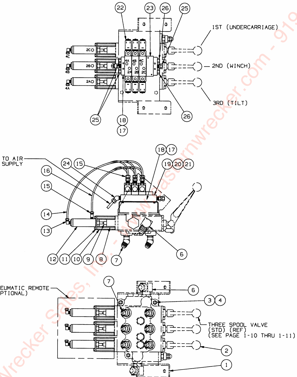
Figure 1-6 Valve Assembly - 3 Spool
