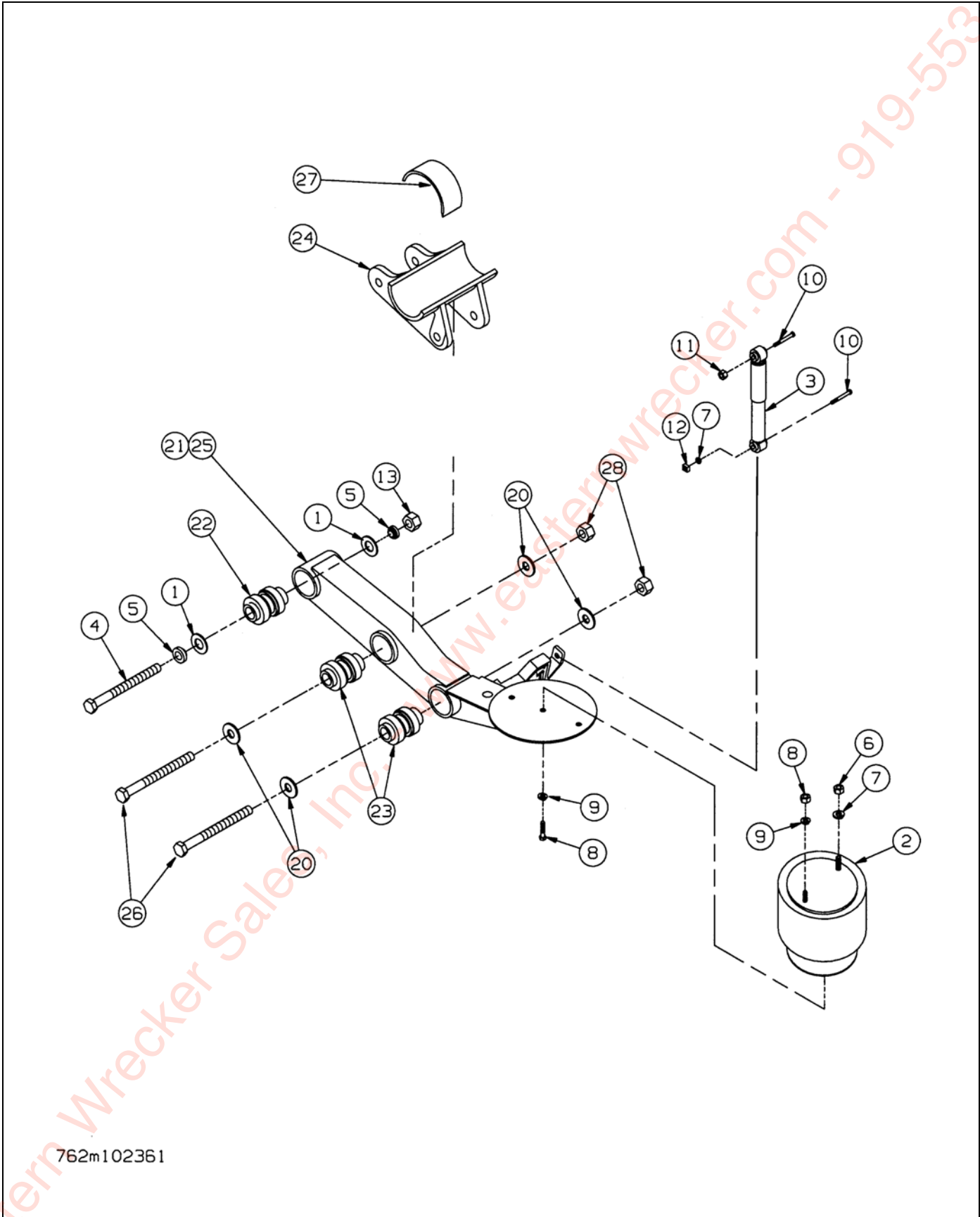
Figure 2-21: Suspension Hanger Assembly RLU-228
