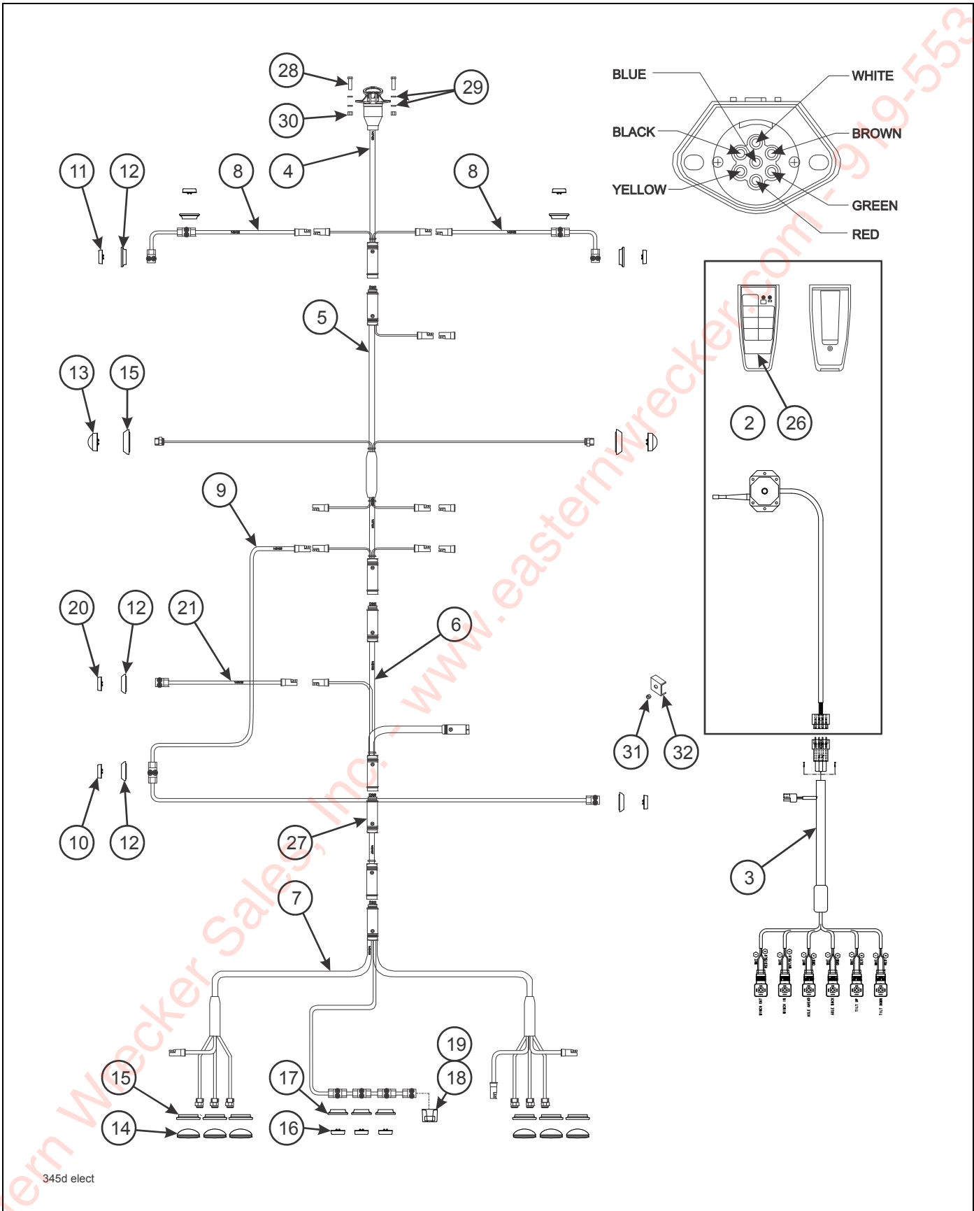
Figure 2-12: Electrical Assembly
