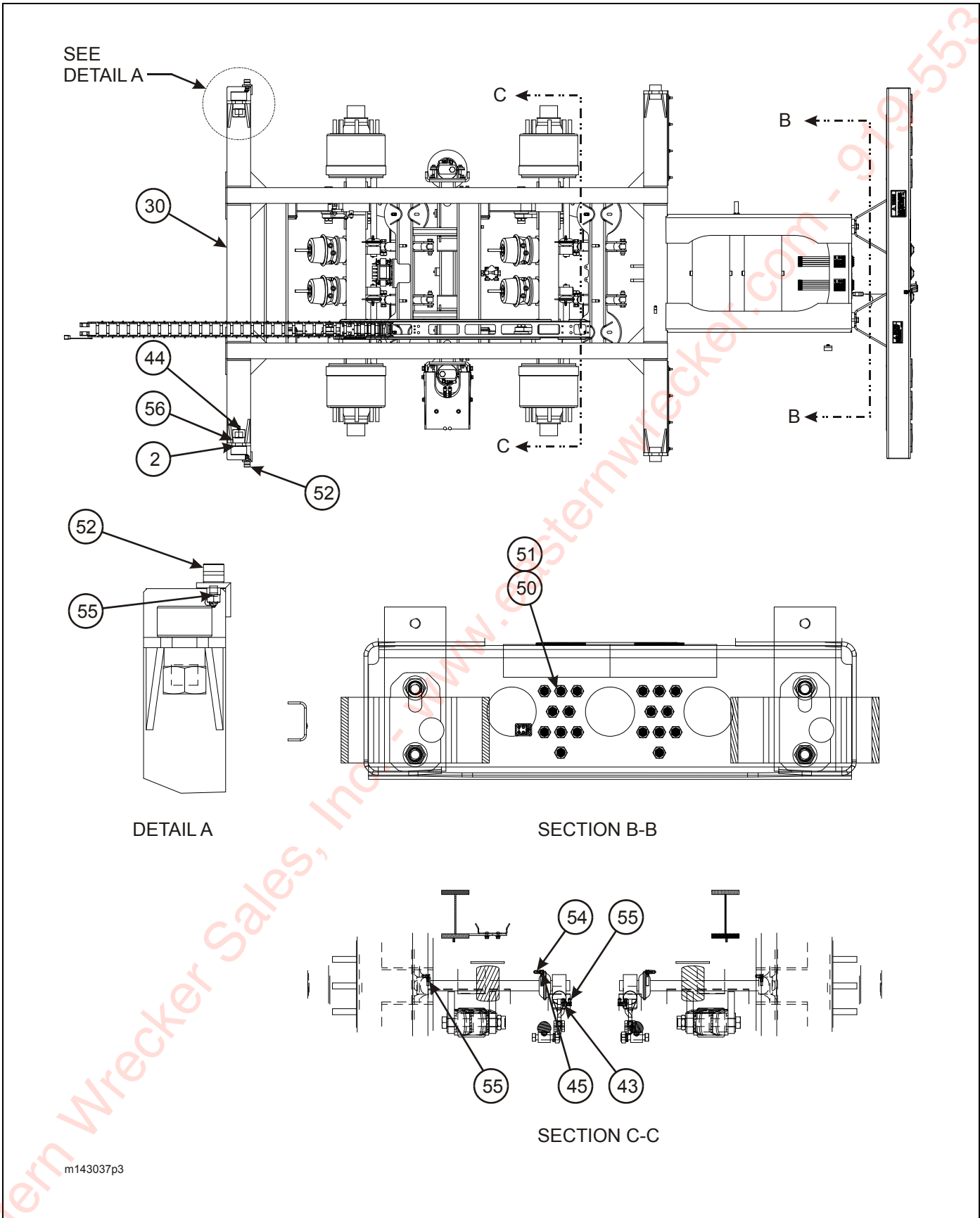
Figure 2-18: Undercarriage Assembly - Air Ride (3 of 3)
