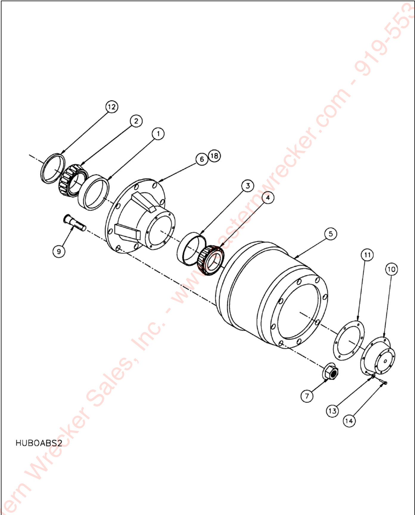
Figure 2-24: Outboard Hub and Drum Assembly
