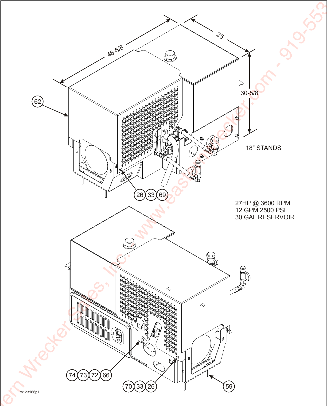
Figure 2-34: Engine Drive, 20 HP (1 of 4)
