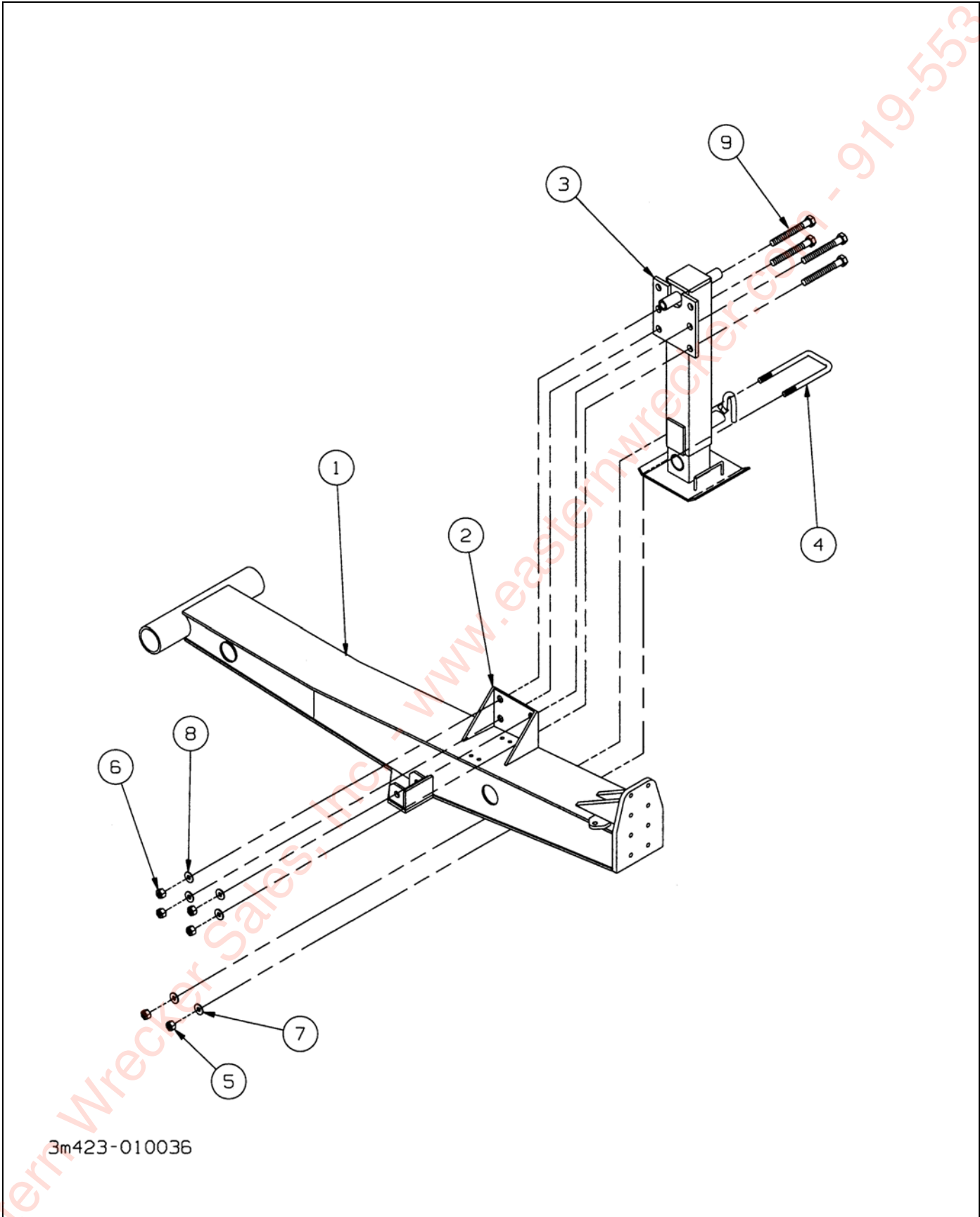
Figure 2-48: Jack Installation, 12K, 5" Hitch Dock Level w/ E-Chain
