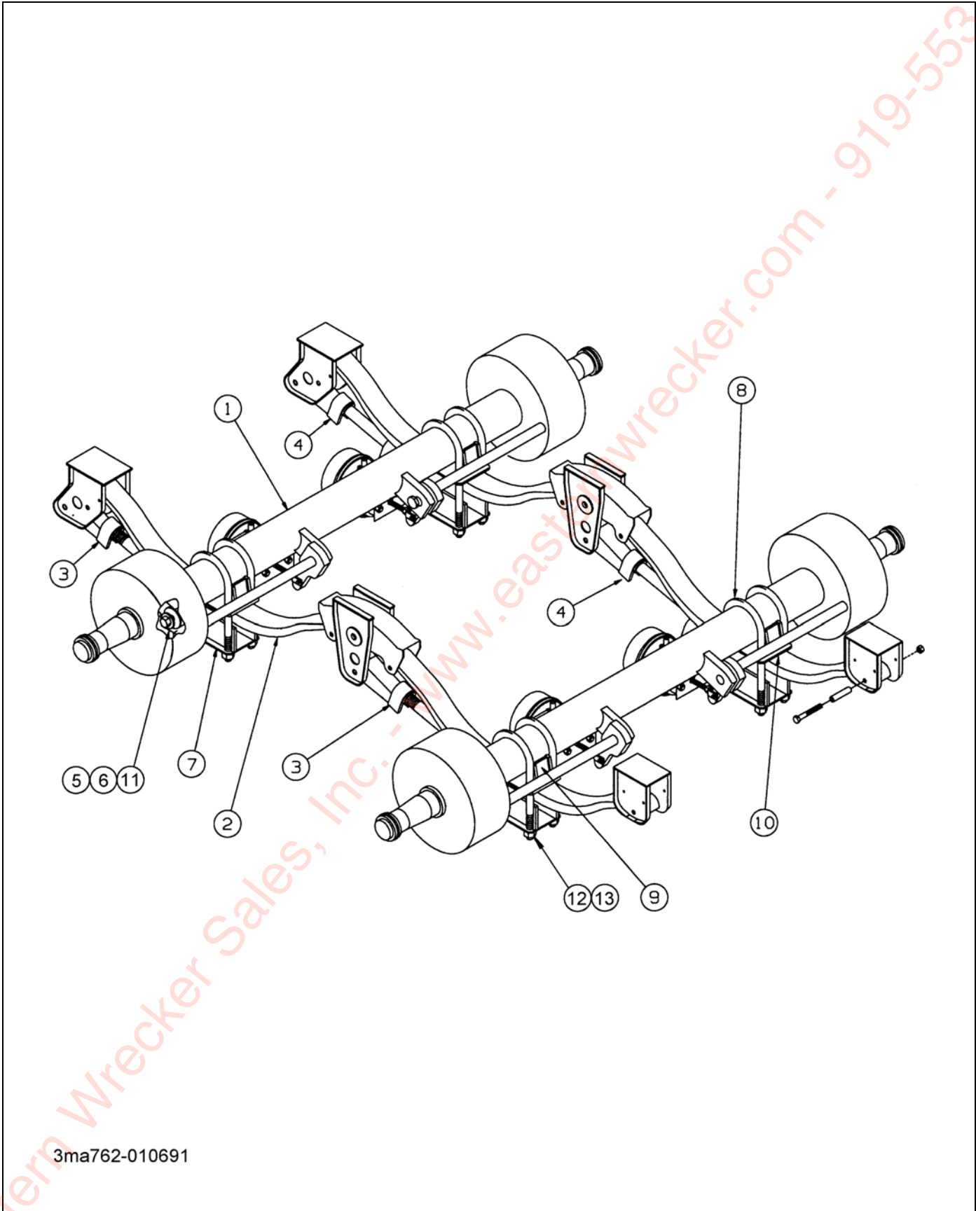
Figure 2-15: Suspension Assembly - Spring Ride
