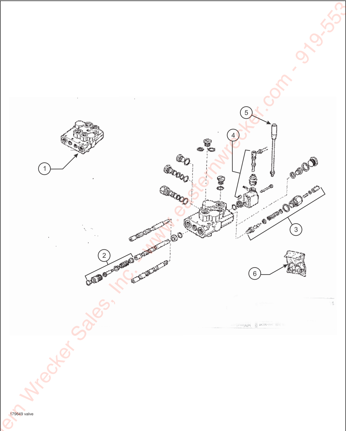
Figure 2-45: Dock Leveler Valve (After 01/15/2014)
