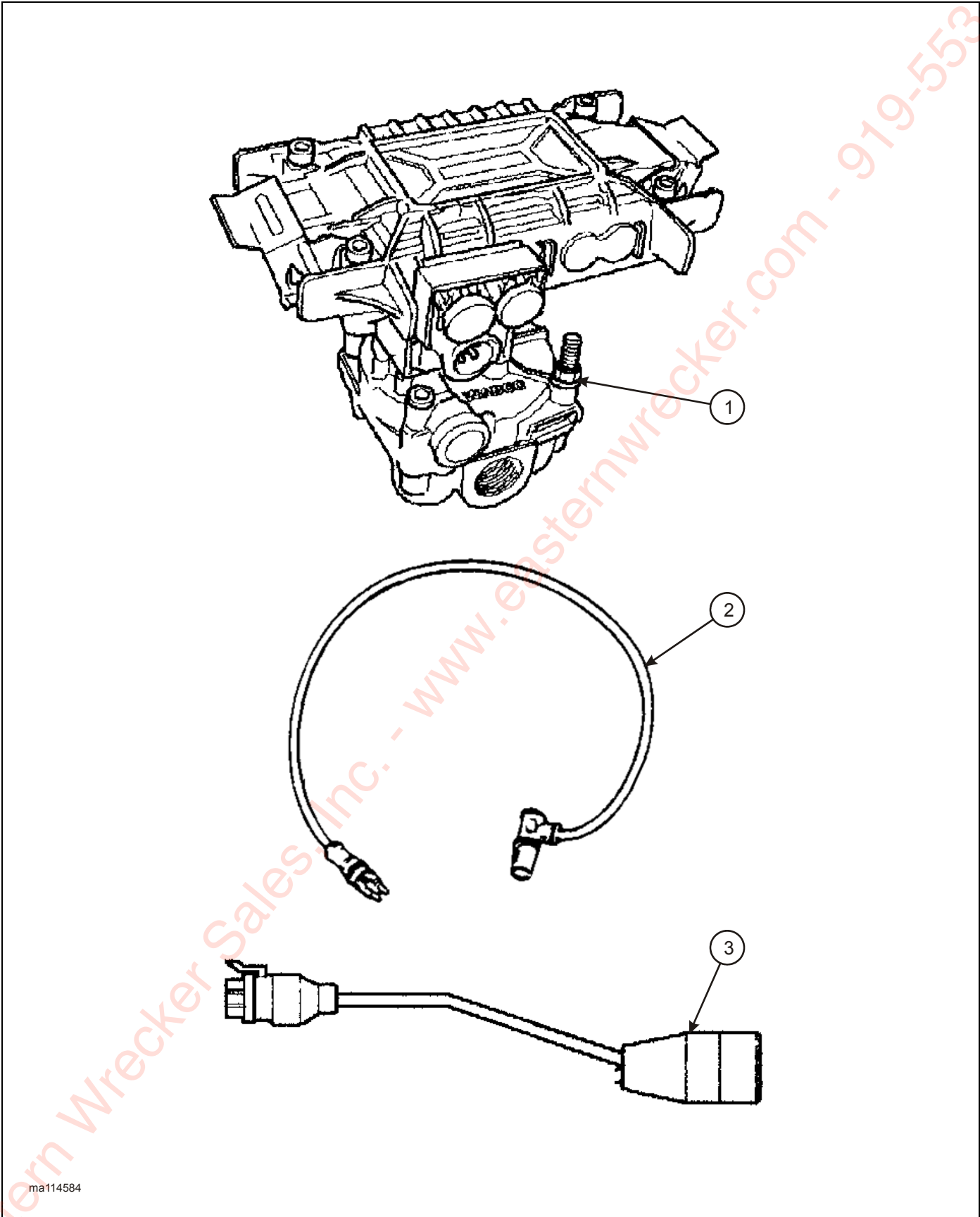
Figure 2-23: Brake Kit, Rockwell ABS 4S/2M
