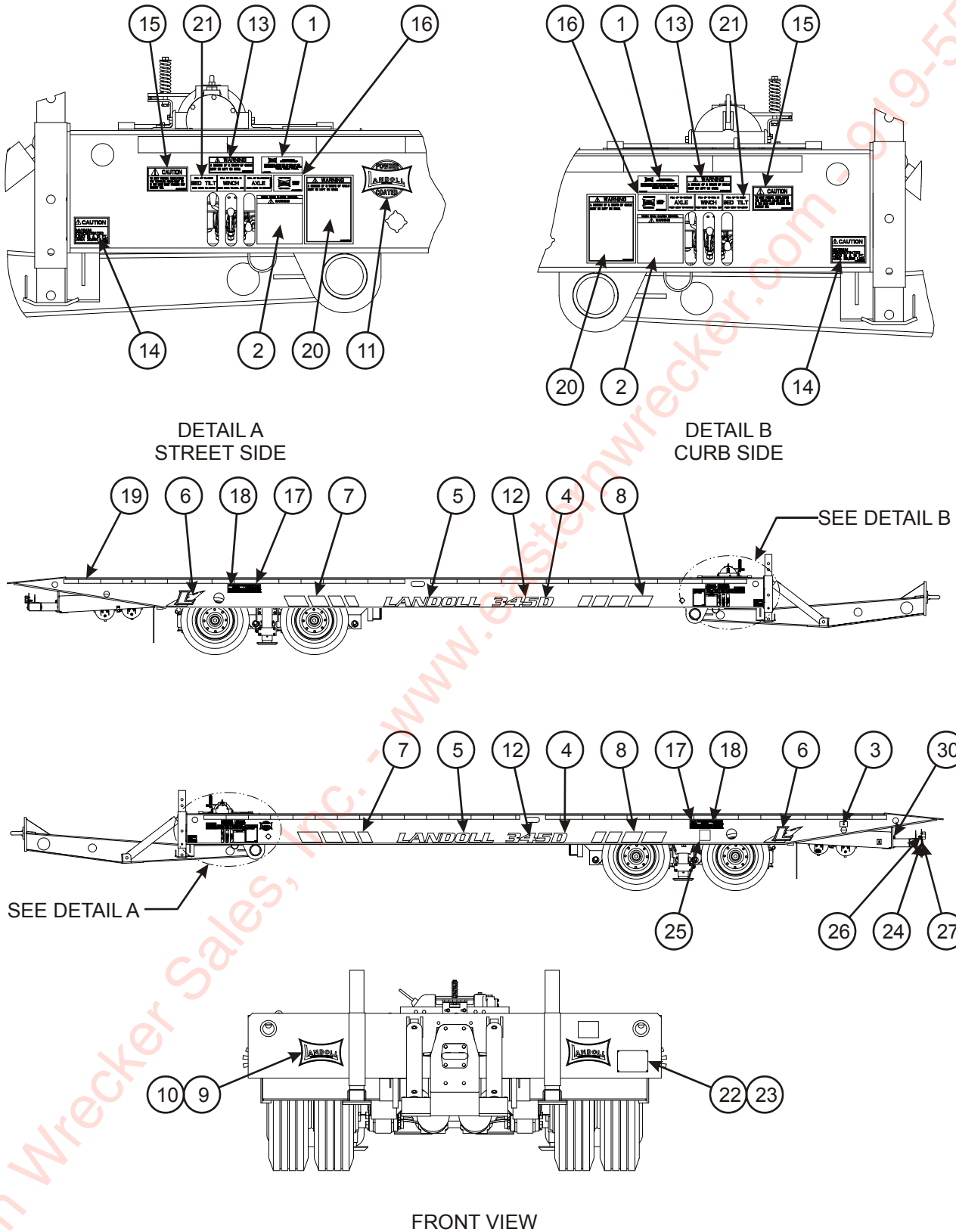
Figure 2-32: Decal Installation
