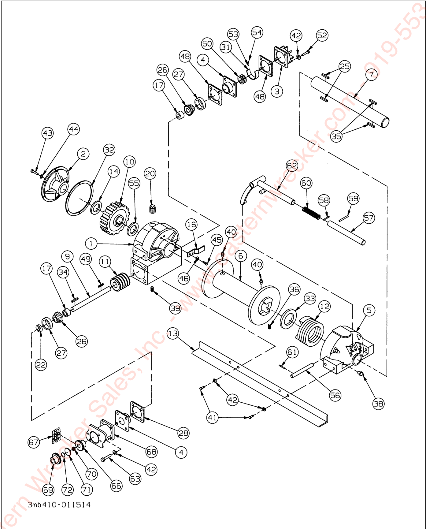
Figure 2-27: 12,000# Winch Items
