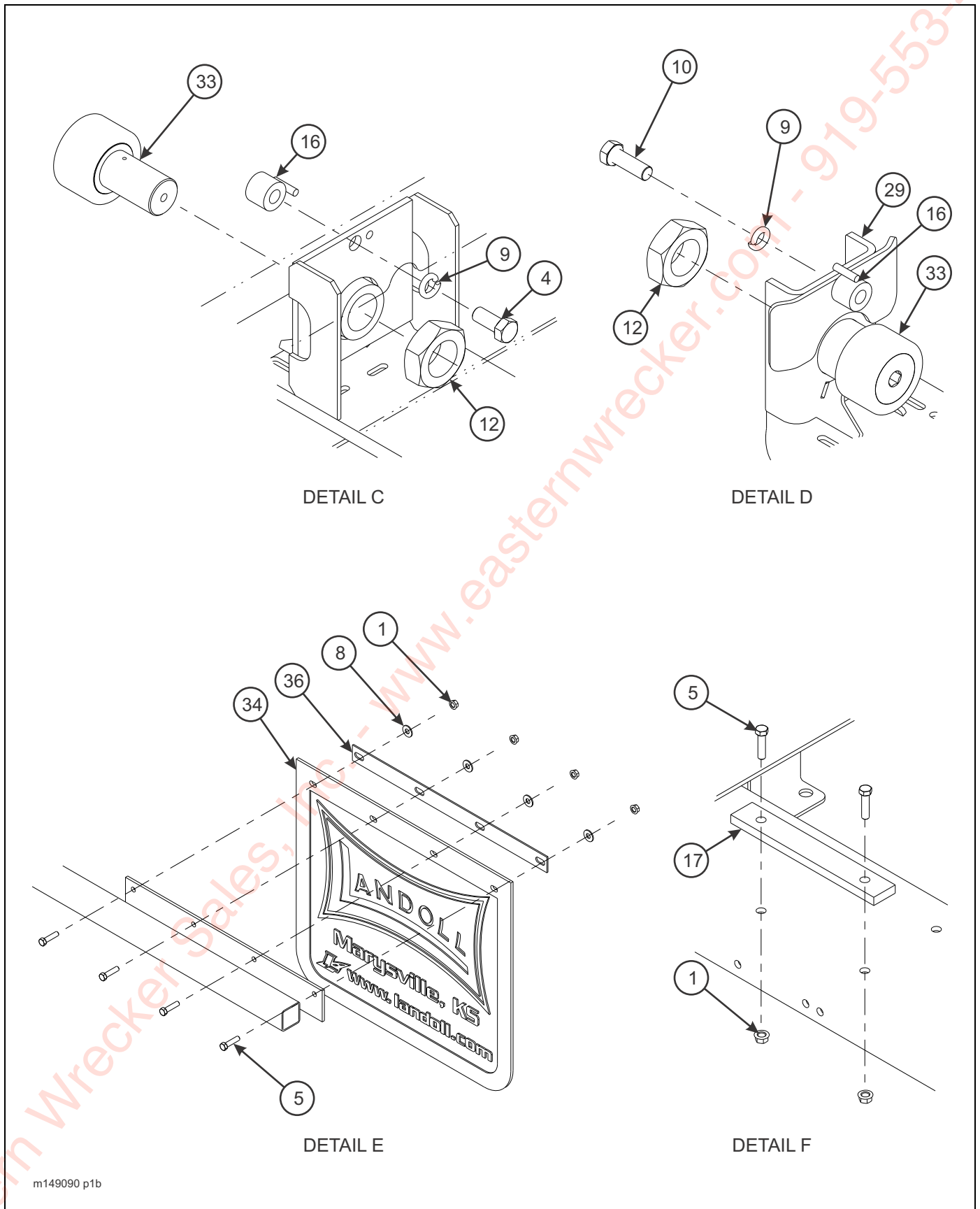
Figure 2-16: Undercarriage Assembly - Spring Ride (2 of 3)
