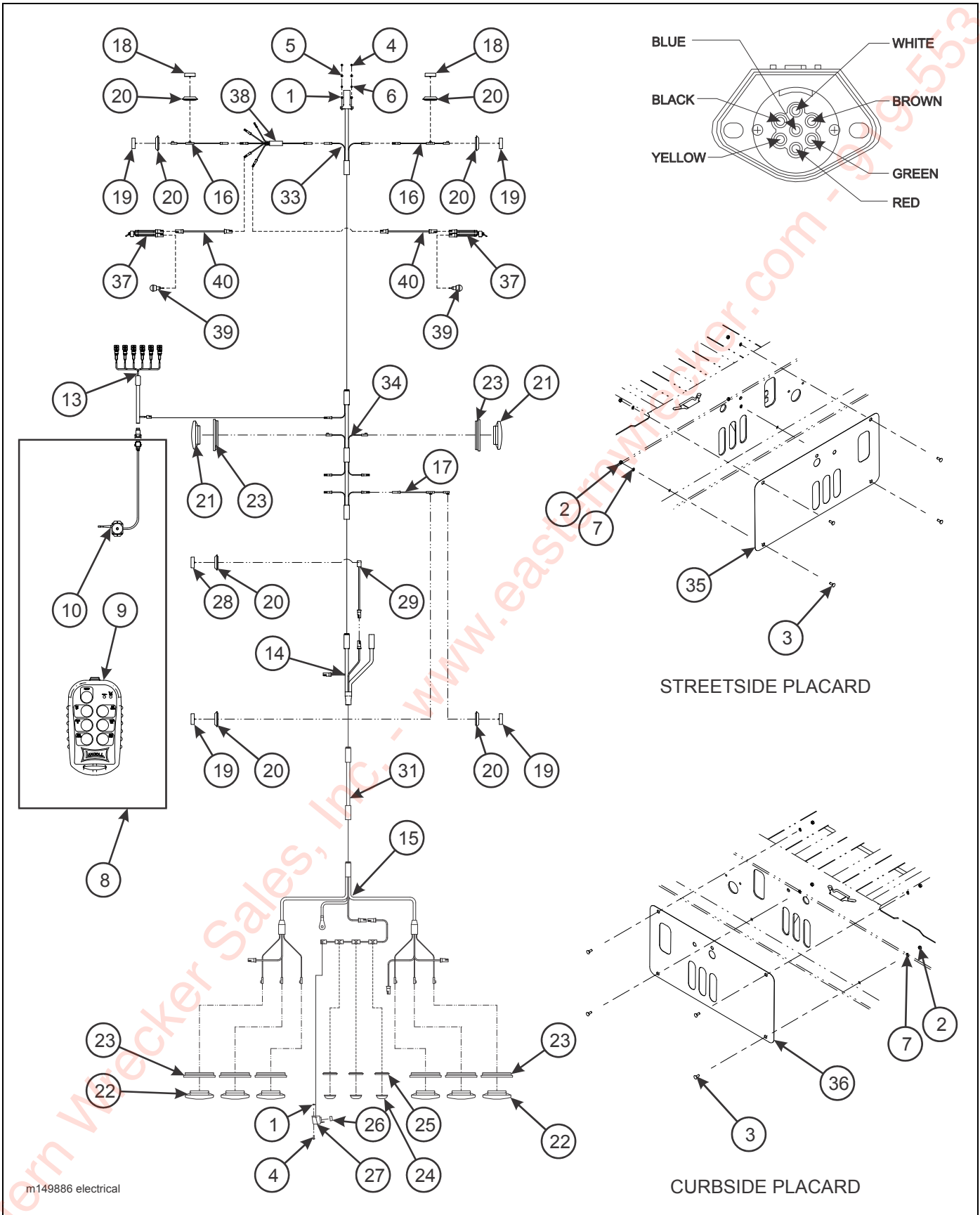
Figure 2-14: Electrical Assembly
