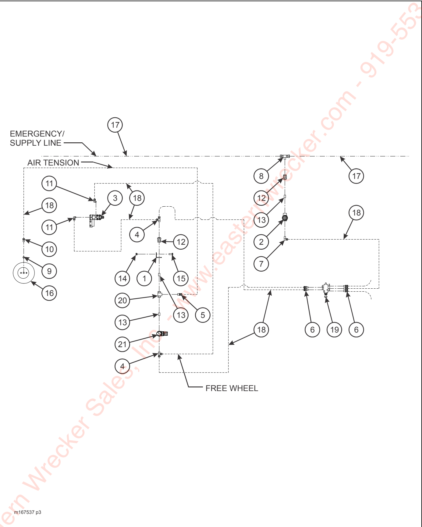
Figure 2-35: Winch Installation, Guide Air T/R - Air
