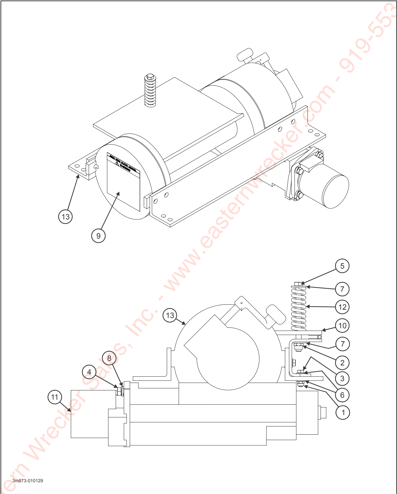
Figure 2-33: Winch Installation
