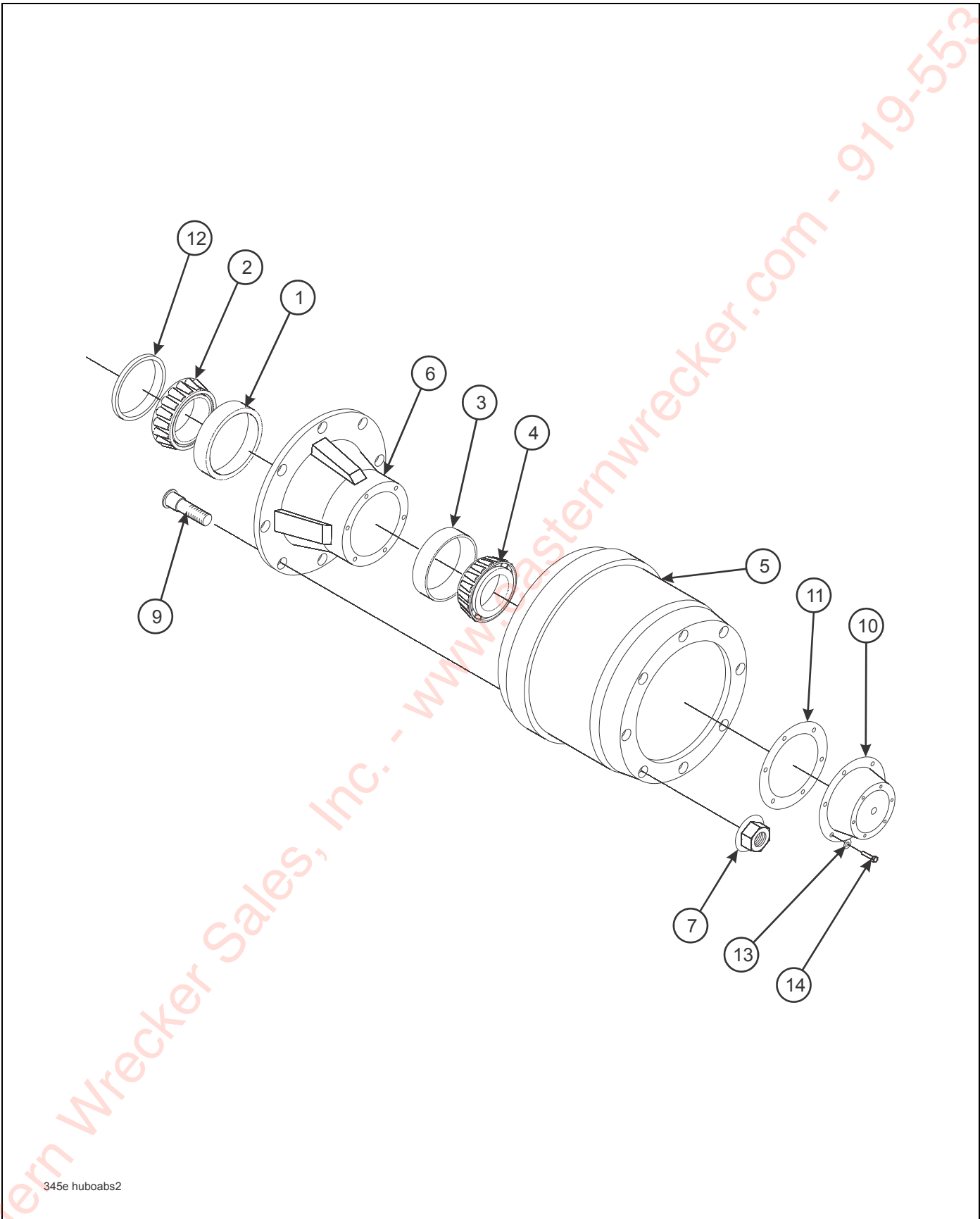
Figure 2-29: Outboard Hub and Drum Assembly
