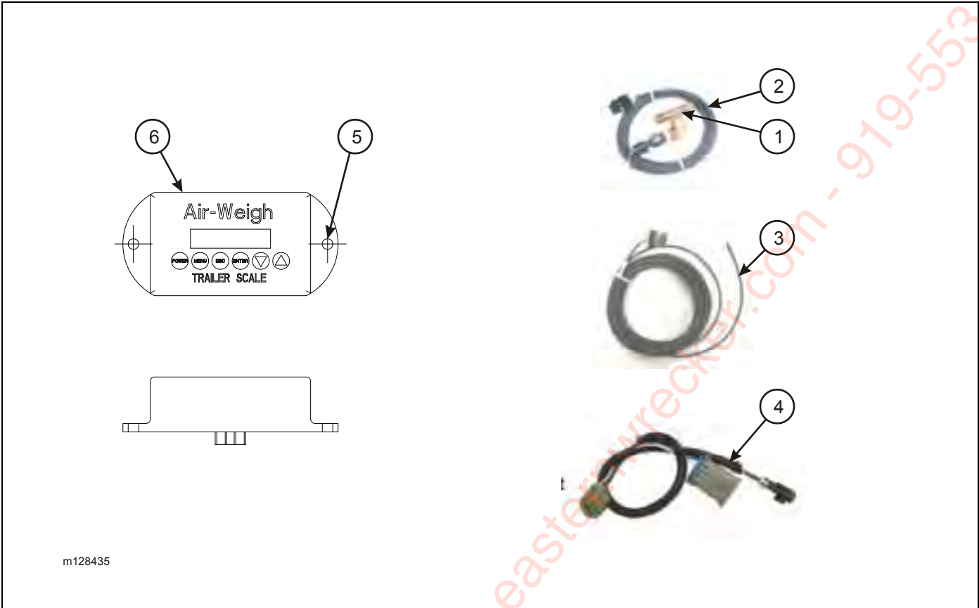
Figure 2-63: Air Digital Scale (Option)
