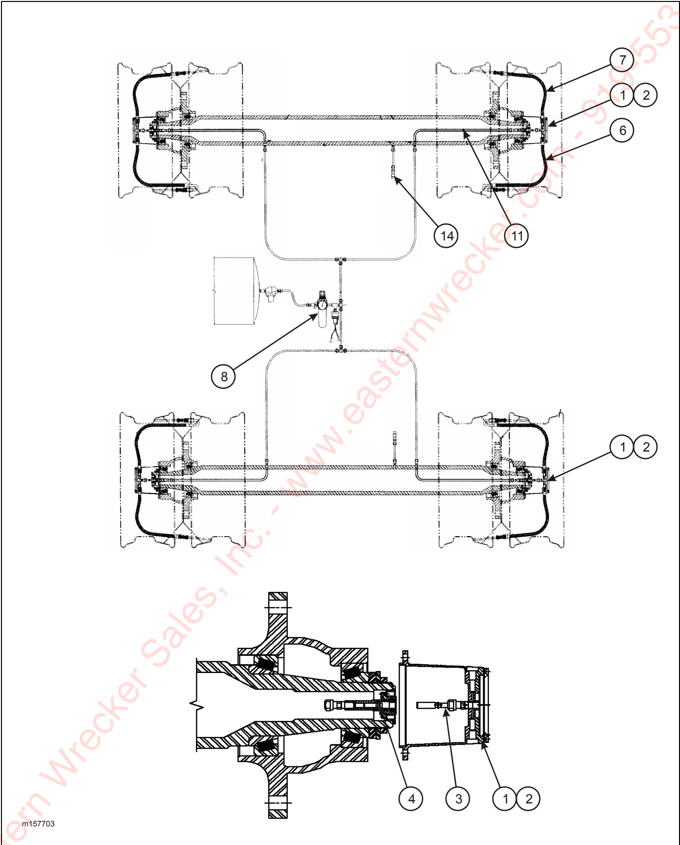
Figure 2-67: Tire Inflation System (Option)
