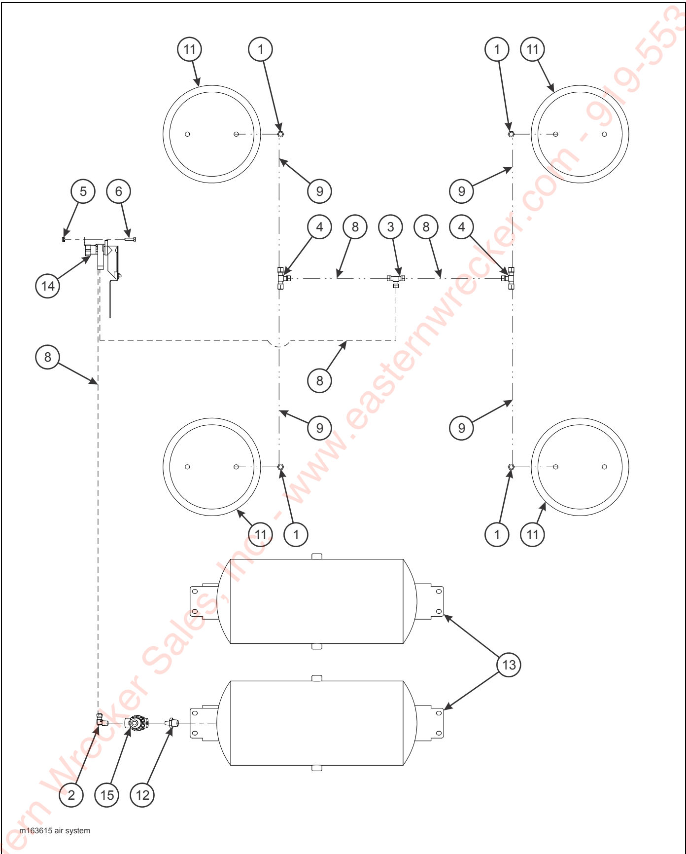
Figure 2-23: Air Ride Suspension, Air System (Tandem)
