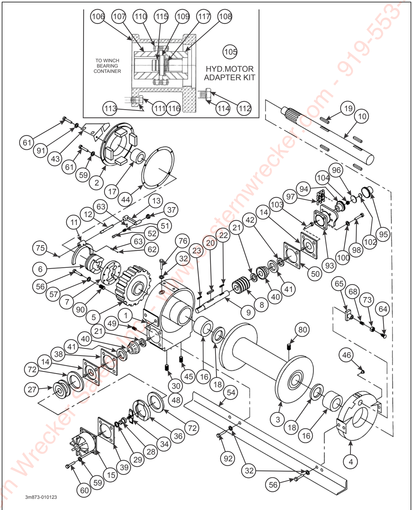
Figure 2-39: 20,000# Winch Items
