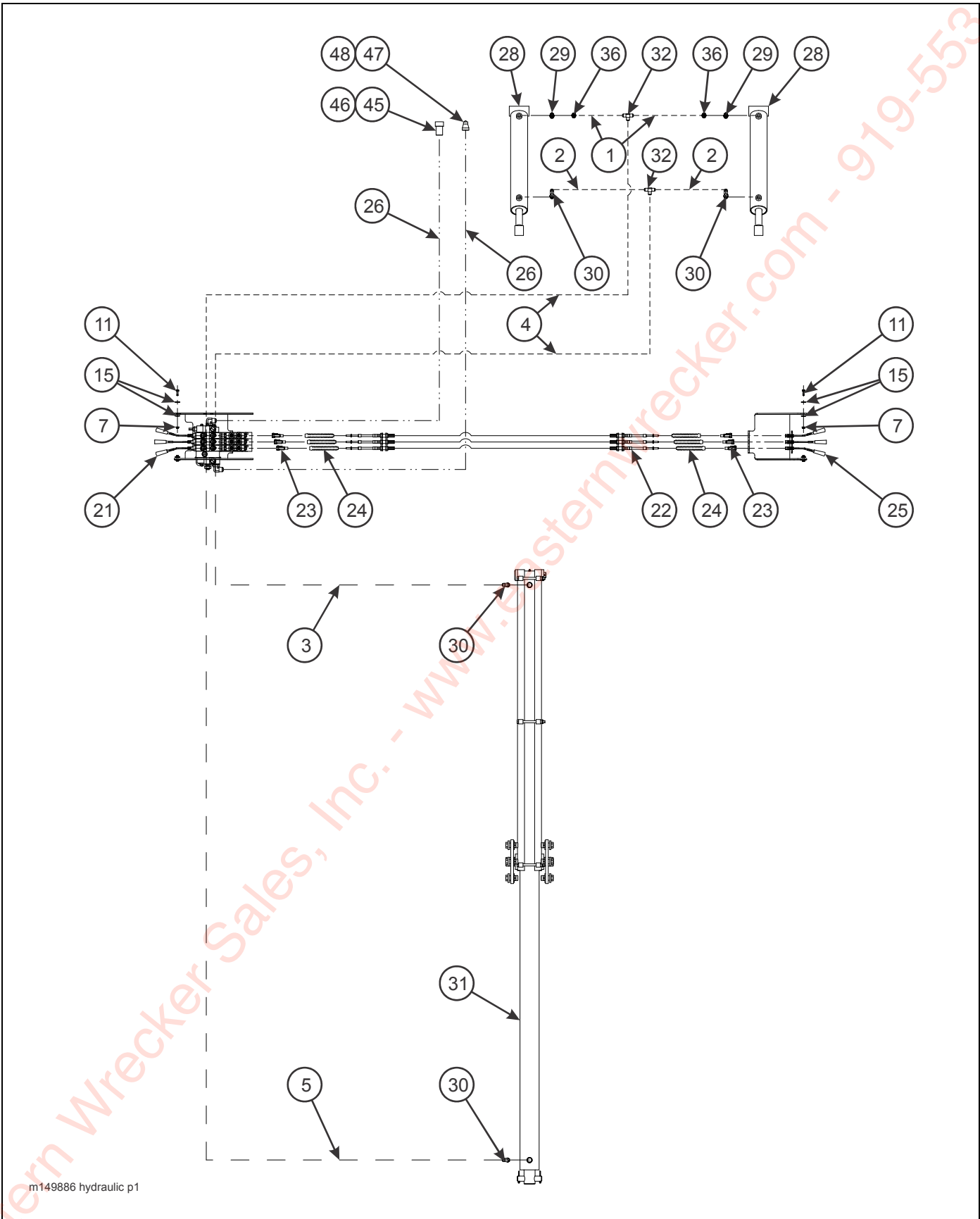
Figure 2-7: Hydraulic Assembly (1 of 3)
