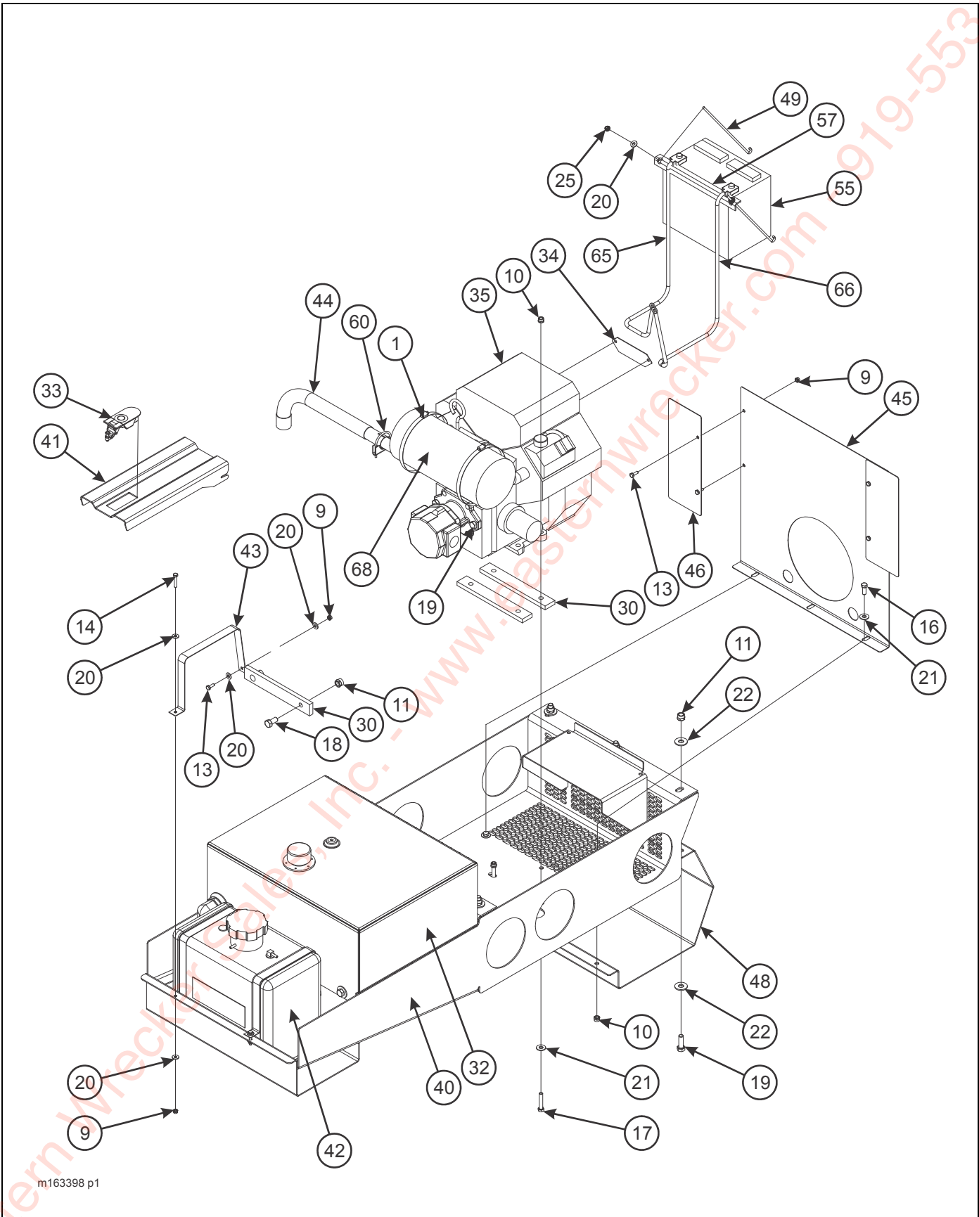
Figure 2-57: Engine Drive, 27 HP (1 of 4)
