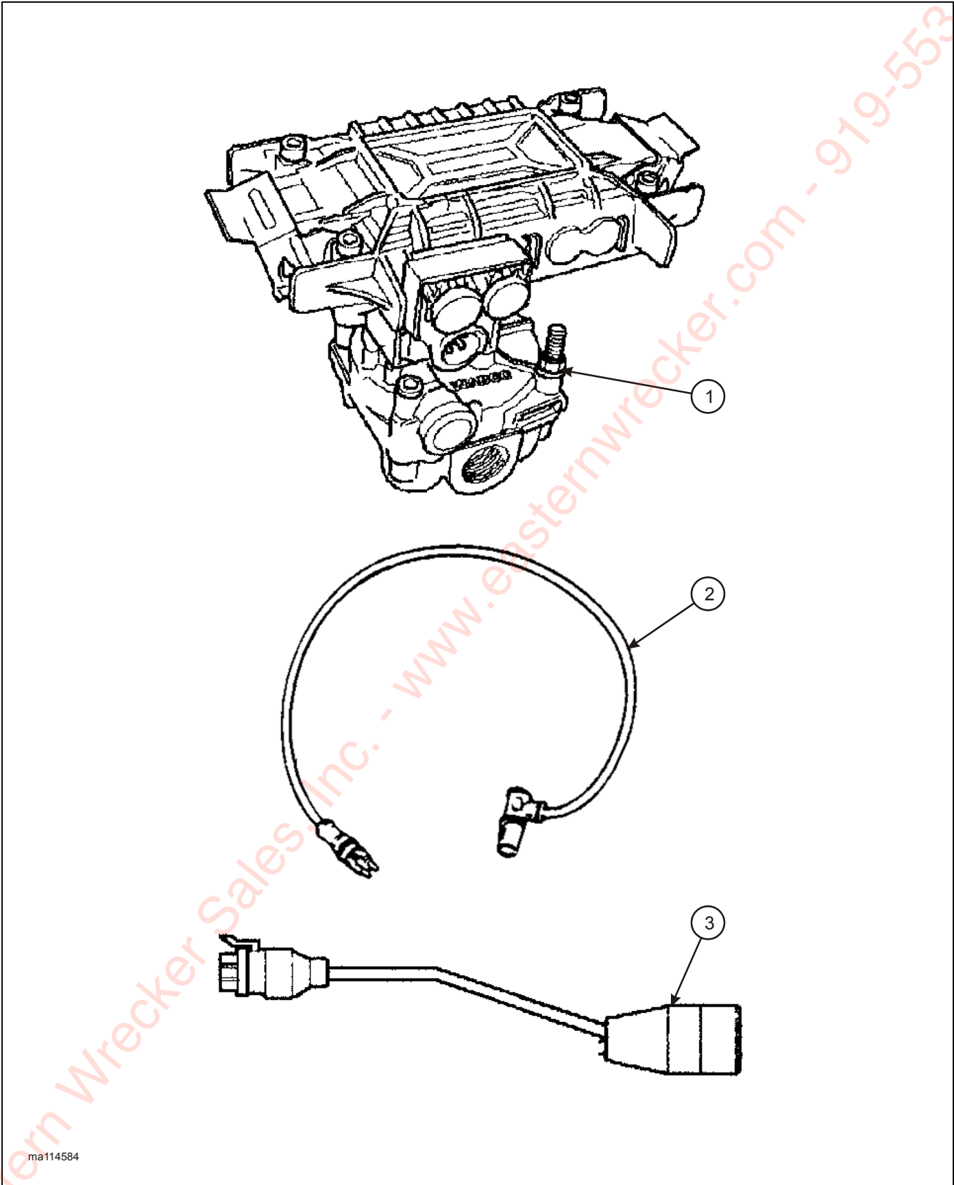
Figure 2-28: Brake Kit, Rockwell ABS 4S/2M
