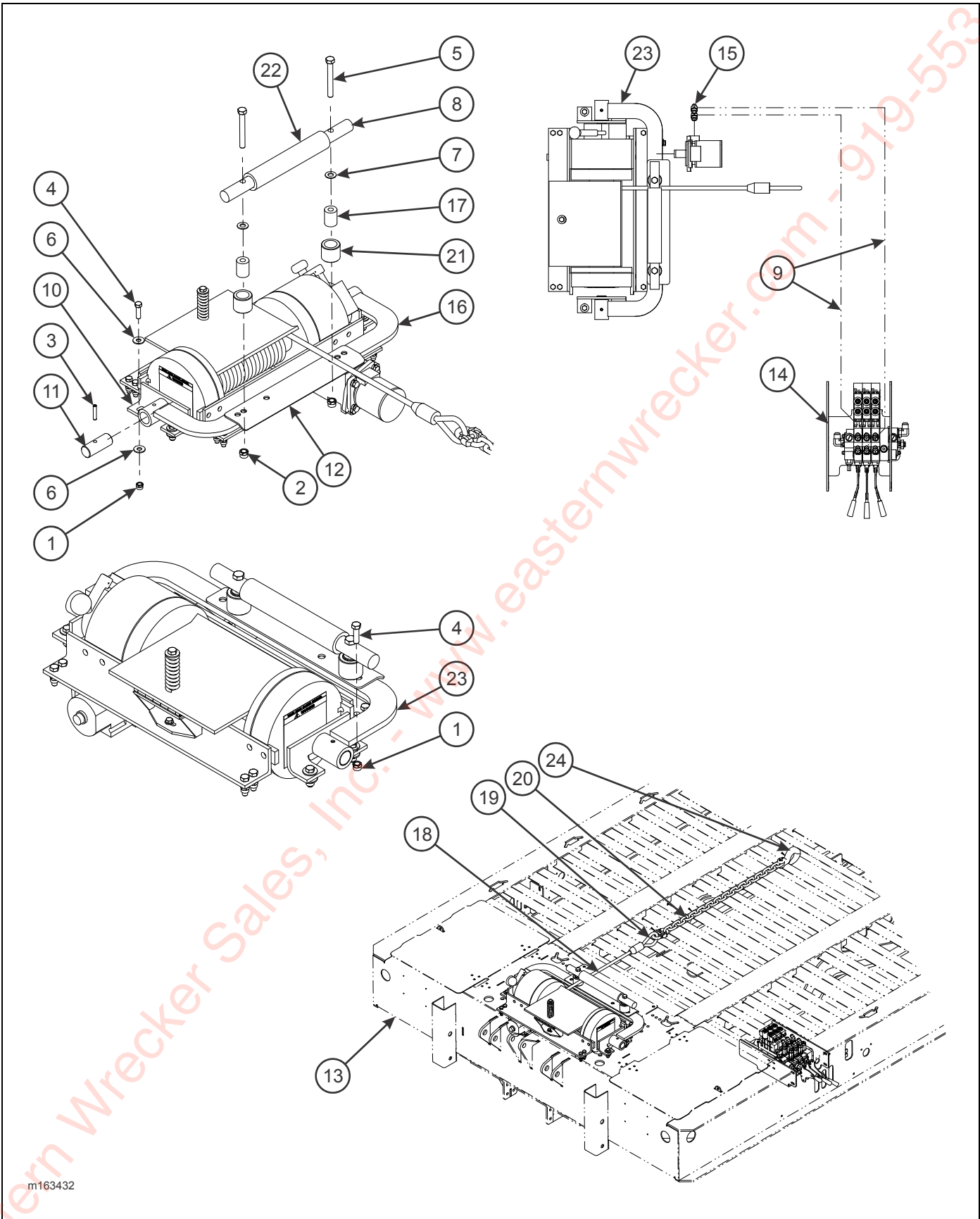
Figure 2-32: Winch Installation
