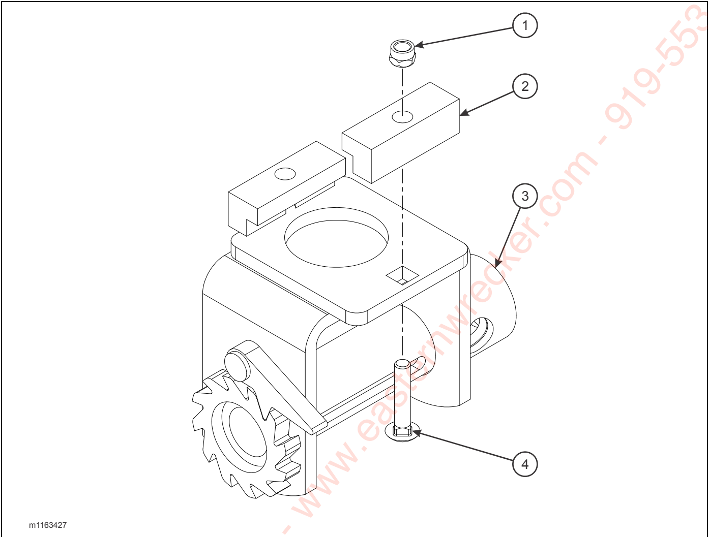
Figure 2-44: Winch Assembly, 4" Webbing Sliding (Option)
