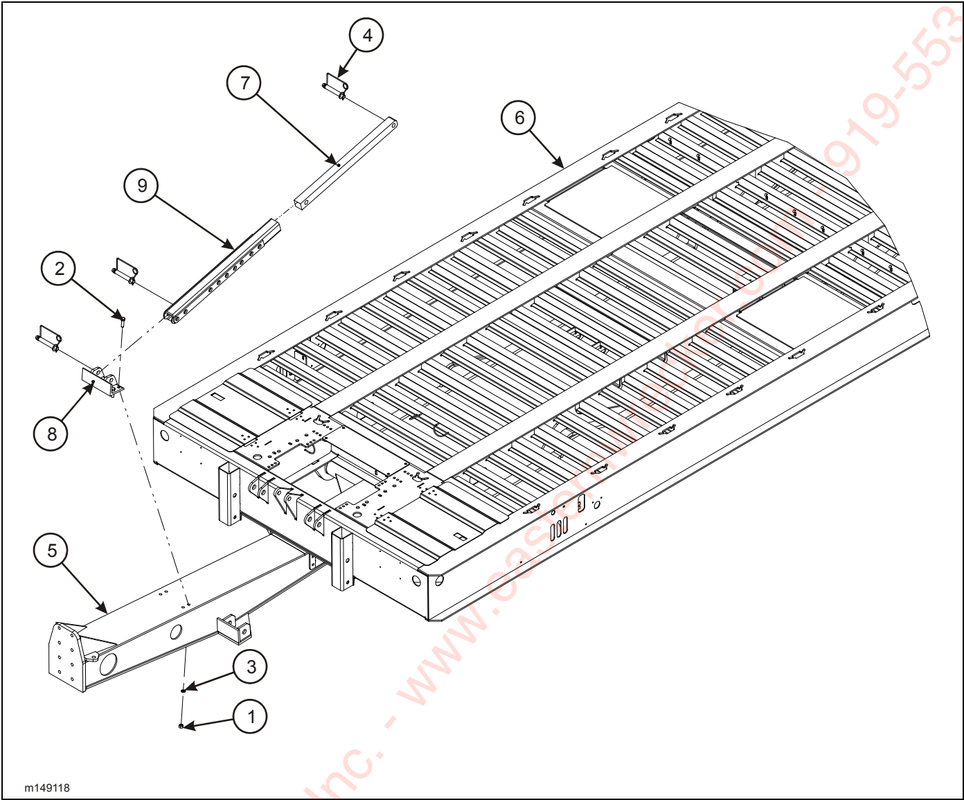
Figure 2-61: Hitch Lock Installation (Option)
