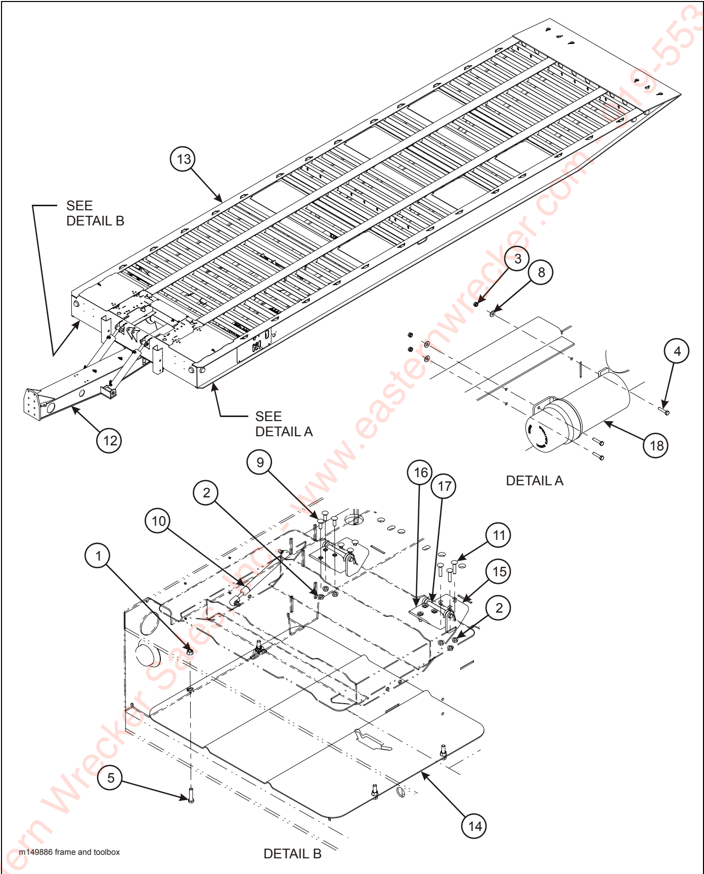
Figure 2-6: Frame and Toolbox Assembly
