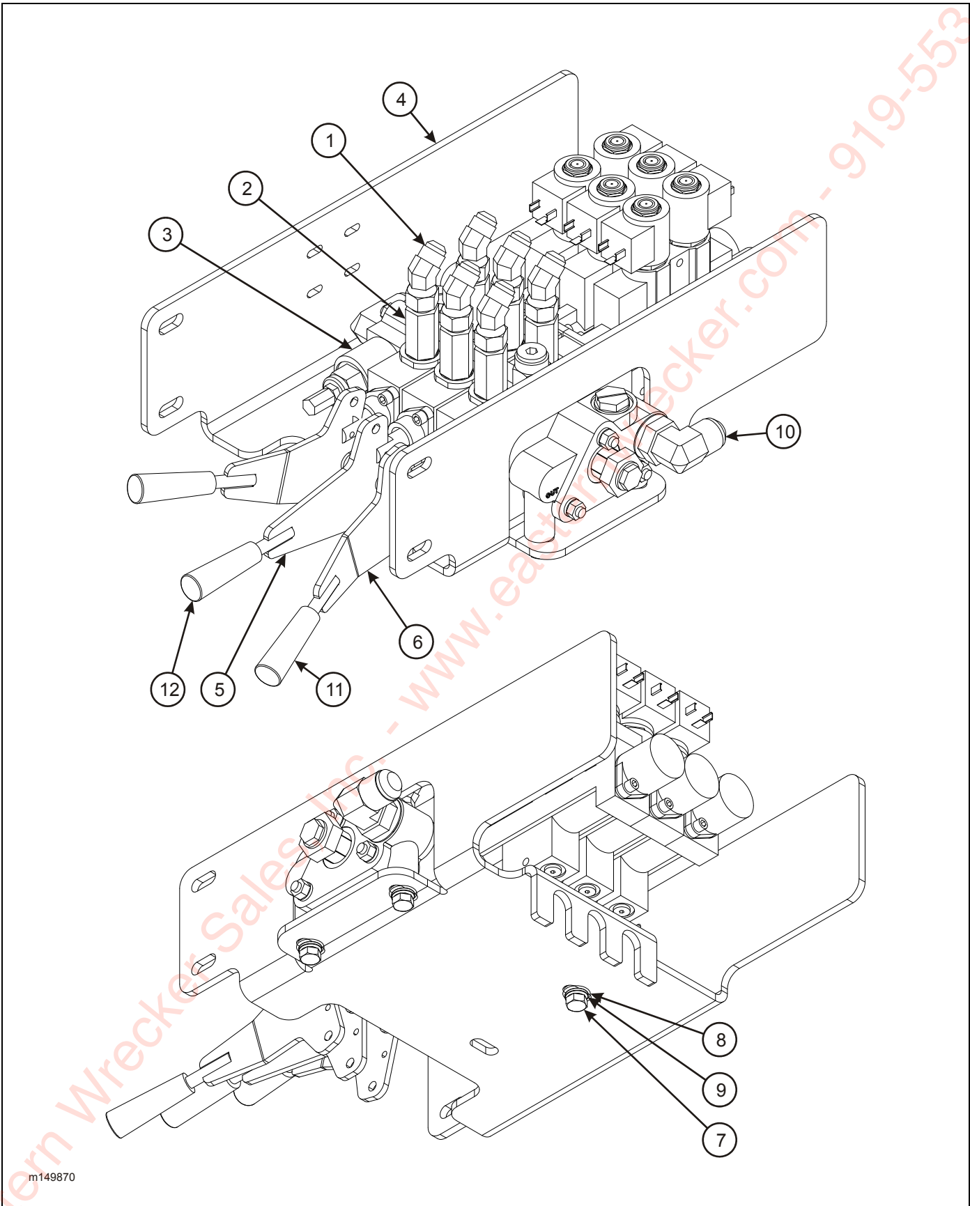
Figure 2-12: Valve Assembly - 3 Spool
