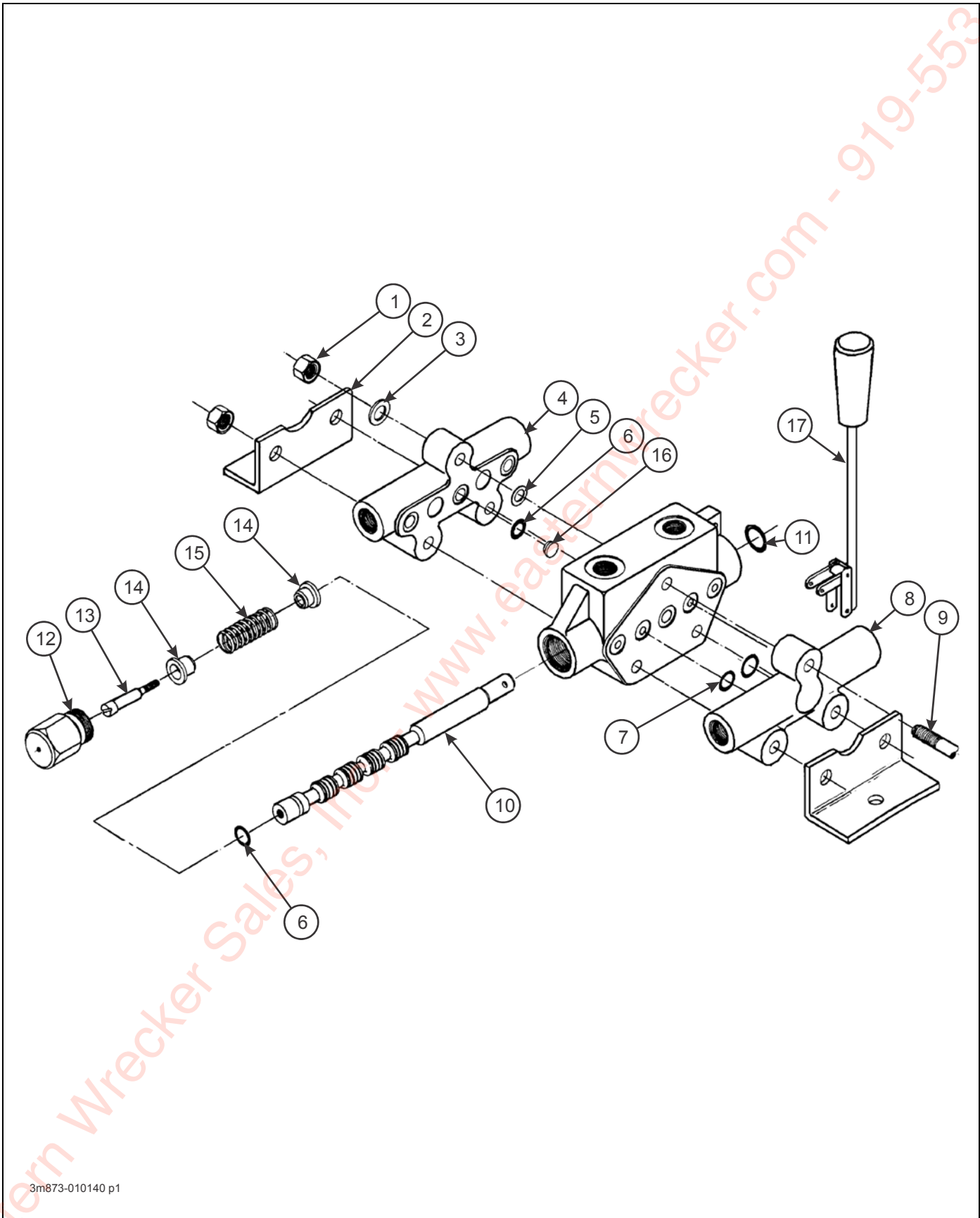
Figure 2-55: Dock Leveler Valve (Before 01/15/2014)
