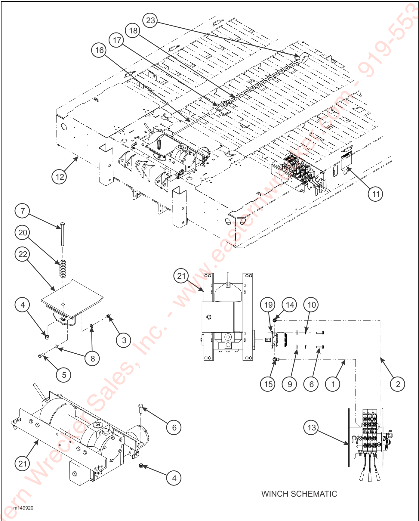
Figure 2-37: Winch Installation
