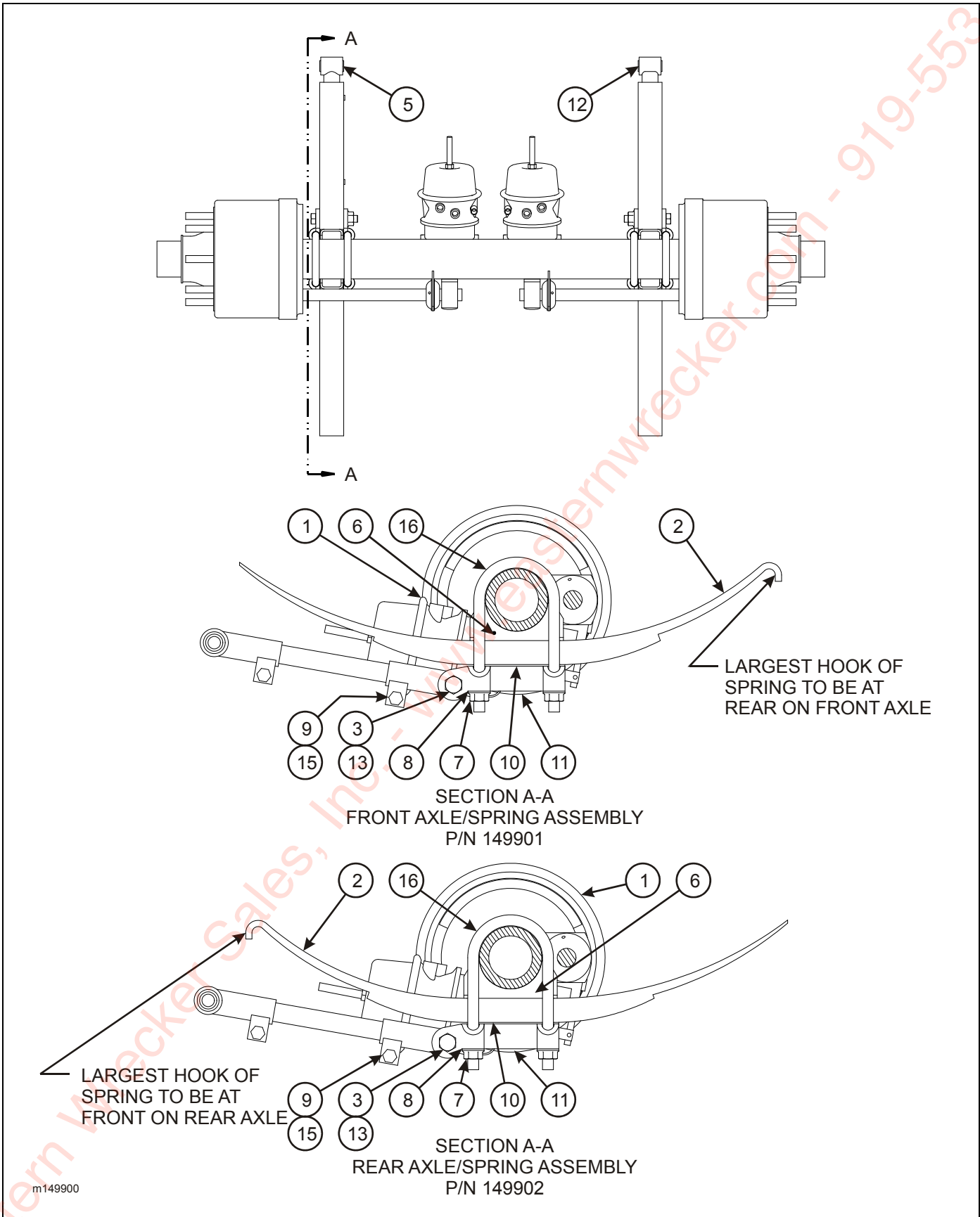
Figure 2-18: Axle/Spring Assembly
