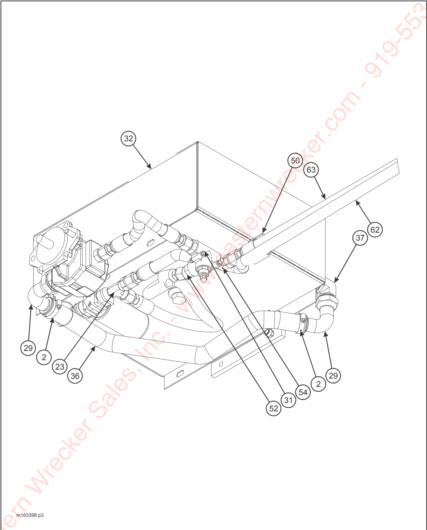
Figure 2-59: Engine Drive, 27 HP (3 of 4)
