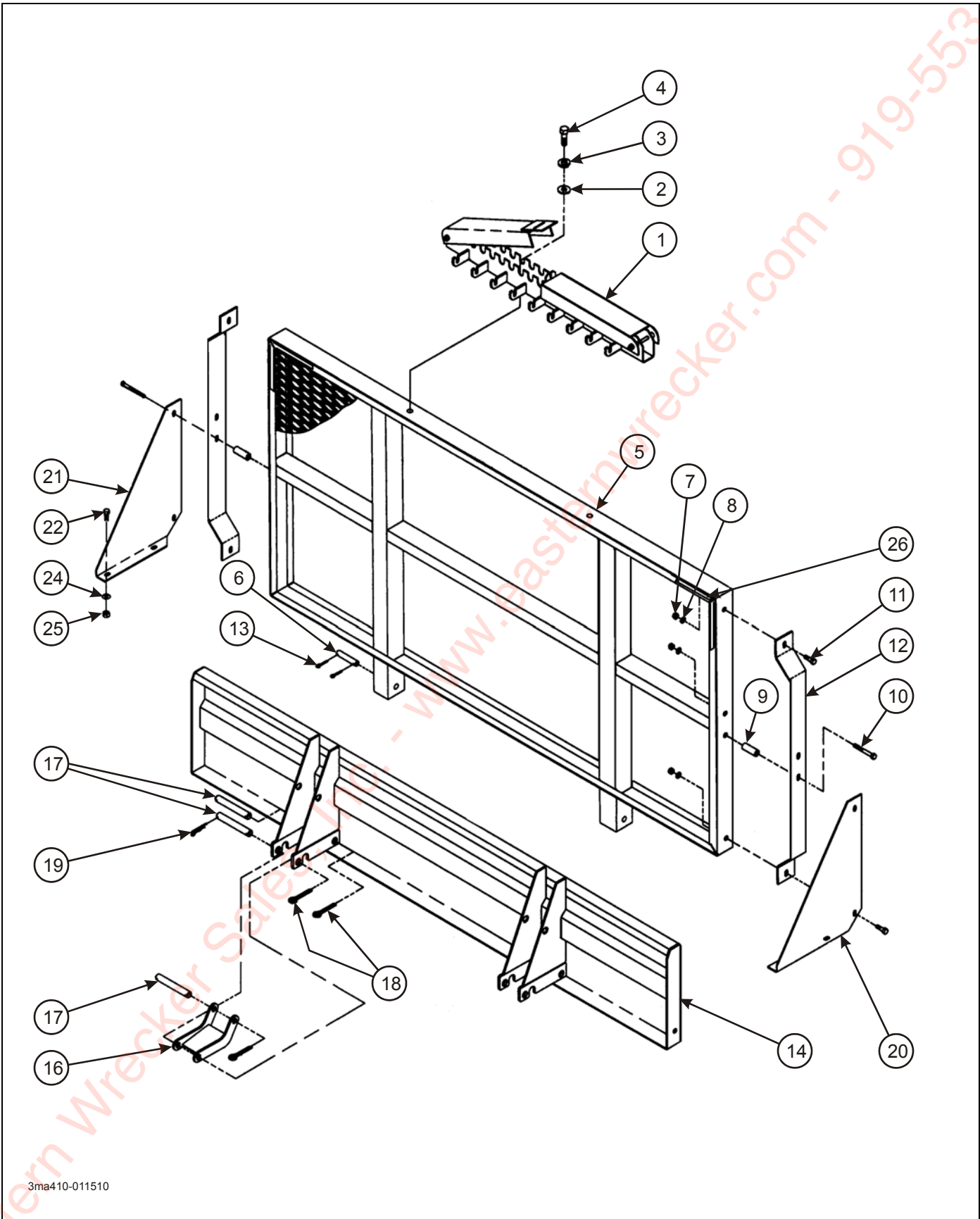
Figure 2-60: Front Extension and Bulkhead (Option)
