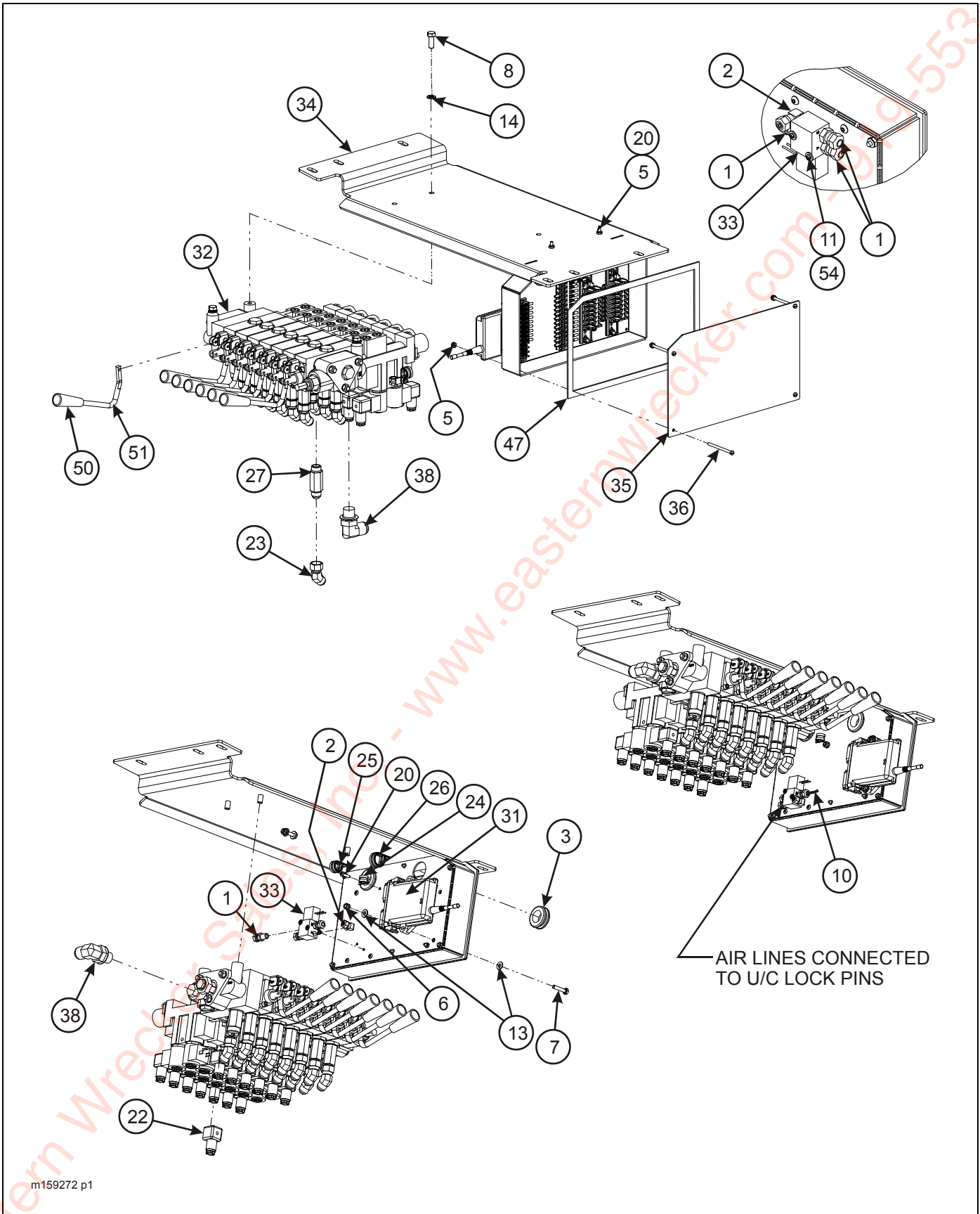
Figure 2-11: Valve Assembly, 7 Spool (1 of 2)
