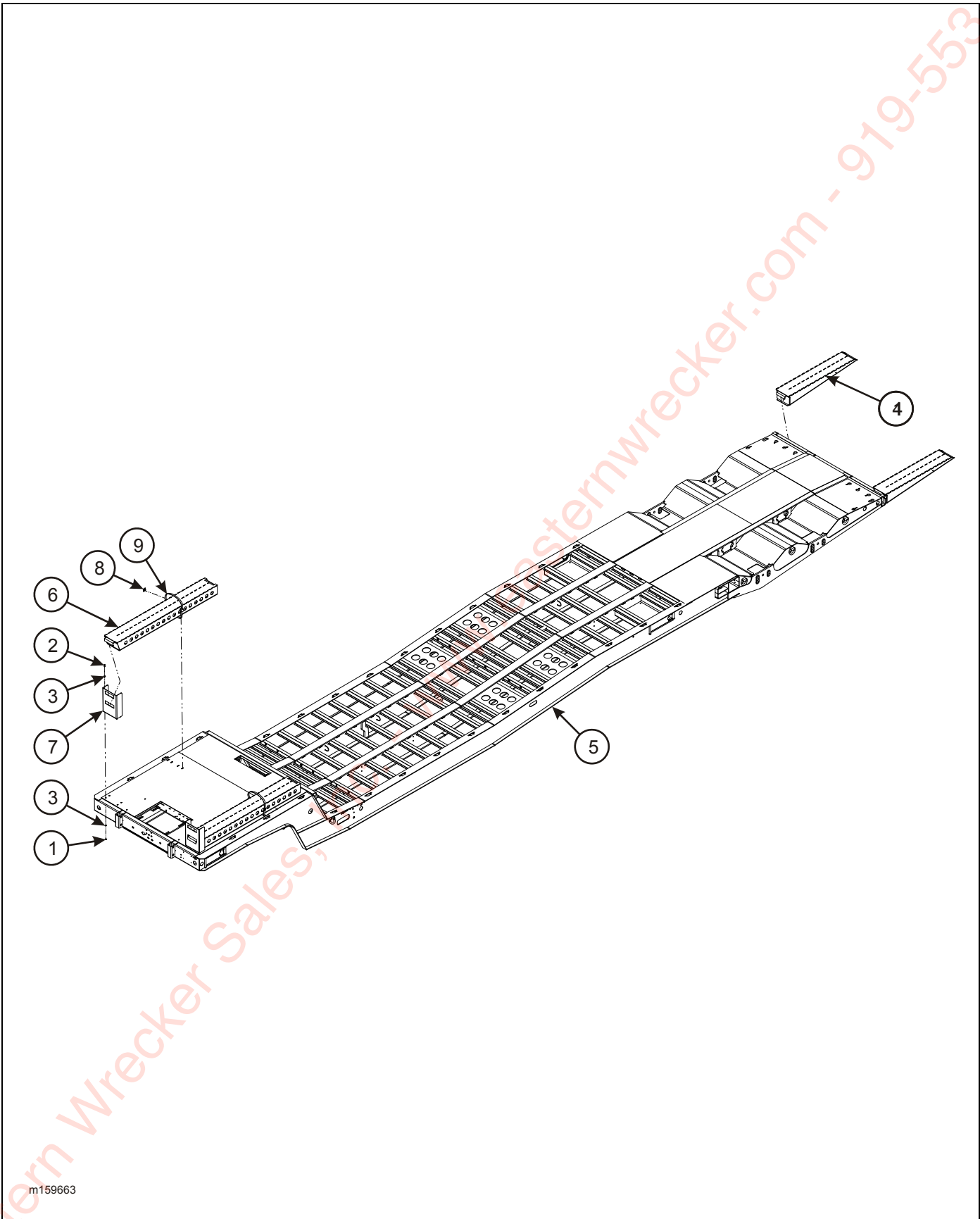
Figure 2-62: Aluminum Ramp Assembly
