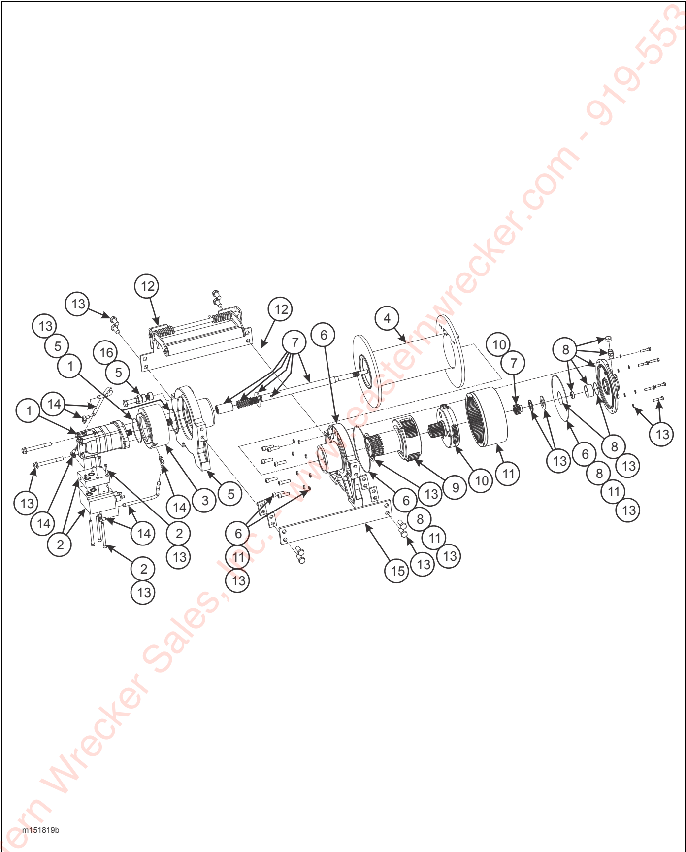
Figure 2-37: 20K Winch Items
