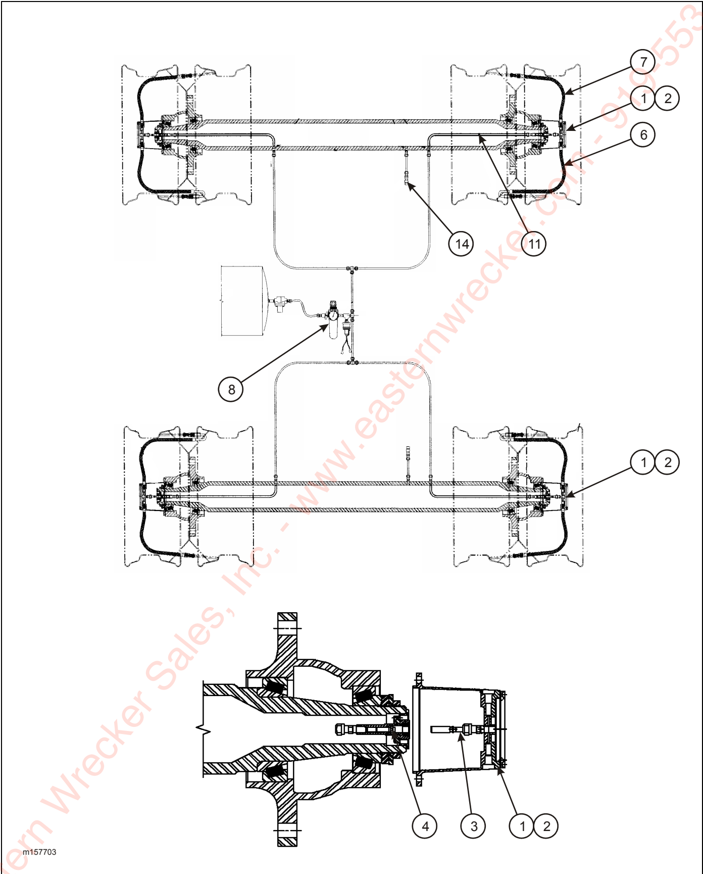
Figure 2-67: Tire Inflation System
