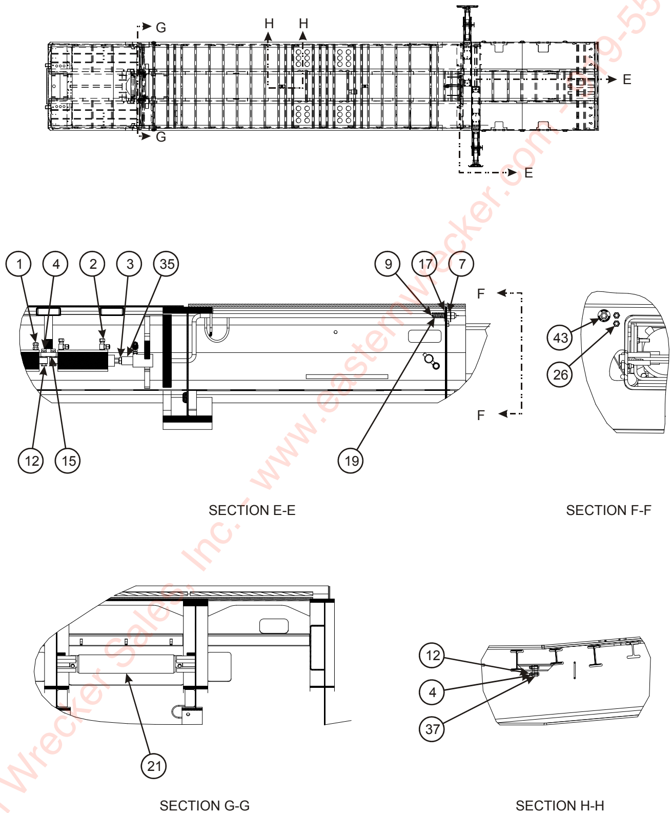
Figure 2-14: Bus Hauler Accessories (2 of 3)
