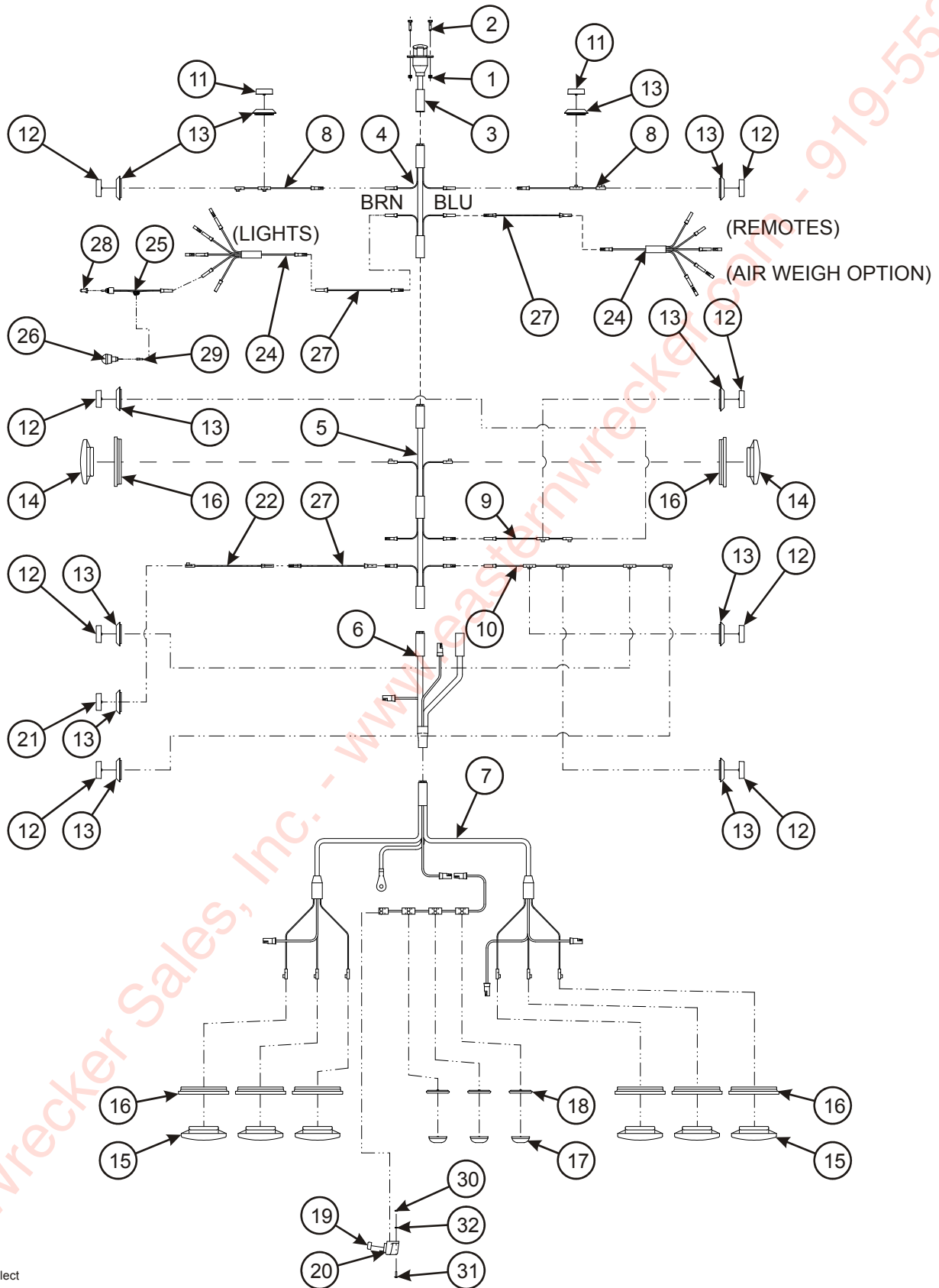
Figure 2-20: Electrical System
