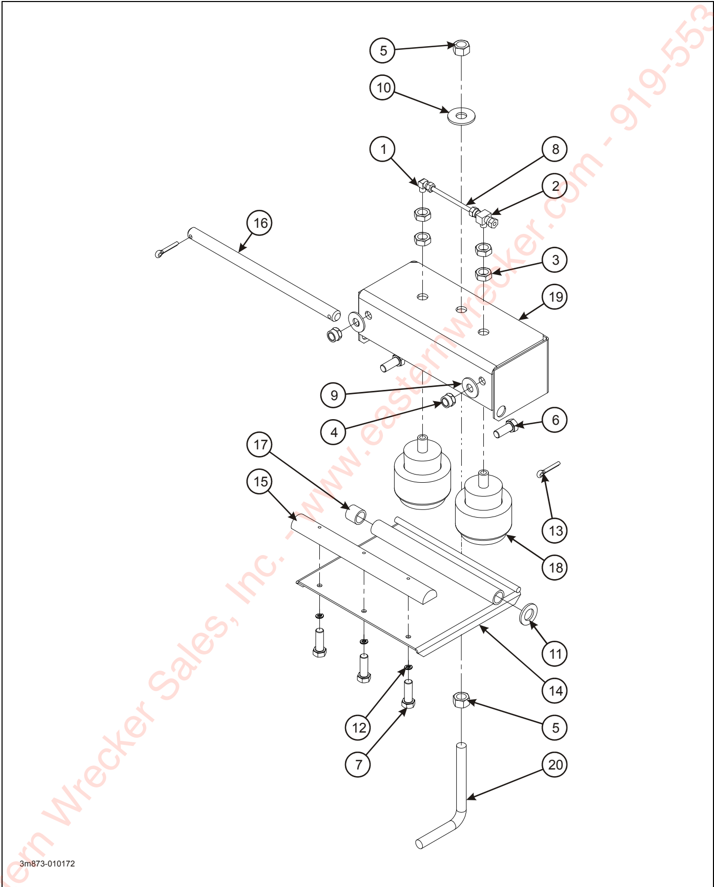
Figure 2-50: Winch Cable Air Tension 30K
