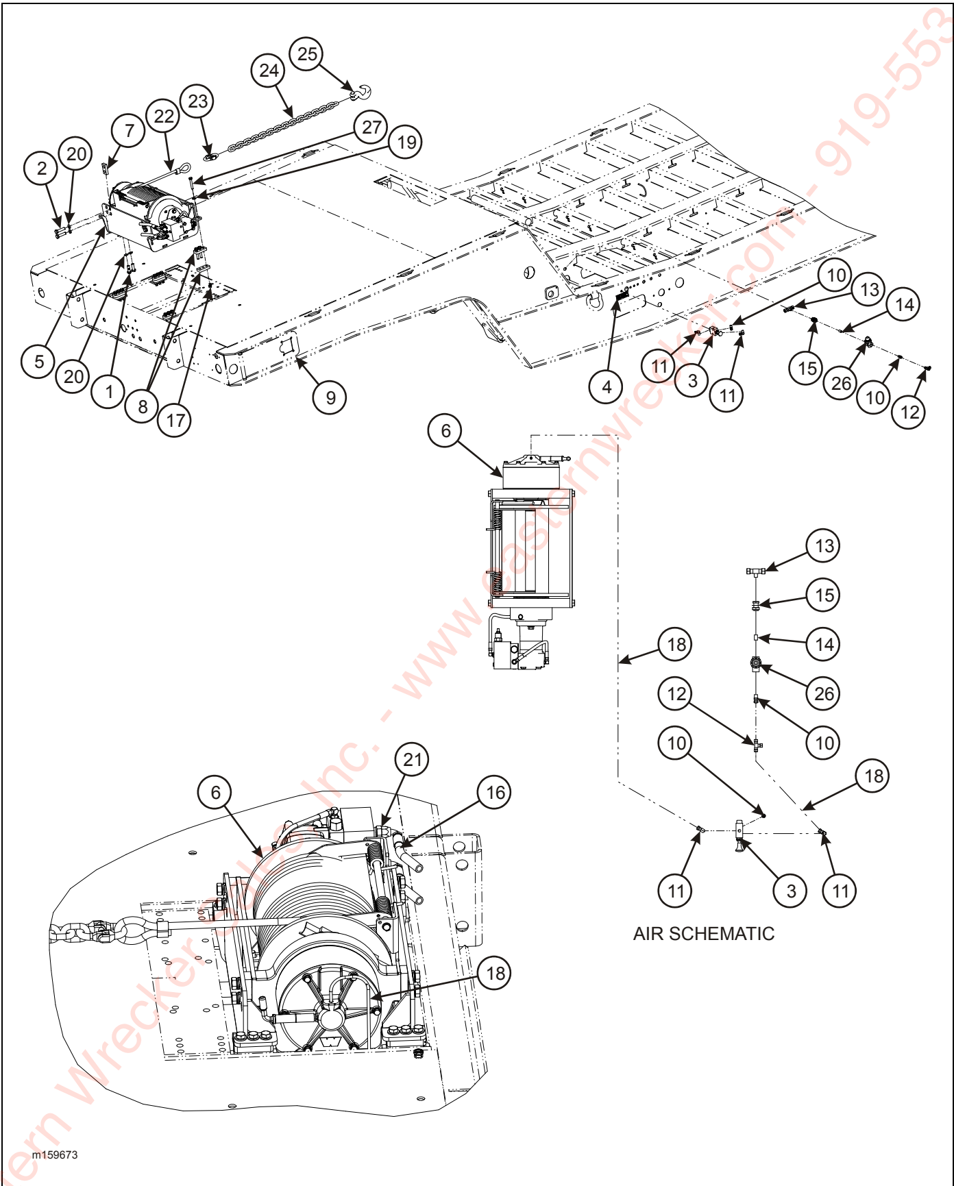
Figure 2-35: Winch Installation, 20K (1 of 2)
