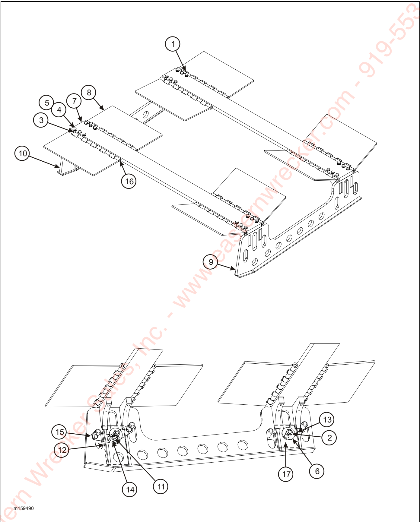
Figure 2-5: Lift Well Group
