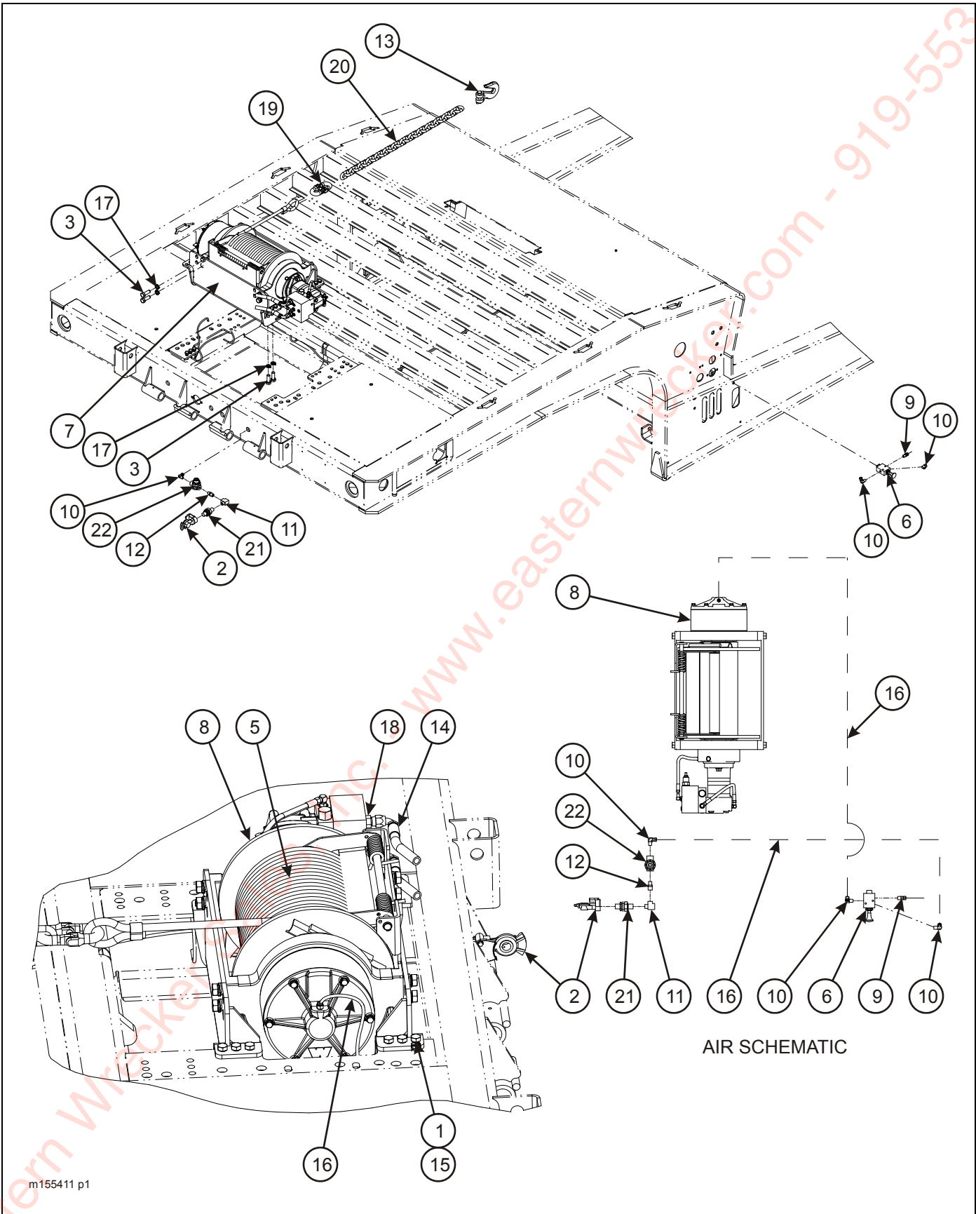
Figure 2-43: Winch Installation, 30K (1 of 2)
