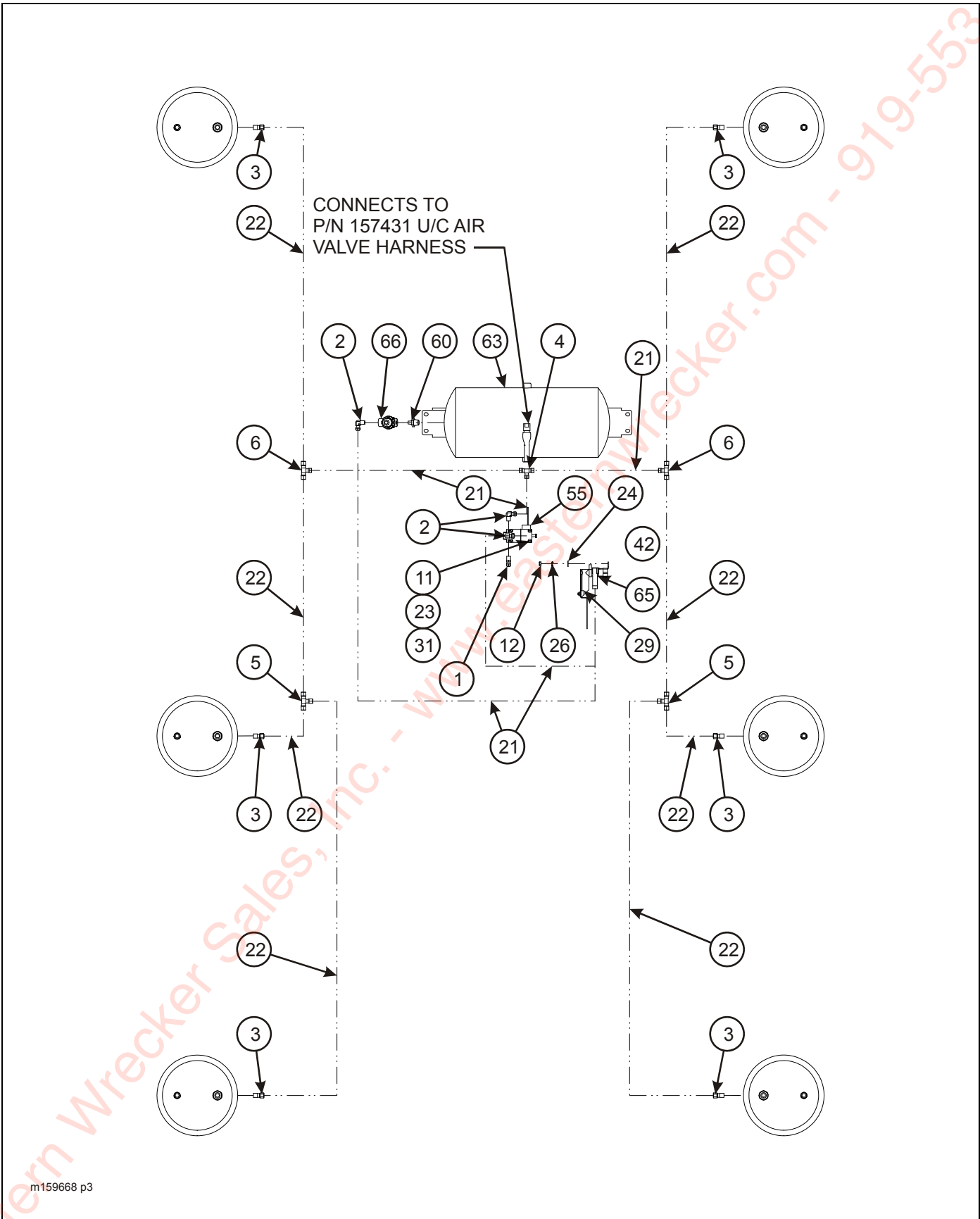
Figure 2-27: Suspension Assembly, Air Ride (3 of 4)
