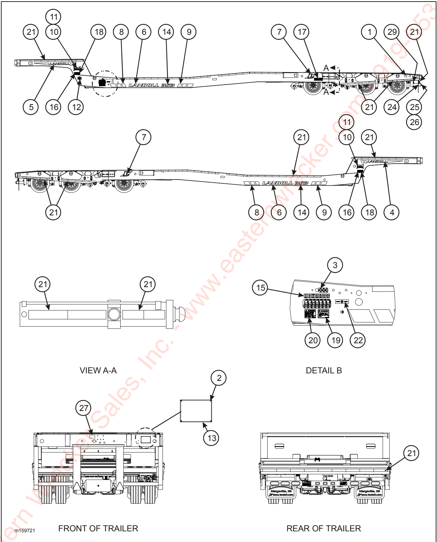
Figure 2-72: Decal Installation (2 of 2)
