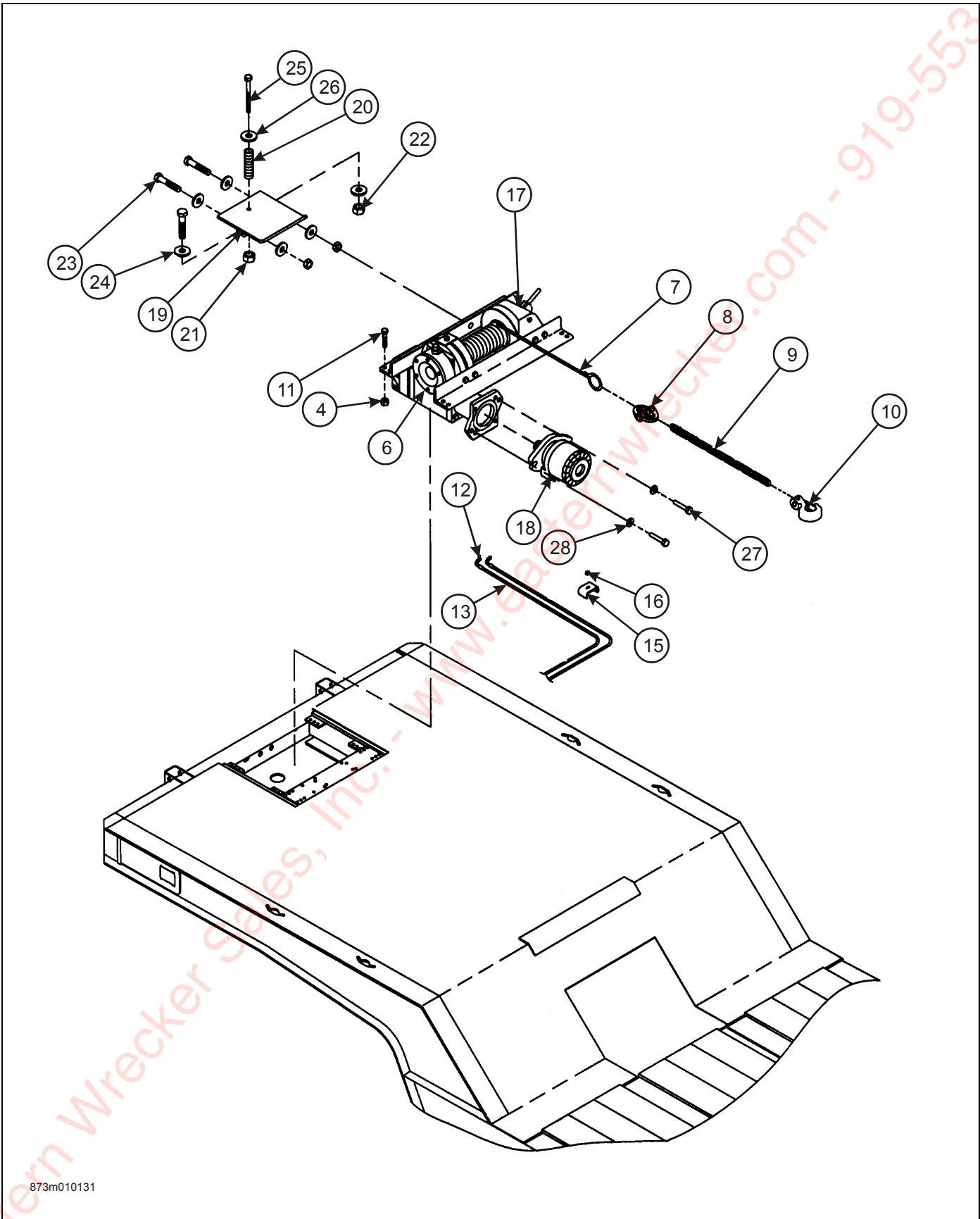
Figure 2-38: Winch Installation, Upper Deck
