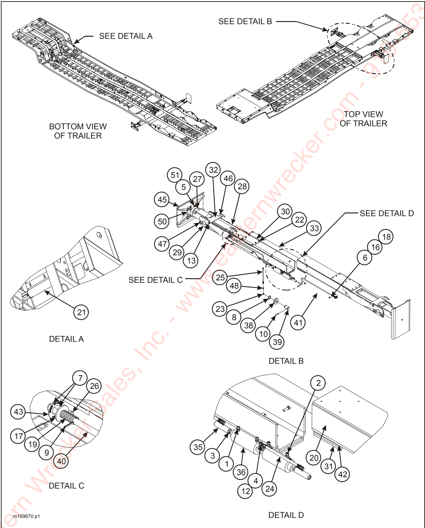
Figure 2-13: Bus Hauler Accessories (1 of 3)
