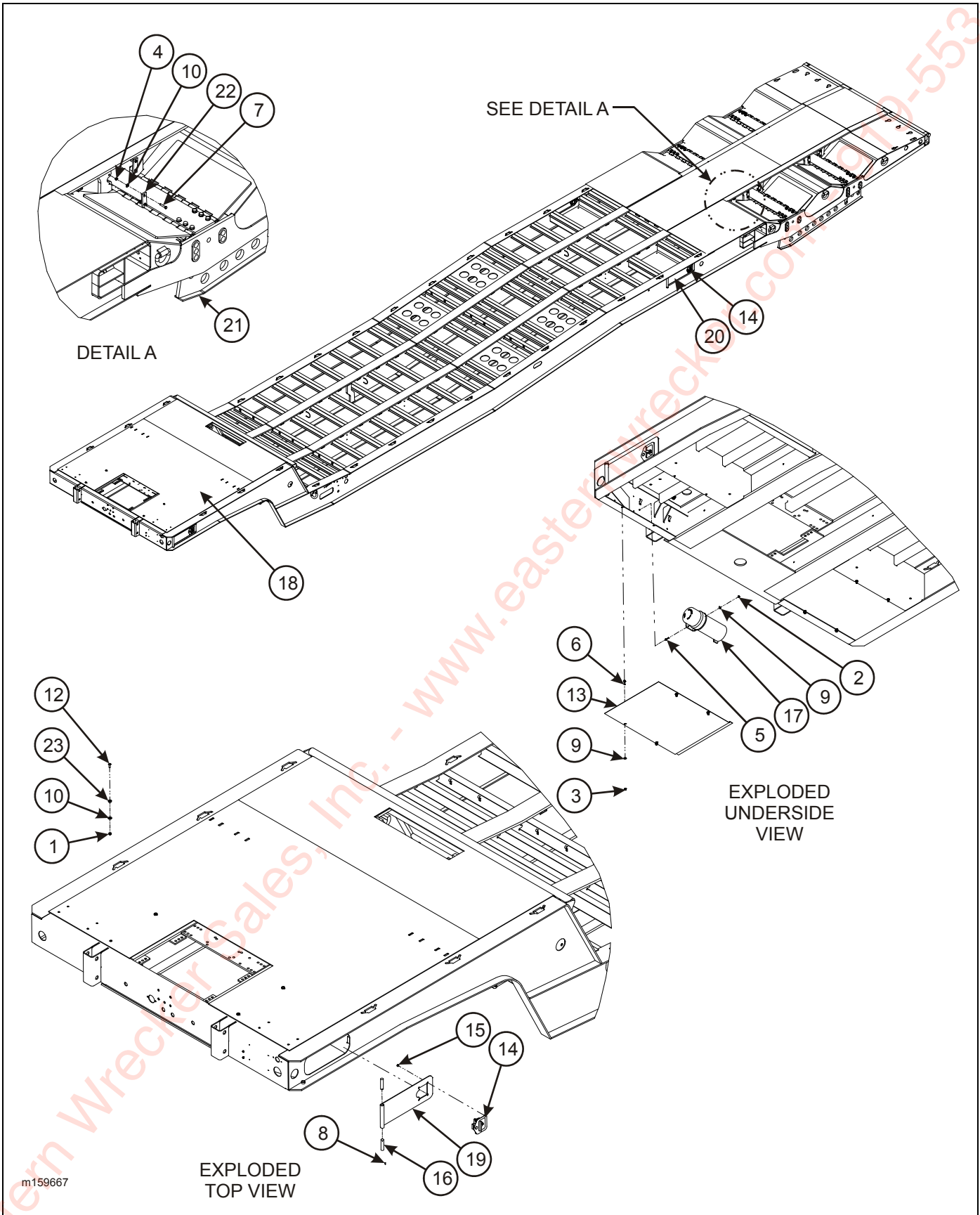
Figure 2-4: Door Latch and Toolbox Assembly
