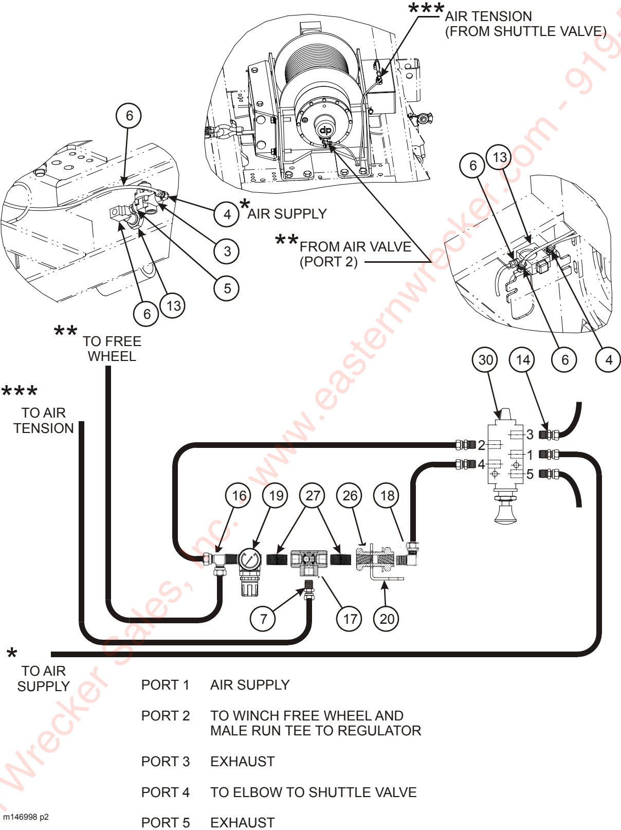
Figure 2-48: 30K Upper Deck Winch Installation (Option) (3 of 3)
