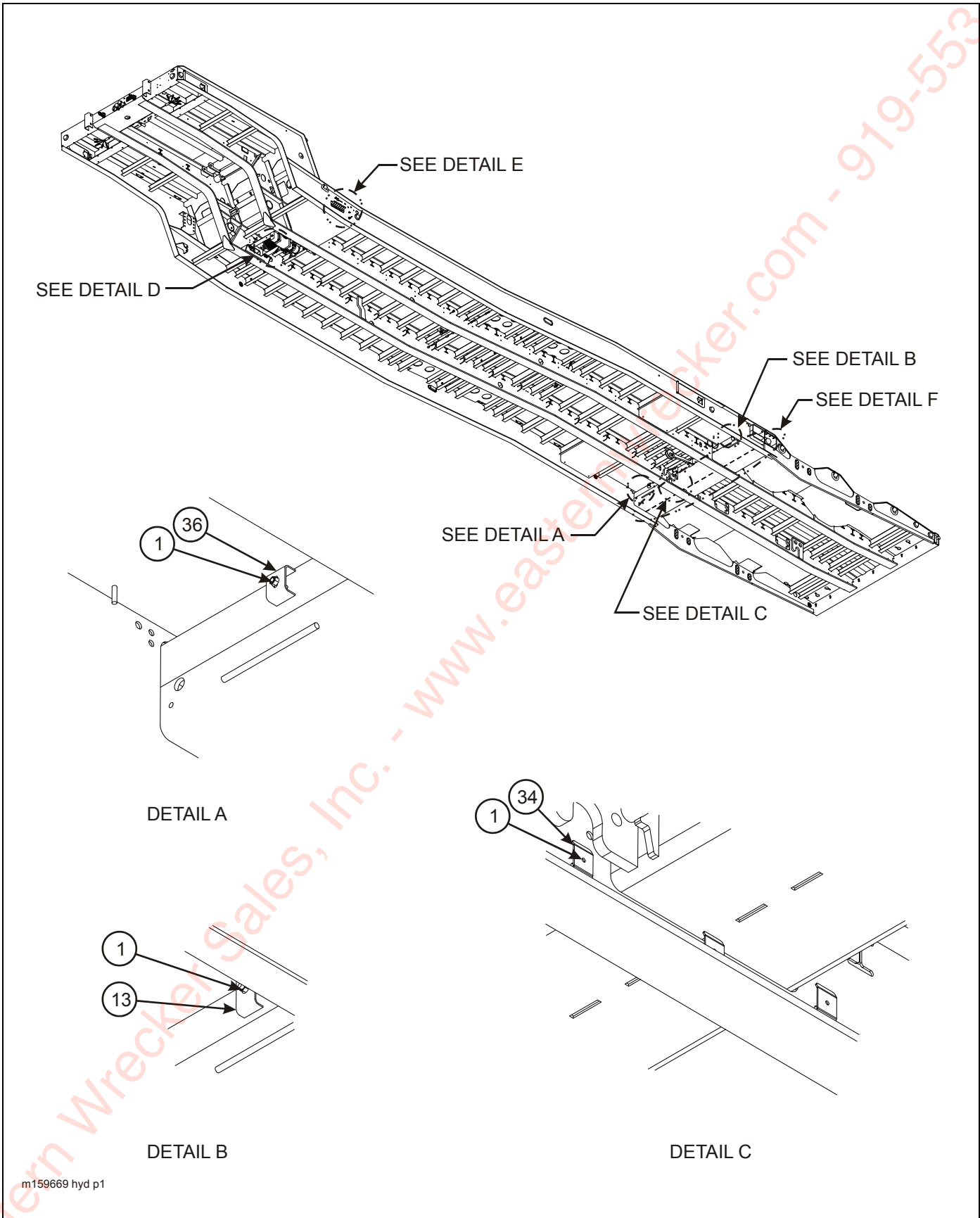
Figure 2-6: Hydraulic System (1 of 5)
