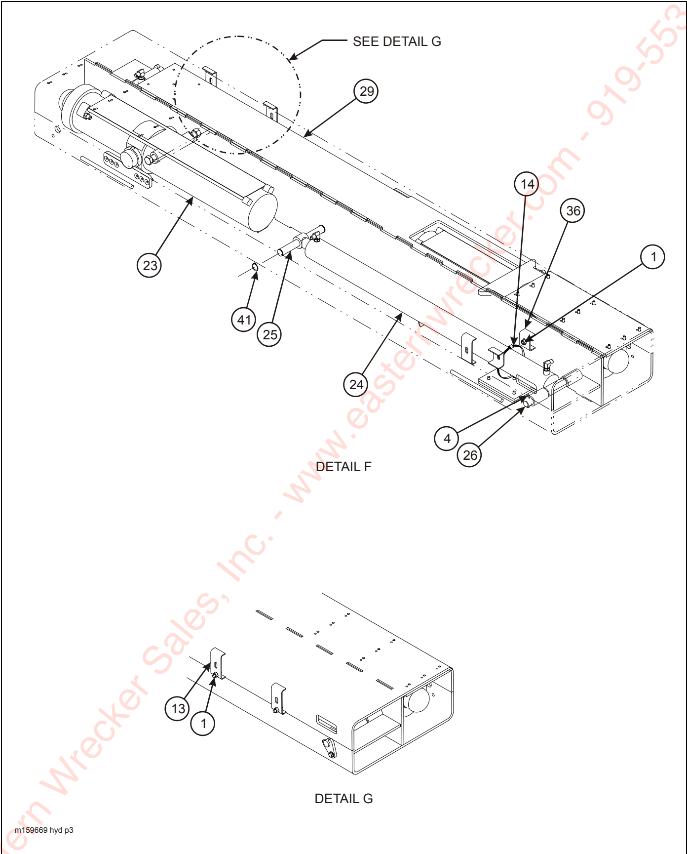
Figure 2-8: Hydraulic System (3 of 5)
