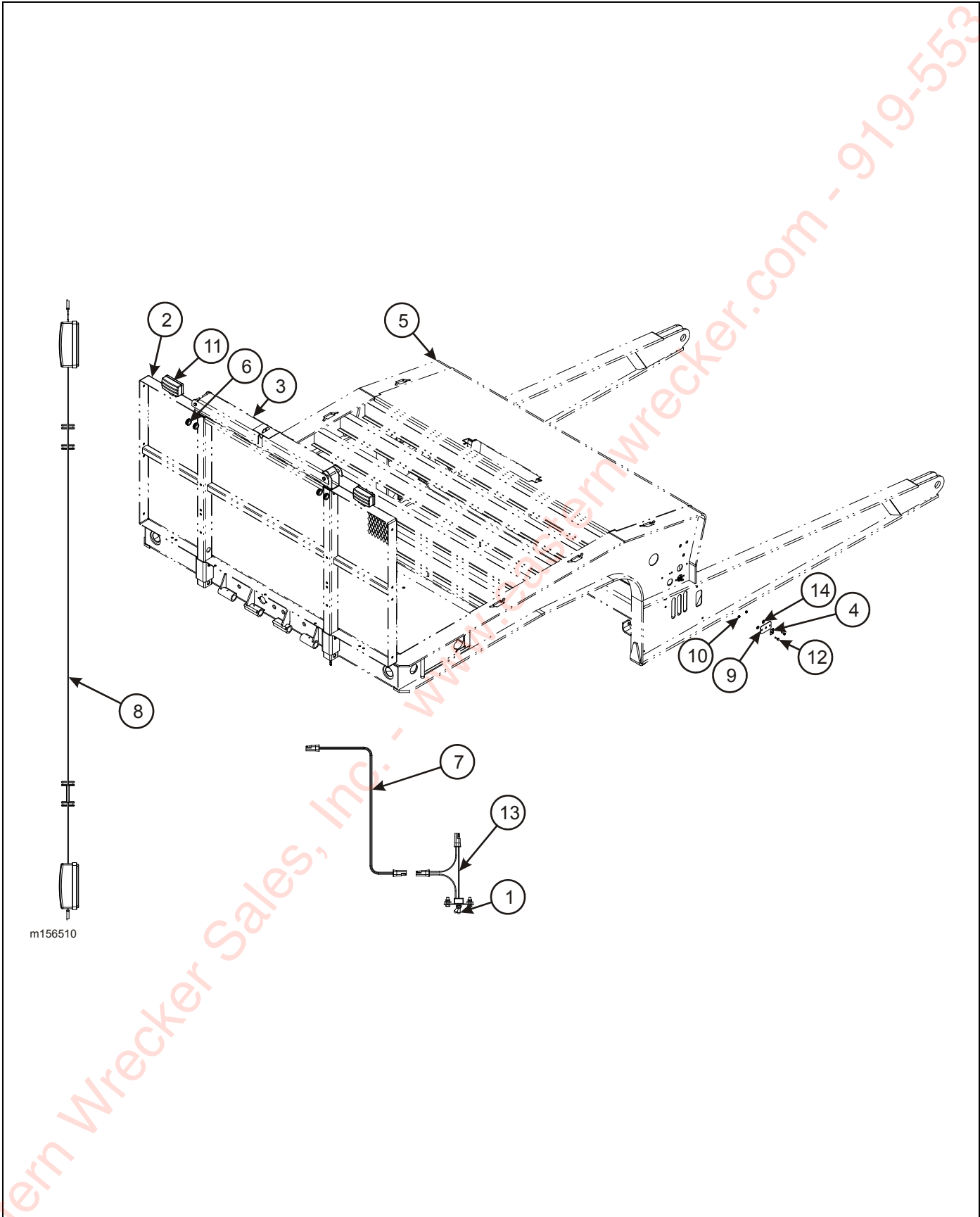
Figure 2-23: Work Light Assembly, Bulkhead (Option)
