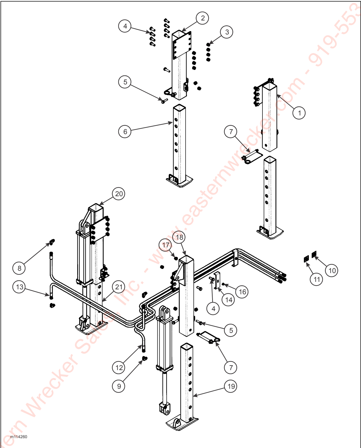
Figure 2-66: Landing Gear Installation - Bolt-On
