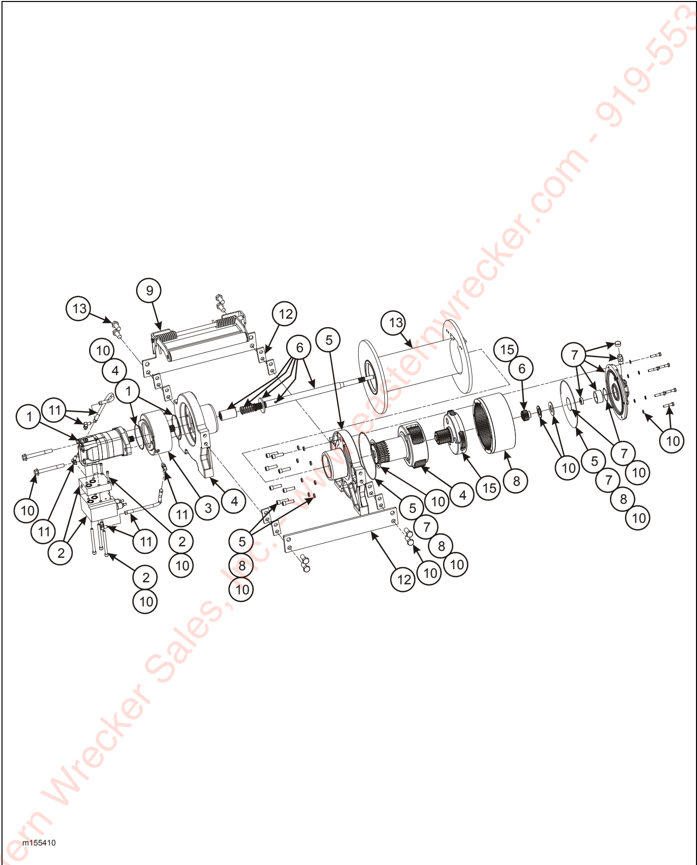
Figure 2-45: 30K Winch Items
