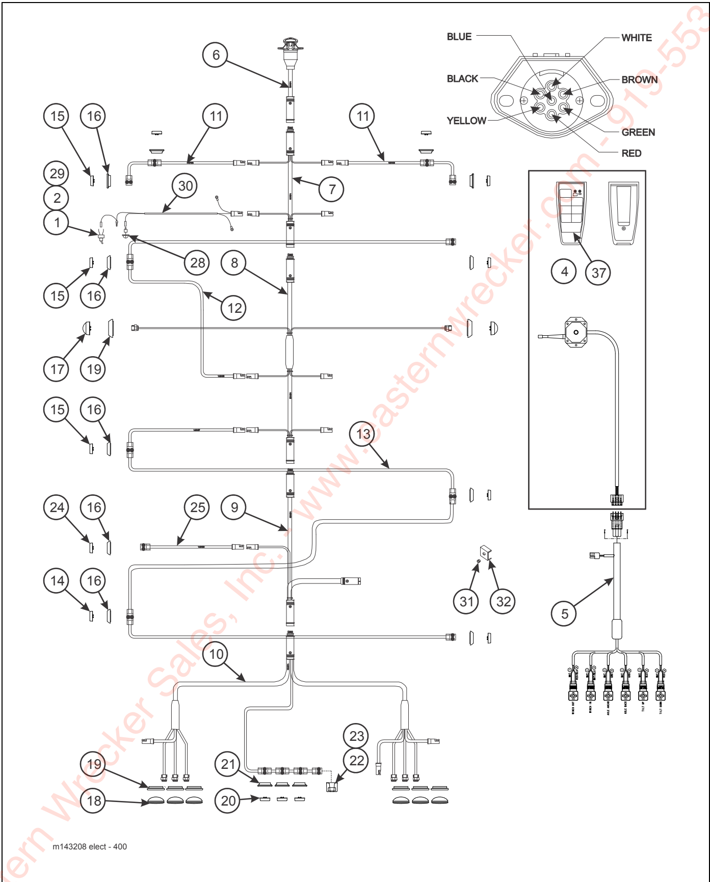
Figure 2-21: Electrical System
