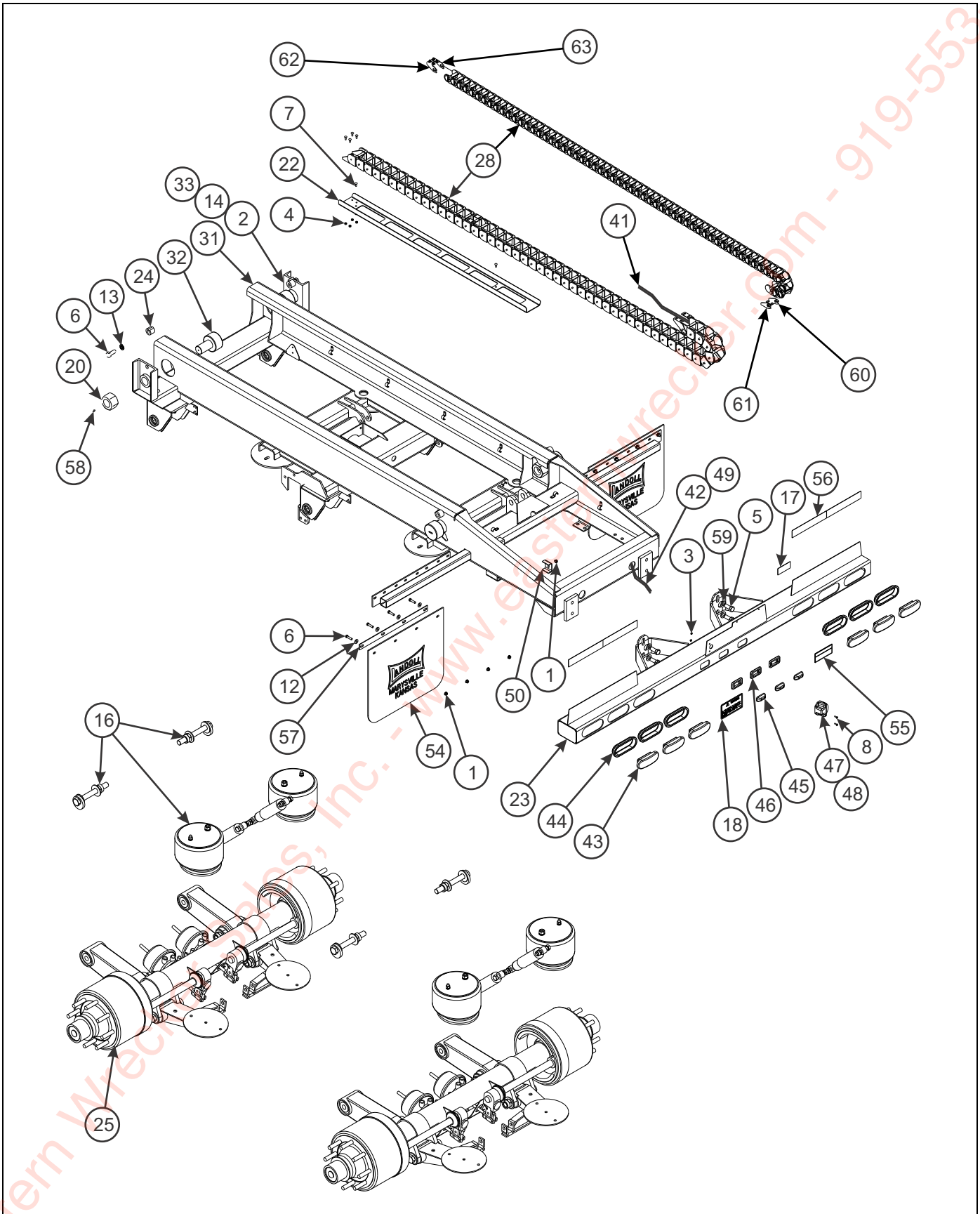
Figure 2-26: U/C Assembly, Air Ride Suspension (425 & 435) (1 of 4)
