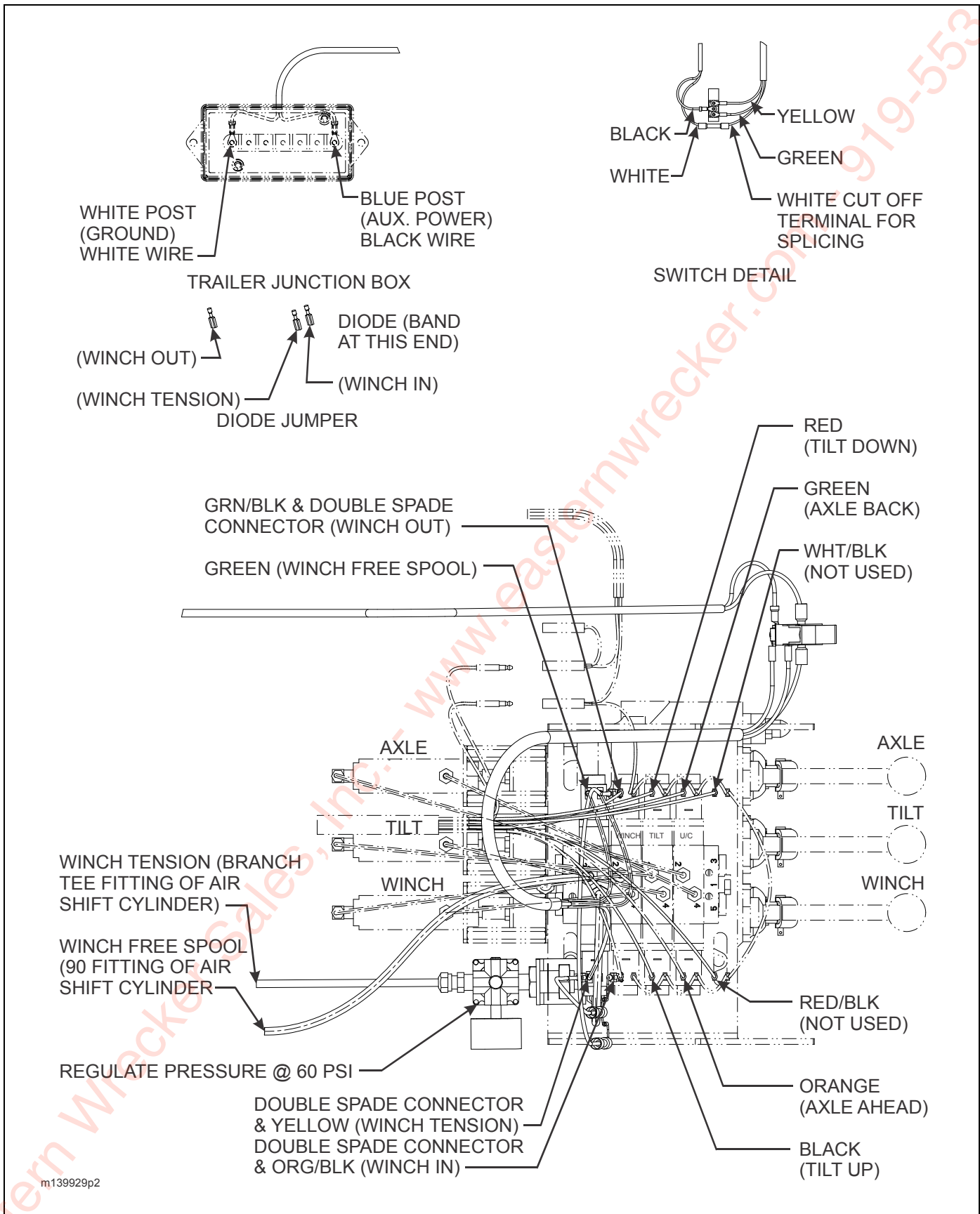
Figure 2-43: Winch Installation (2 of 2)
