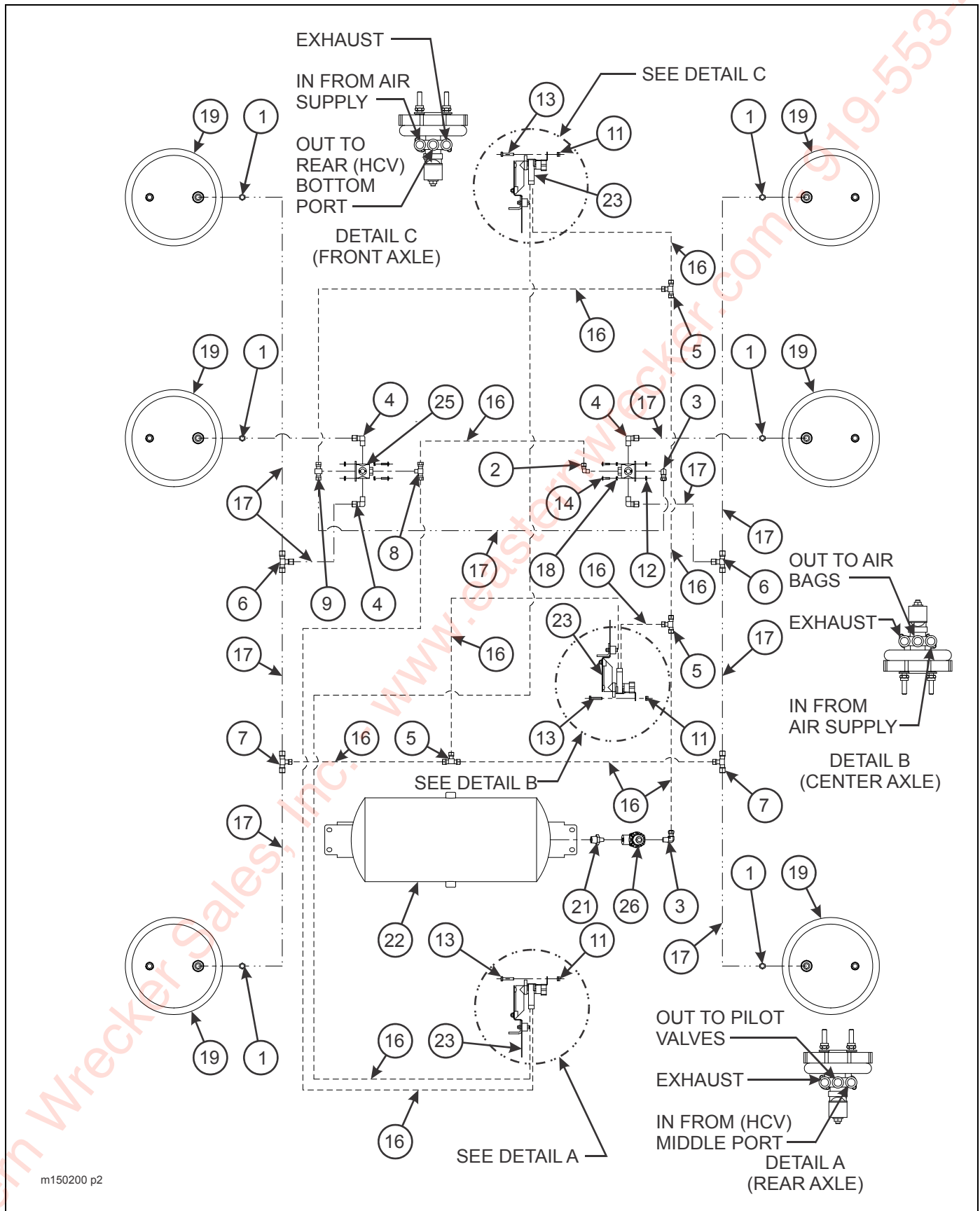
Figure 2-31: Air Ride Suspension, Air System (Triple)
