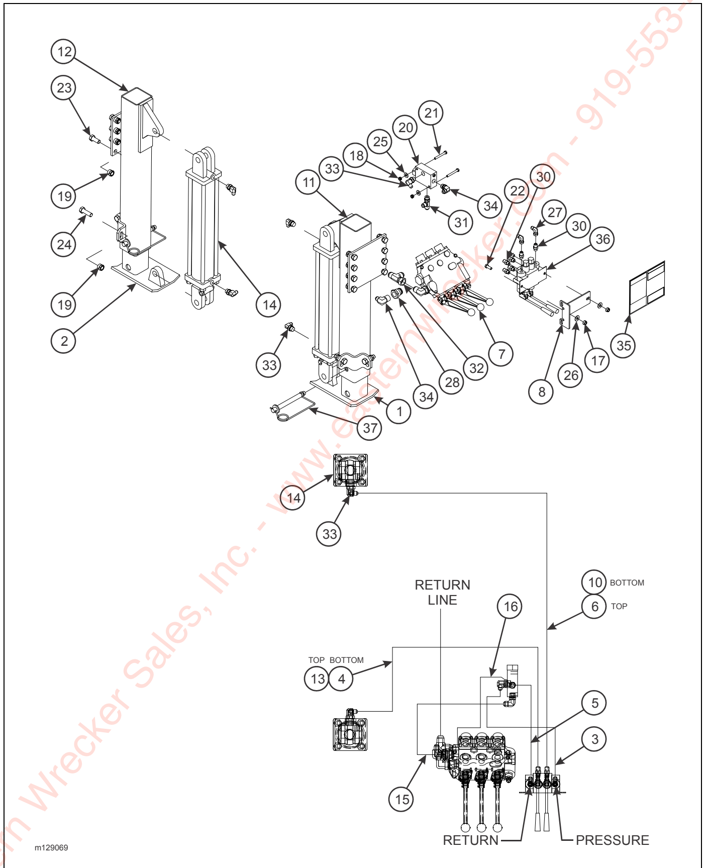
Figure 2-74: Hydraulic Park Stand Installation
