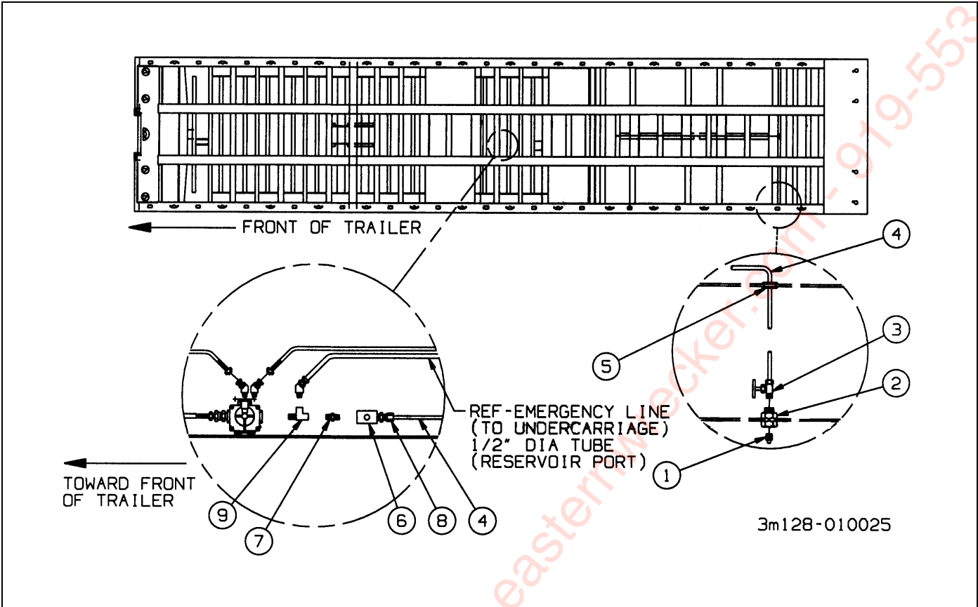
Figure 2-84: Air Outlet Accessory (Option)
