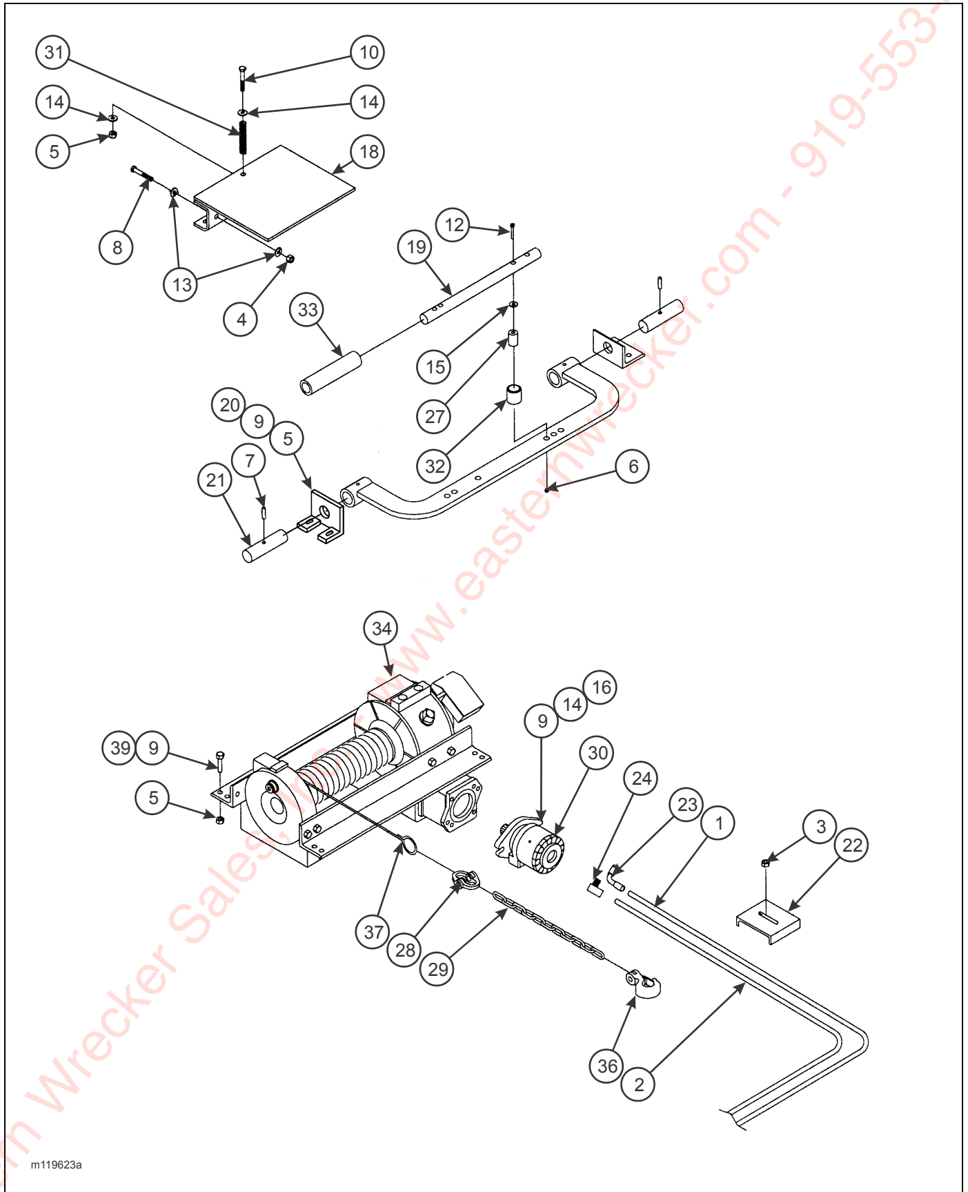
Figure 2-44: Winch Installation, Spring Tension Cable Roller
