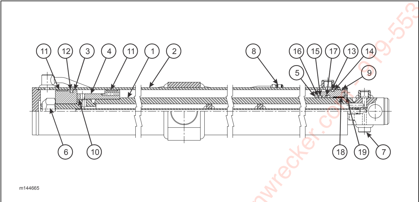
Figure 2-14: Cylinder, Hydraulic 4 x 126 Ported Rod (Streetside) (410-50/53/55HD, 435-48/50CA)
