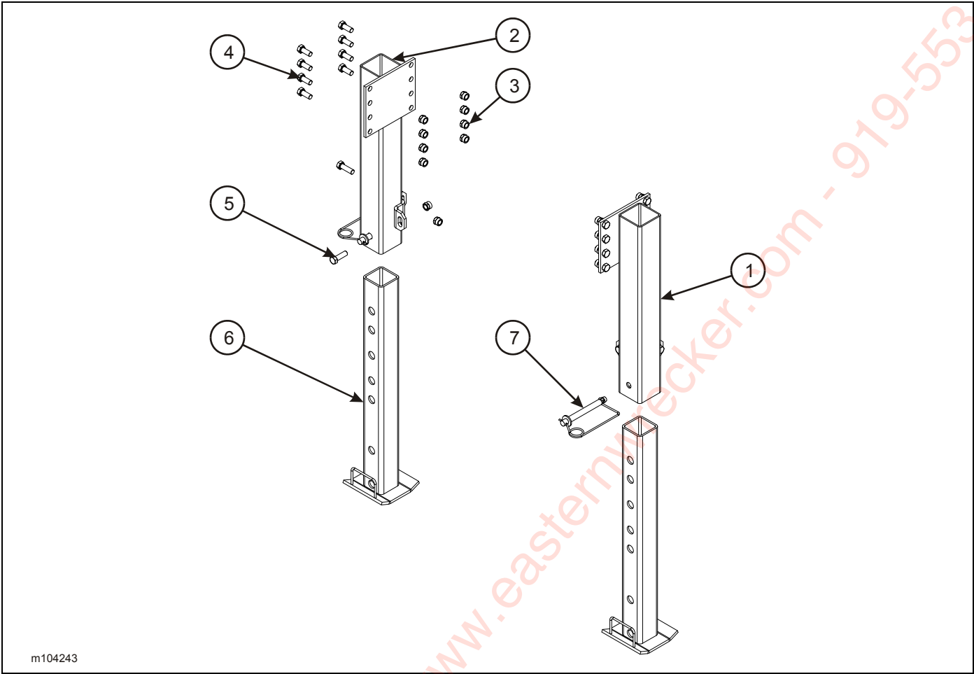
Figure 2-73: Landing Gear Installation
