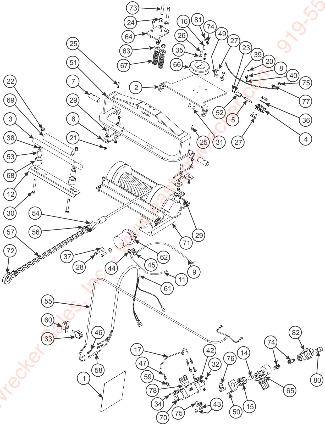
Figure 2-42: Winch Installation (1 of 2)
