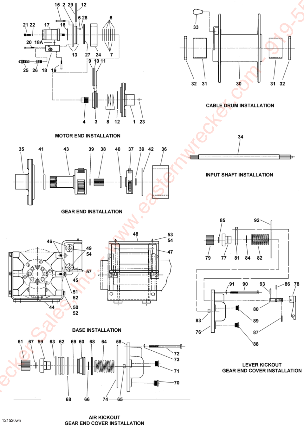
Figure 2-59: 12K, 15K, & 20K Winch Items (DP Planetary)
