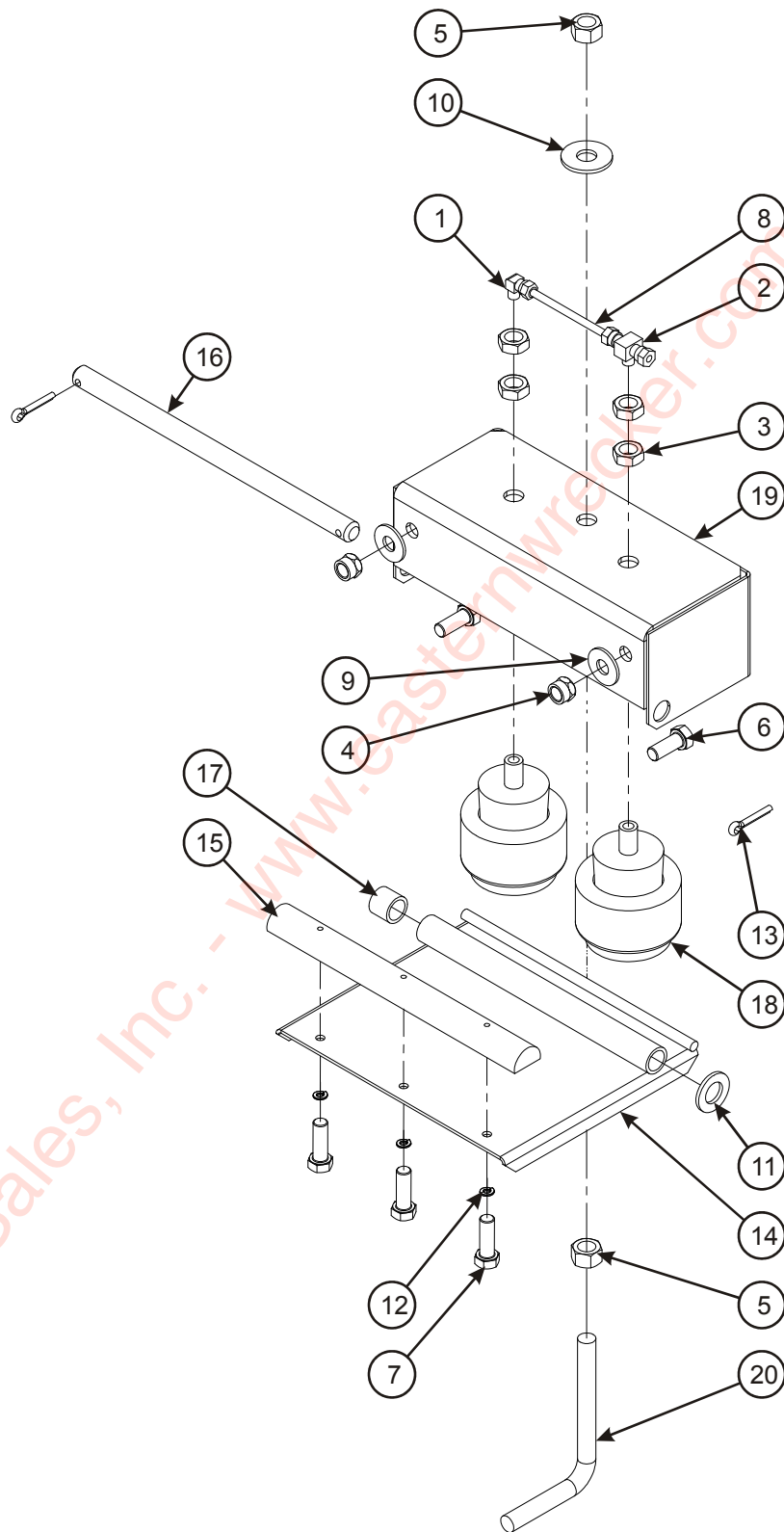
Figure 2-56: Winch, Cable Air Tension
