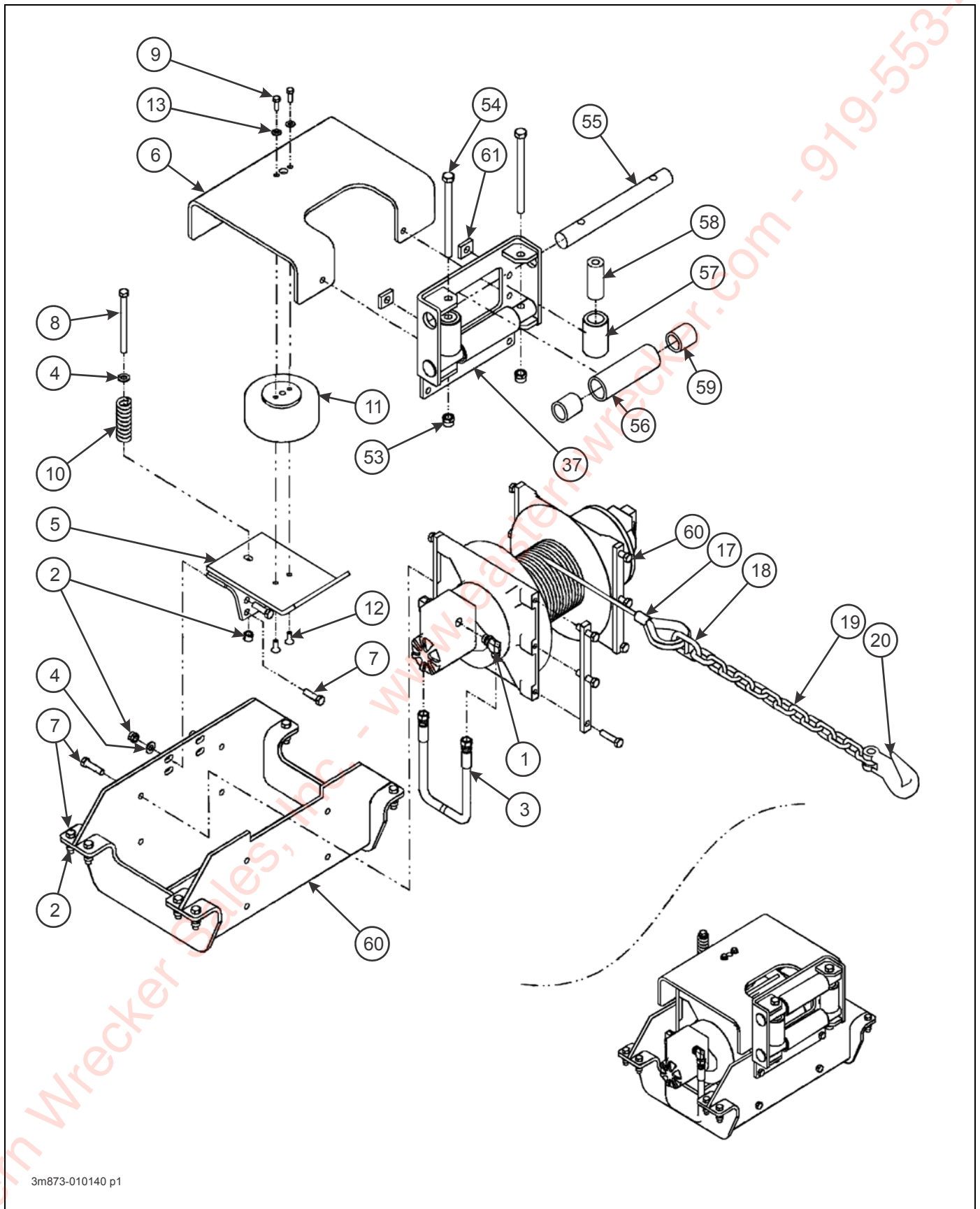
Figure 2-57: 12K, 15K, & 20K Upper Deck Winch (DP) (1 of 2)
