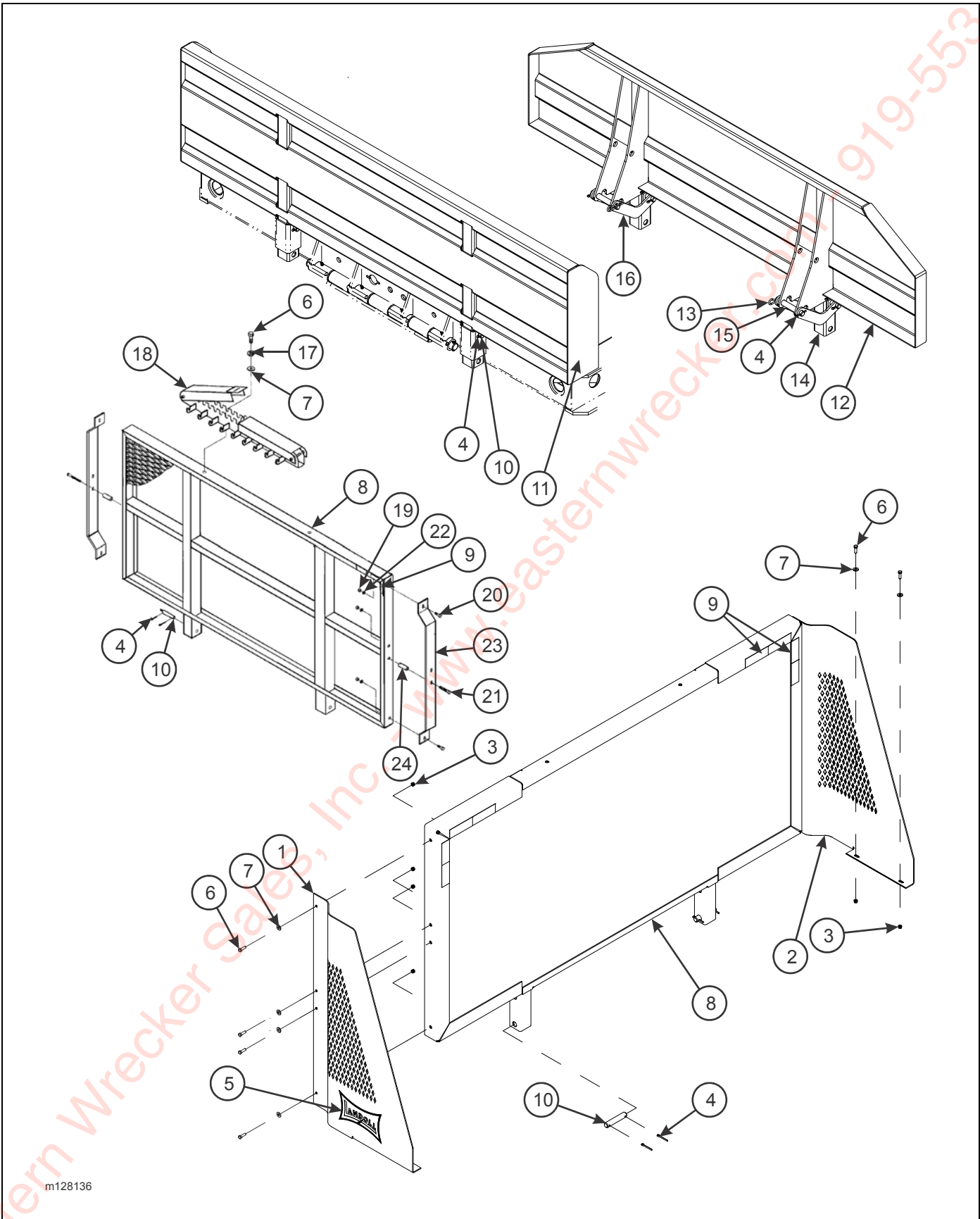
Figure 2-4: Bulkhead Assembly
