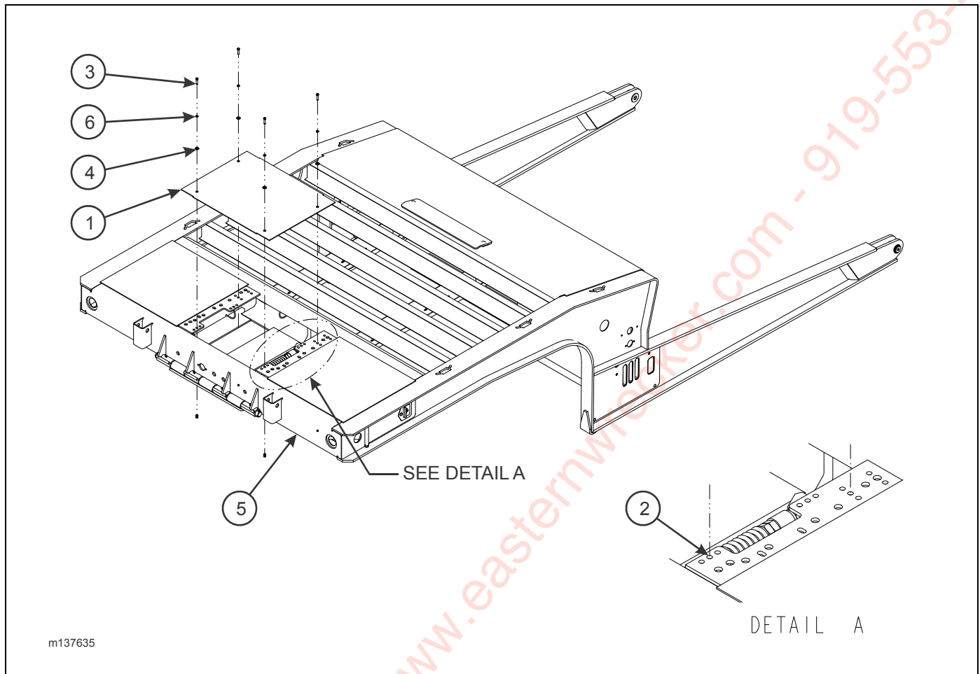
Figure 2-60: Upper Deck Cover Assembly (Option)
