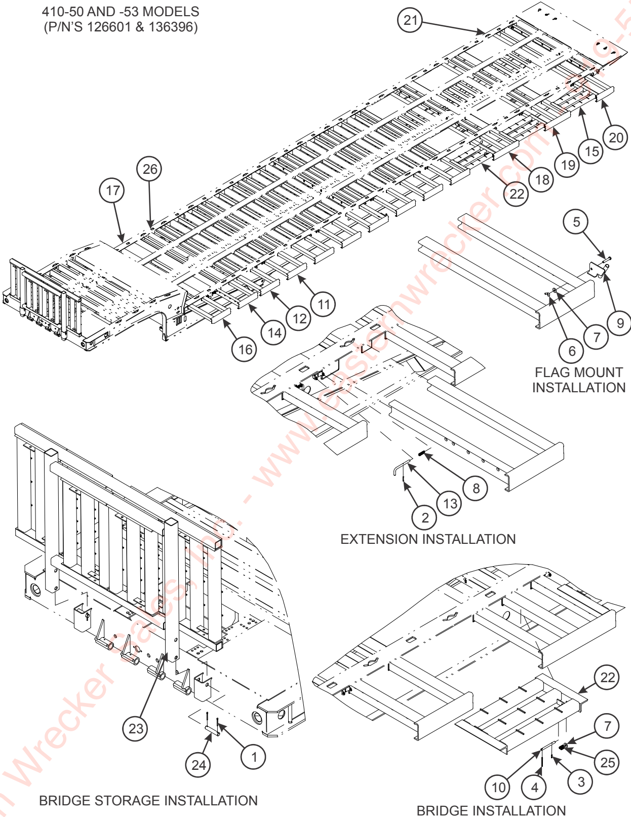
Figure 2-5: Pullout Installation (1 of 2)
