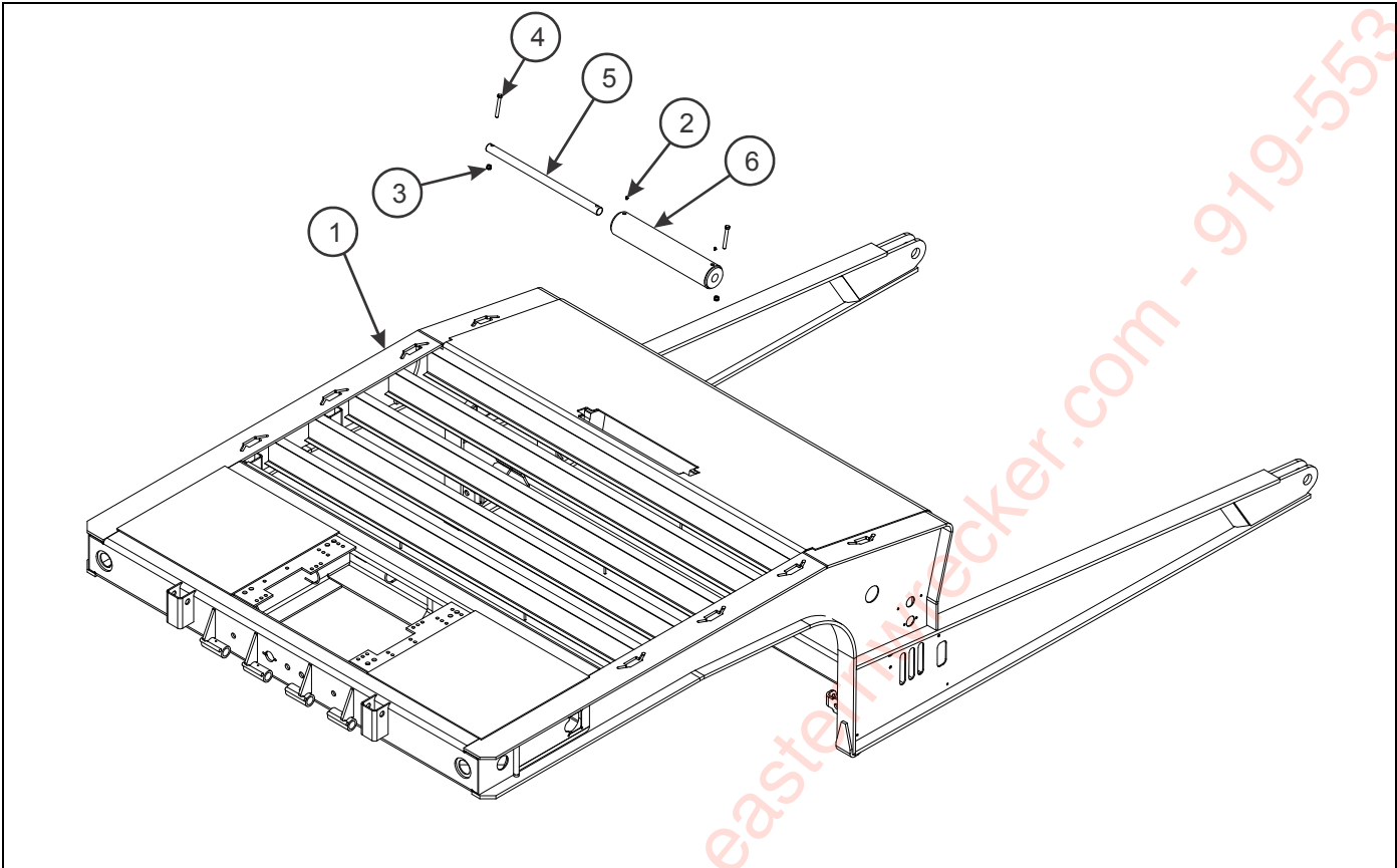
Figure 2-92: Upper Deck Extension Bridge Storage Rack (Option)
