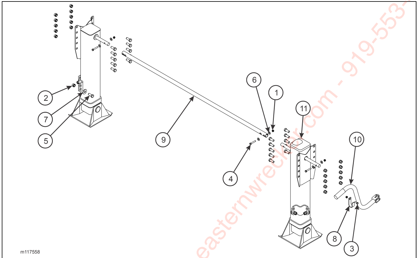
Figure 2-72: Landing Gear Installation
