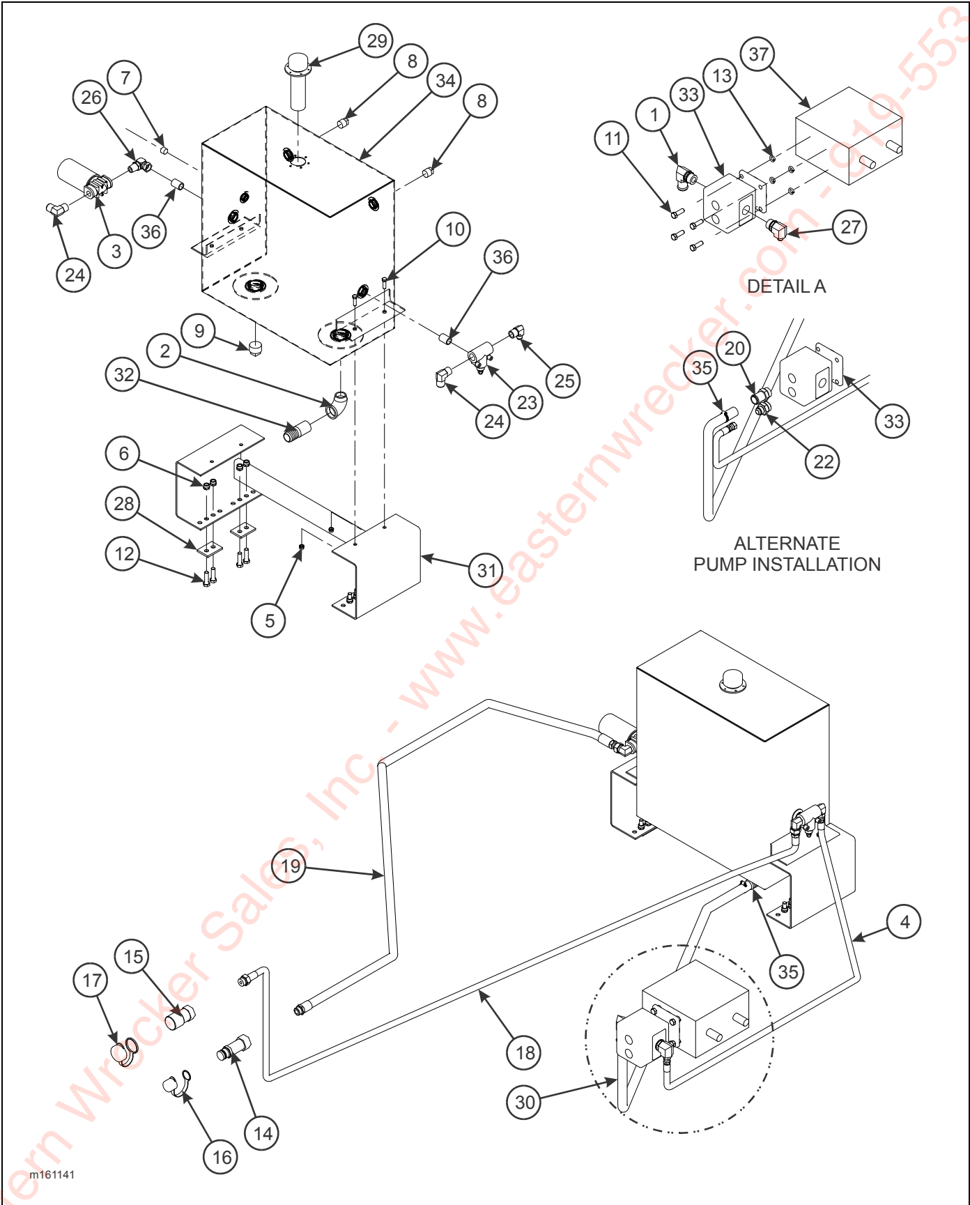
Figure 2-20: 30 Gallon Hydraulic Wet Kit Items
