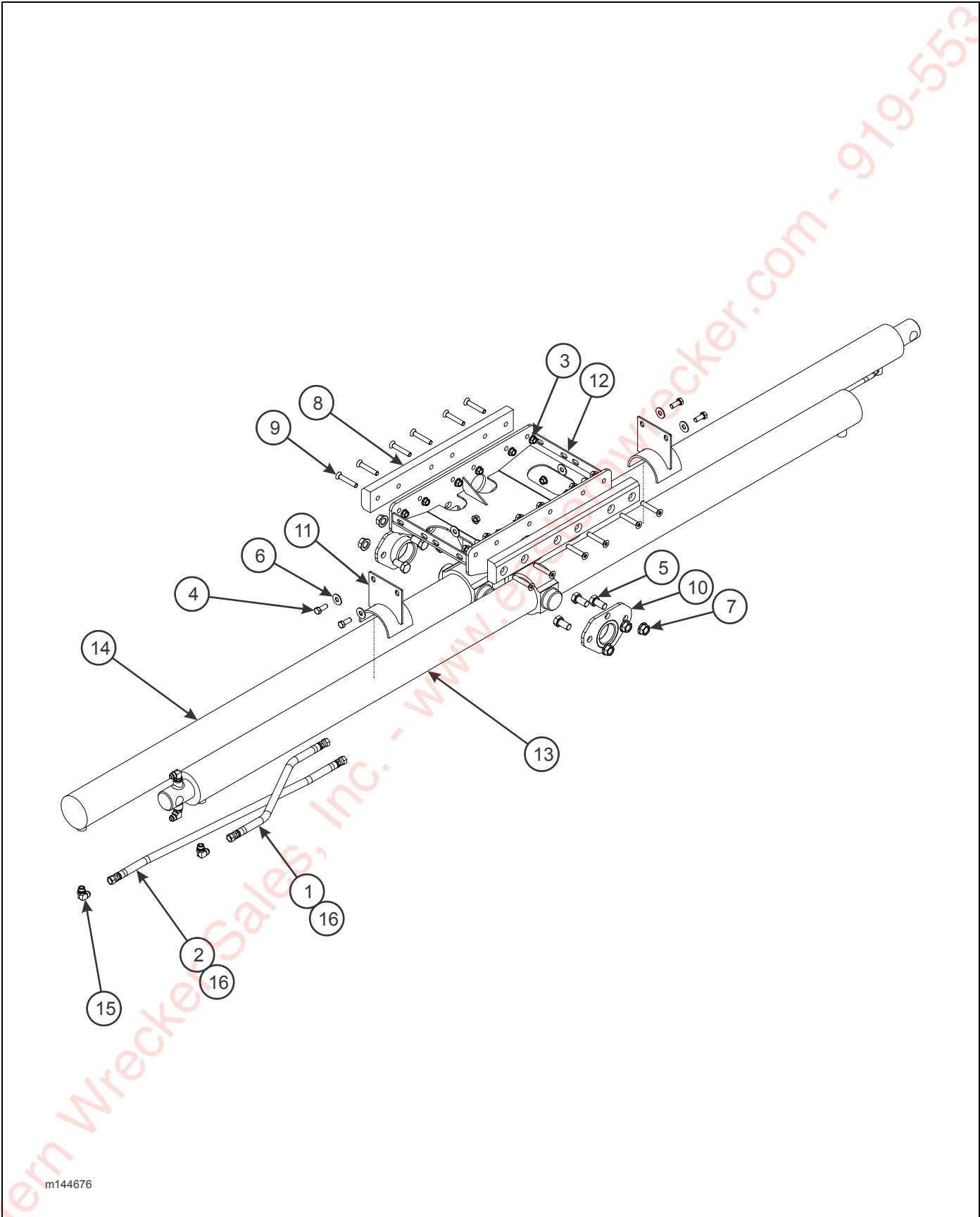
Figure 2-11: U/C Cylinder Assembly
