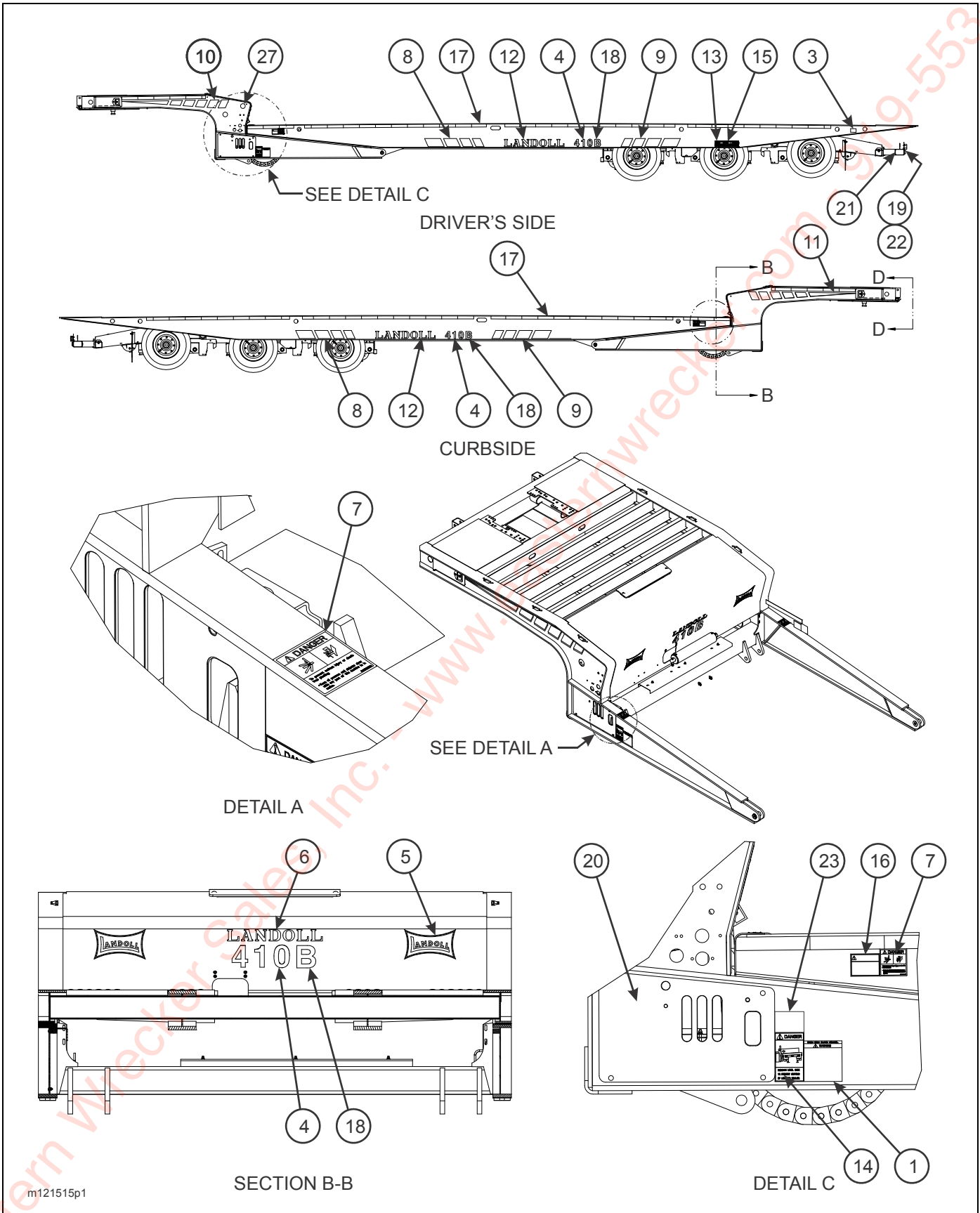
Figure 2-70: Decal Installation (1 of 2)
