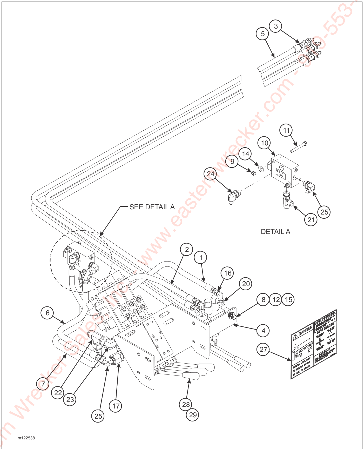
Figure 2-62: Dock Leveler Hydraulic Installation (Option)
