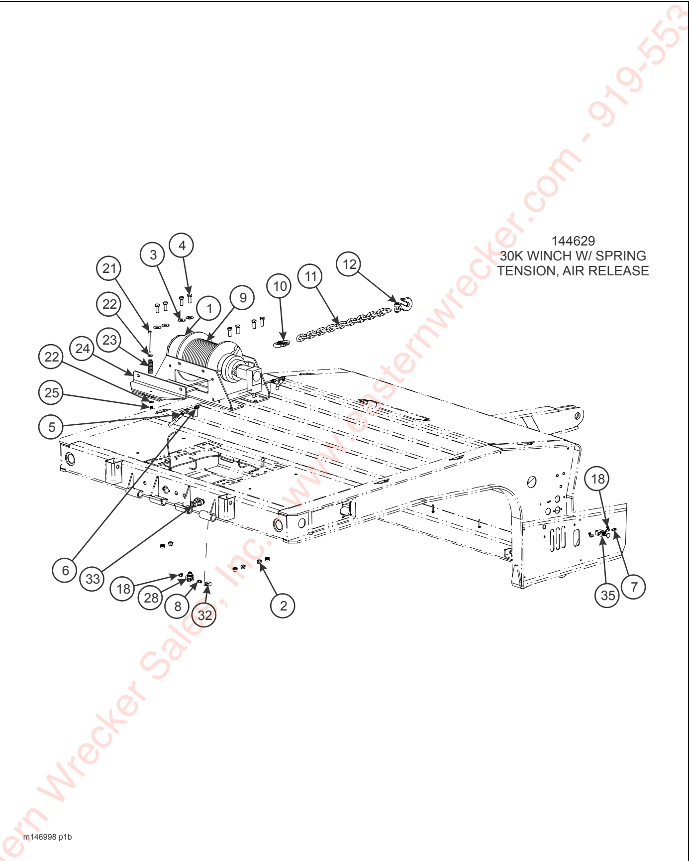
Figure 2-50: 30,000 Lb. Upper Deck Winch Installation (2 of 3)
