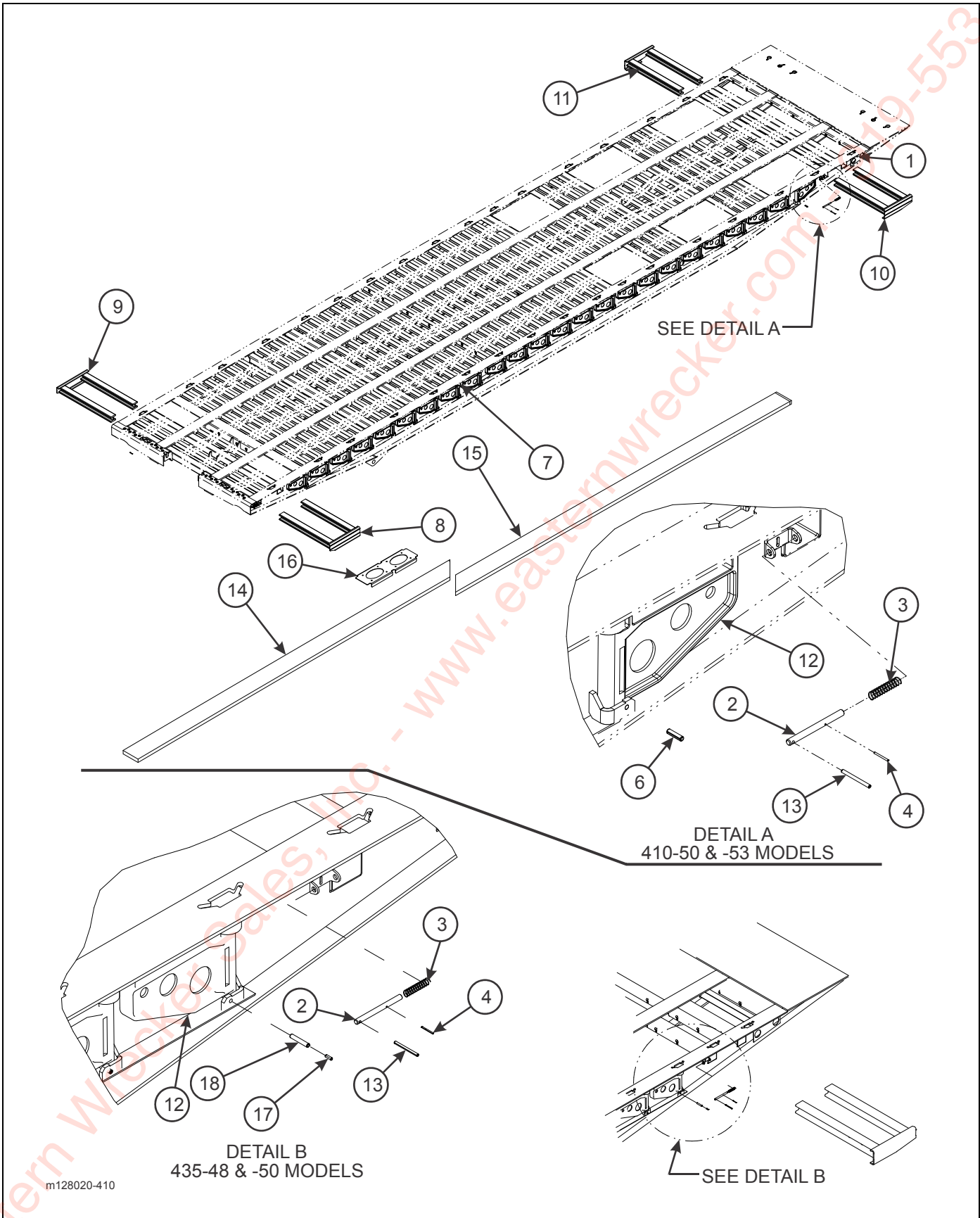
Figure 2-7: Outrigger Installation (Option)
