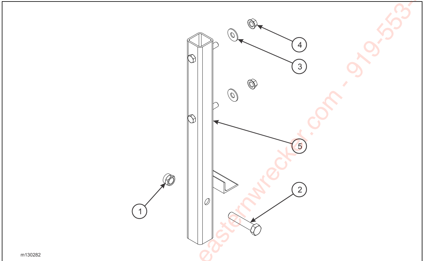
Figure 2-91: Spare Tire Mount Assembly
