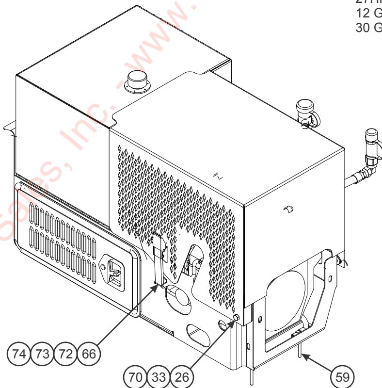
Figure 2-77: Upper Deck Engine Installation (1 of 4)
