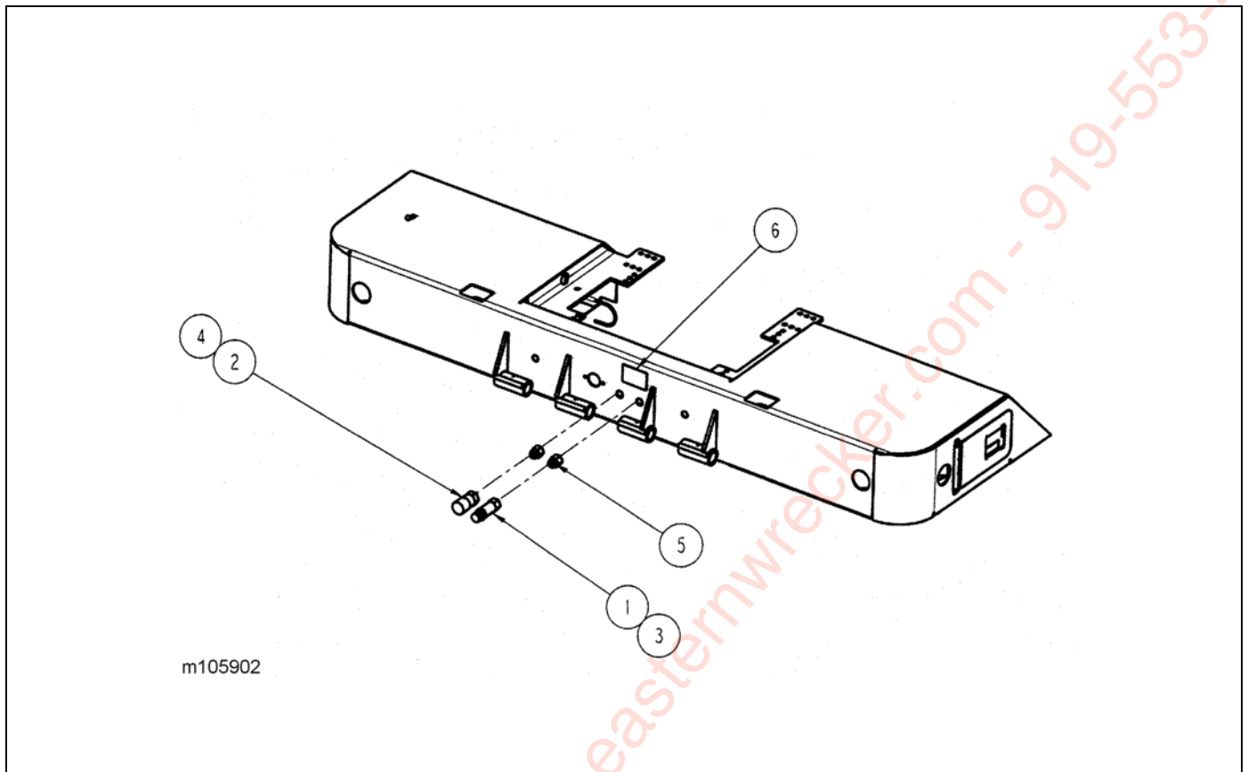
Figure 2-89: Hydraulic Conversion Kit, Ball to Flat (Option)
