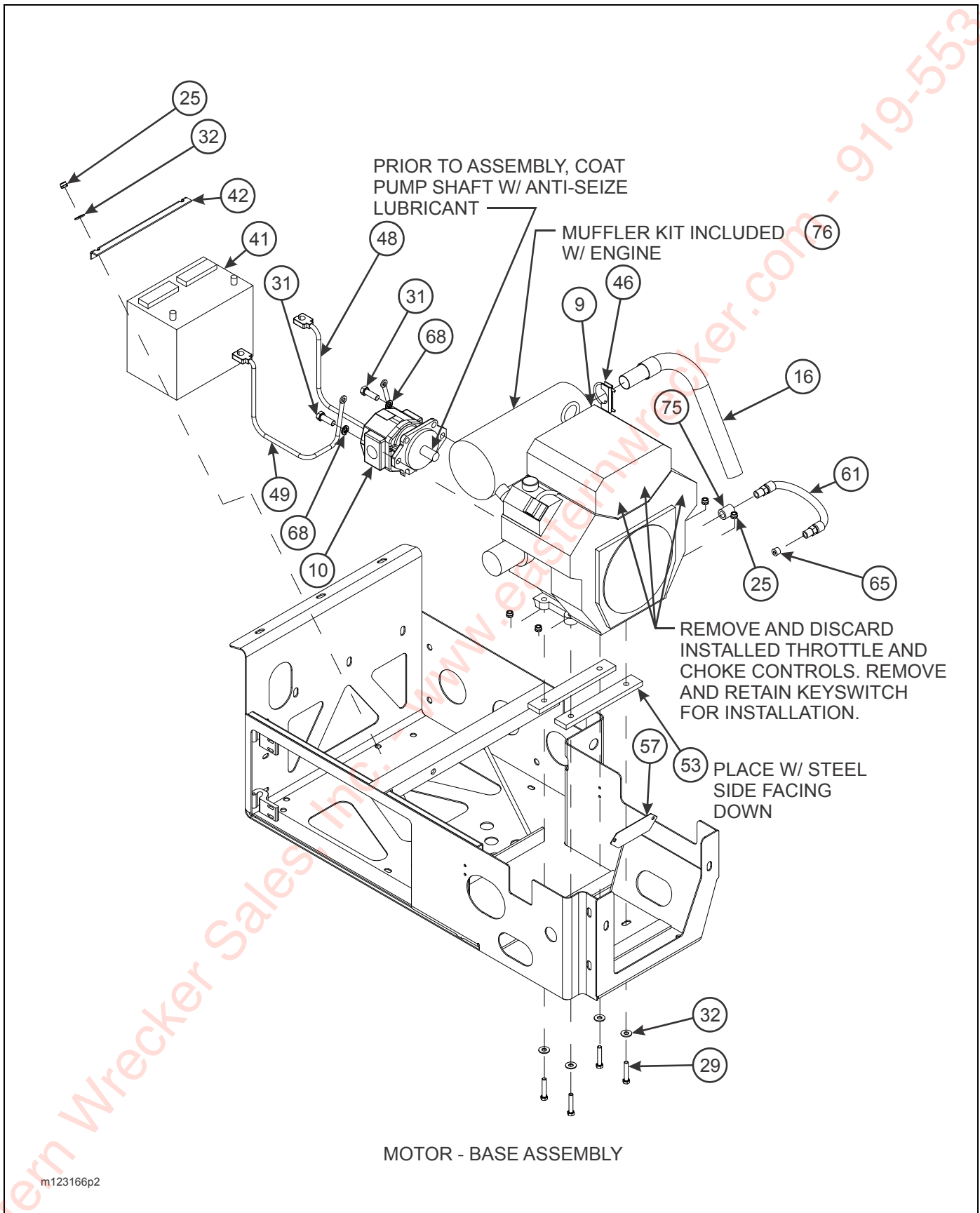
Figure 2-78: Upper Deck Engine Installation (2 of 4)
