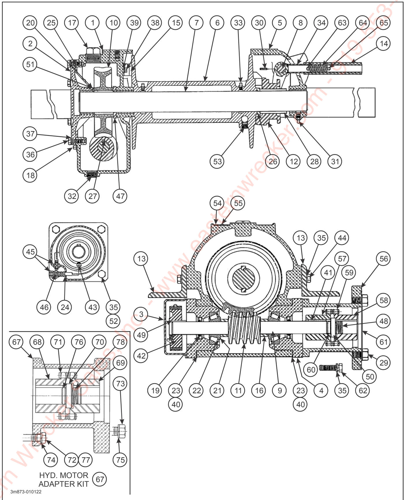
Figure 2-45: 12,000 Lb. Winch Items
