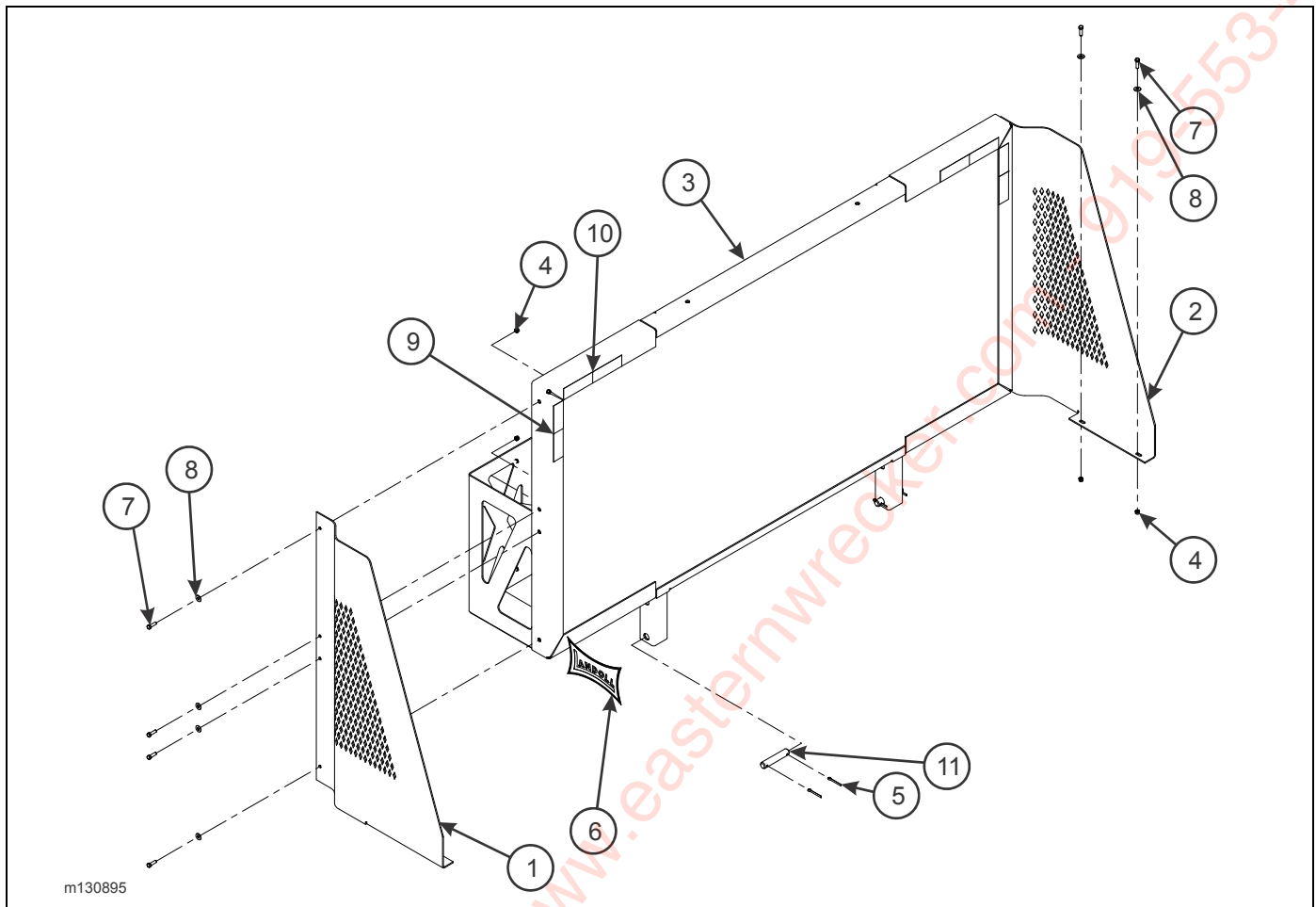
Figure 2-87: Special Bulkhead Installation (Option)
