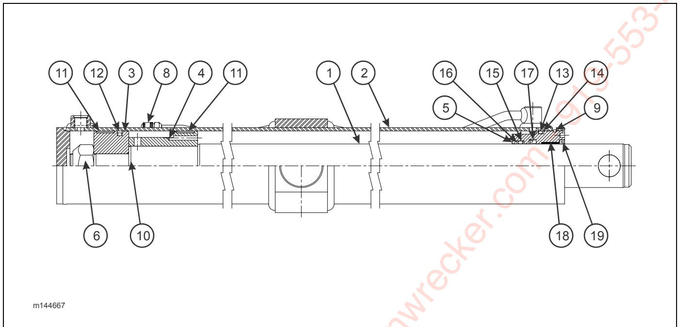
Figure 2-15: Cylinder, Hydraulic 4 x 126 (Curbside) (410-50/53/55HD, 435-48/50CA)
