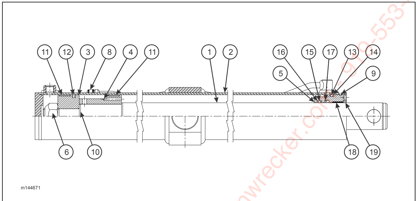
Figure 2-17: Cylinder, Hydraulic 4 x 138 (Curbside) (435-53)
