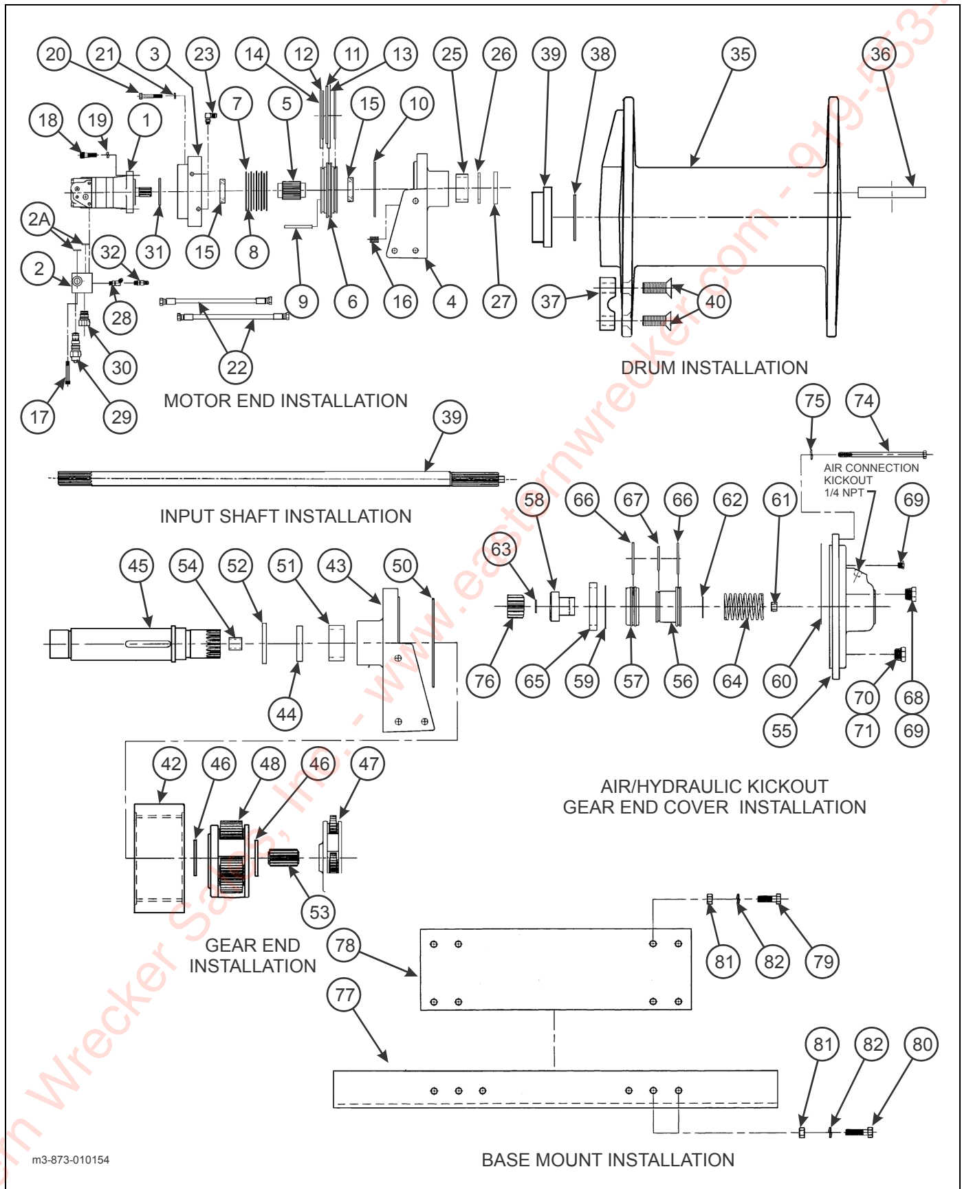
Figure 2-54: 30,000 Lb. Winch Items
