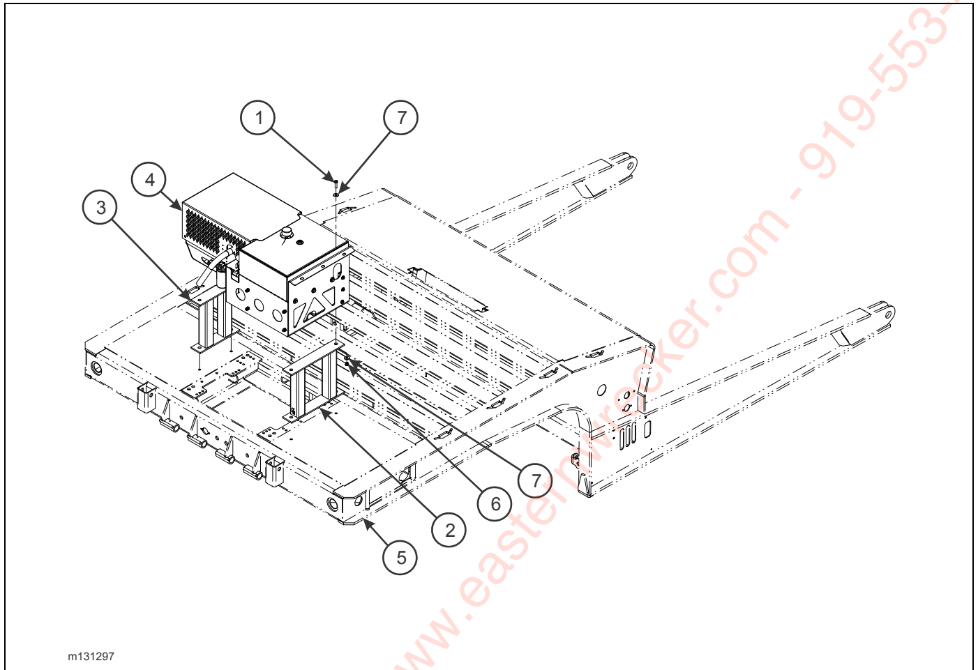
Figure 2-81: Upper Deck Engine Stand Installation
