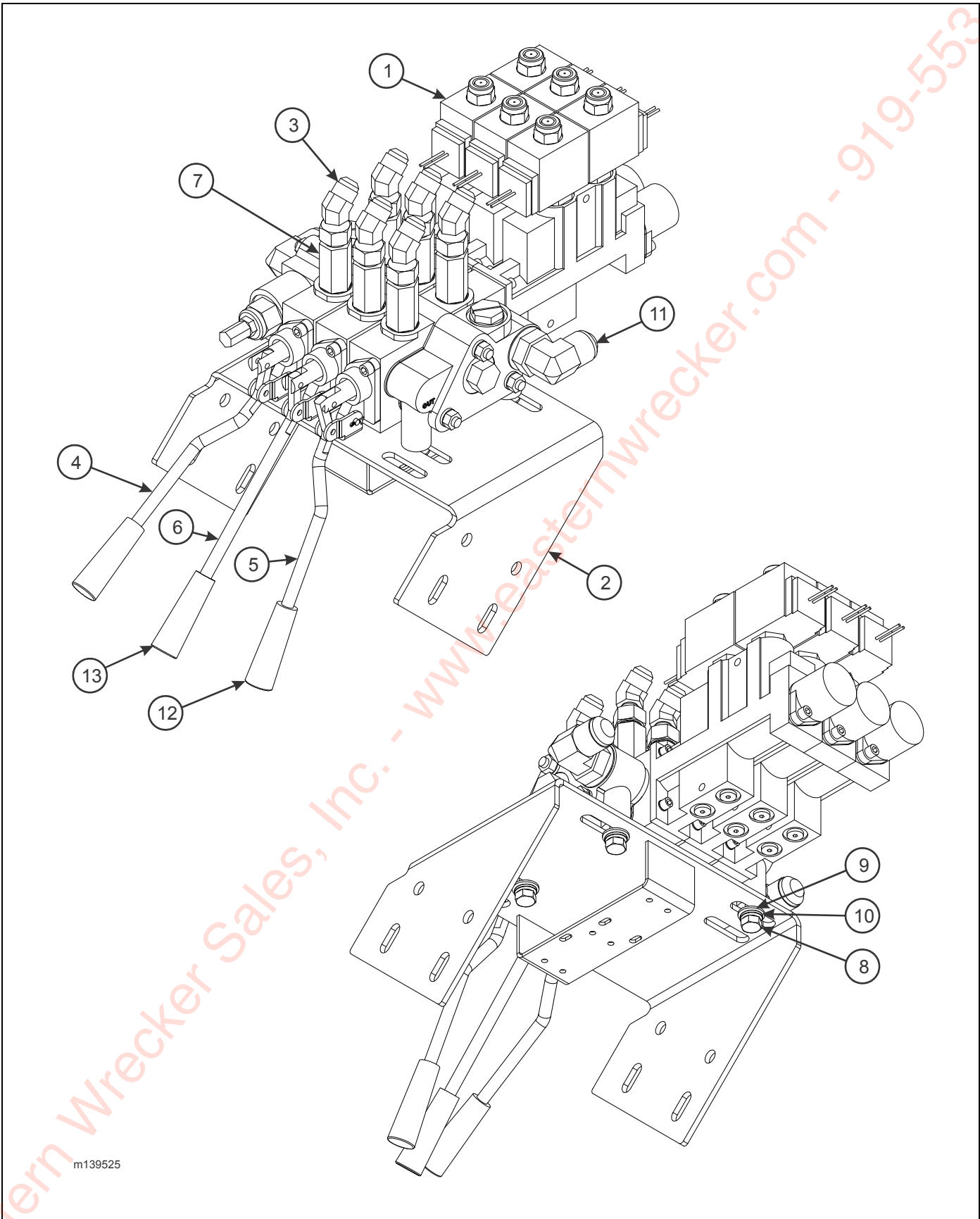
Figure 2-9: Three Spool Valve Assembly
