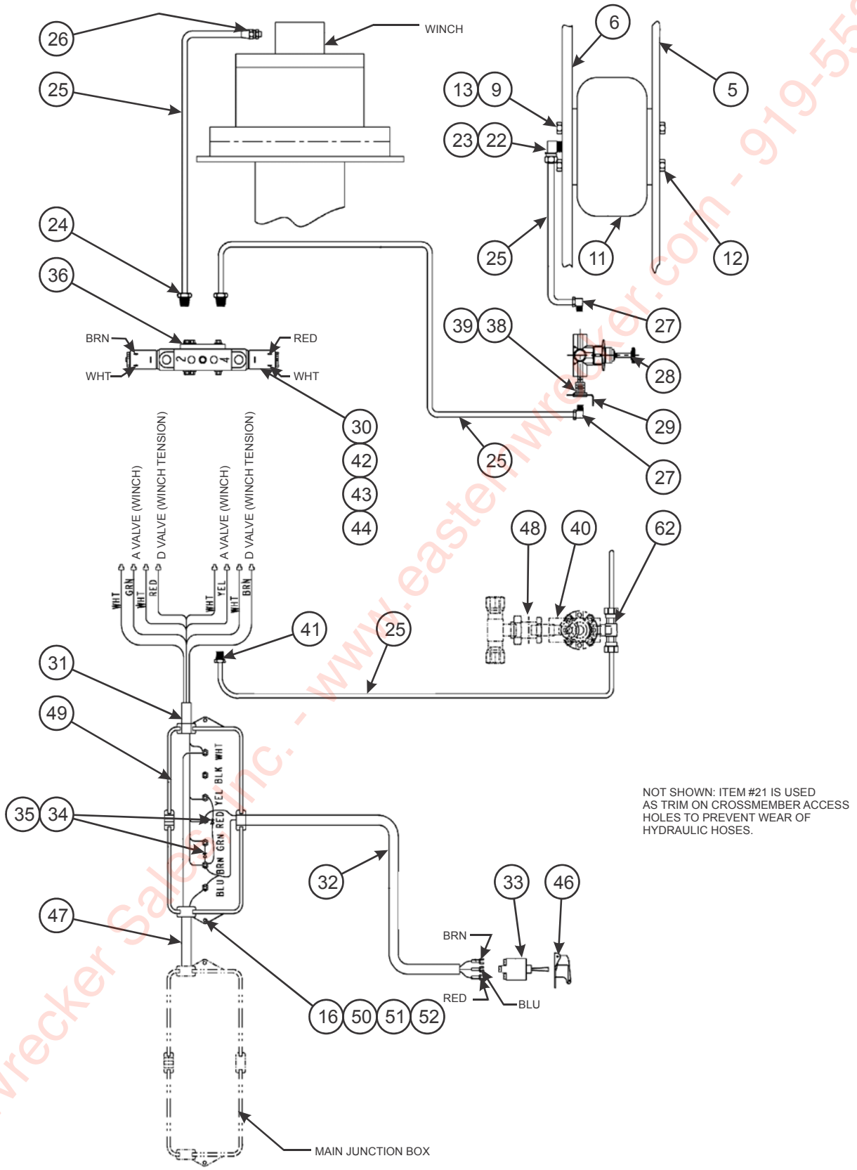
Figure 2-58: 12K, 15K, & 20K Upper Deck Winch (DP) (2 of 2)
