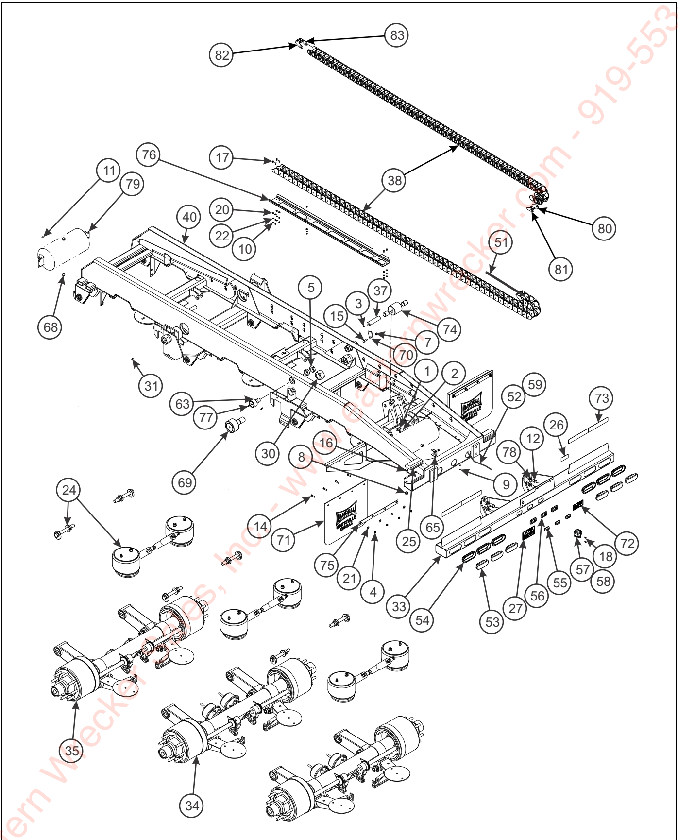
Figure 2-22: U/C Assembly, Air Ride Suspension (410) (1 of 4)
