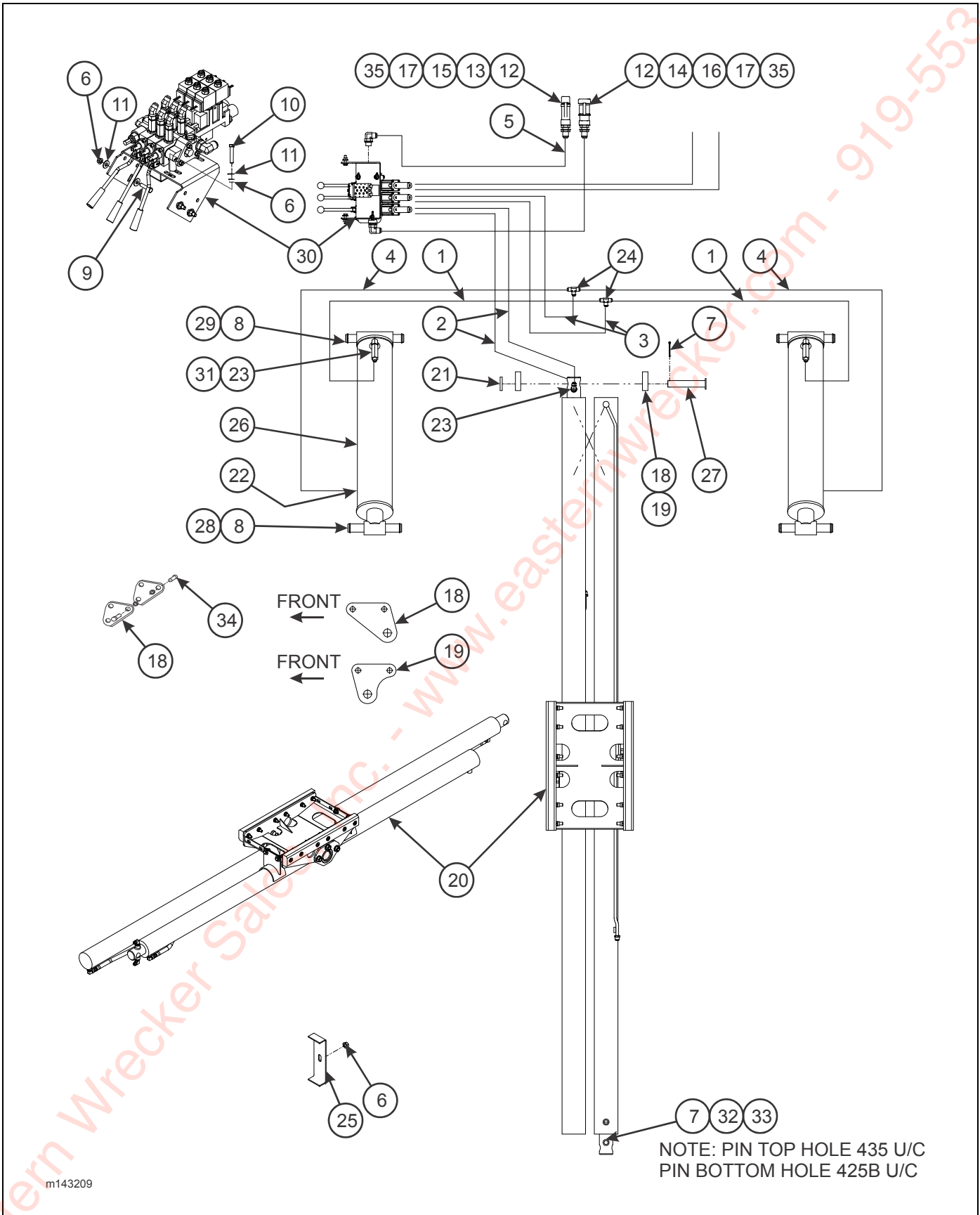
Figure 2-8: Hydraulic System
