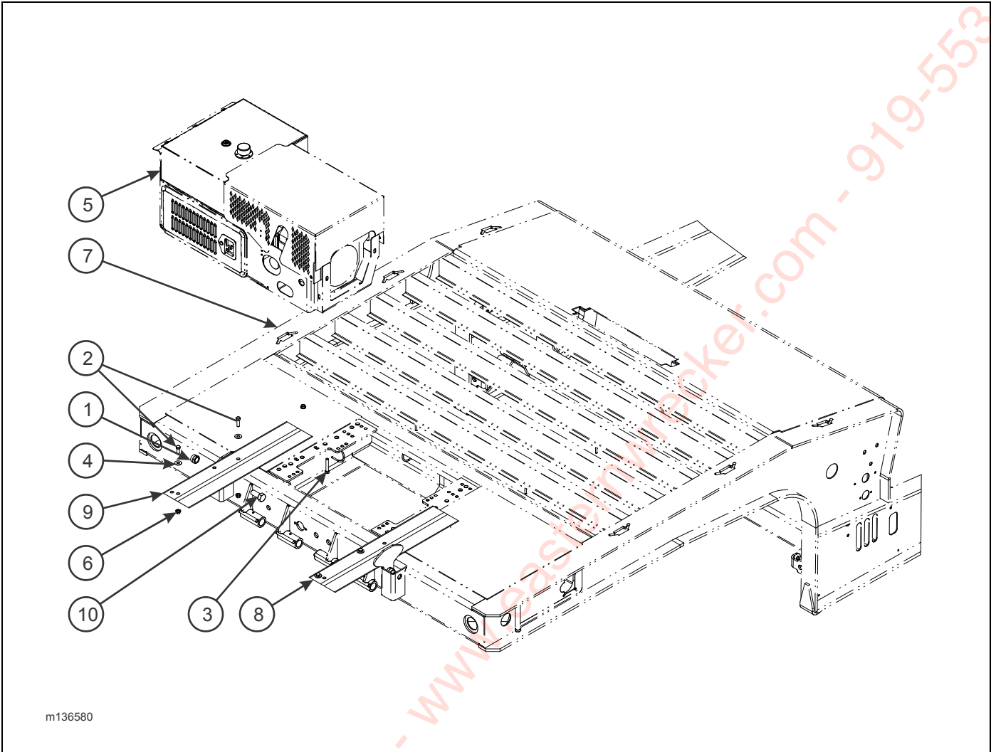
Figure 2-82: Upper Deck Engine Stand Installation
