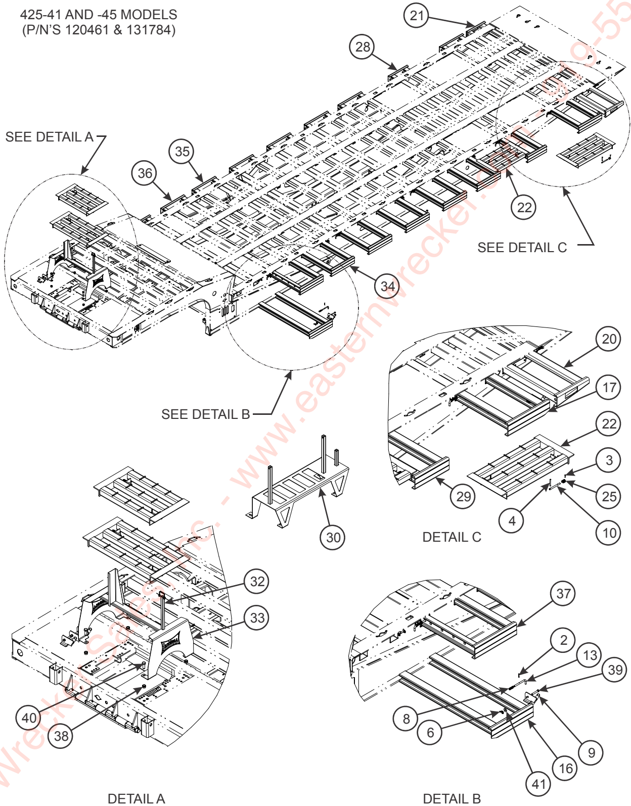
Figure 2-6: Pullout Installation (2 of 2)
