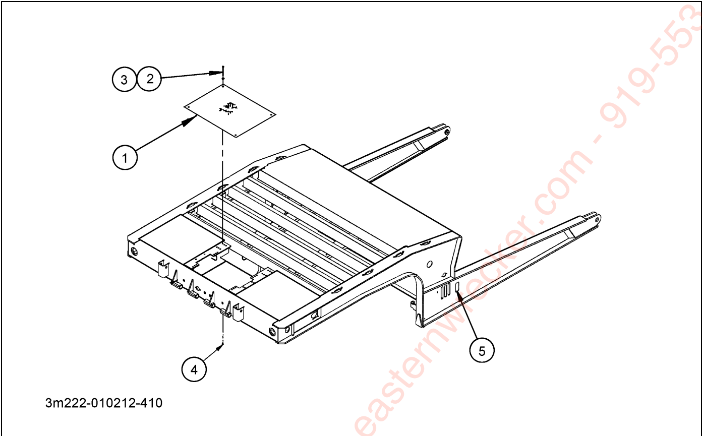
Figure 2-88: Upper Deck Cover Installation (Option)
