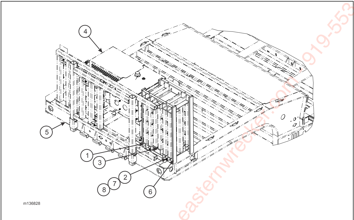
Figure 2-90: Upper Deck Extension Bridge Storage Rack (Option)
