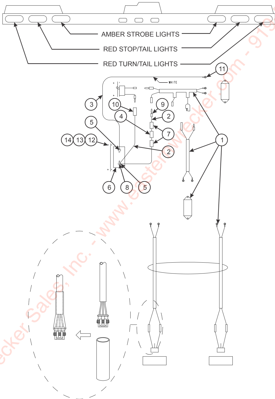
Figure 2-97: Battery Backup Strobe Light Installation (Option)
