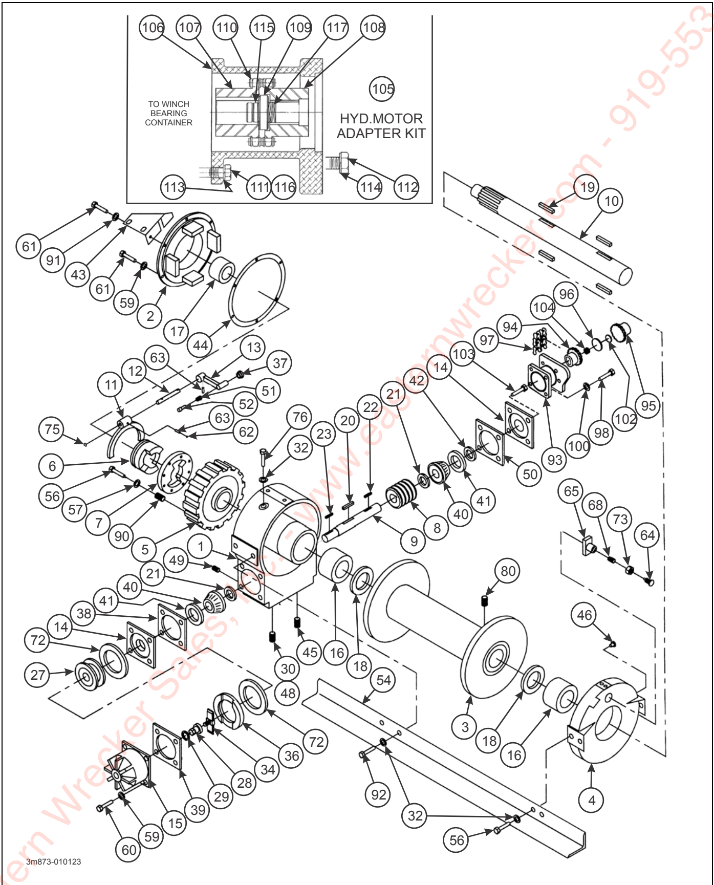
Figure 2-46: 20,000 Lb. Winch Items
