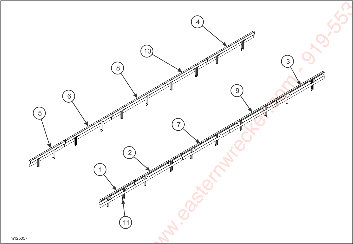
Figure 2-86: 8" Metal Sideboard Installation (Option) (425)
