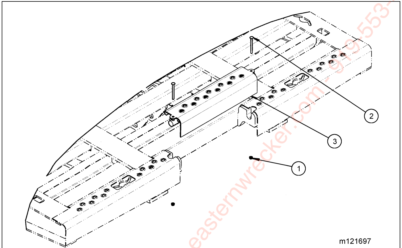
Figure 2-85: Center Rub Plate Cover Installation (Option)
