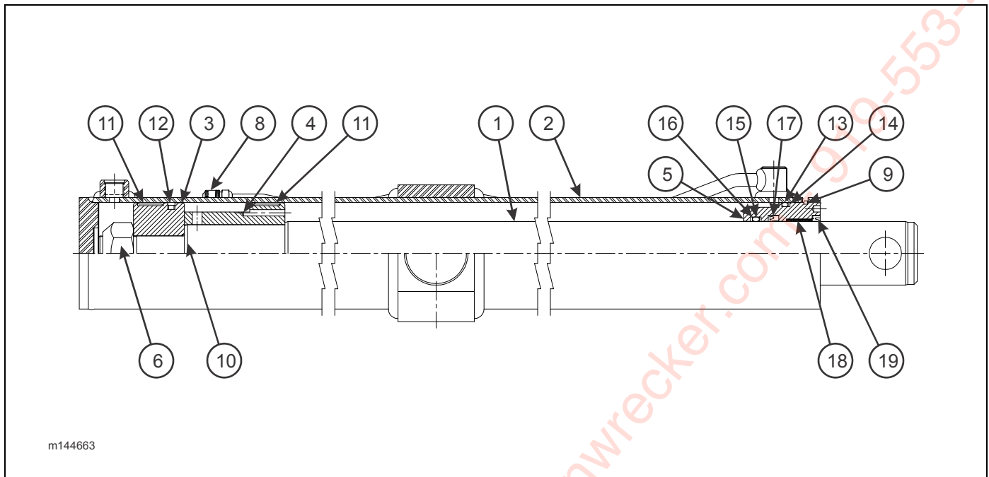
Figure 2-13: Cylinder, Hydraulic 4 x 100 (Curbside) (425-41, 435-41)
