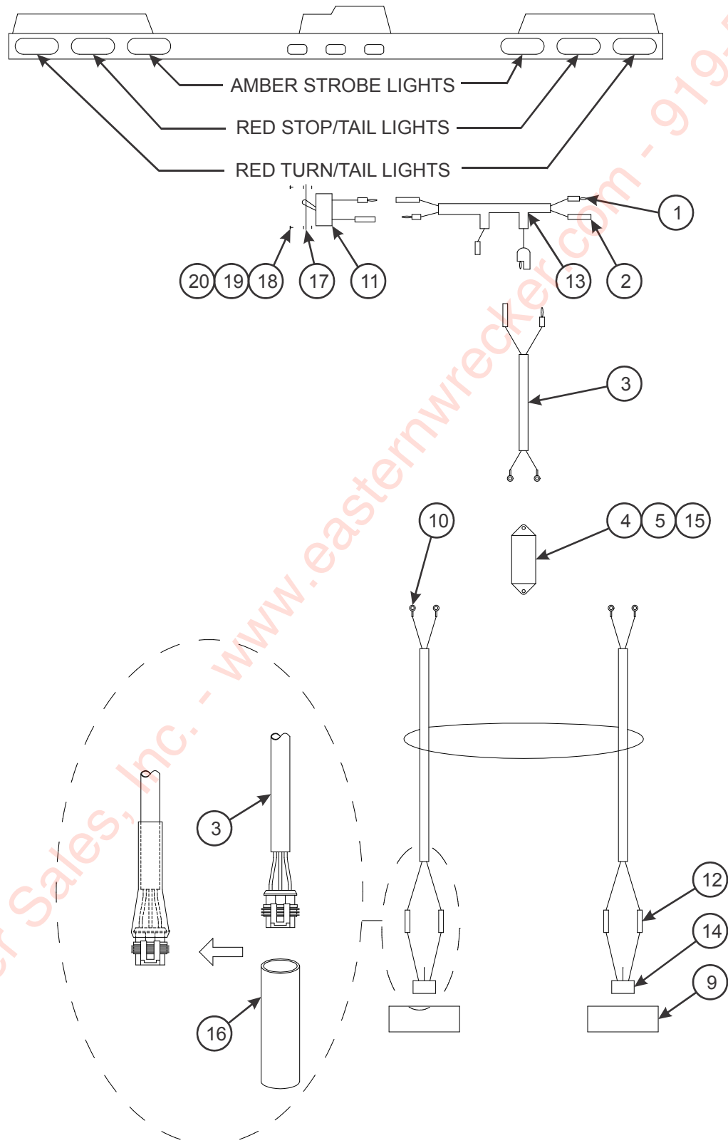
Figure 2-96: Rear Strobe Light Installation (Option)
