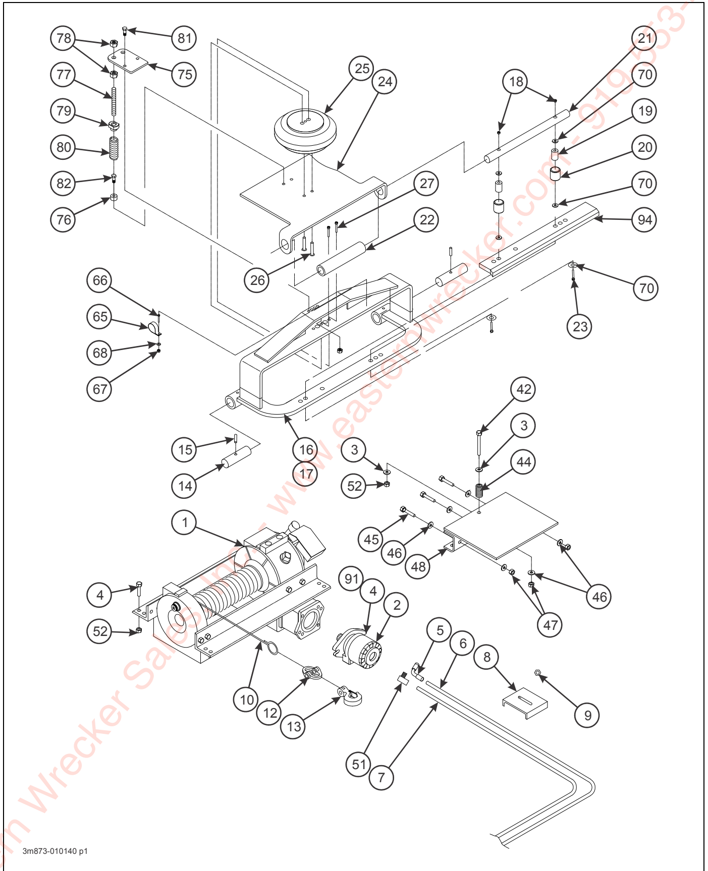
Figure 2-40: Winch Installation (1 of 2)
