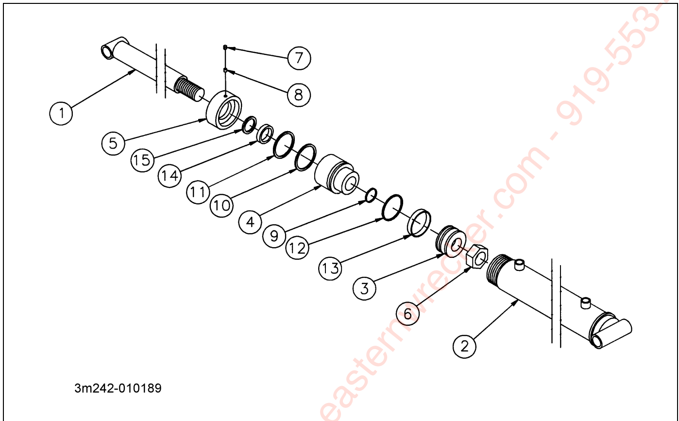
Figure 2-19: Cylinder, Hydraulic 6 X 41 (435 & 410)
