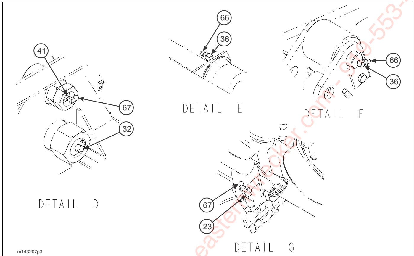
Figure 2-25: U/C Assembly, Air Ride Suspension (410) (4 of 4)
