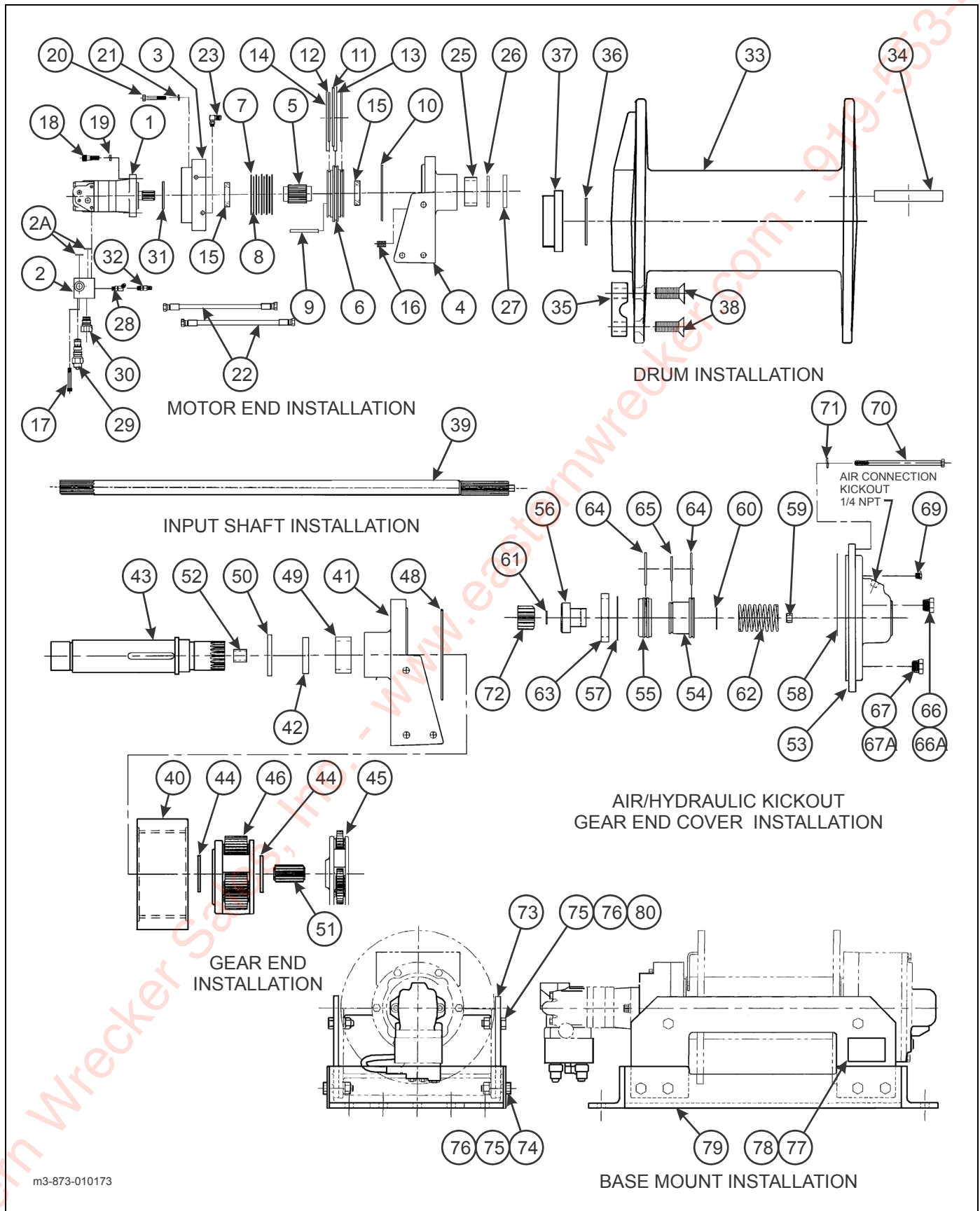
Figure 2-52: 30,000 Lb. Winch Items
