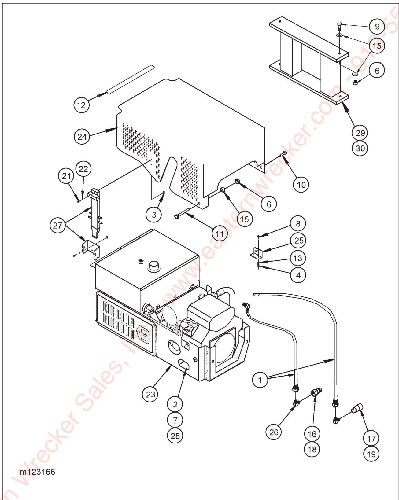
Figure 1-63 Upper Deck Engine Installation
