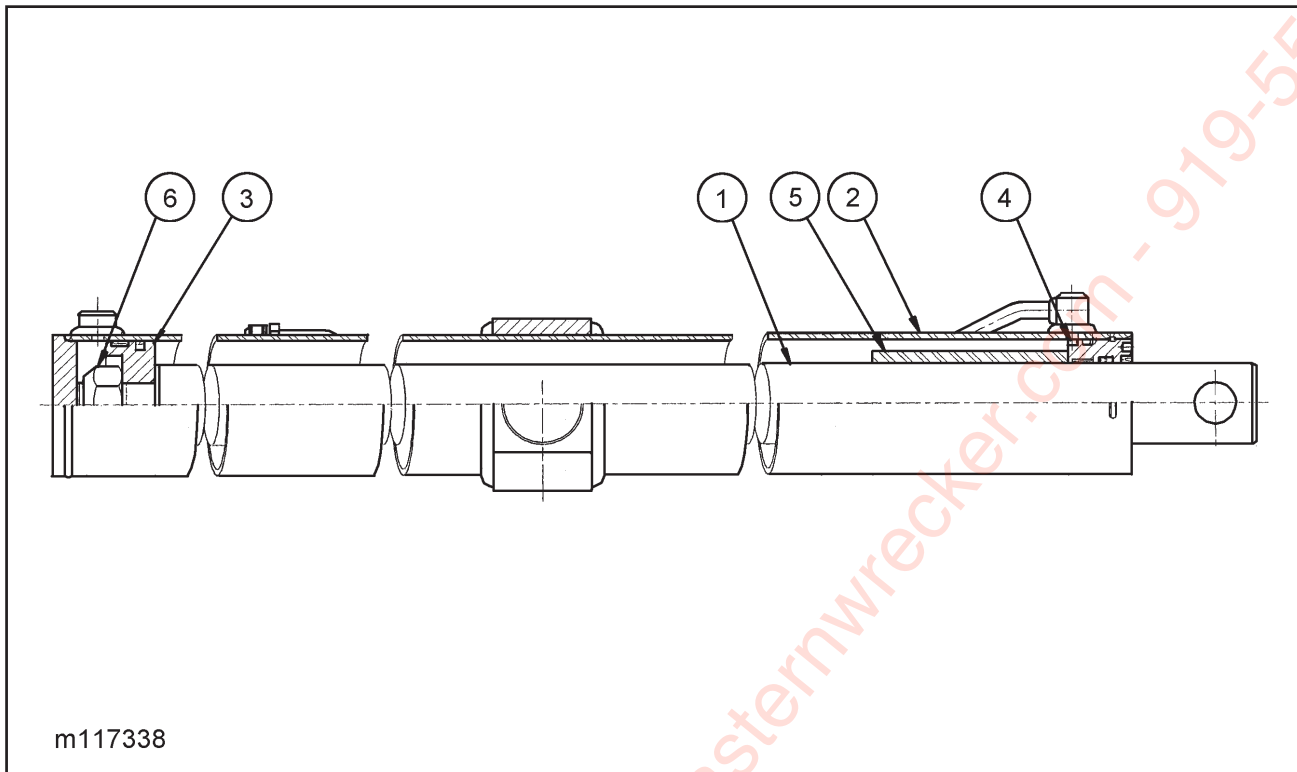
Figure 1-8 Cylinder, Hydraulic 4 x 100 (Curbside) (410-48 & 425)
