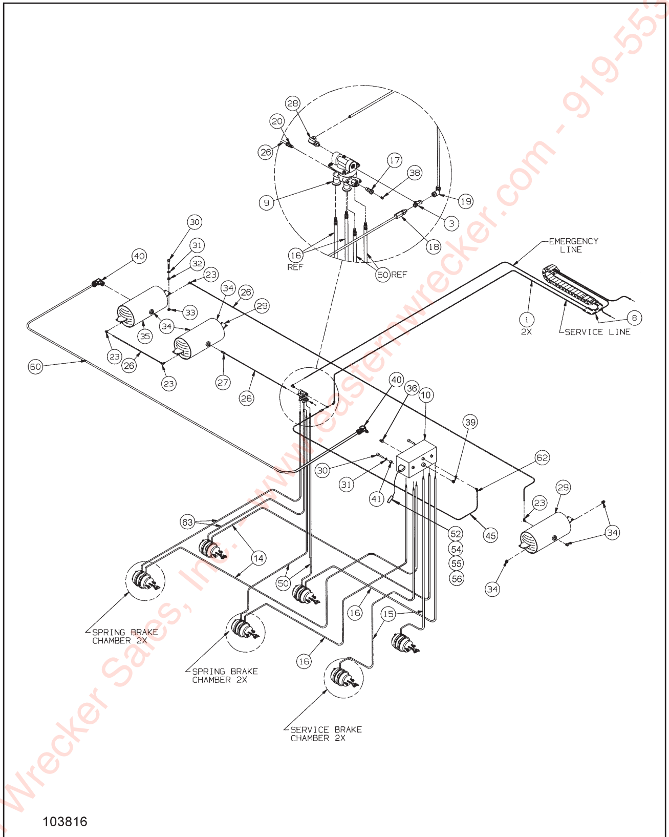
Figure 1-27 Spring Air Brake System w/ ABS (410)
