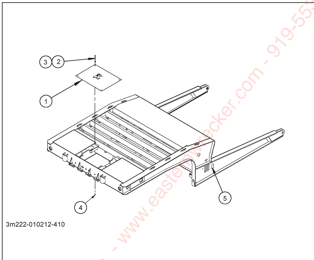
Figure 1-71 Upper Deck Cover Installation (Option)
