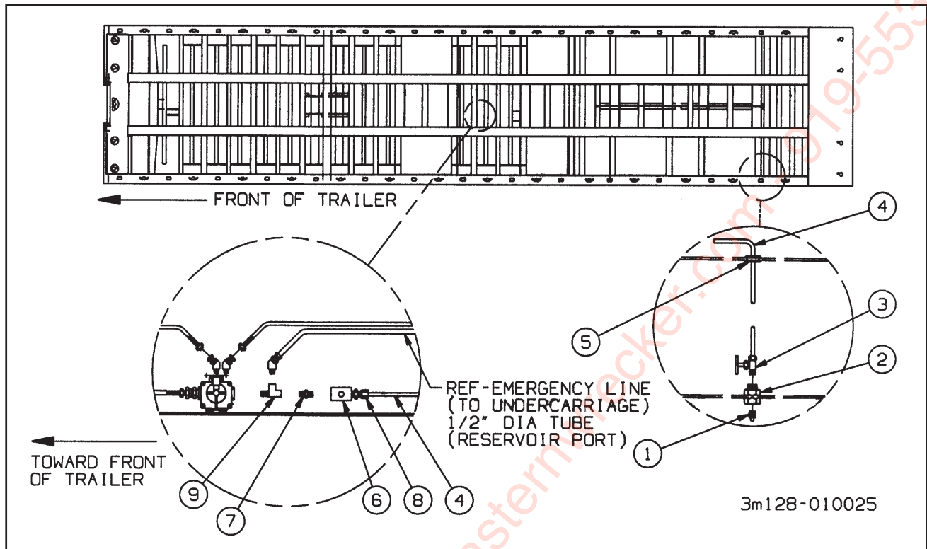
Figure 1-67 Air Outlet Accessory (Option)
