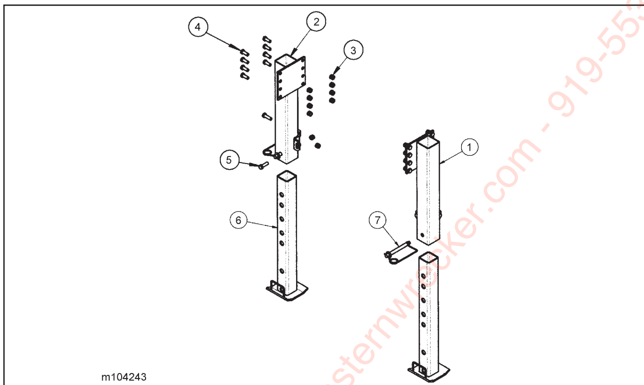
Figure 1-61 Landing Gear Installation - Bolt-on
