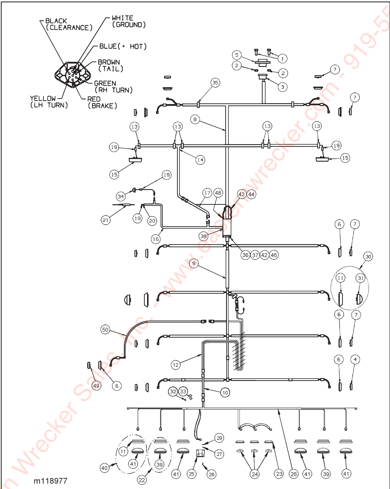
Figure 1-18 Electrical System Schematic
