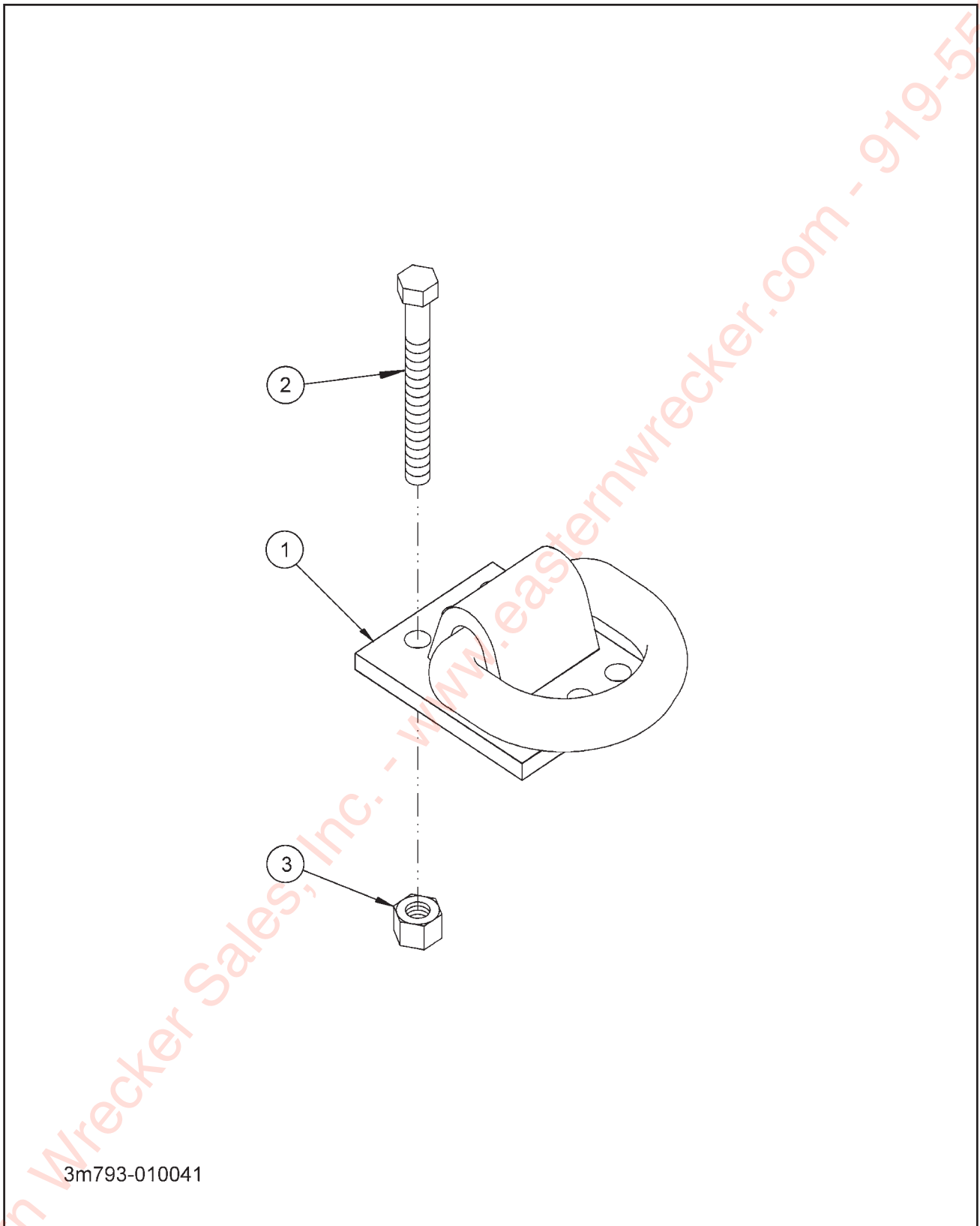
Figure 1-48 Tie Down Installation (Option)
