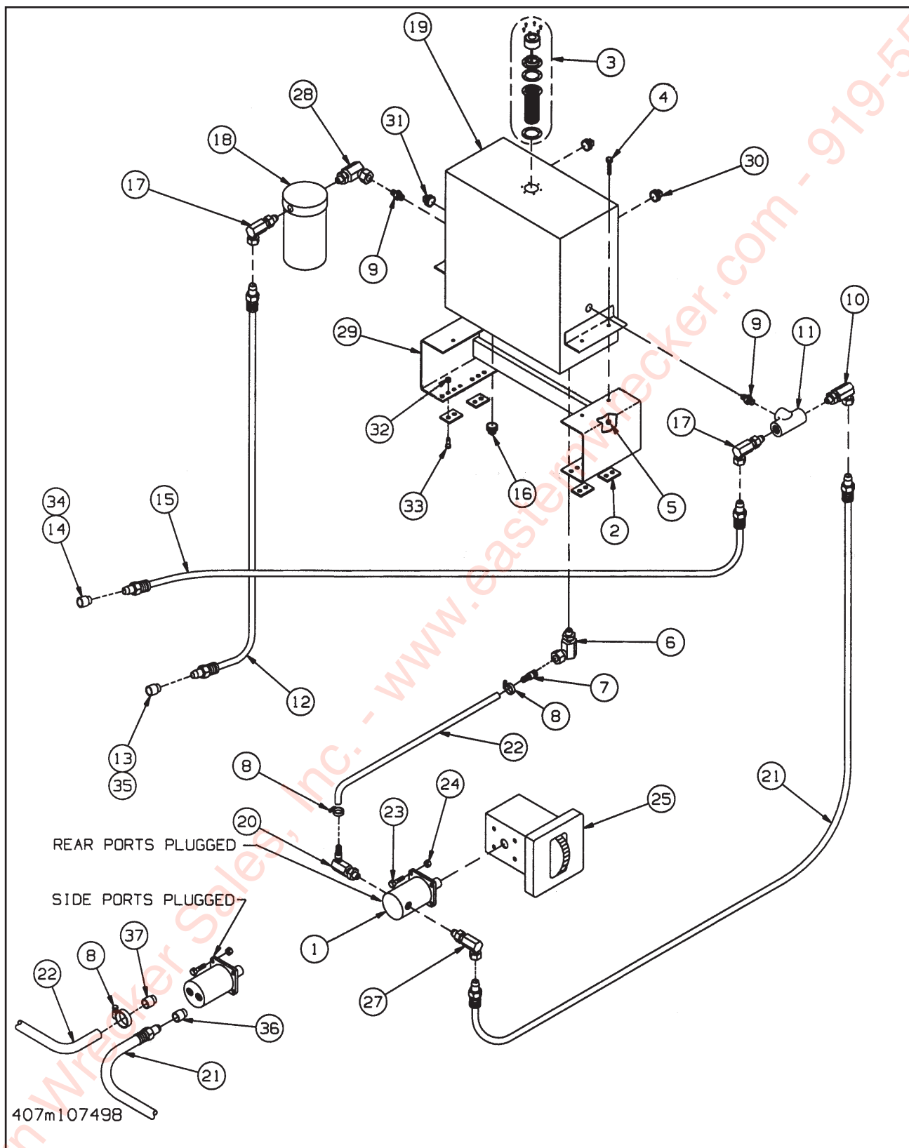
Figure 1-16 Transmission Mounted Wet Kit Items
