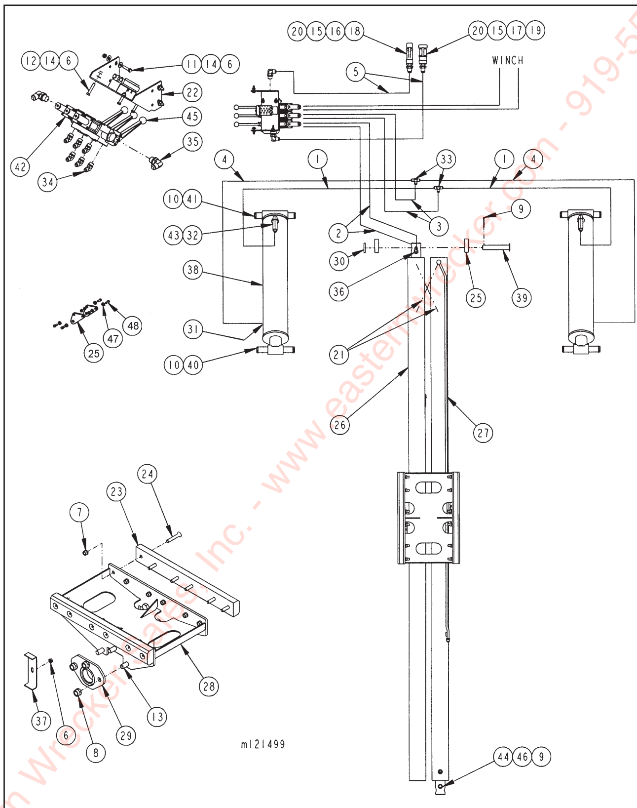
Figure 1-6 Hydraulic System
