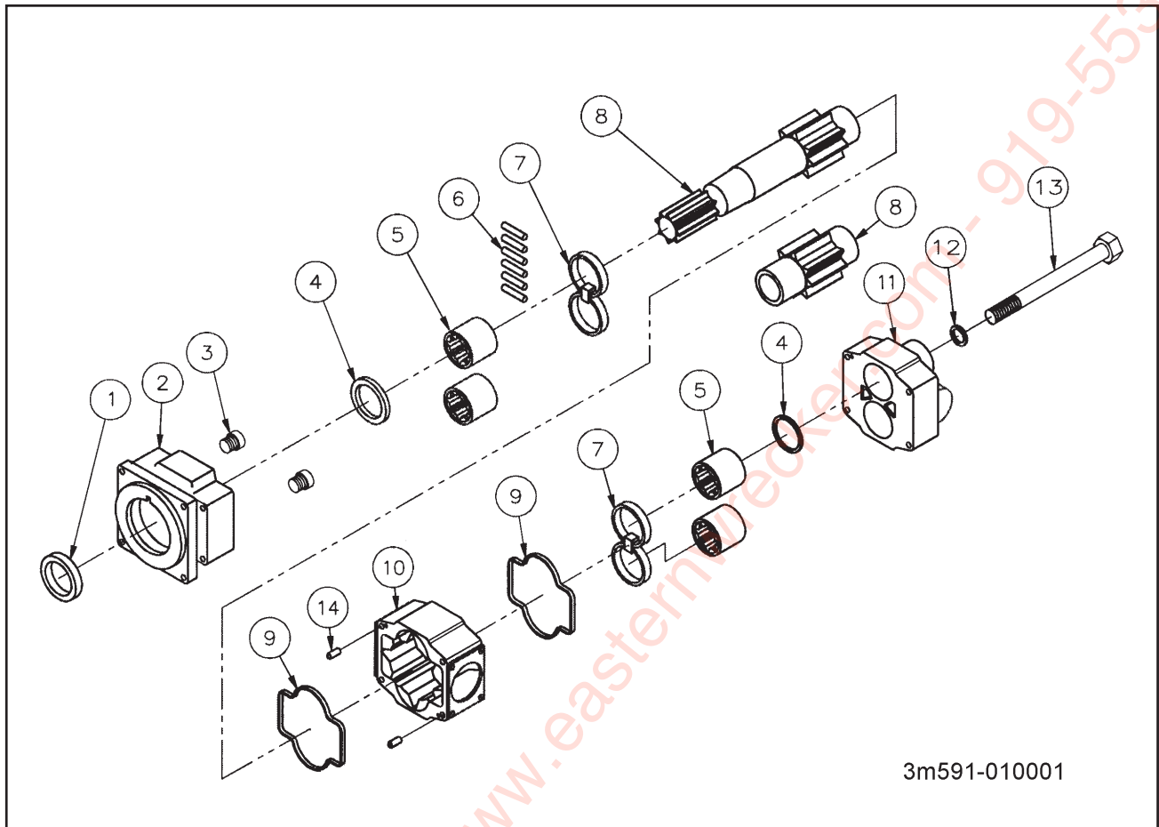
Figure 1-15 Pump, Wet Kit Hydraulic
