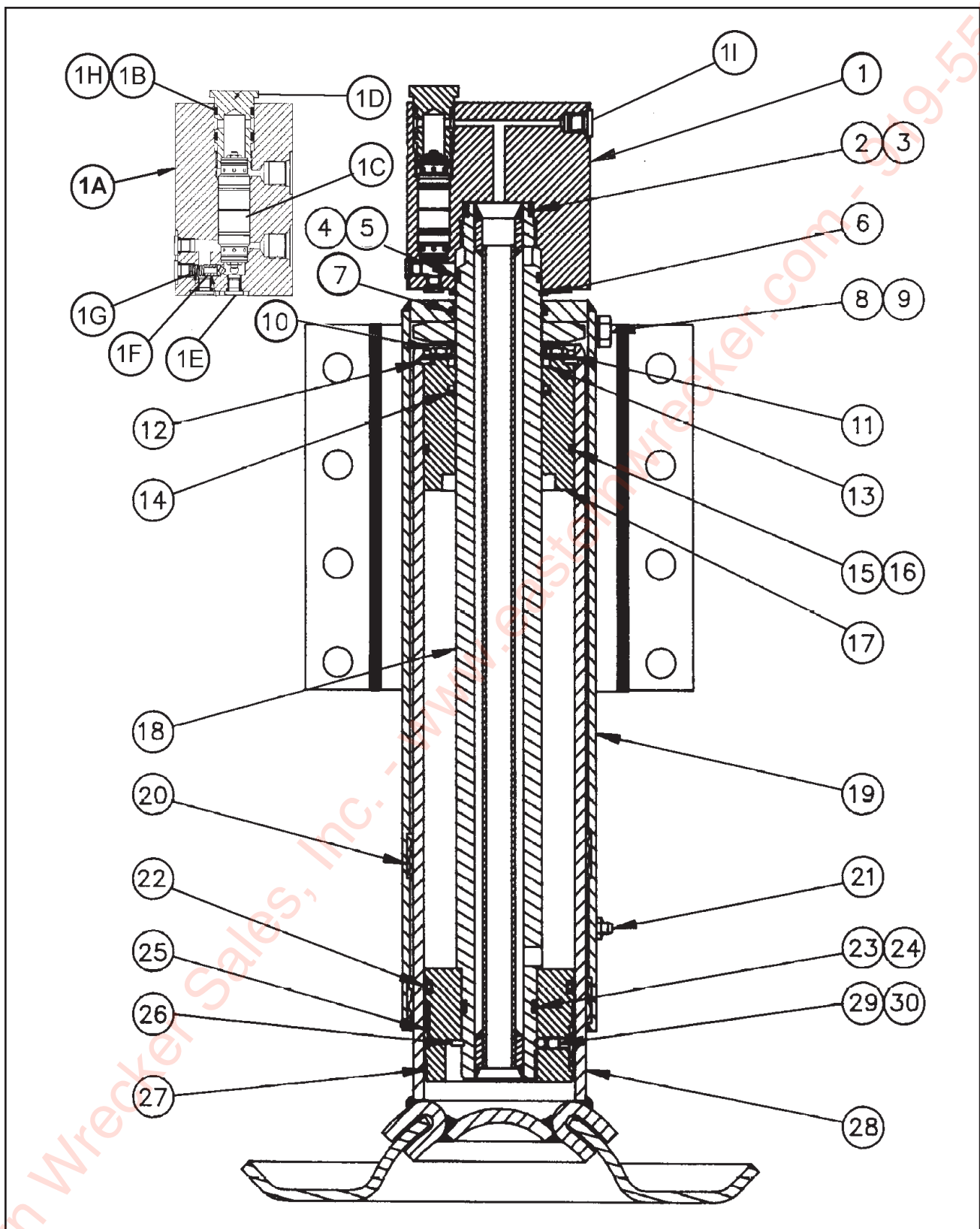
Figure 1-56 Dock Leveler Leg Assembly w/ Lock Valve
