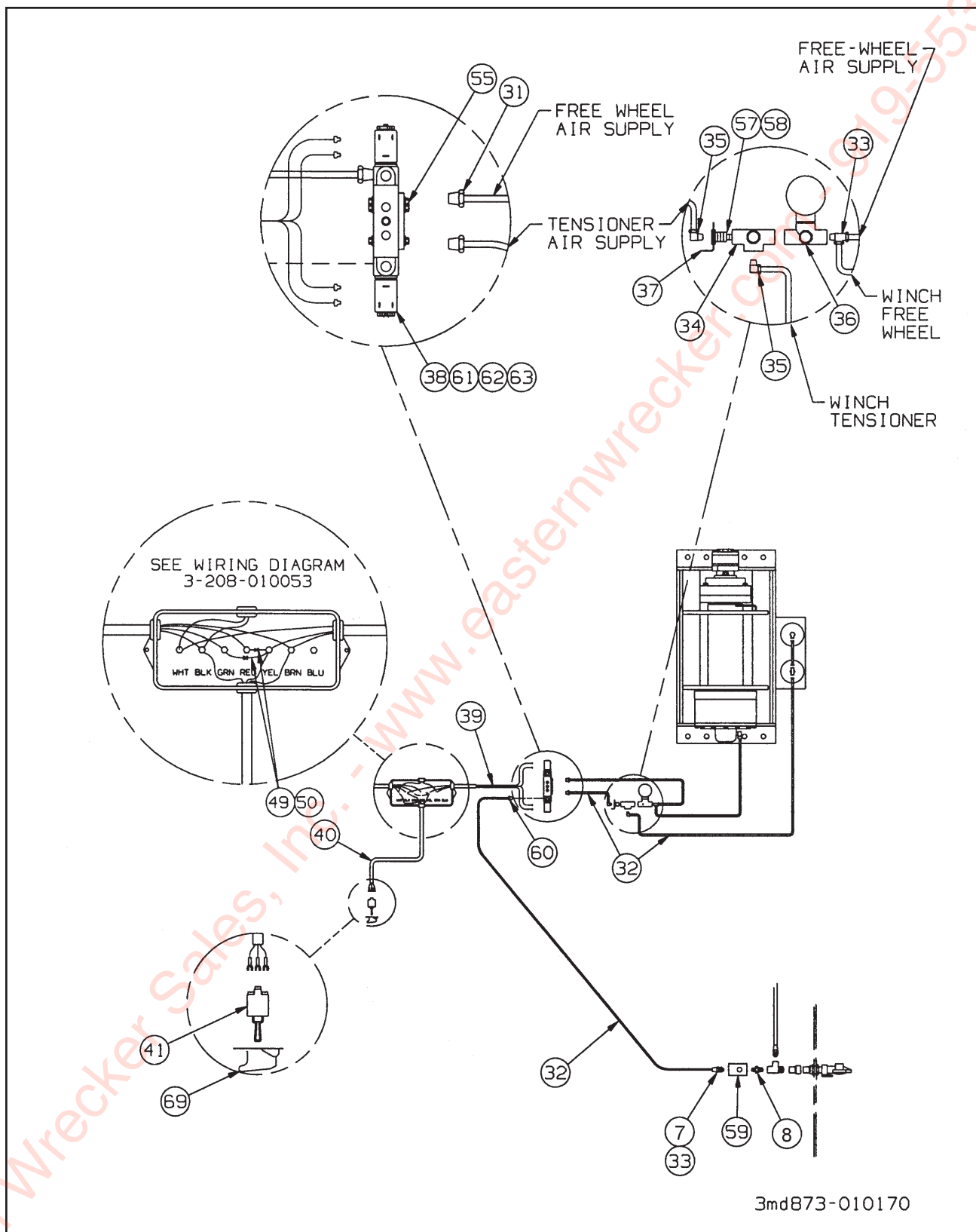
Figure 1-39 30K Upper Deck Winch Installation (2 of 2)
