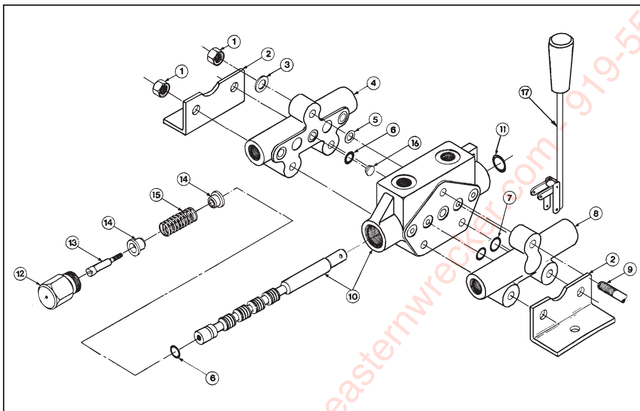
Figure 1-57 Dock Leveler Valve
