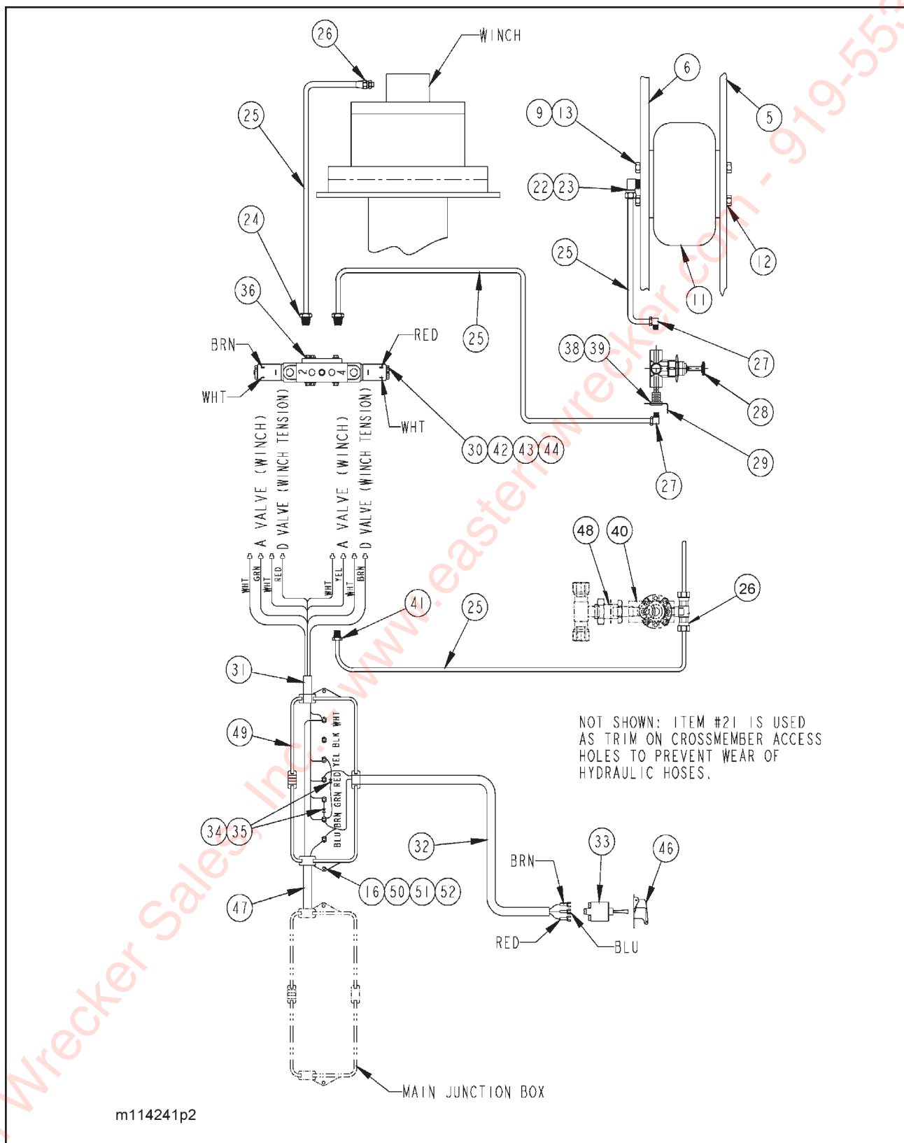
Figure 1-46 12K, 15K, & 20K Upper Deck Winch (DP) (2 of 2)
