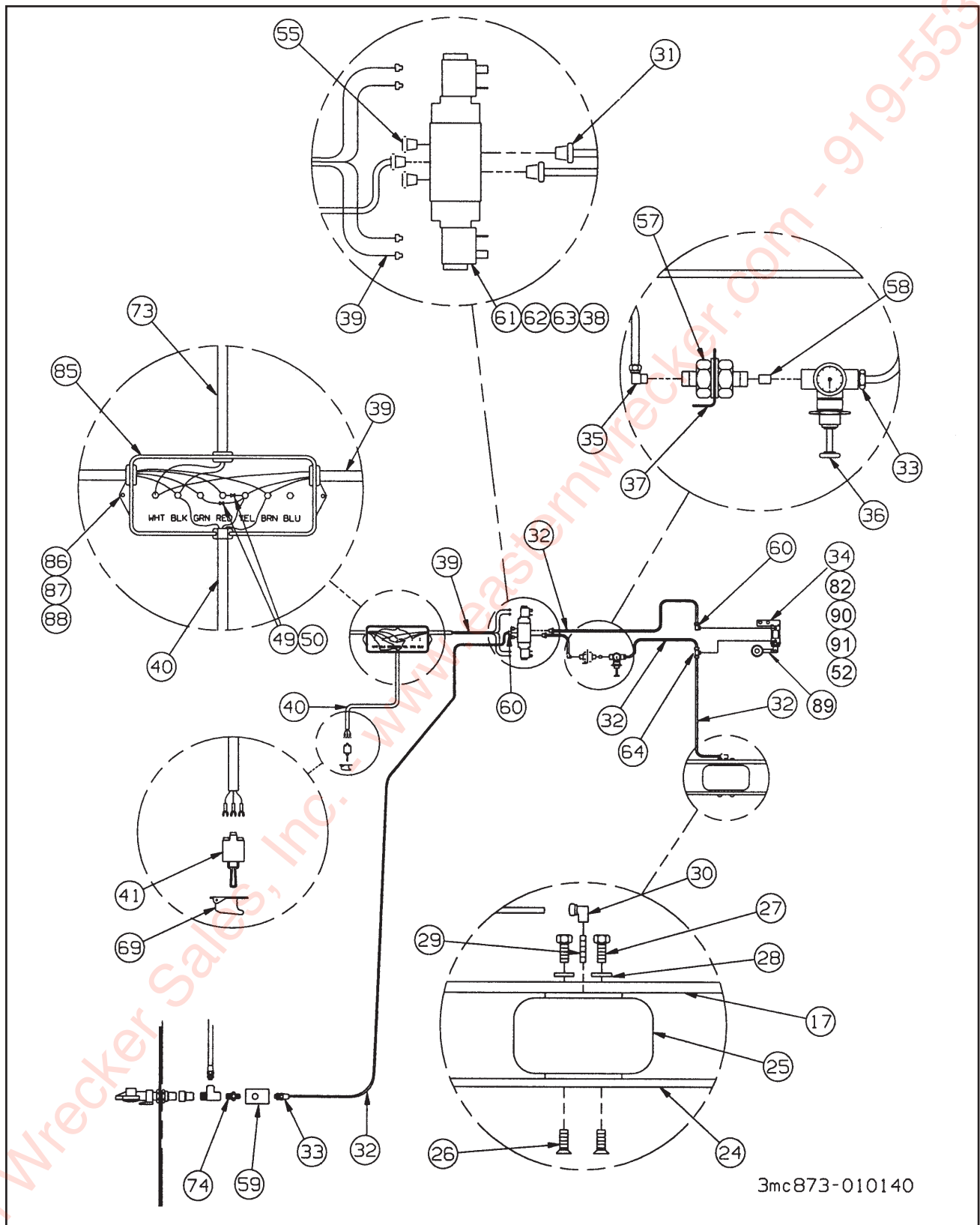
Figure 1-32 Winch Installation (2 of 2)
