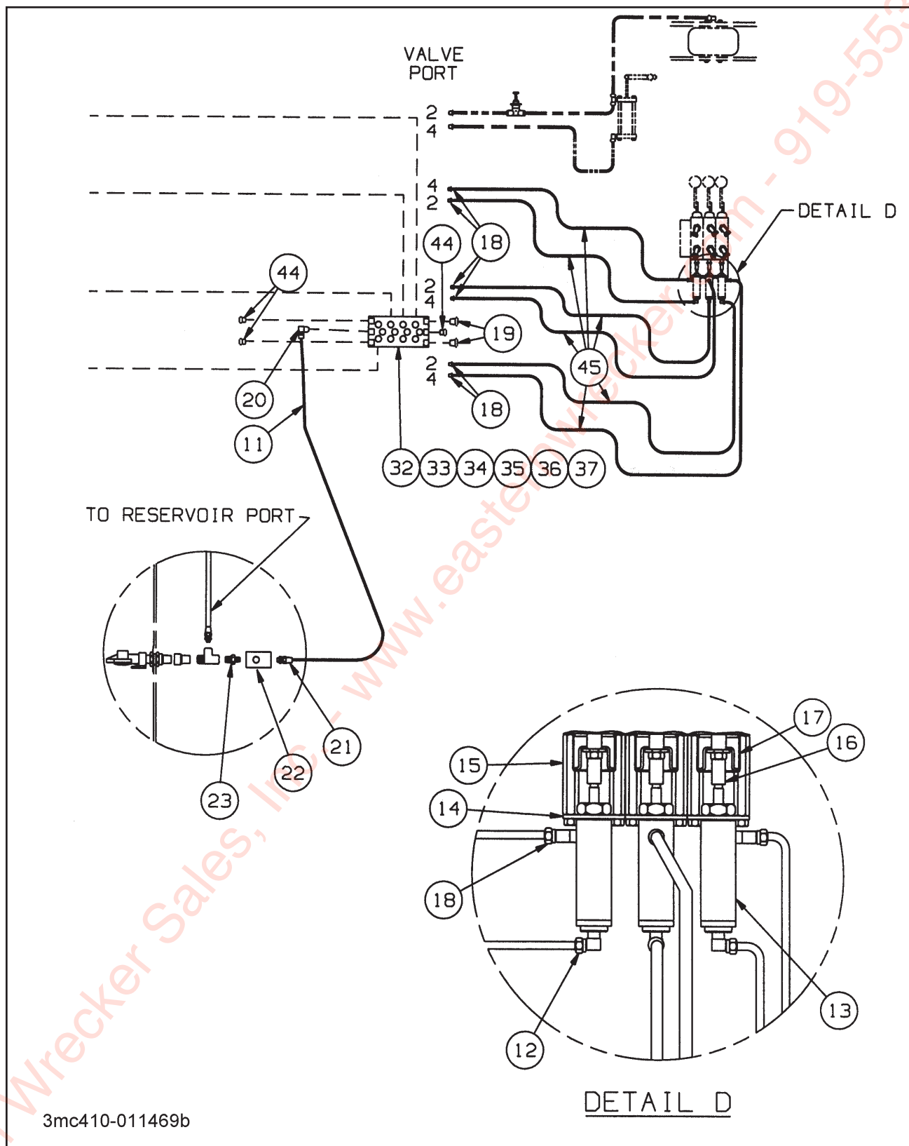
Figure 1-50 Remote Control Items (2 of 2)
