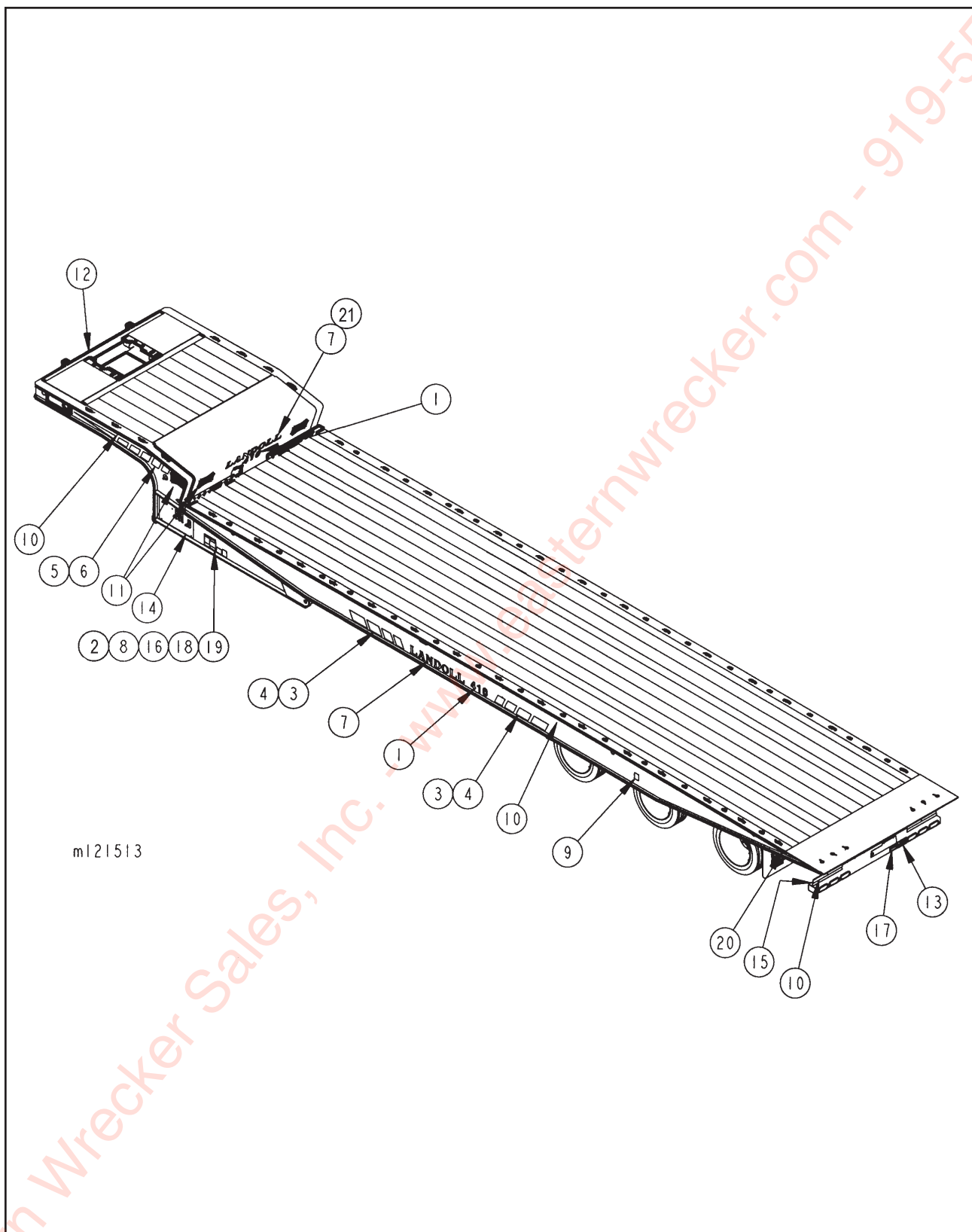
Figure 1-59 Decal Placement
