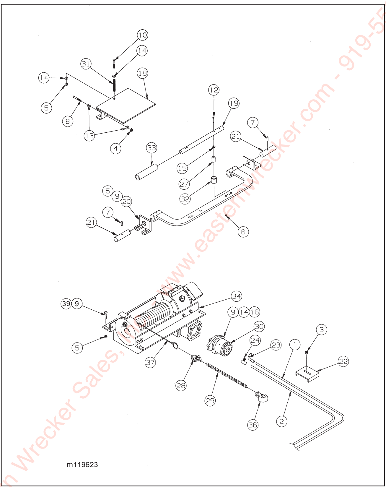
Figure 1-33 Winch Installation, Spring Tension Cable Roller
