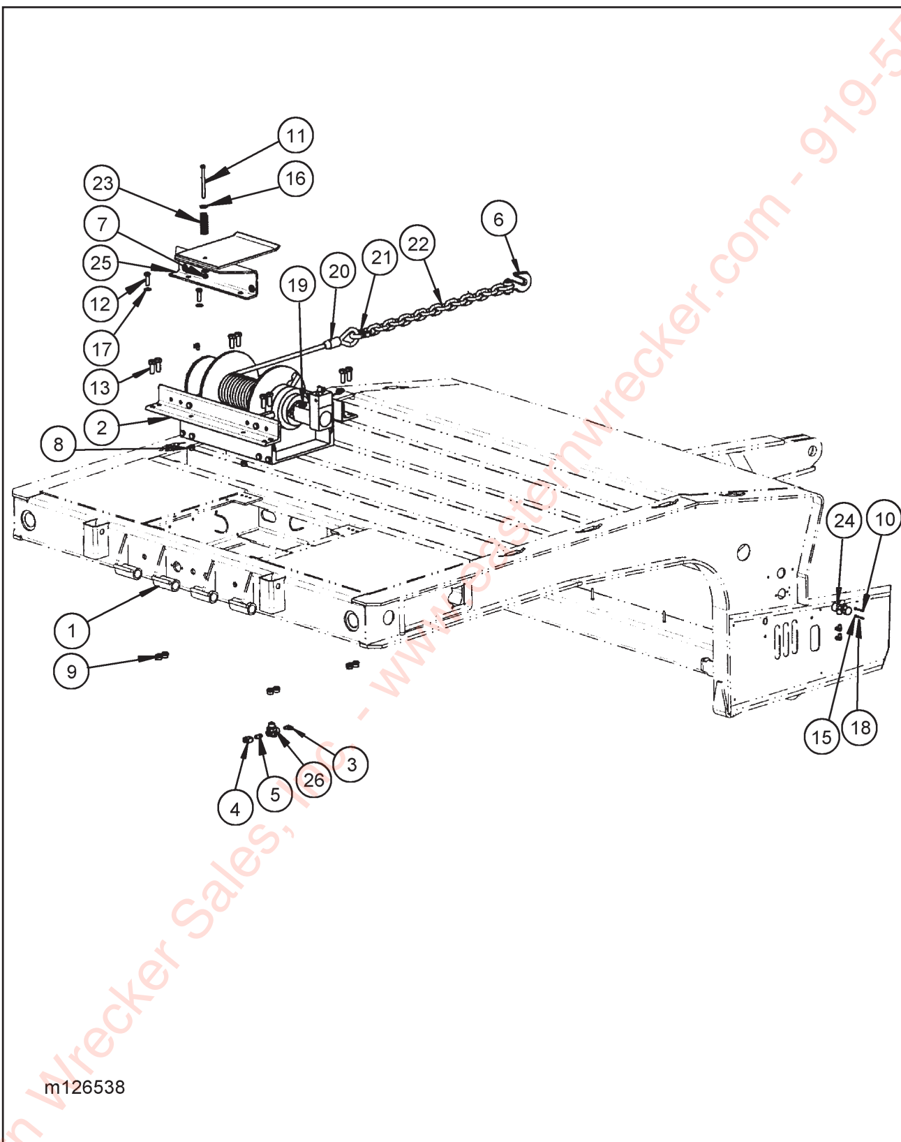
Figure 1-41 30K Upper Deck Winch Installation (1 of 2)
