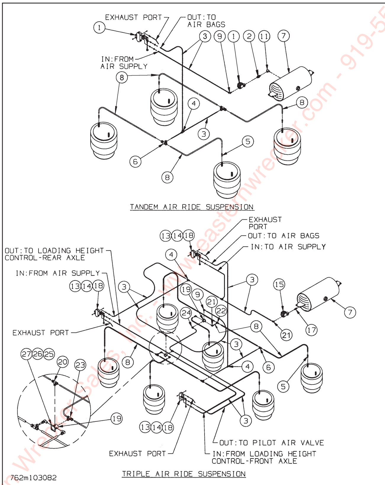
Figure 1-22 Air Ride Suspension, Air System
