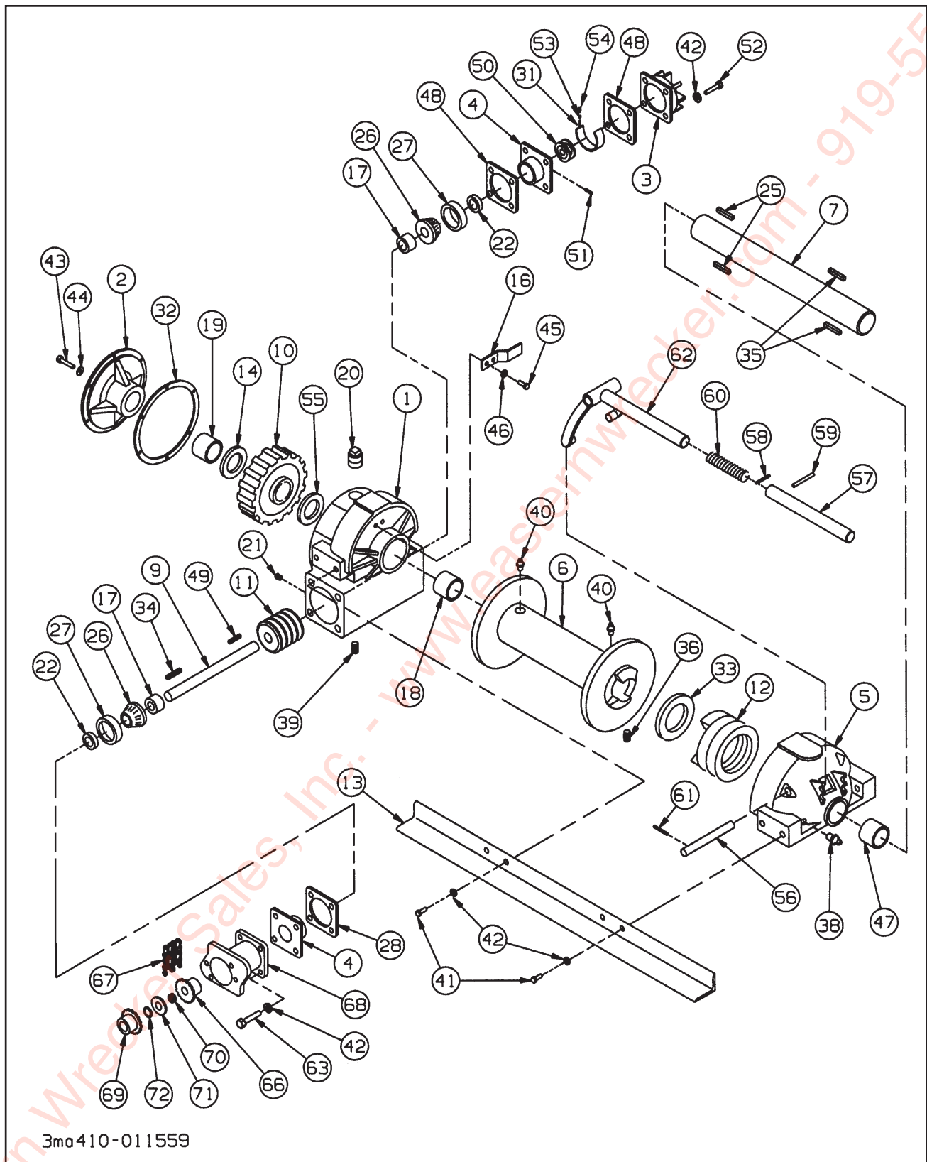
Figure 1-34 12,000# Winch Items
