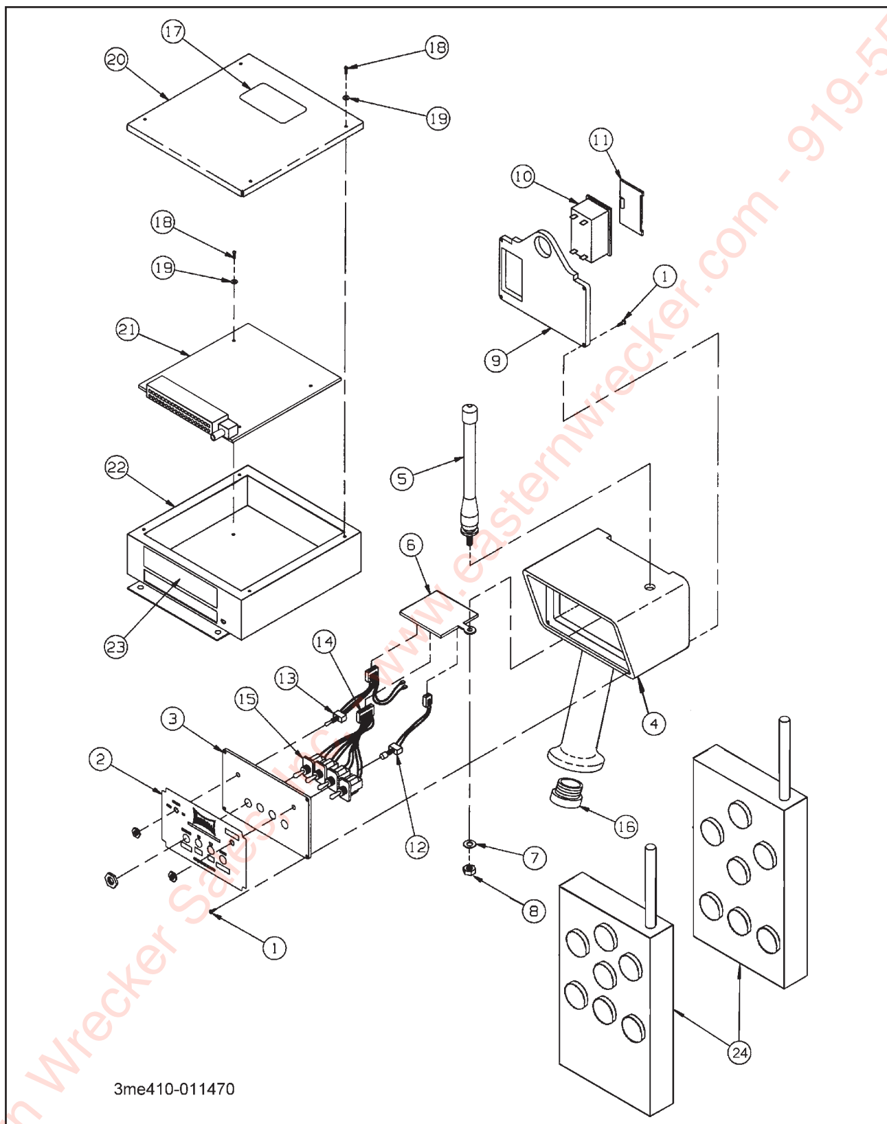
Figure 1-53 Wireless Remote Control
