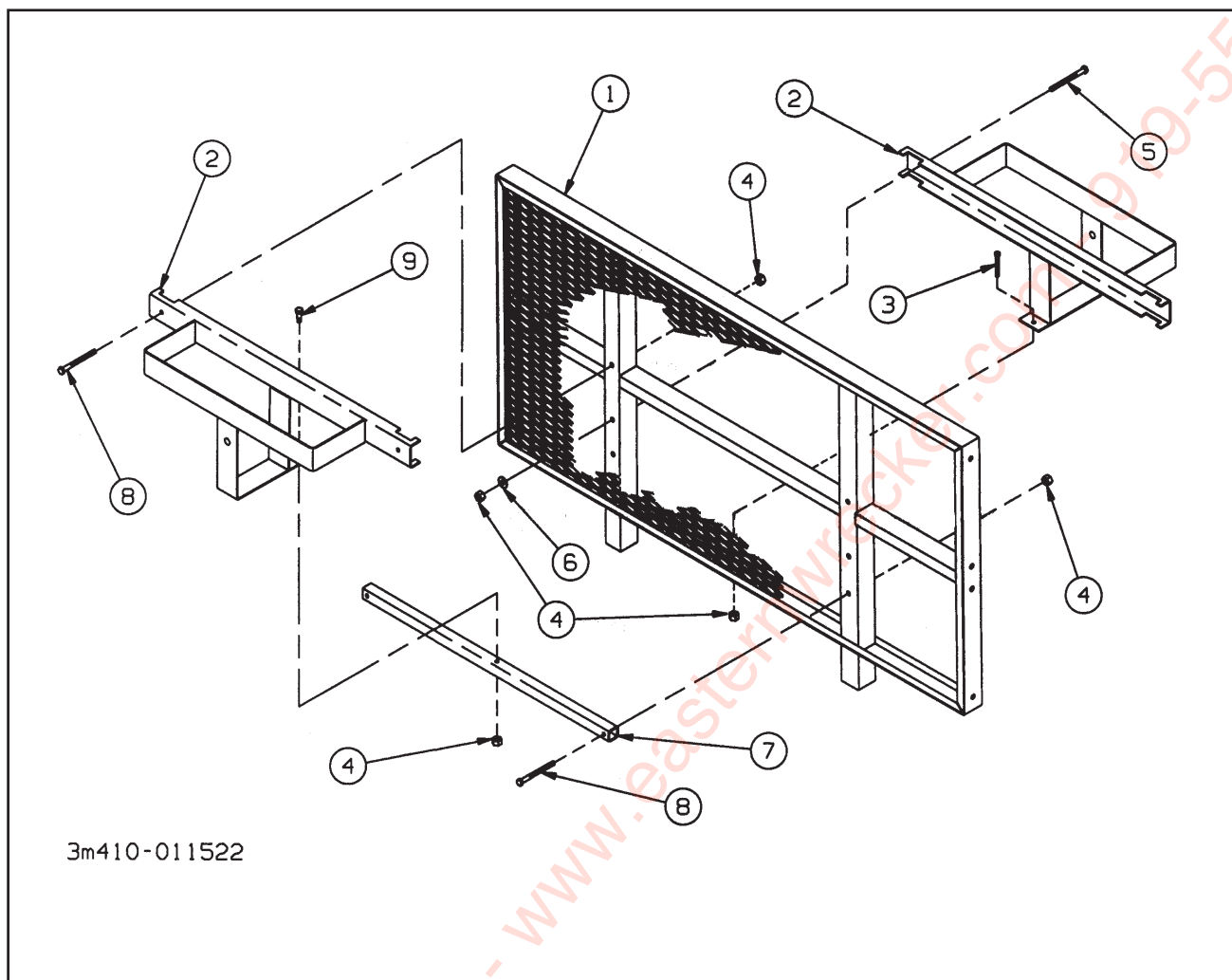
Figure 1-66 Spare Tire Carrier (Option)
