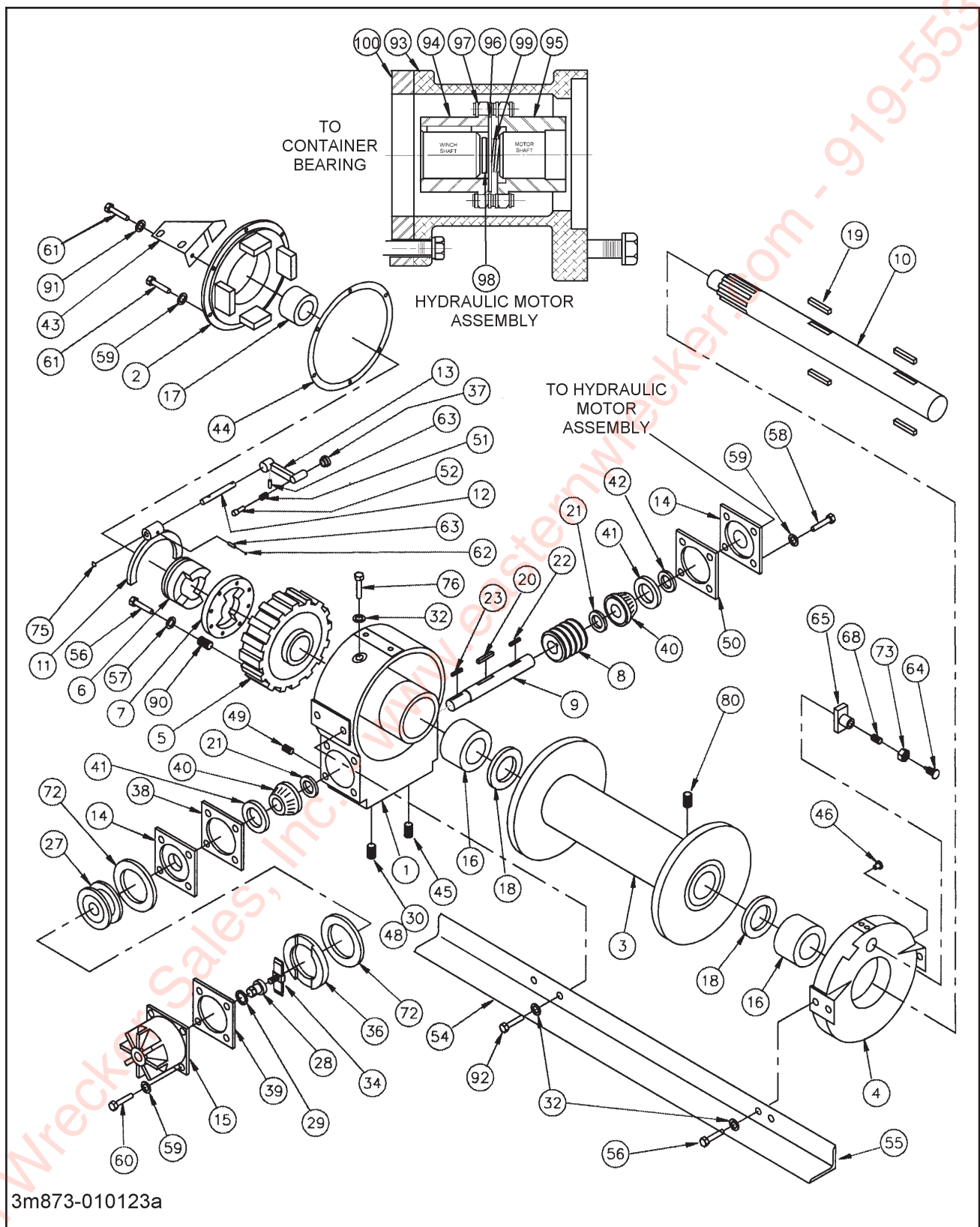
Figure 1-35 20,000# Winch Items
