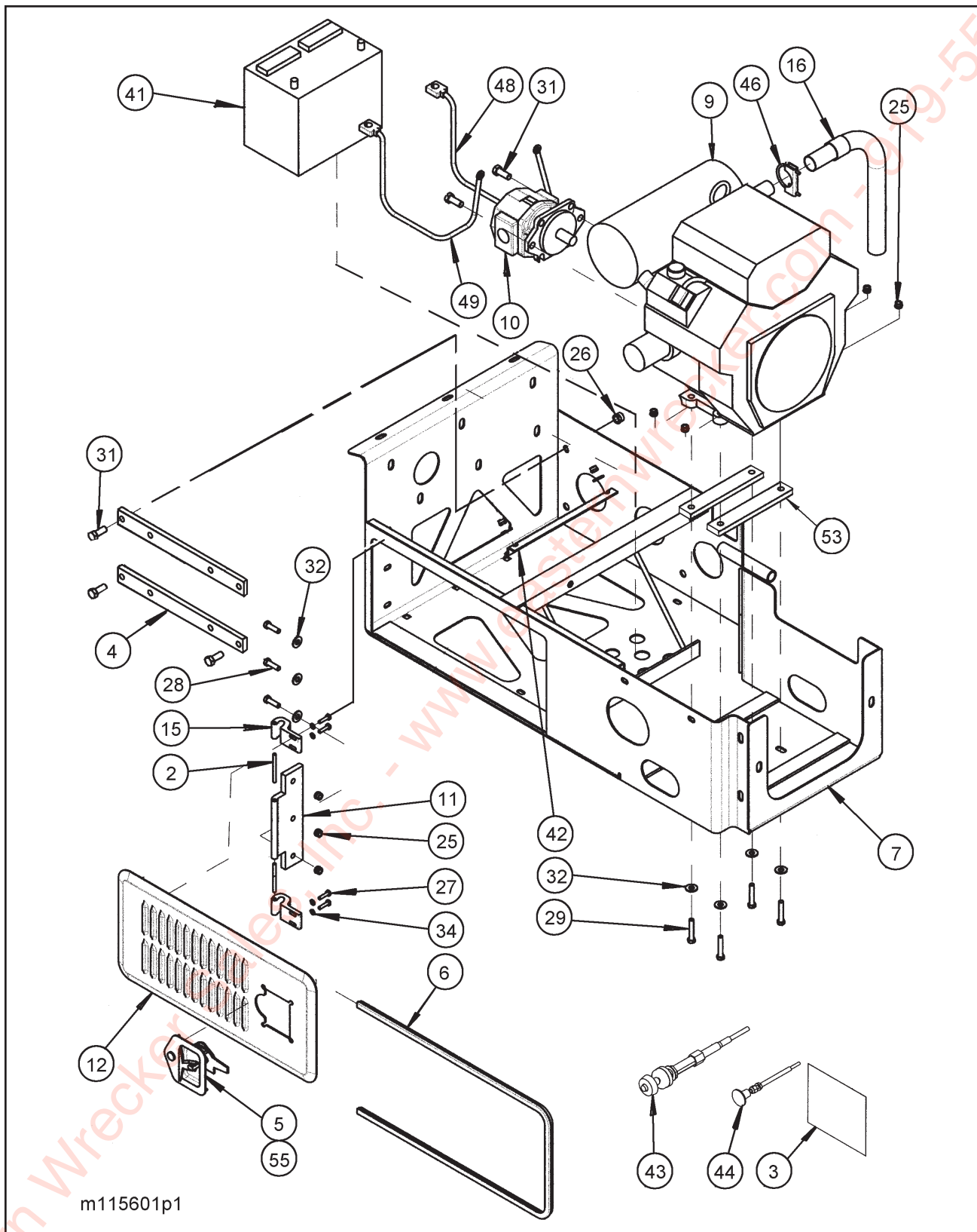
Figure 1-64 Hydraulic Engine, Standard Mount (1 of 2)
