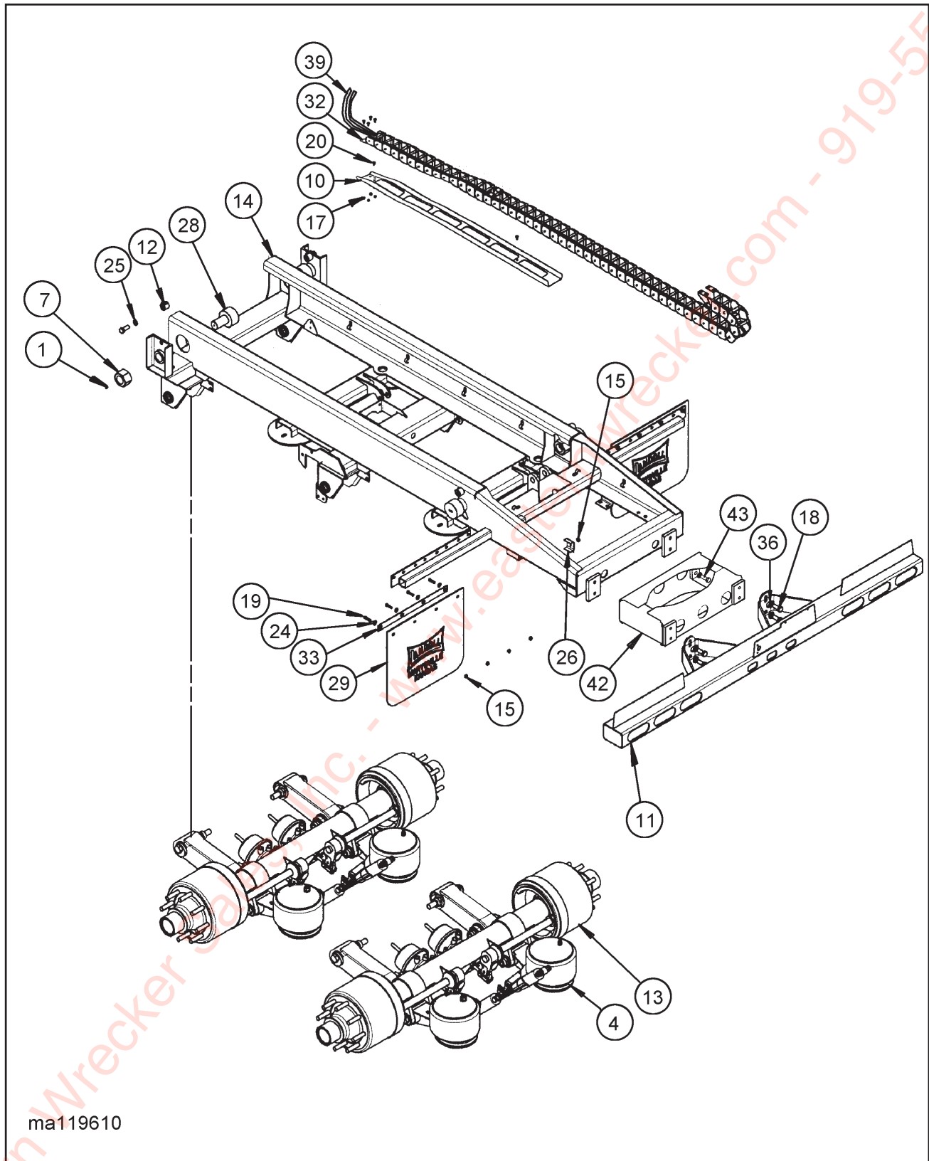
Figure 1-21 U/C Assembly, Air Ride Suspension (425 & 435)
