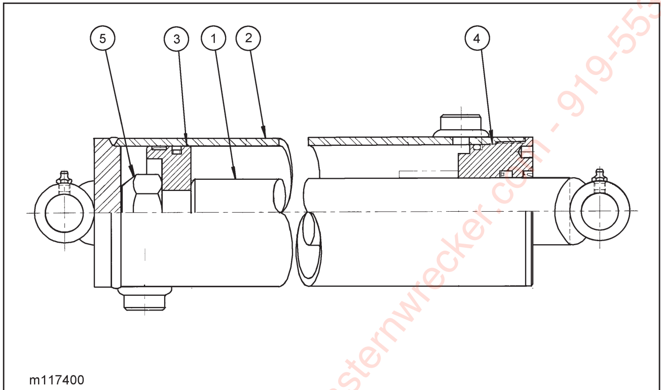
Figure 1-13 Cylinder, Hydraulic 4-1/2 x 30 (425)
