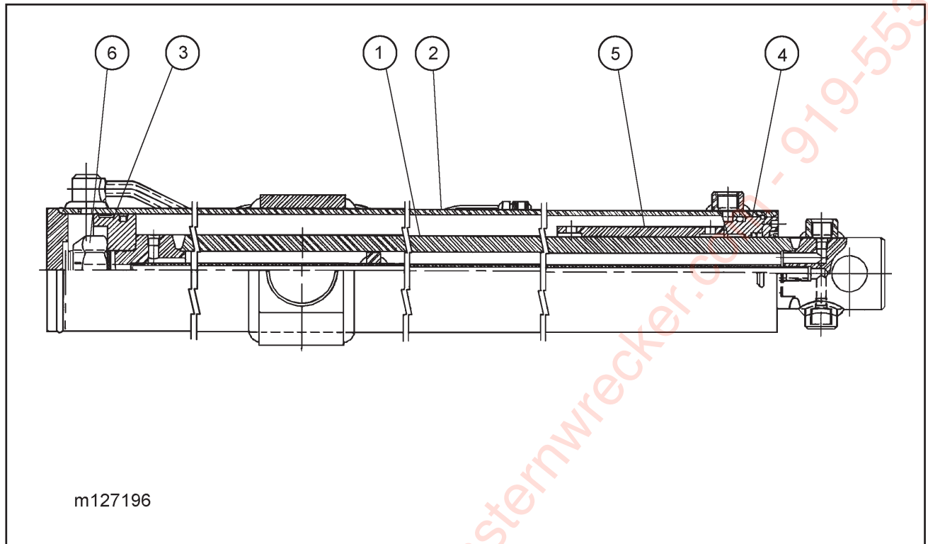
Figure 1-11 Cylinder, Hydraulic 4 x 138 Ported Rod (Streetside) (435-53)
