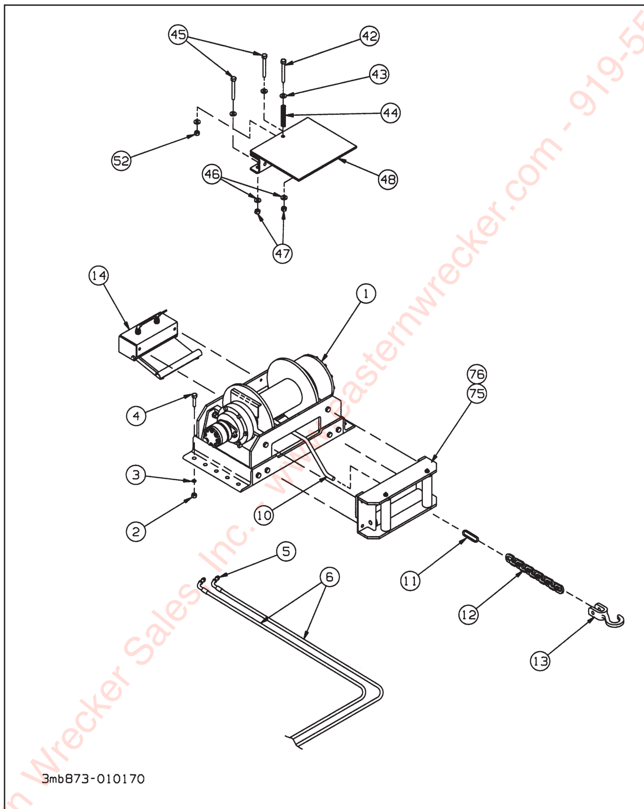
Figure 1-38 30K Upper Deck Winch Installation (1 of 2)
