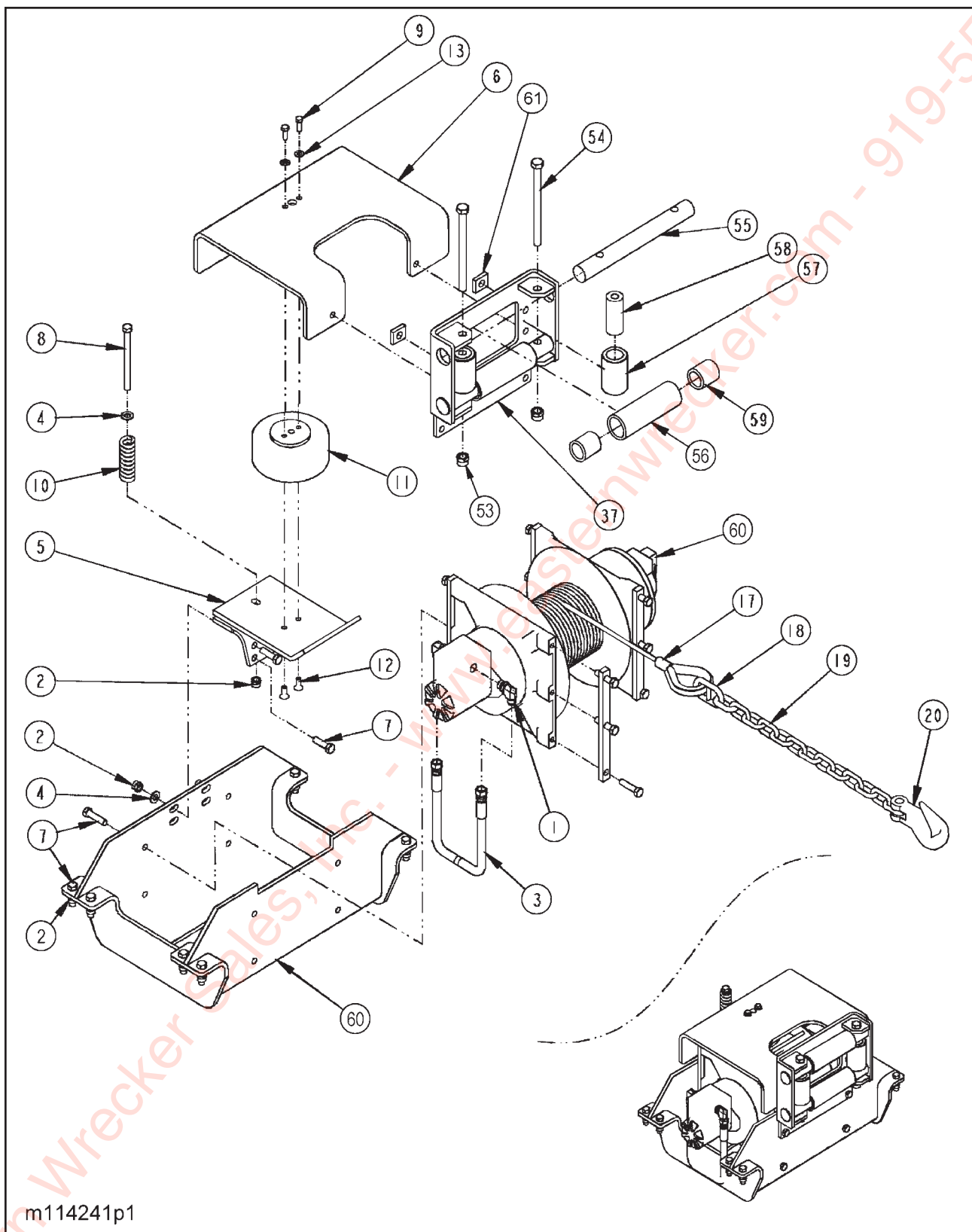
Figure 1-45 12K, 15K, & 20K Upper Deck Winch (DP) (1 of 2)
