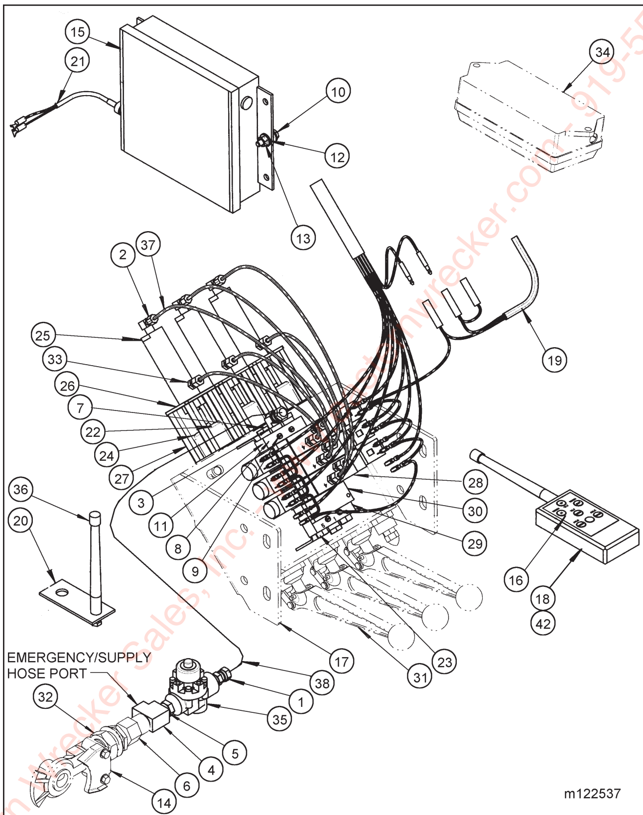
Figure 1-51 Radio Remote Control Assembly Winch/Tilt/Axle
