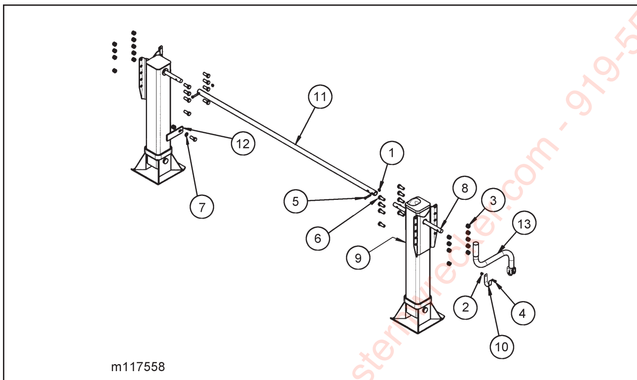
Figure 1-60 Landing Gear Installation
