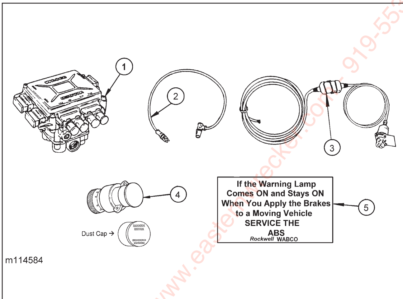
Figure 1-28 Brake Kit, Rockwell ABS
