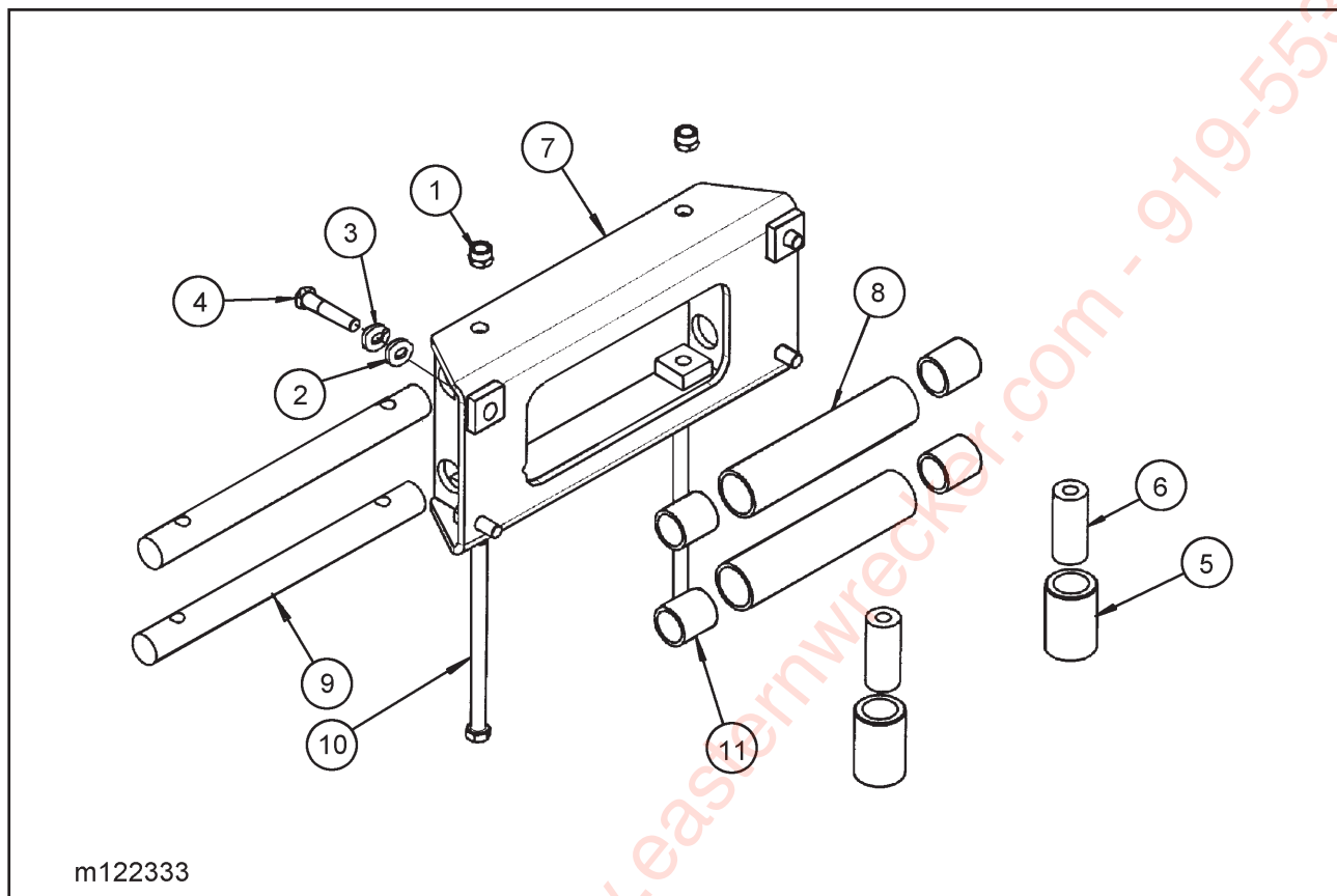
Figure 1-43 Winch Roller Guide - 30K
