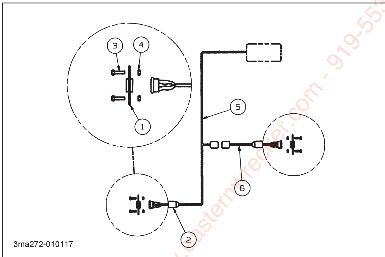
Figure 1-19 Electrical Installation - Rear Remote
