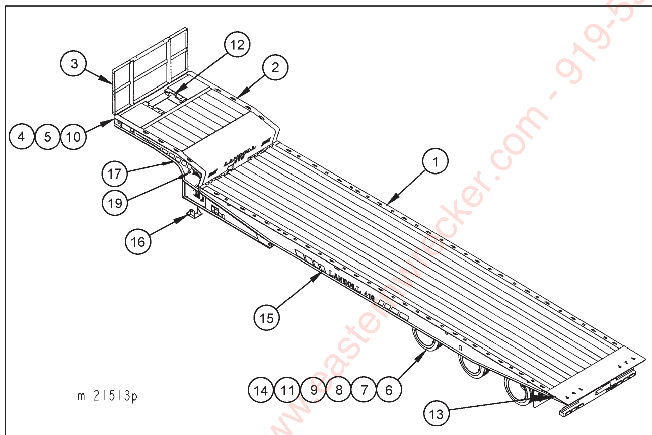
Figure 1-1 General Assembly
