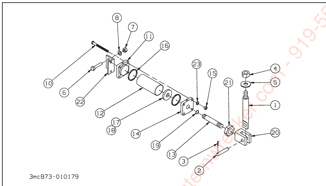
Figure 1-36 Winch Air Shift Cylinder for 20,000# Winch
