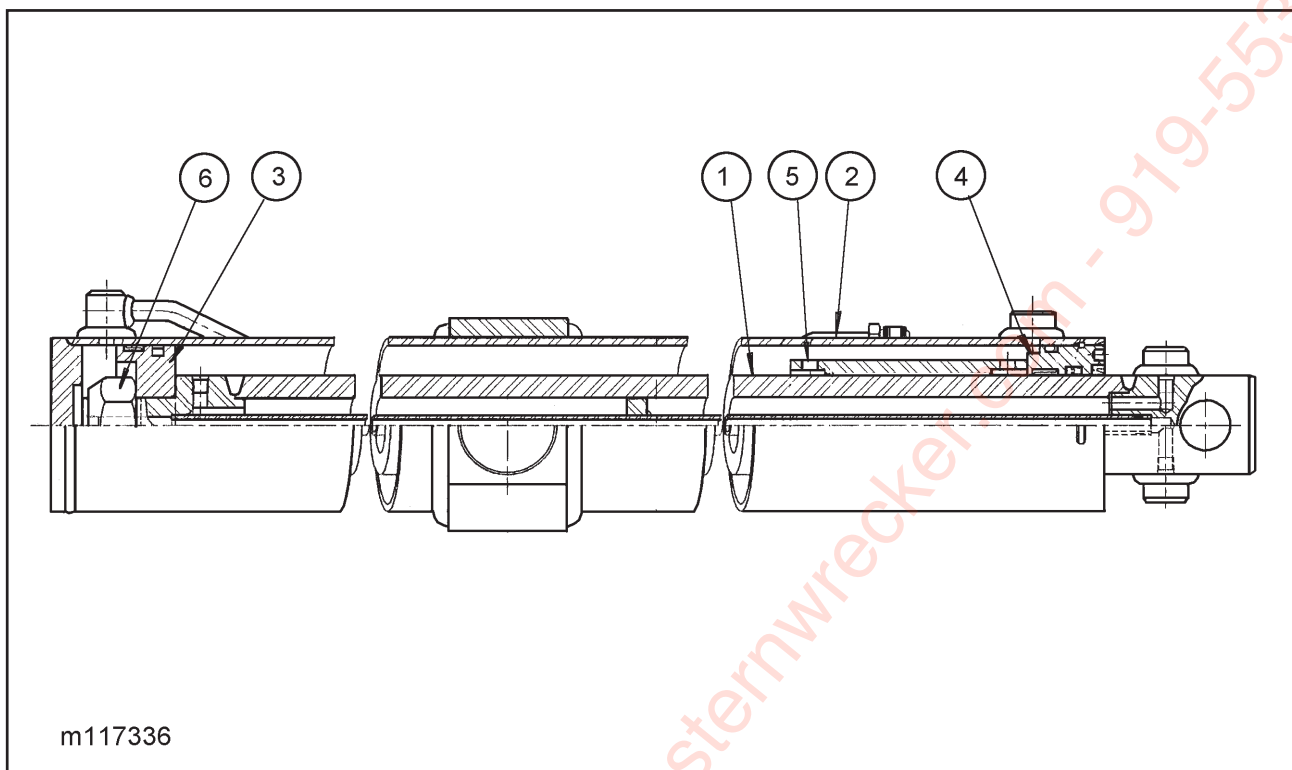
Figure 1-7 Cylinder, Hydraulic 4 x 100 (Streetside) (410-48, 410-50CA, & 425-41)
