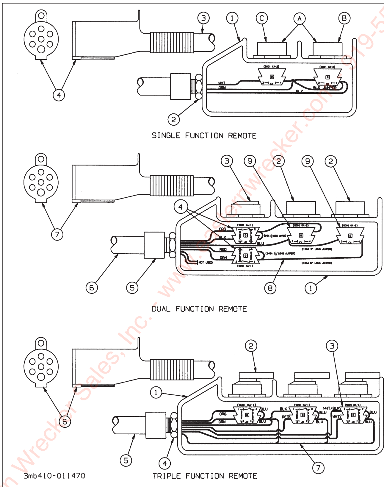
Figure 1-52 Wired Remote Control
