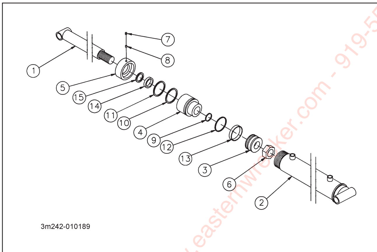
Figure 1-14 Cylinder 6" X 41" (410 & 435)
