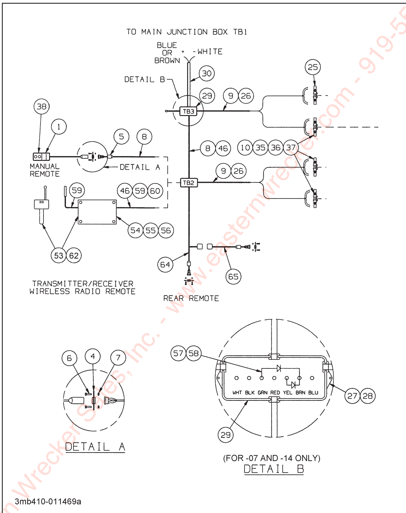
Figure 1-49 Remote Control Items (1 of 2)
