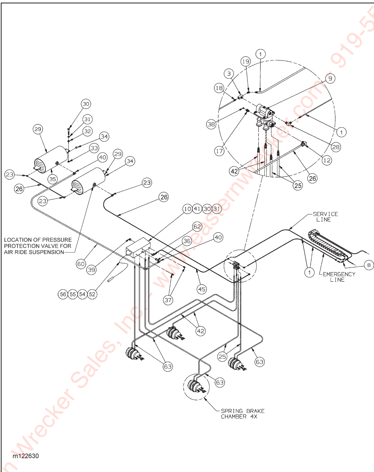
Figure 1-26 Spring Air Brake System w/ ABS (425 & 435)
