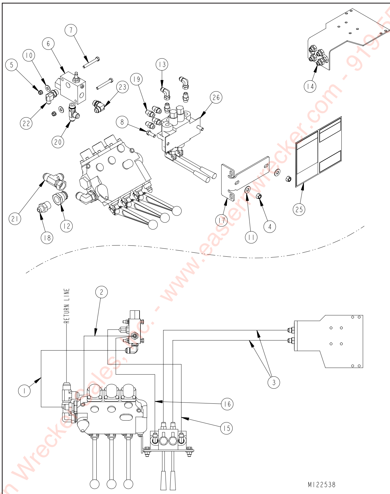
Figure 1-54 Dock Leveler Hydraulic Installation (Option)
