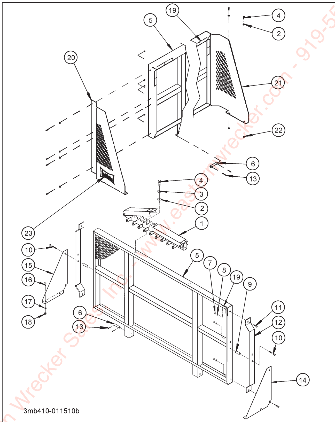
Figure 1-3 Bulkhead Assembly
