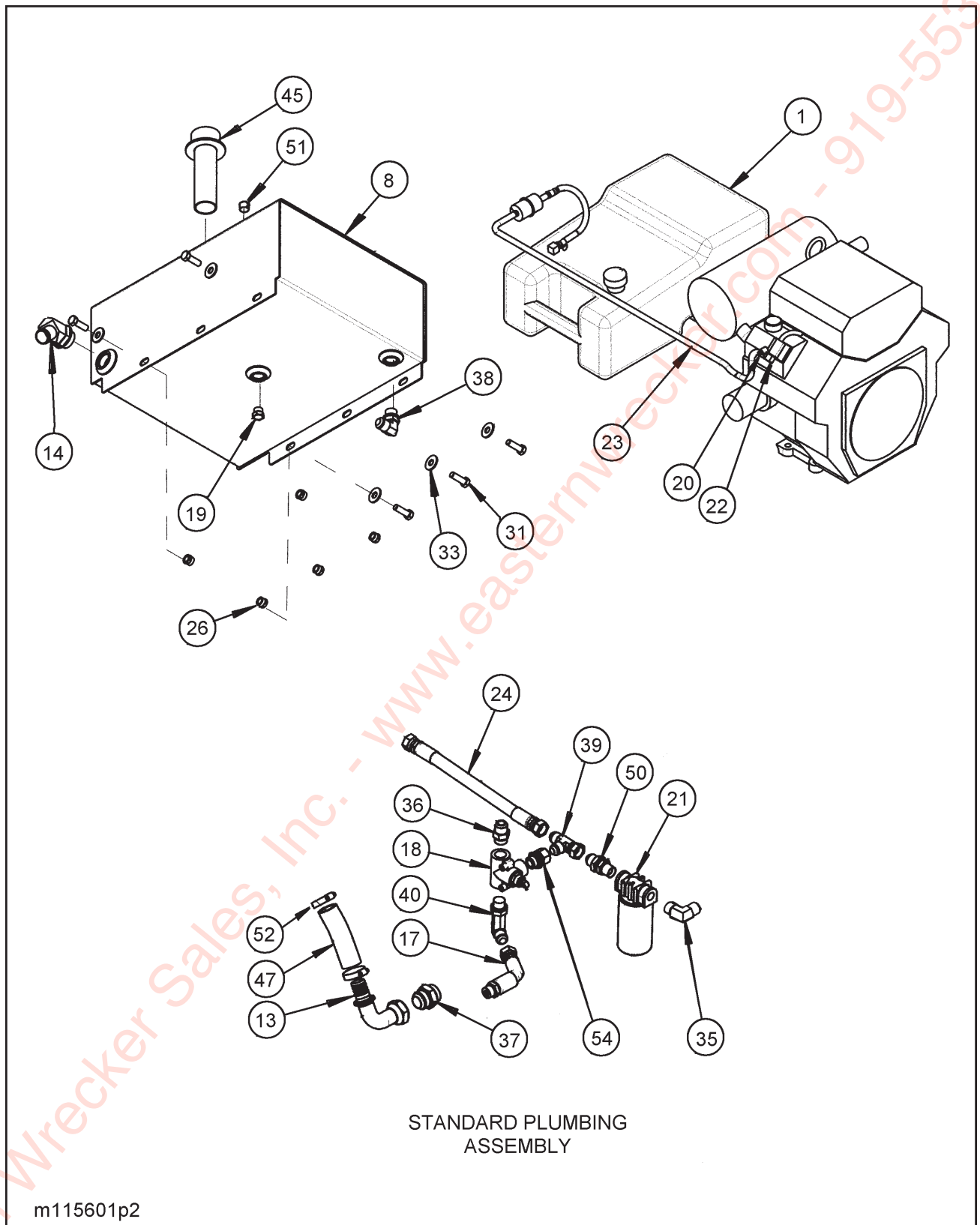
Figure 1-65 Hydraulic Engine, Standard Mount (2 of 2)
