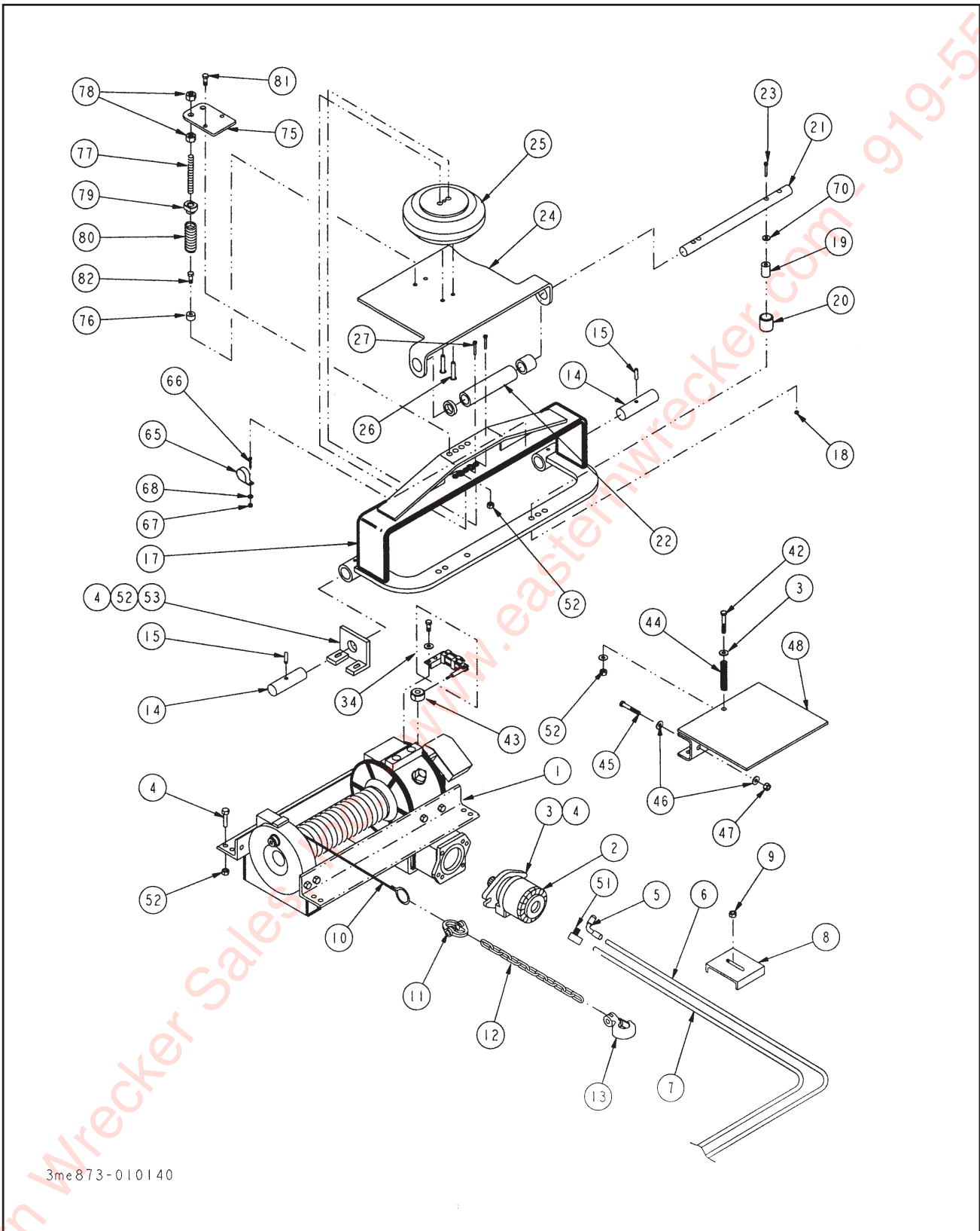
Figure 1-31 Winch Installation (1 of 2)
