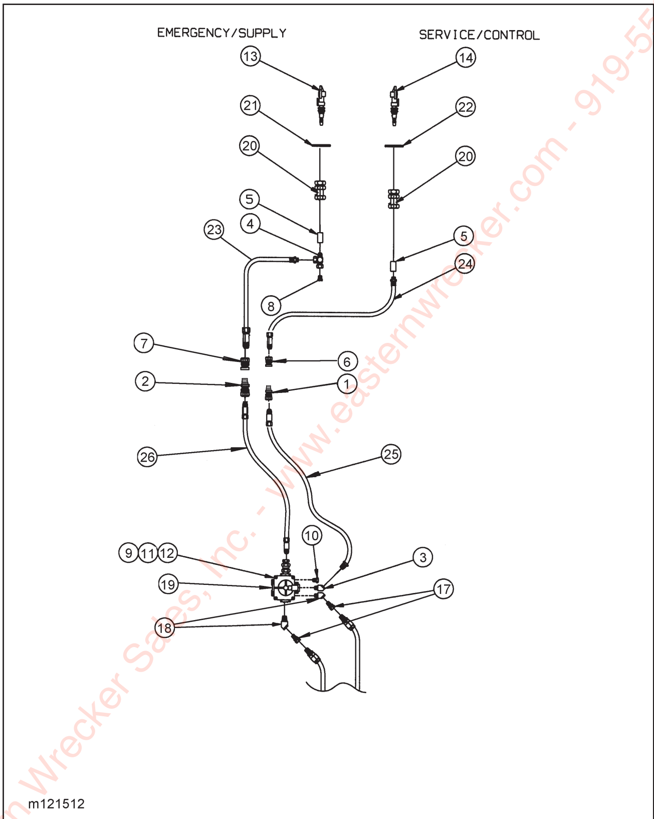
Figure 1-29 Air System ABS
