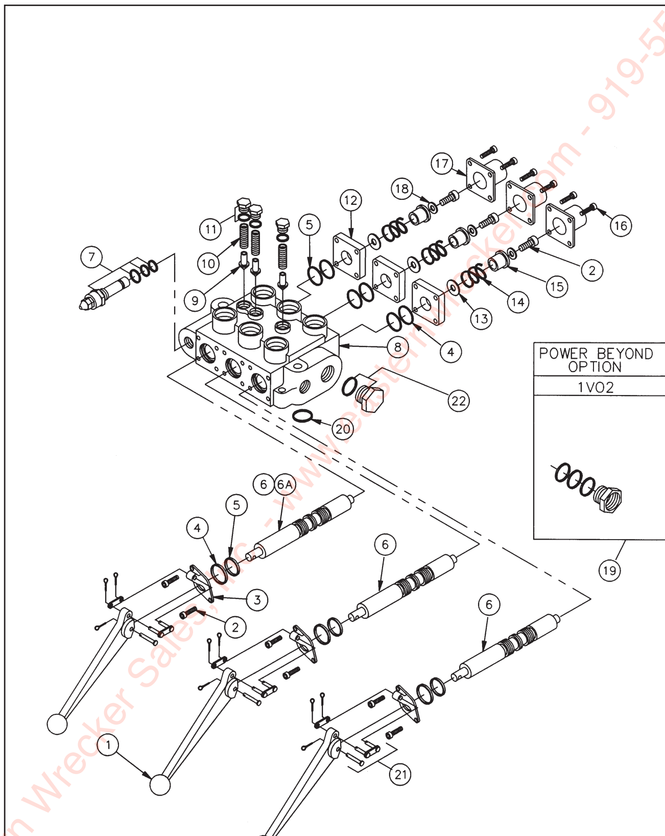
Figure 1-17 Three Spool Valve
