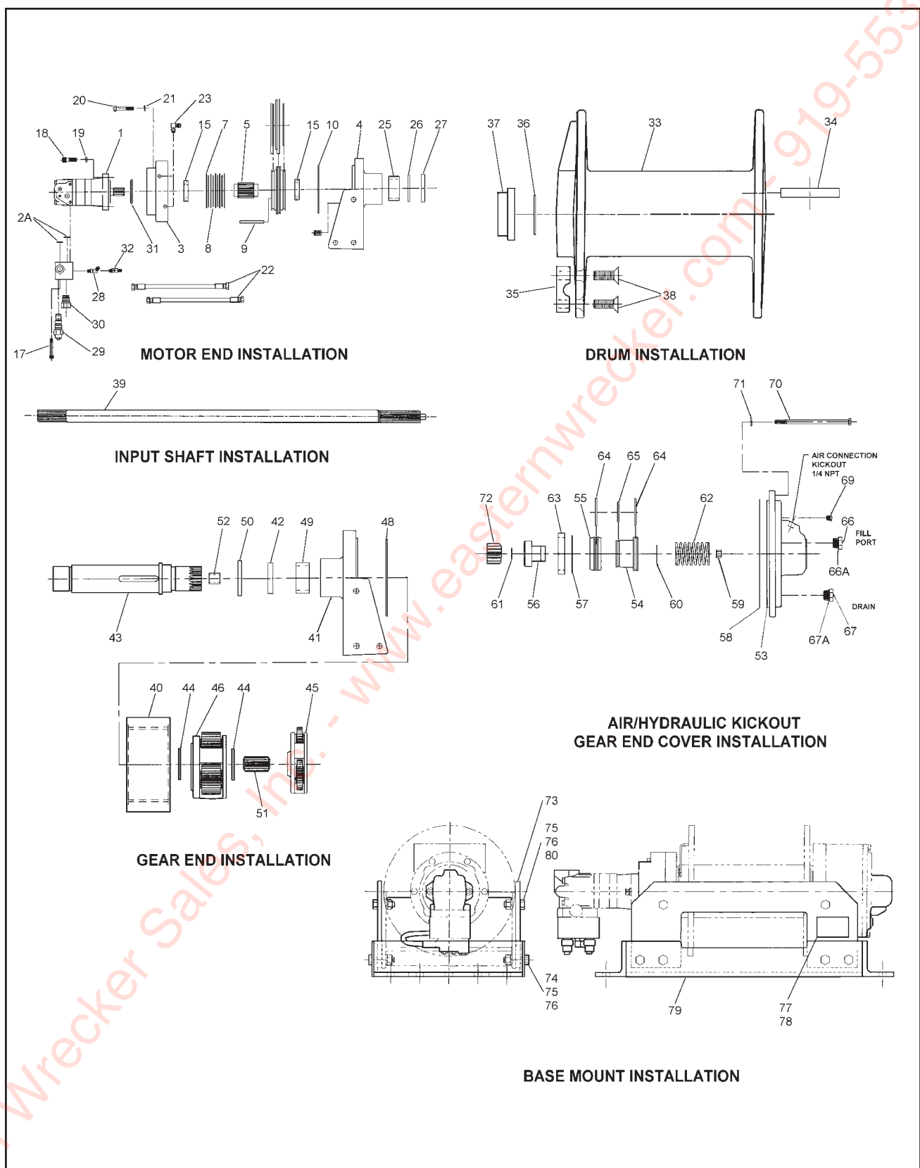
Figure 1-40 30,000# Winch Items
