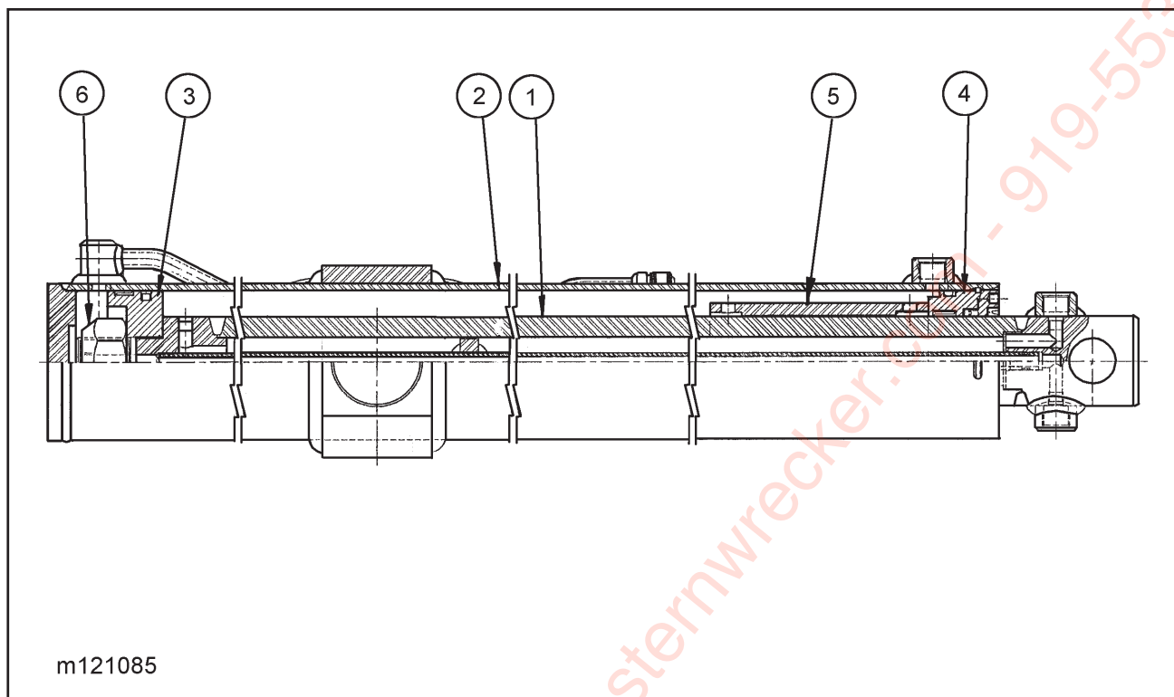
Figure 1-9 Cylinder, Hydraulic 4 x 126 (Streetside) (410-50/53 & 435-48/50CA)
