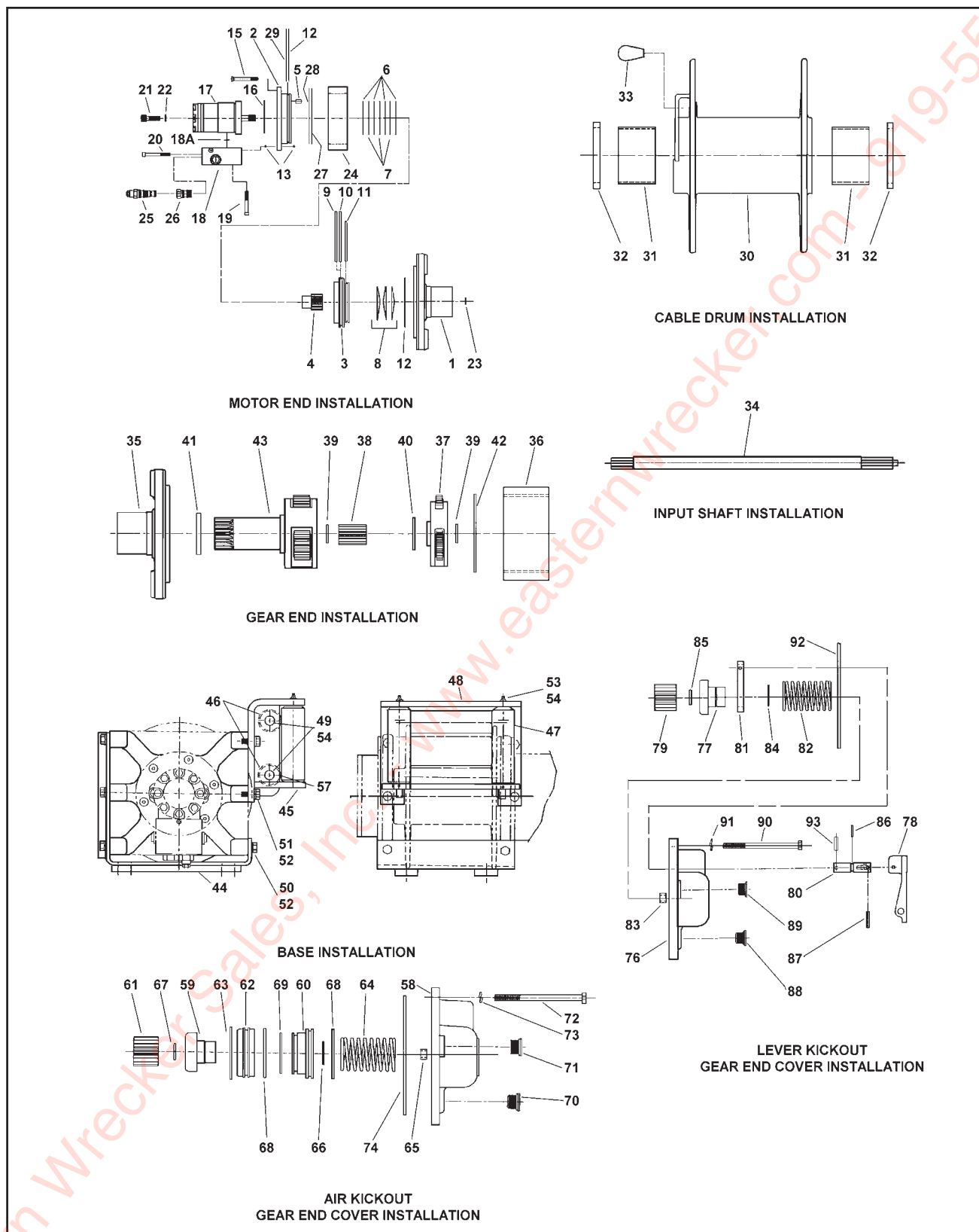
Figure 1-47 12K, 15K, & 20K Winch Items (DP Planetary)
