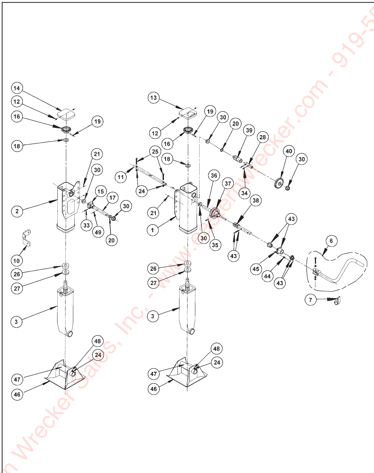
Figure 1-62 Crank Landing Gear
