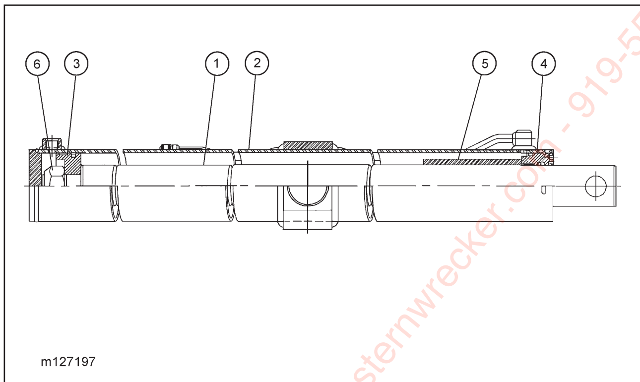
Figure 1-12 Cylinder, Hydraulic 4 x 138 (Curbside) (435-50CA/53)
