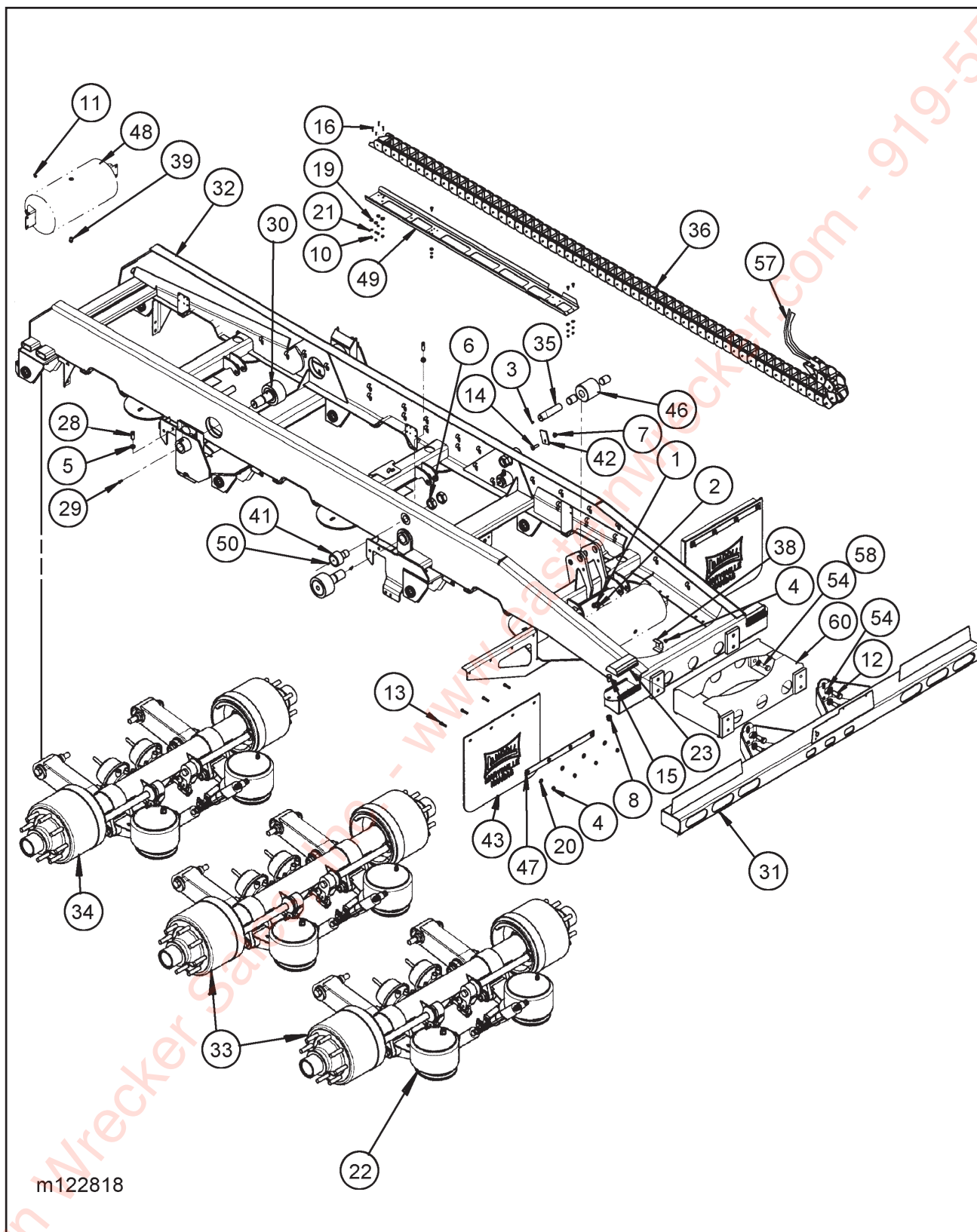
Figure 1-20 U/C Assembly, Air Ride Suspension (410)
