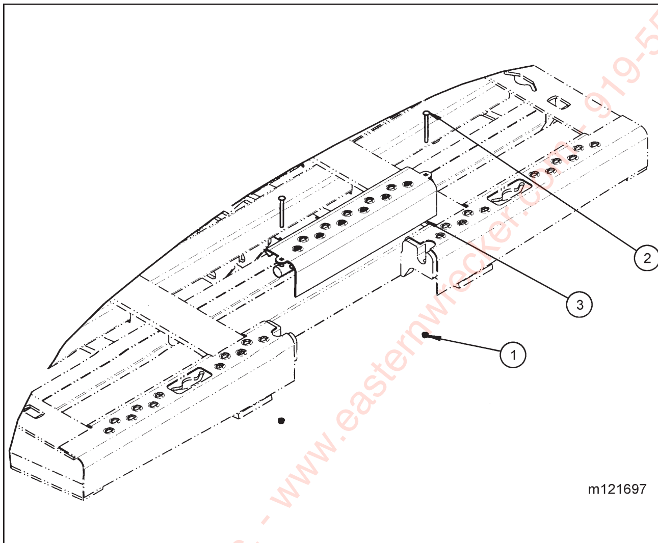
Figure 1-68 Center Rub Plate Cover Installation (Option)
