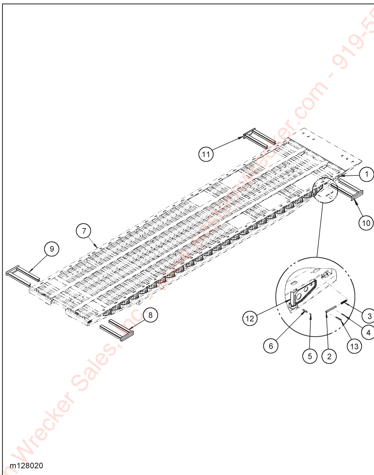
Figure 1-5 Outrigger Installation (Option)
