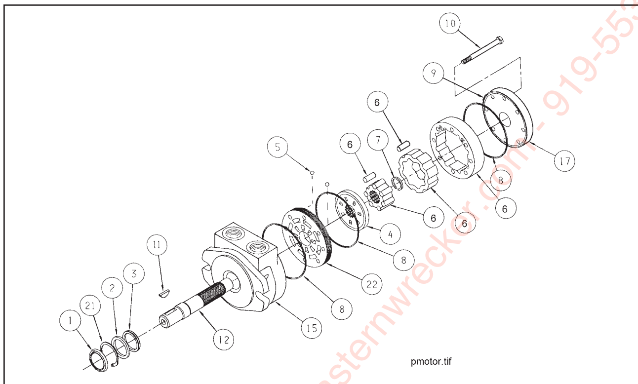
Figure 1-37 Winch Motor Assembly
