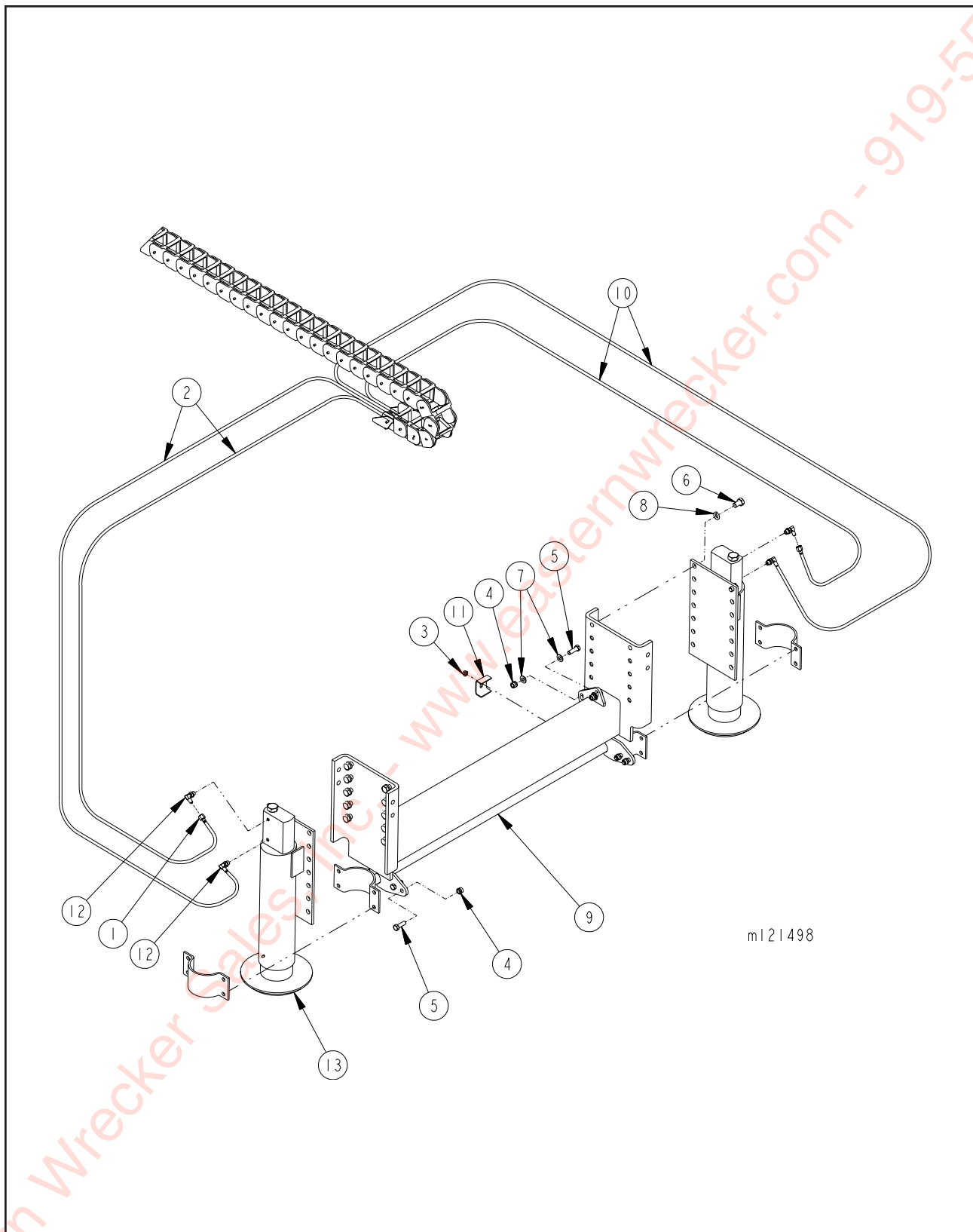
Figure 1-55 Dock Leveler Assembly, Single 60K
