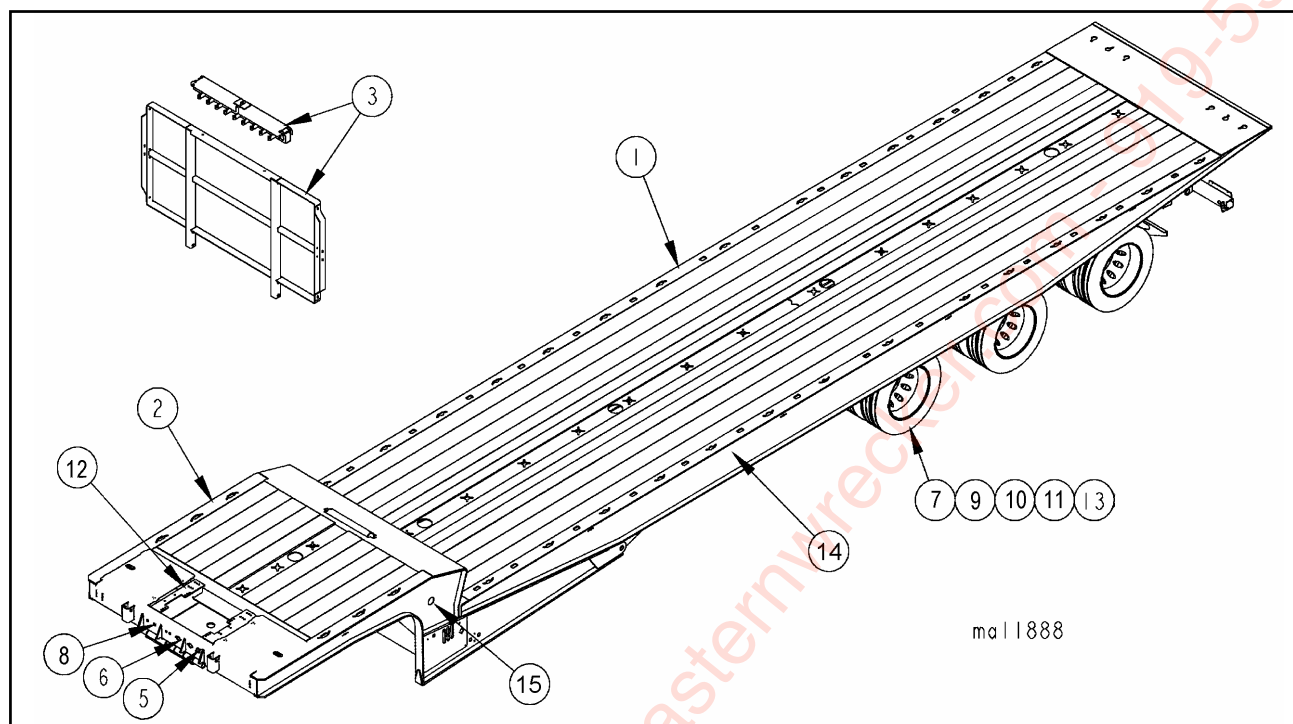
Figure 1-1 General Assembly
