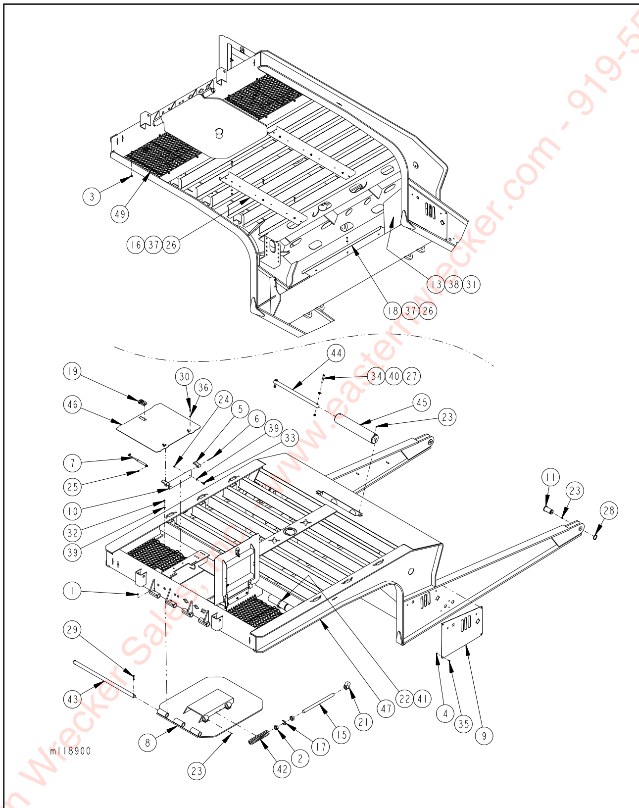
Figure 1-2 Gooseneck Frame Assembly
