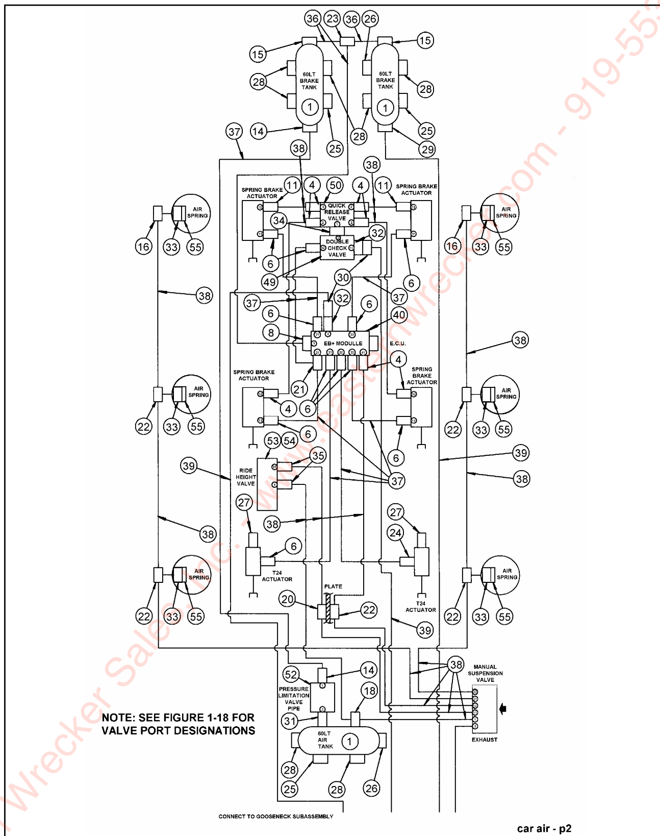
Figure 1-17 Air System - Undercarriage (2 of 3)
