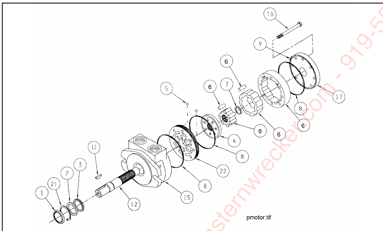
Figure 1-23 Winch Motor Assembly
