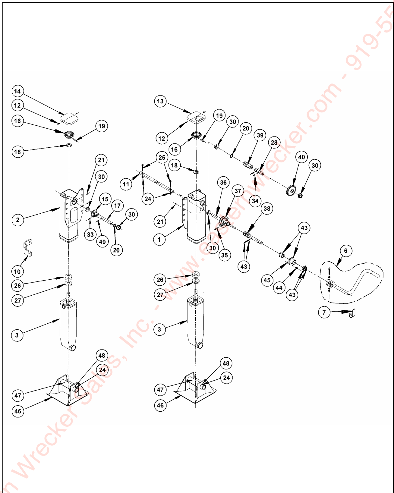
Figure 1-32 Crank Landing Gear
