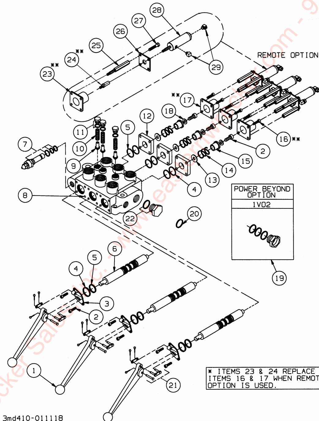
Figure 1-10 Three Spool Valve
