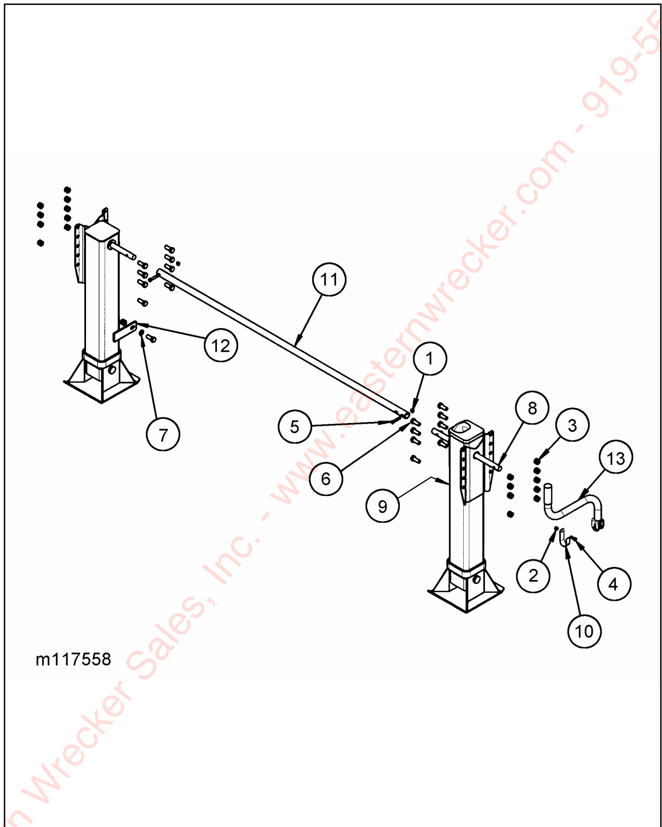
Figure 1-31 Landing Gear Installation
