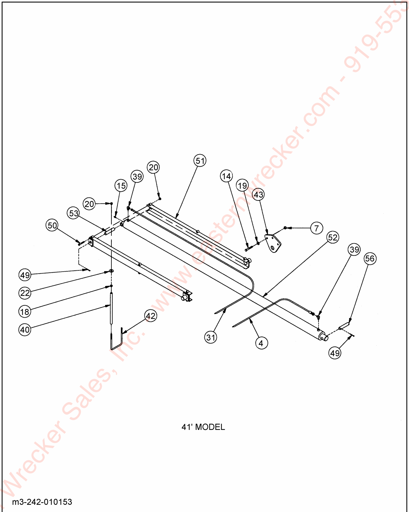
Figure 1-6 Hydraulic System (2 of 2)
