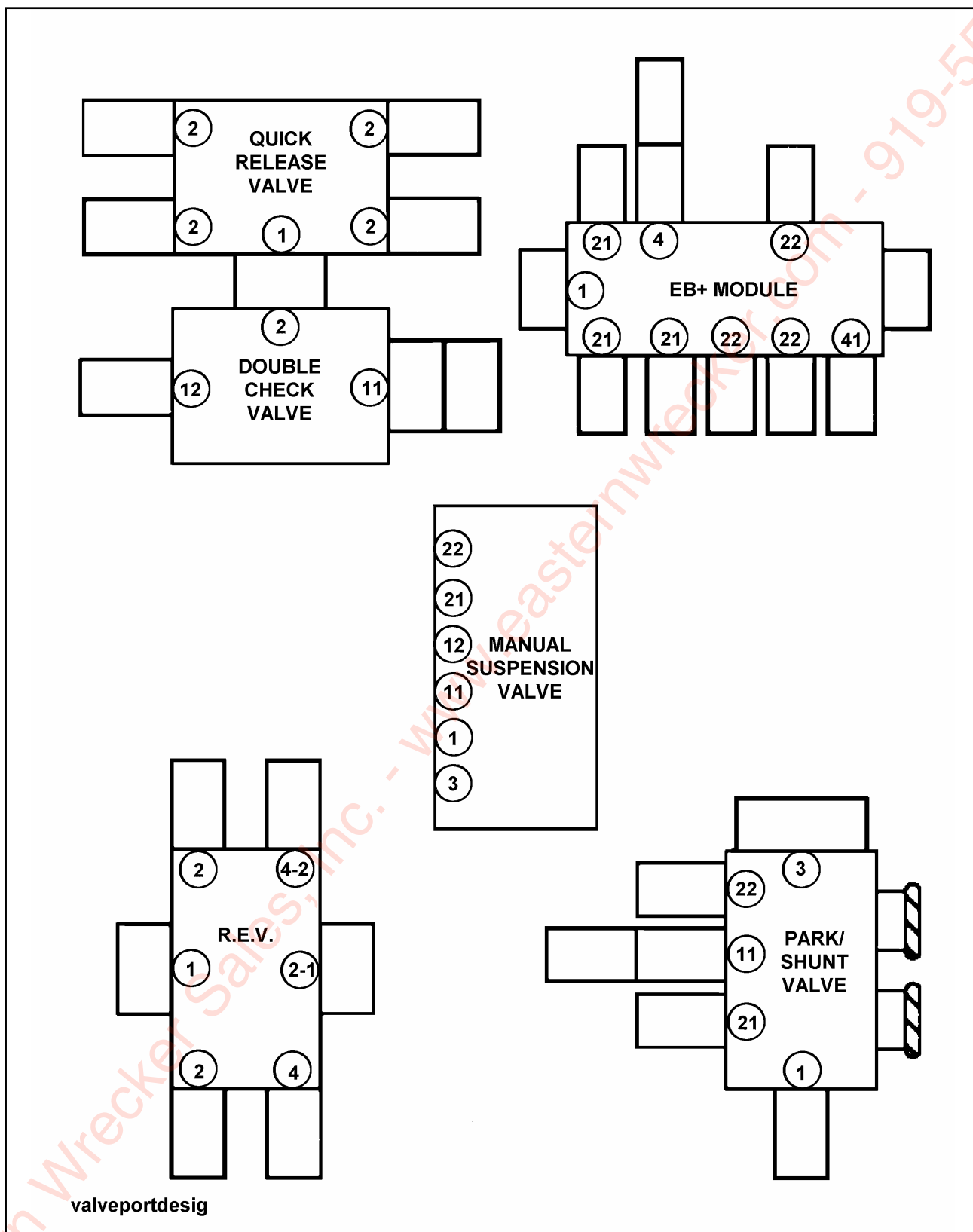
Figure 1-18 Valve Port Designations (3 of 3)
