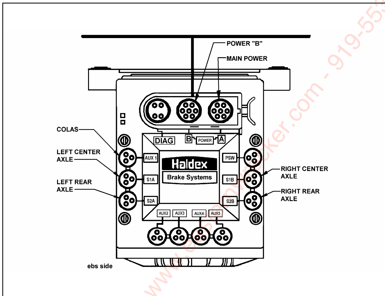
Figure 1-13 EBS Modulator Valve - Side View
