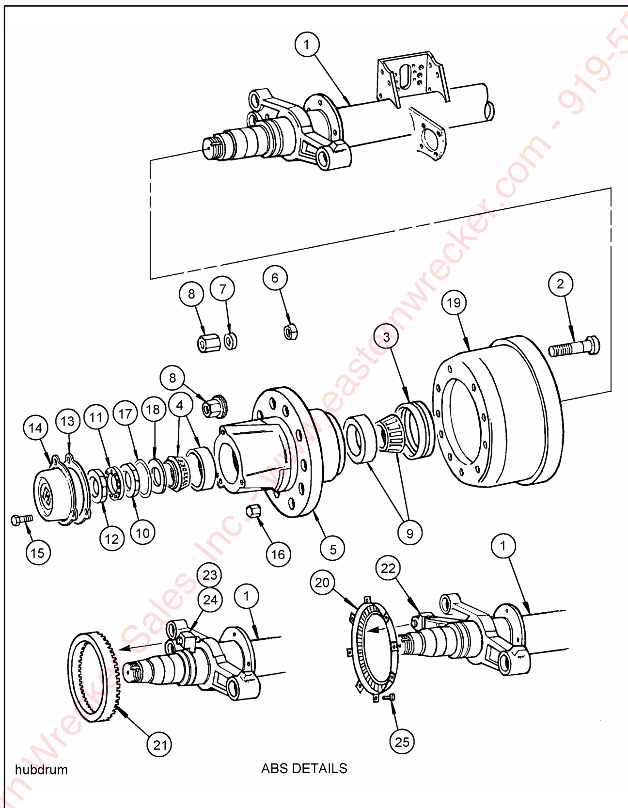
Figure 1-21 Inboard Pilot Mount Hub and Drum
