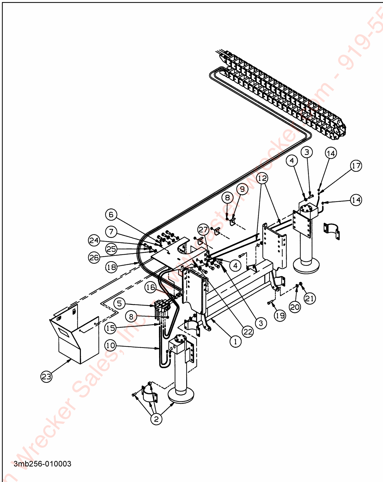
Figure 1-25 Dock Leveler, 60K
