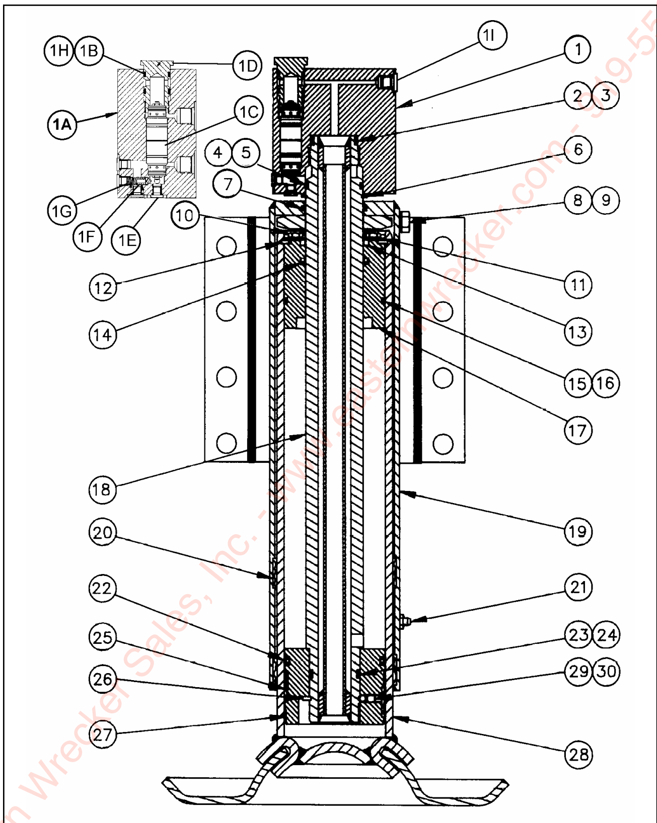
Figure 1-27 Dock Leveler Leg Assembly w/ Lock Valve
