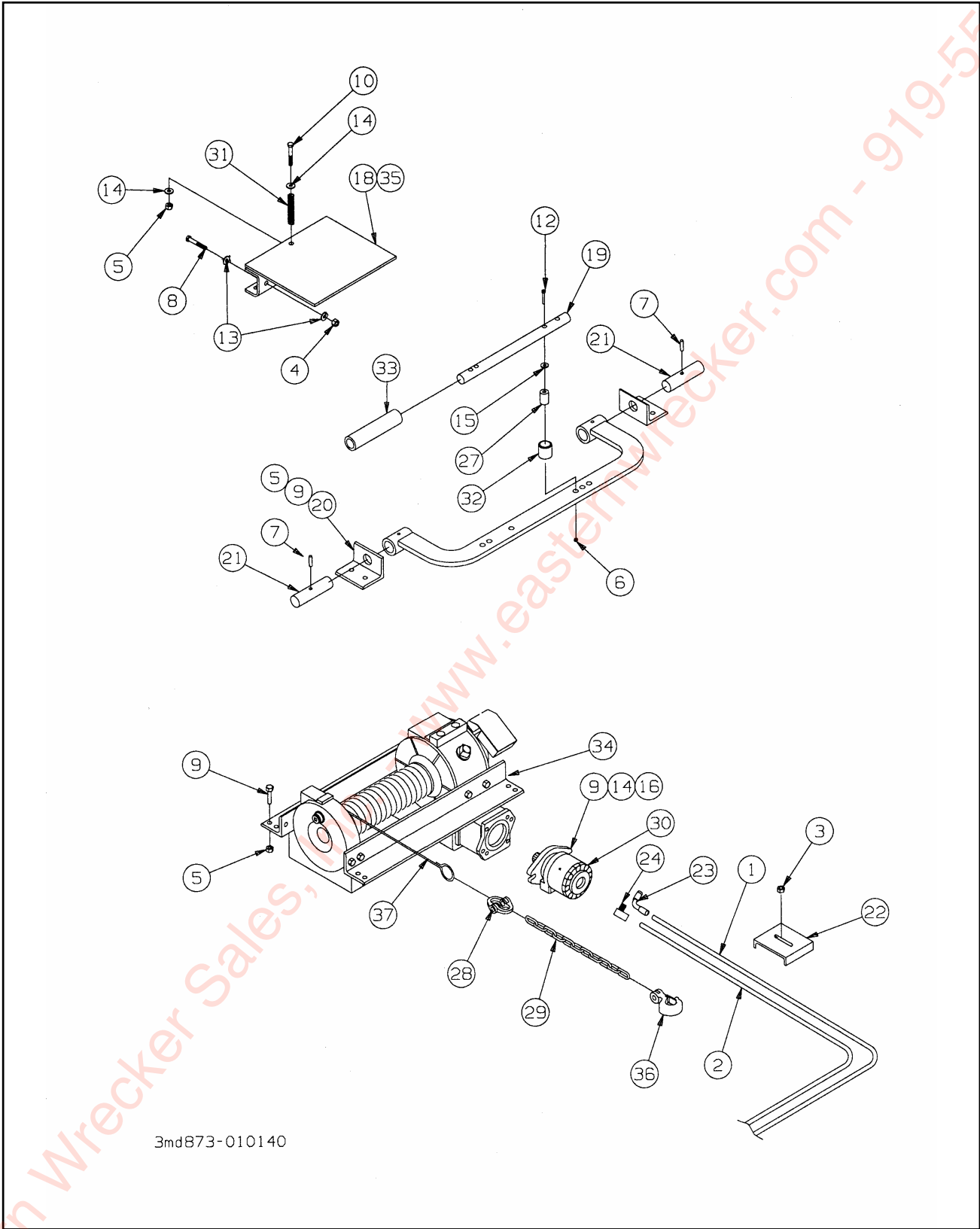
Figure 1-22 Winch Installation
