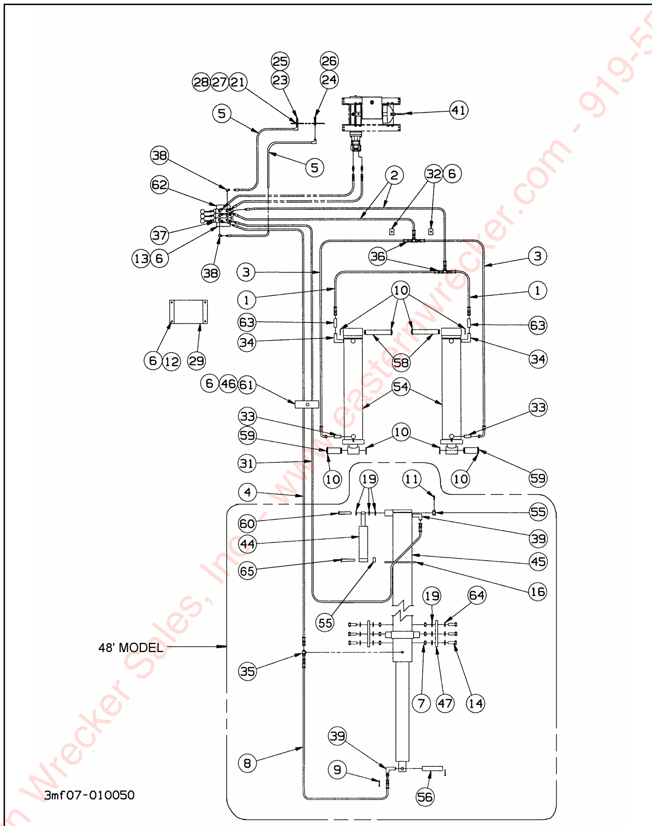
Figure 1-5 Hydraulic System (1 of 2)
