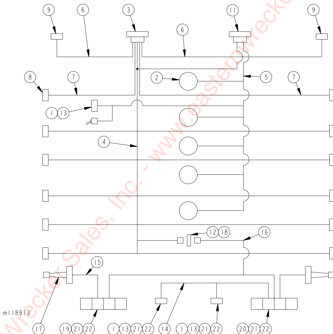
Figure 1-11 Lighting System Schematic
