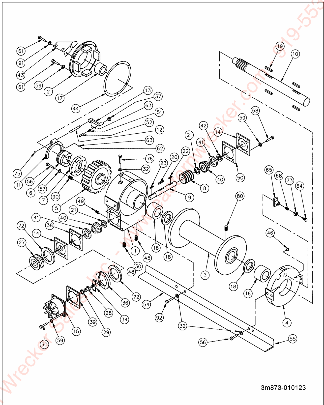
Figure 1-24 20,000# Winch Items
