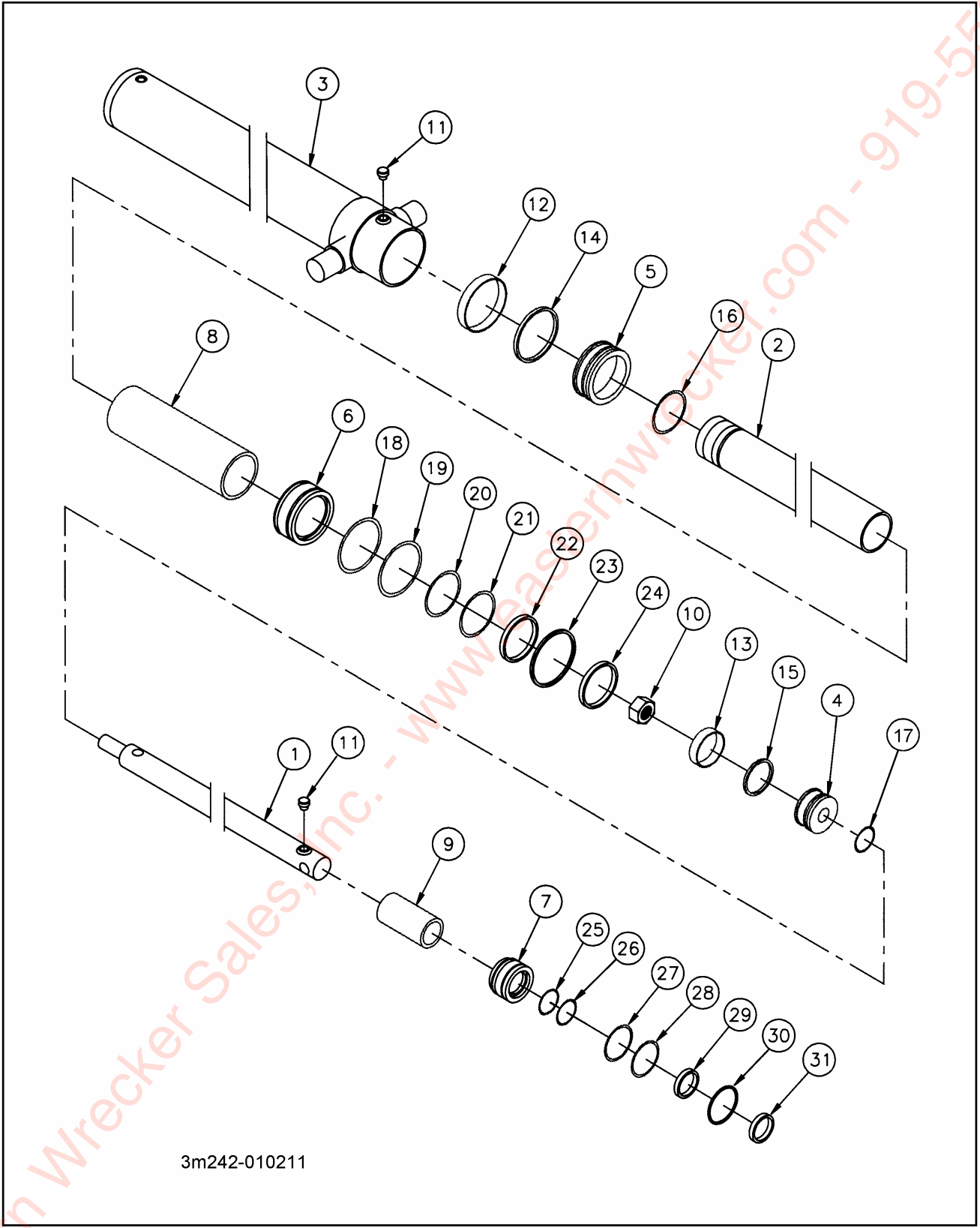
Figure 1-7 Cylinder, Telescopic
