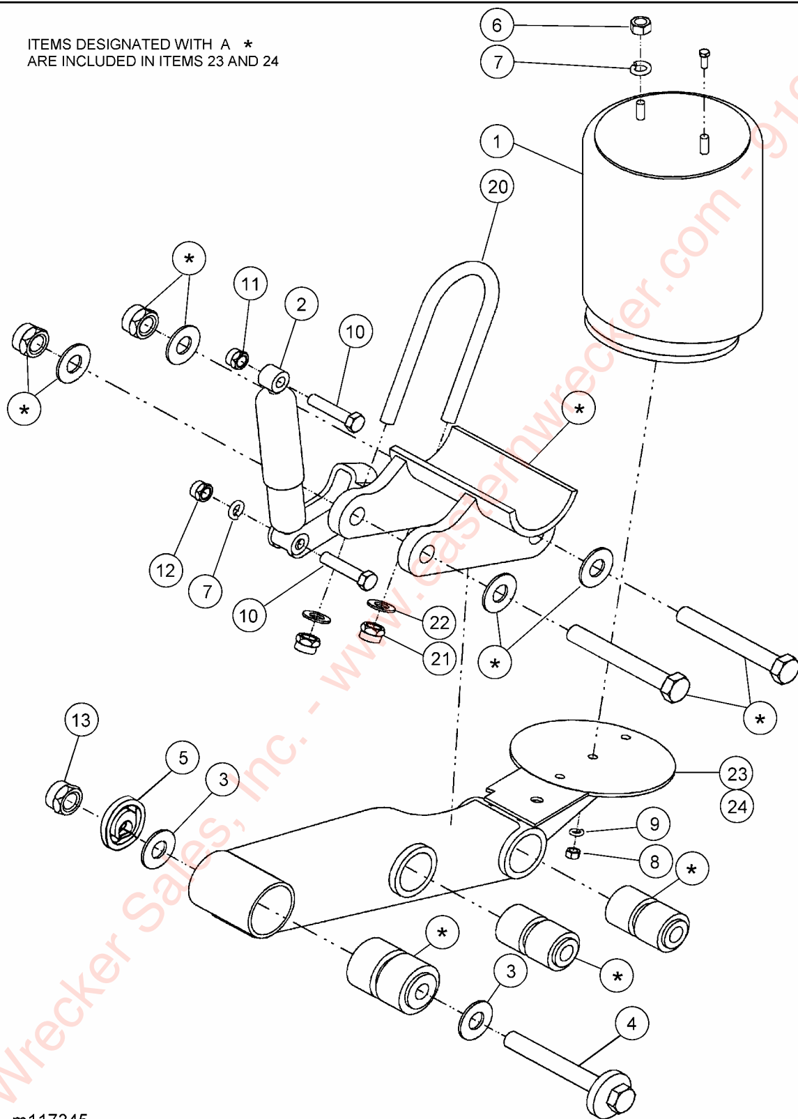
Figure 1-20 Suspension Hanger RLU-250
