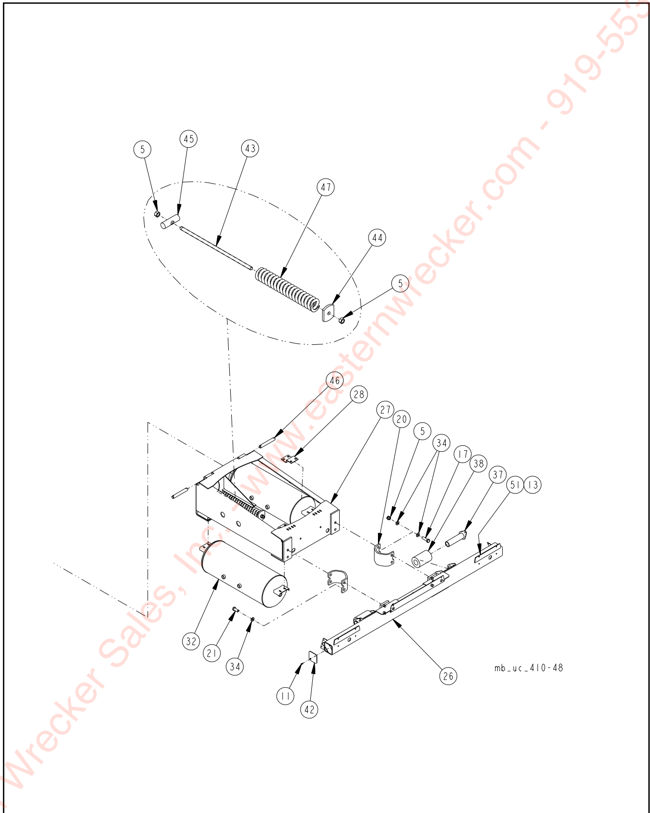
Figure 1-15 U/C Assembly, Air Ride Suspension
