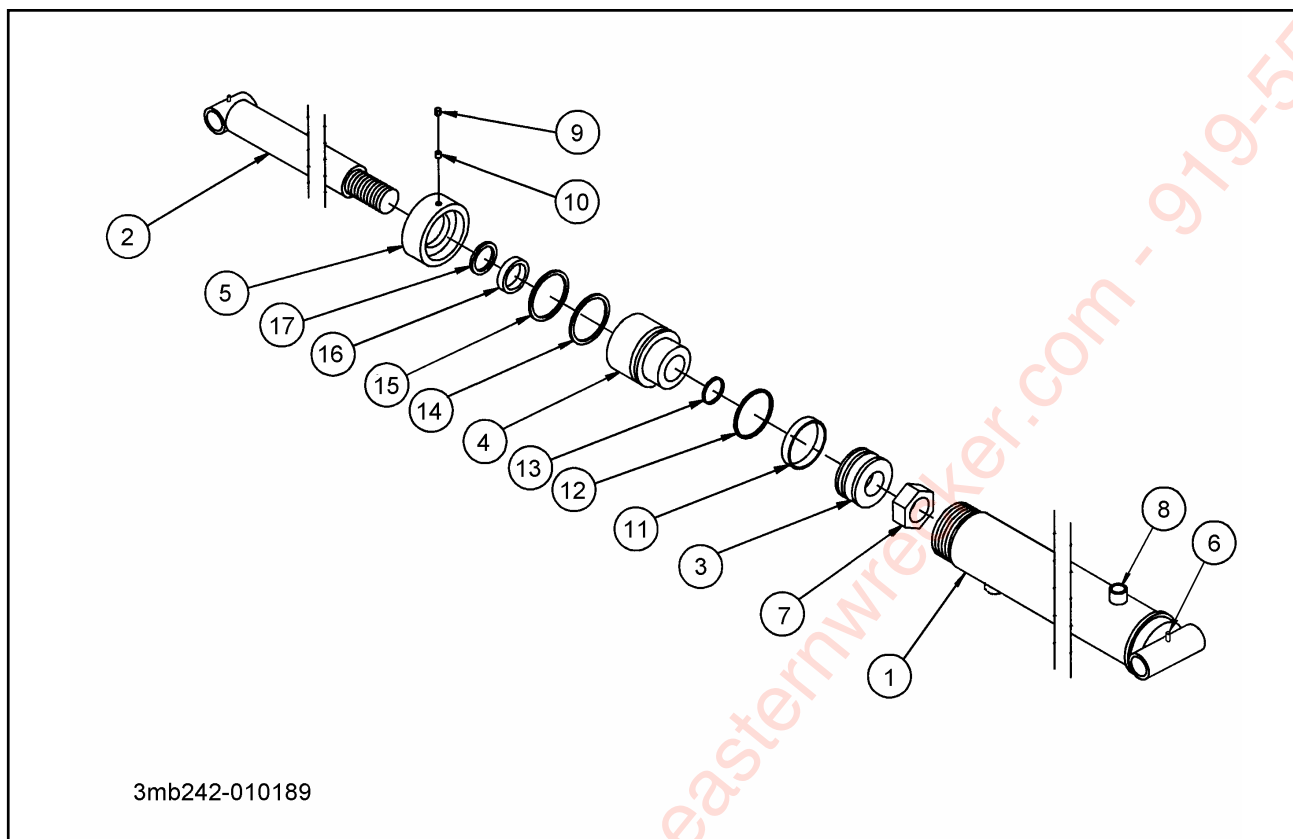
Figure 1-8 Cylinder 6" X 41"
