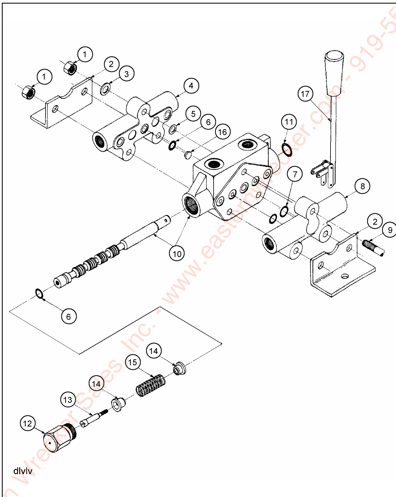
Figure 1-28 Dock Leveler Valve
