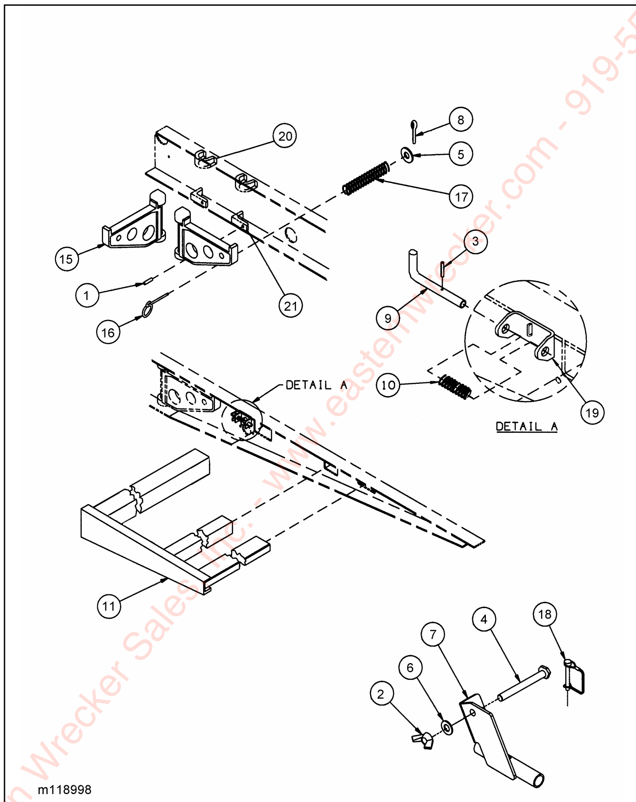
Figure 1-4 Outrigger/Pullout Installation
