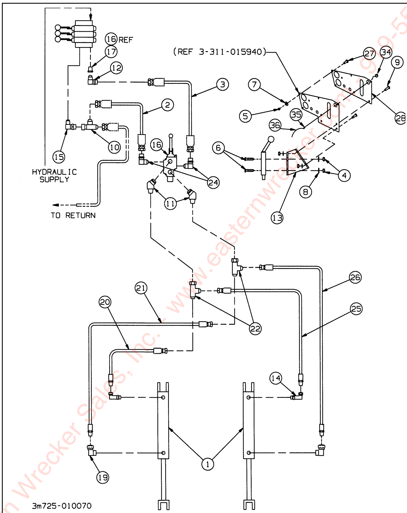
Figure 1-55 Hydraulic Landing Gear
