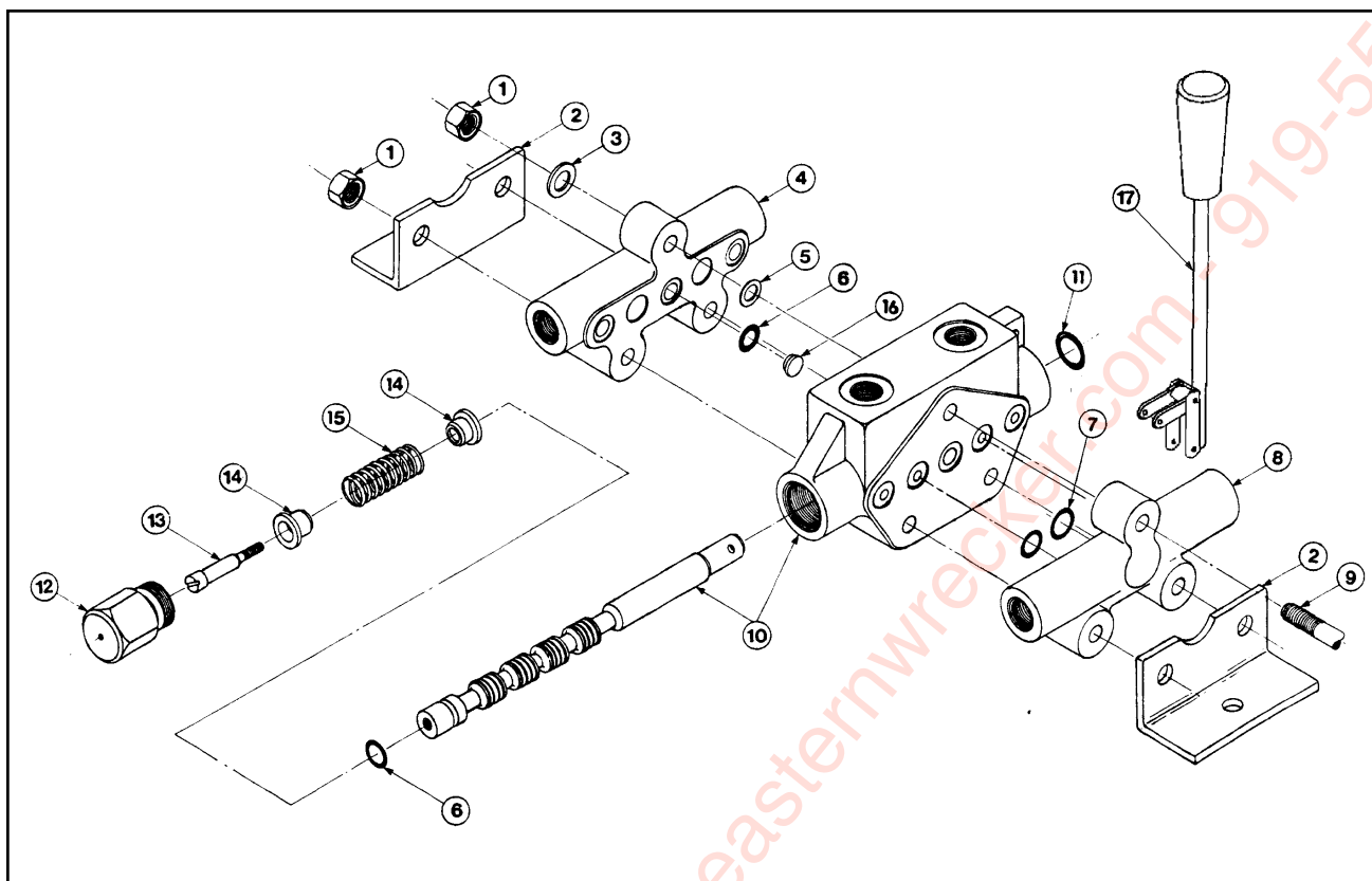
Figure 1-51 Dock Leveler Valve
