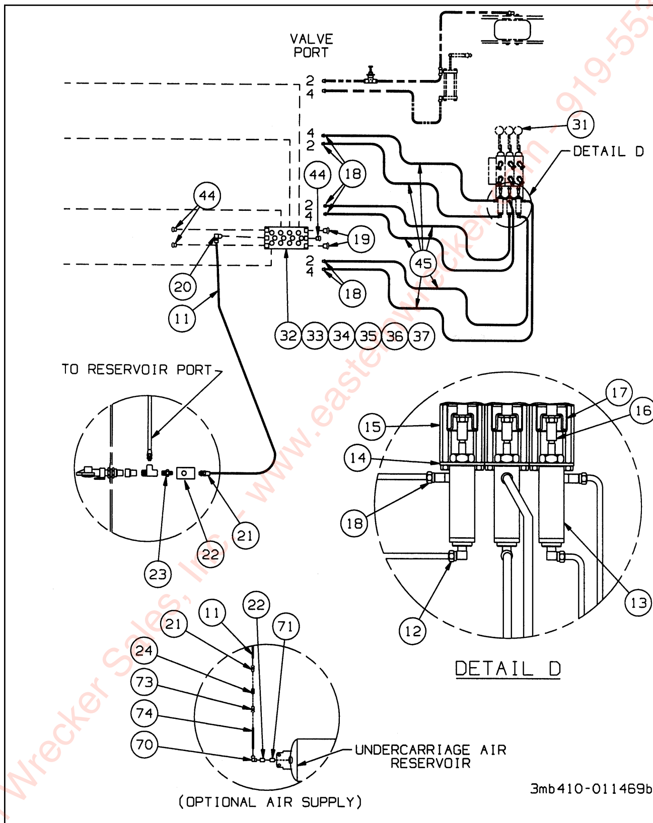
Figure 1-45 Remote Control Items (2 of 2)
