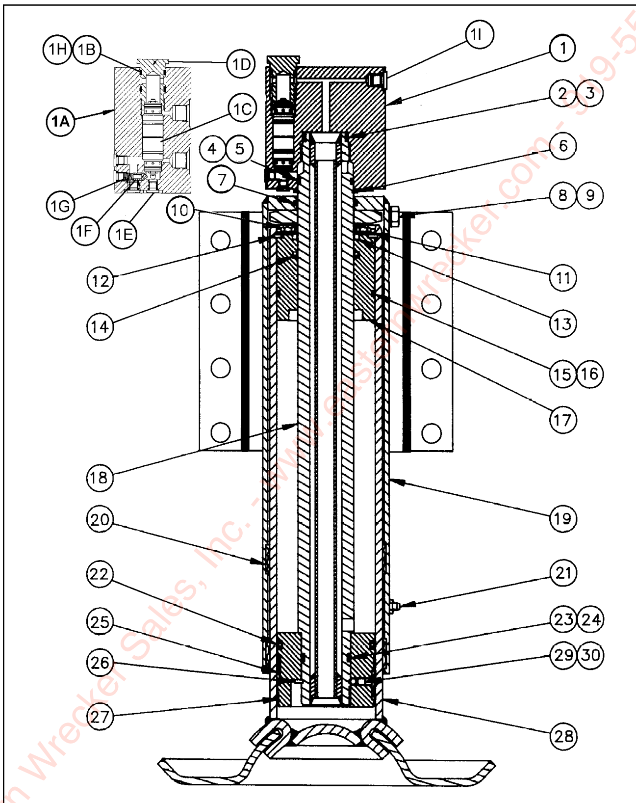
Figure 1-50 Dock Leveler Leg Assembly w/ Lock Valve
