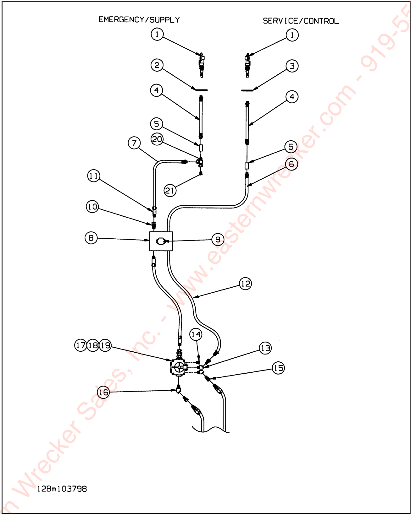
Figure 1-28 Air System ABS
