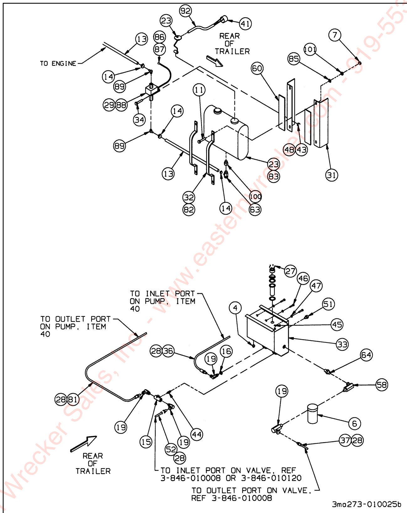
Figure 1-58 Hydraulic Engine, Standard Mount (2 of 2)
