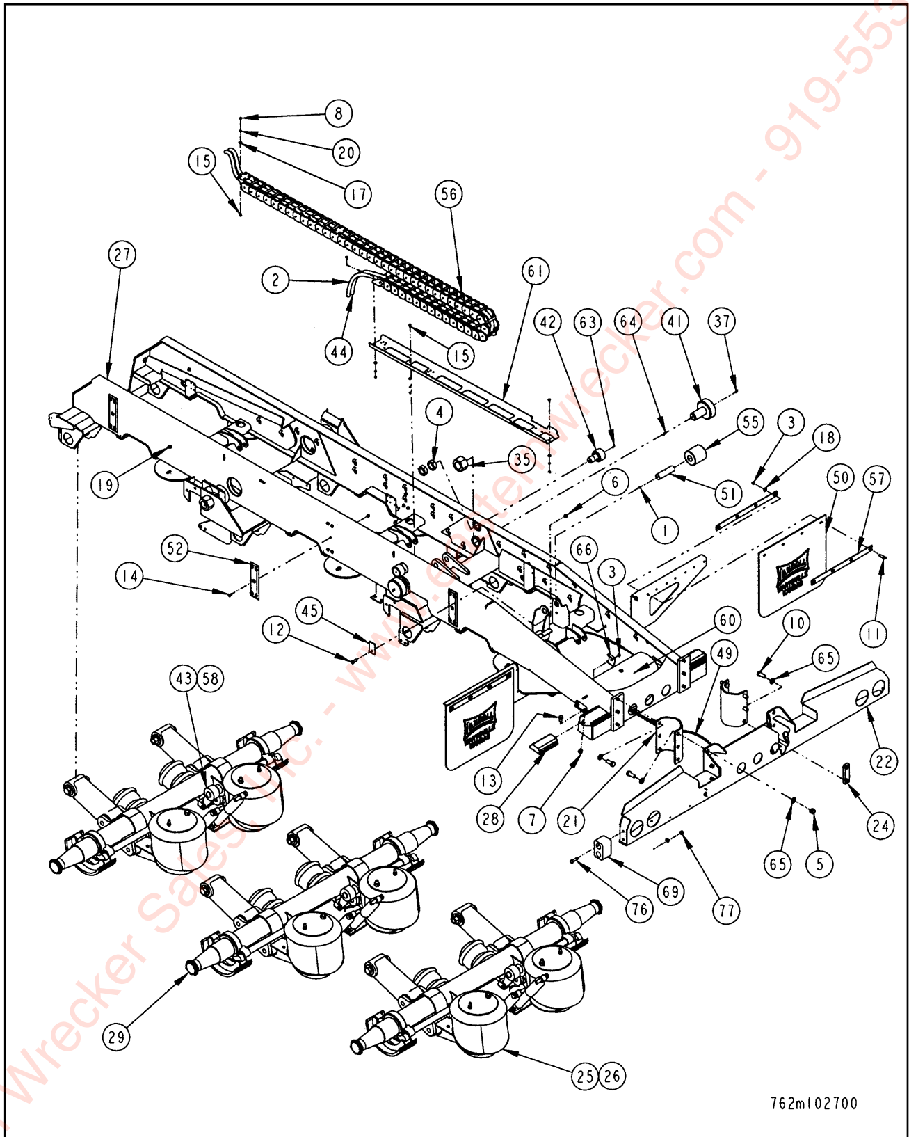
Figure 1-19 U/C Assembly, Air Ride Suspension (2 of 2)
