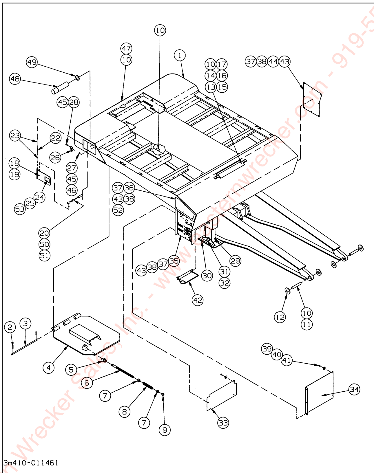
Figure 1-2 Upper Deck Assembly
