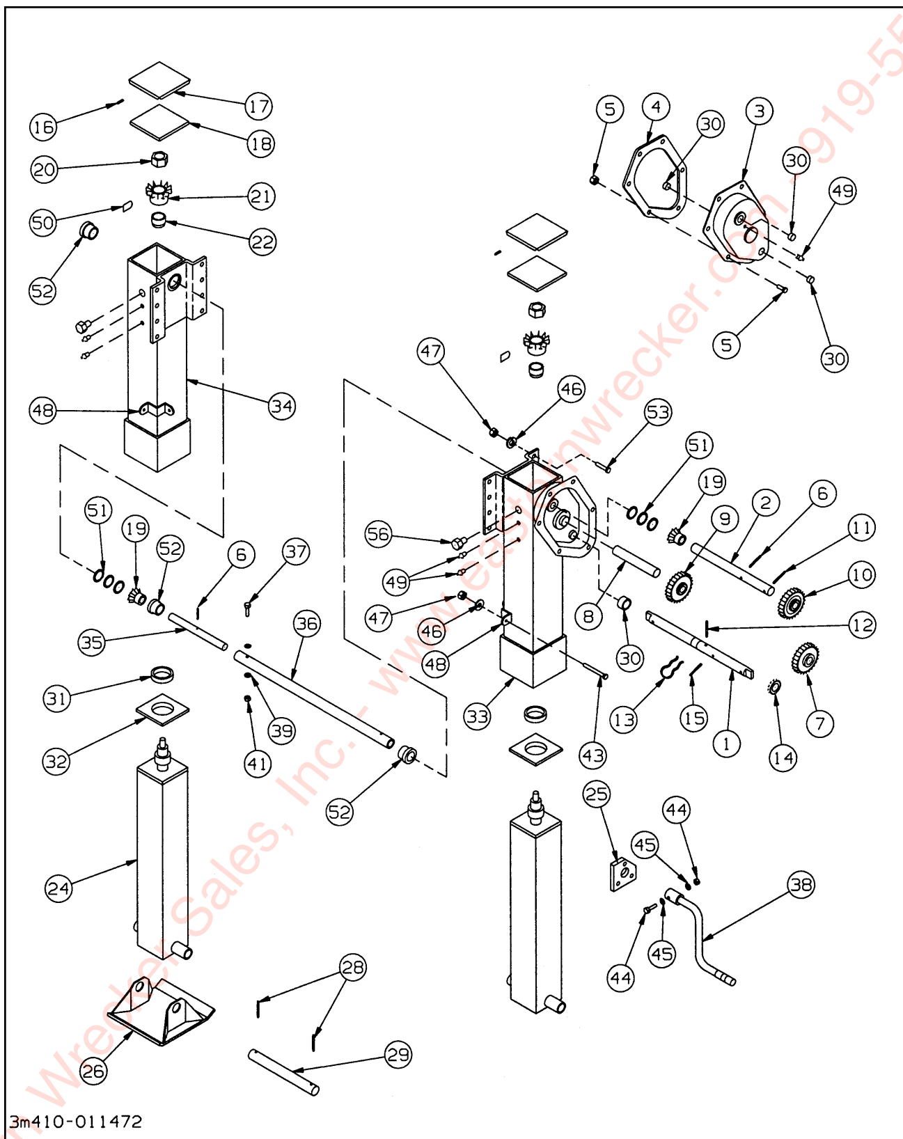
Figure 1-54 Crank Landing Gear
