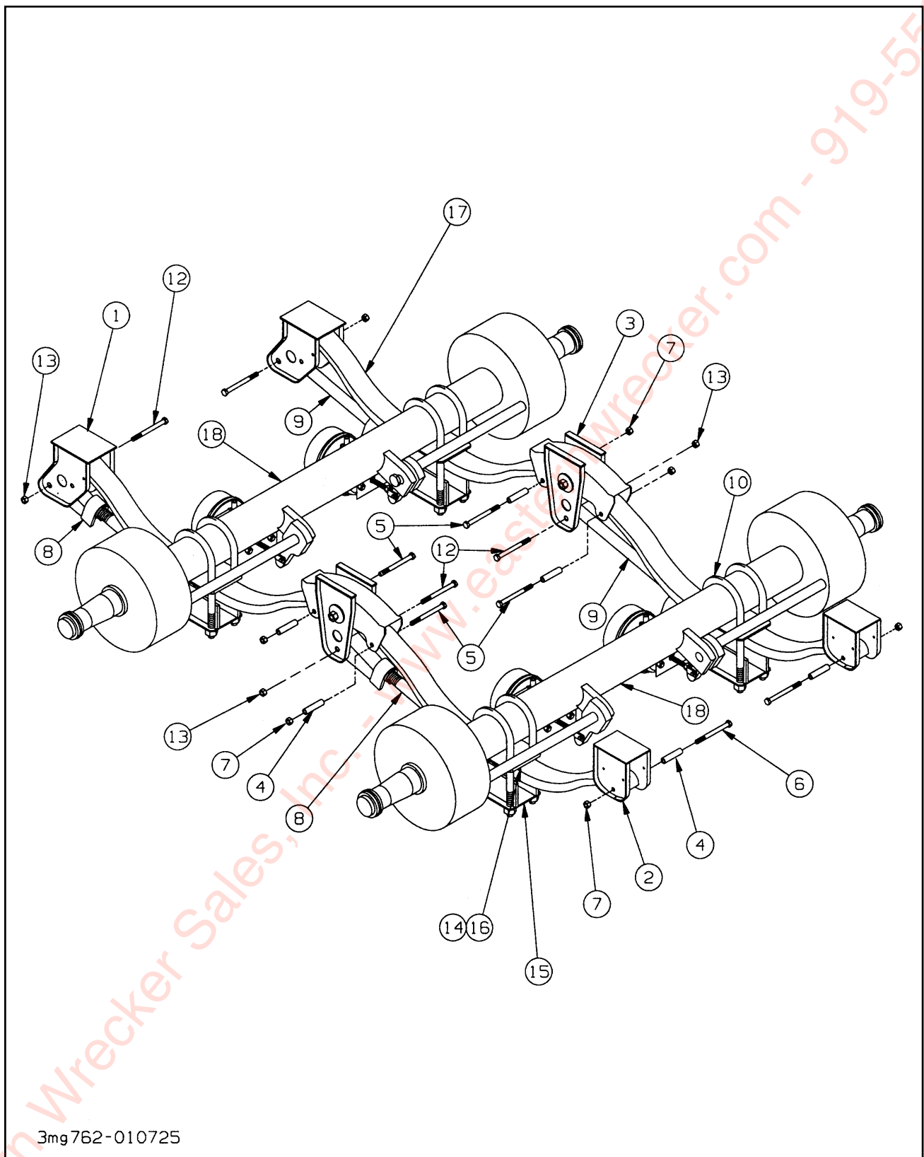
Figure 1-17 Suspension, Single Leaf Spring
