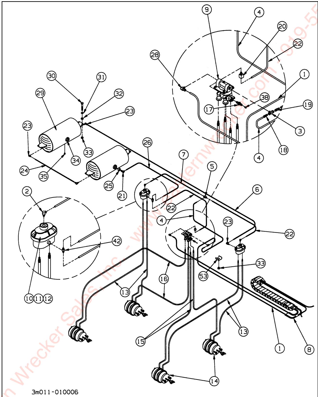
Figure 1-25 Spring Air Brake System w/o ABS, Tandem
