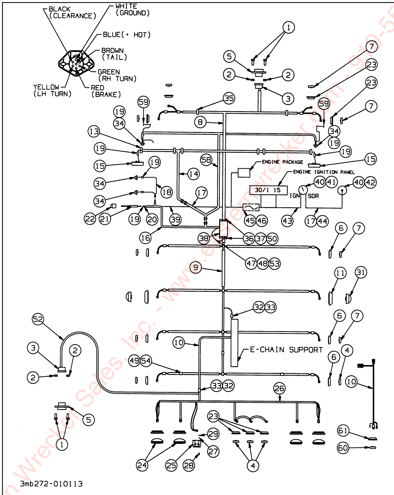
Figure 1-15 Electrical System Schematic
