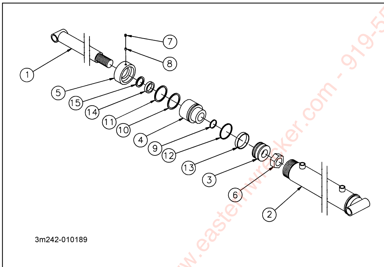
Figure 1-11 Cylinder 6" X 41"
