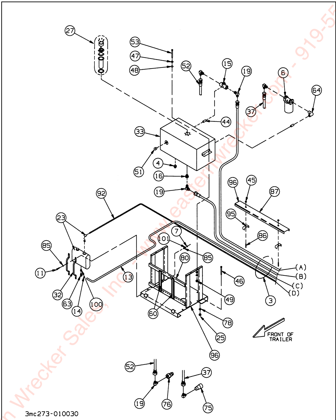
Figure 1-59 Hydraulic Engine, Split Mount (1 of 2)
