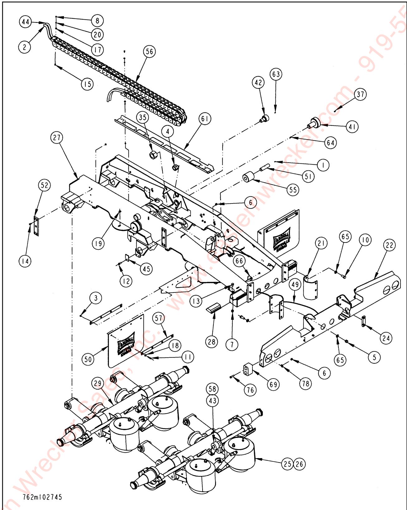
Figure 1-18 U/C Assembly, Air Ride Suspension (1 of 2)
