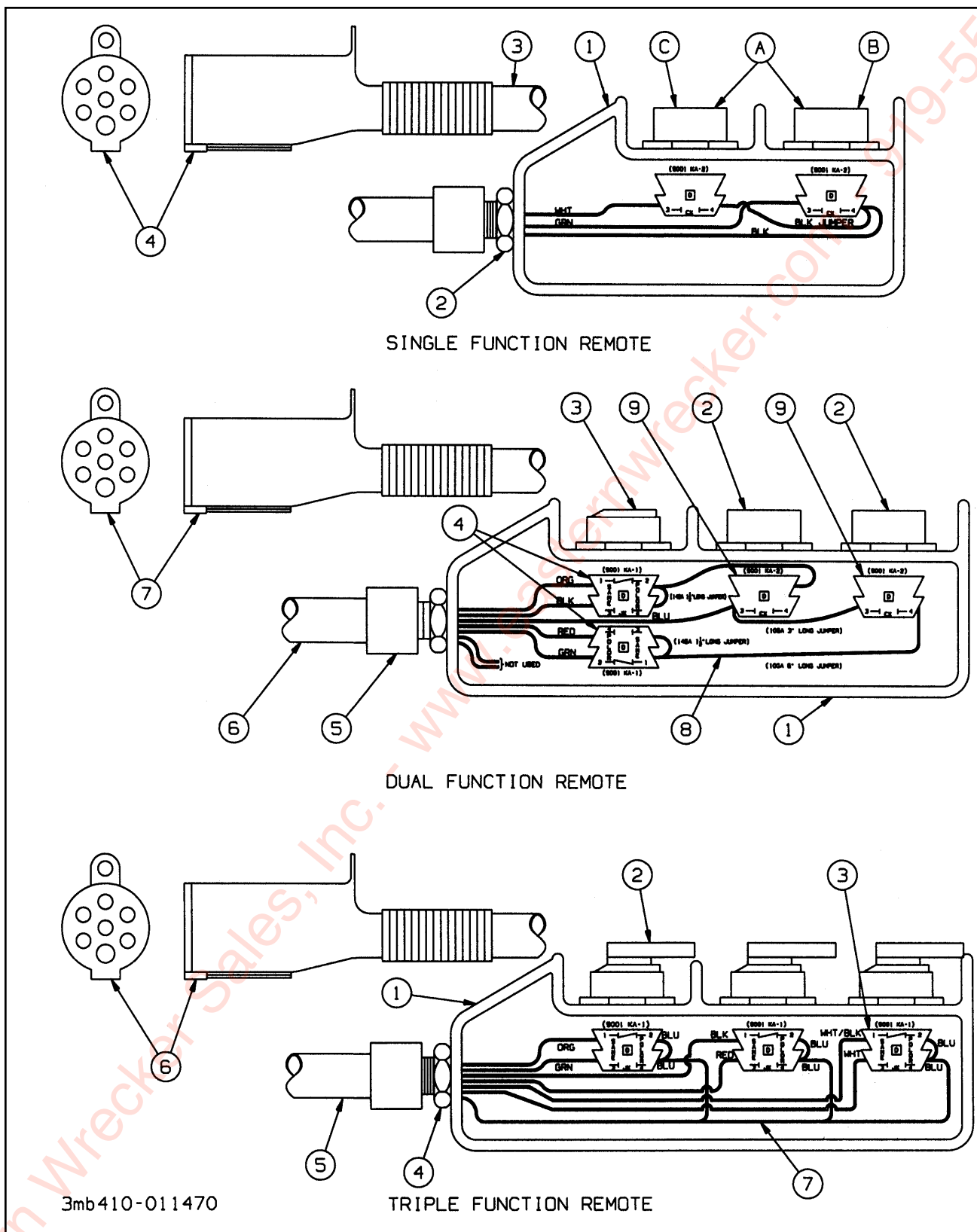
Figure 1-46 Wired Remote Control
