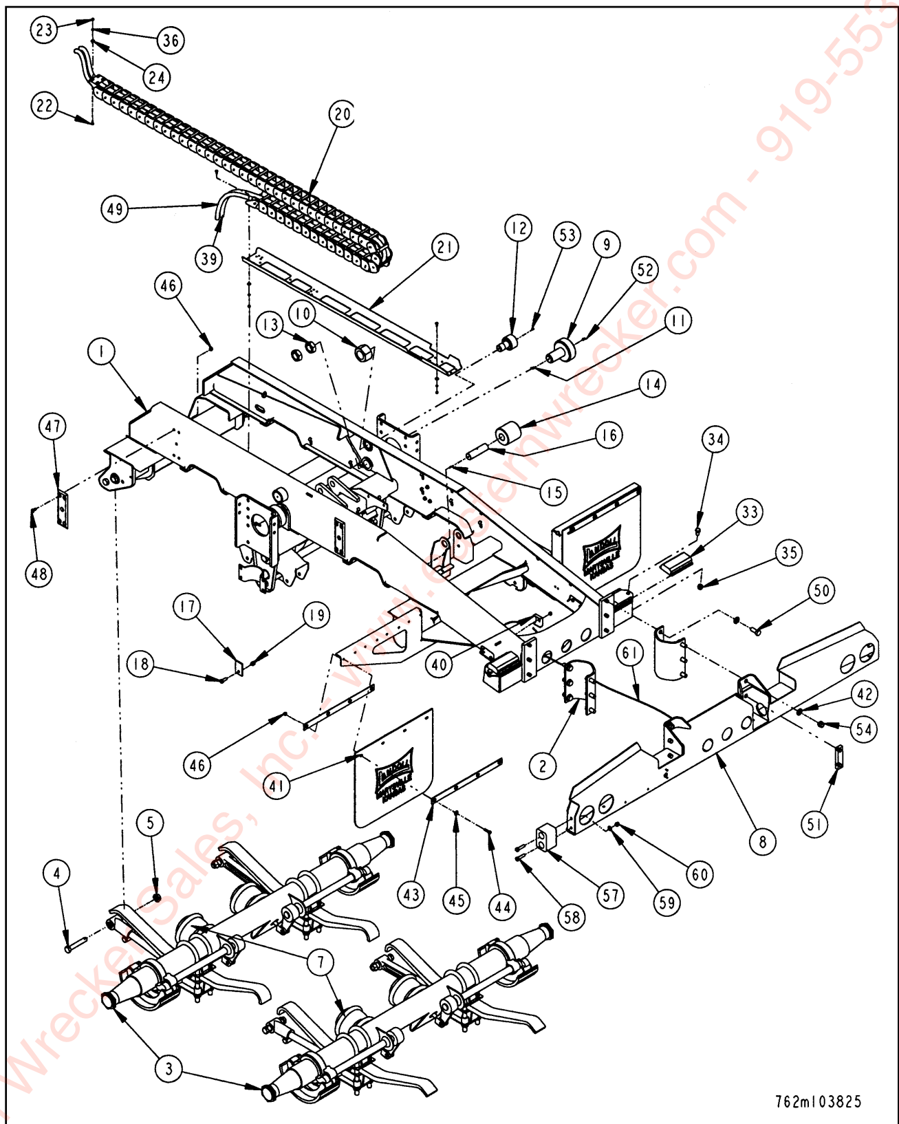
Figure 1-16 Undercarriage Assembly - Spring Suspension
