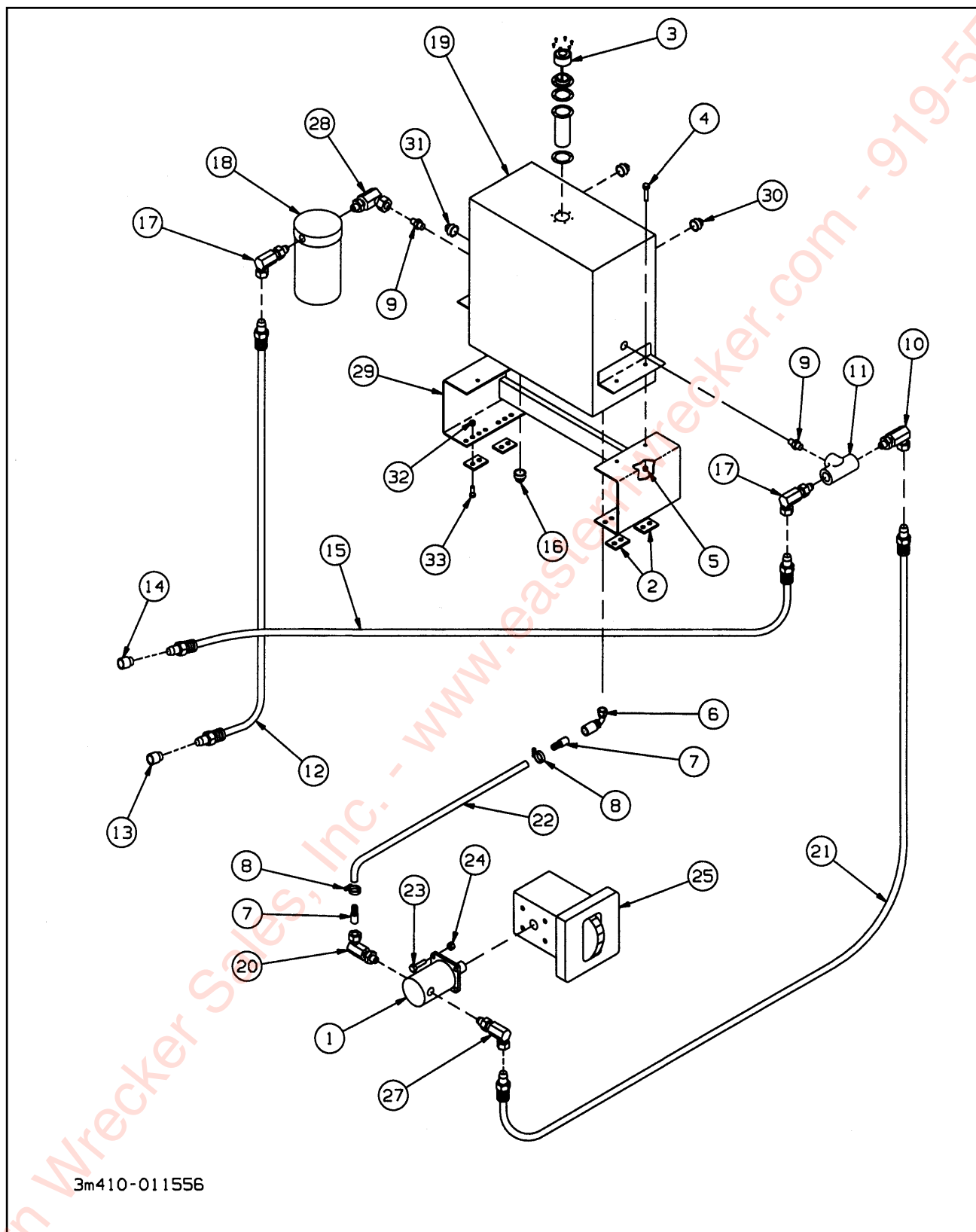
Figure 1-13 Transmission Mounted Wet Kit Items
