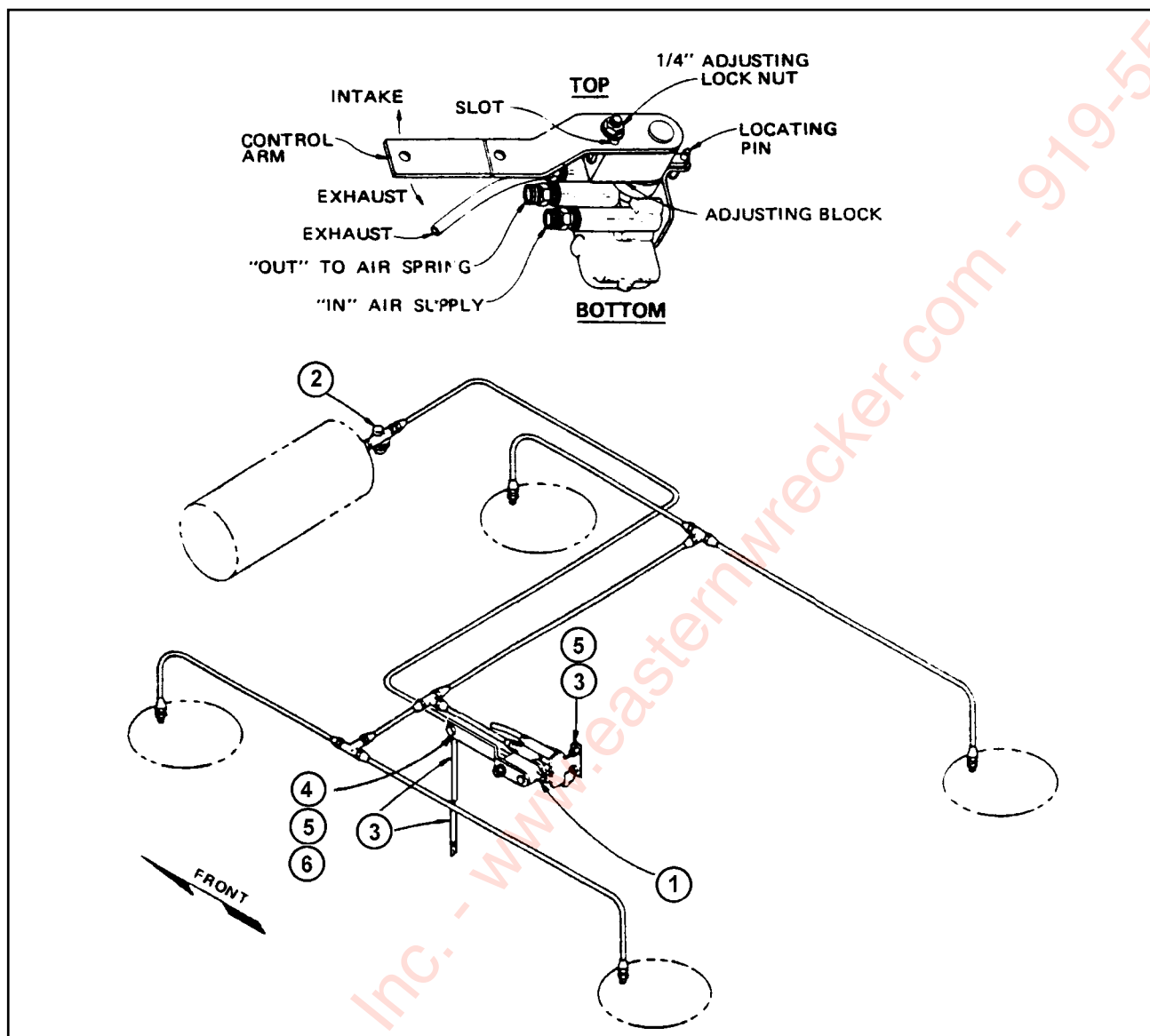
Figure 1-21 Air Control Kit
