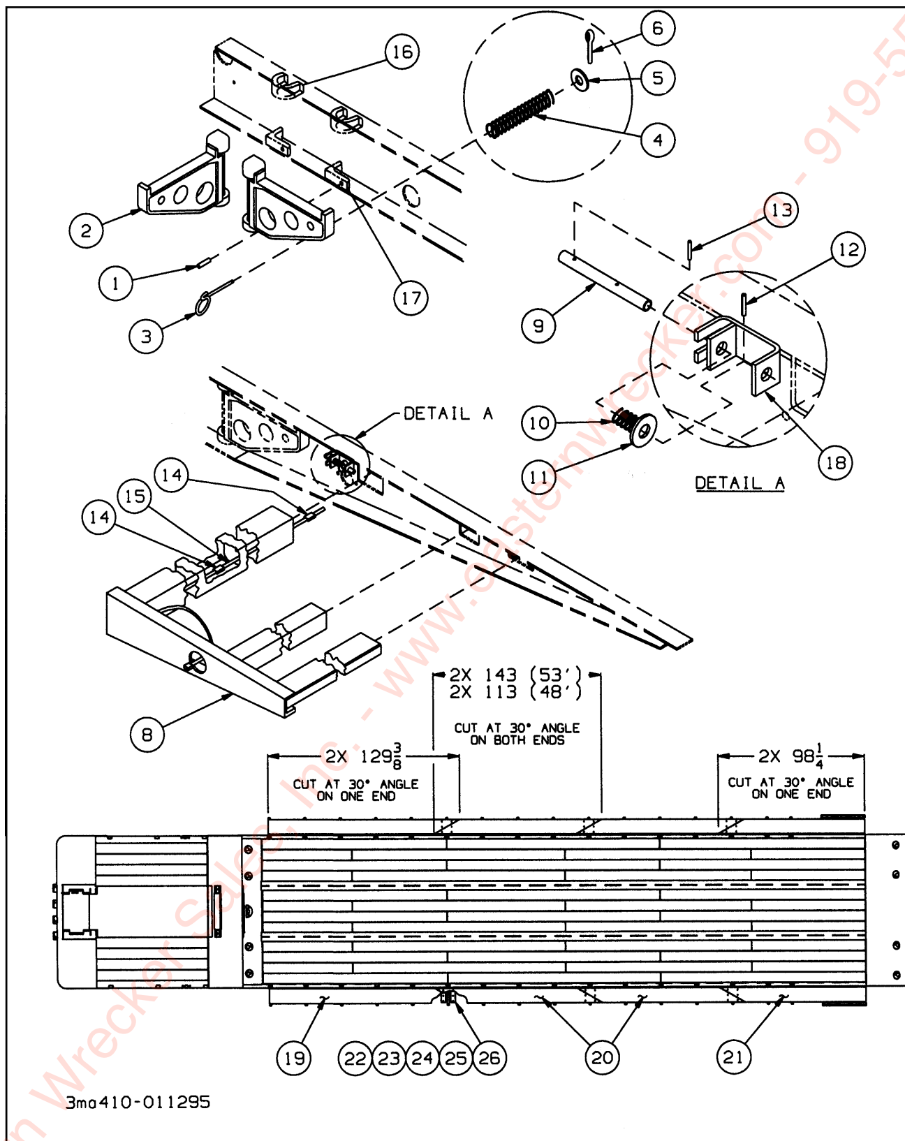
Figure 1-5 Outrigger Installation
