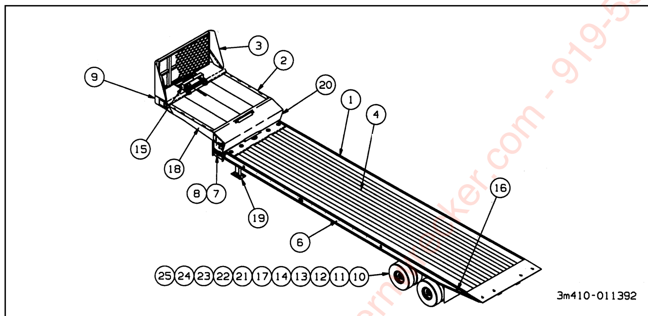
Figure 1-1 General Assembly
