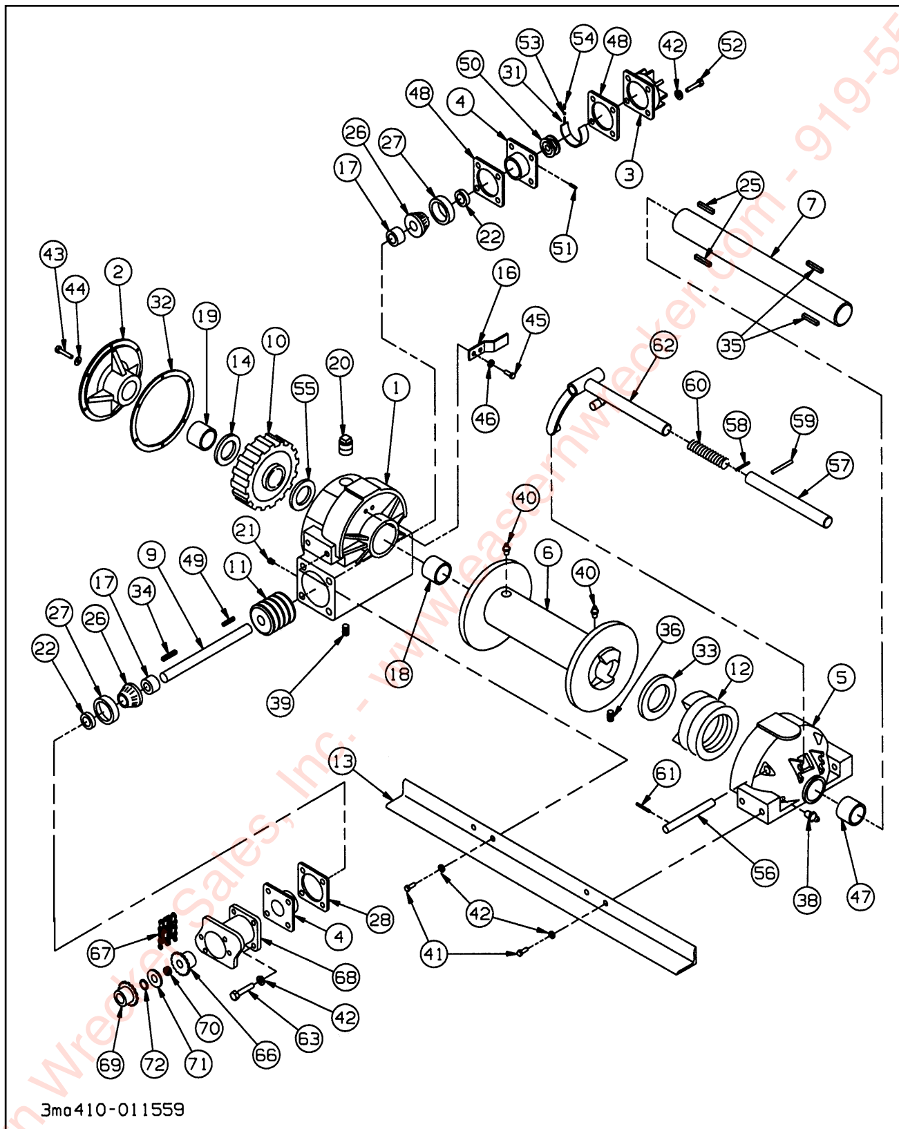
Figure 1-35 12,000# Winch Items
