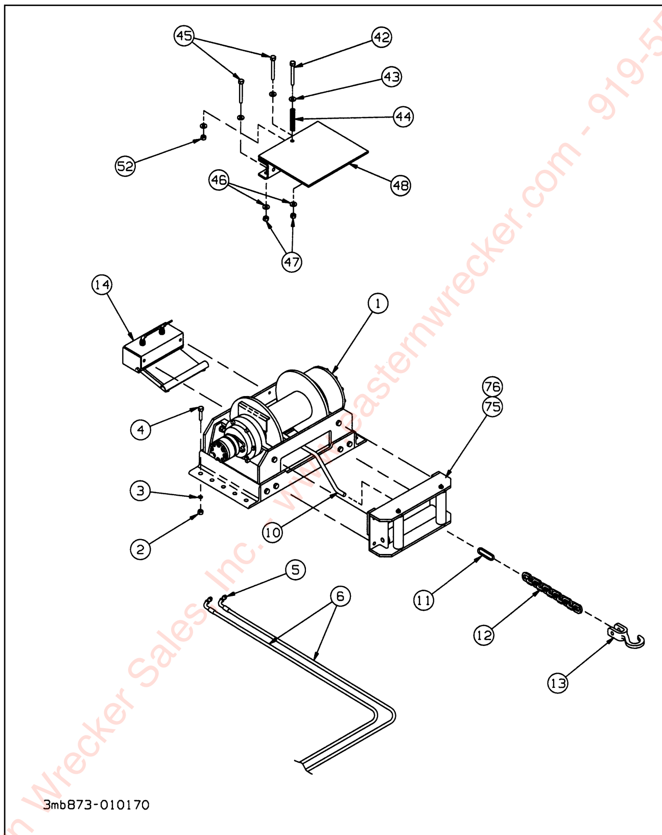
Figure 1-39 30K Upper Deck Winch Installation (1 of 2)
