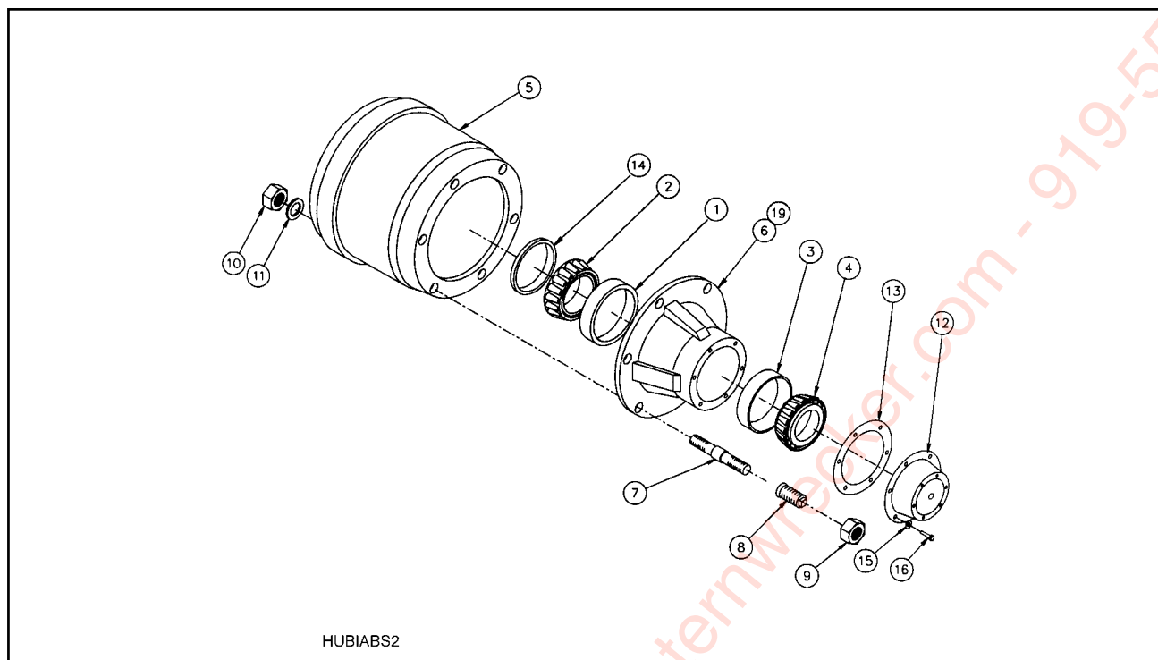
Figure 1-30 Inboard Ball Seat Mount Hub and Drum
