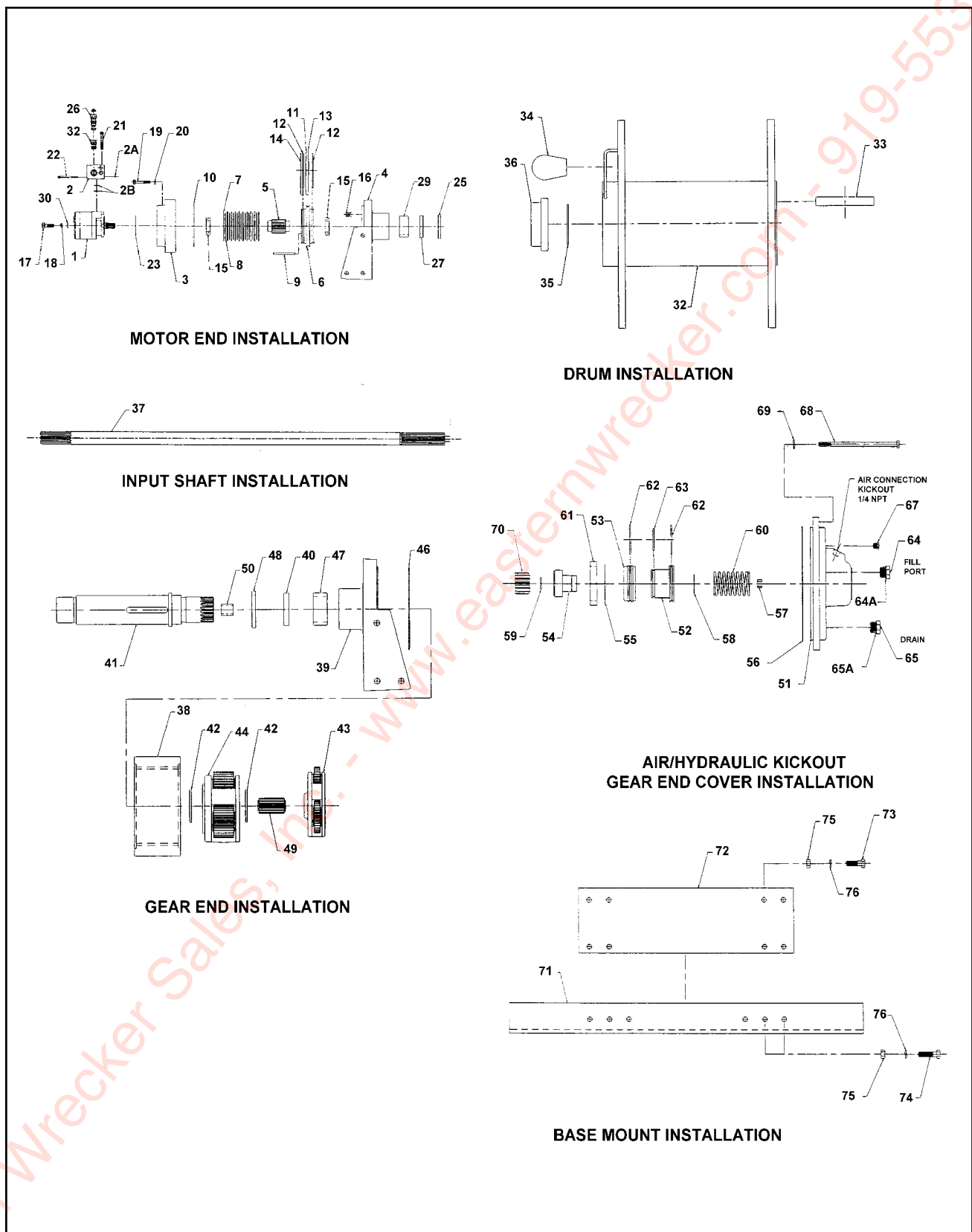
Figure 1-41 30,000# Winch Items
