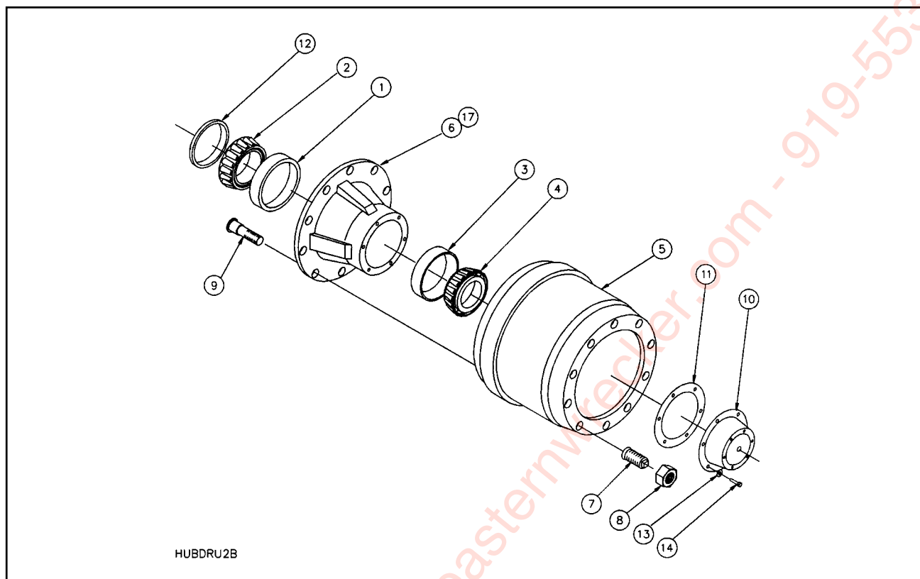
Figure 1-31 Outboard Ball Seat Mount Hub and Drum
