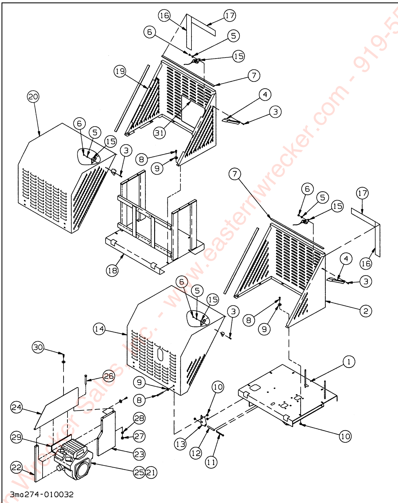
Figure 1-61 Engine Cover, Split Mount
