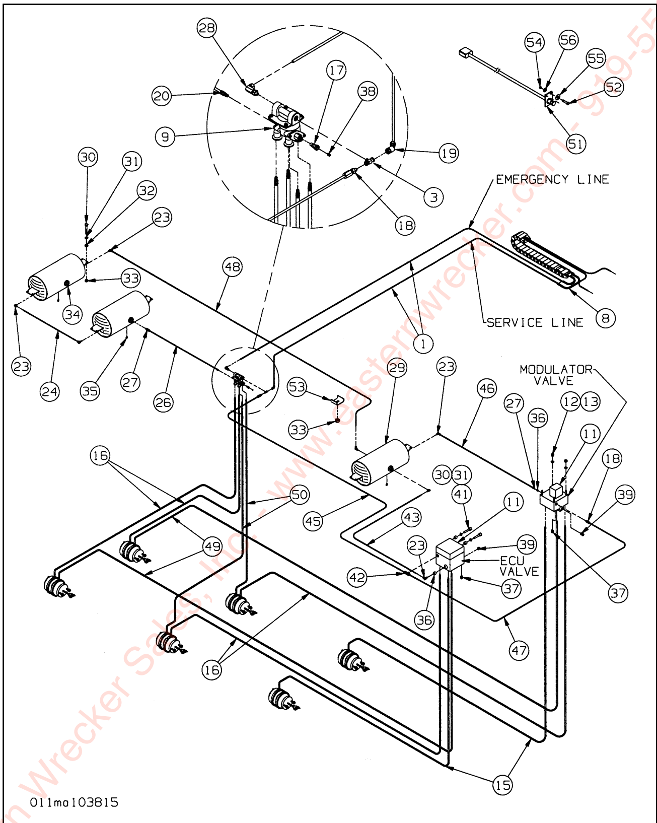
Figure 1-26 Spring Air Brake System w/ ABS, Triple
