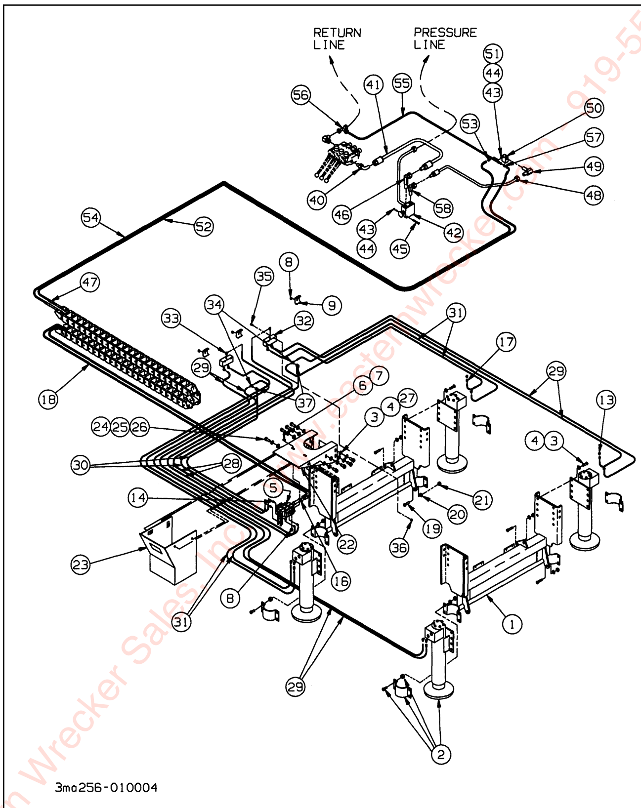
Figure 1-49 Dock Leveler, Optional Double Cylinder
