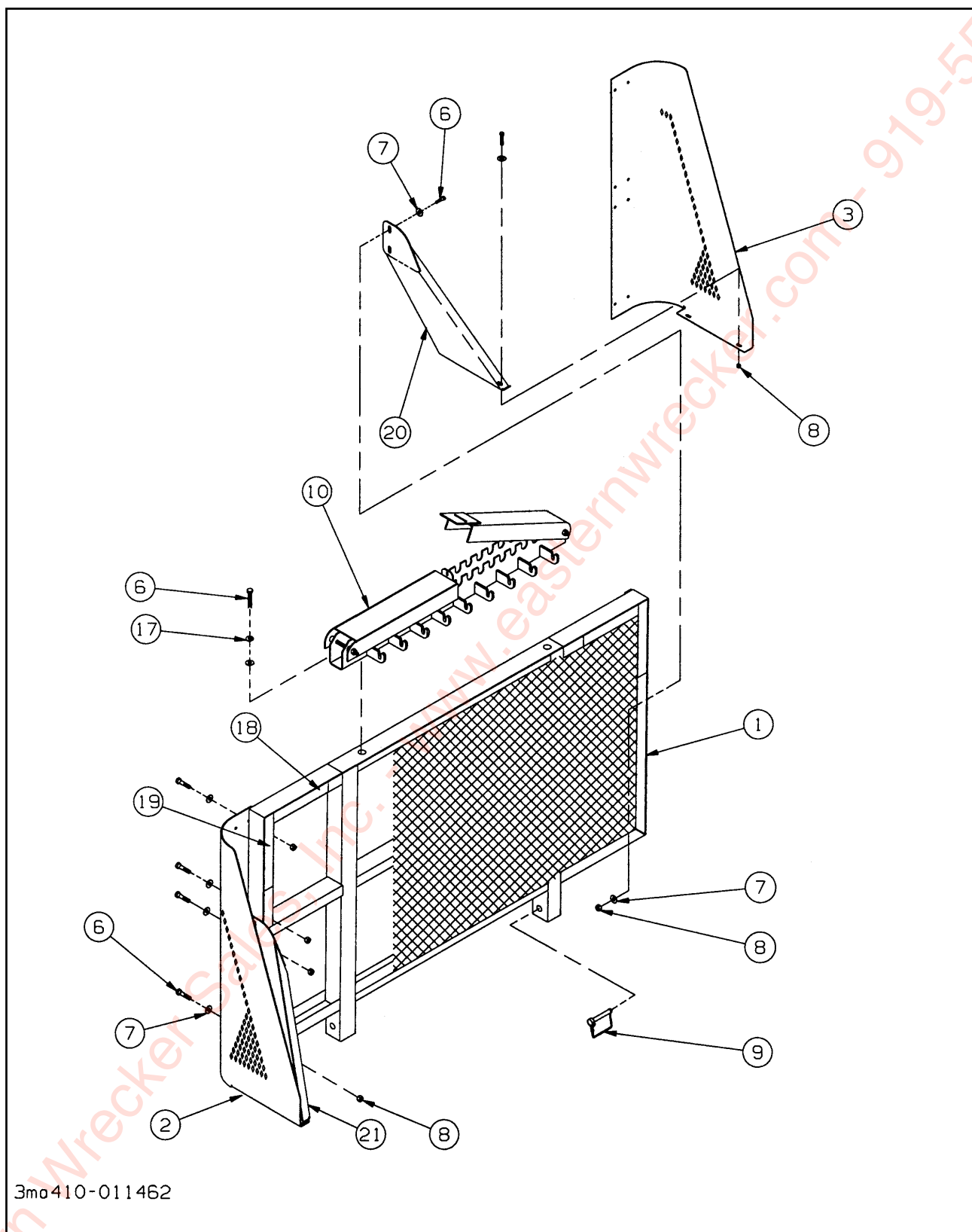
Figure 1-3 Bulkhead Assembly
