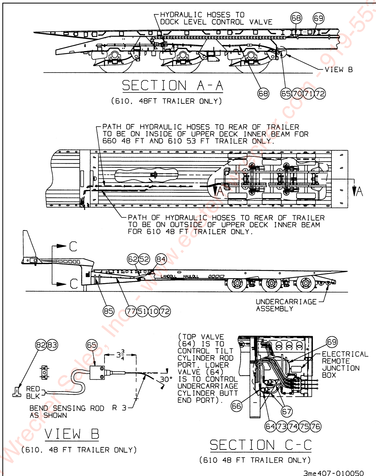
Figure 1-8 Hydraulic System (2 of 2)
