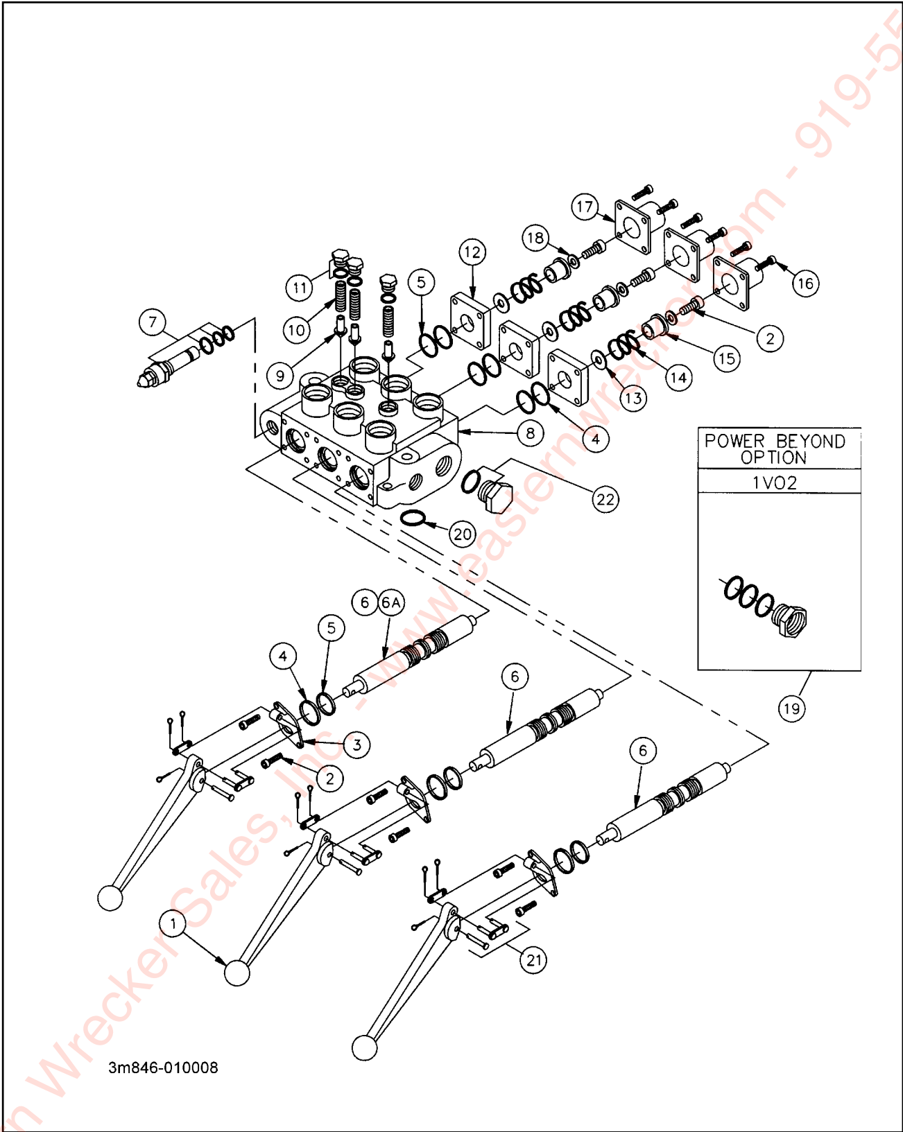
Figure 1-14 Three Spool Valve
