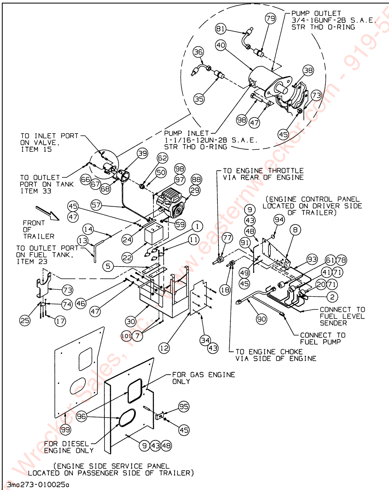
Figure 1-57 Hydraulic Engine, Standard Mount (1 of 2)
