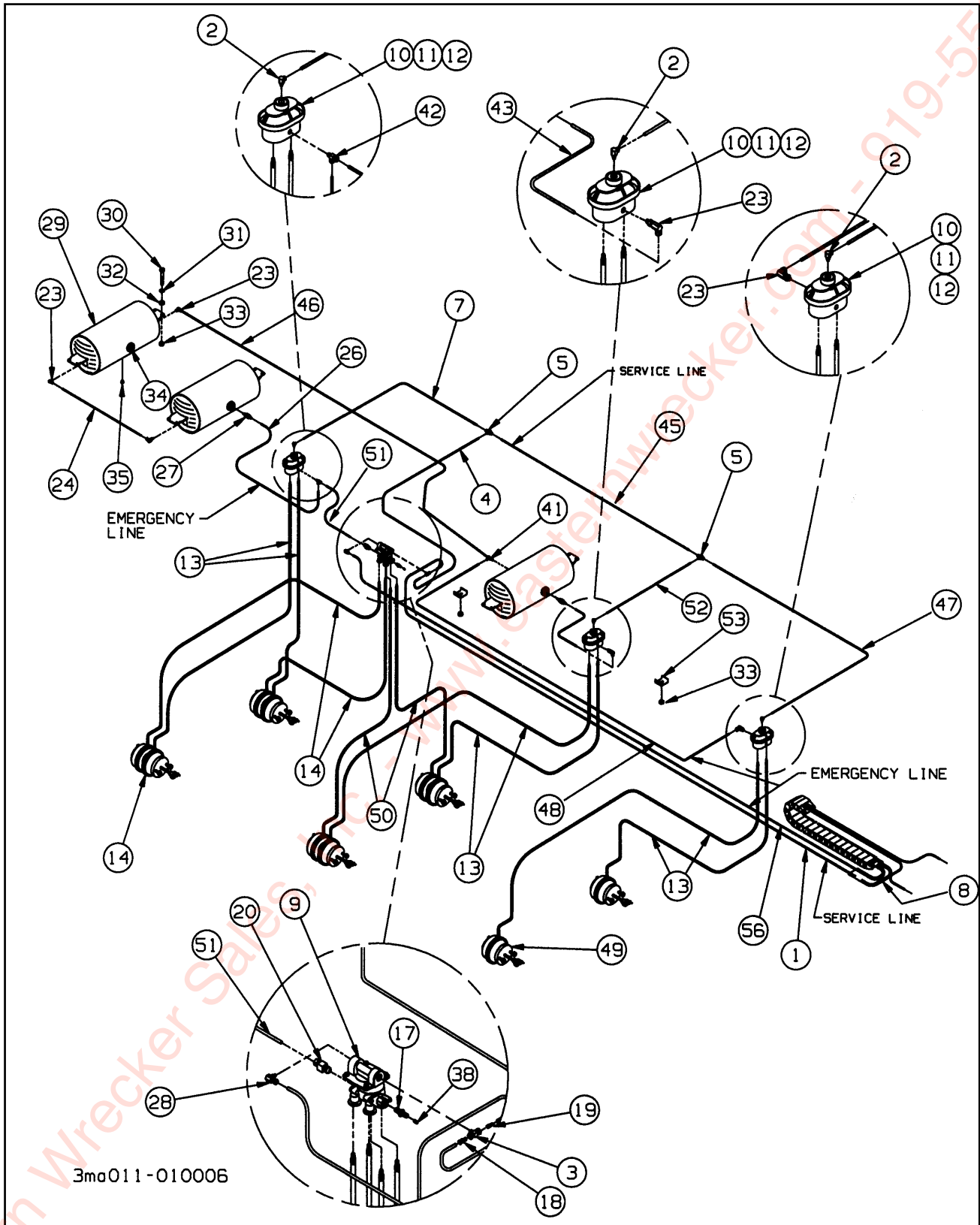
Figure 1-27 Spring Air Brake System w/o ABS, Triple
