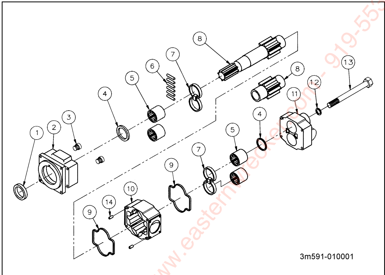
Figure 1-12 Pump, Wet Kit Hydraulic
