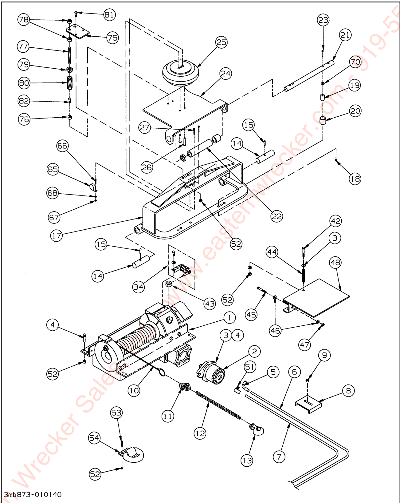
Figure 1-33 Winch Installation (1 of 2)
