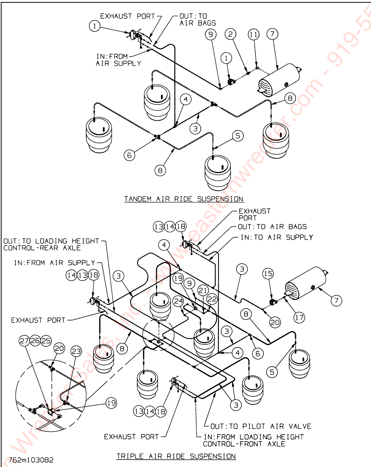
Figure 1-20 Air Ride Suspension, Air System
