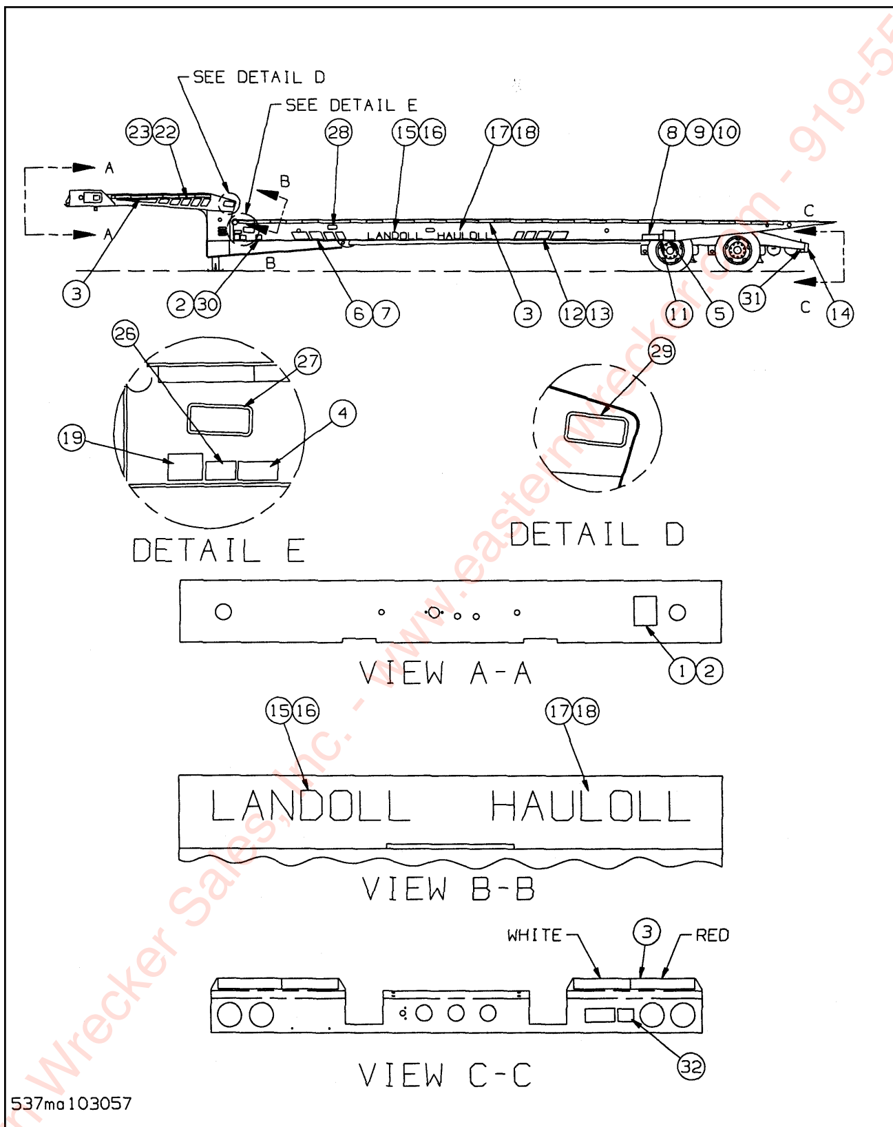
Figure 1-53 Decal Placement
