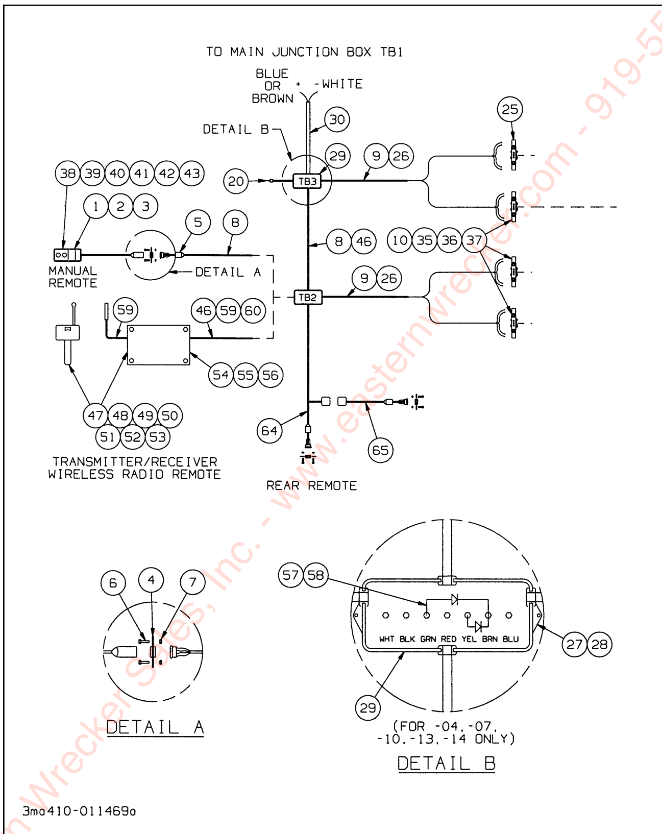
Figure 1-44 Remote Control Items (1 of 2)
