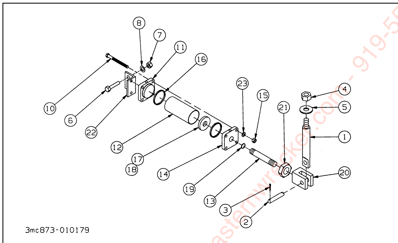
Figure 1-37 Winch Air Shift Cylinder for 20,000# Winch
