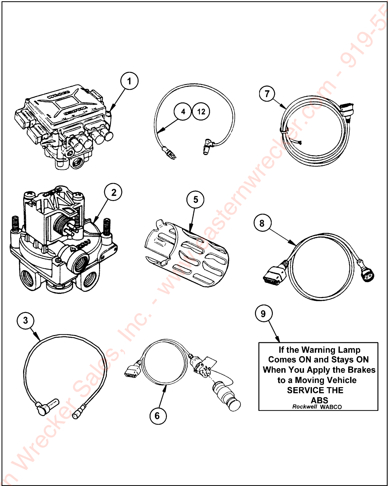
Figure 1-29 Brake Kit, Rockwell ABS
