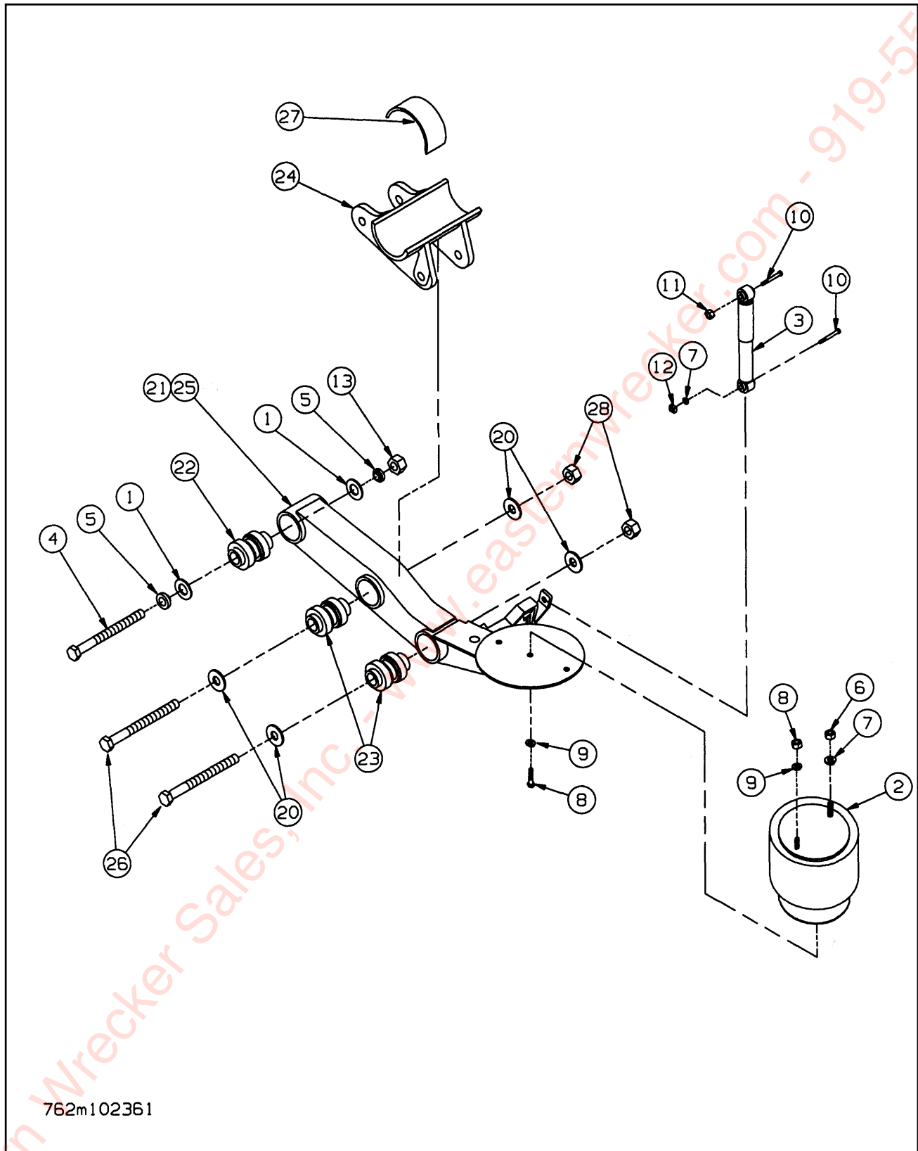
Figure 1-23 Suspension Hanger RLU-228
