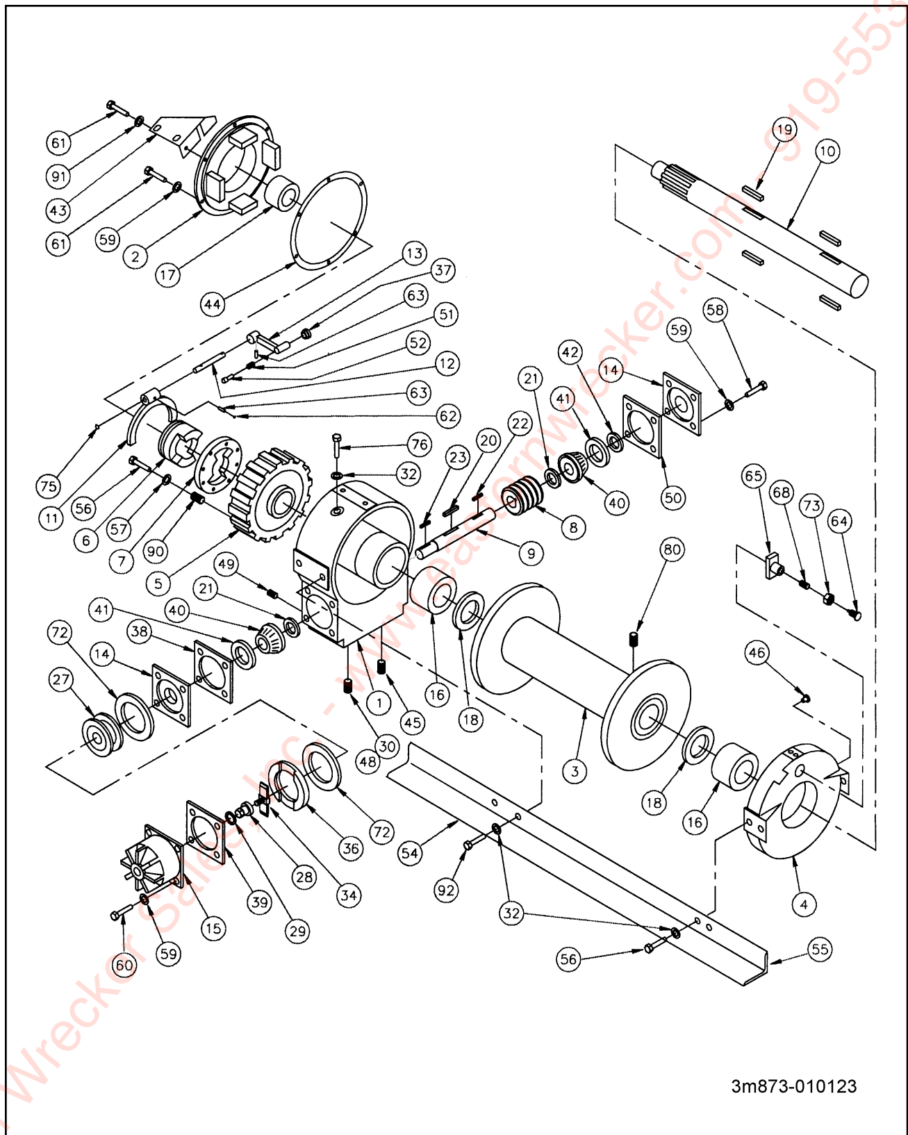
Figure 1-36 20,000# Winch Items
