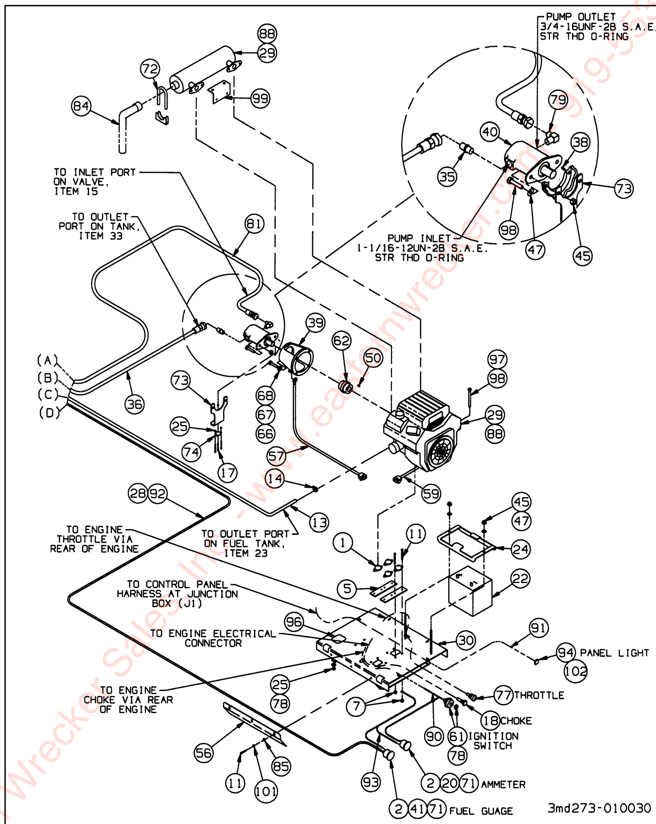
Figure 1-60 Hydraulic Engine, Split Mount (2 of 2)
