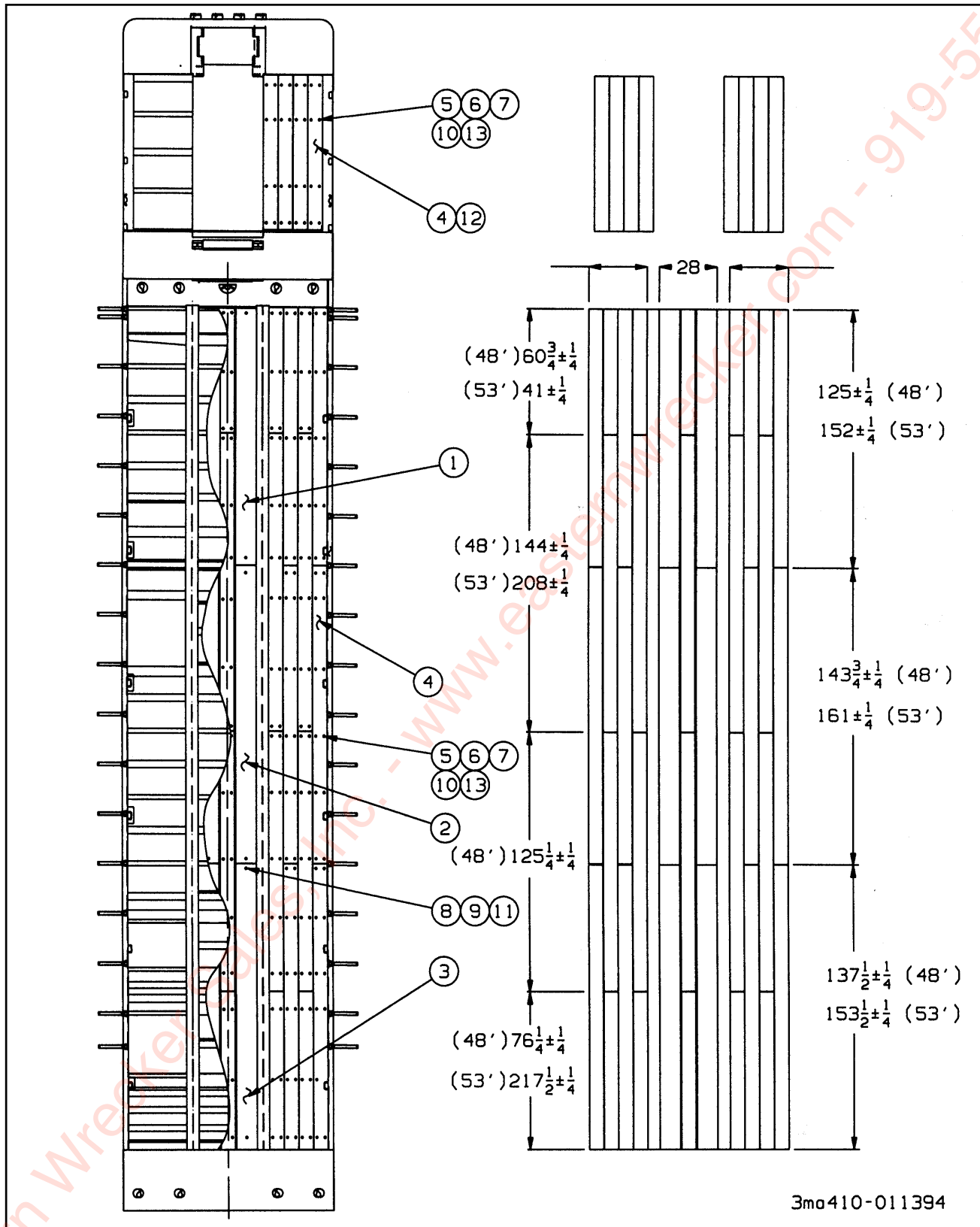
Figure 1-4 Floor Assembly
