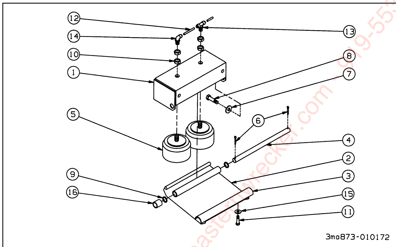
Figure 1-43 Winch, Cable Air Tension
