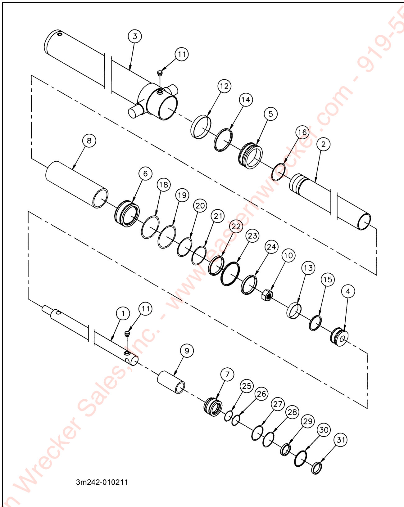
Figure 1-10 Cylinder, Telescopic 212
