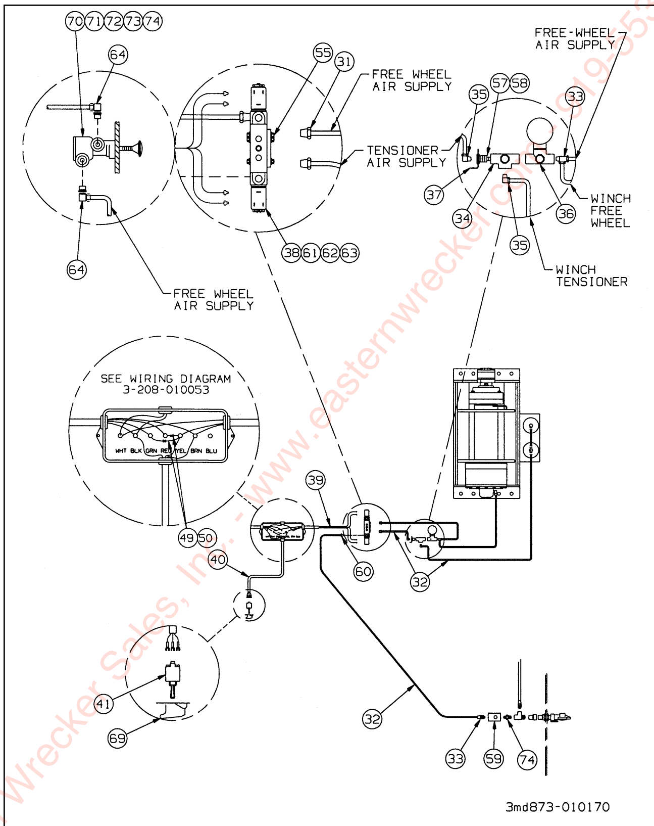
Figure 1-40 30K Upper Deck Winch Installation (2 of 2)
