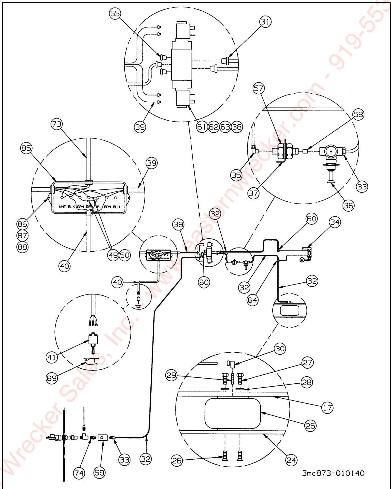
Figure 1-34 Winch Installation (2 of 2)
