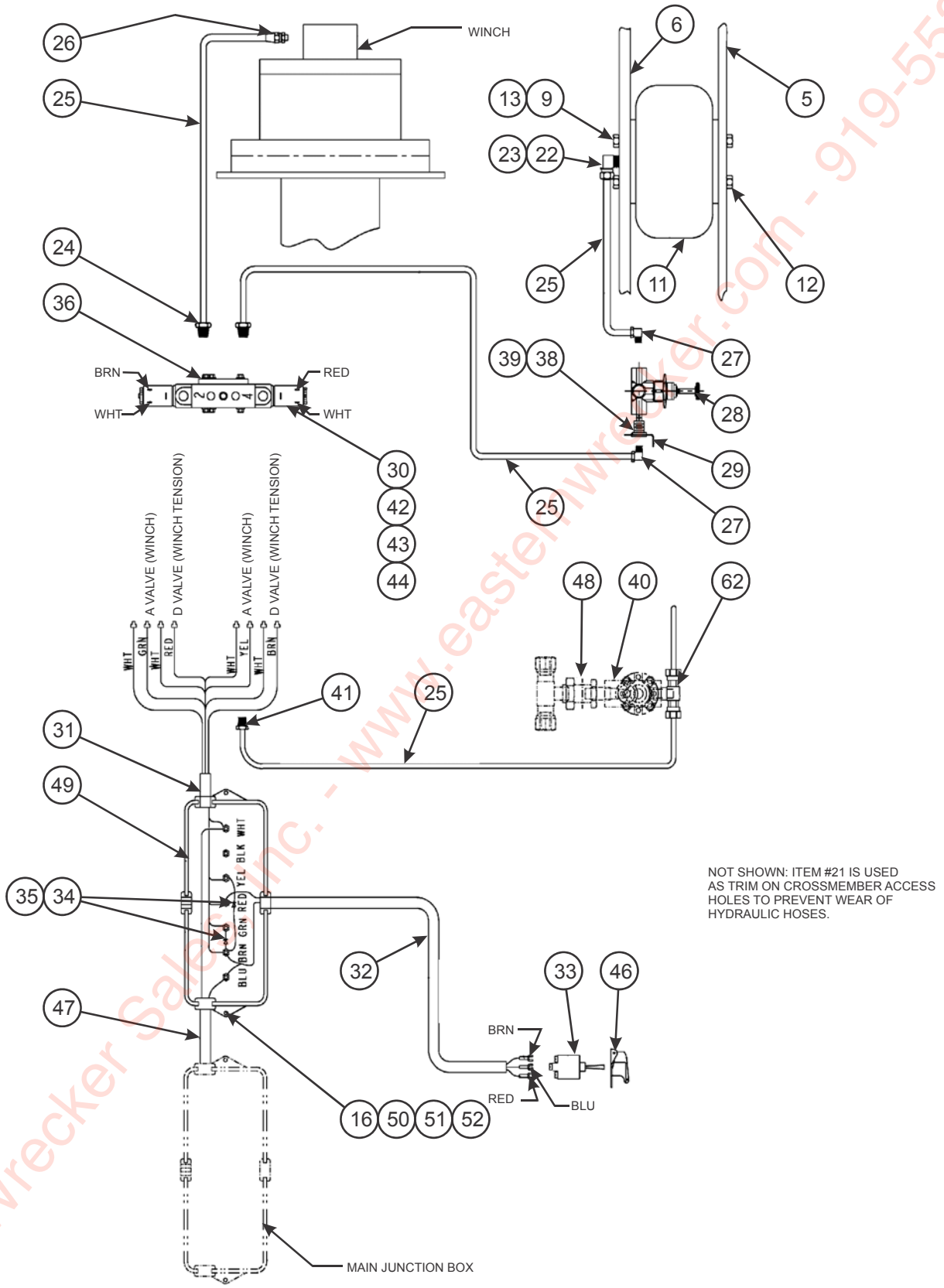
Figure 2-46: 12K, 15K, & 20K Upper Deck Winch (DP) (2 of 2)
