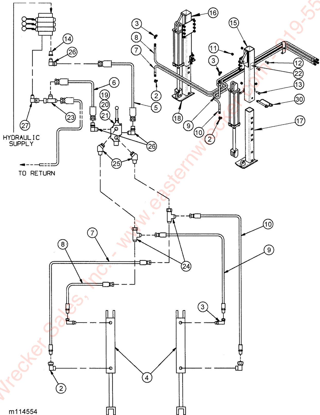
Figure 2-60: Hydraulic Landing Gear Installation
