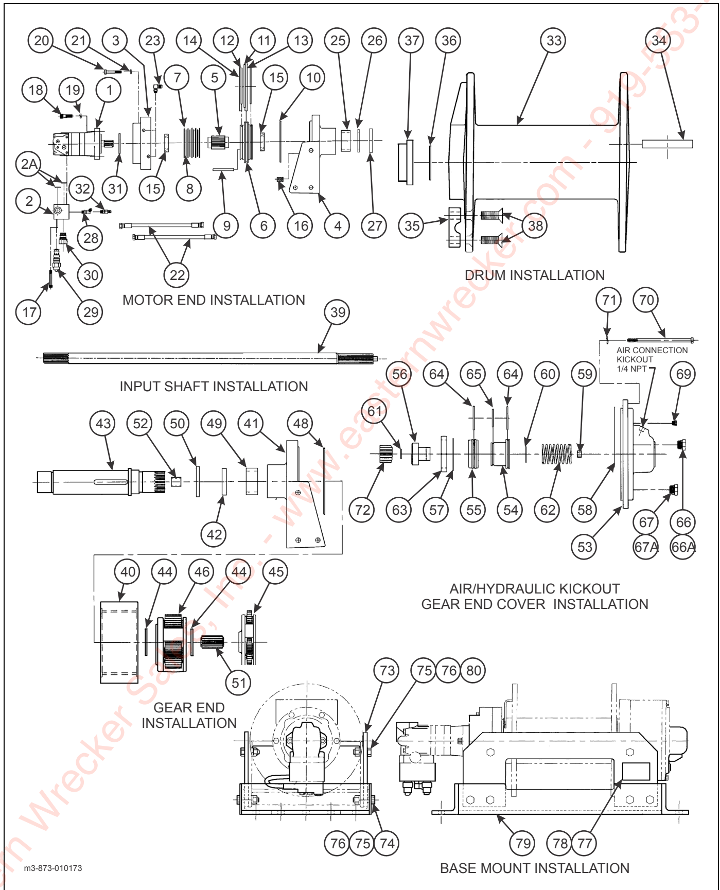
Figure 2-42: 30,000 Lb. Winch Items
