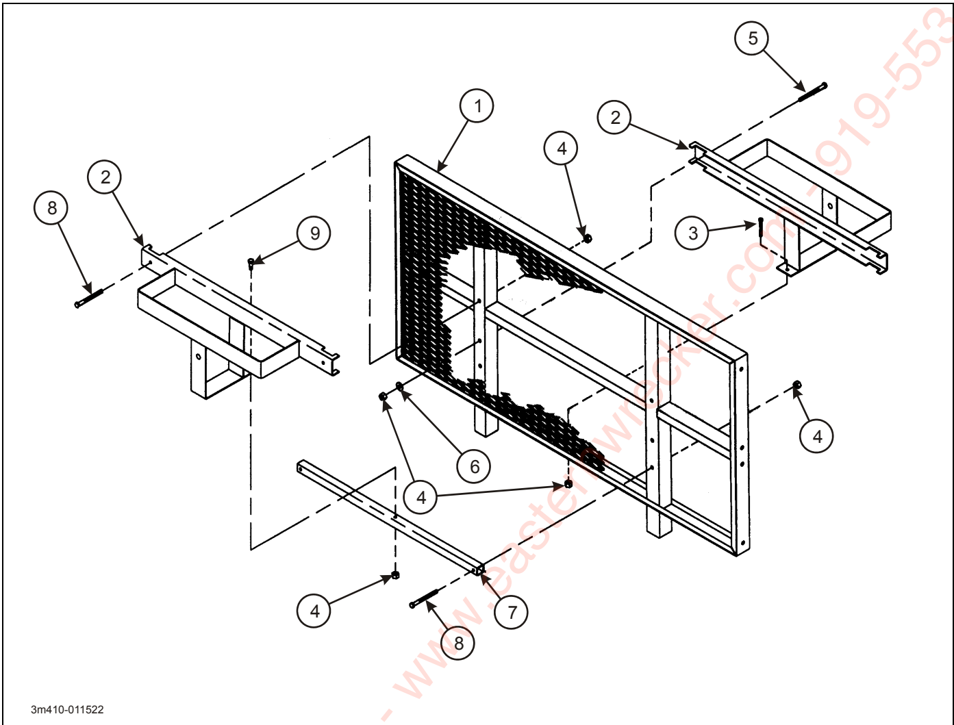
Figure 2-73: Spare Tire Carrier (Option)
