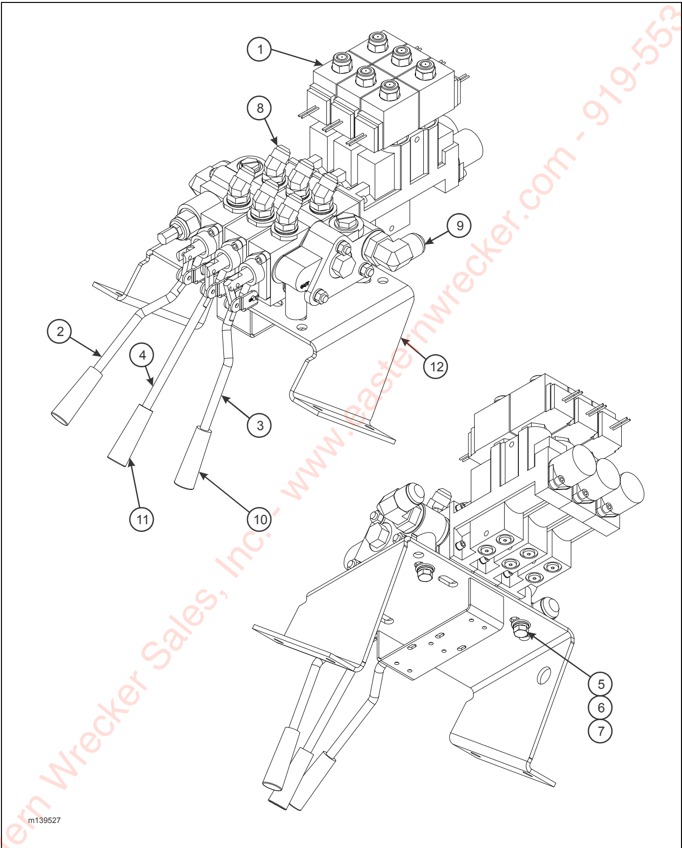
Figure 2-13: Three Spool Valve Assembly (Prior 01/10/2008)
