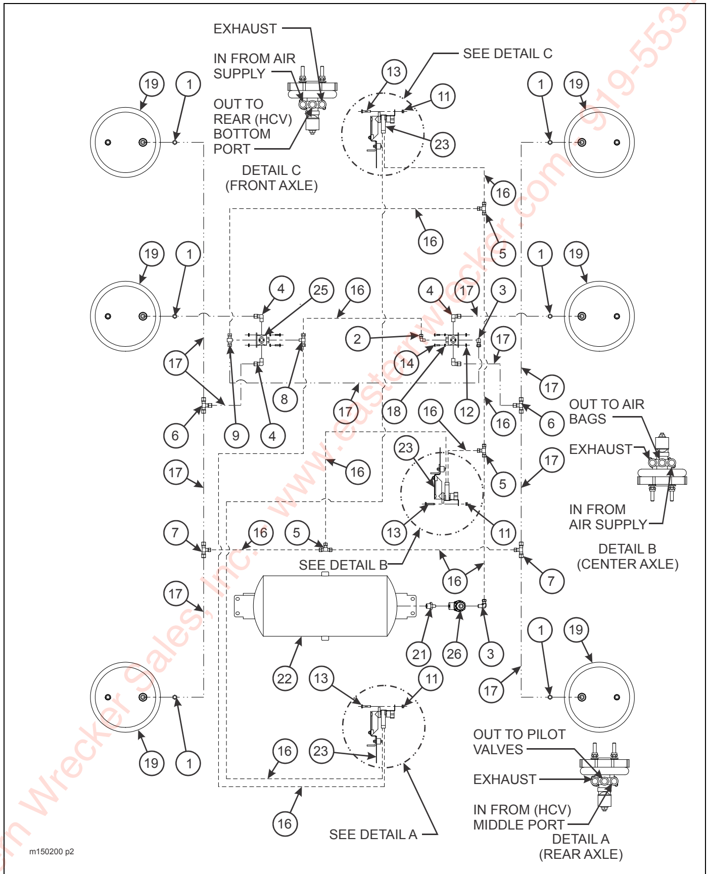
Figure 2-23: Air Ride Suspension, Air System (Triple)
