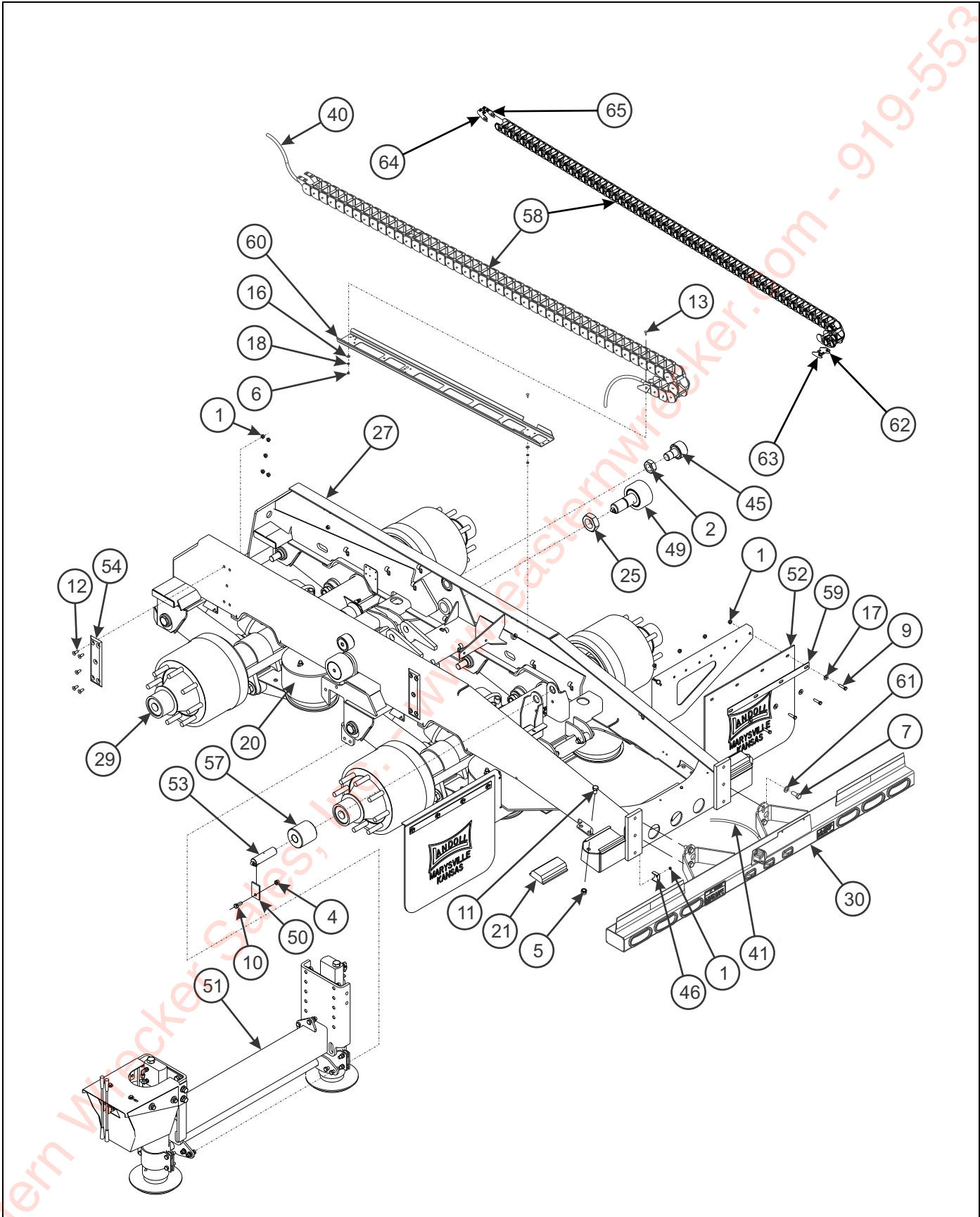
Figure 2-18: U/C Assembly, Air Ride Suspension (Tandem Axle) (1 of 2)
