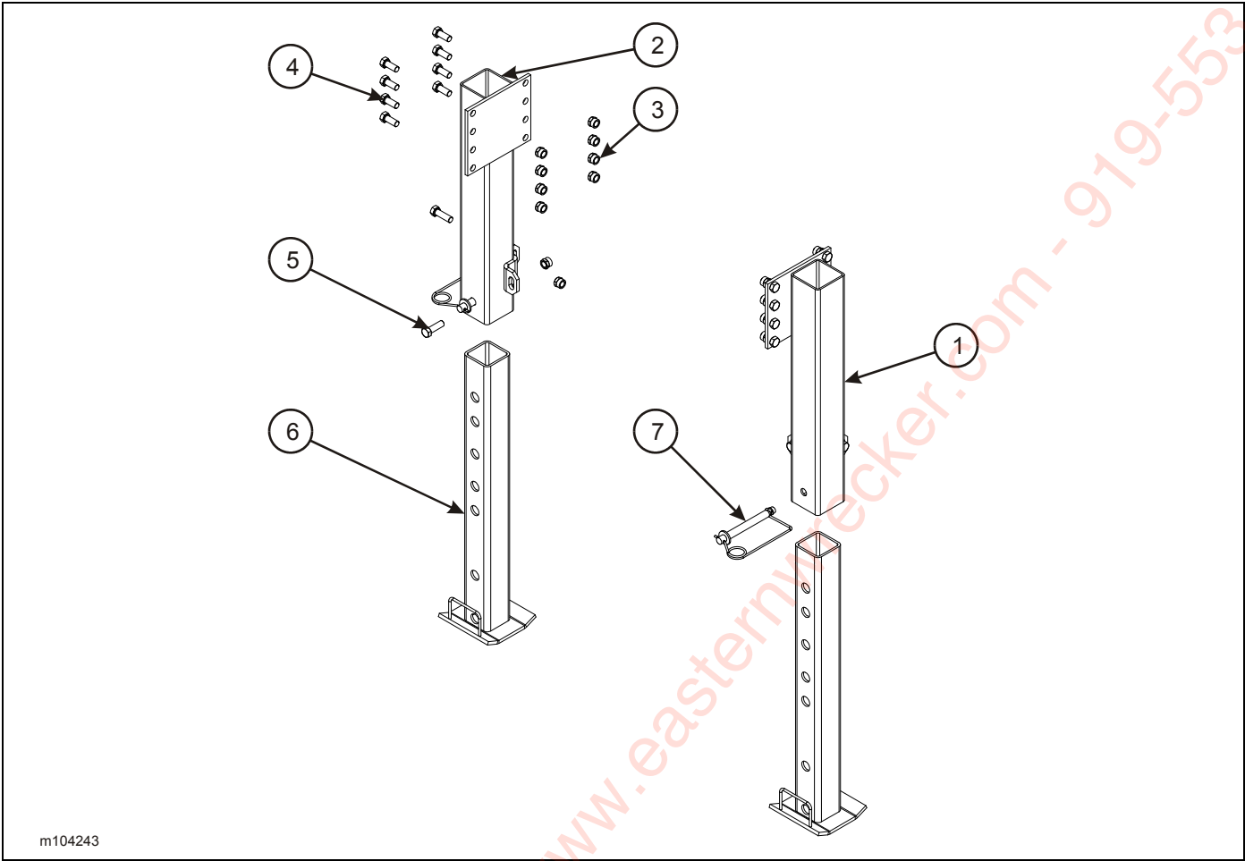
Figure 2-59: Landing Gear Installation
