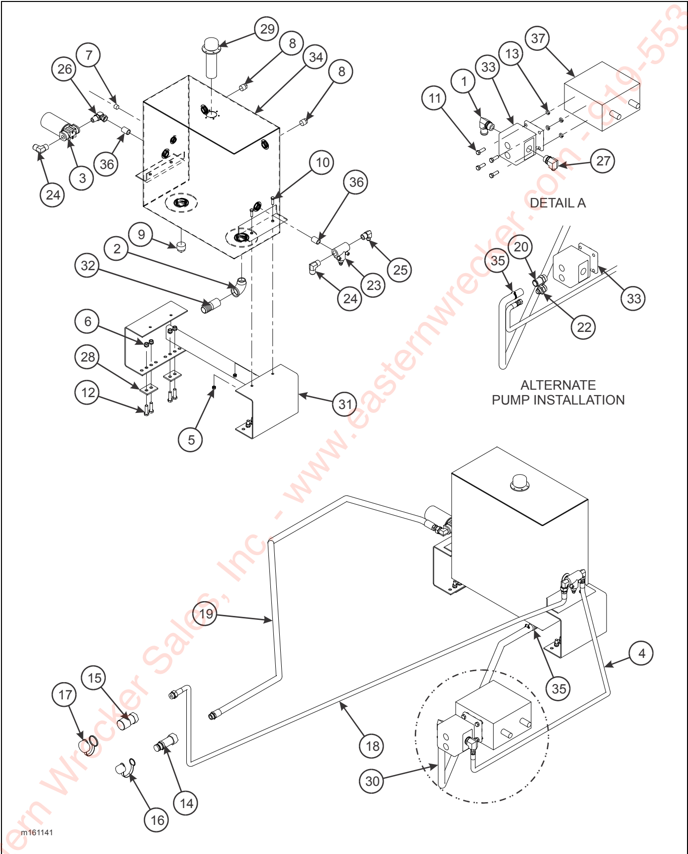
Figure 2-12: 30 Gallon Hydraulic Wet Kit Items
