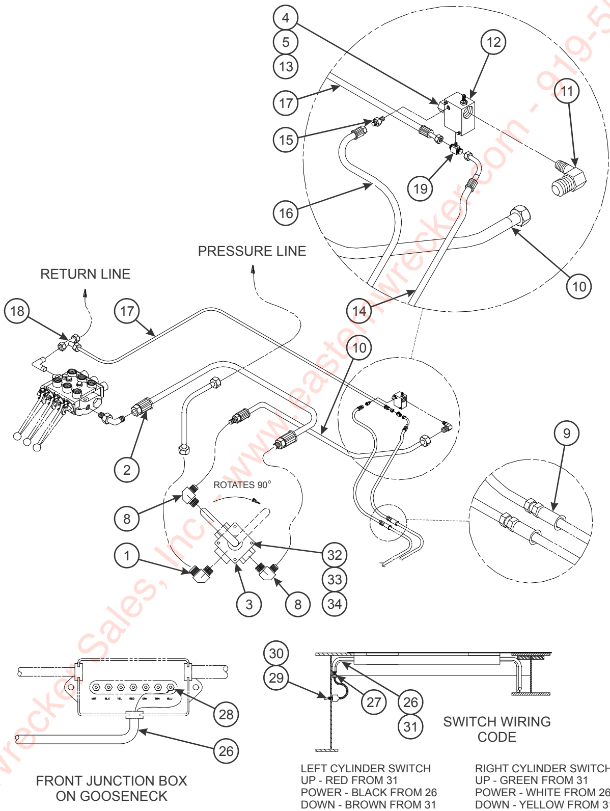
Figure 2-51: Dock Leveler Hydraulic Installation (Option)
