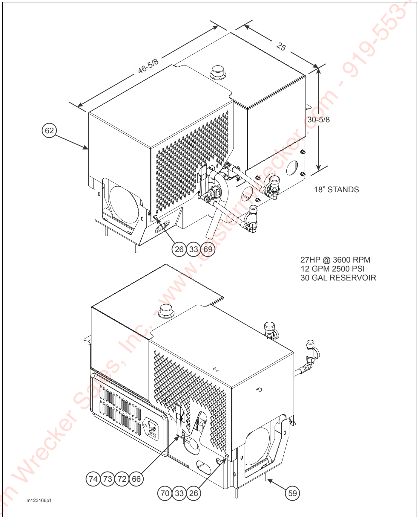
Figure 2-65: Upper Deck Engine Installation (1 of 4)
