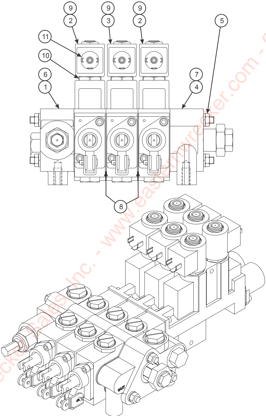
Figure 2-14: Three Spool Valve (Prior 01/10/2008)
