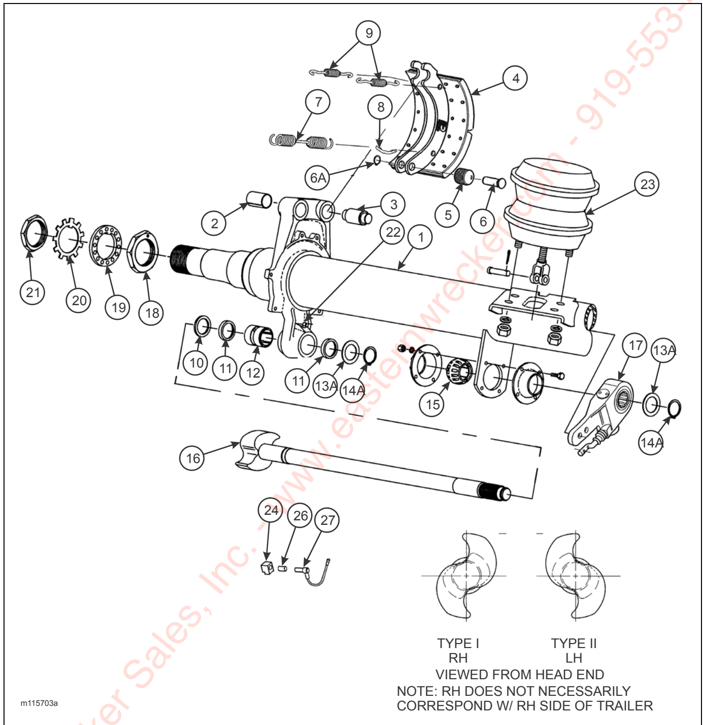
Figure 2-26: Axle and Brake Assembly (12-1/4 x 7-1/2")
