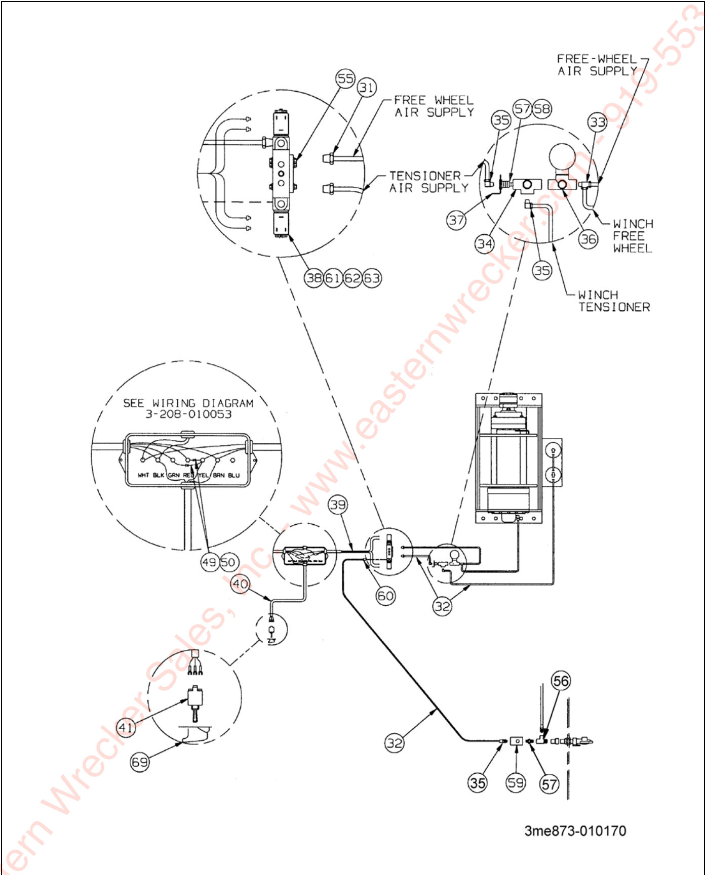
Figure 2-41: 30K Upper Deck Winch Installation (2 of 2)
