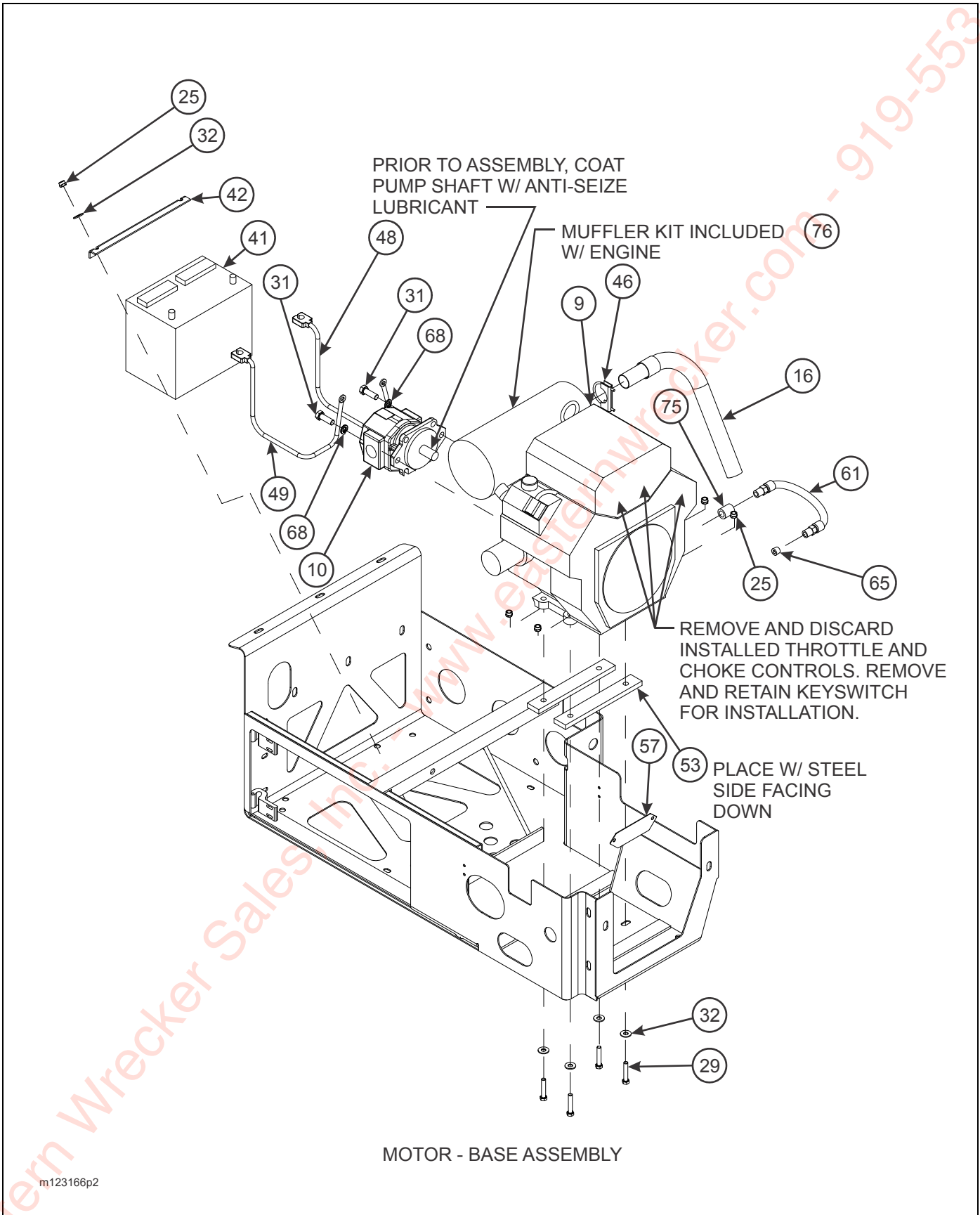
Figure 2-66: Upper Deck Engine Installation (2 of 4)
