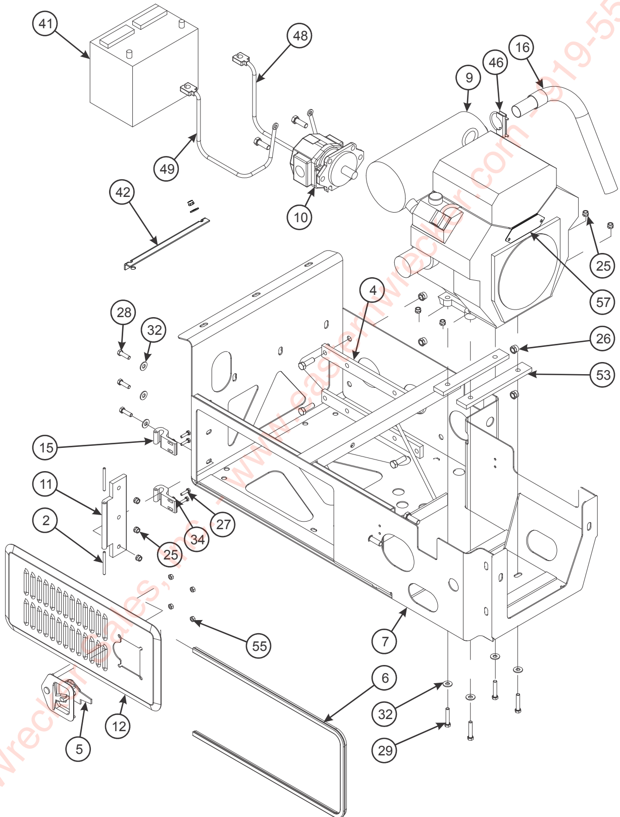
Figure 2-63: 27 HP Gas Engine Installation (1 of 2)
