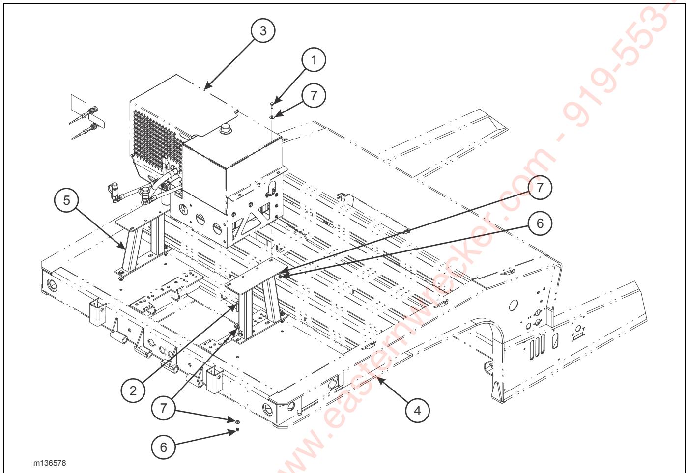
Figure 2-70: Upper Deck Engine Stand Installation
