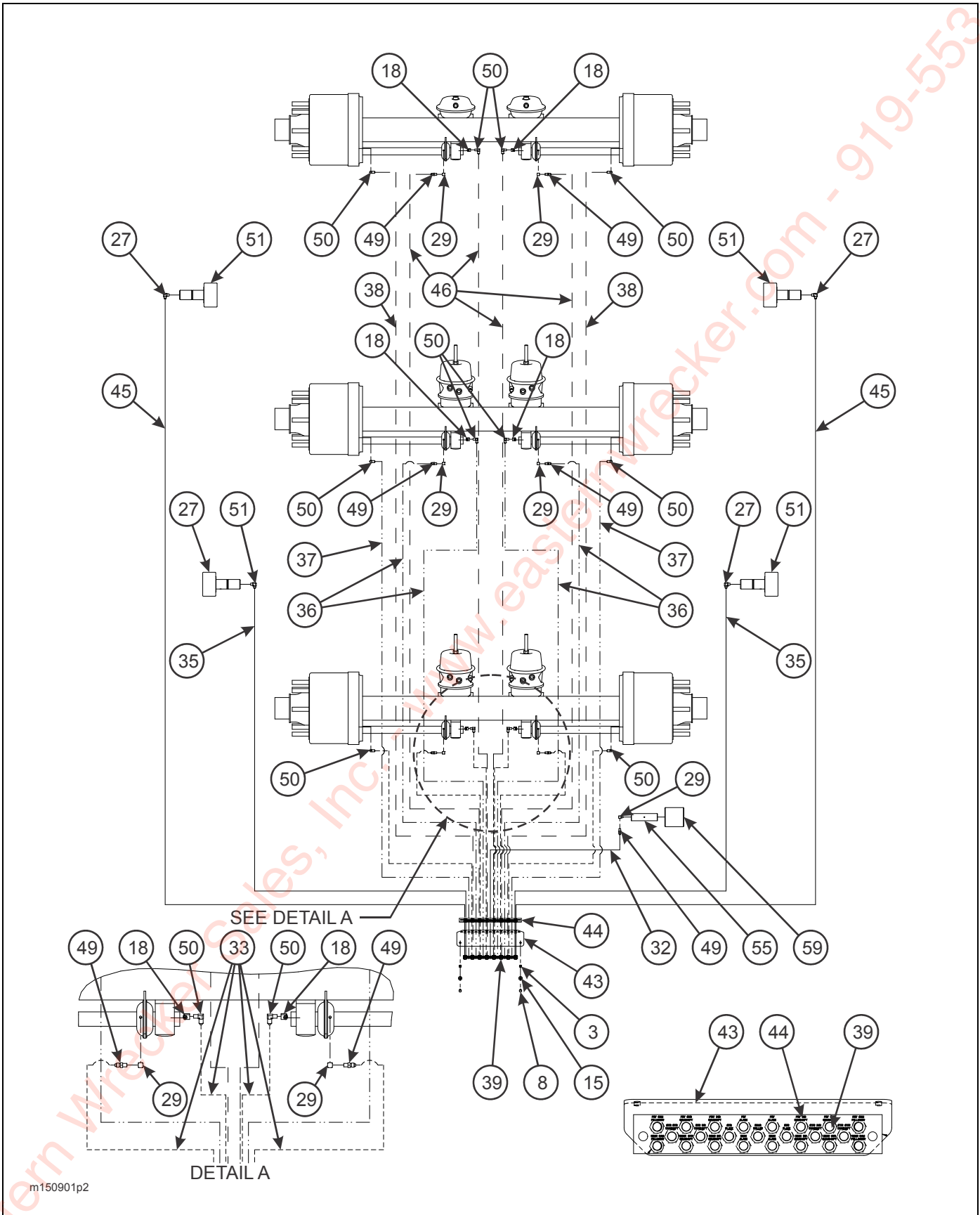
Figure 2-20: U/C Assembly, Air Ride Suspension (Triple Axle) (1 of 2)
