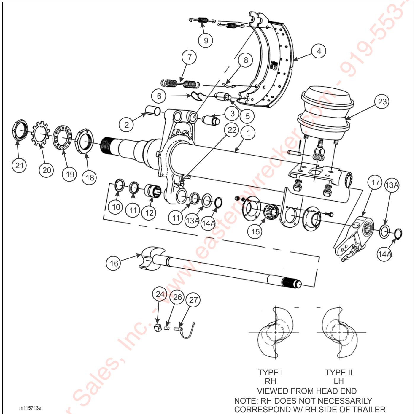
Figure 2-27: Axle and Brake Assembly (16-1/2" x 7")
