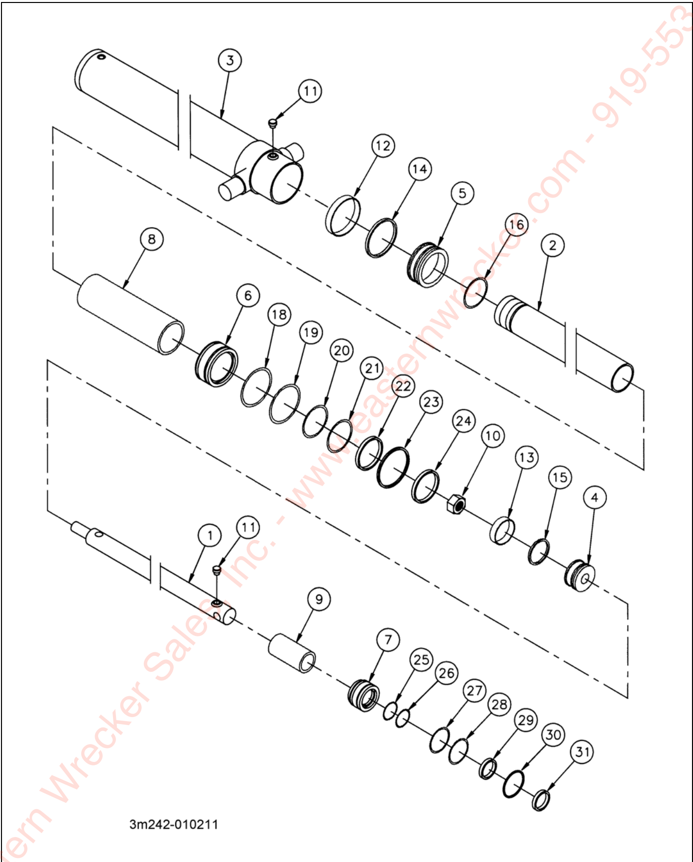
Figure 2-10: Cylinder, Hydraulic 6 x 4 x 212
