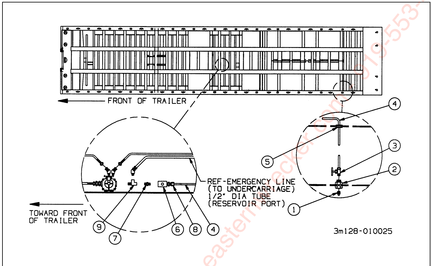
Figure 2-74: Air Outlet Accessory (Option)
