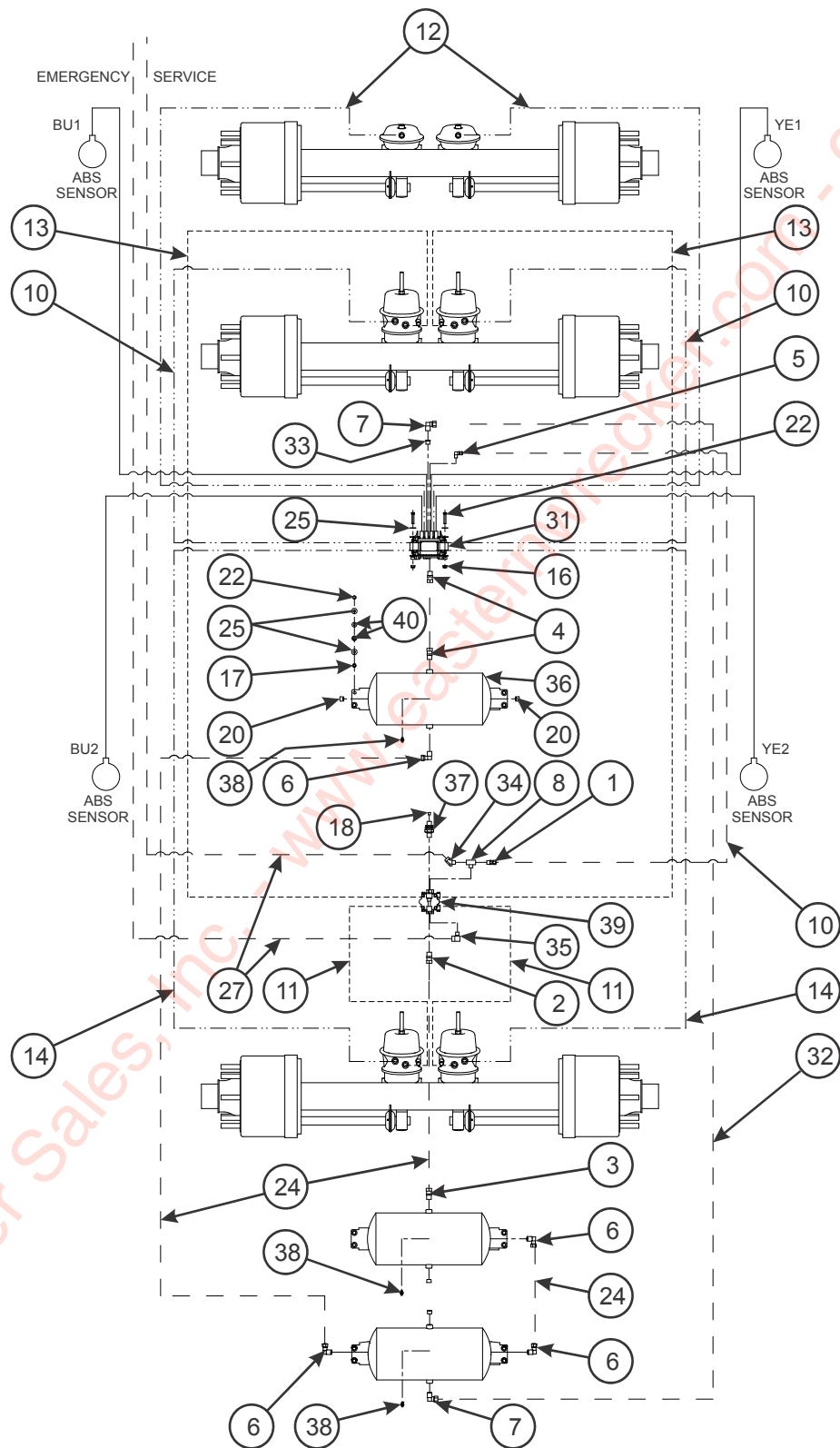
Figure 2-31: Spring Air Brake System w/ ABS (Triple Axle)
