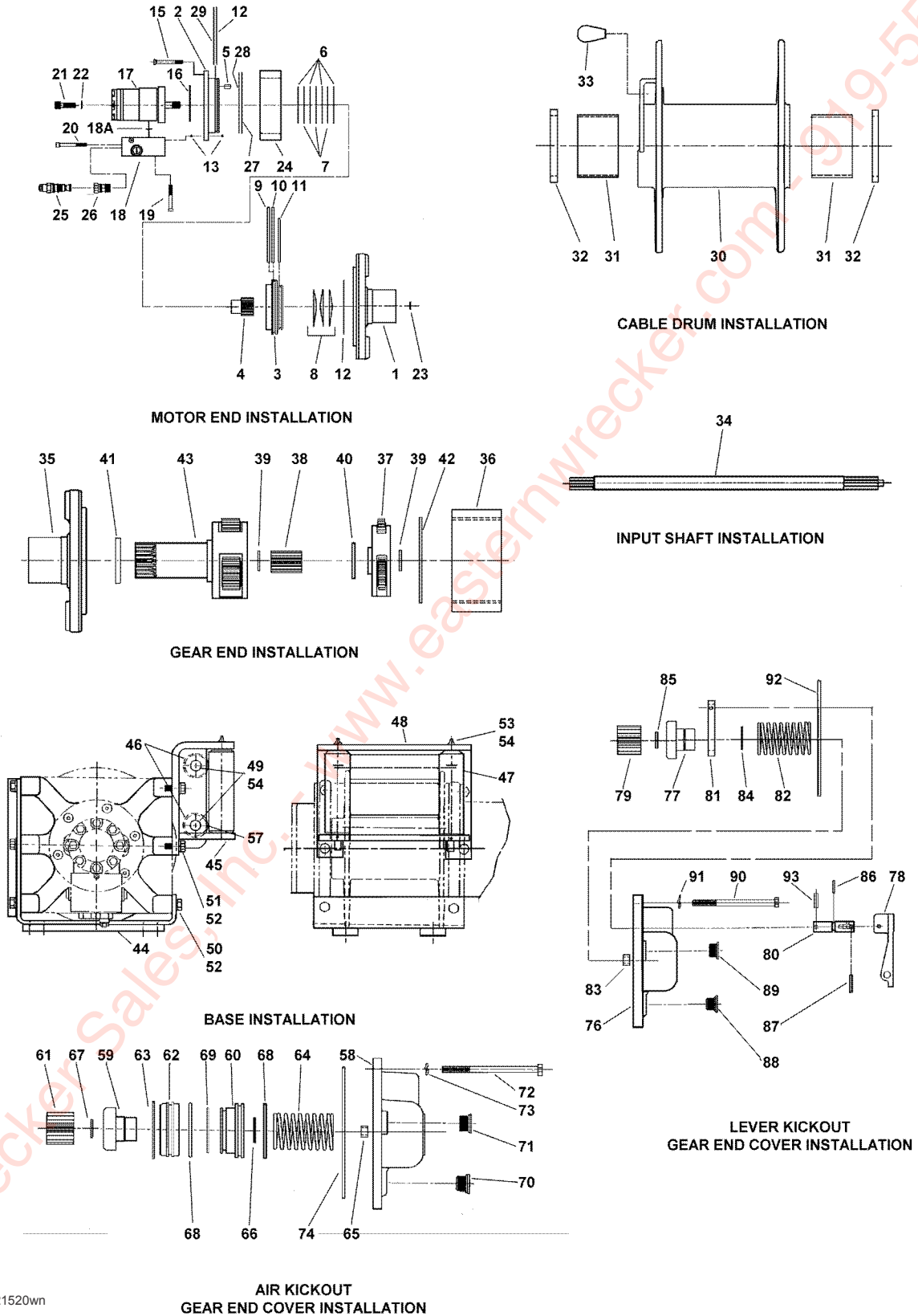
Figure 2-47: 12K, 15K, & 20K Winch Items (DP Planetary)
