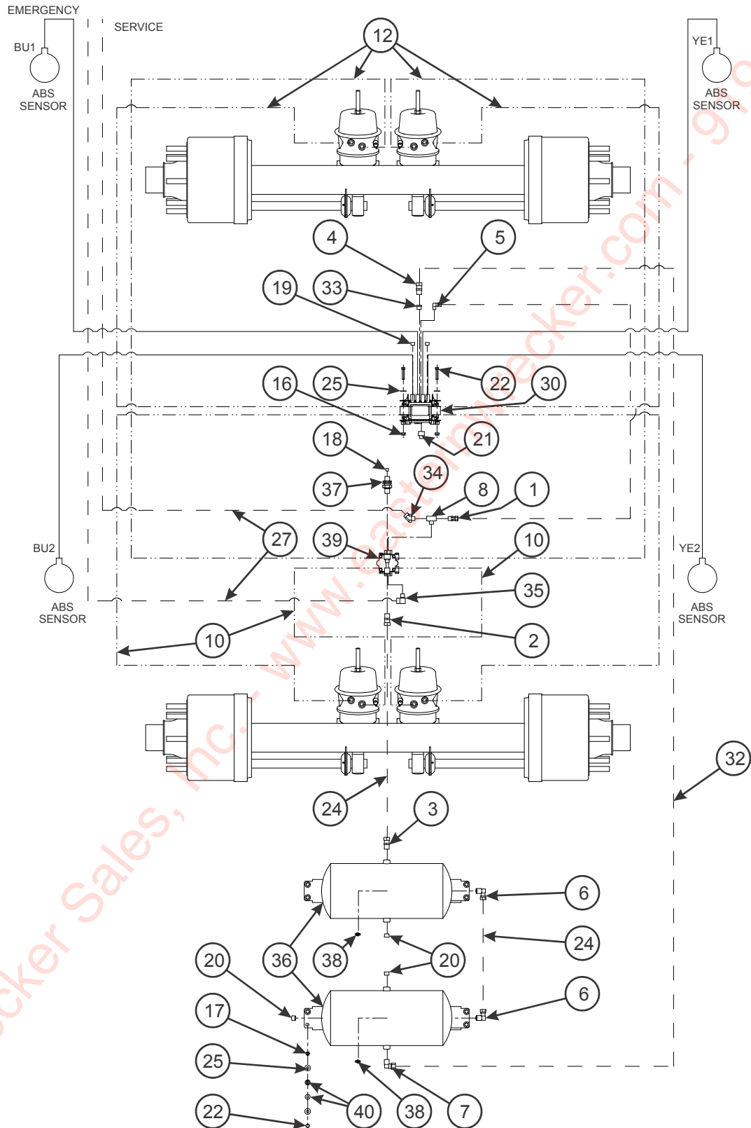
Figure 2-29: Spring Air Brake System w/ ABS (Tandem Axle)
