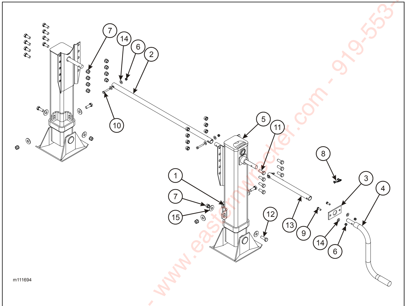
Figure 2-58: Landing Gear Installation
