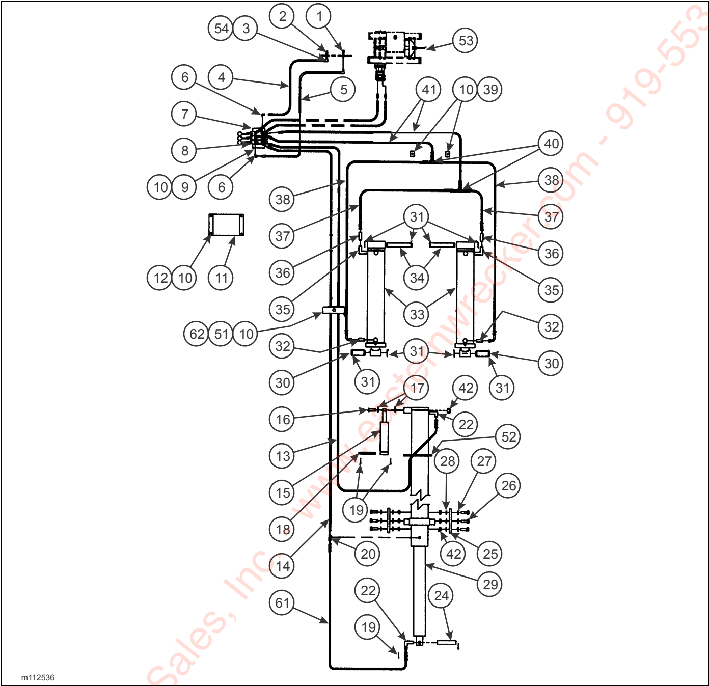
Figure 2-9: Hydraulic System
