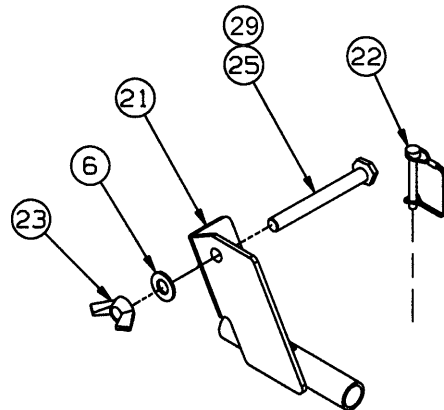
FLAG HOLDER ASSEMBLY
