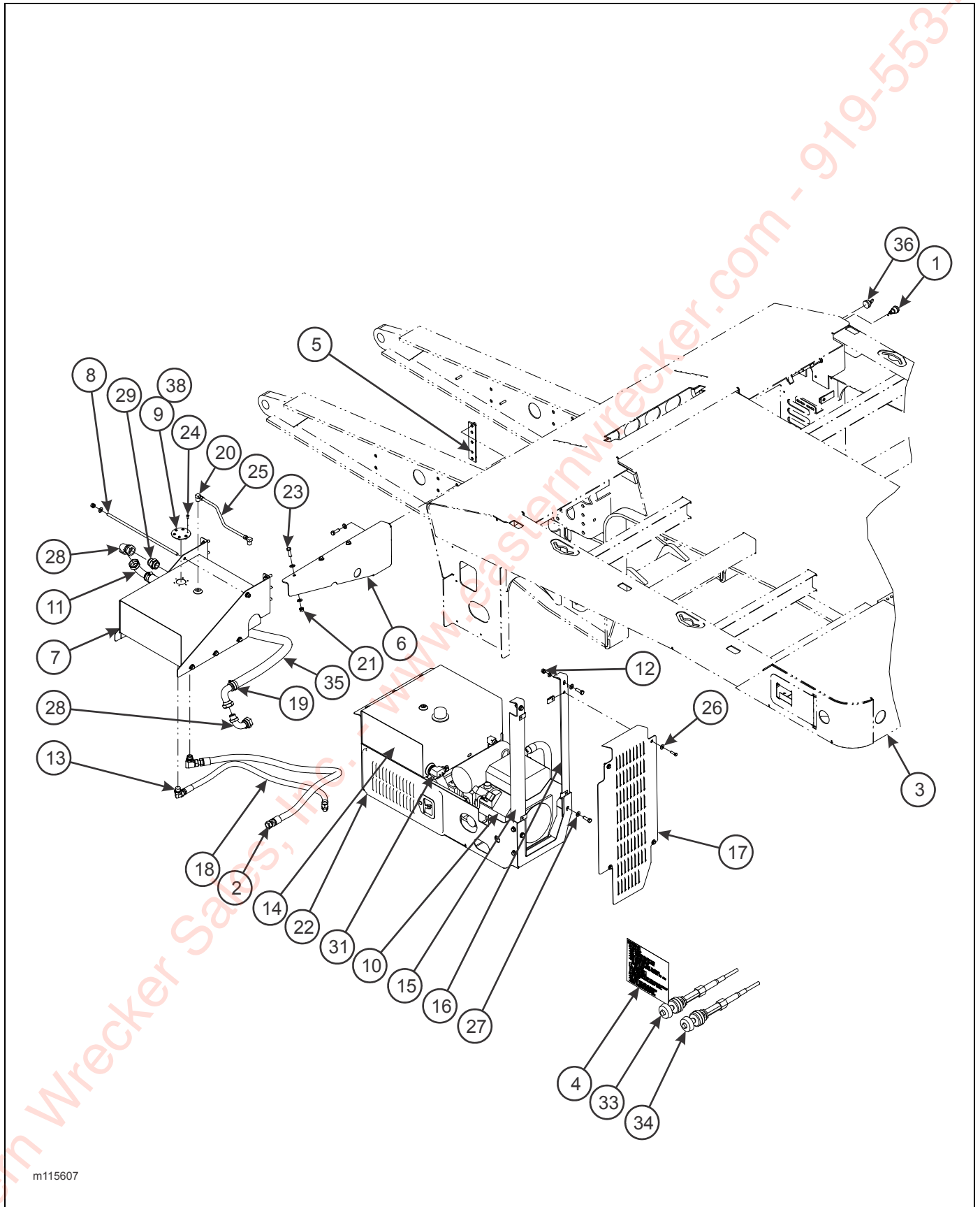
Figure 2-69: Engine Package Bracket Kit
