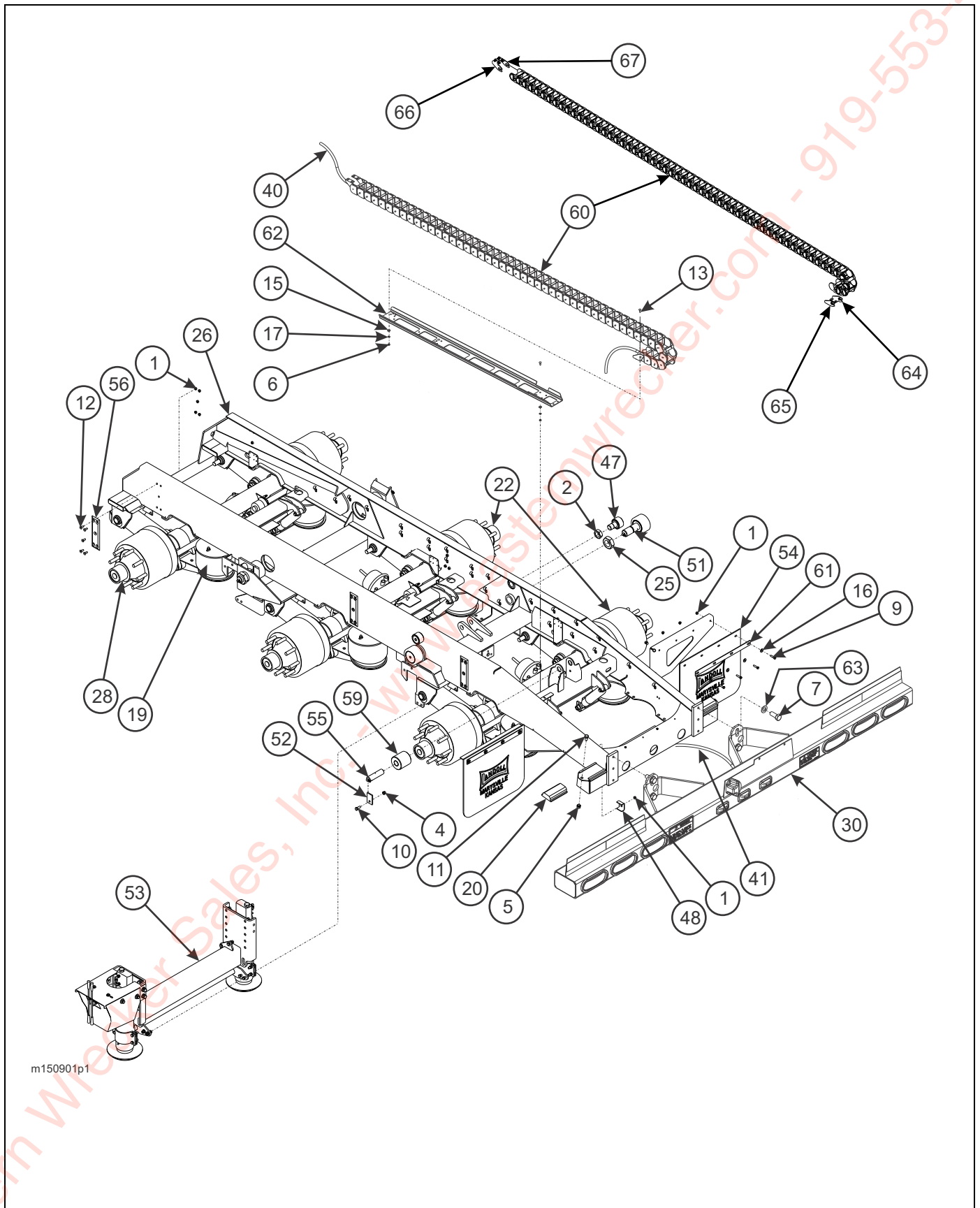
Figure 2-21: U/C Assembly, Air Ride Suspension (Triple Axle) (2 of 2)
