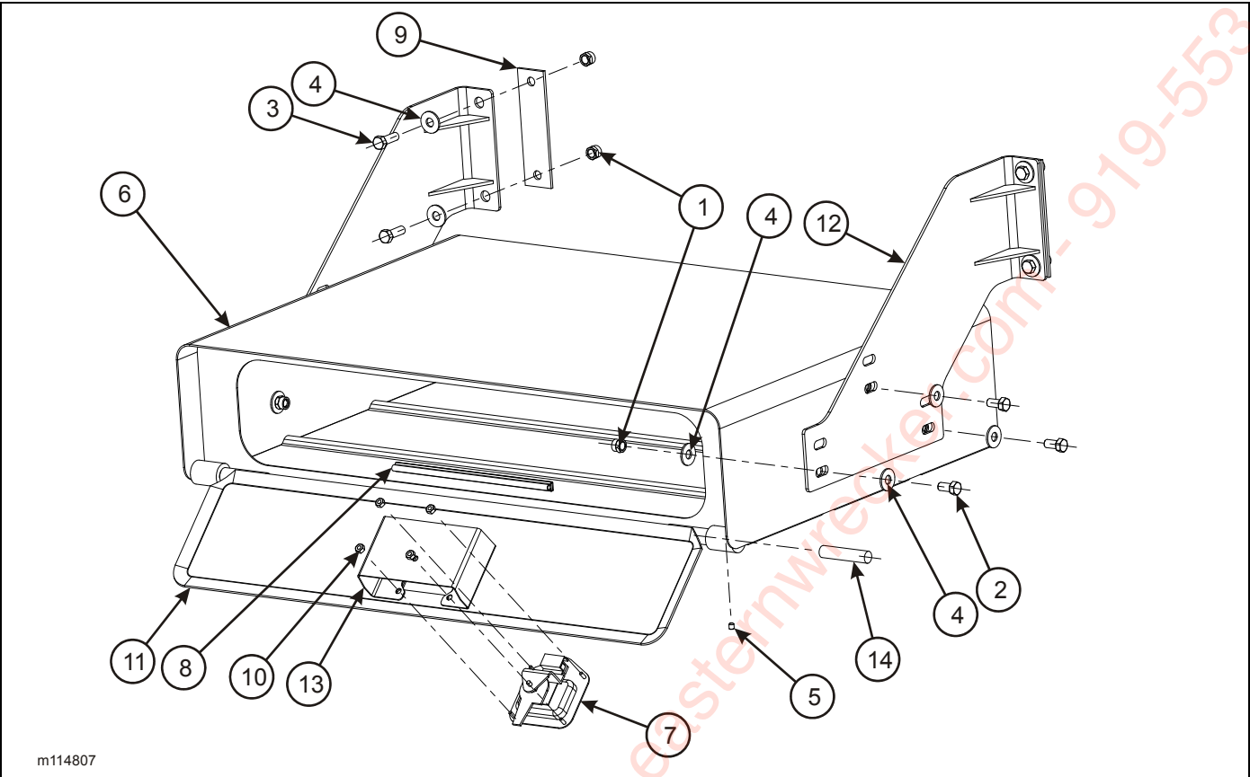
Figure 2-75: Toolbox Installation (Option)
