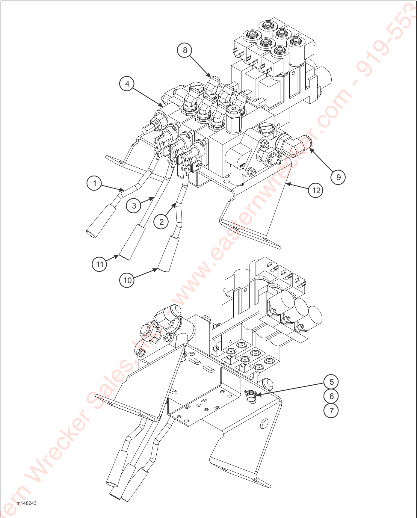
Figure 2-15: Three Spool Valve Assembly (After 01/10/2008)
