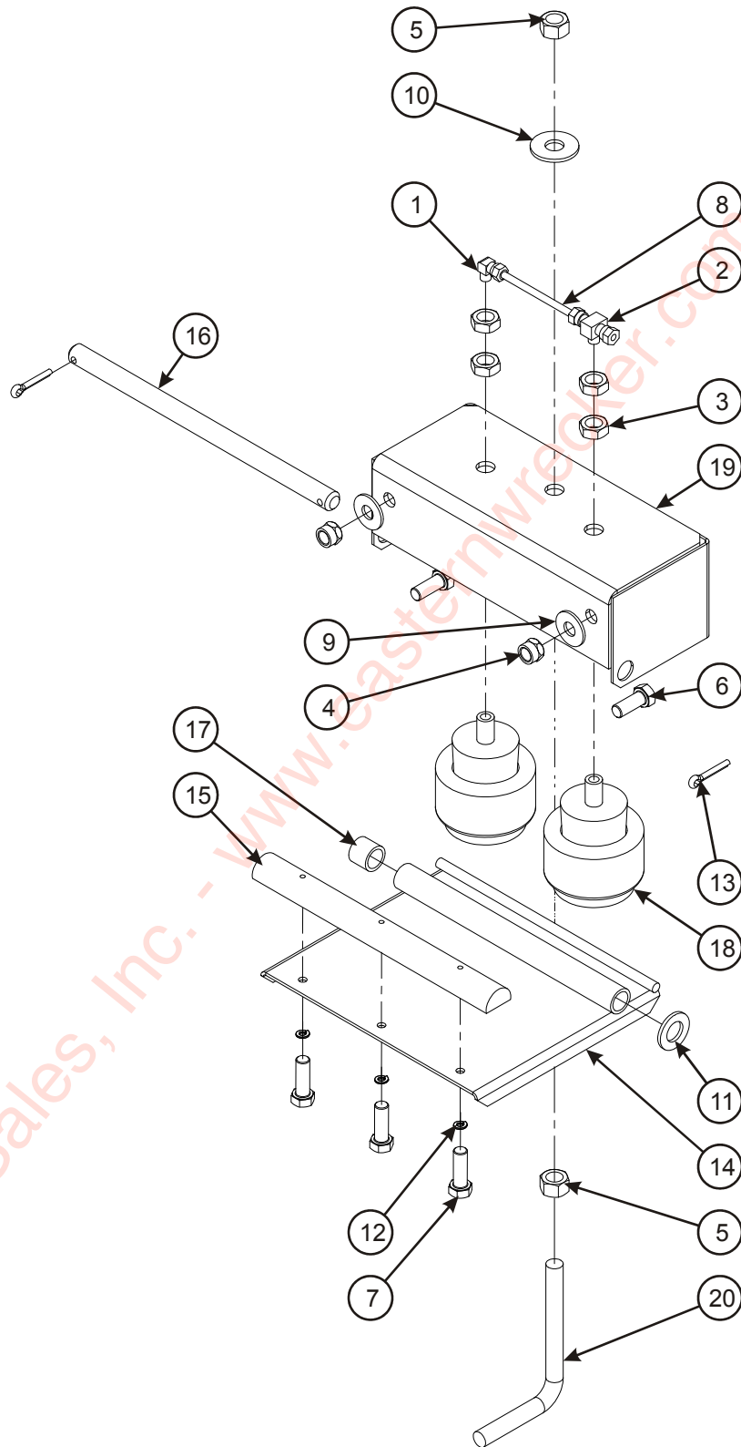
Figure 2-44: Winch, Cable Air Tension
