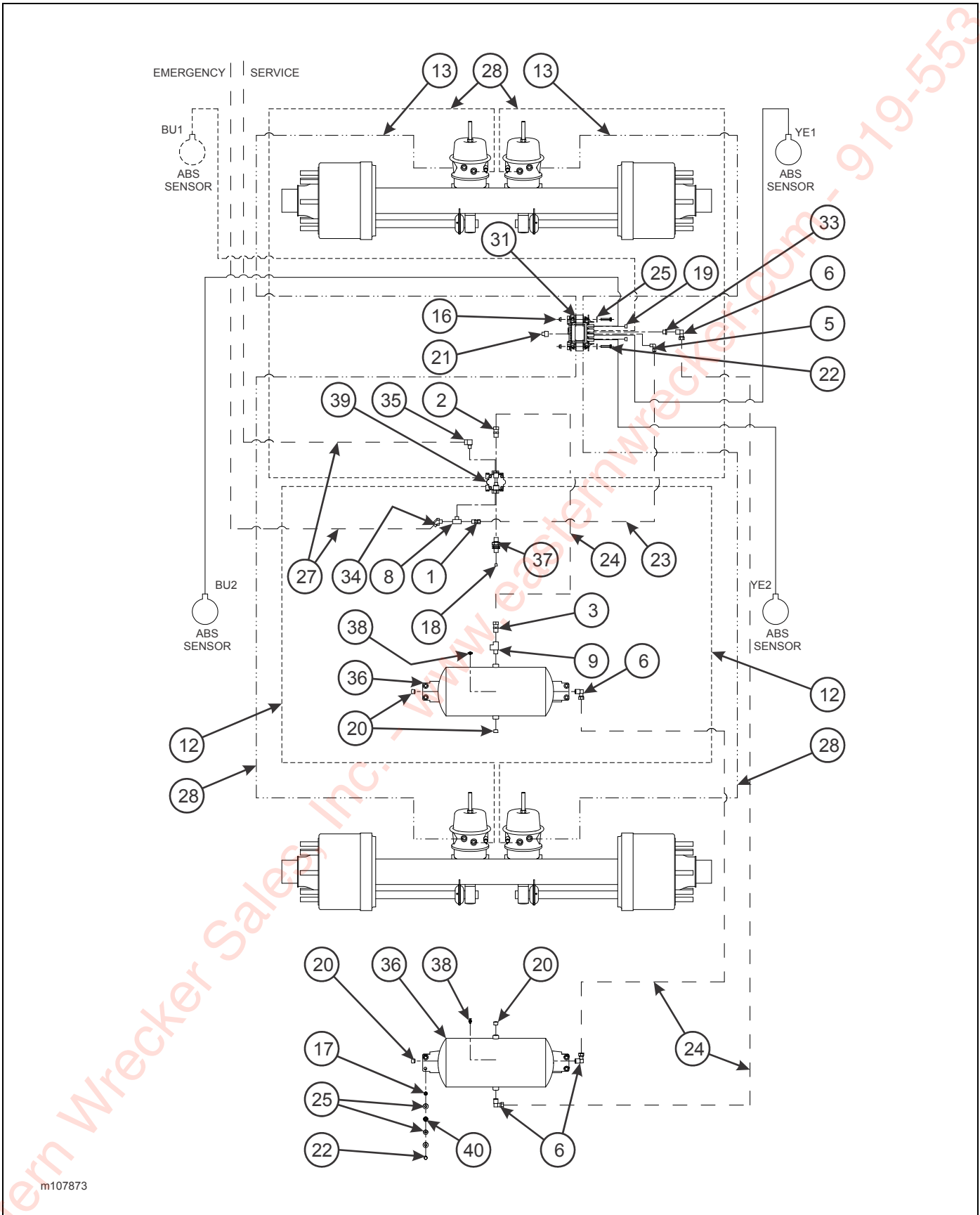
Figure 2-30: Spring Air Brake System w/ ABS (Spread Axle)
