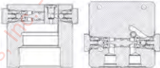
FRONT SECTION TOP SECTION
