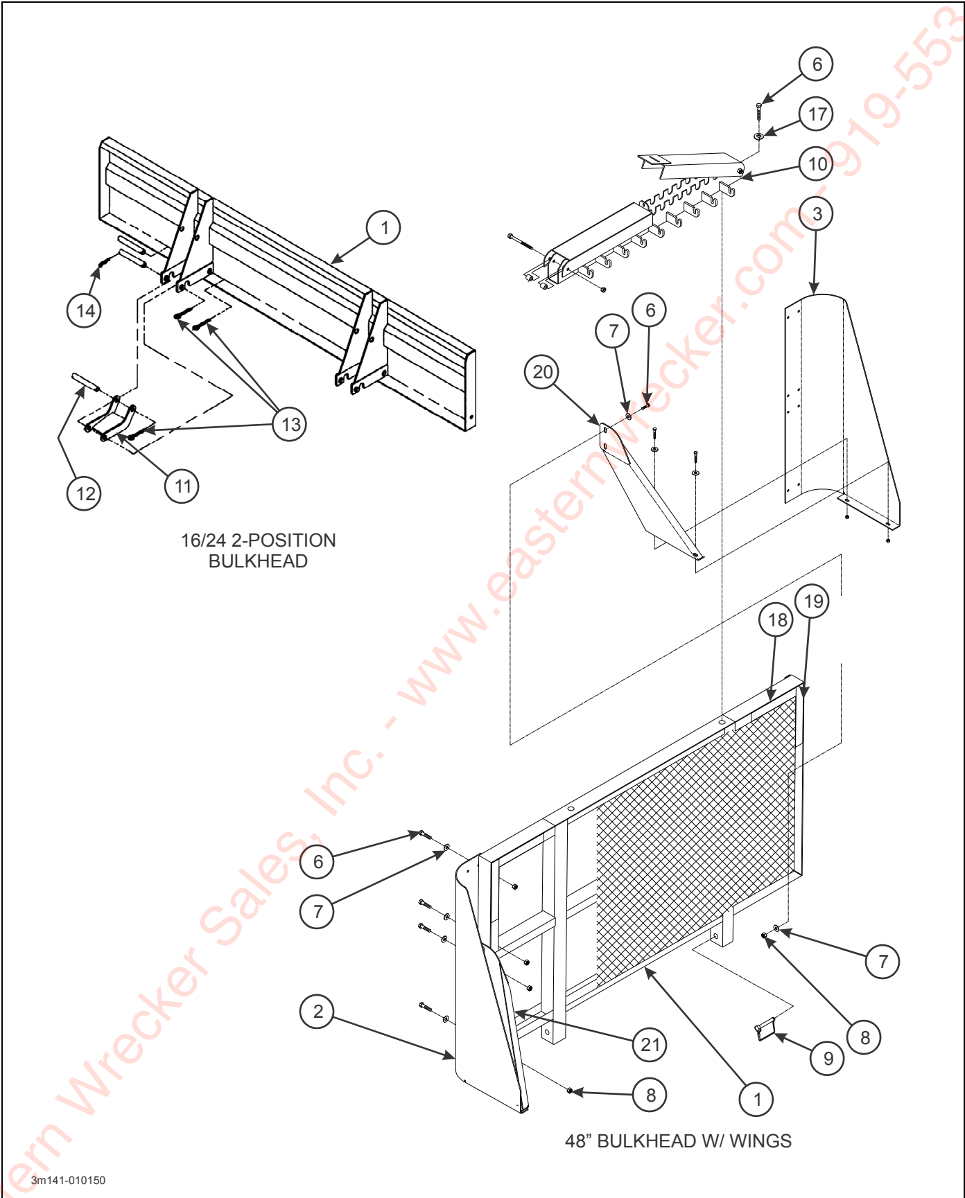
Figure 2-4: Bulkhead Assembly
