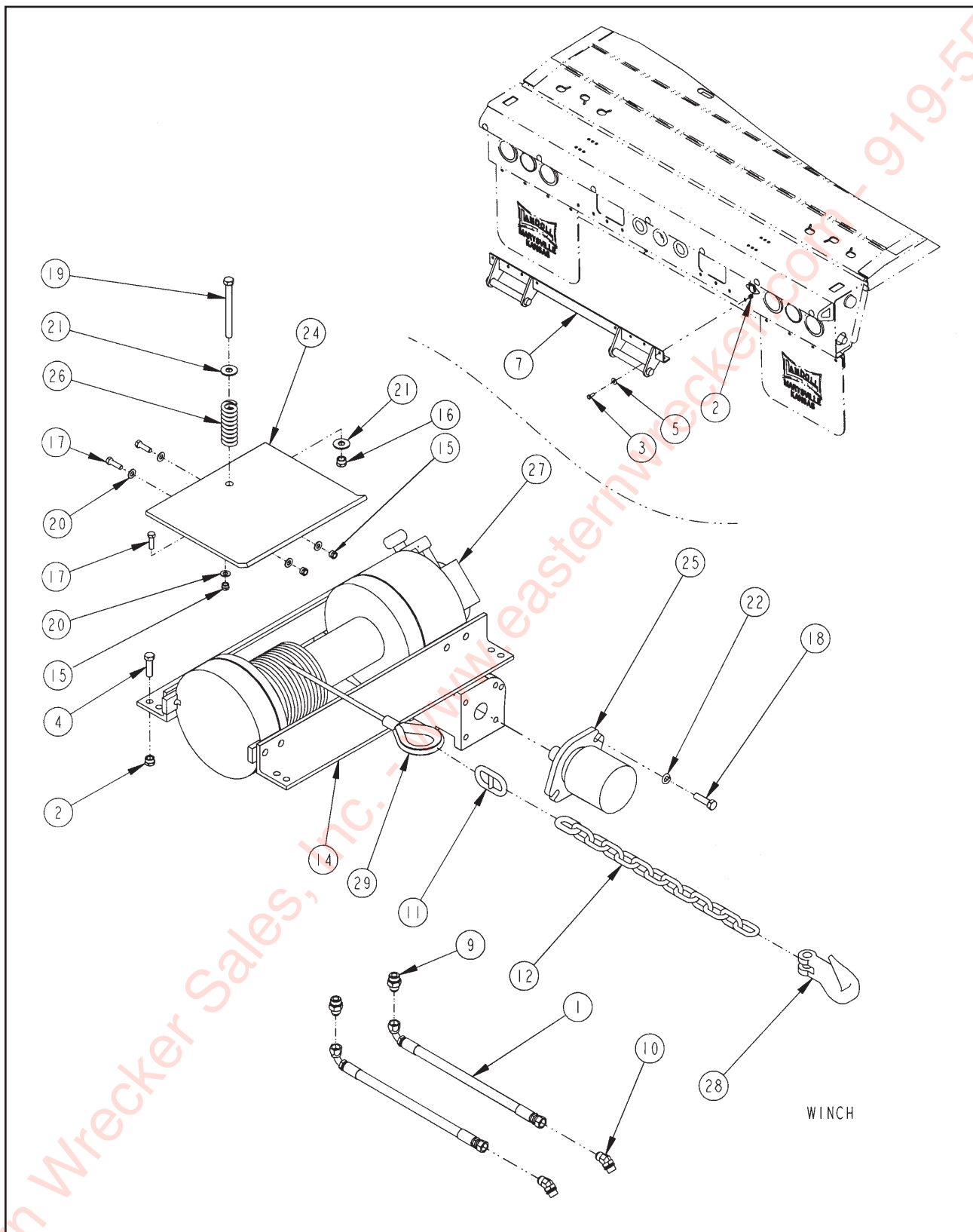
Figure 1-46 Winch Installation
