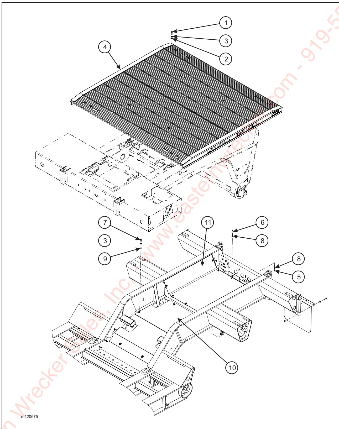
Figure 1-5 Bed Installation (Trunnion and Gooseneck)
