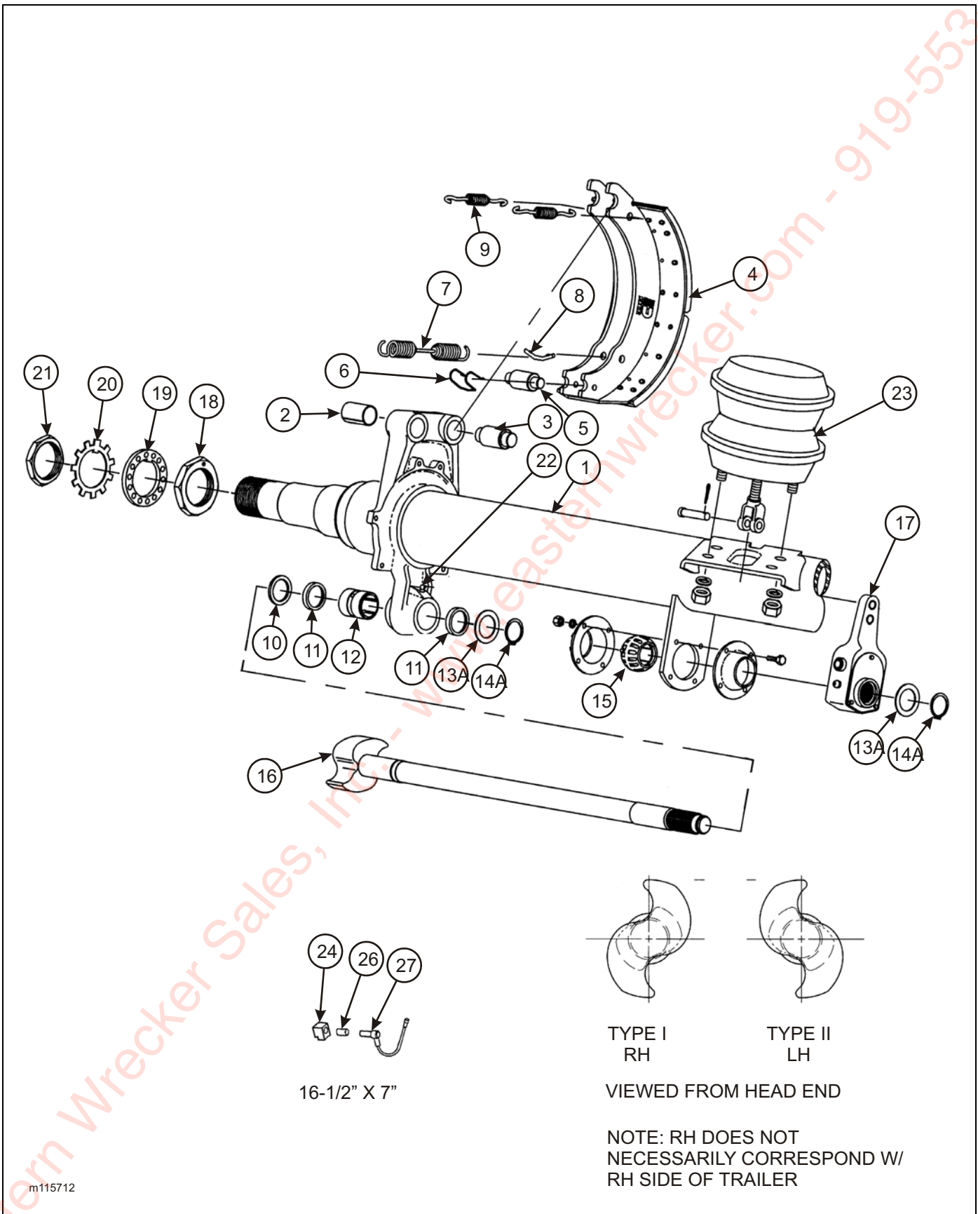
Figure 1-25 Axle and Brake Assembly
