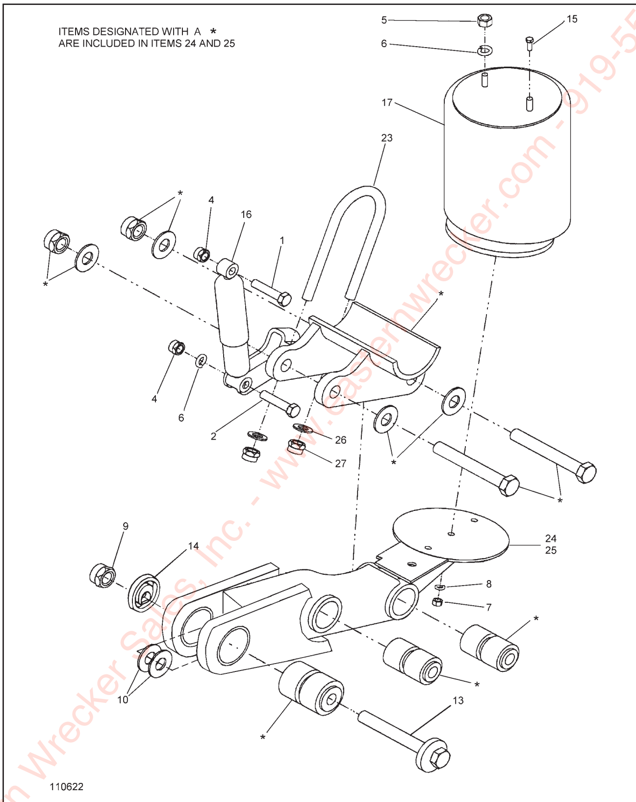
Figure 1-22 Suspension Fastener, AR-80-9 FMT
