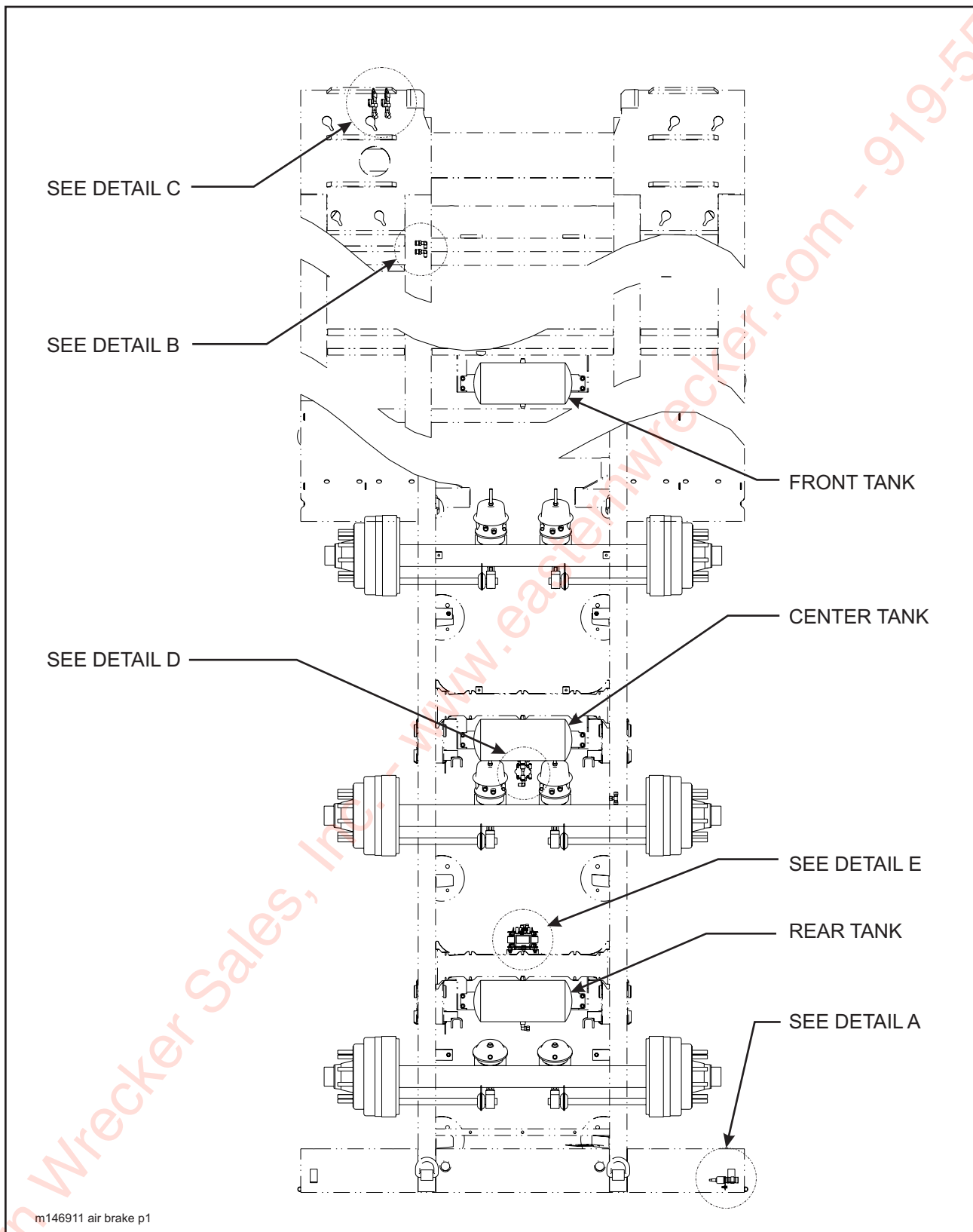
Figure 1-40 Air Brake System (835B Triple Axle)
