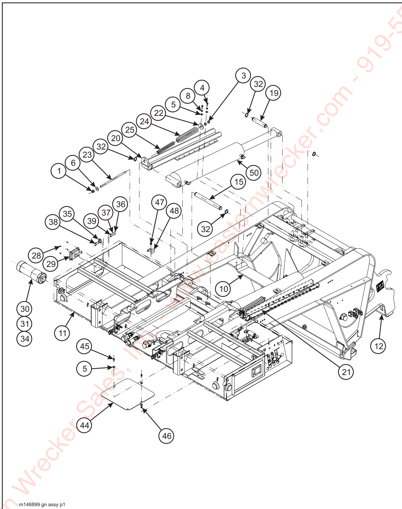
Figure 1-2 Gooseneck Assembly (1 of 2)
