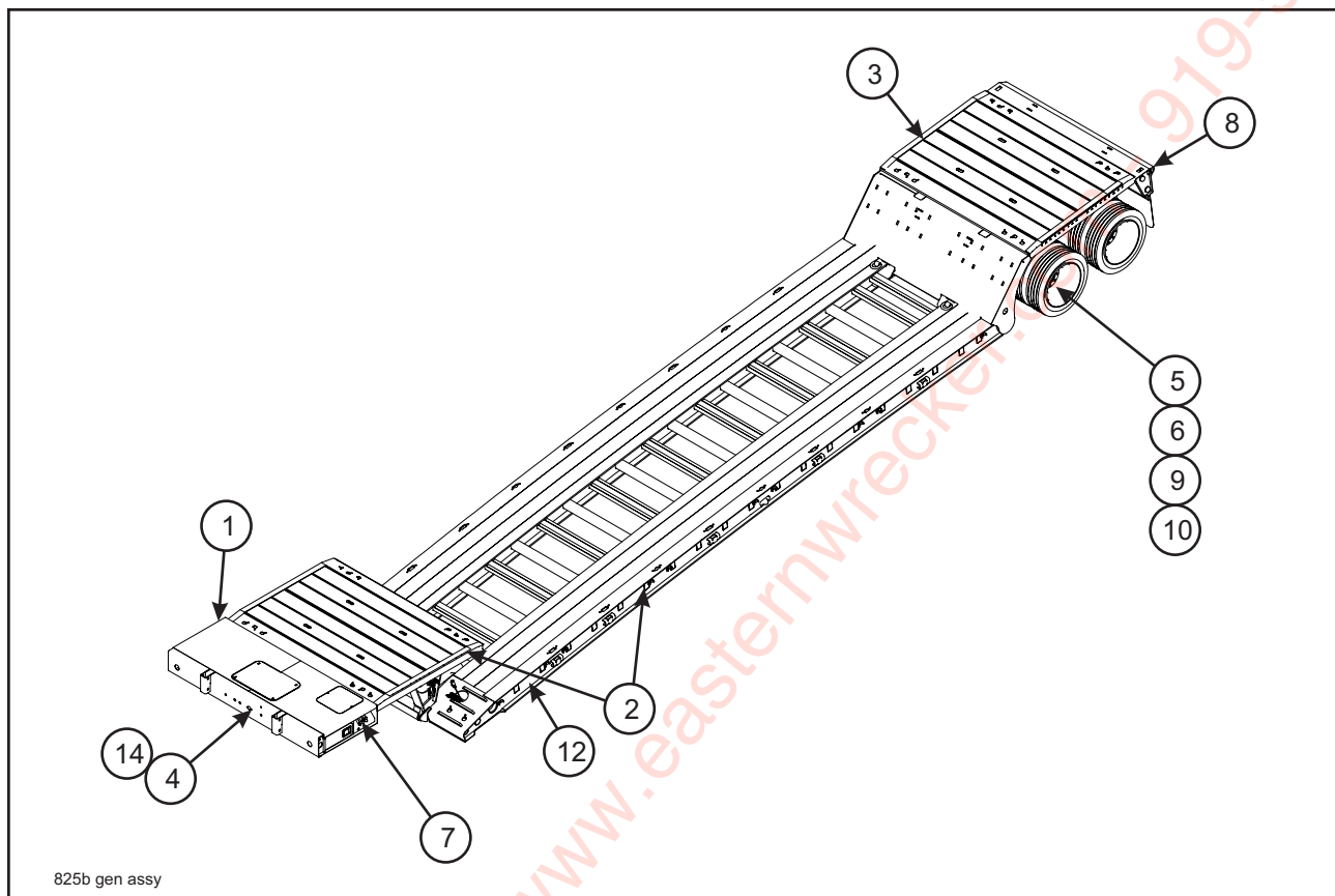
Figure 1-1 General Assembly
