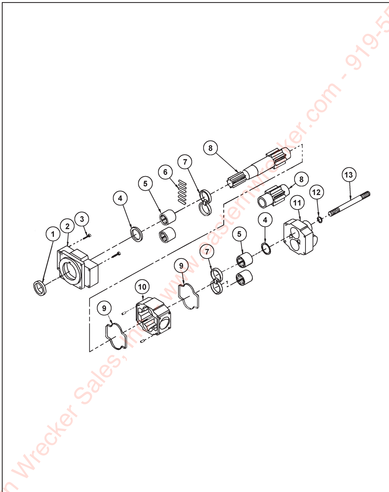
Figure 1-62 Hydraulic Pump, Wet Kit (Option)
