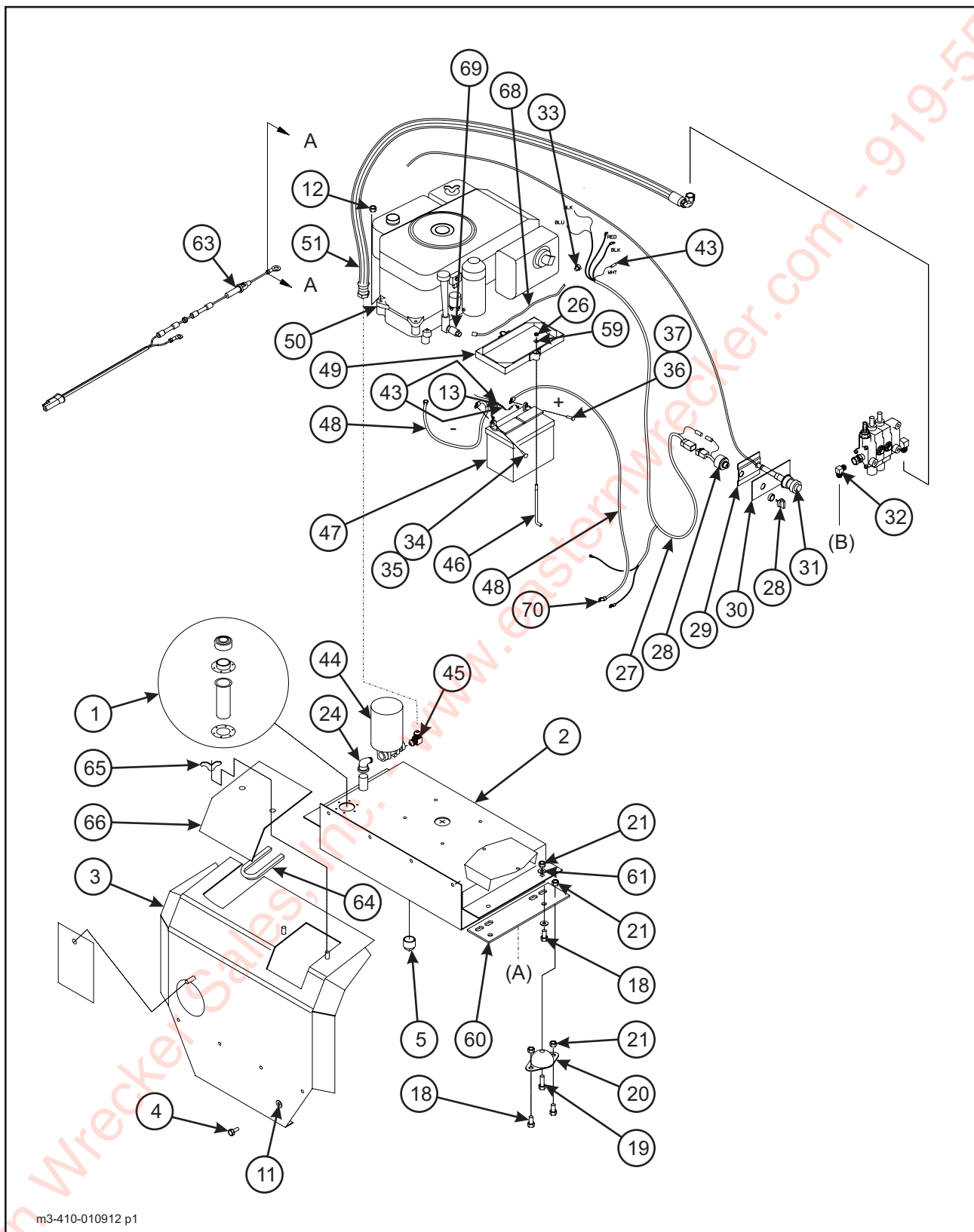
Figure 1-58 42-11 HP Honda Engine Drive Installation (Option) (1 of 2)
