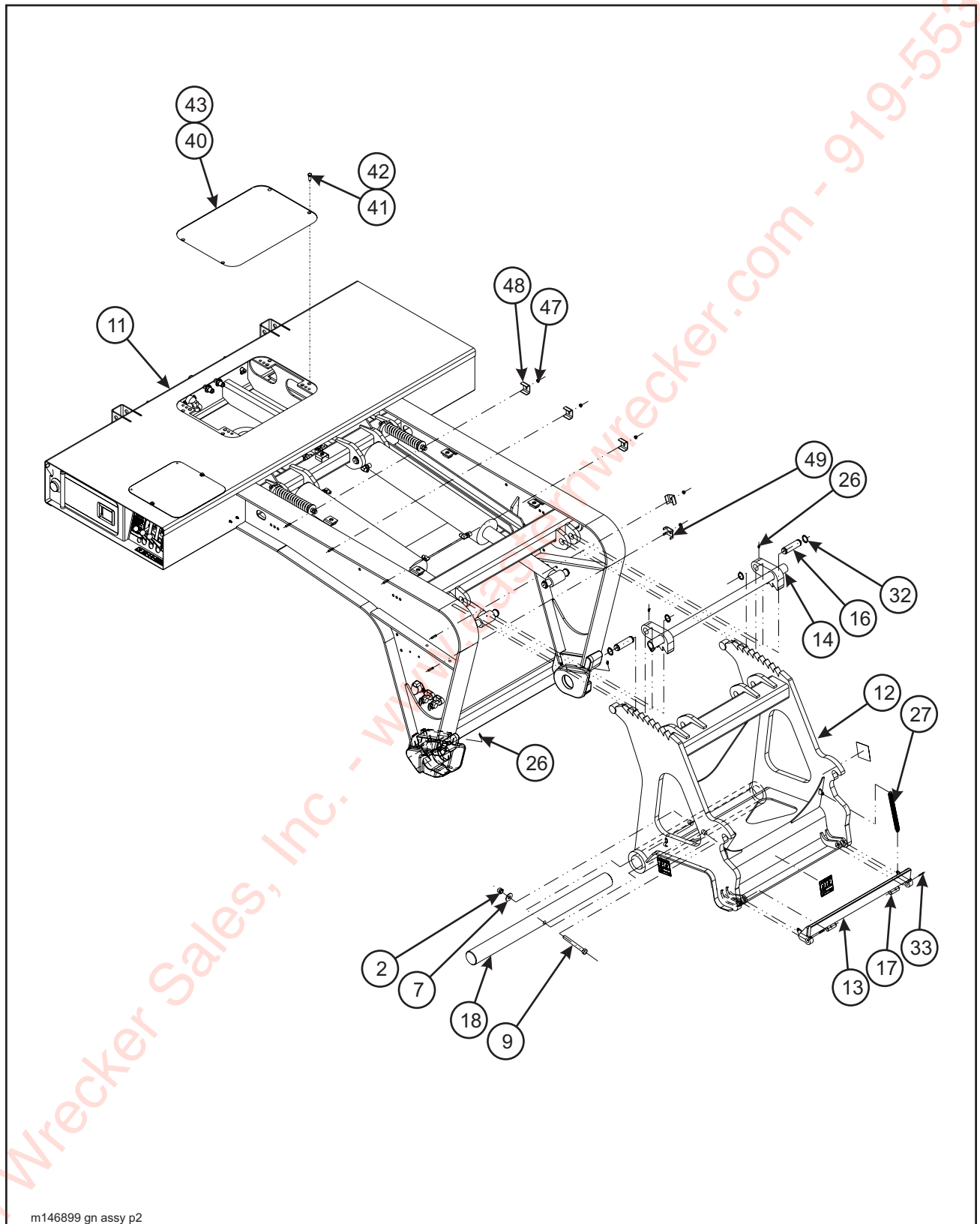
Figure 1-3 Gooseneck Assembly (2 of 2)
