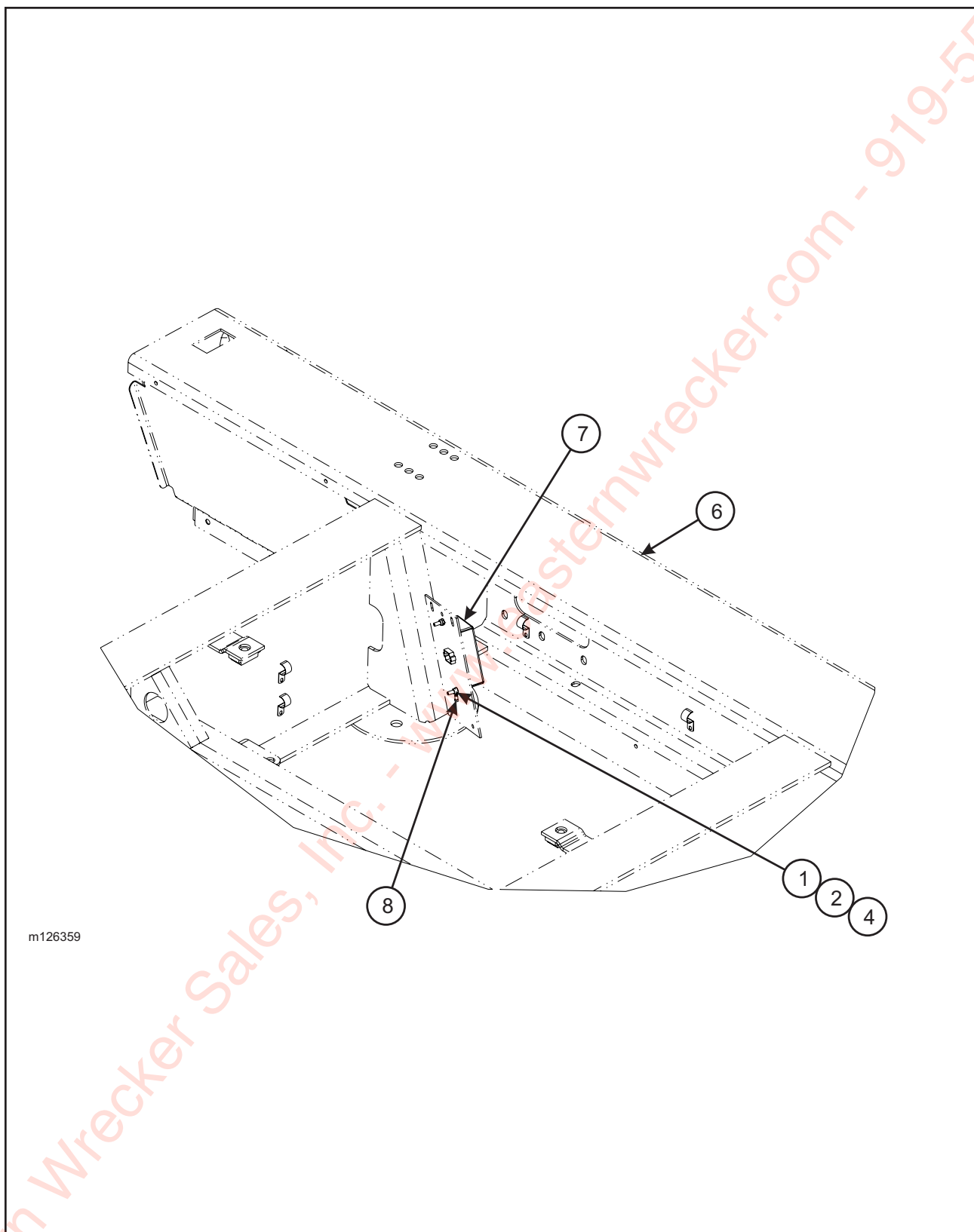
Figure 1-63 Air Weigh Scale Installation (Option)
