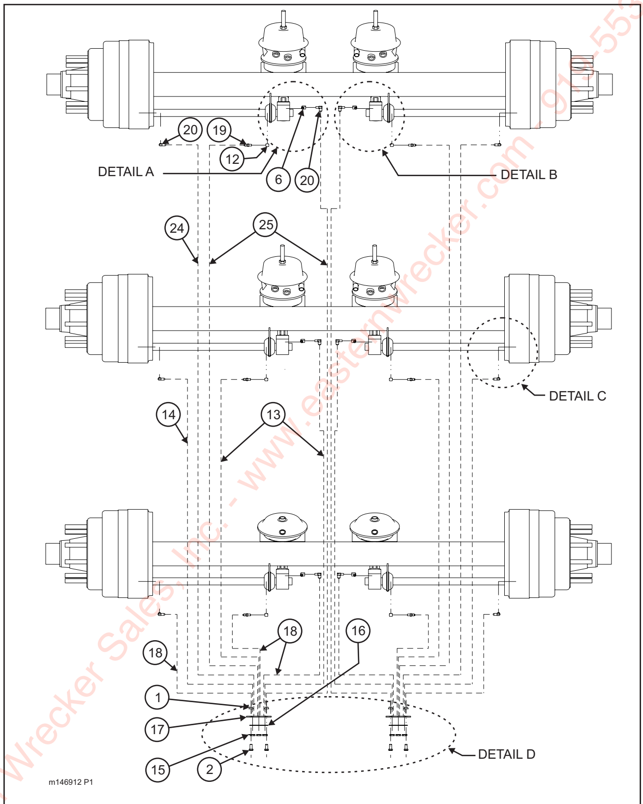
Figure 1-14 Frame Assembly and Grease System (835B - Triple) (4 of 5)
