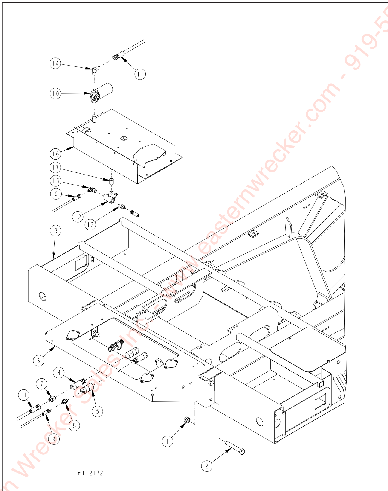
Figure 1-57 Engine Installation Front Mount (Option)
