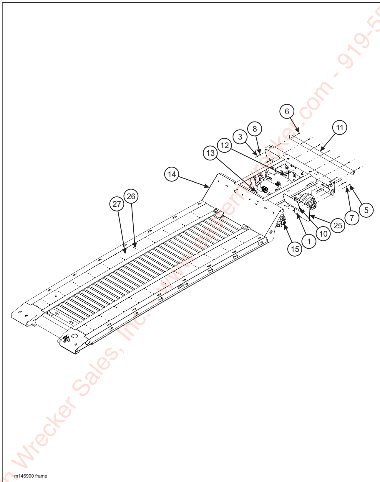
Figure 1-8 Frame Assembly and Grease System (825B) (1 of 3)
