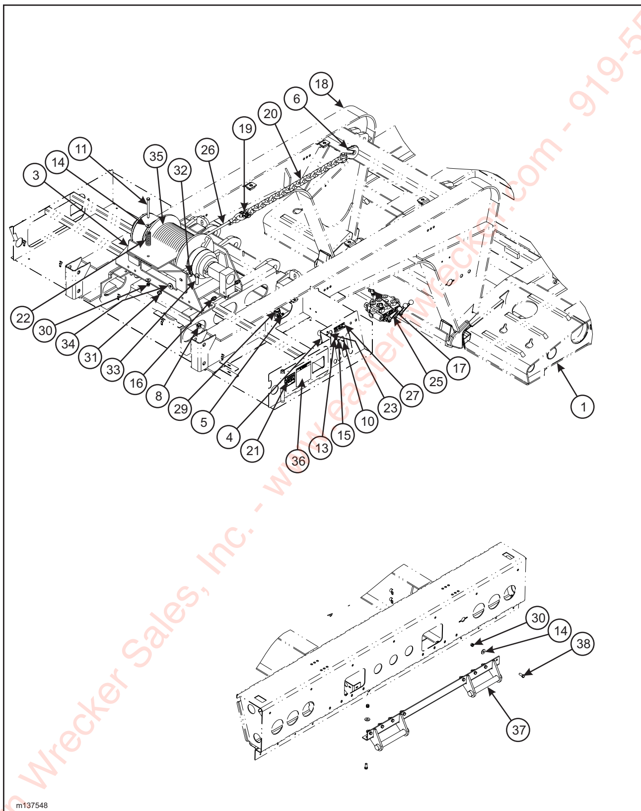
Figure 1-51 30K DP Winch Installation
