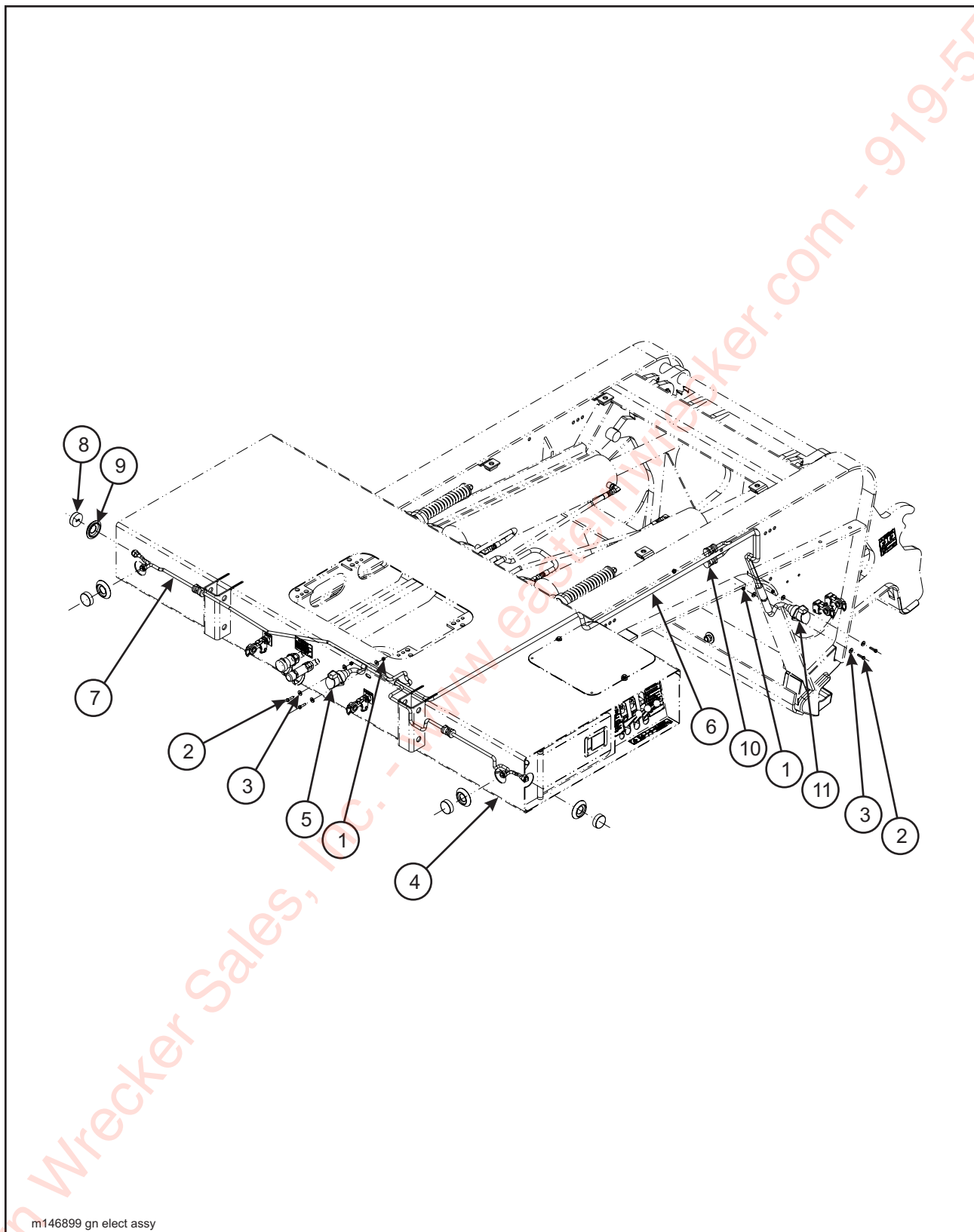
Figure 1-30 Gooseneck Electrical System
