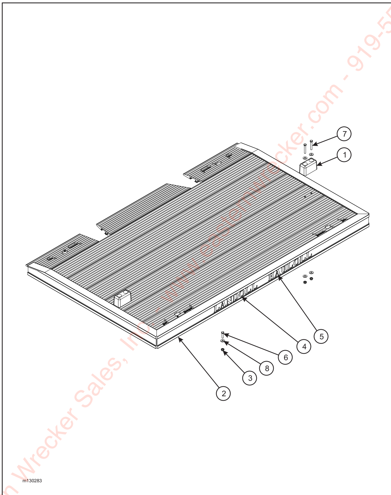
Figure 1-6 Bed Installation (Flip Axle)
