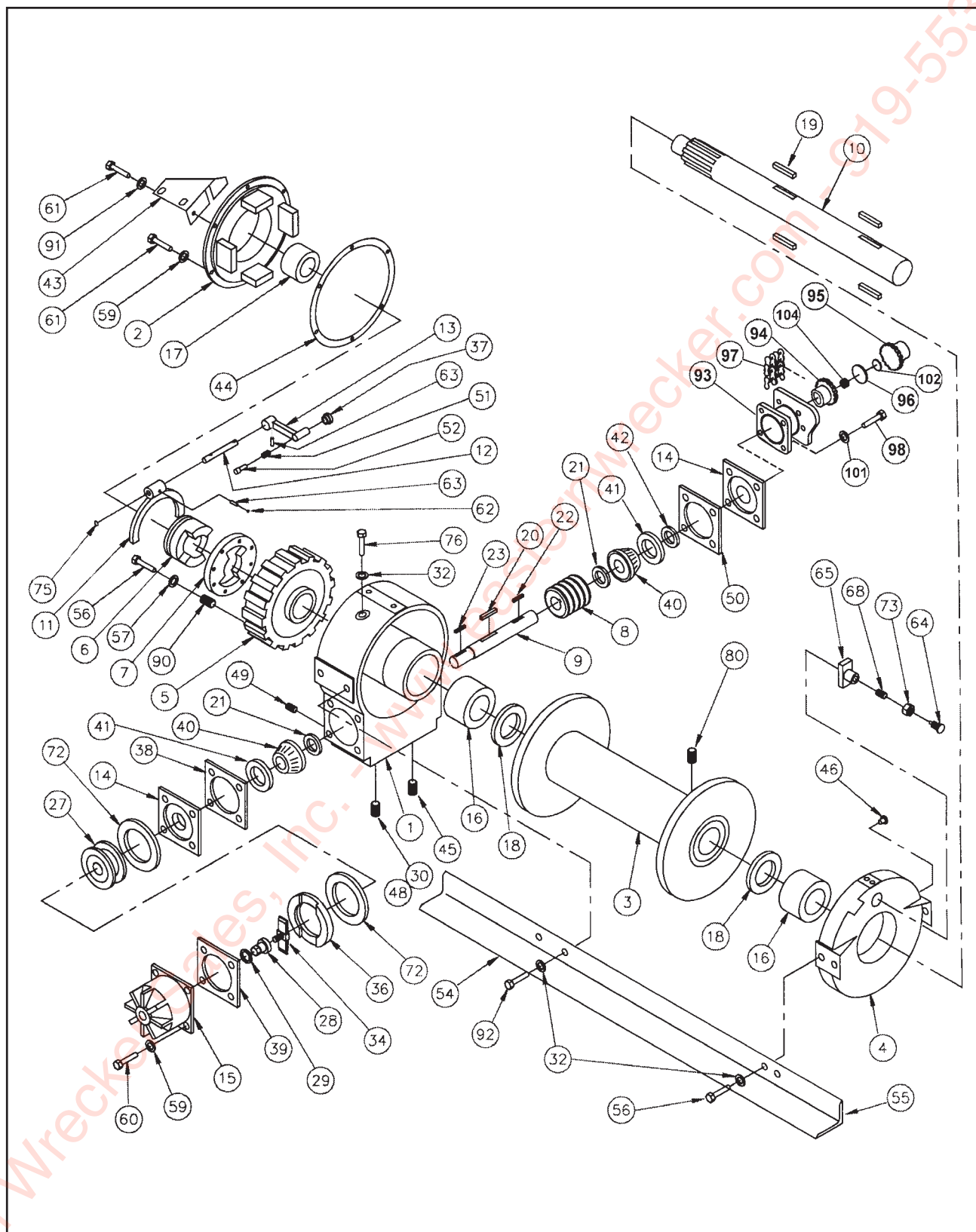
Figure 1-48 20,000# Winch Assembly
