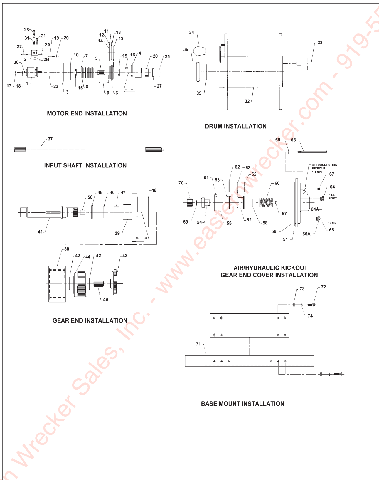
Figure 1-53 30K DP Winch Installation
