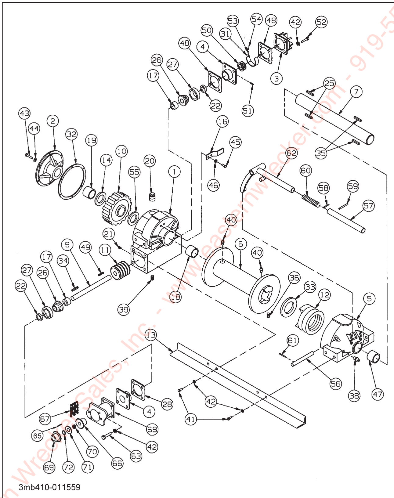
Figure 1-47 12,000# Winch Assembly
