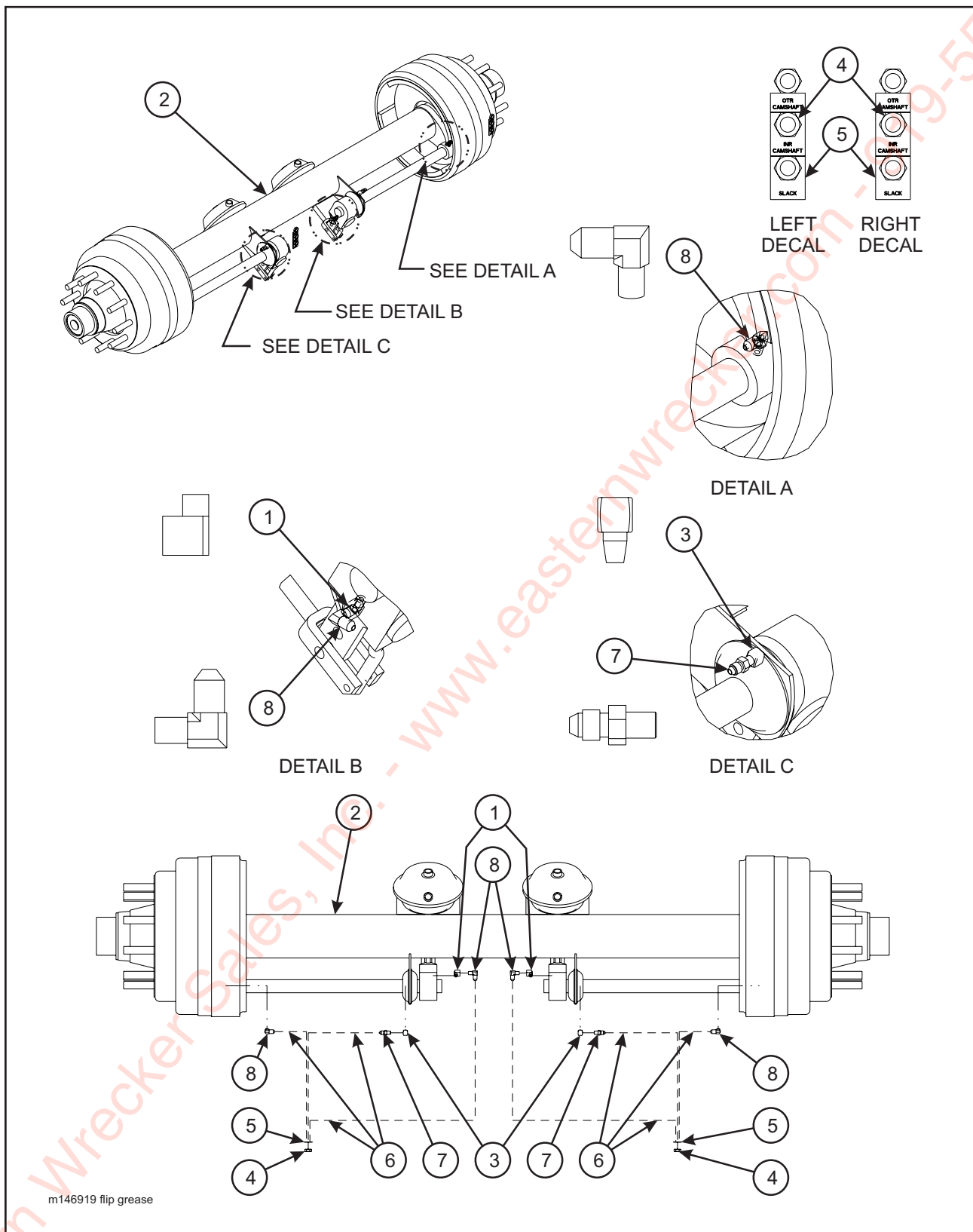
Figure 1-20 Flip Assembly - Air Ride Suspension
