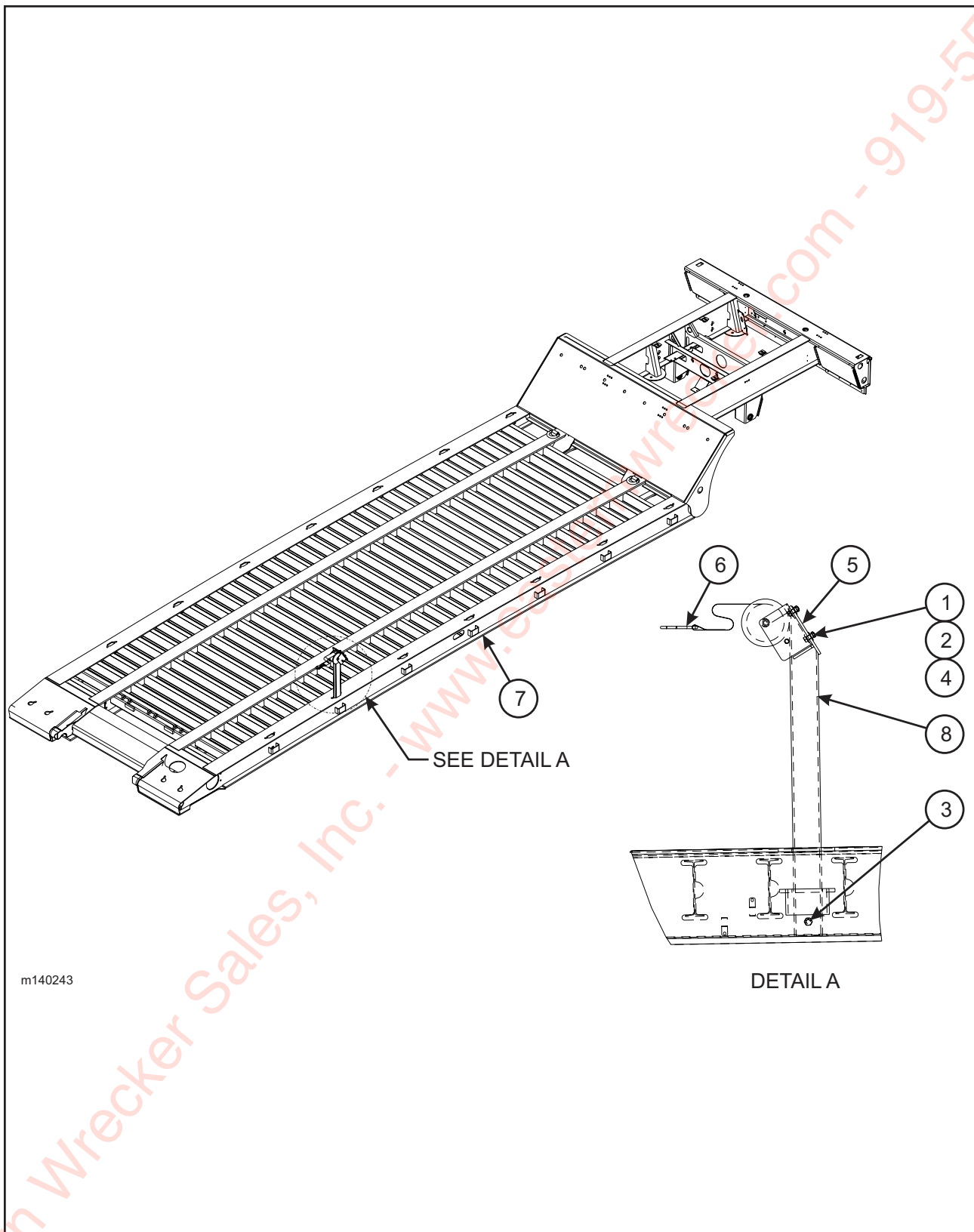
Figure 1-71 Ramp Lift Assembly (Option)
