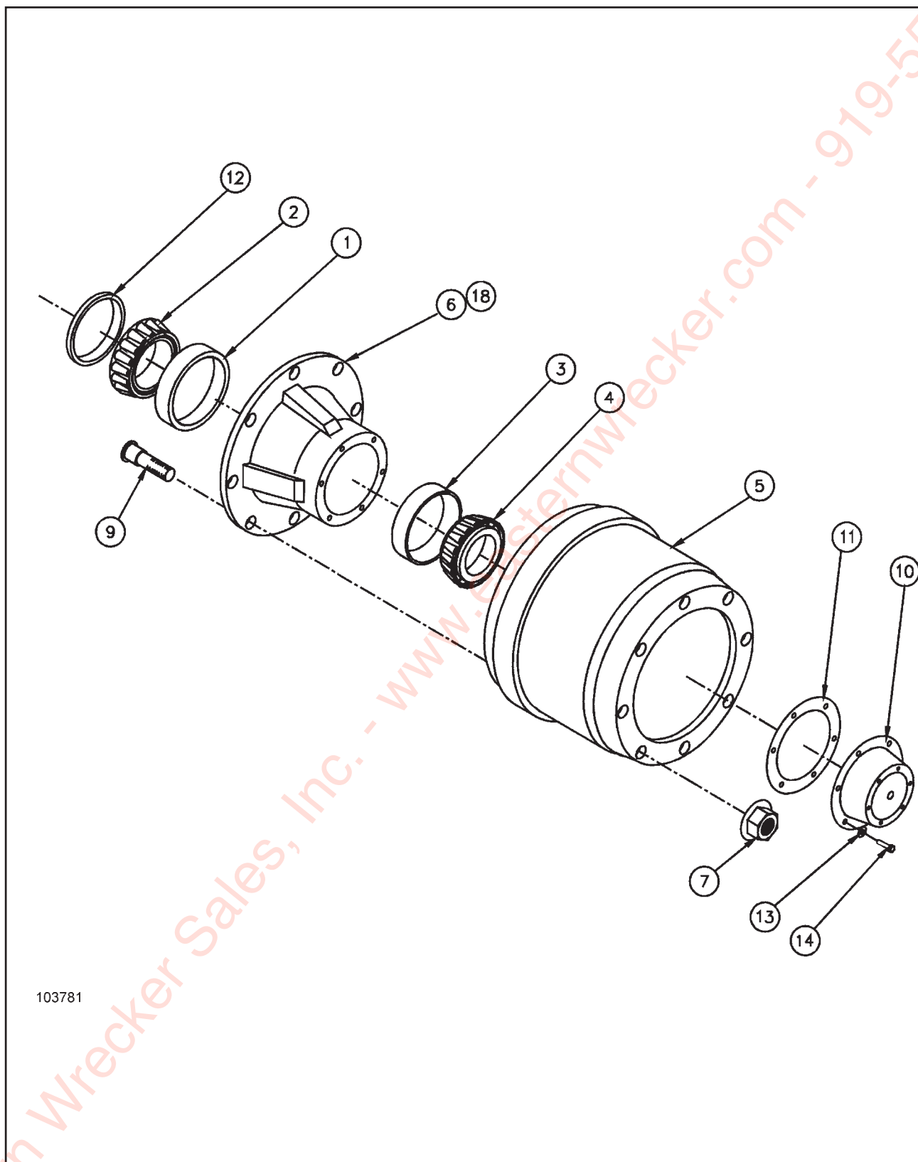
Figure 1-45 Outboard Pilot Mount Hub and Drum
