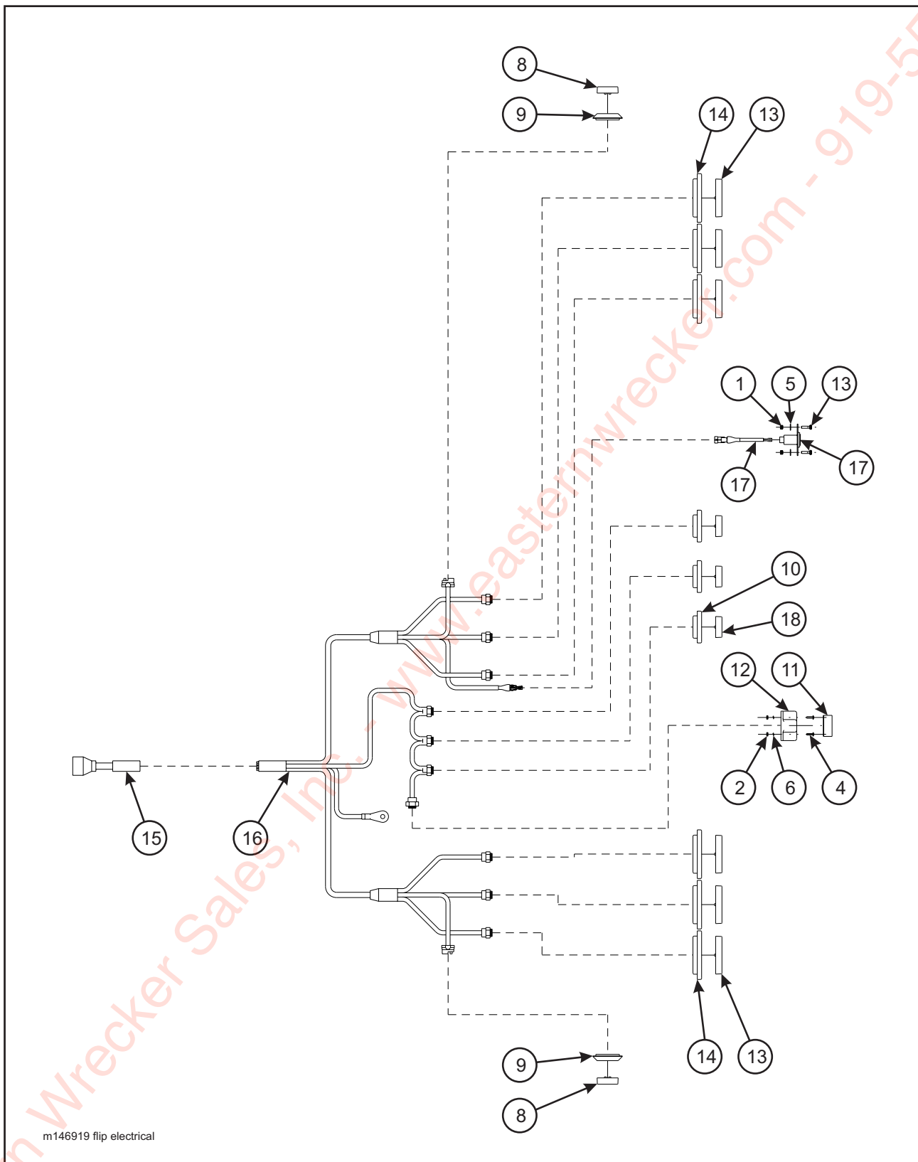
Figure 1-32 Flip Axle Electrical System (835B)
