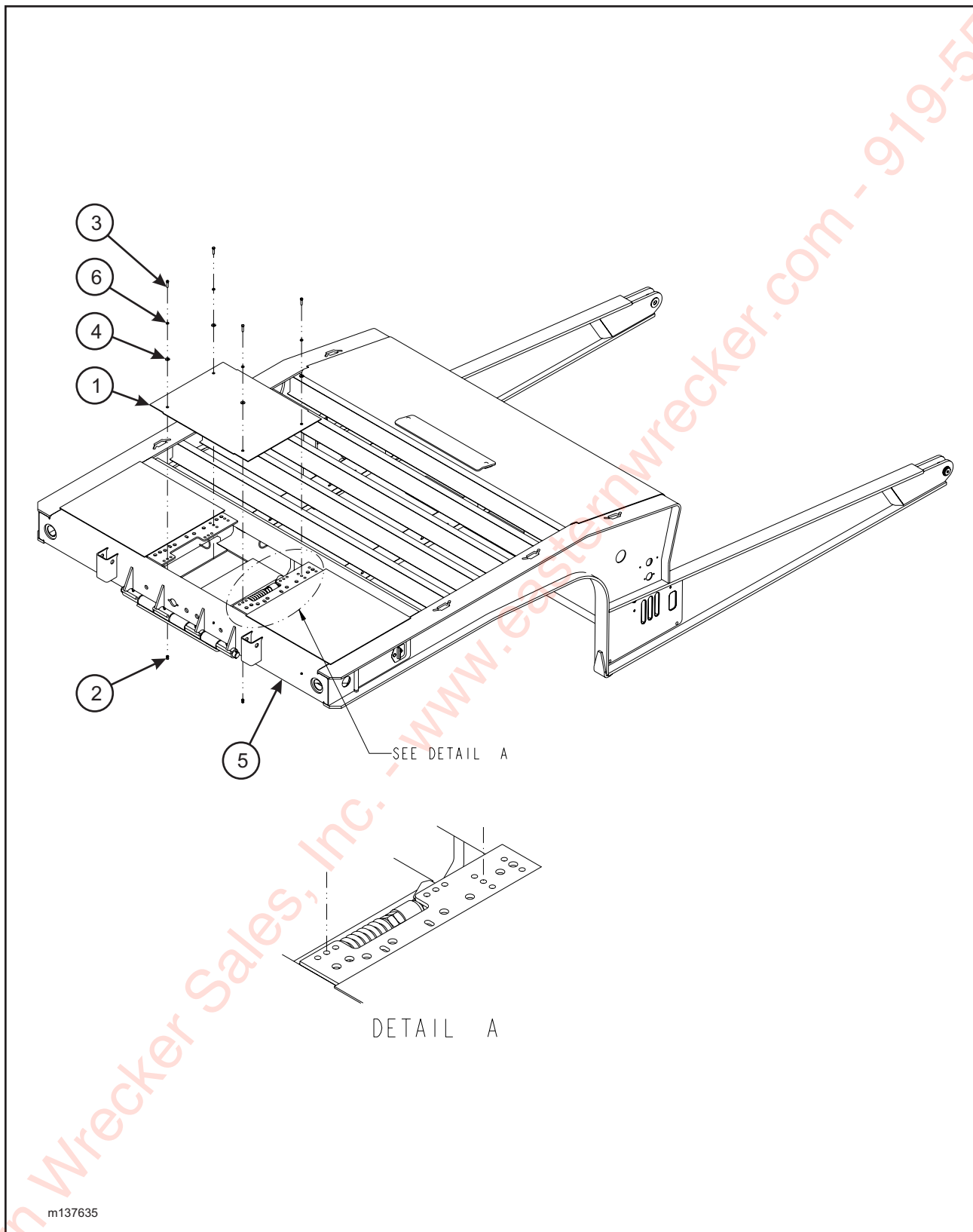
Figure 1-40 Cover Assembly, Upper Deck
