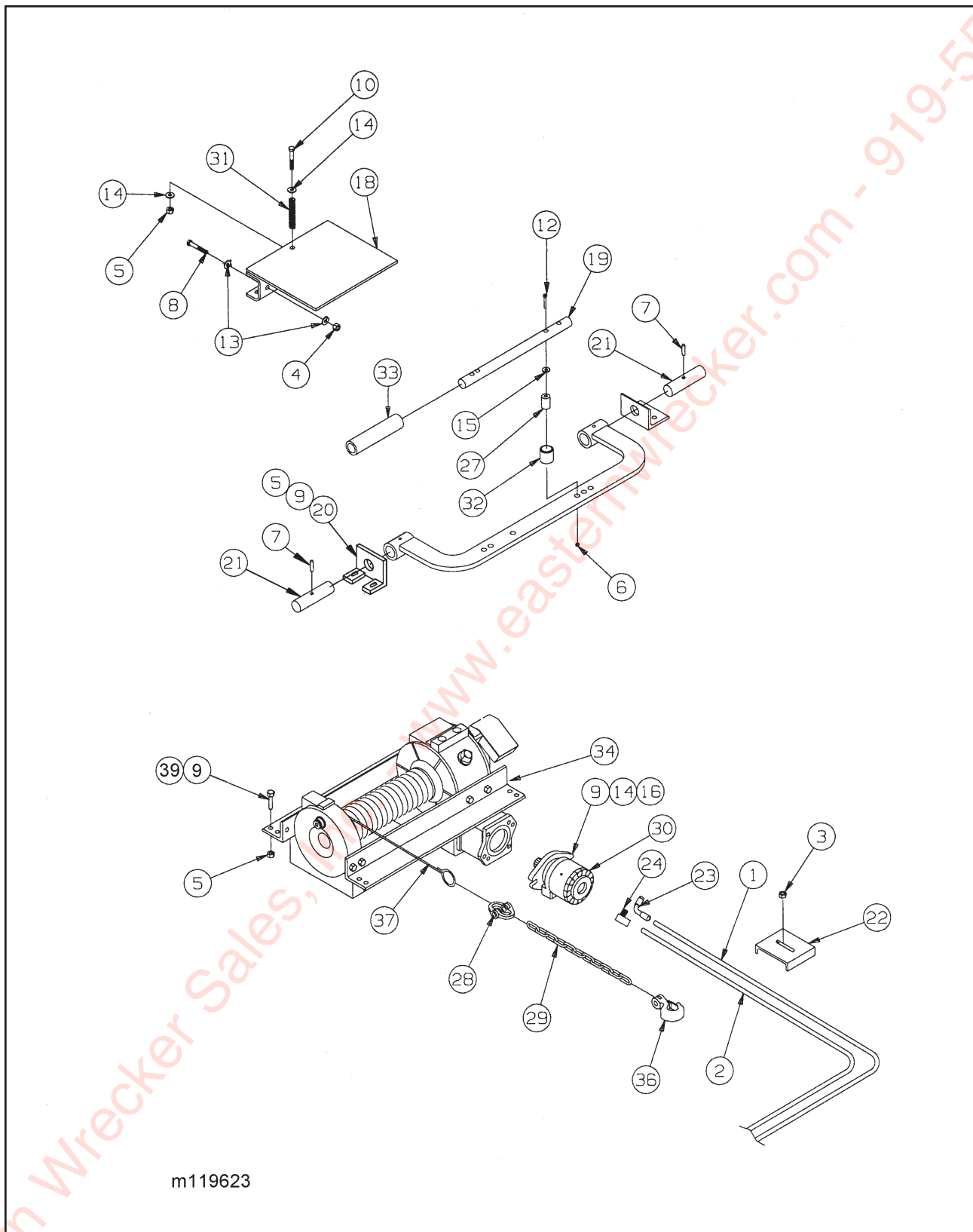
Figure 1-26 Winch Installation, Spring Tension Cable Roller
