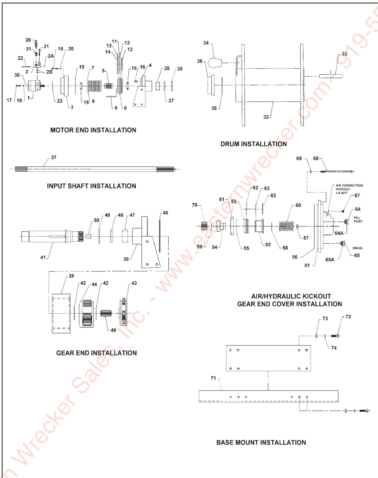
Figure 1-33 30,000# Winch Items (DP Planetary)
