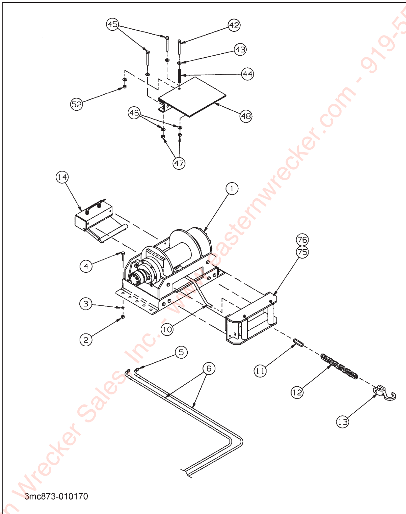
Figure 1-31 30K Upper Deck Winch (DP) (1 of 2)
