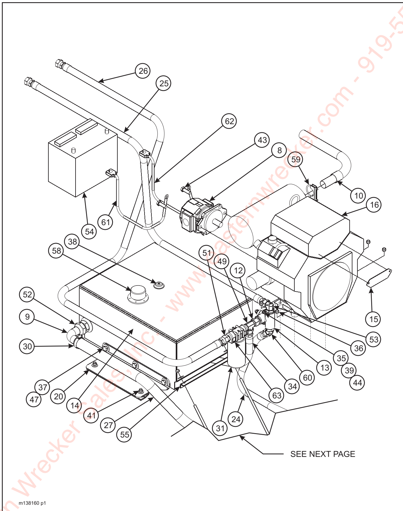
Figure 1-52 Hydraulic Engine, 27HP Slope (1 of 2)
