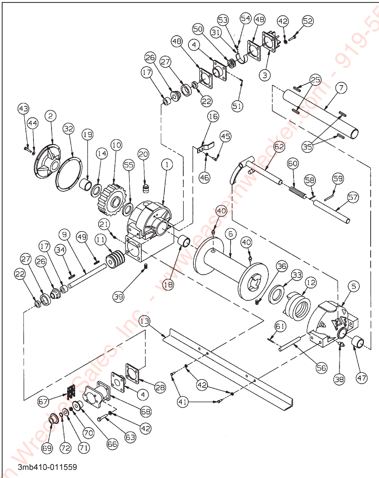
Figure 1-27 12,000# Winch Items (Braden Worm Gear)
