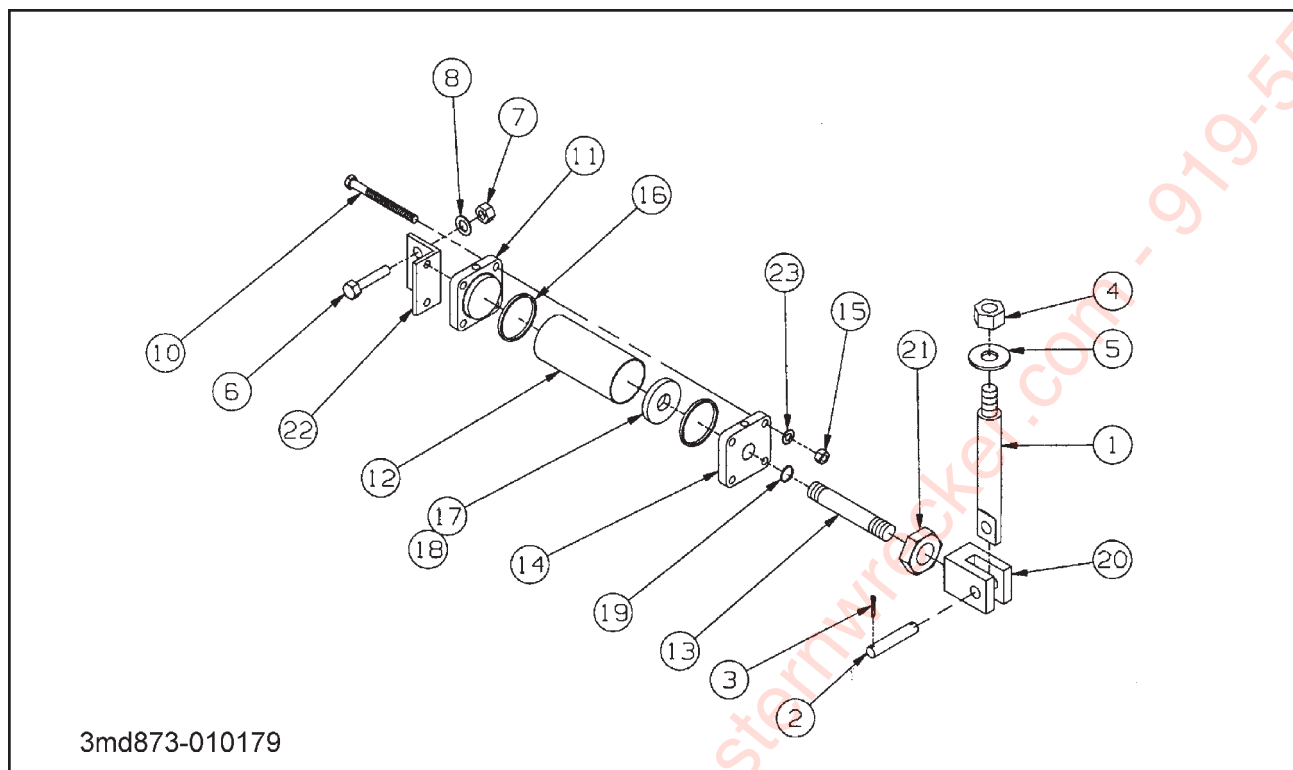
Figure 1-29 Winch Air Shift Cylinder for 20,000# Winch
