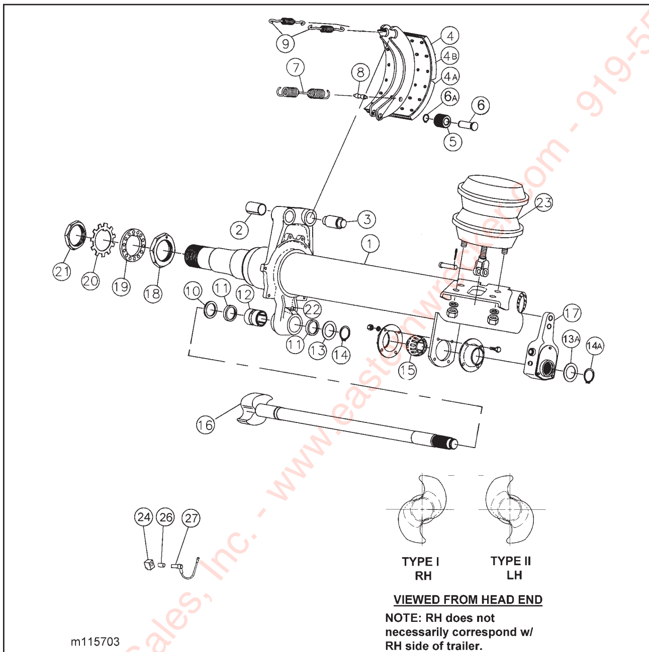
Figure 1-17 Axle and Brake Assembly
