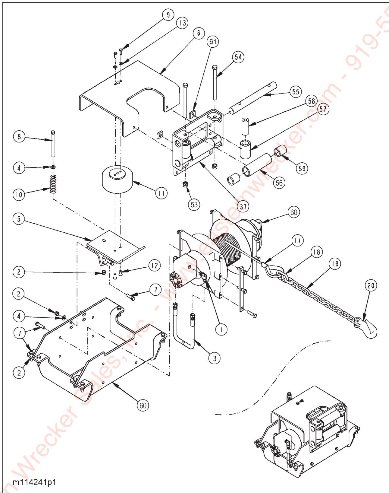
Figure 1-37 12K, 15K, & 20K Upper Deck Winch (DP) (1 of 2)
