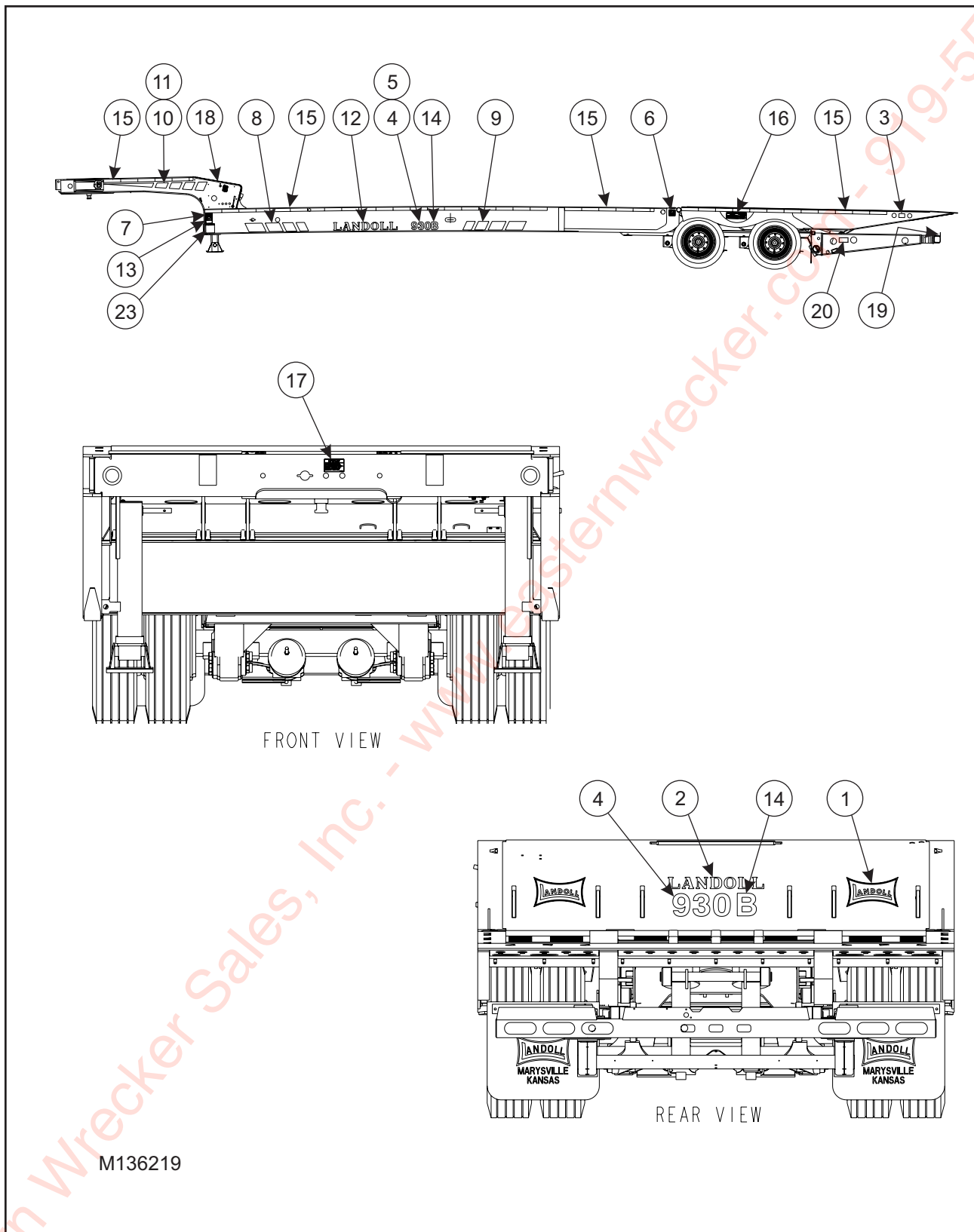
Figure 1-46 Decal Placement
