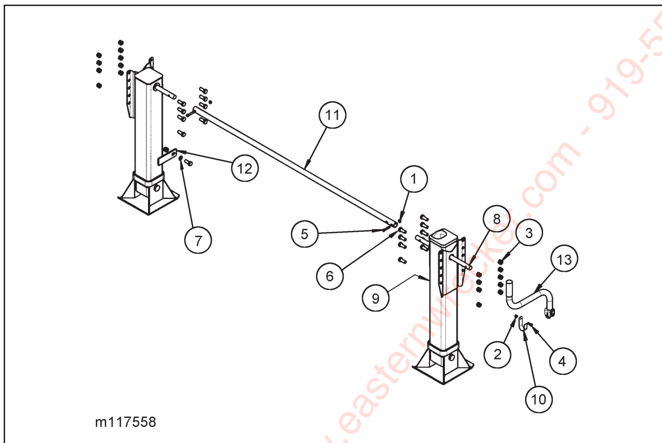
Figure 1-47 Landing Gear
