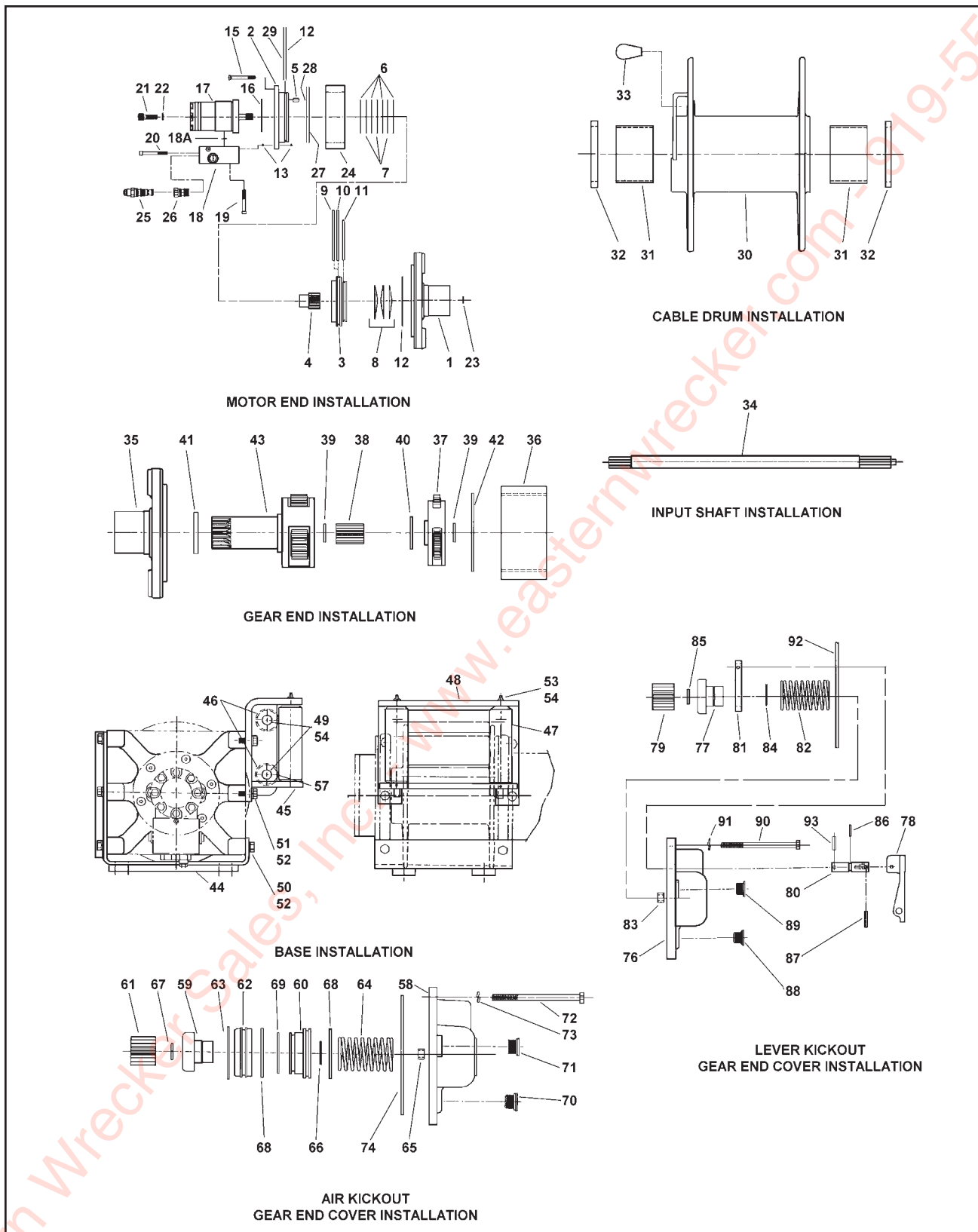
Figure 1-39 12K, 15K, & 20K Winch Items (DP Planetary)
