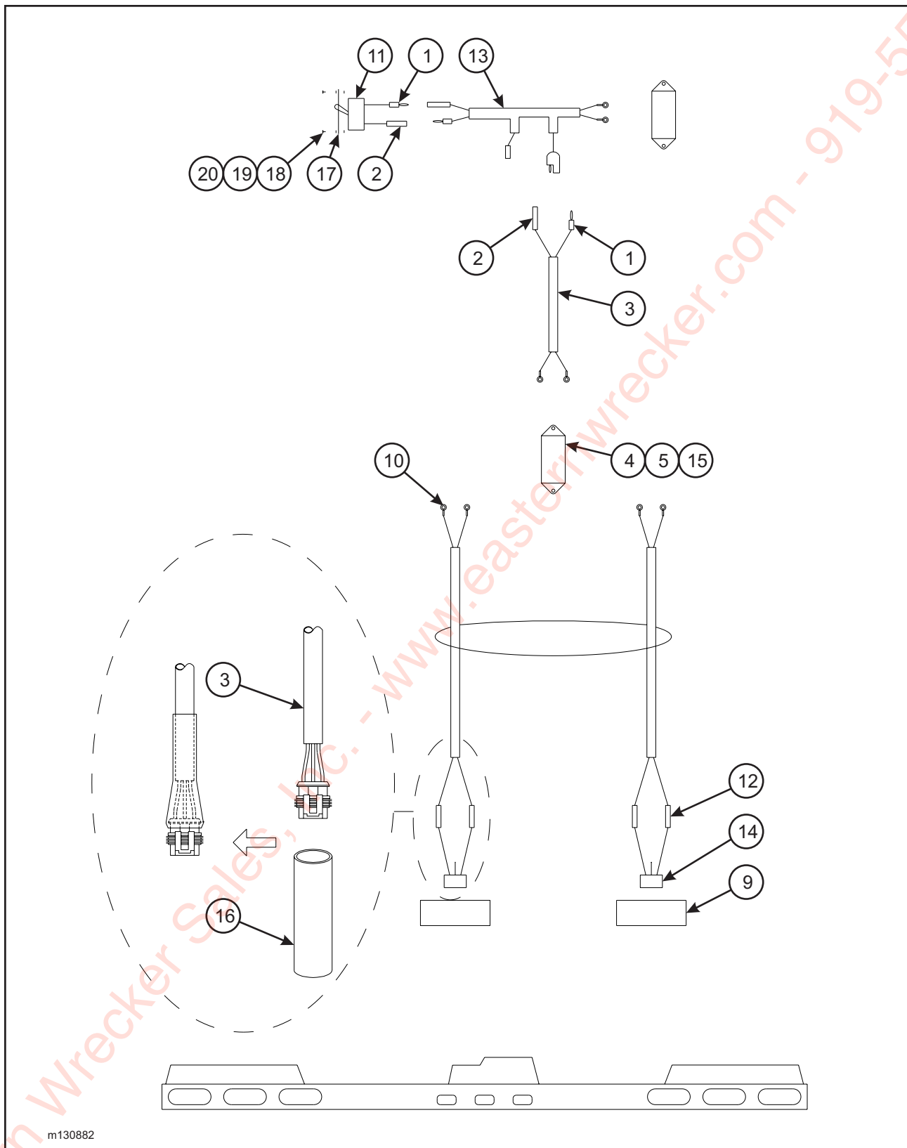
Figure 1-68 Rear Strobe Light Installation (Option)
