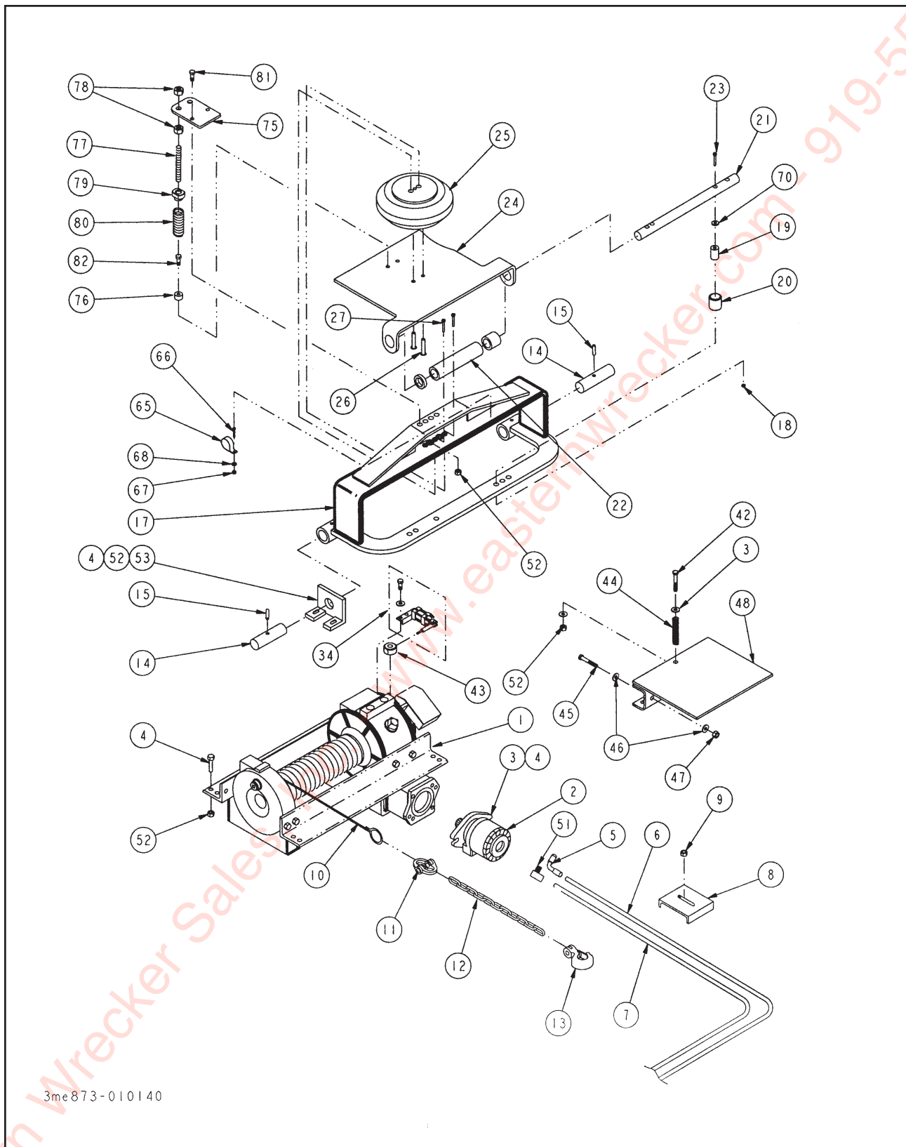
Figure 1-24 12K & 20K Upper Deck Winch (Braden) (1 of 2)
