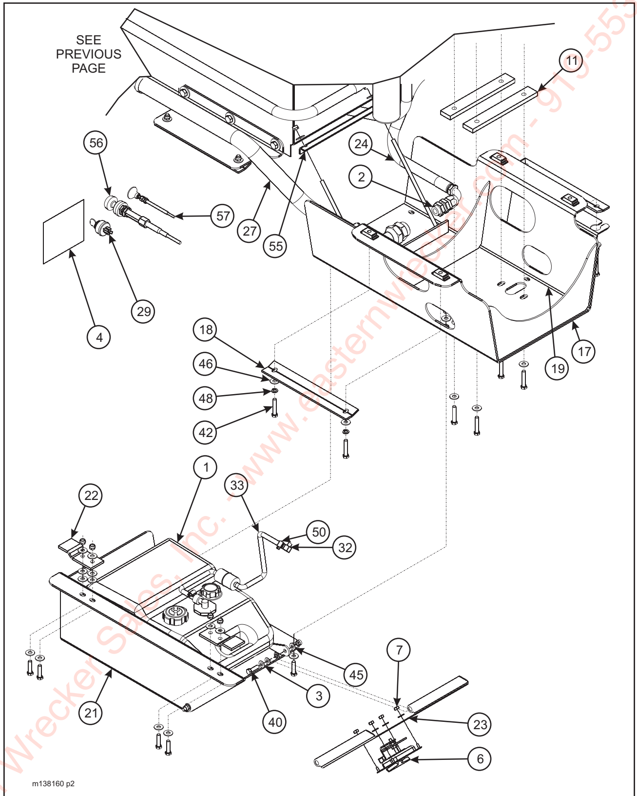
Figure 1-53 Hydraulic Engine, 27HP Slope (2 of 2)
