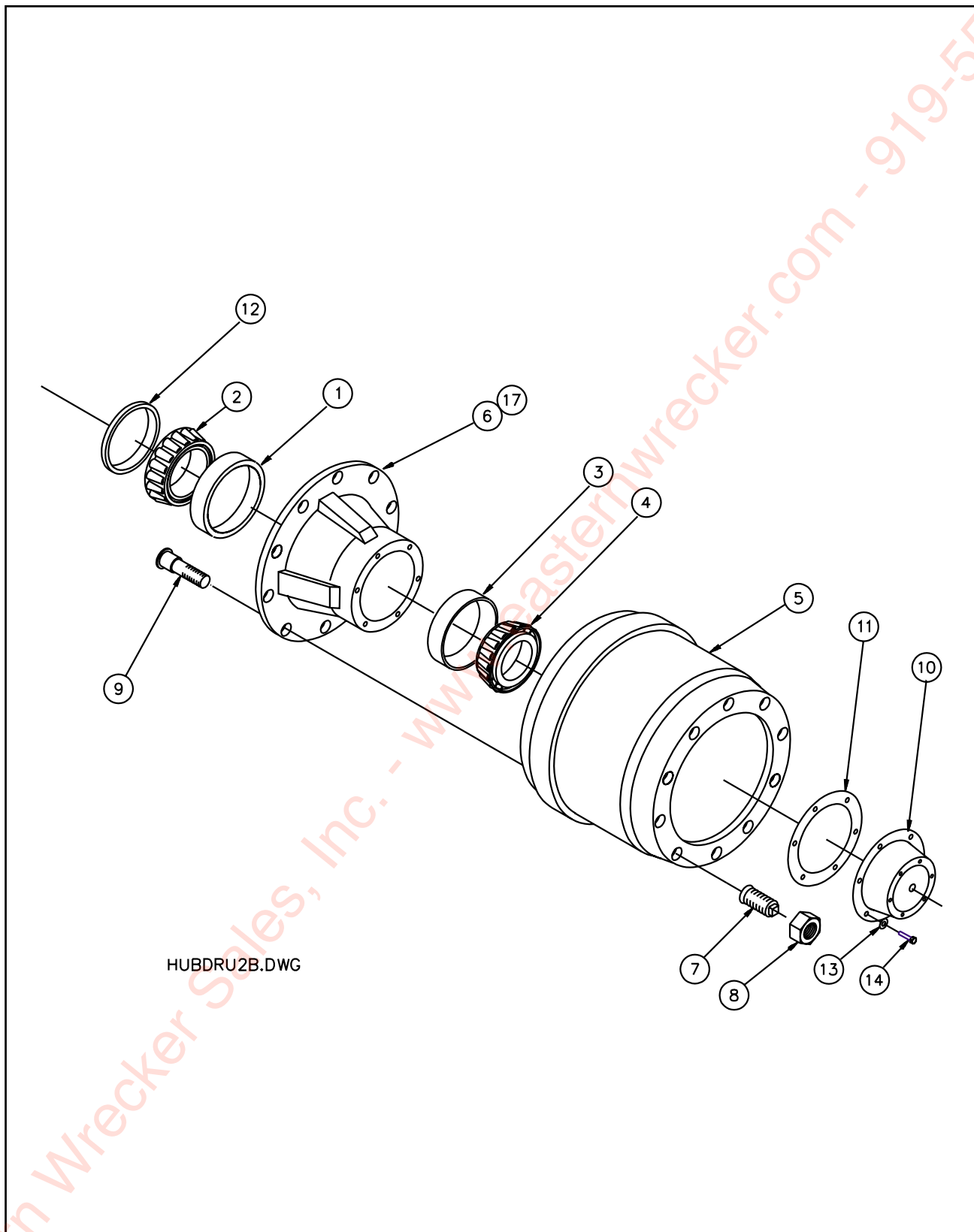
Figure 1-24 Outboard Ball Seat Mount Hub and Drum
