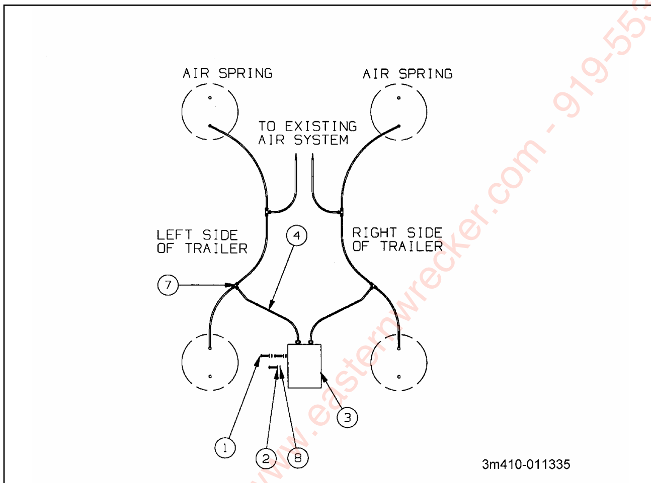
Figure 1-60 Scale-o-matic Installation (Optional)
