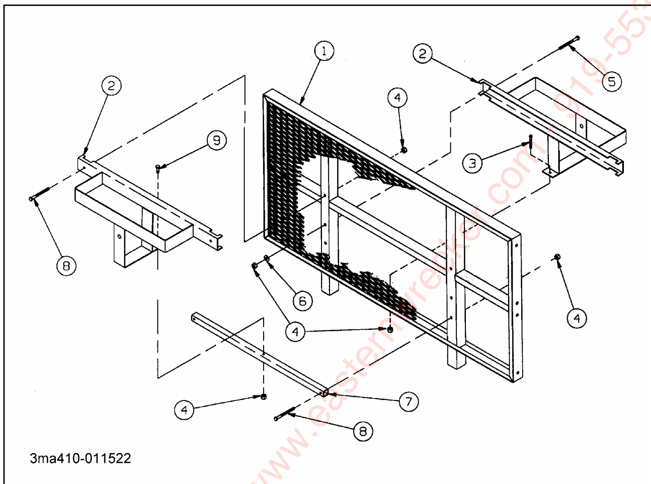
Figure 1-58 Spare Tire Carrier (Optional)
