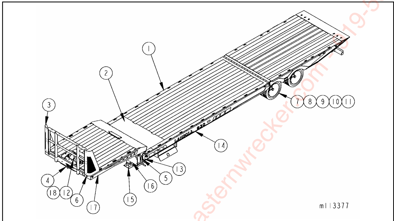
Figure 1-1 General Assembly
