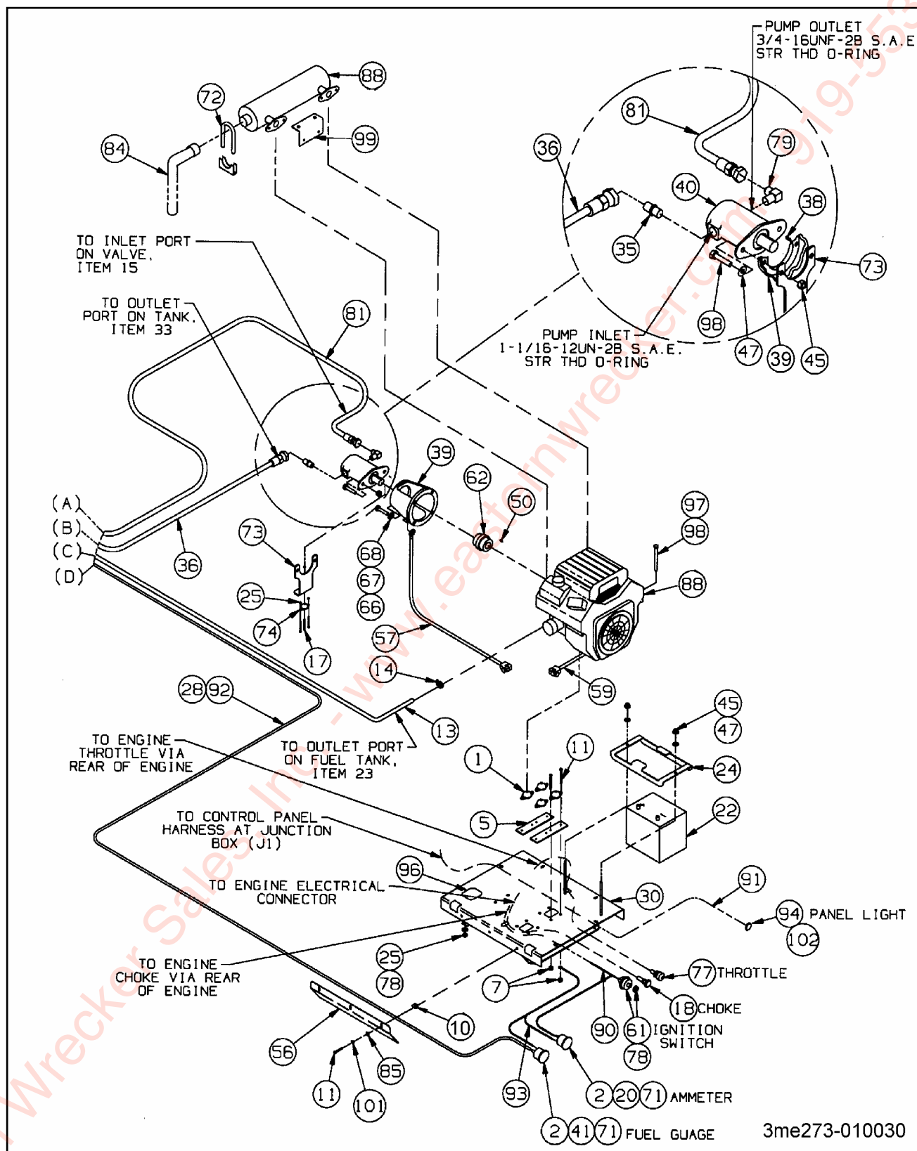
Figure 1-53 Hydraulic Engine, Split Mount (2 of 2)
