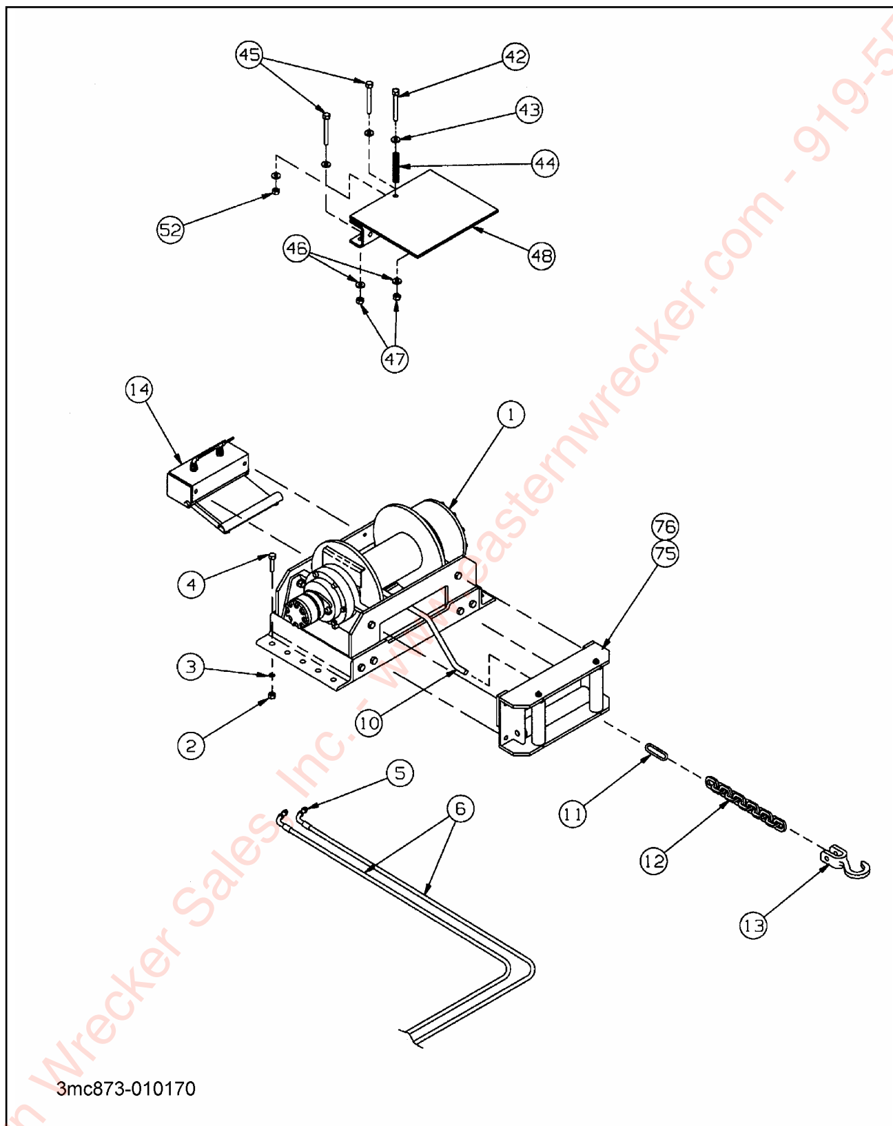
Figure 1-33 30K Upper Deck Winch (DP) (1 of 2)
