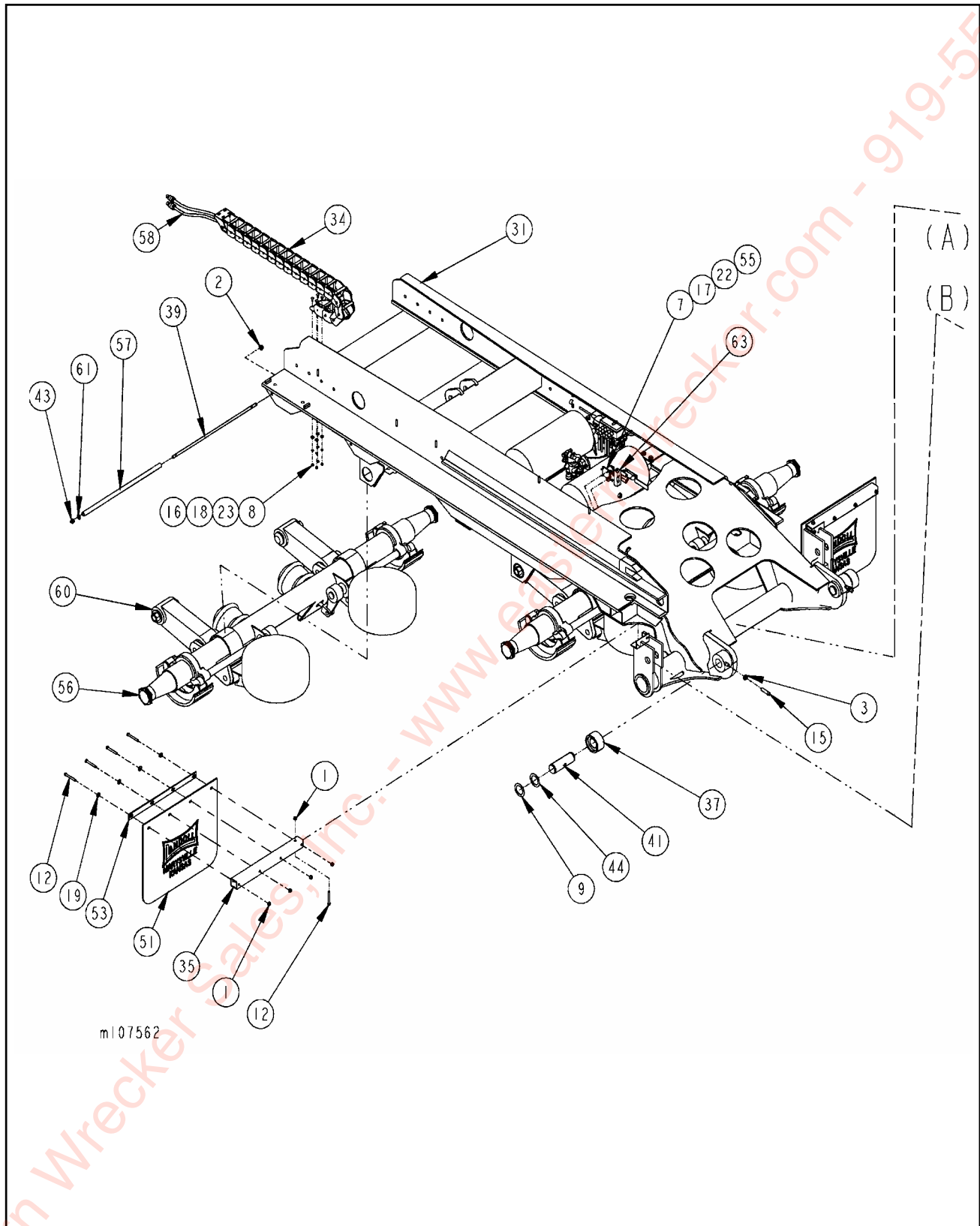
Figure 1-11 U/C Assembly, Air Ride Suspension, Tandem (1 of 2)
