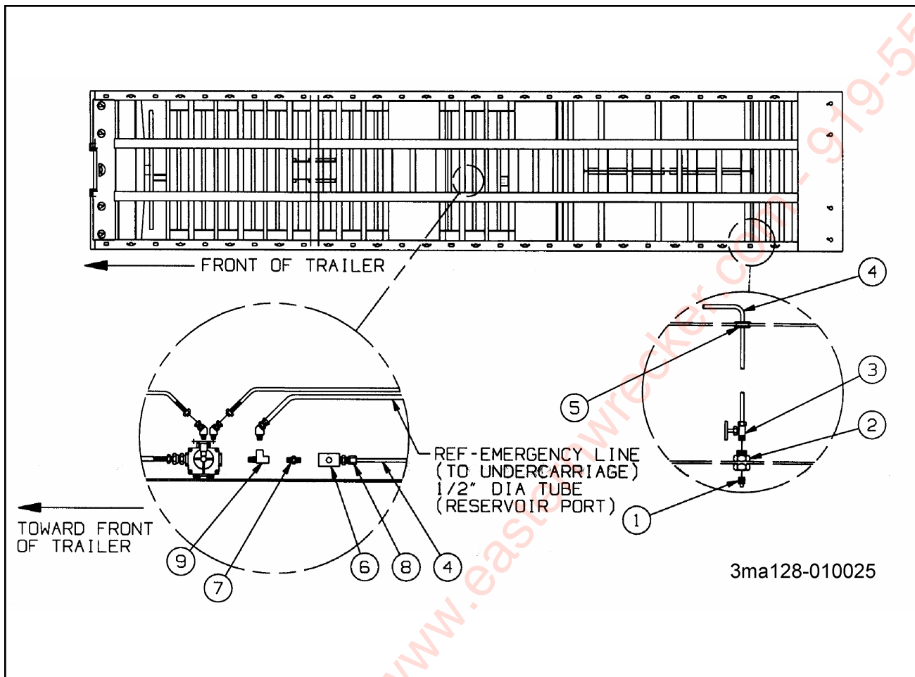
Figure 1-59 Air Outlet Assembly (Optional)
