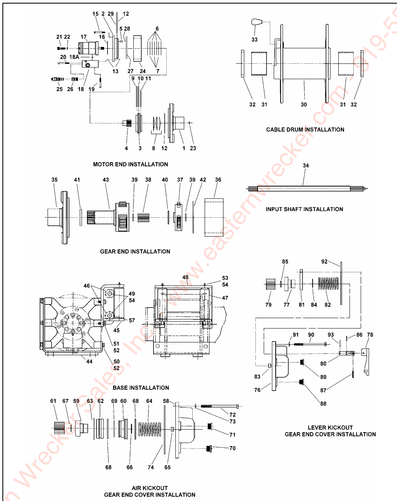
Figure 1-40 12K, 15K, & 20K Winch Items (DP Planetary)
