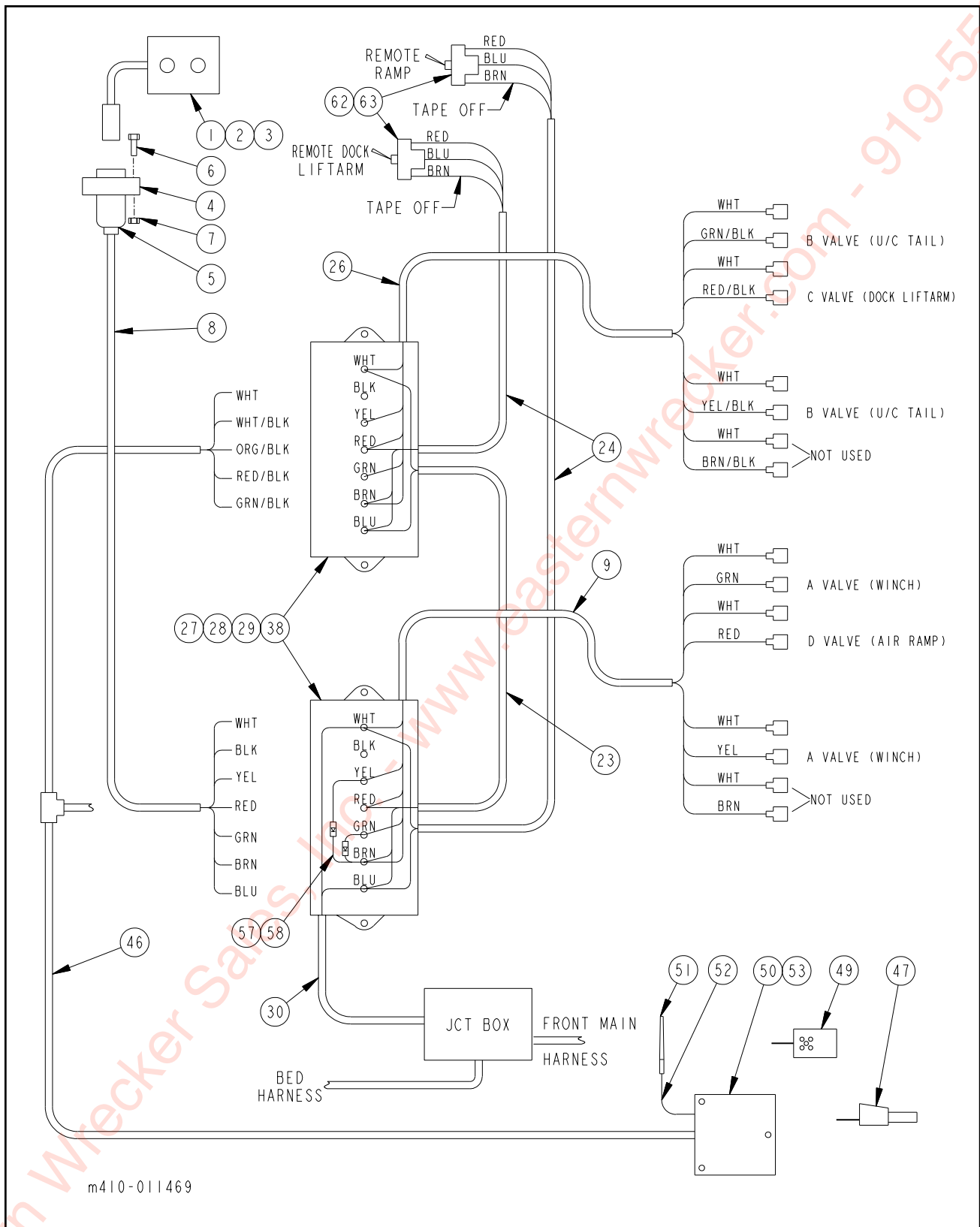
Figure 1-41 Remote Control Items (1 of 2)
