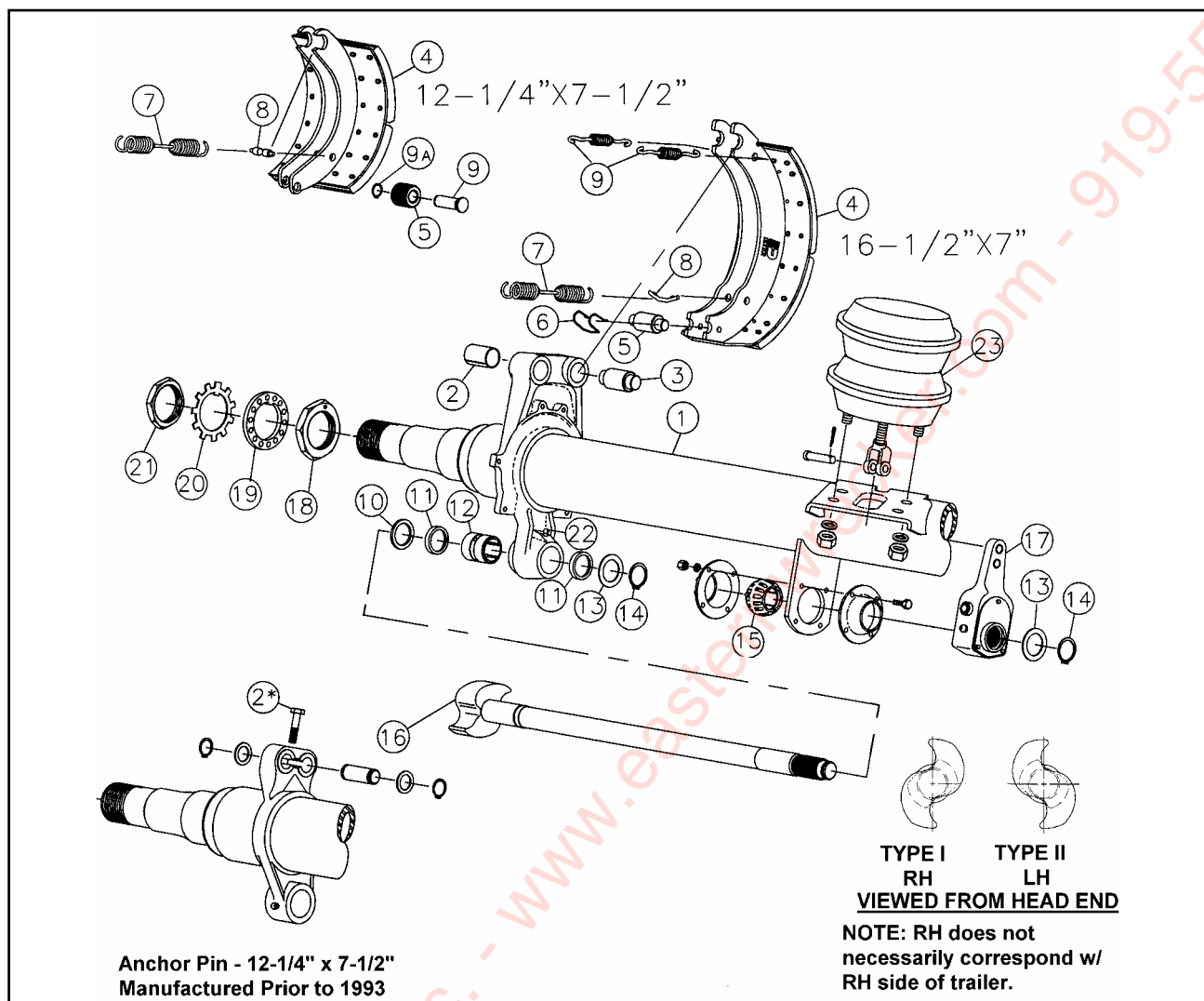
Figure 1-17 Axle and Brake Assembly
