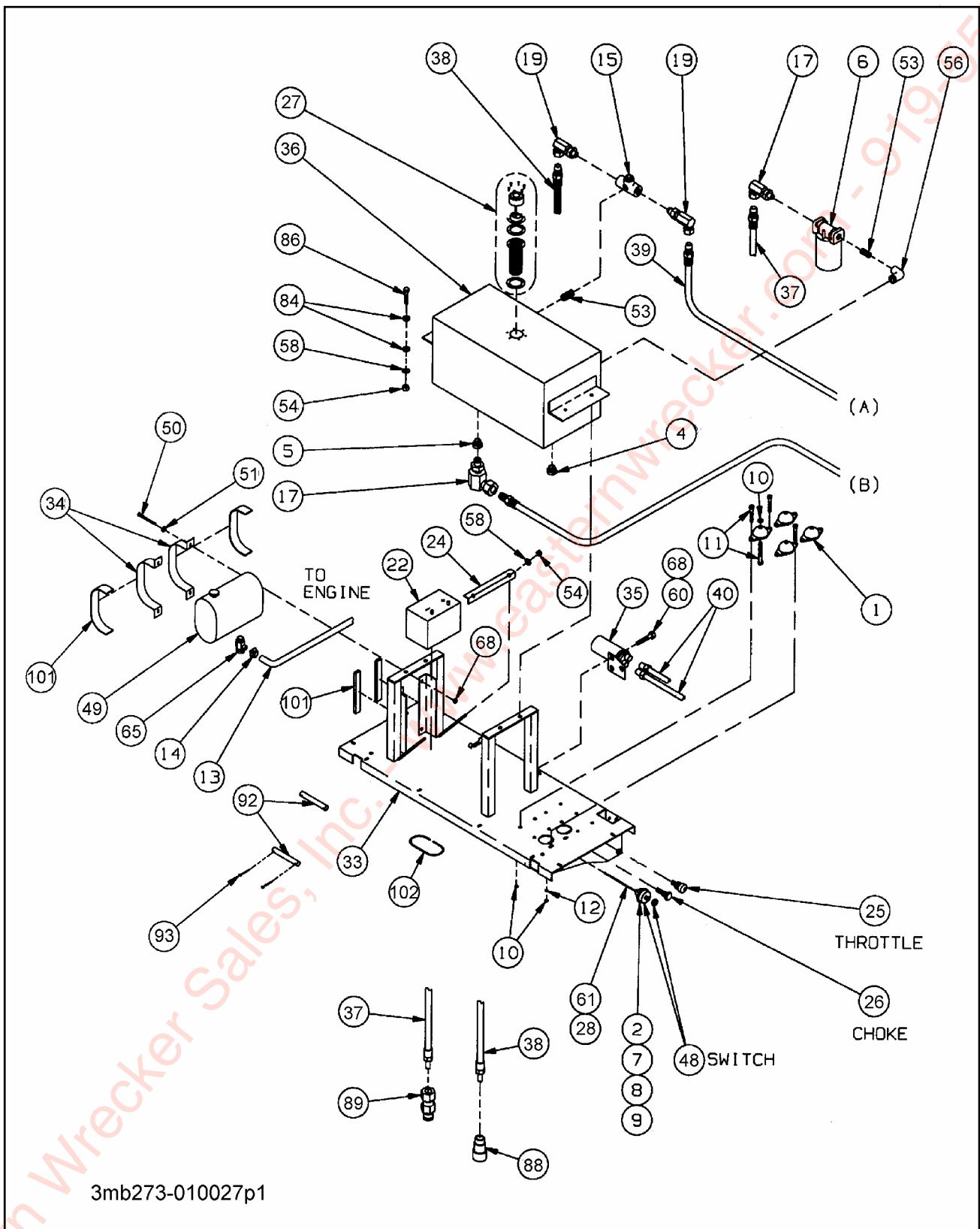
Figure 1-55 Hydraulic Engine, Front Mount (1of 2)
