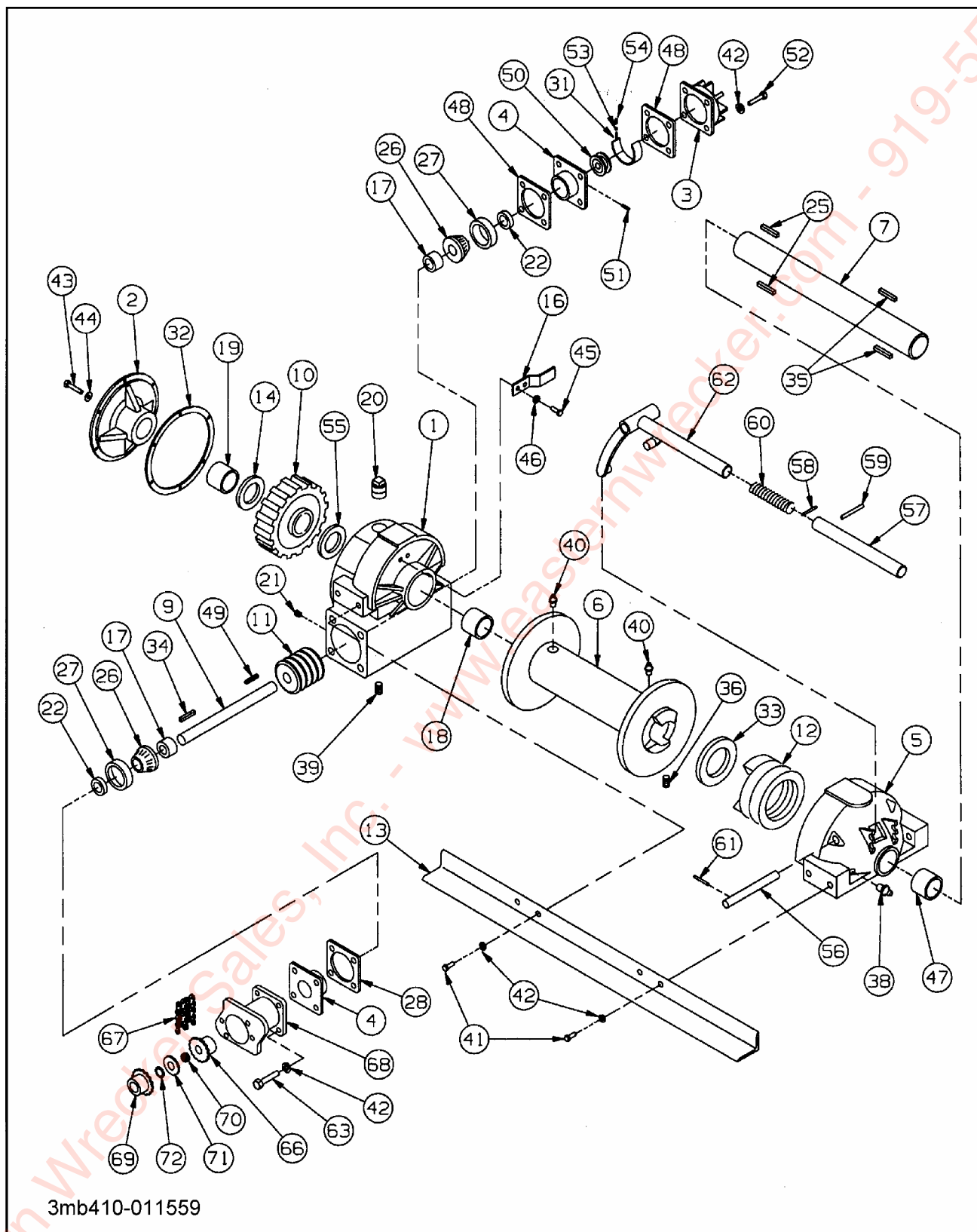
Figure 1-29 12,000# Winch Items (Braden Worm Gear)
