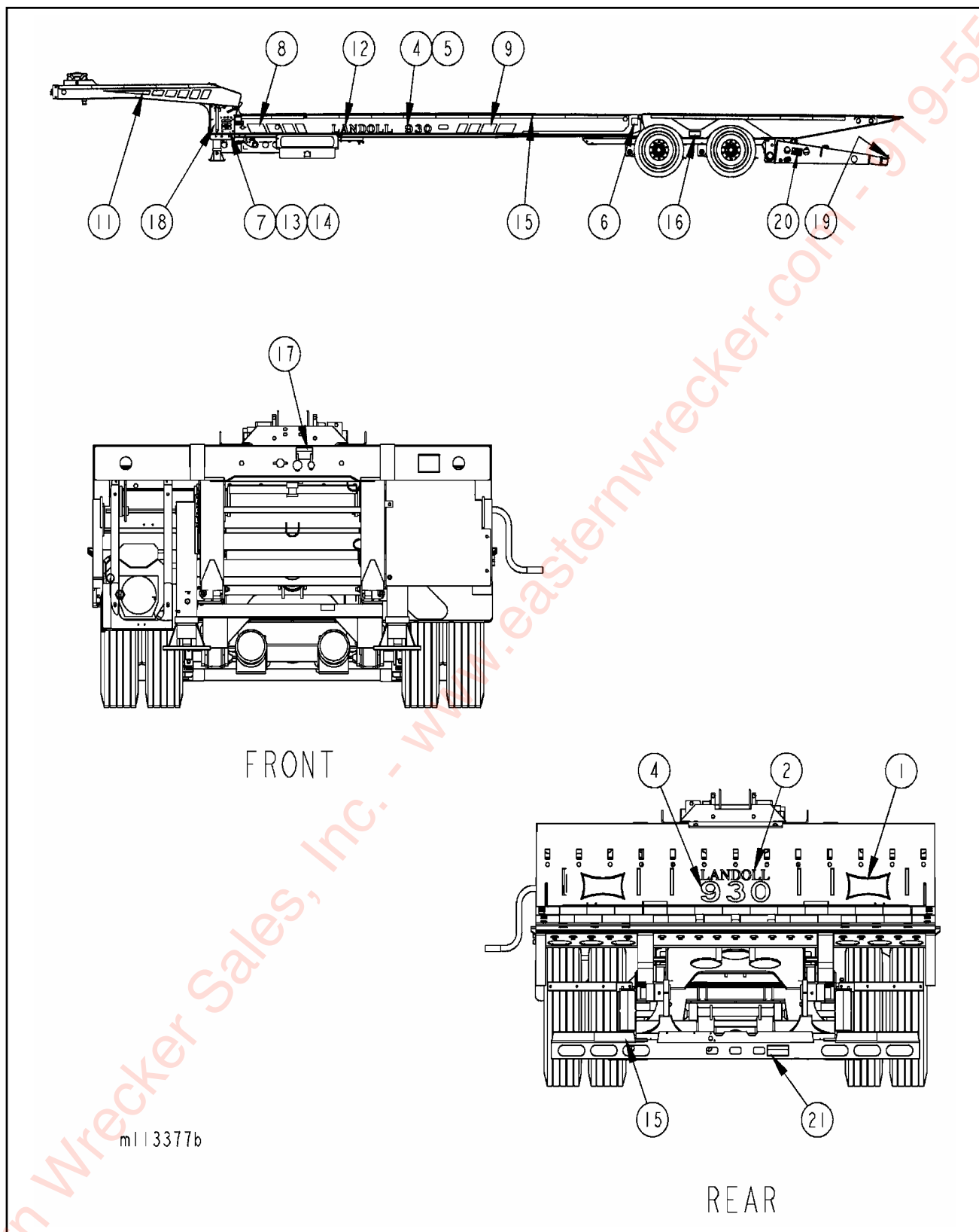
Figure 1-47 Decal Placement
