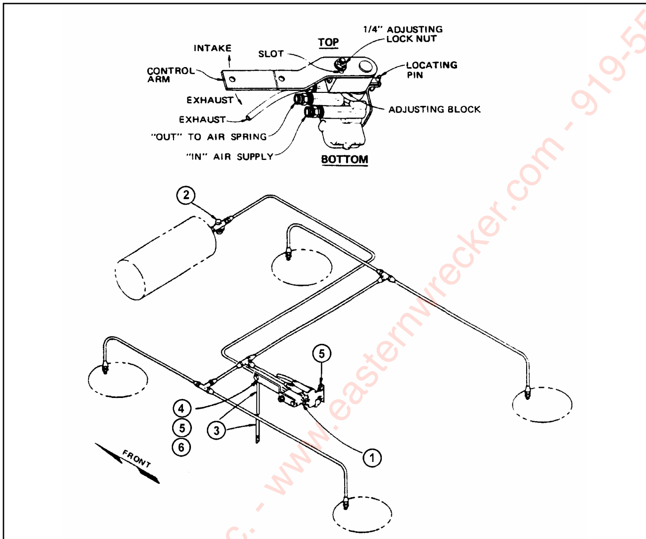
Figure 1-15 Air Control Kit
