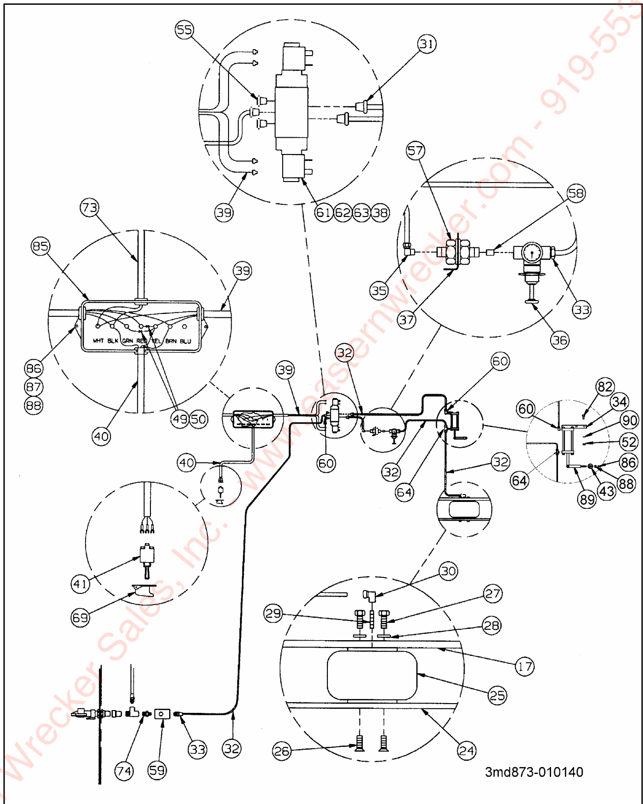
Figure 1-27 12K & 20K Upper Deck Winch (Braden) (2 of 2)
