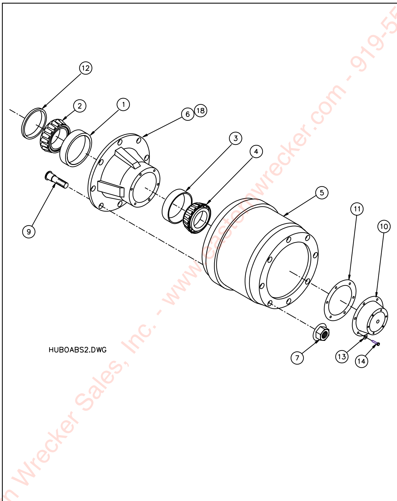
Figure 1-25 Outboard Pilot Mount Hub and Drum
