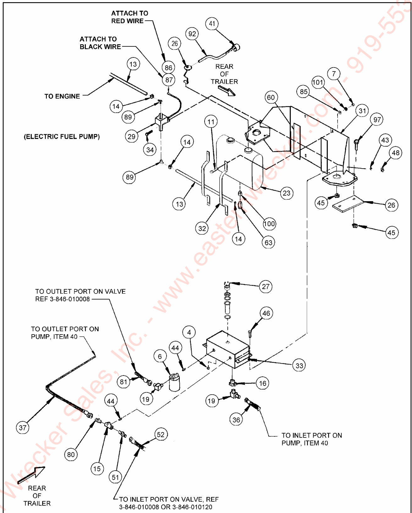
Figure 1-51 Hydraulic Engine, 22HP Slope (2 of 2)
