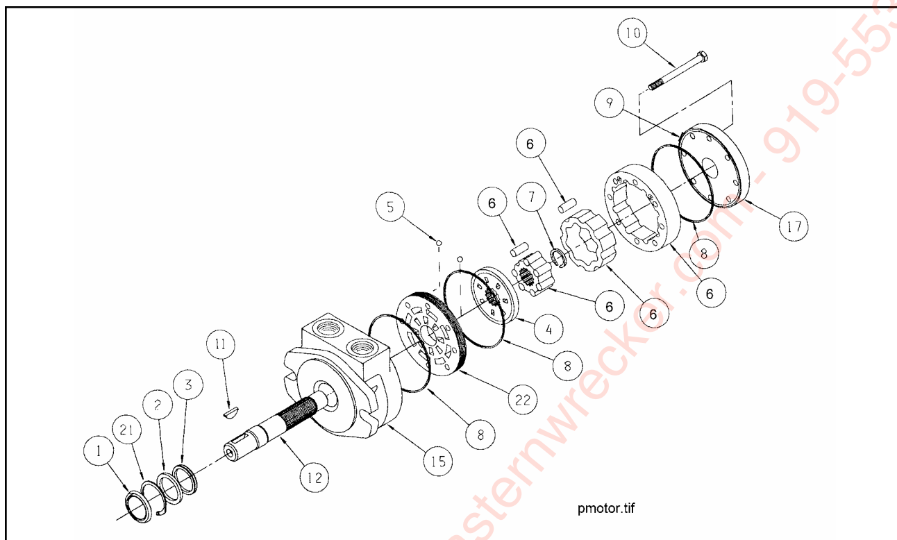
Figure 1-32 Winch Motor Assembly
