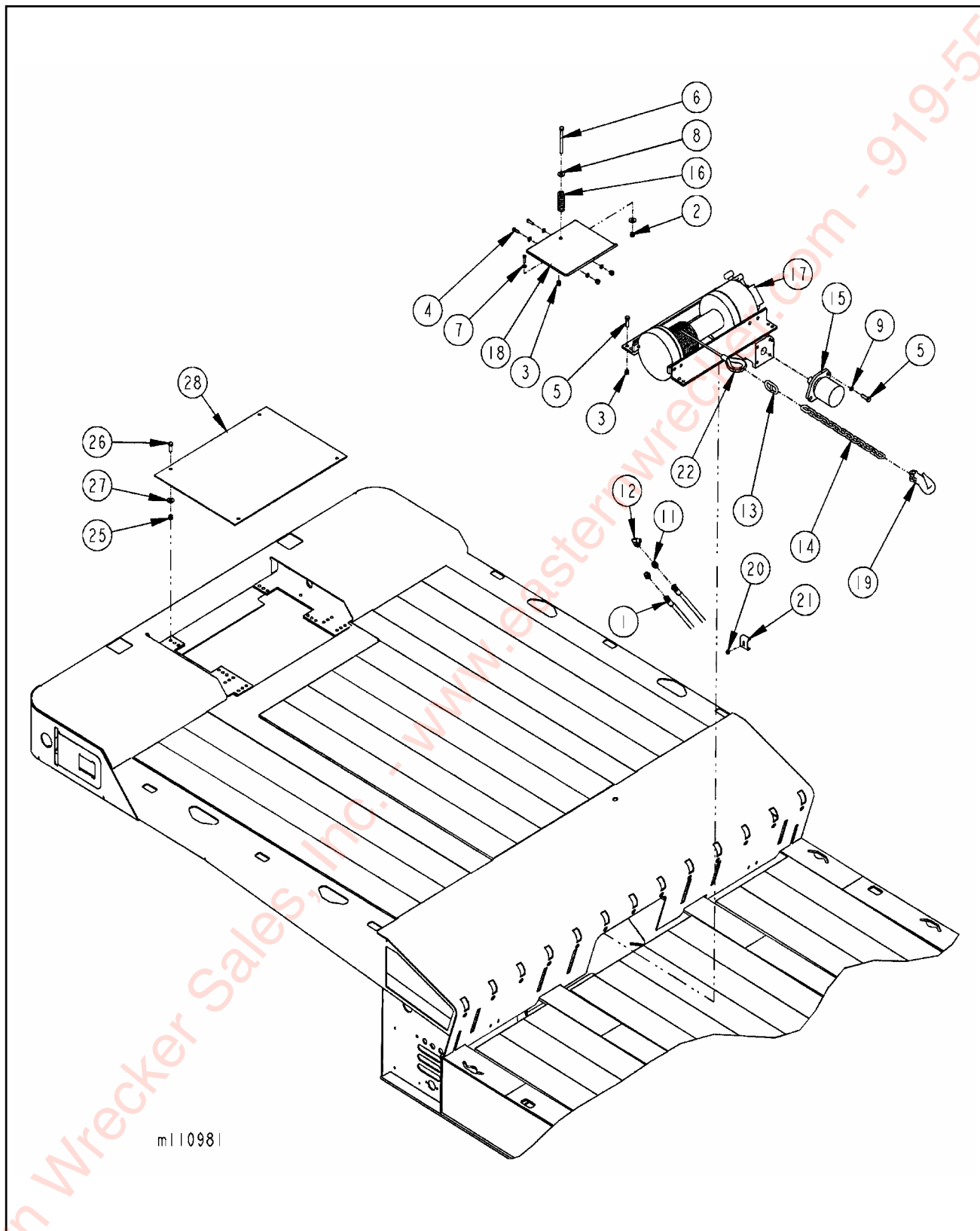
Figure 1-28 12K & 20K Slope Winch (Braden)
