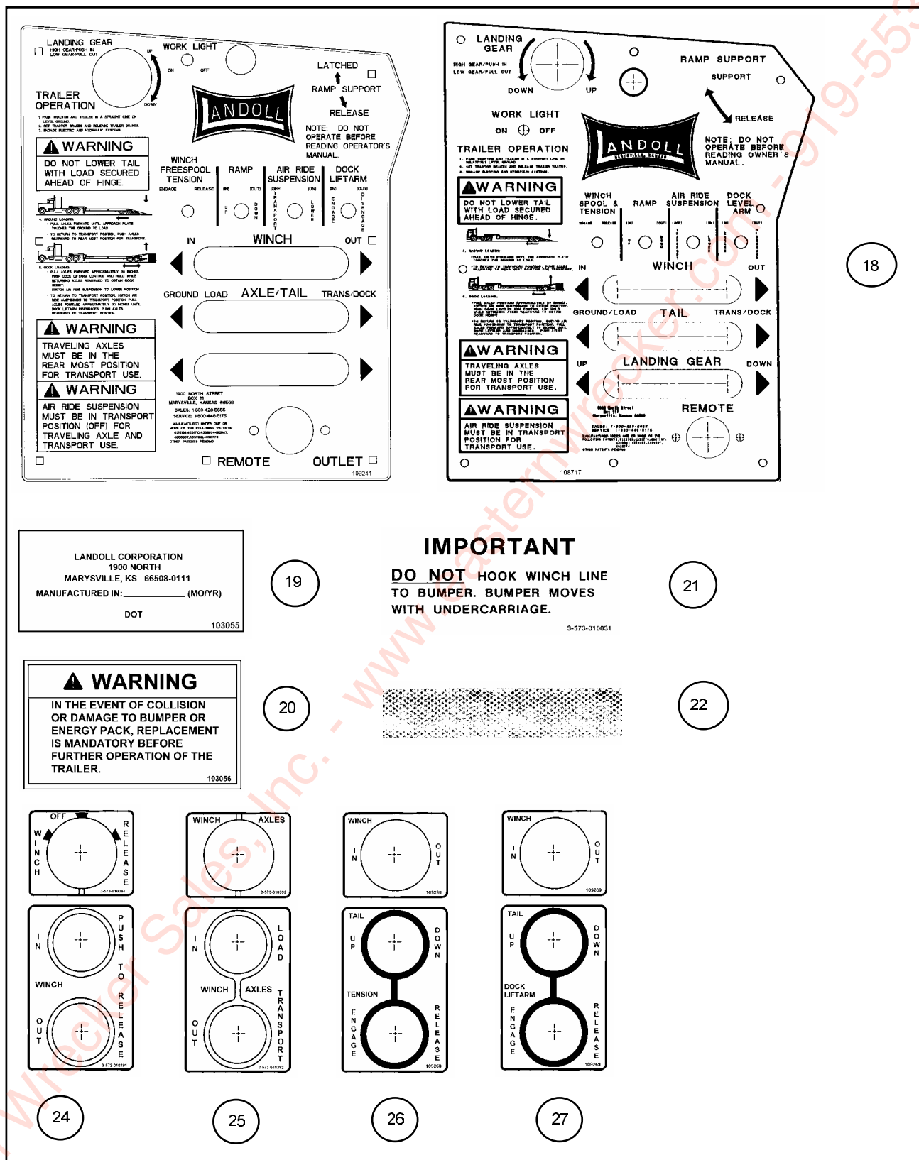
Figure 1-46 Decals
