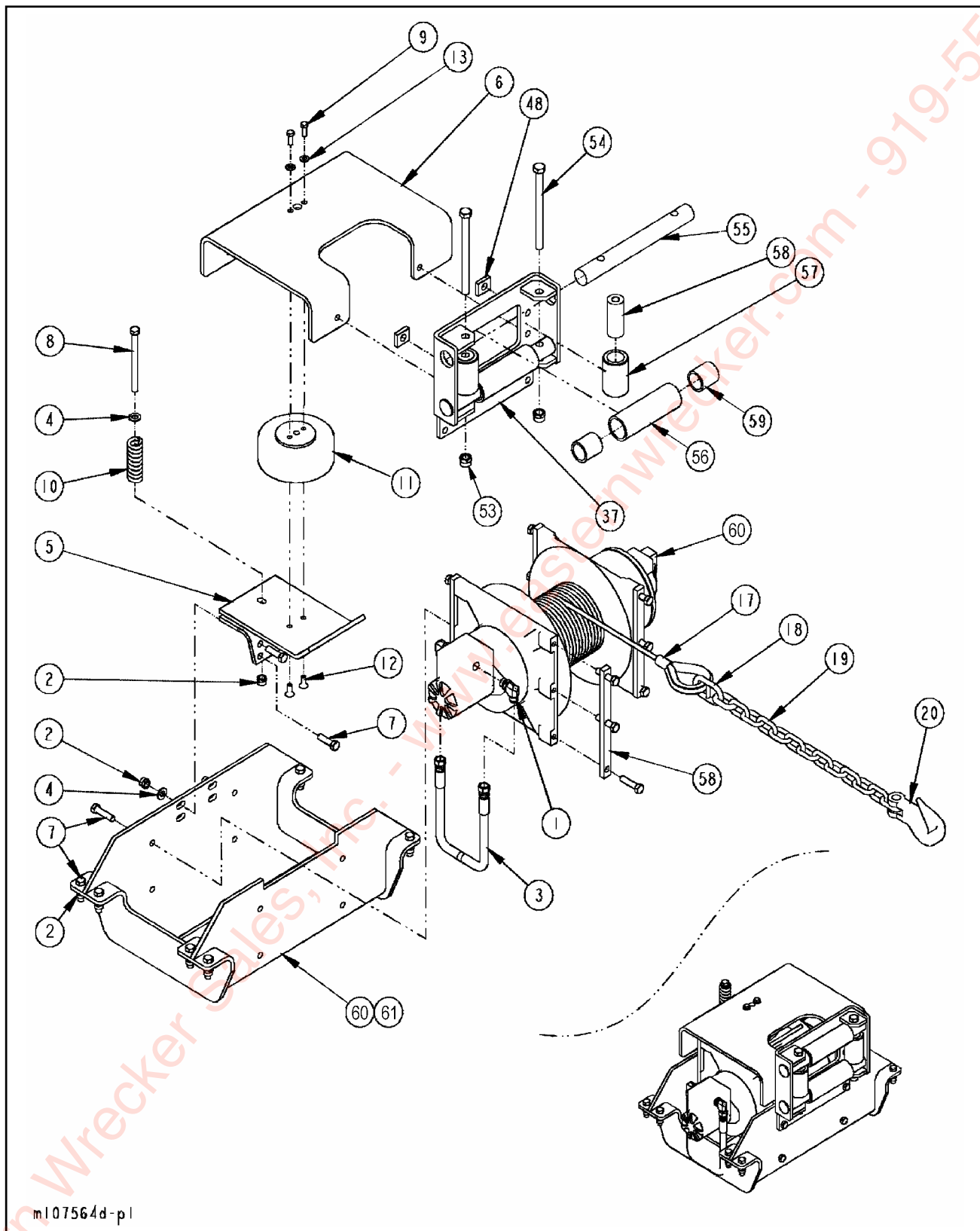
Figure 1-38 12K, 15K, & 20K Upper Deck Winch (DP) (1 of 2)
