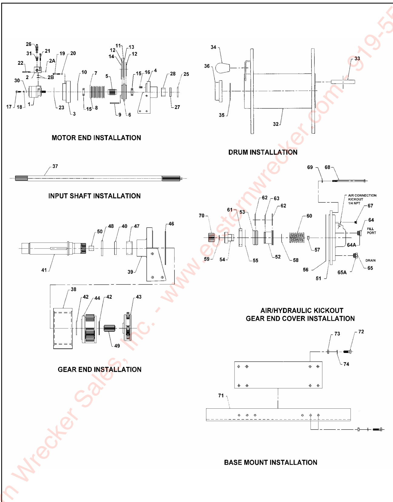
Figure 1-35 30,000# Winch Items (DP Planetary)
