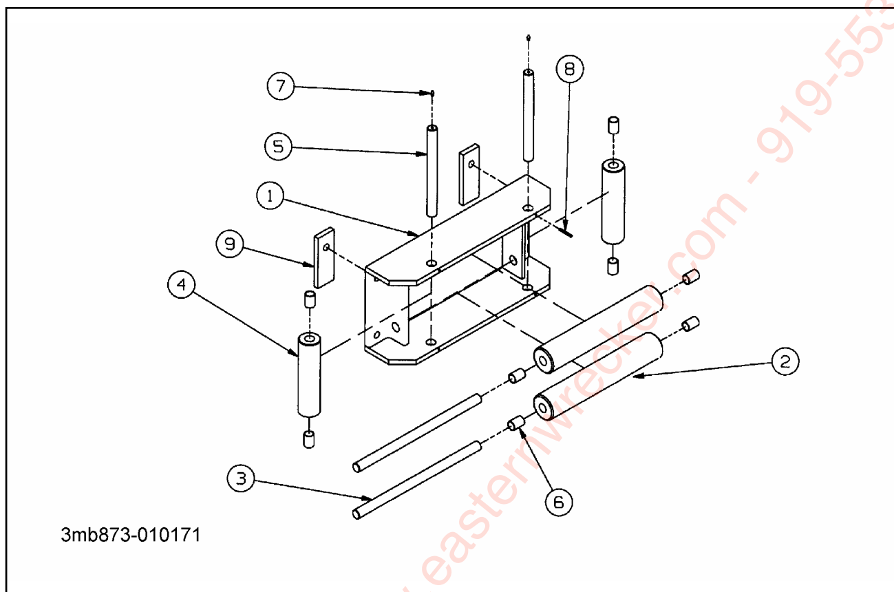
Figure 1-36 Winch Roller Guide - 30K
