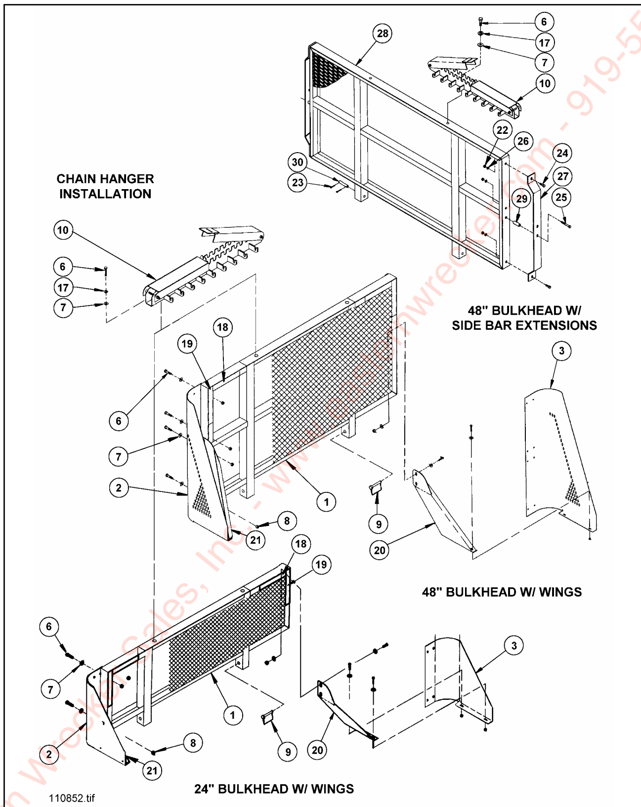
Figure 1-5 Bulkhead Assembly
