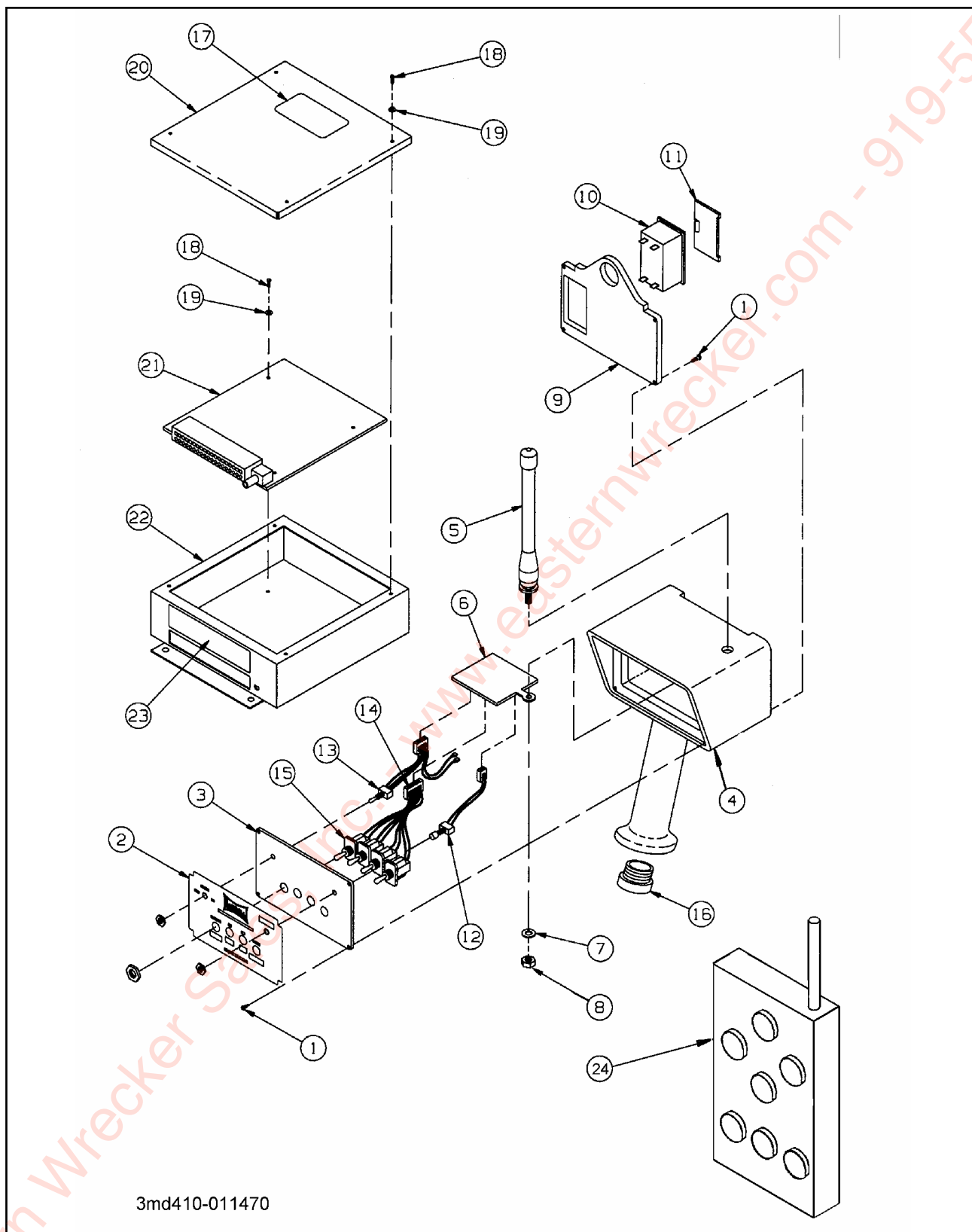
Figure 1-44 Wireless Remote Control
