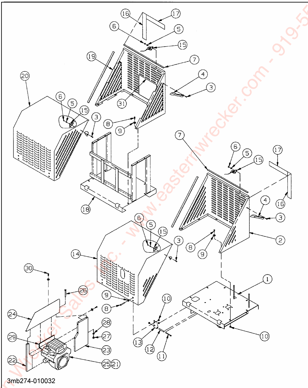
Figure 1-54 Engine Cover, Split Mount
