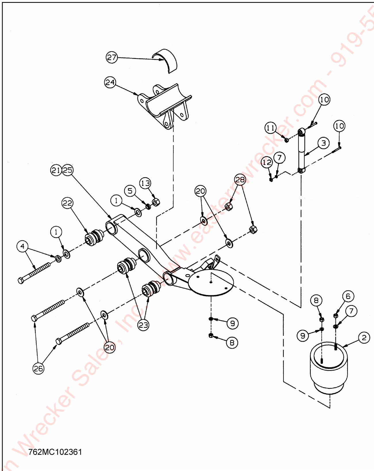
Figure 1-18 Suspension Hanger RLU-228
