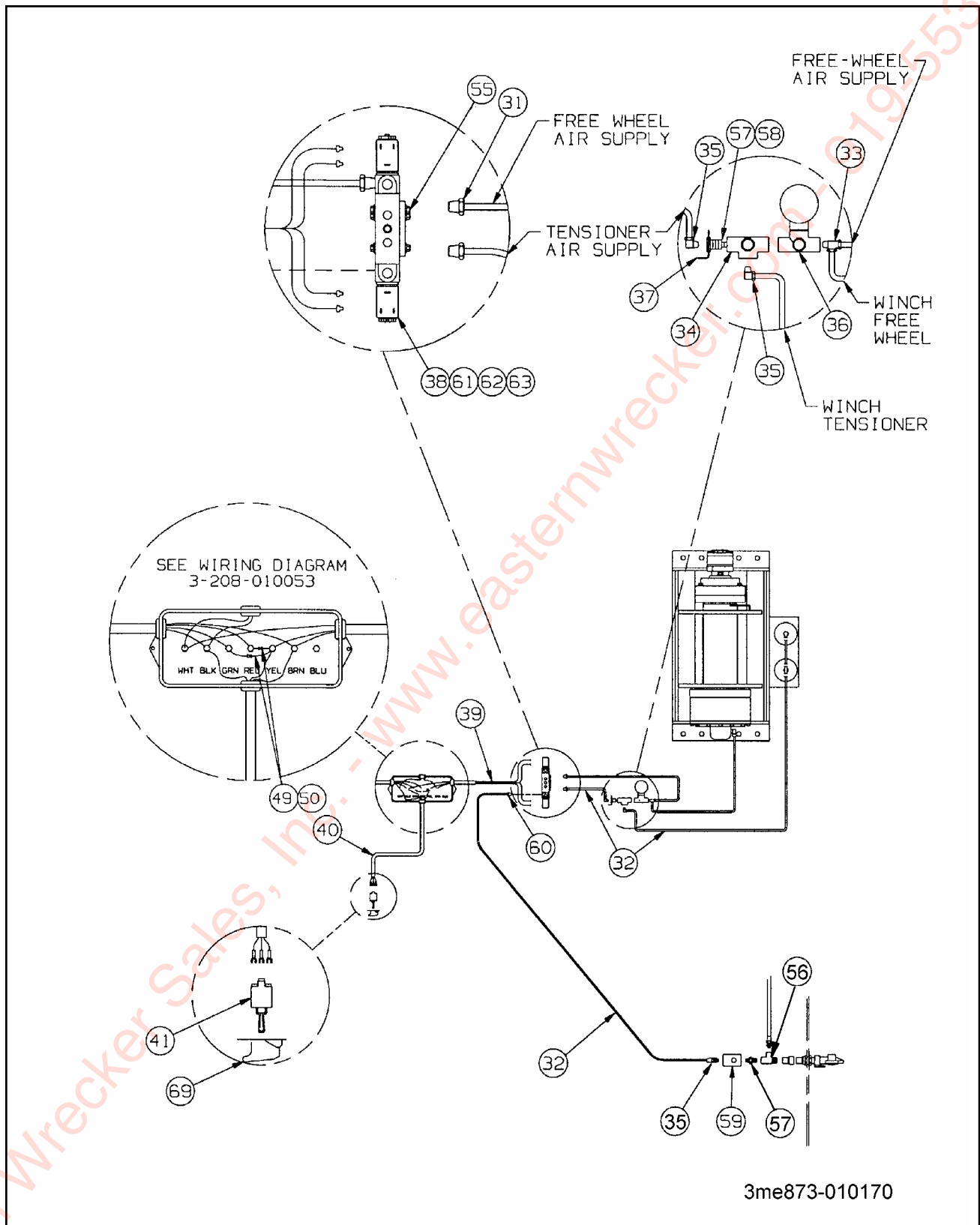
Figure 1-34 30K Upper Deck Winch (DP) (2 of 2)
