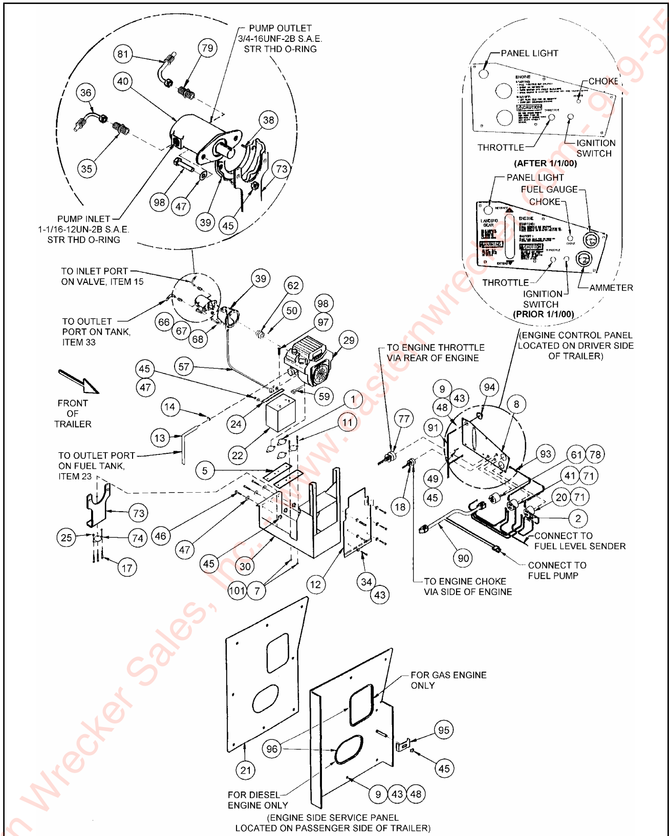
Figure 1-50 Hydraulic Engine, 22HP Slope (1 of 2)
