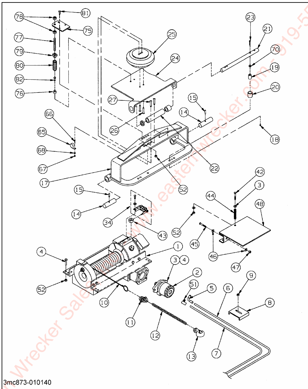
Figure 1-26 12K & 20K Upper Deck Winch (Braden) (1 of 2)
