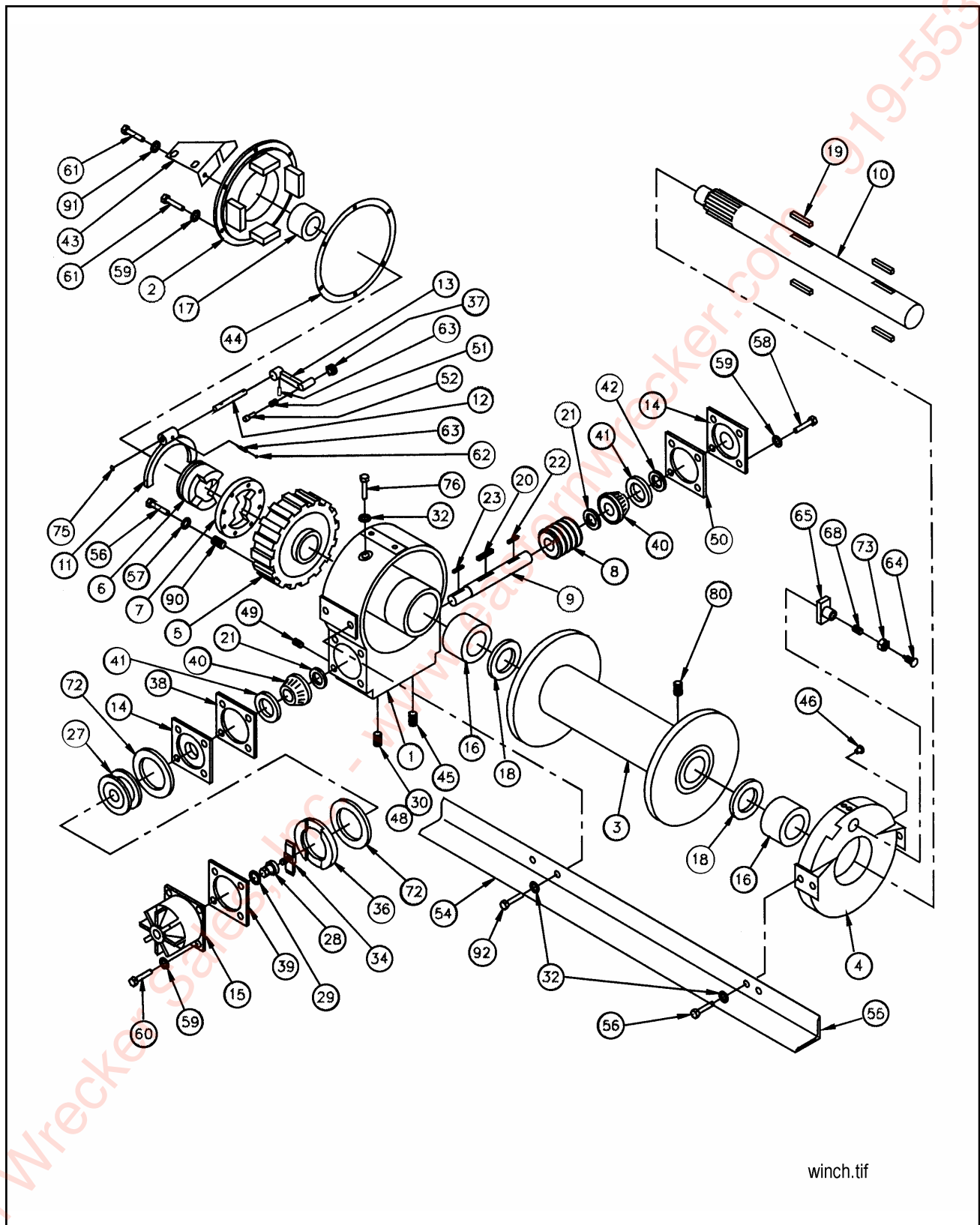
Figure 1-30 20,000# Winch Items (Braden Worm Gear)
