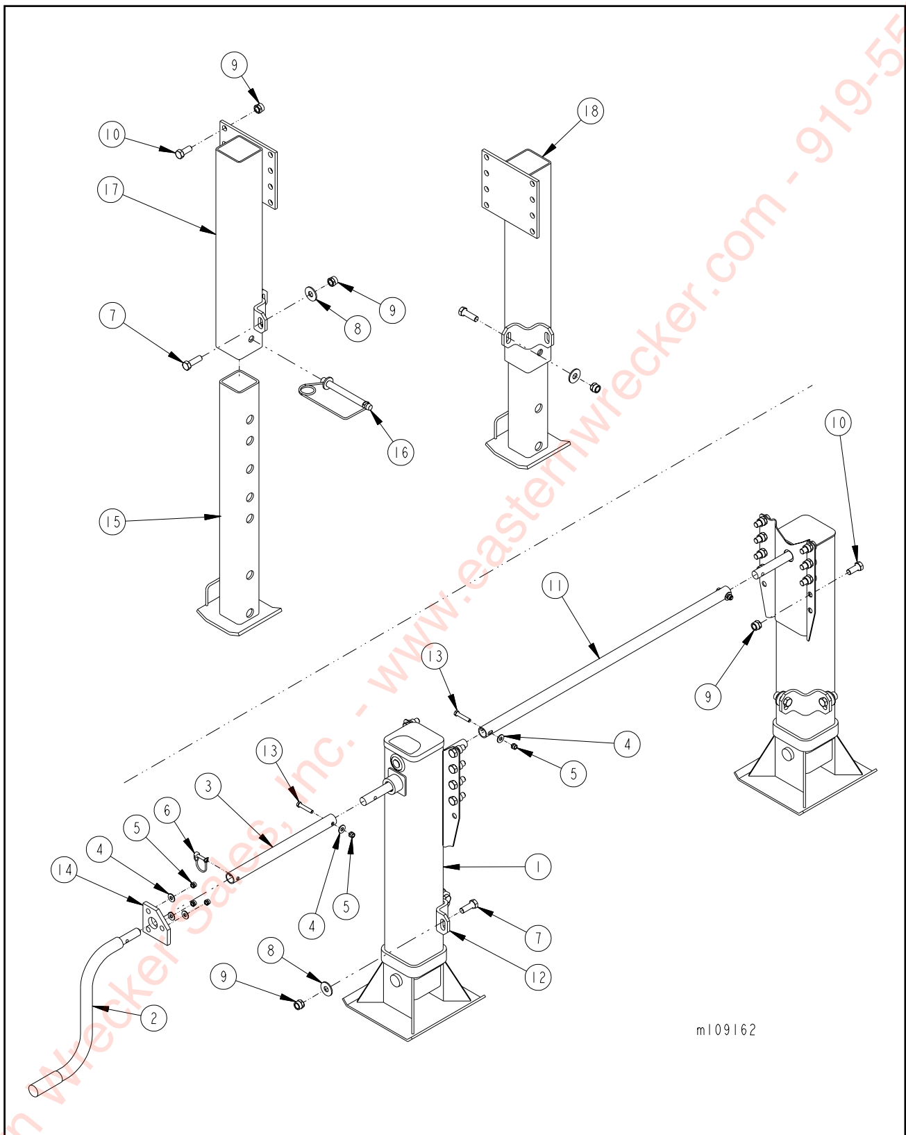
Figure 1-48 Landing Gear
