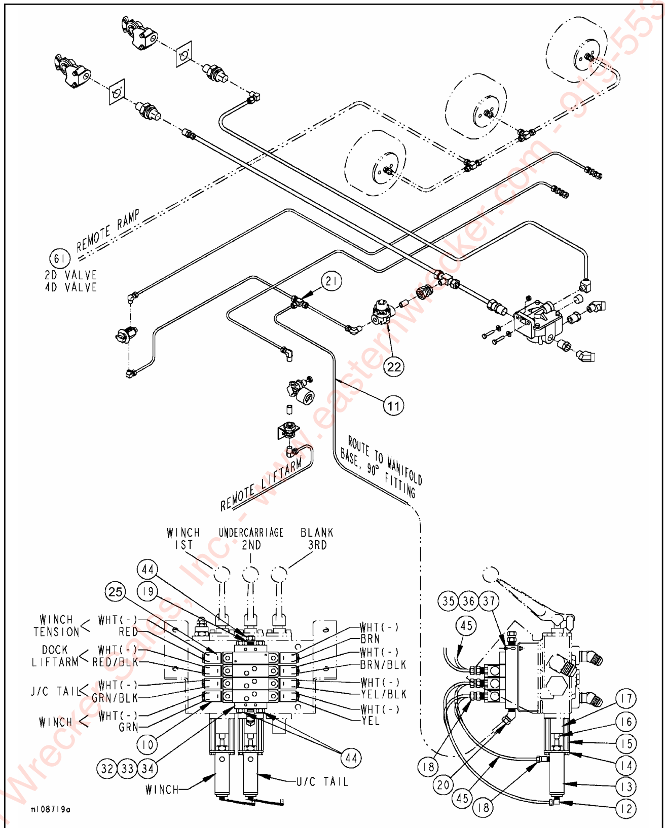
Figure 1-42 Remote Control Items (2 of 2)
