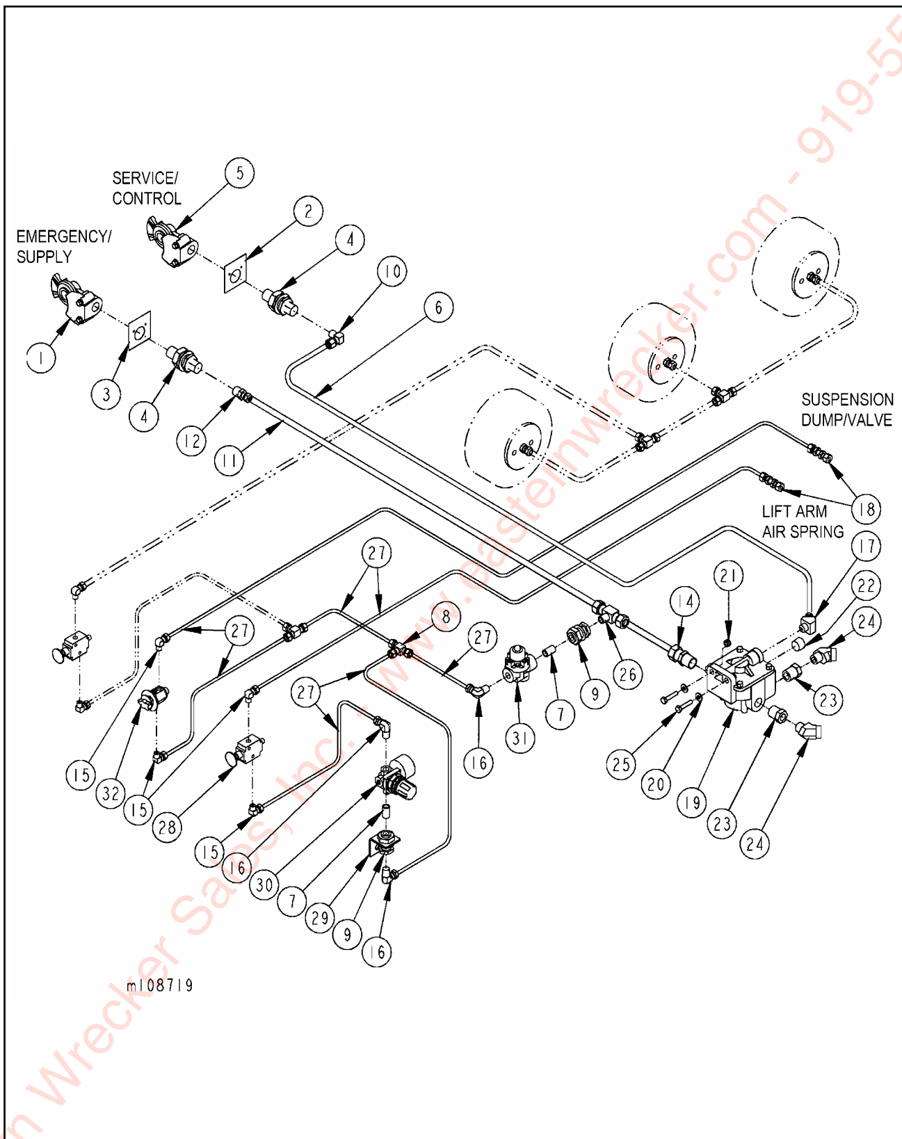
Figure 1-21 Air System ABS
