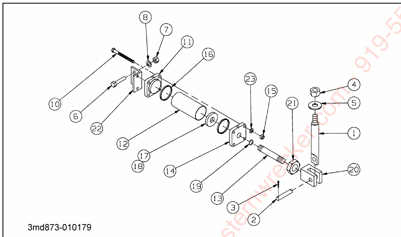
Figure 1-31 Winch Air Shift Cylinder for 20,000# Winch
