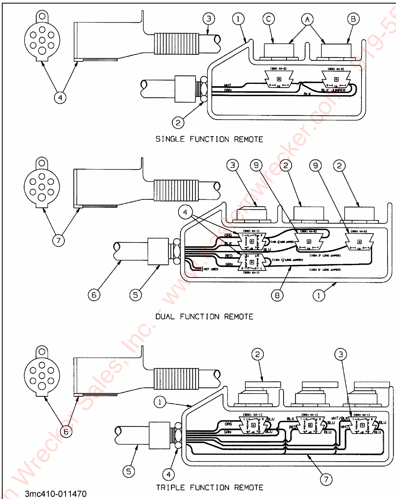
Figure 1-43 Wired Remote Control
