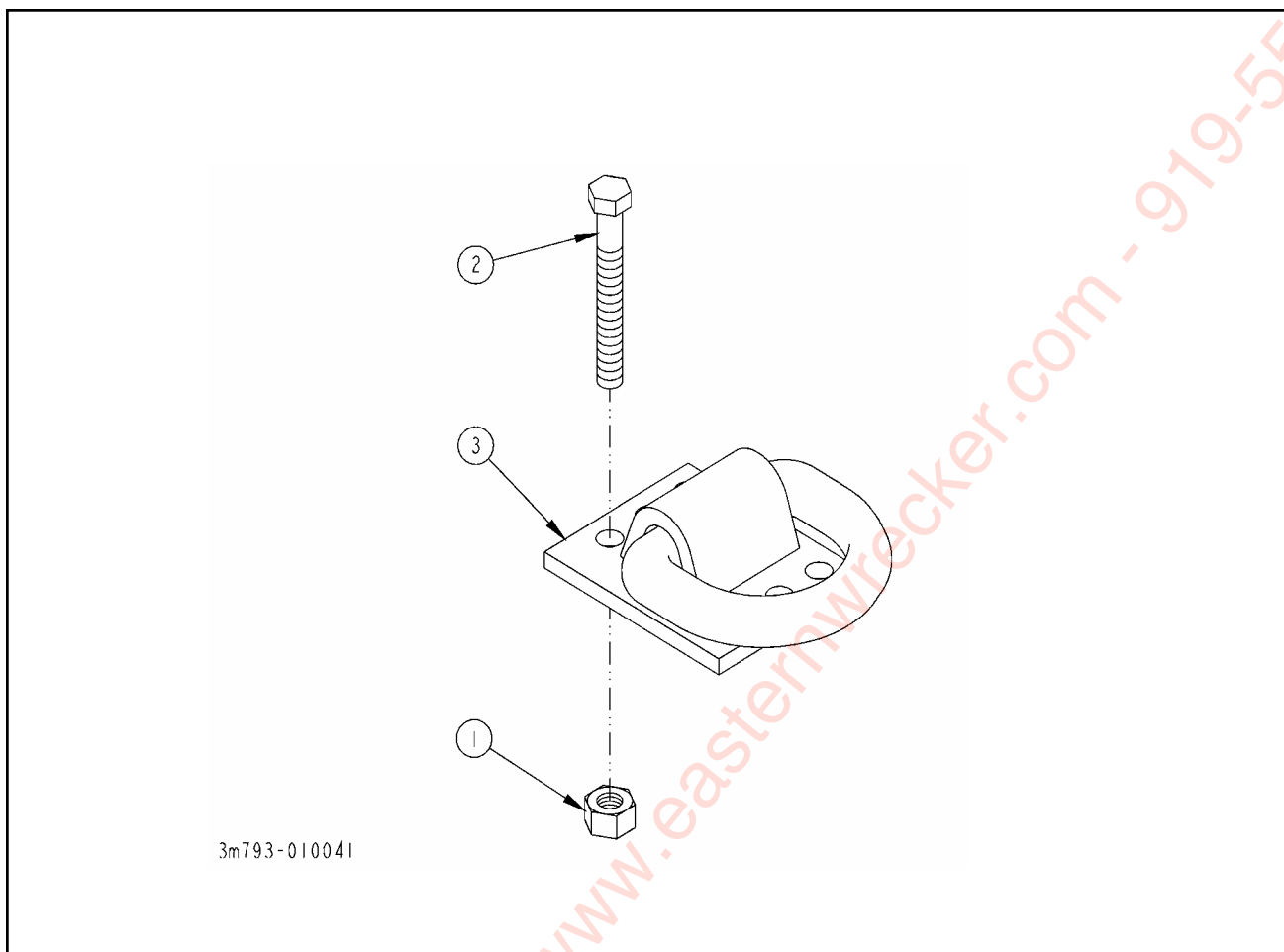
Figure 1-61 D-Ring Installations (Optional)
