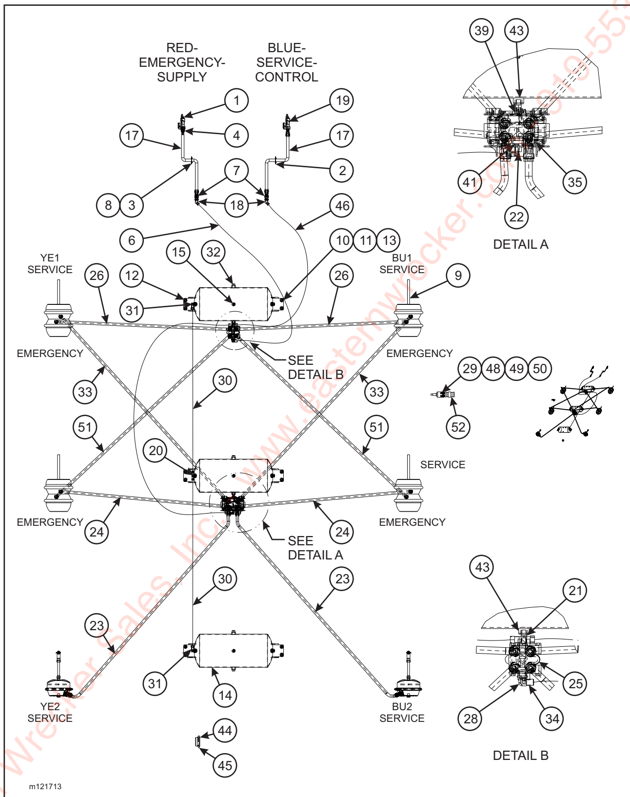
Figure 1-8 Air System (L5029)
