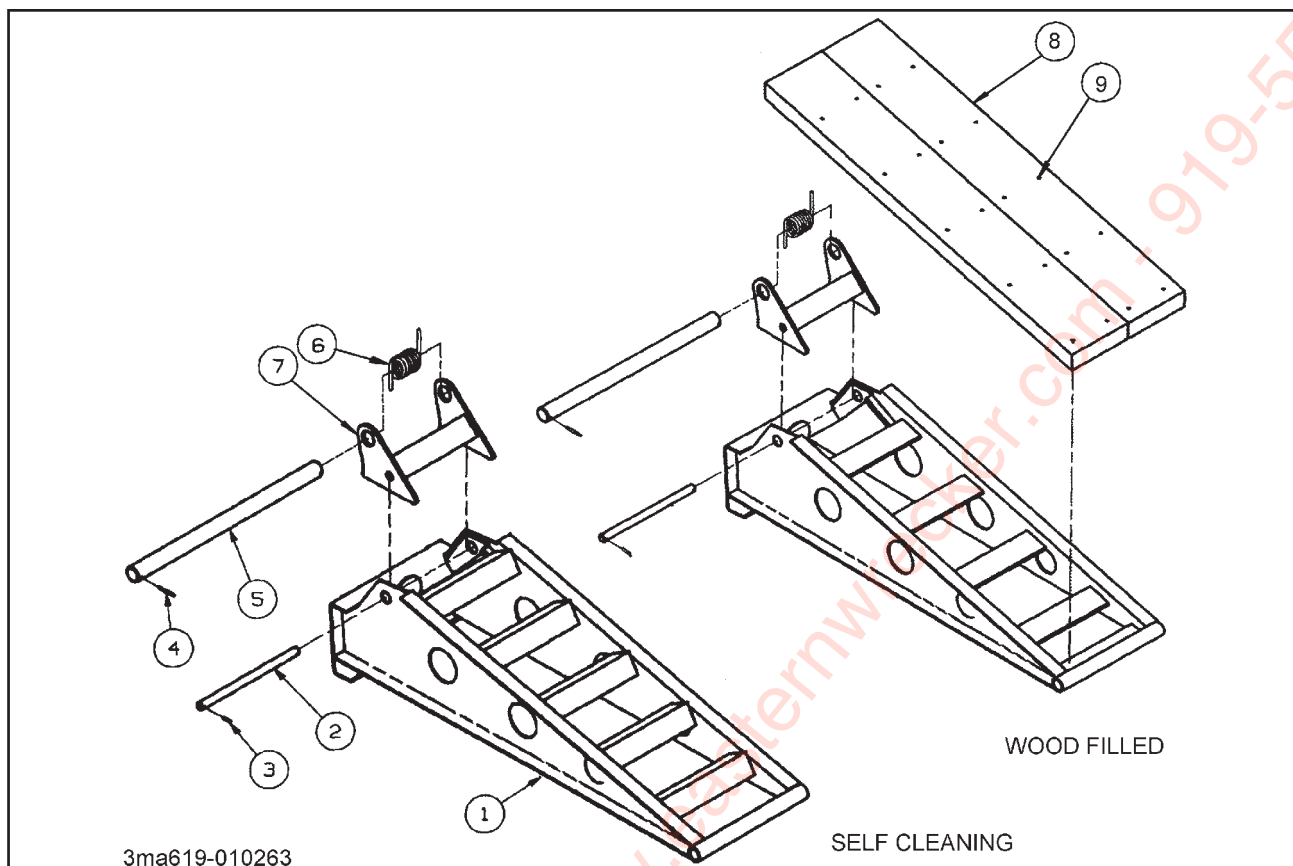
Figure 1-14 Ramp Assembly
