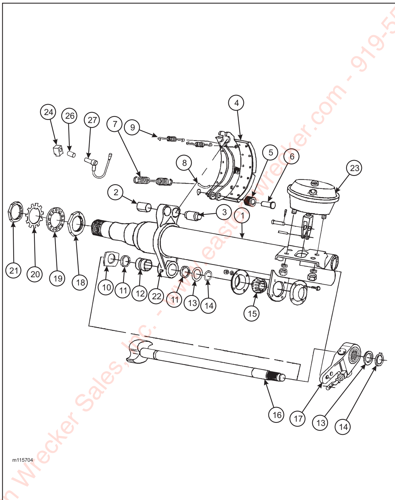
Figure 1-5 Axle and Brake Assembly
