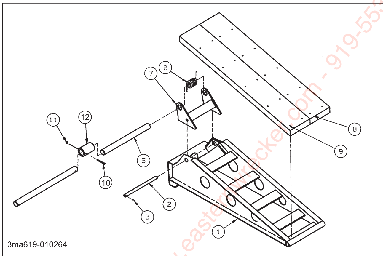
Figure 1-15 Ramp Assembly - Center (Option)
