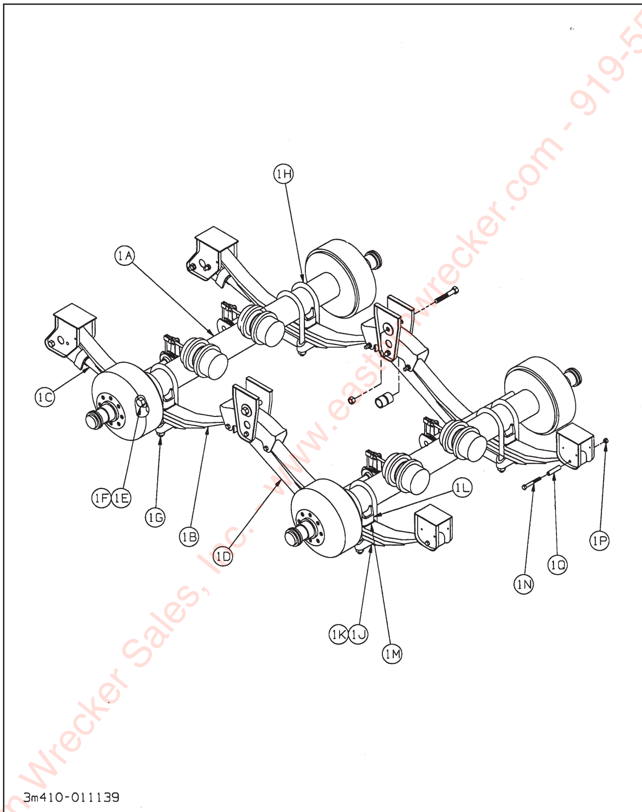
Figure 1-4 Suspension Assembly
