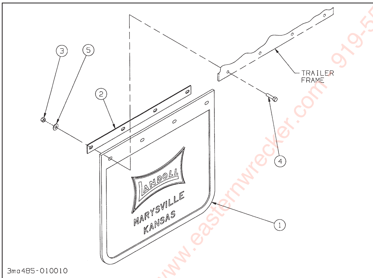
Figure 1-11 Mud Flap Assembly
