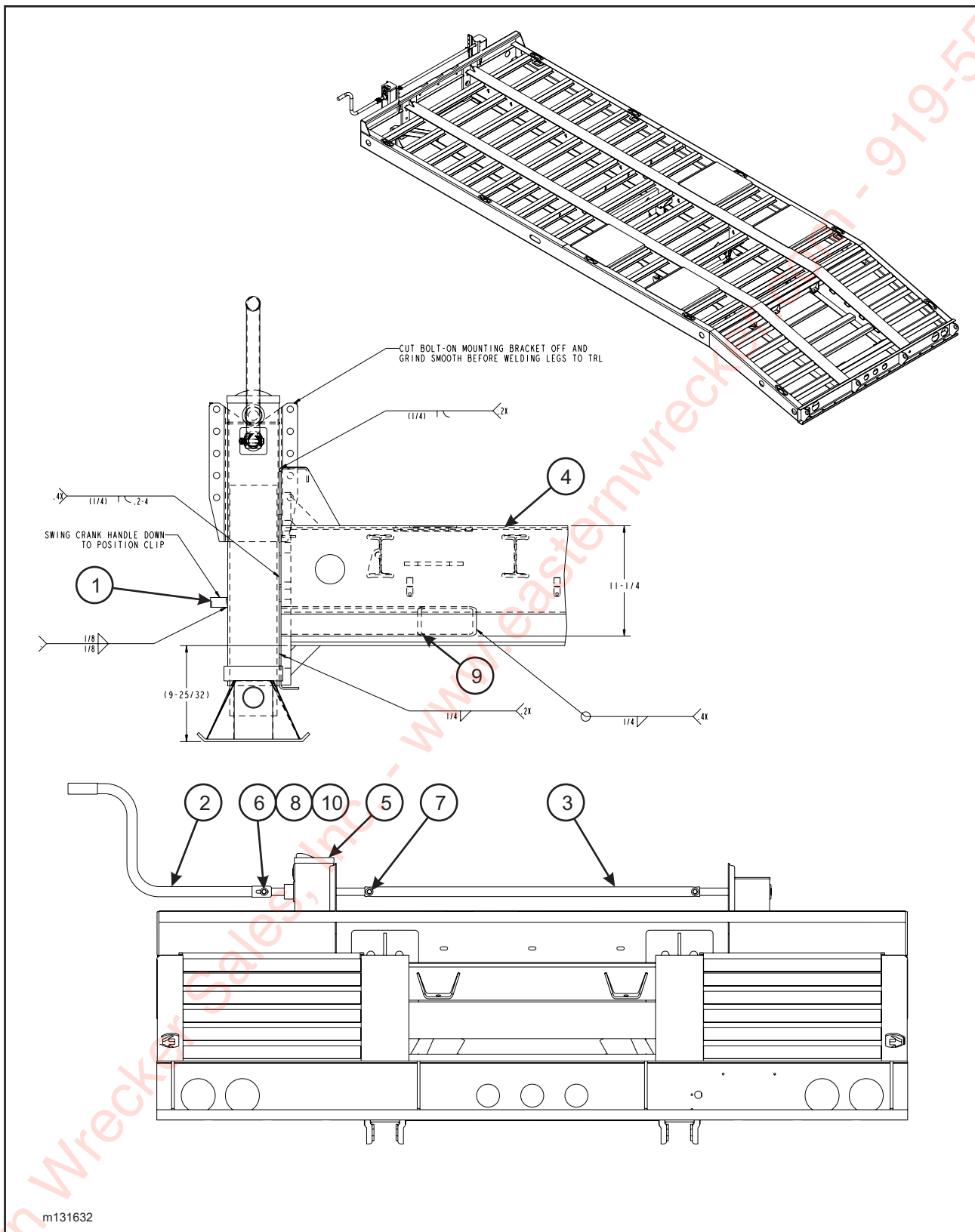
Figure 1-18 Landing Gear Installation - 2 Speed
