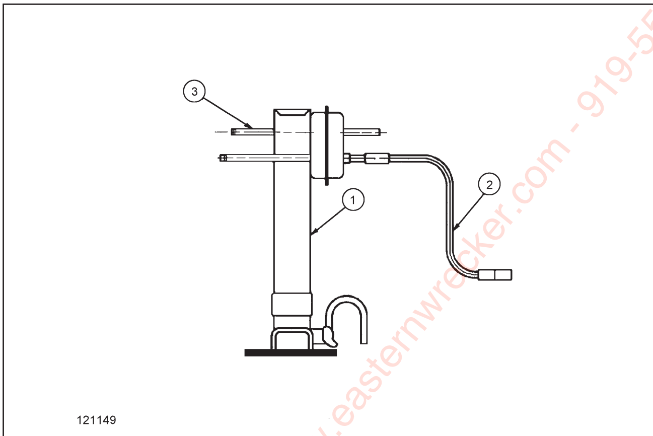
Figure 1-23 Landing Gear Assembly - 2 Speed Drop Leg
