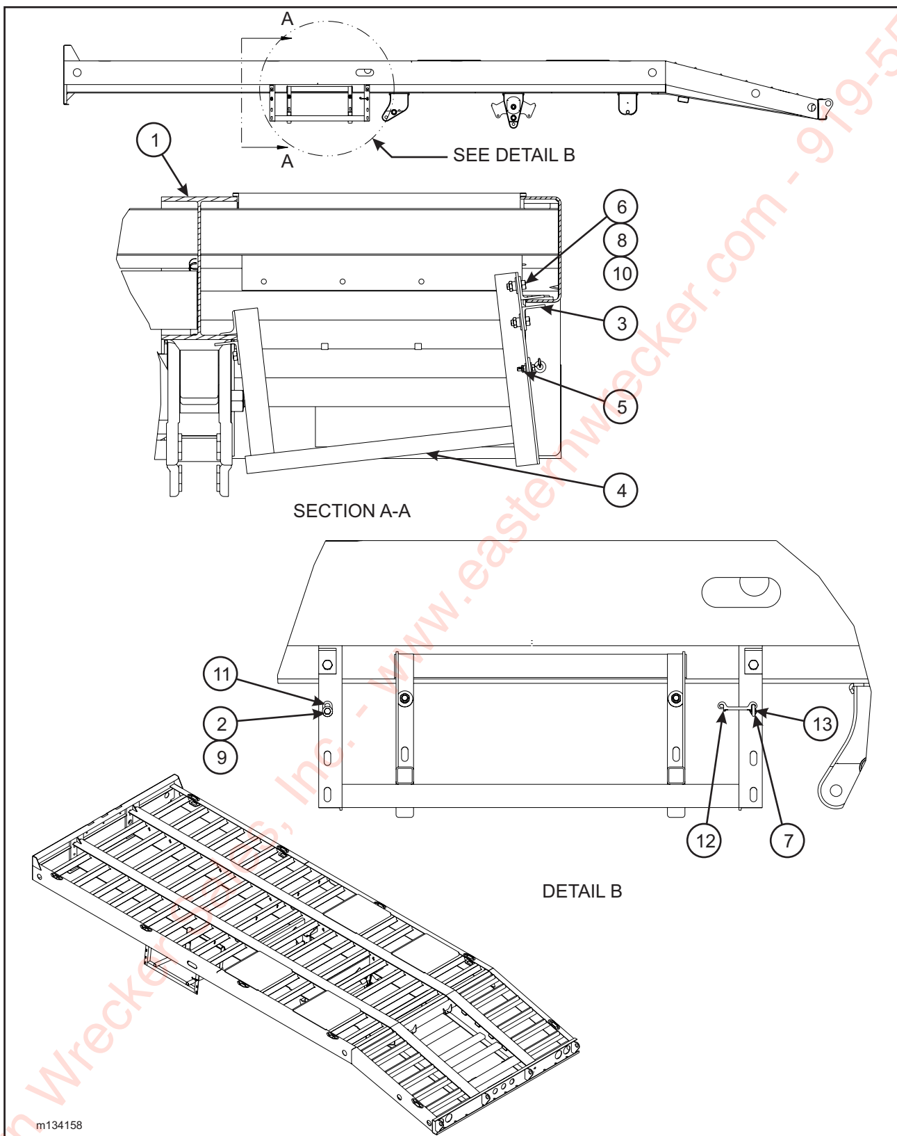
Figure 1-21 Spare Tire Carrier Assembly
