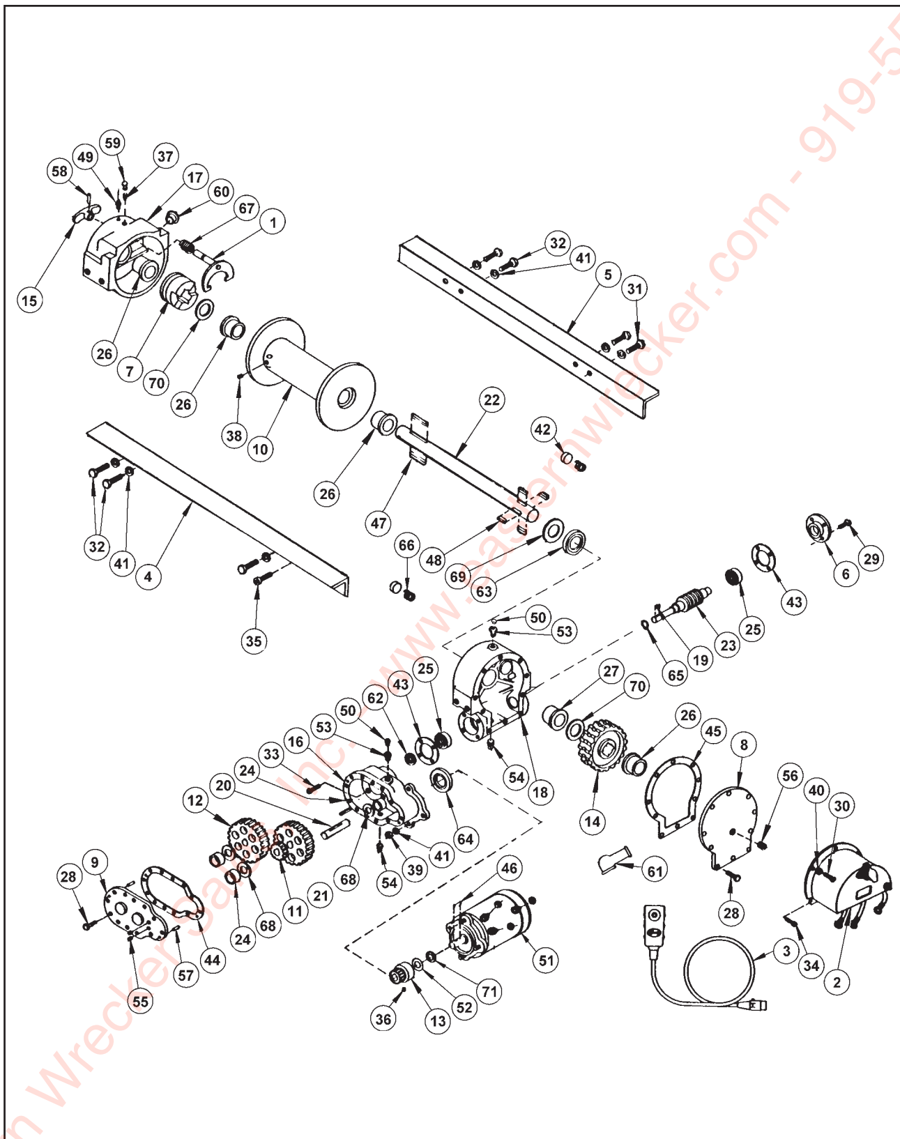
Figure 1-27 Winch Breakdown
