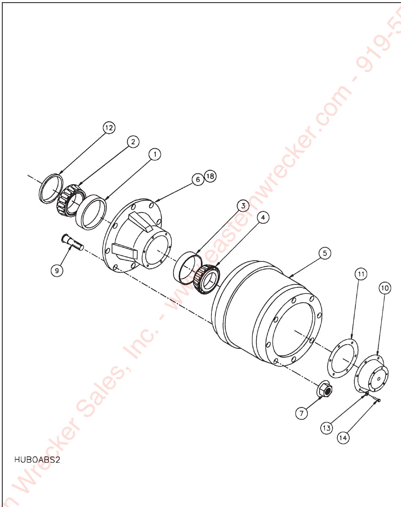
Figure 1-6 Outboard Pilot Mount Hub and Drum Assembly
