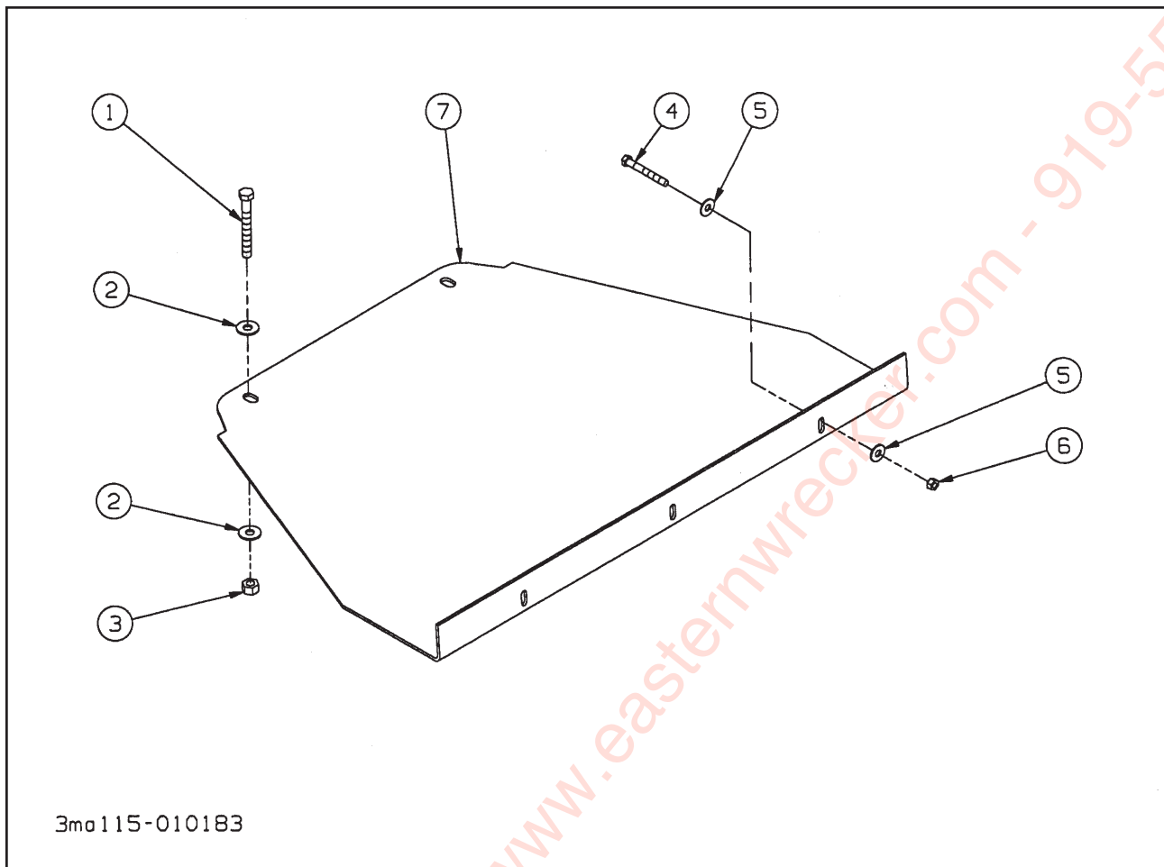
Figure 1-16 Toolbox Bottom Assembly
