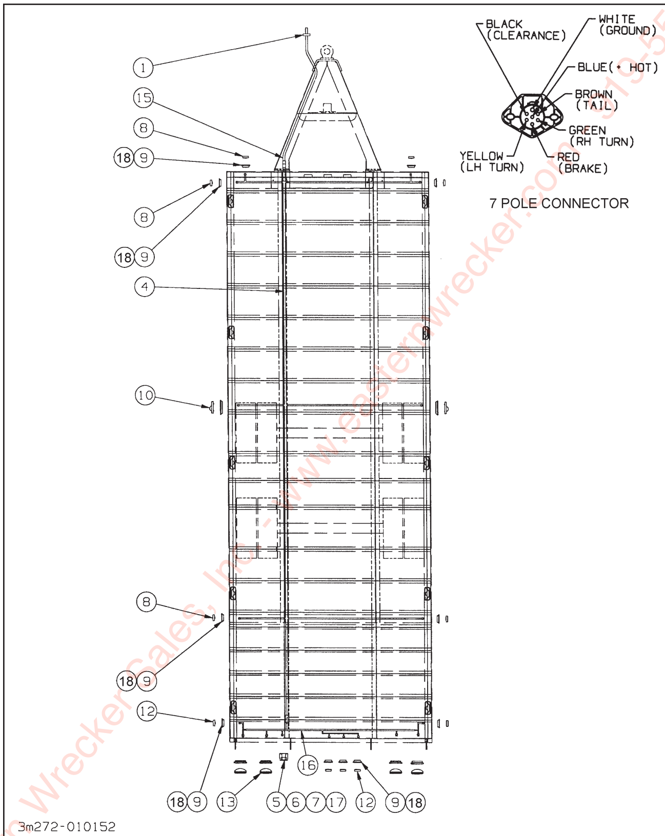
Figure 1-10 Electrical Assembly
