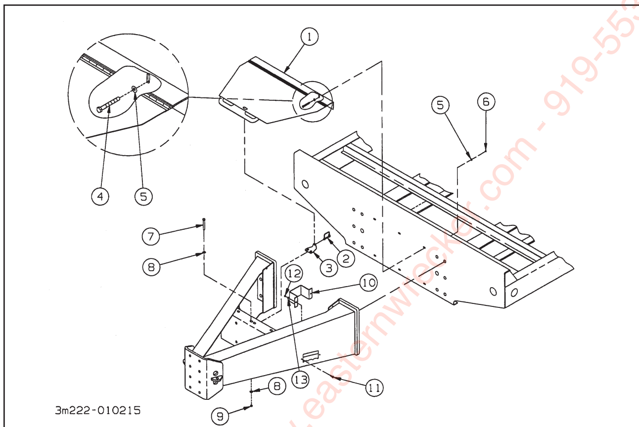
Figure 1-17 Toolbox Compartment Cover Assembly
