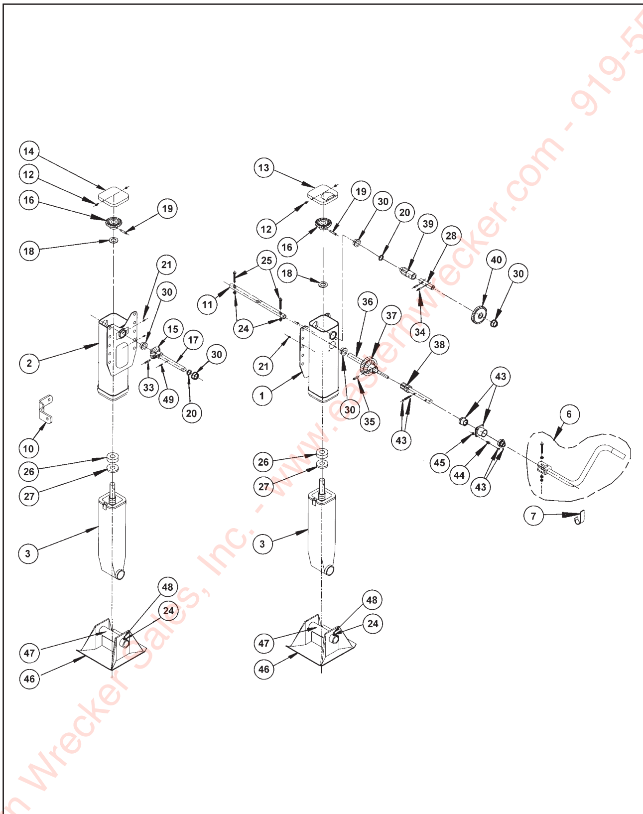
Figure 1-19 Crank Landing Gear
