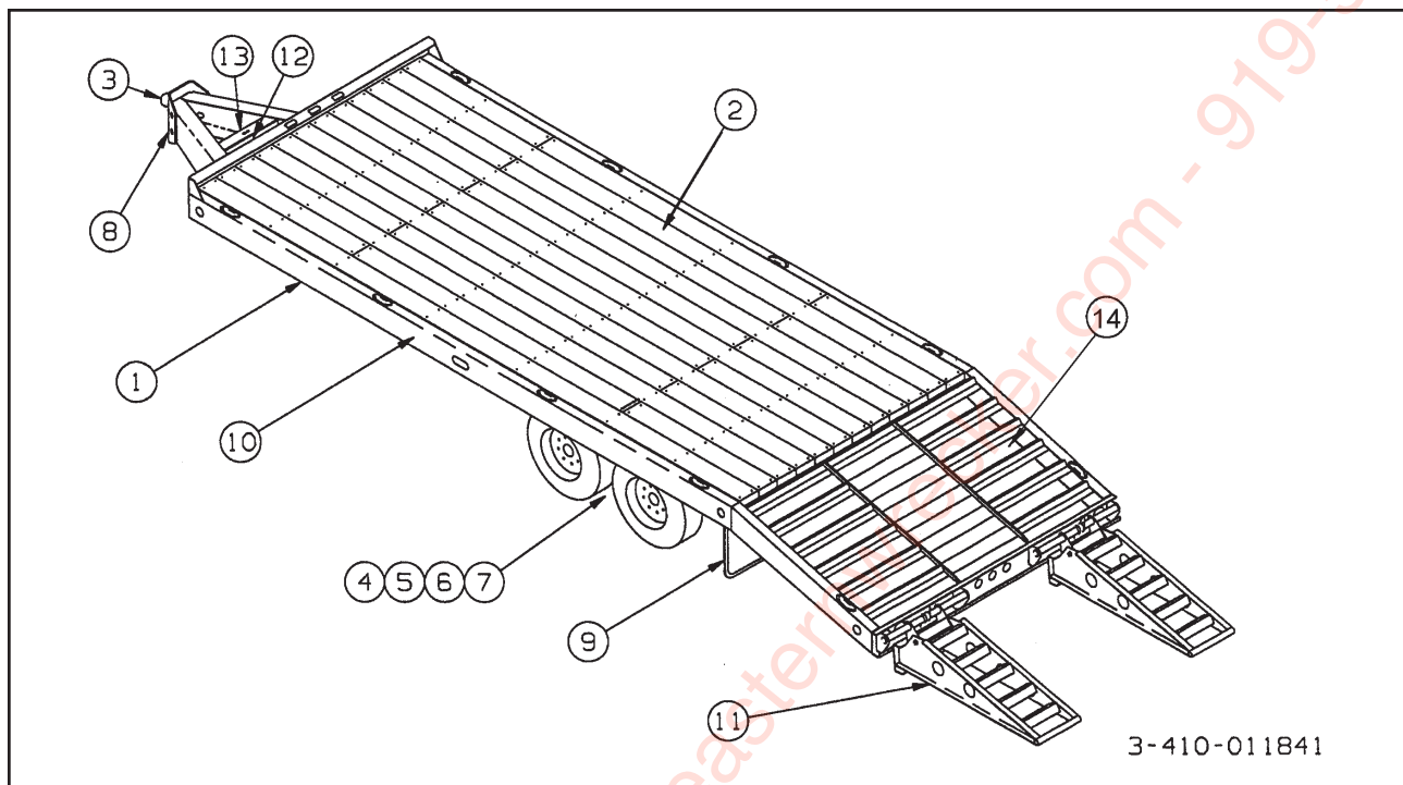
Figure 1-1 General Assembly
