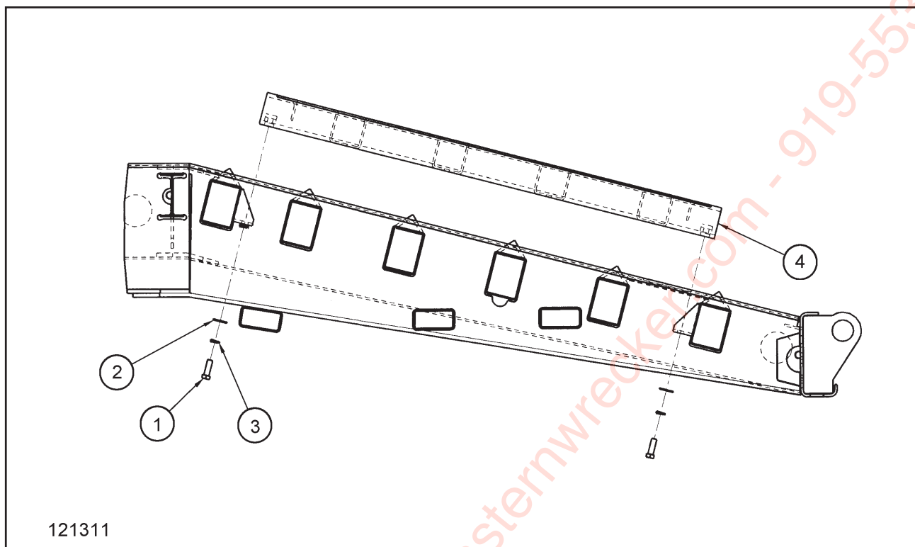
Figure 1-26 Beavertail Filler Installation
