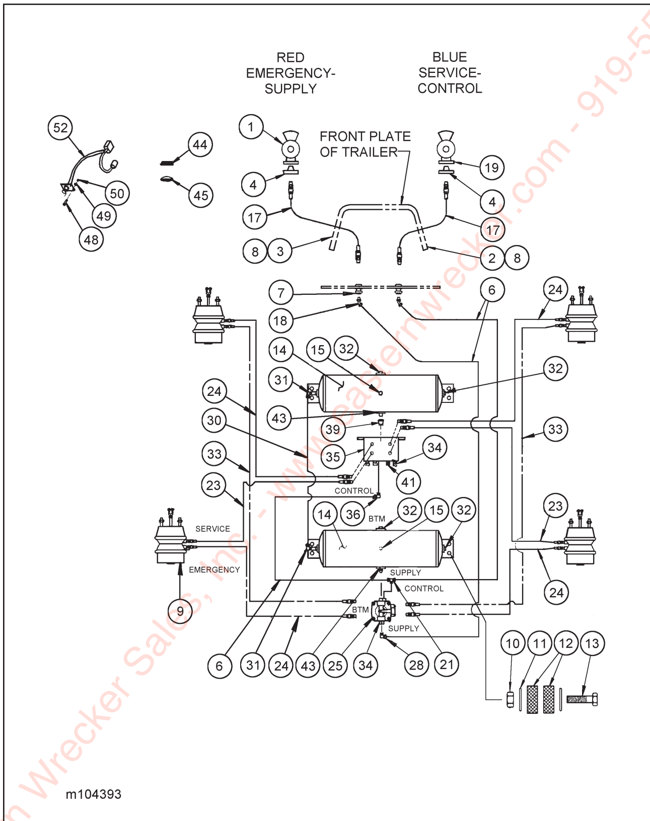
Figure 1-7 Air System (L4024)
