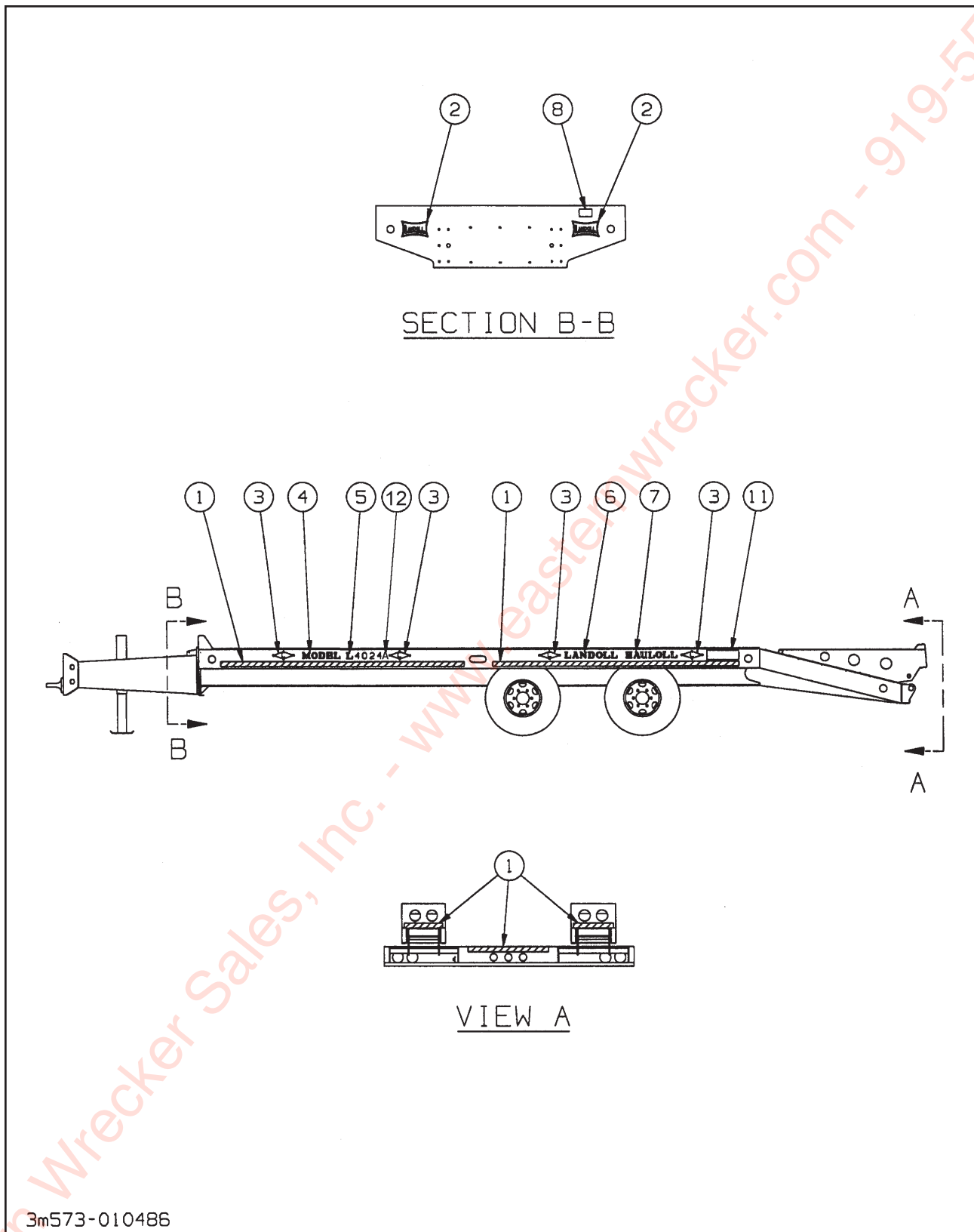
Figure 1-13 Decal Installation
