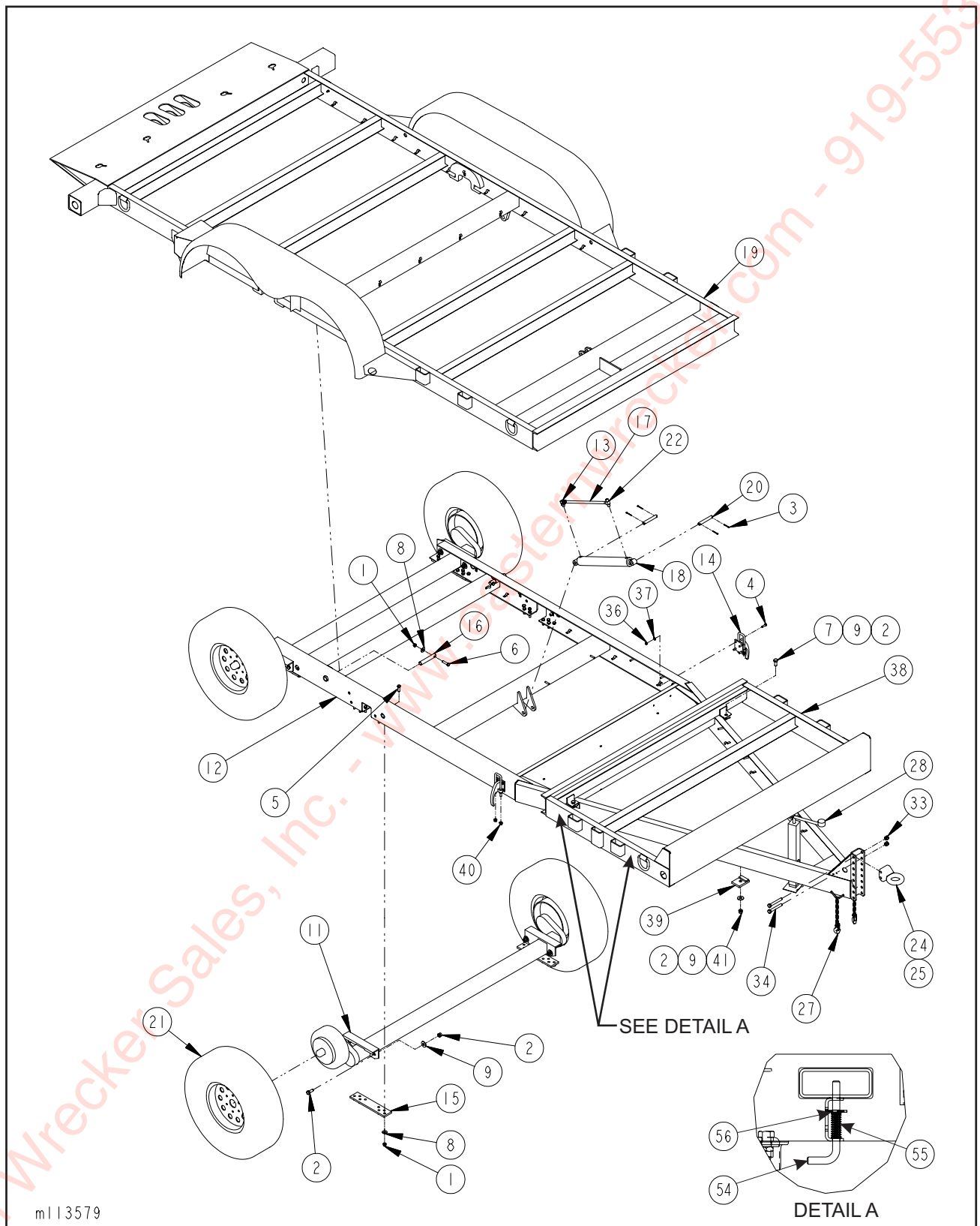
Figure 1-3 Trailer Assembly w/ Pintle Hitch (Electric Brakes) (LT1016-4) (2 of 3)
