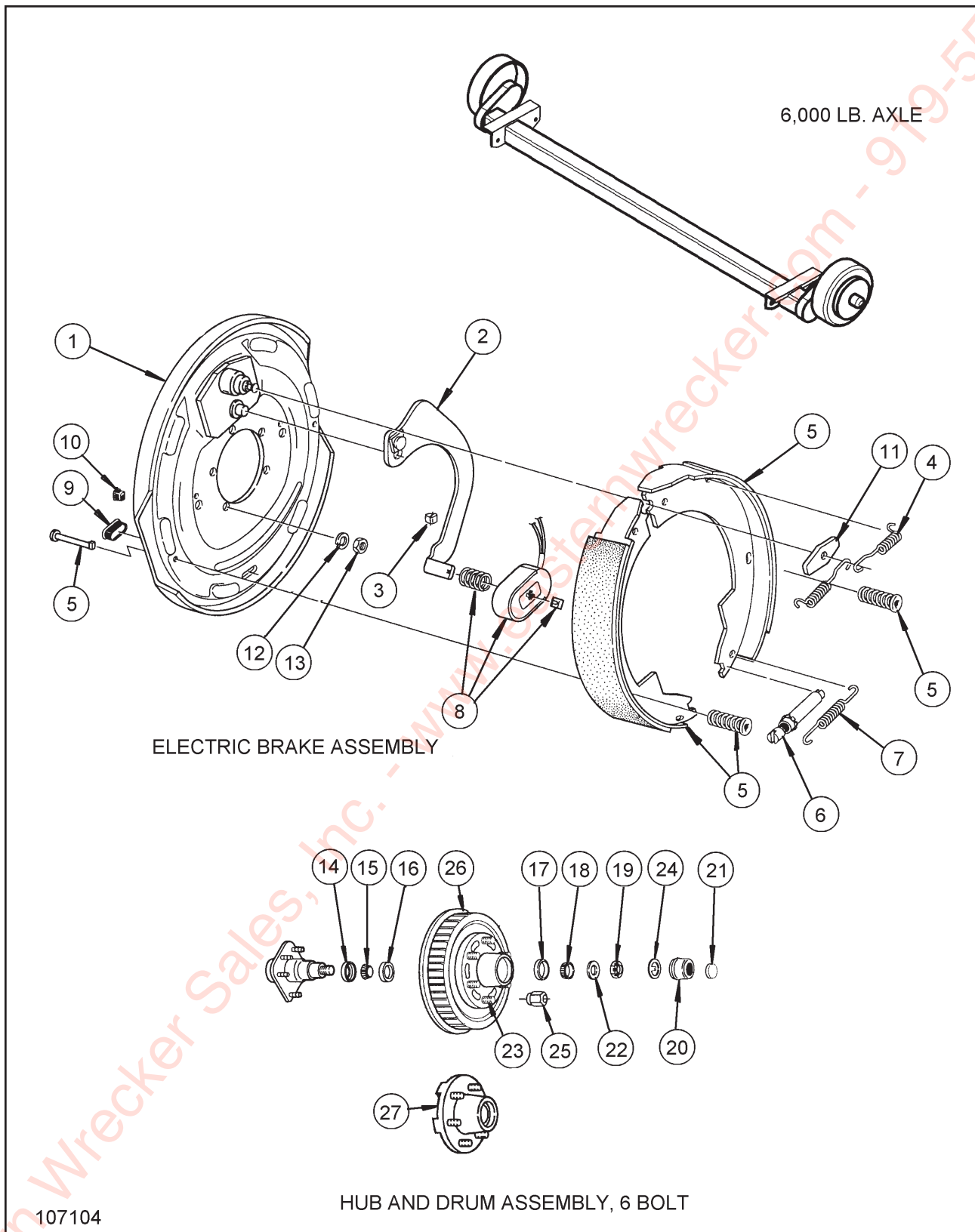
Figure 1-10 6000# E-Z Lube Axle Assy 6 Bolt
