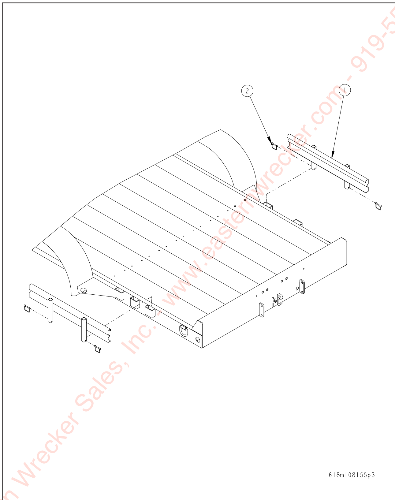
Figure 1-22 Siderail (Option)
