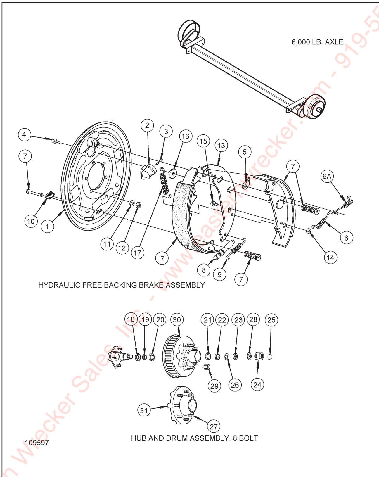
Figure 1-13 6000 Lb. E-Z Lube Hydr. Axle Assembly- 8 Bolt
