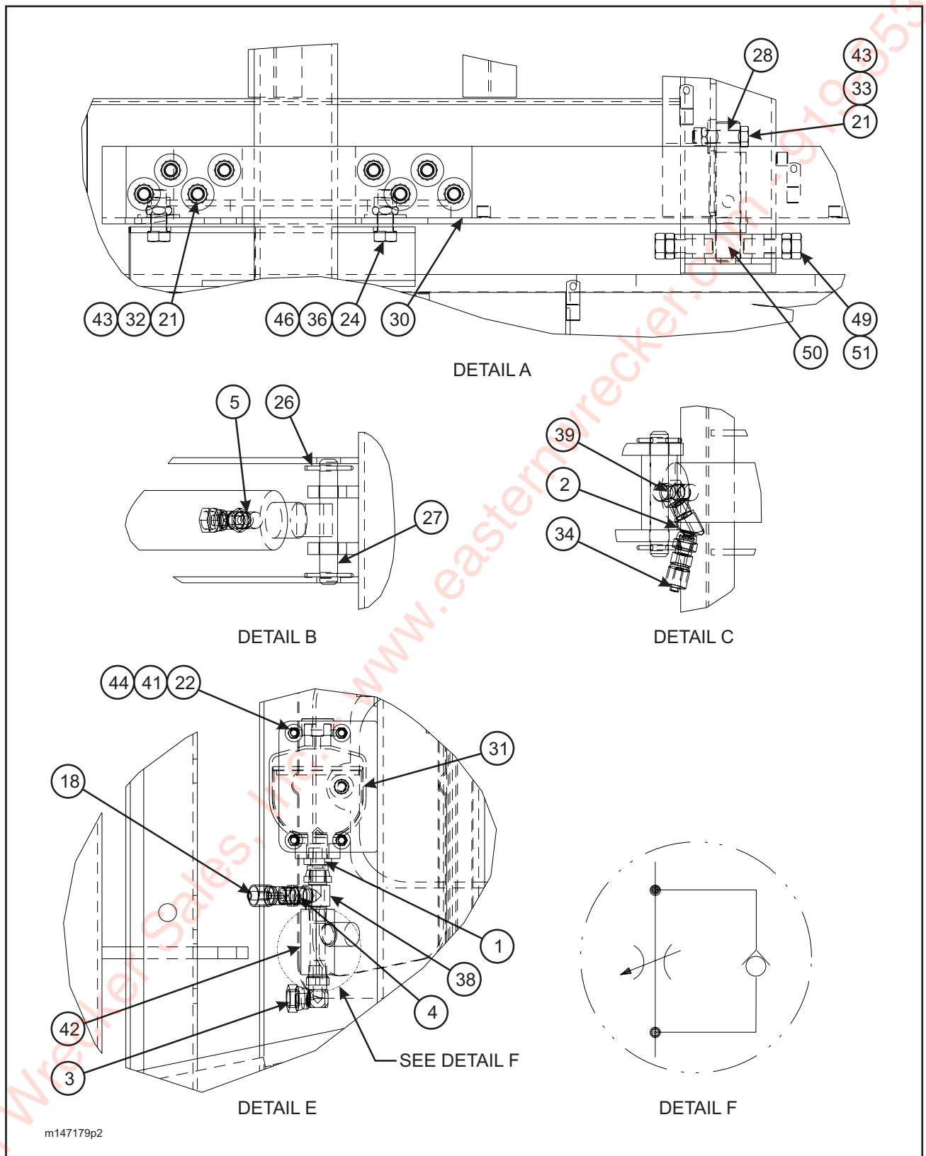
Figure 1-6 Trailer Assembly w/ Gooseneck Hitch (Electric Brakes) (LT1220 and LT1420) (2 of 2)
