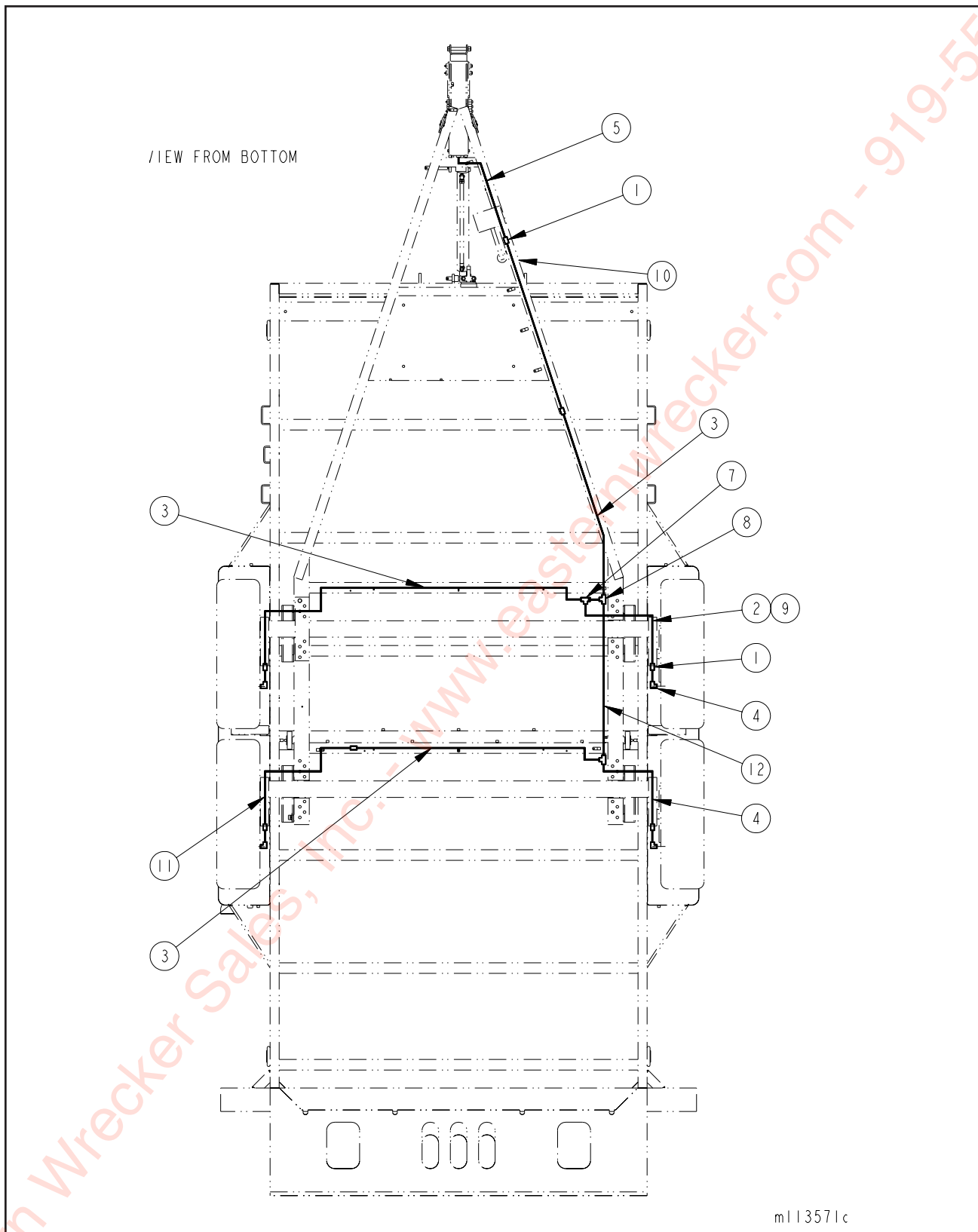
Figure 1-9 Surge Brake Line Schematic
