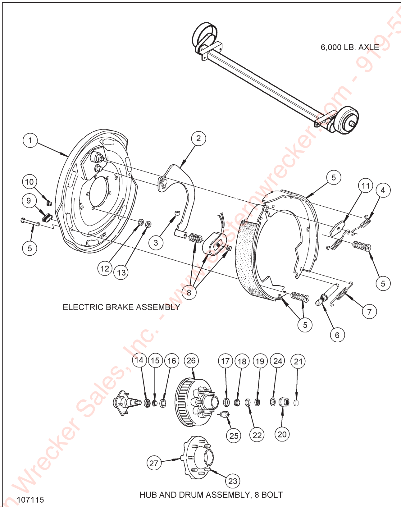
Figure 1-11 6000# E-Z Lube Axle Assy 8 Bolt
