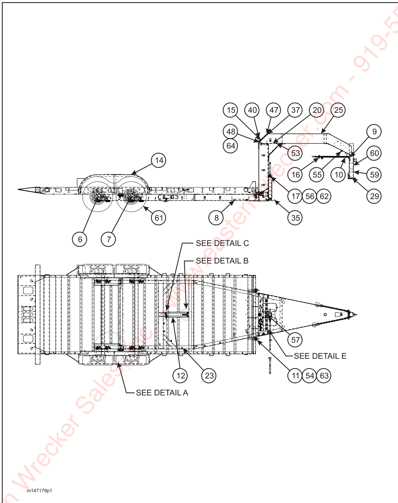
Figure 1-5 Trailer Assembly w/ Gooseneck Hitch (Electric Brakes) (LT1220 and LT1420) (1 of 2)
