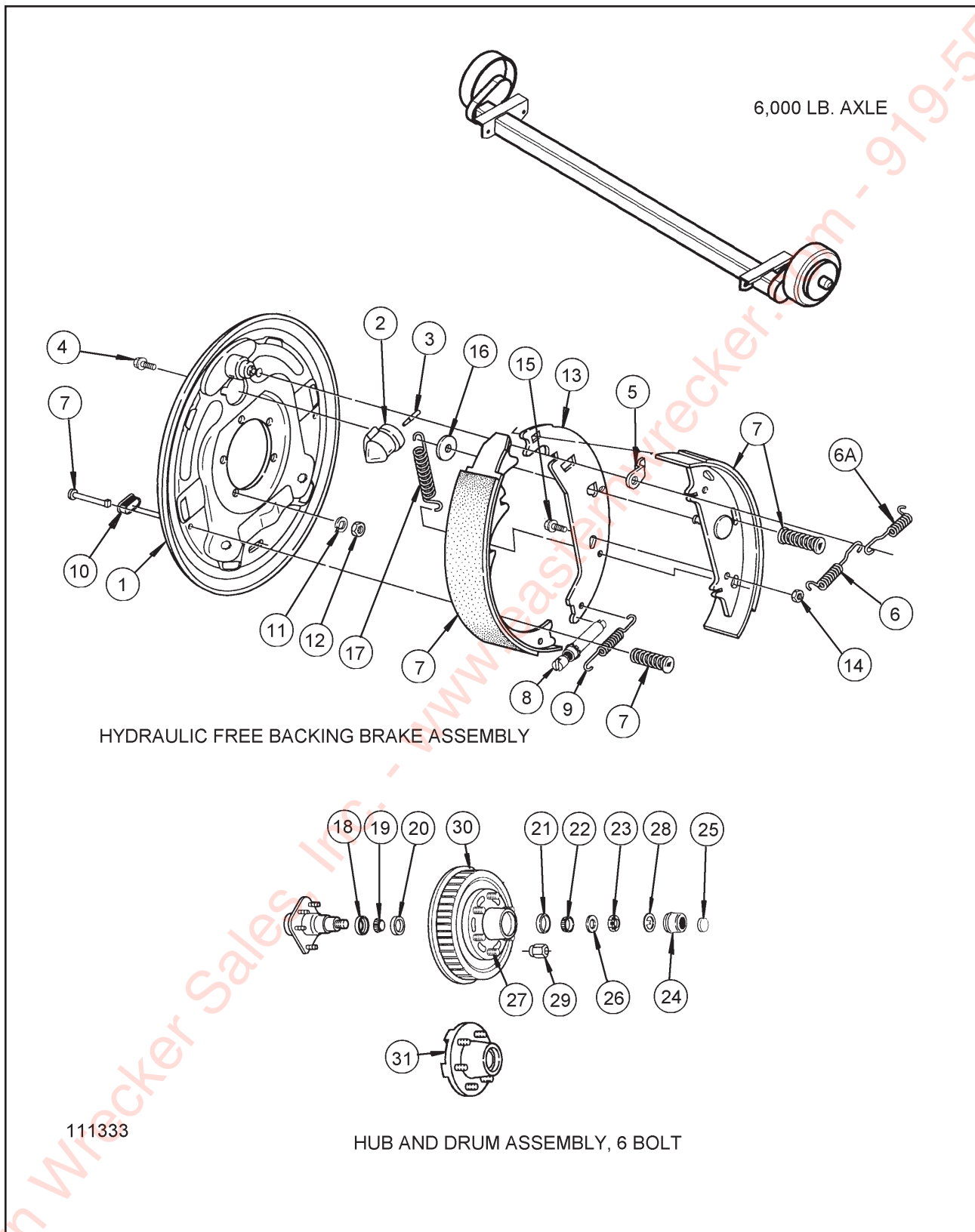
Figure 1-12 6000 Lb. E-Z Lube Hydr. Axle Assembly- 6 Bolt
