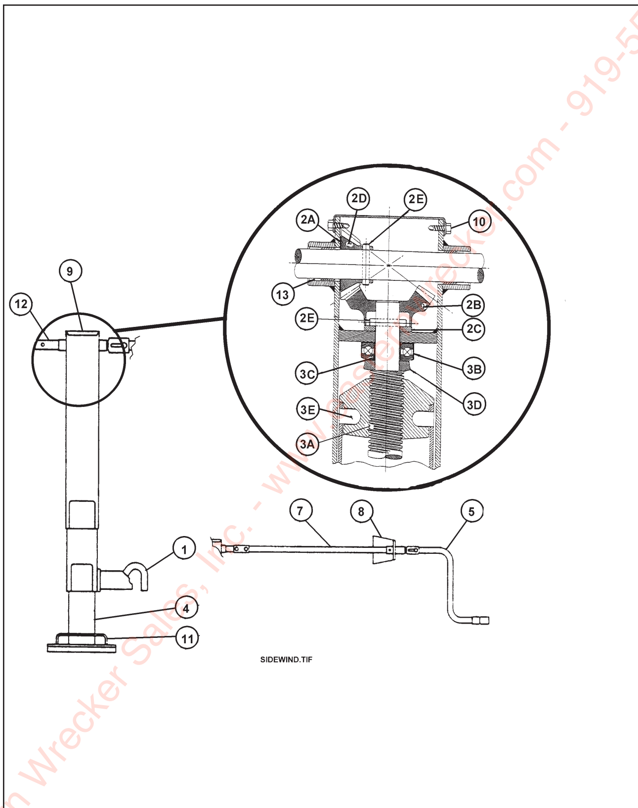
Figure 1-29 Jackstand Assembly (Gooseneck Hitch)
