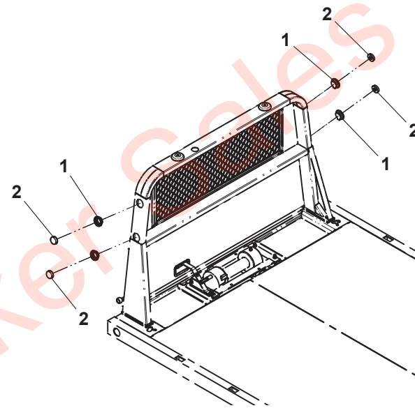
FOR 45", 50" & 57" HEADBOARD
