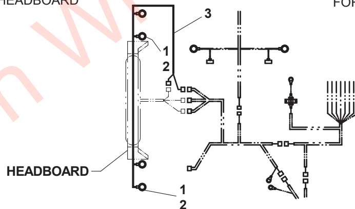
FOR 36" & 40" HEADBOARD
