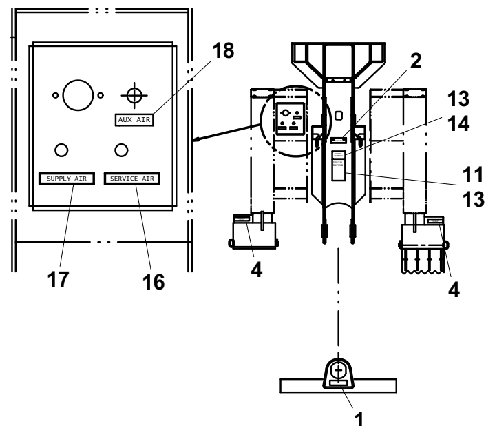
VIEW B-B
