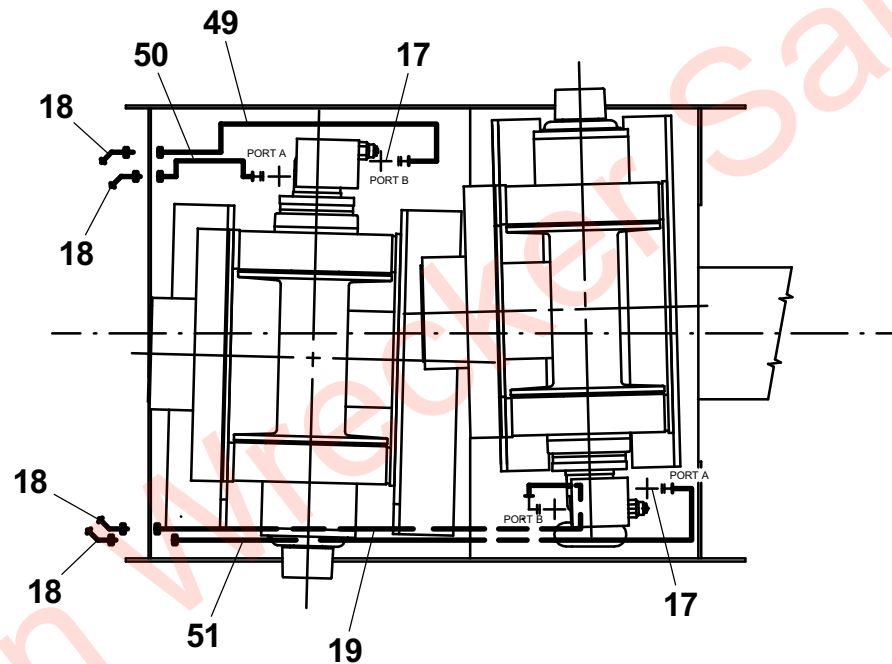
PLANETARY WINCH
