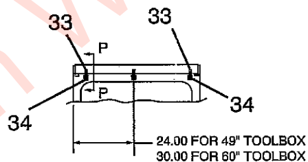
SECTION N - N 49" & 60" TOOLBOX'S ONLY
