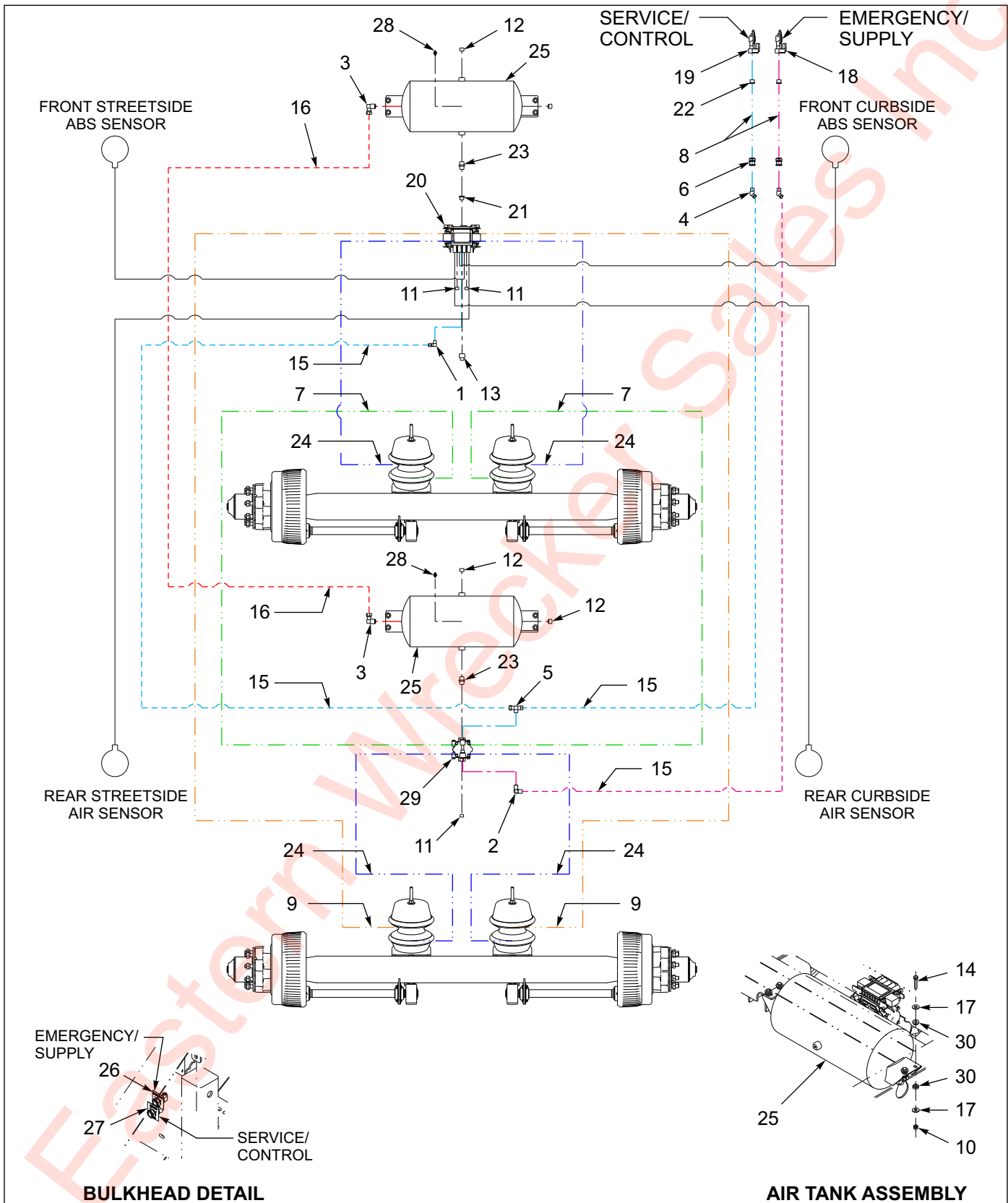
Figure 1-10: Air System W/ ABS
