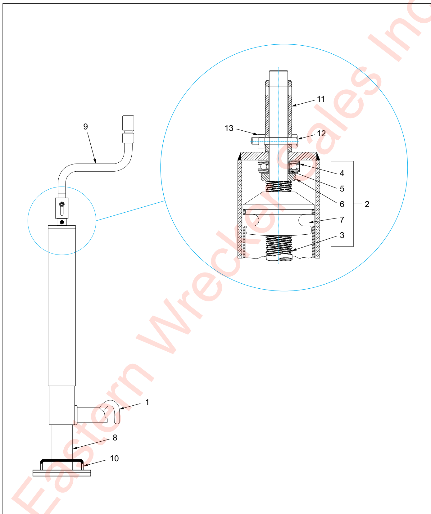
Figure 1-16: Jackstand Assembly - Pintle Hitch
