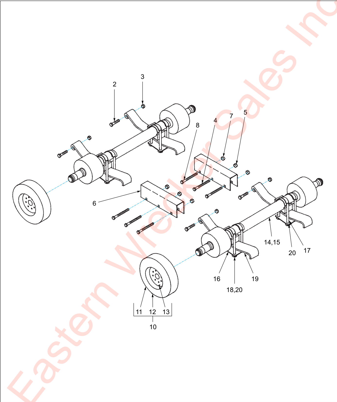
Figure 1-12: Suspension Assembly
