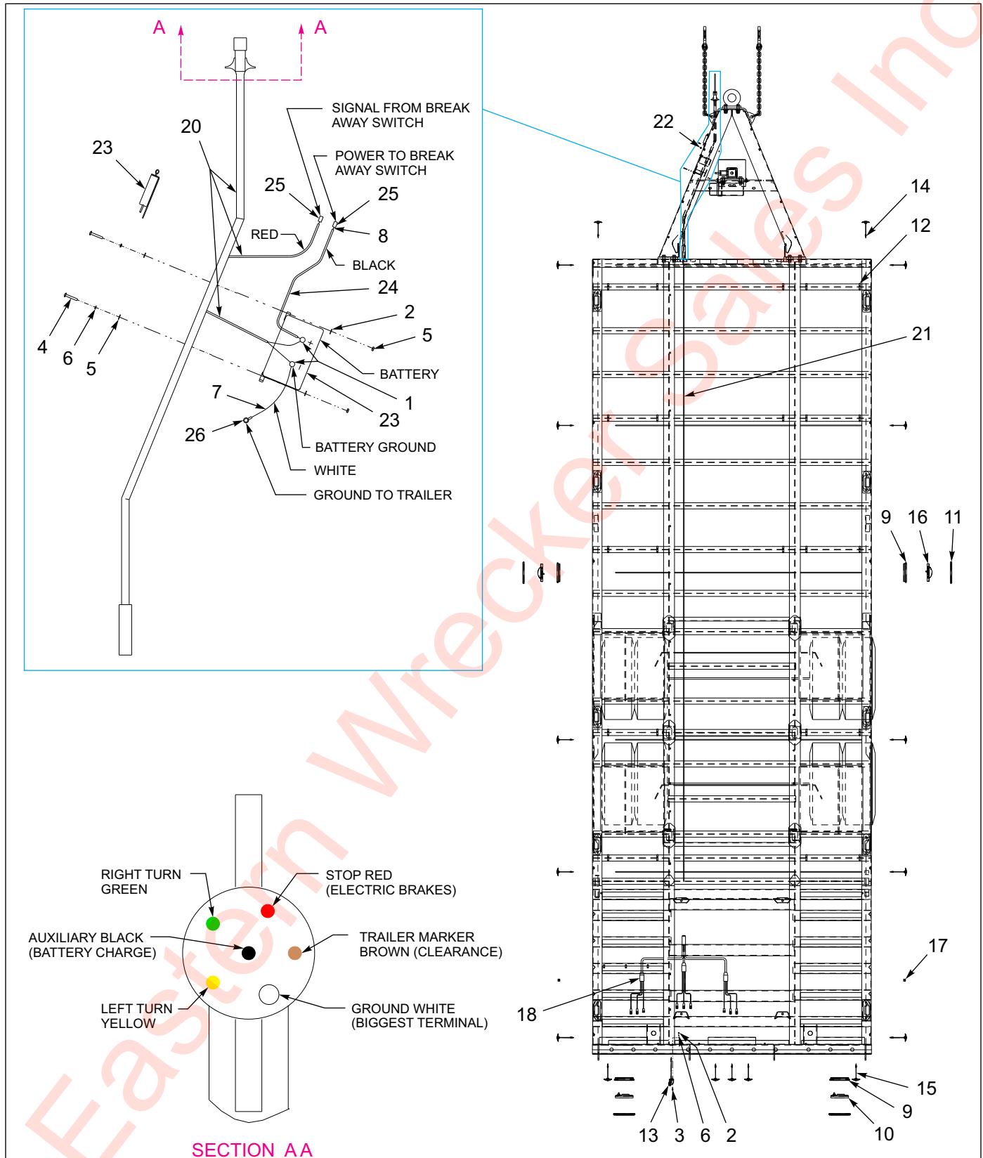
Figure 1-8: Electrical System - W/ Electric Brakes
