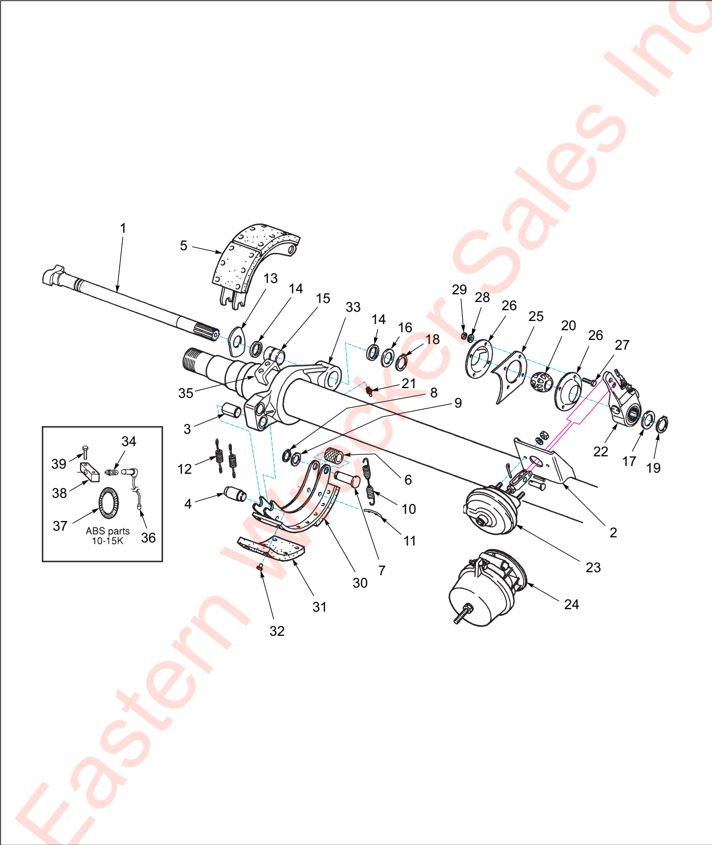
Figure 1-13: Air Brake - 10K HD & 12K
