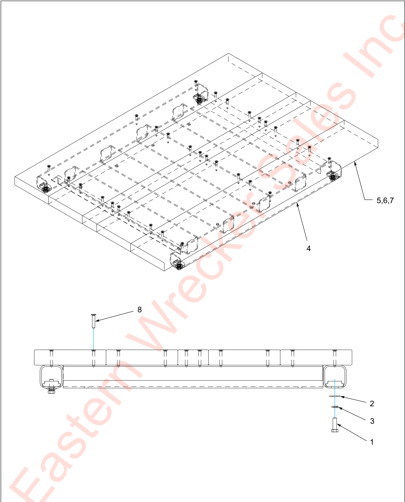
Figure 1-22: Beavertail Filler Installation (Option)
