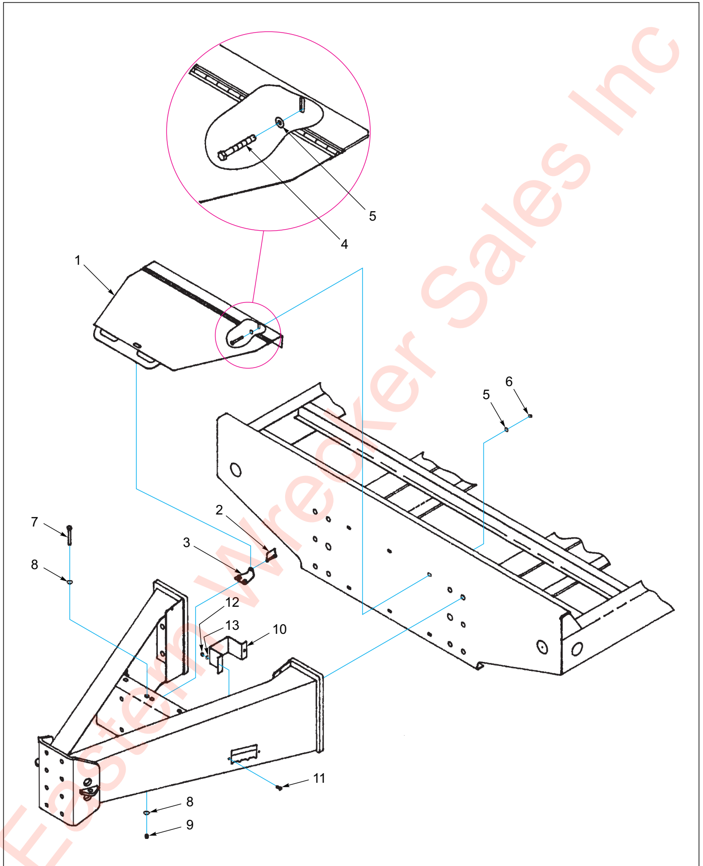
Figure 1-24: Tool Compartment Cover Assembly (Option)
