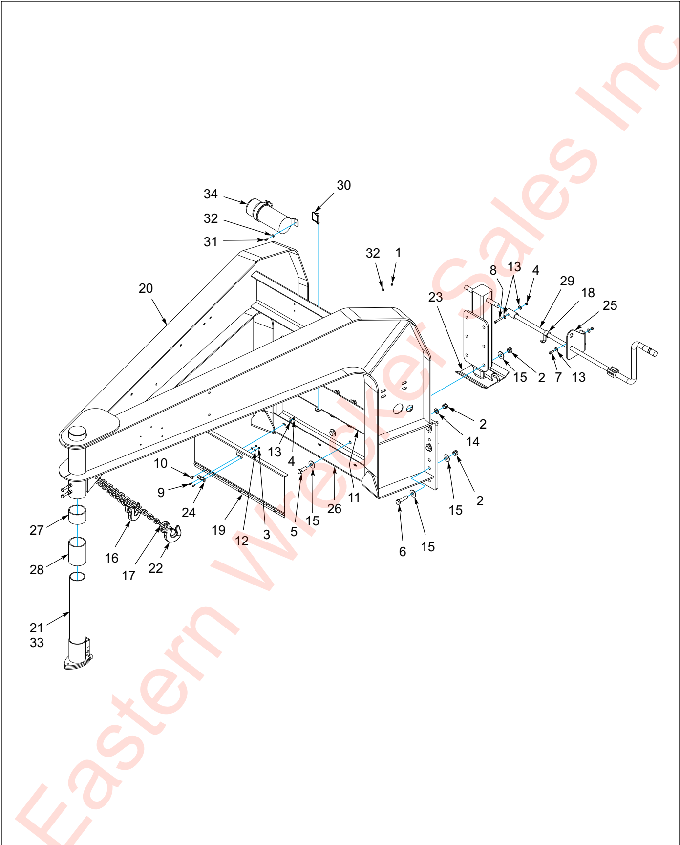
Figure 1-7: Gooseneck Hitch Assembly
