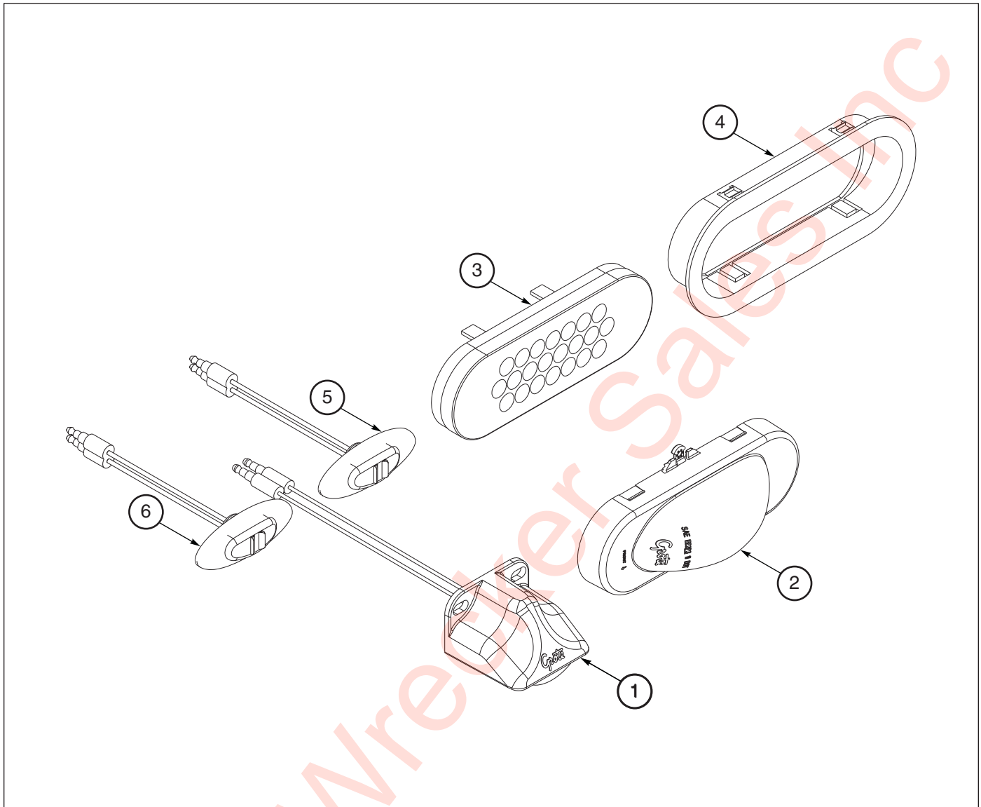
Figure 1-60: Spare Light Kit 343A LED-196586
