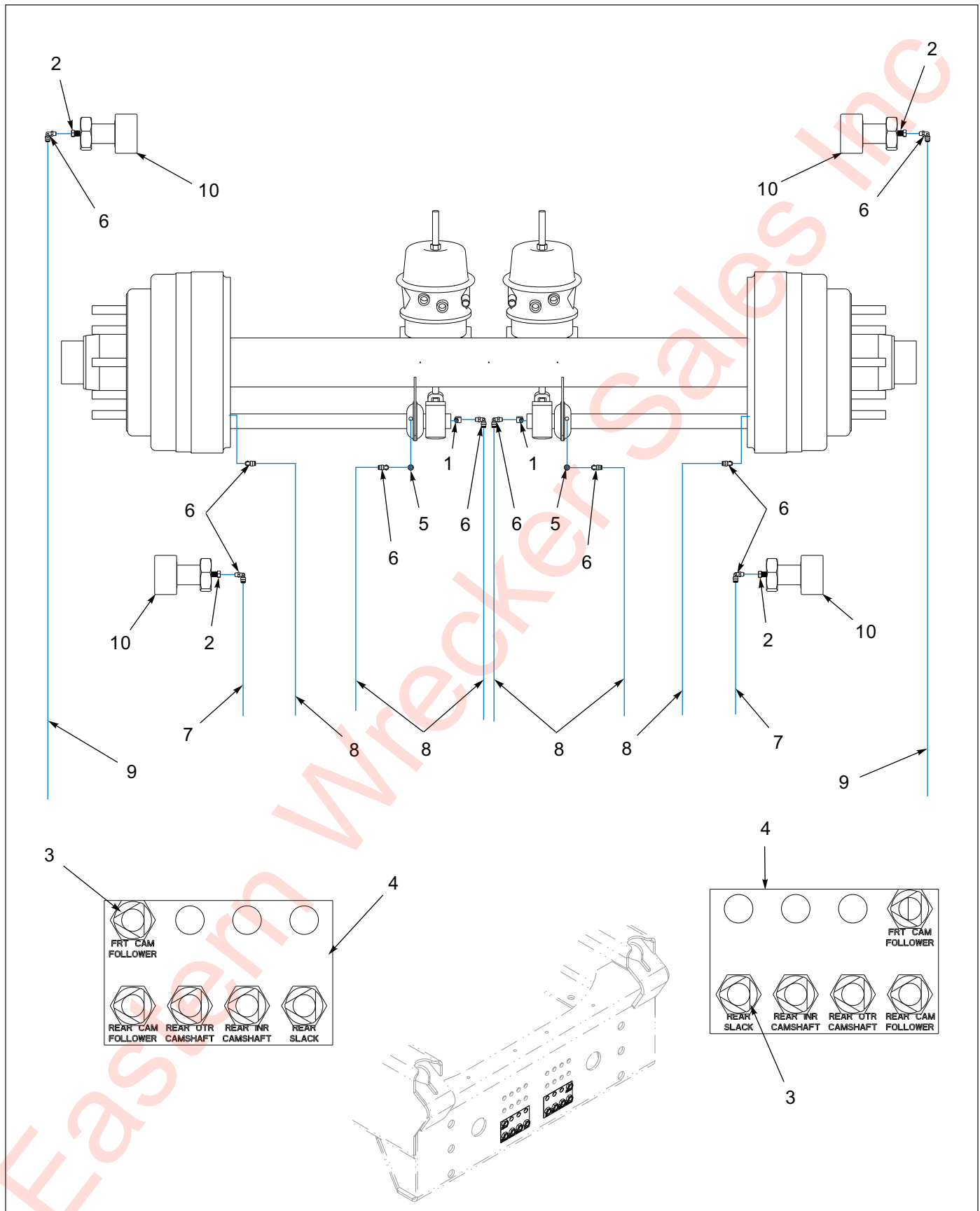
Figure 1-16: Grease System
