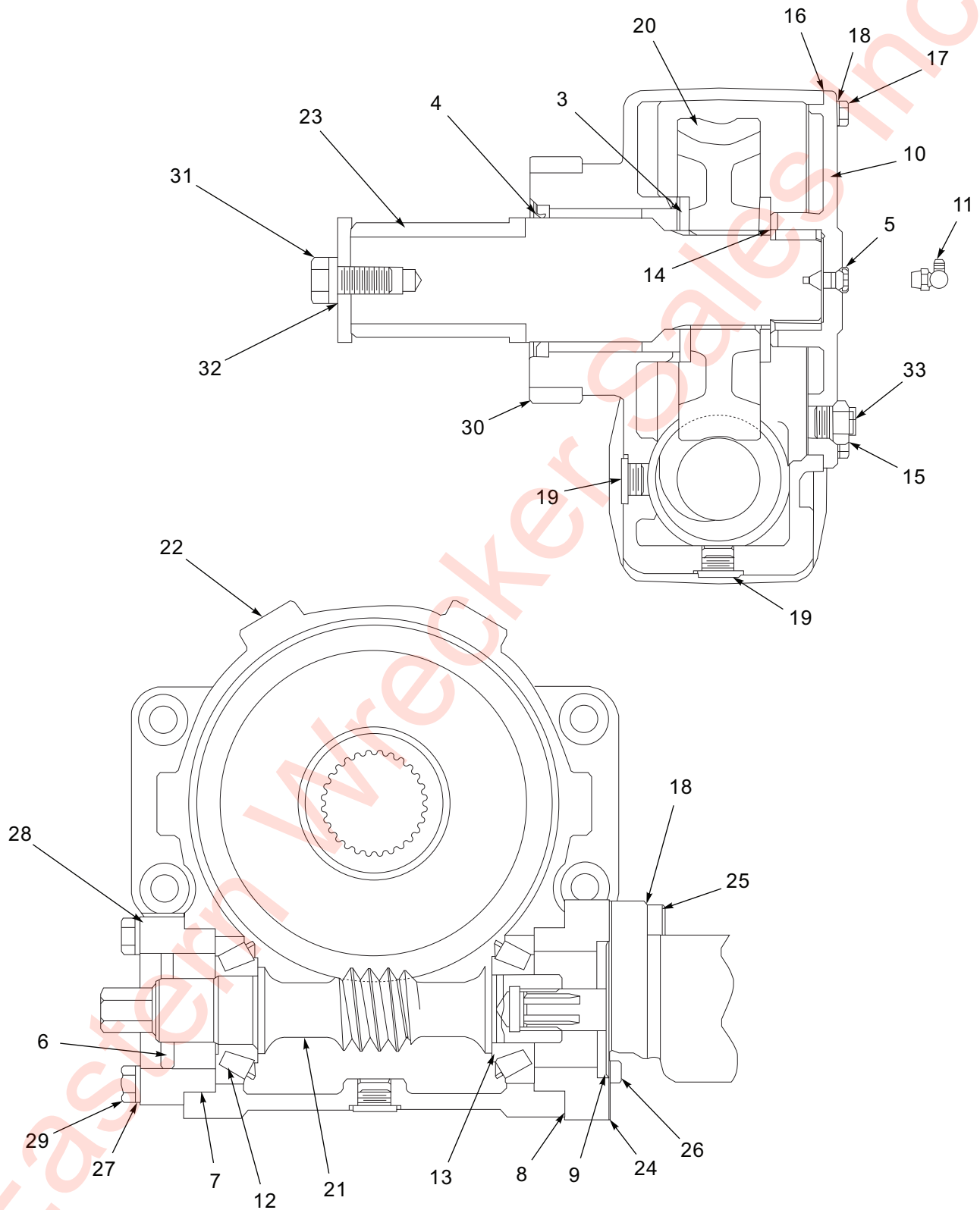
Figure 1-29: Gearbox Items
