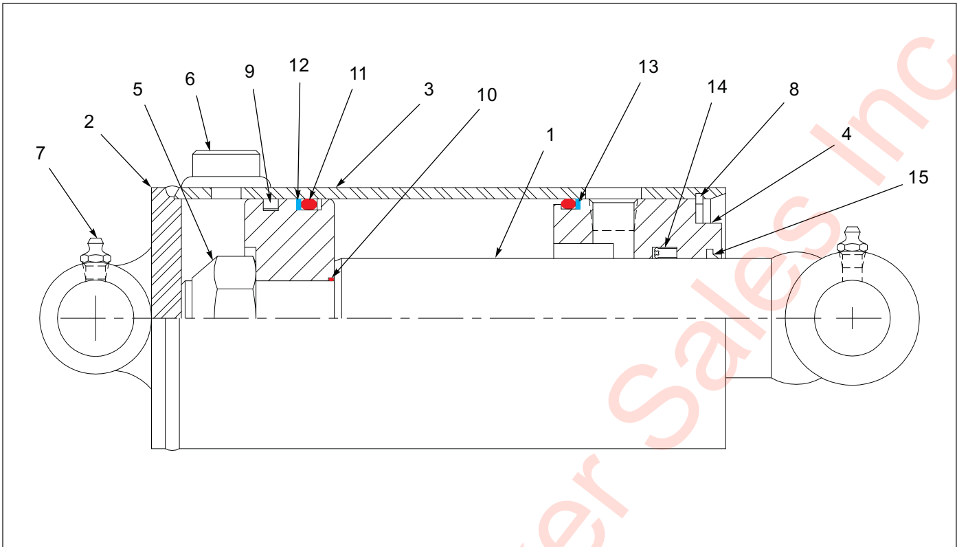
Figure 1-6: Hydraulic Cylinder - 4 x 20
