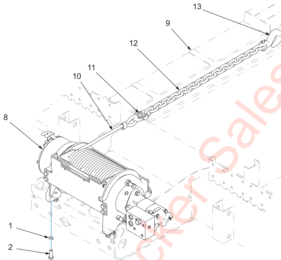
WINCH ASSEMBLY
