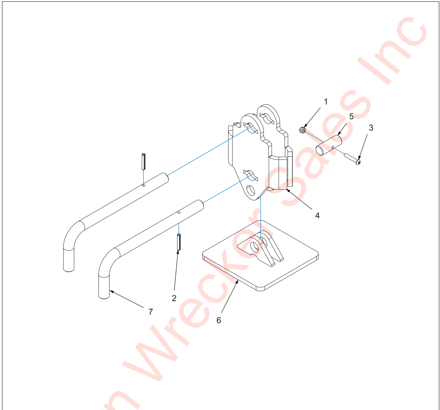
Figure 1-64: Tiedown Assembly - Shoe Lock
