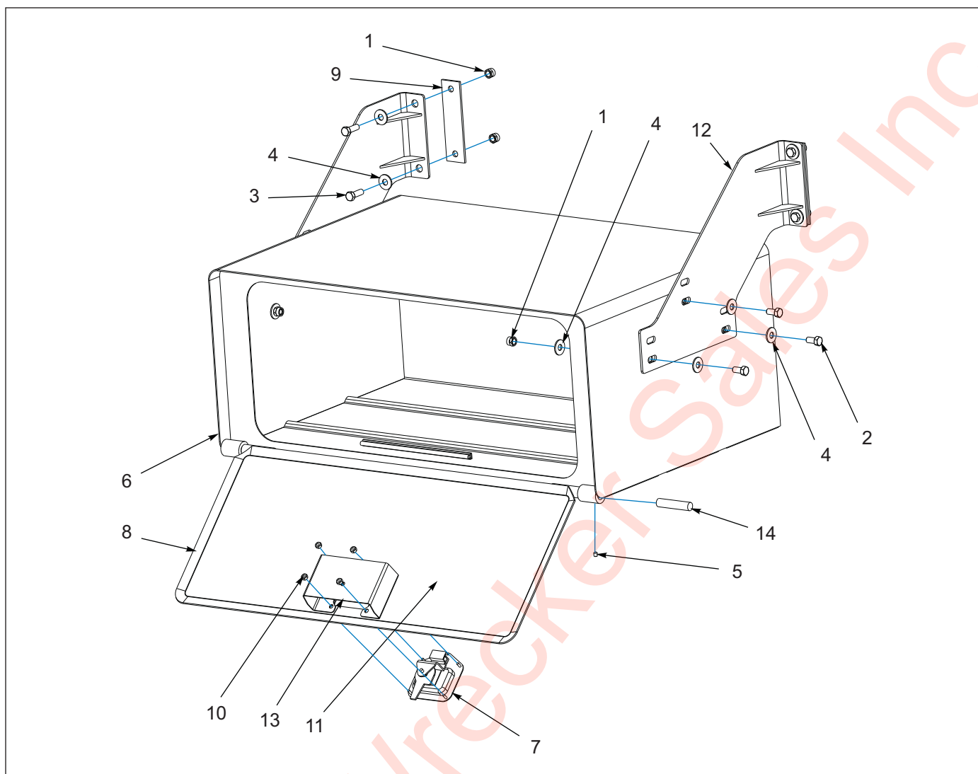
Figure 1-66: Tool Box Installation
