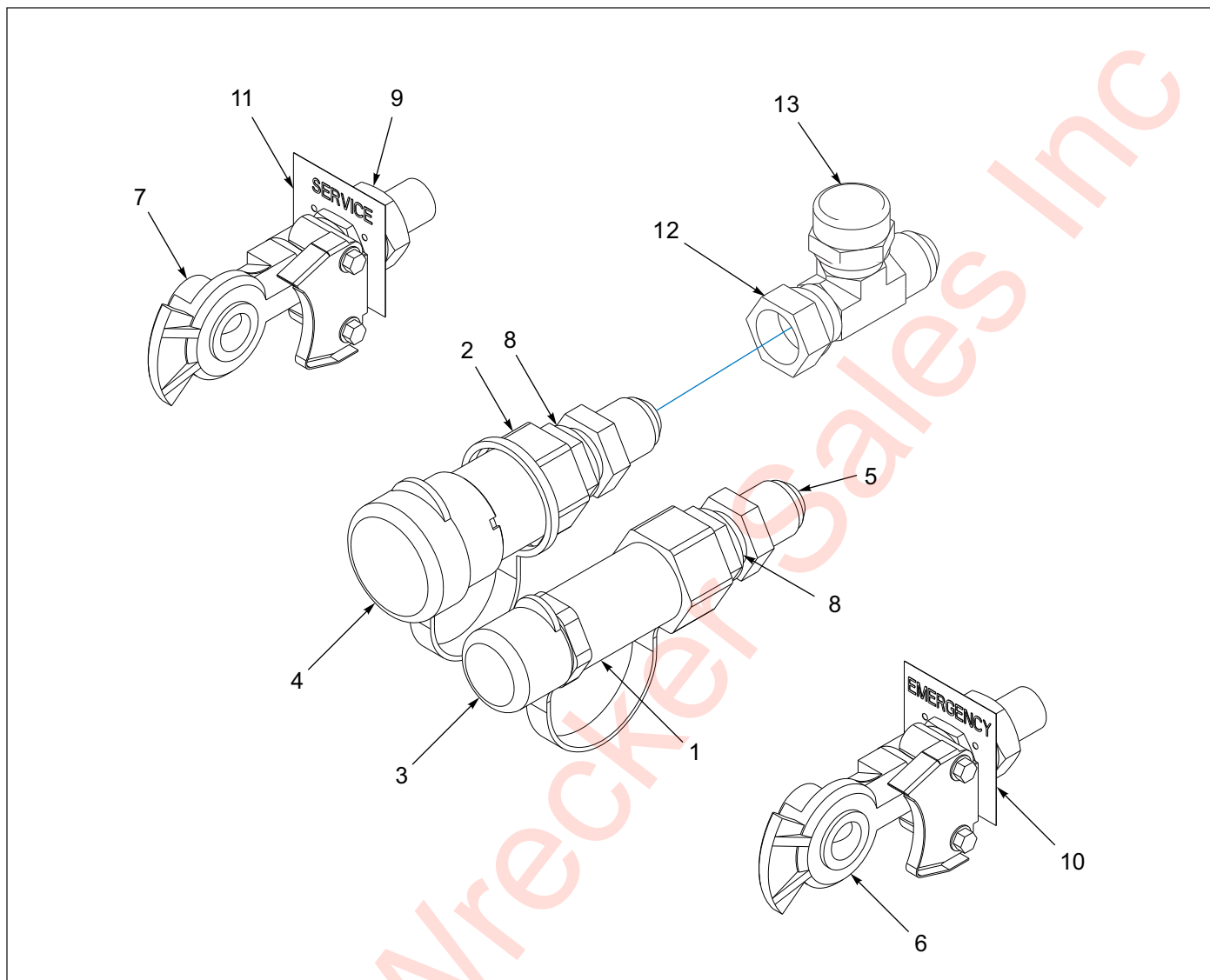
Figure 1-7: Connectors - Front Sub Assembly
