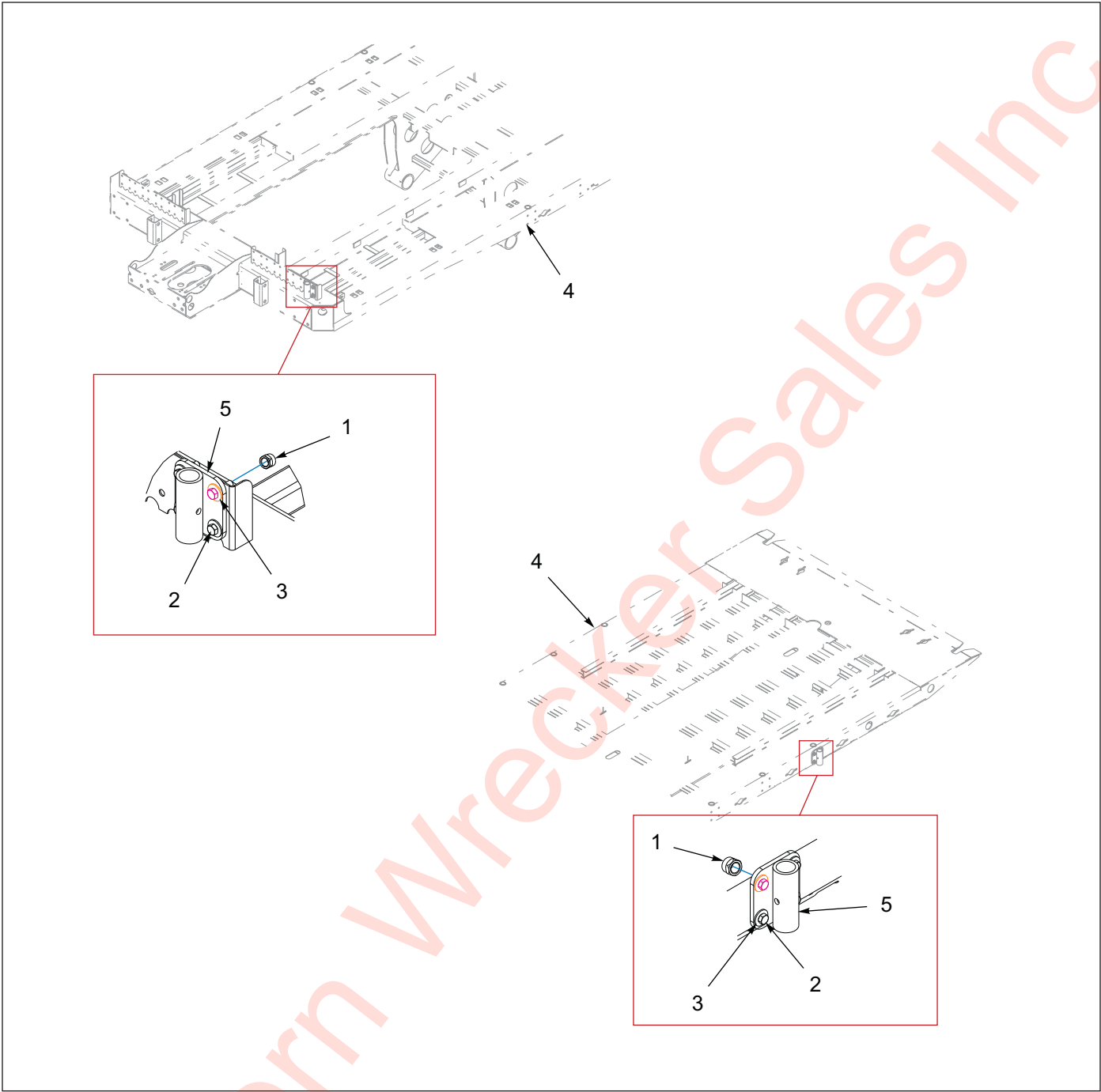
Figure 1-61: Side Guide - Anchor Pair
