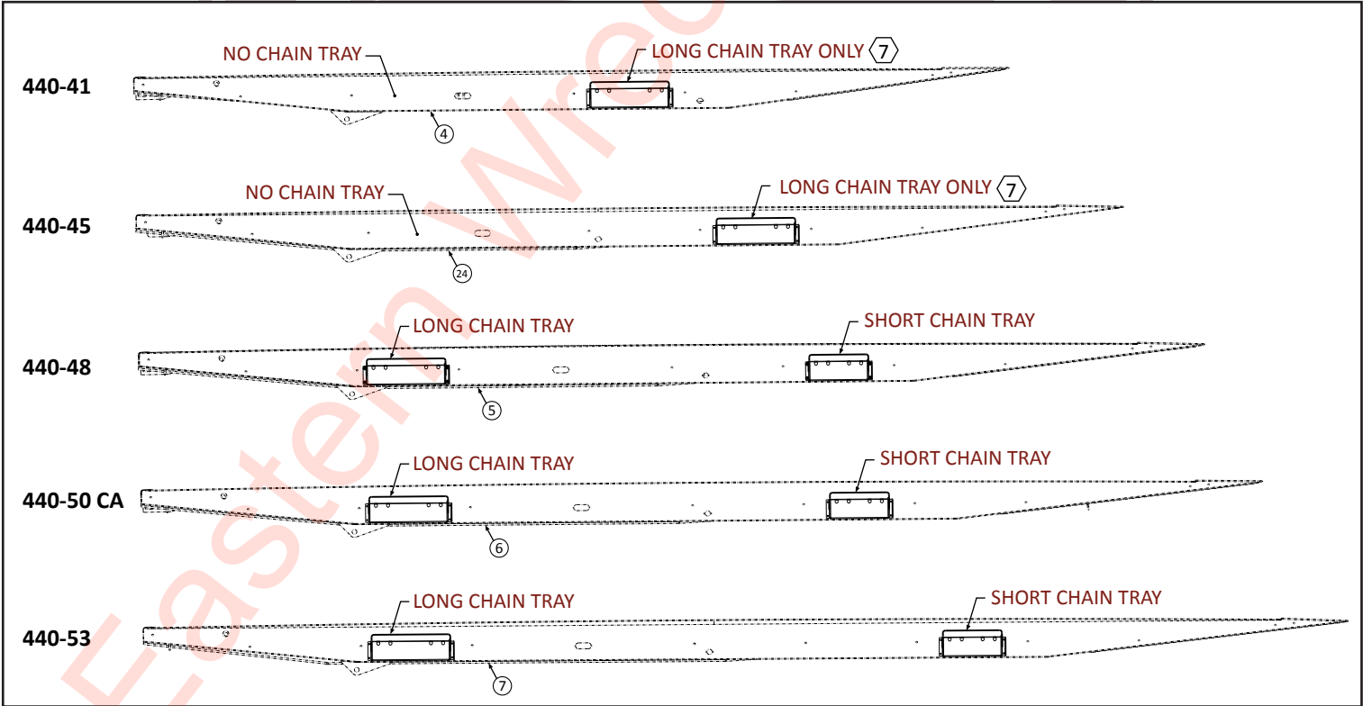
440 Series Web Mounted Chain Tray
