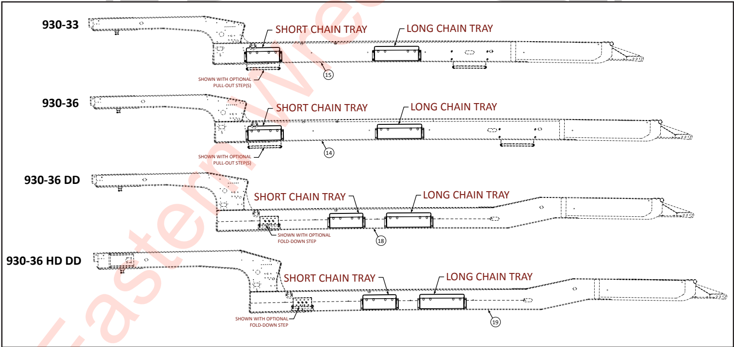
930 Series Web Mounted Chain Tray
