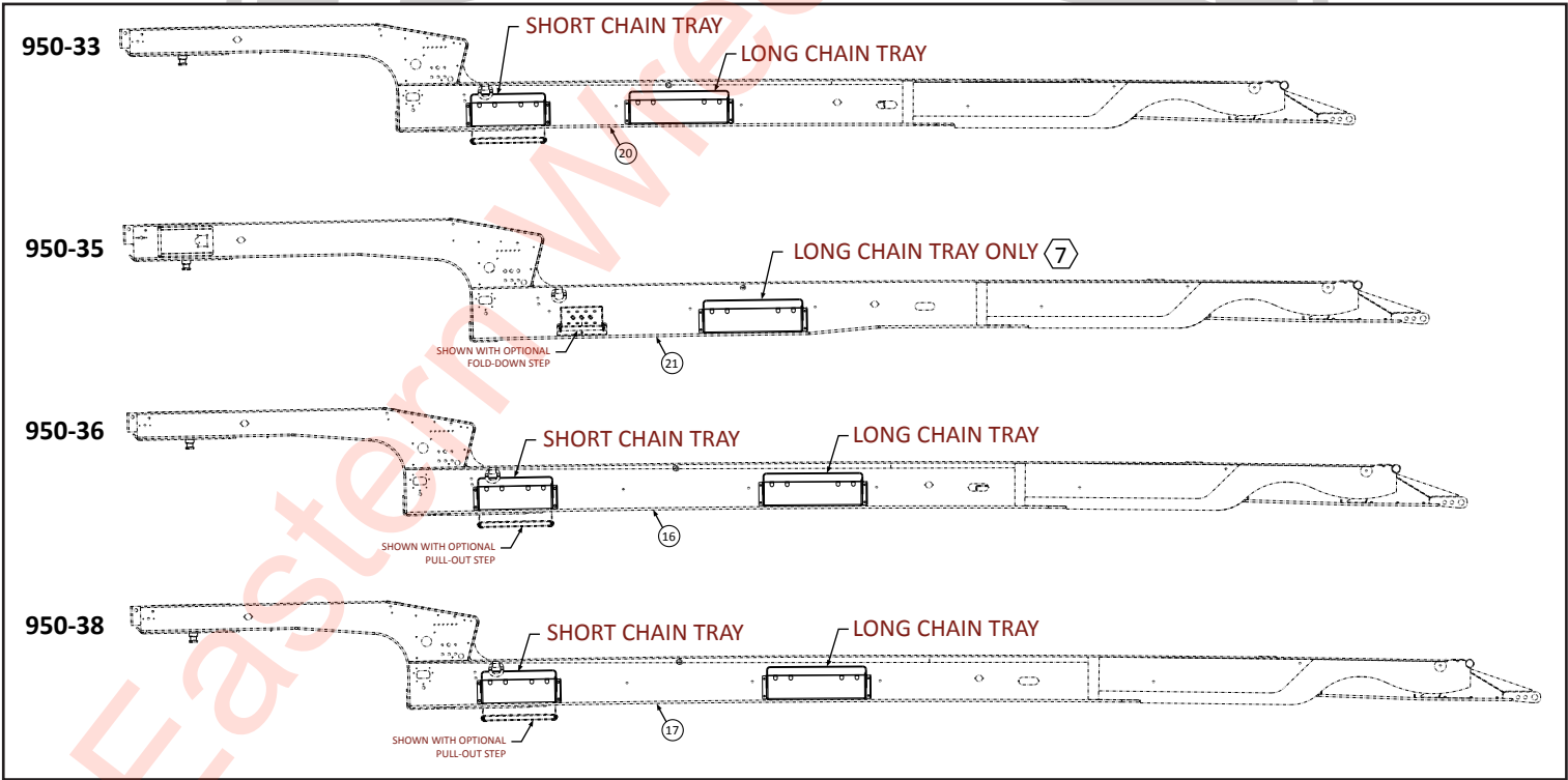
950 Series Web Mounted Chain Tray
